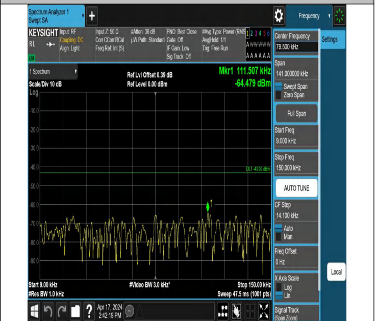
66-66-20MHz-15MHz-QPSK-QPSK-132348-132519-1RB#0-0RB #0-0.009~0.15MHz-PASS
