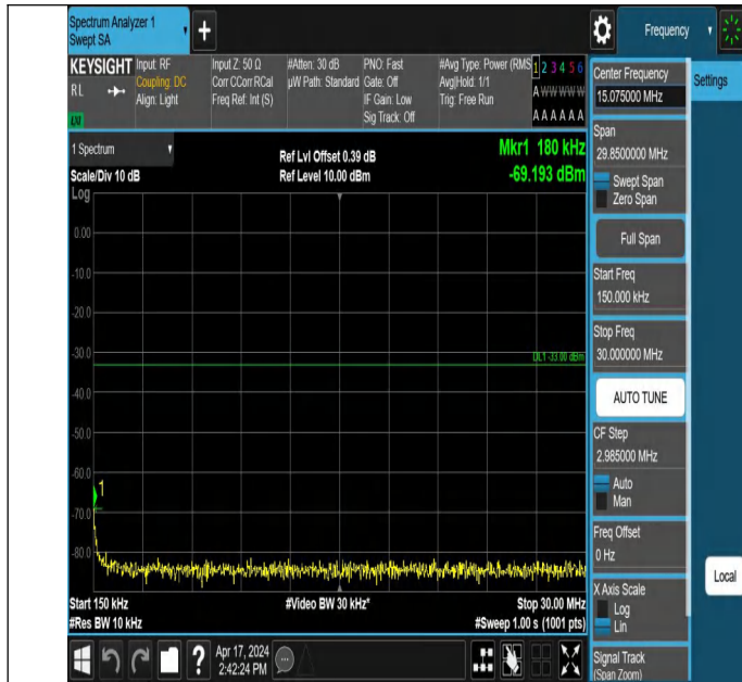
66-66-20MHz-15MHz-QPSK-QPSK-132348-132519-1RB#0-0RB# 0-0.15~30MHz-PASS
