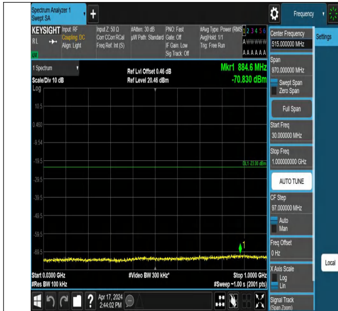
66-66-20MHz-15MHz-QPSK-QPSK-132423-132594-1RB#0-0RB# 0-30~1000MHz-PASS
