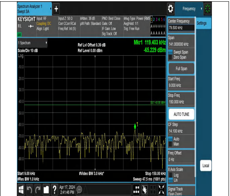
66-66-20MHz-15MHz-QPSK-QPSK-132072-132243-1RB#0-0RB #74-0.009~0.15MHz-PASS
