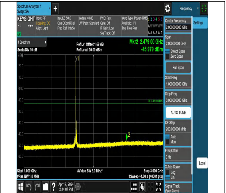
66-66-20MHz-15MHz-QPSK-QPSK-132423-132594-1RB#0-0RB# #0-1000~3000MHz-PASS
