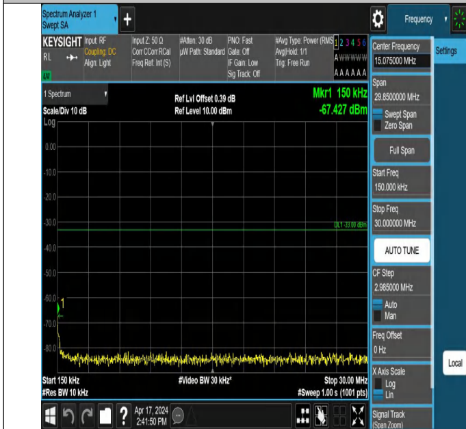
66-66-20MHz-15MHz-QPSK-QPSK-132072-132243-1RB#0-0RB# 74-0.15~30MHz-PASS
