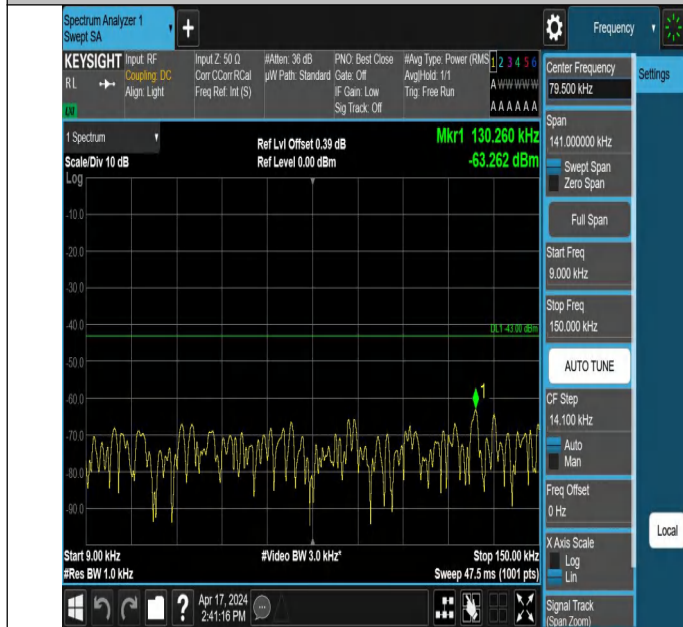
66-66-20MHz-15MHz-QPSK-QPSK-132072-132243-1RB#99-0RB #0-0.009~0.15MHz-PASS
