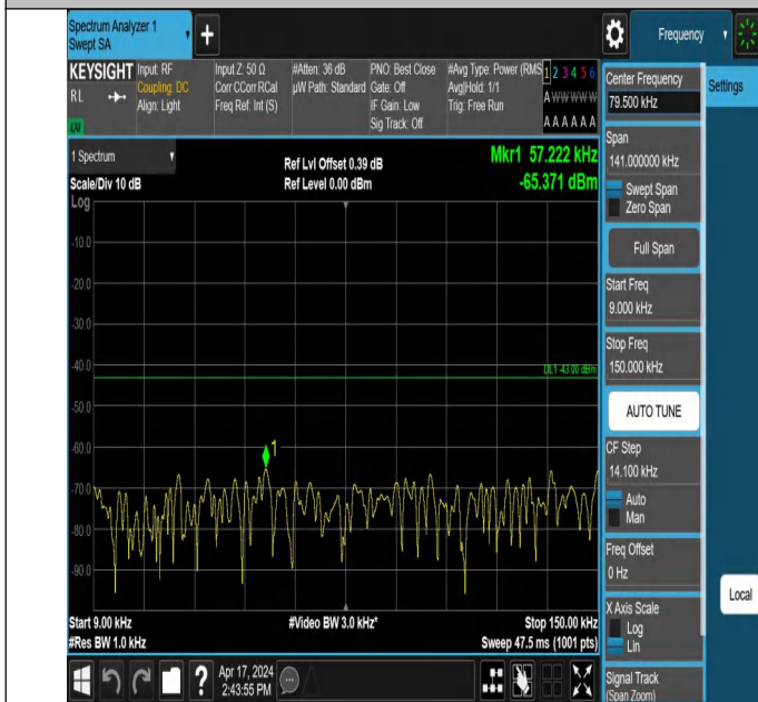
66-66-20MHz-15MHz-QPSK-QPSK-132423-132594-1RB#0-0RB# 0-0.009~0.15MHz-PASS
