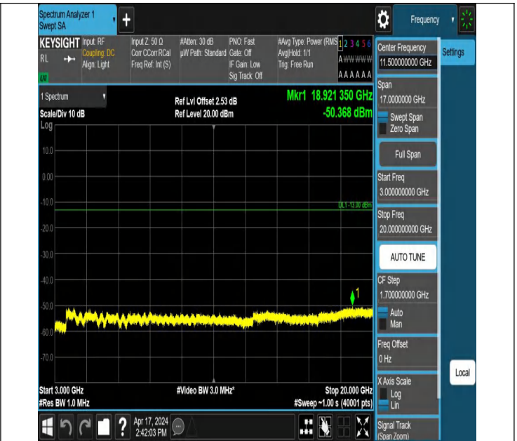
66-66-20MHz-15MHz-QPSK-QPSK-132072-132243-1RB#0-1RB #74-3000~20000MHz-PASS
