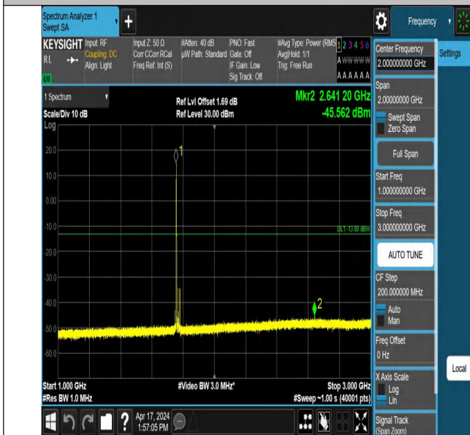
66-66-20MHz-5MHz-QPSK-QPSK-132522-132639-1RB#0-1RB#2 4-1000~3000MHz-PASS
