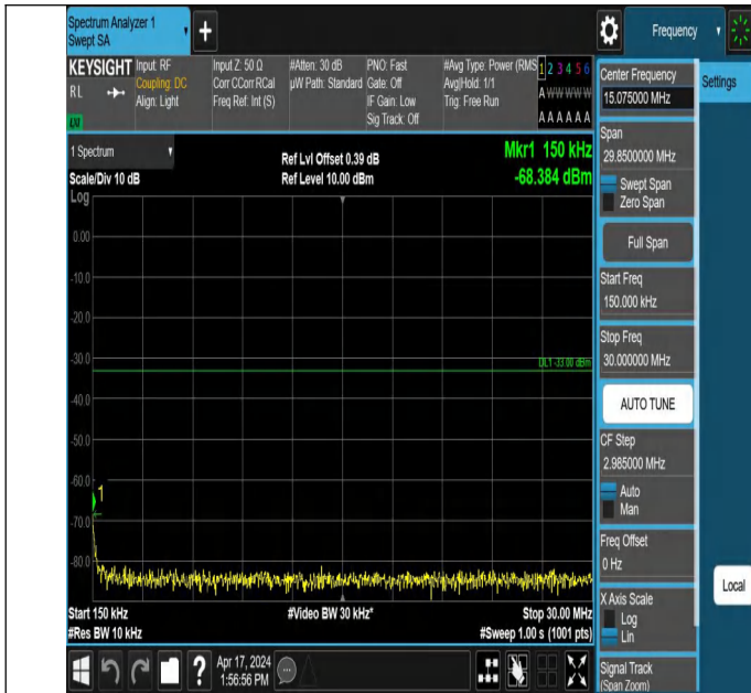
66-66-20MHz-5MHz-QPSK-QPSK-132522-132639-1RB#0-1RB#2 4-0.15~30MHz-PASS
