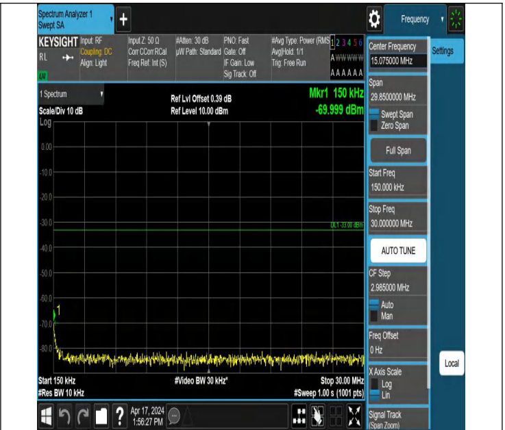
66-66-20MHz-5MHz-QPSK-QPSK-132522-132639-1RB#99-0RB #0-0.15~30MHz-PASS
