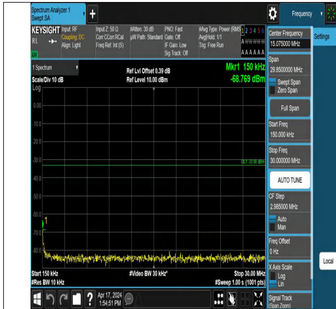
66-66-20MHz-5MHz-QPSK-QPSK-132397-132514-1RB#0-1RB#2 4-0.15~30MHz-PASS
