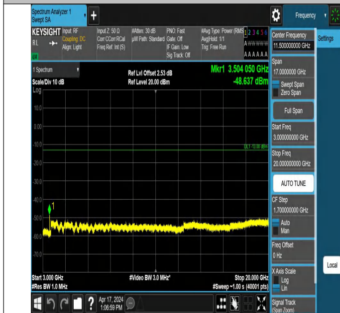
66-66-15MHz-20MHz-QPSK-QPSK-132325-132496-1RB#74-0RB #0-3000~20000MHz-PASS
