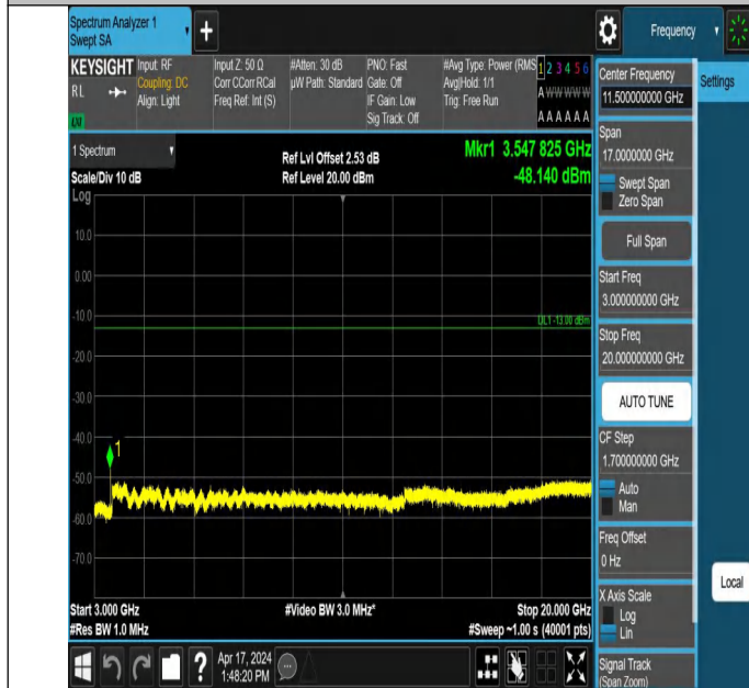
66-66-20MHz-5MHz-16QAM-16QAM-132522-132639-1RB#99-0R B#0-3000~20000MHz-PASS
