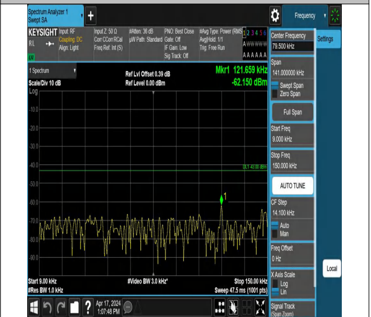
66-66-15MHz-20MHz-QPSK-QPSK-132401-132572-1RB#0-0RB #0-0.009~0.15MHz-PASS
