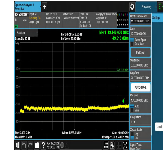
66-66-15MHz-10MHz-QPSK-QPSK-132047-132167-1RB#0-1RB# 49-3000~20000MHz-PASS
