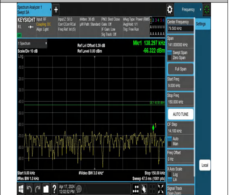
66-66-15MHz-10MHz-QPSK-QPSK-132047-132167-1RB#0-0RB #0-0.009~0.15MHz-PASS
