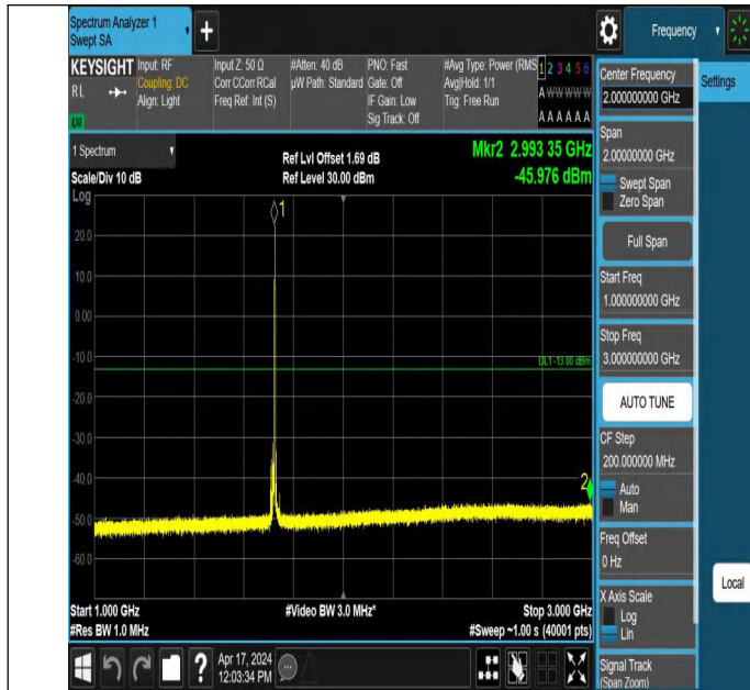
66-66-15MHz-10MHz-QPSK-QPSK-132047-132167-1RB#74-0RB #0-1000~3000MHz-PASS
