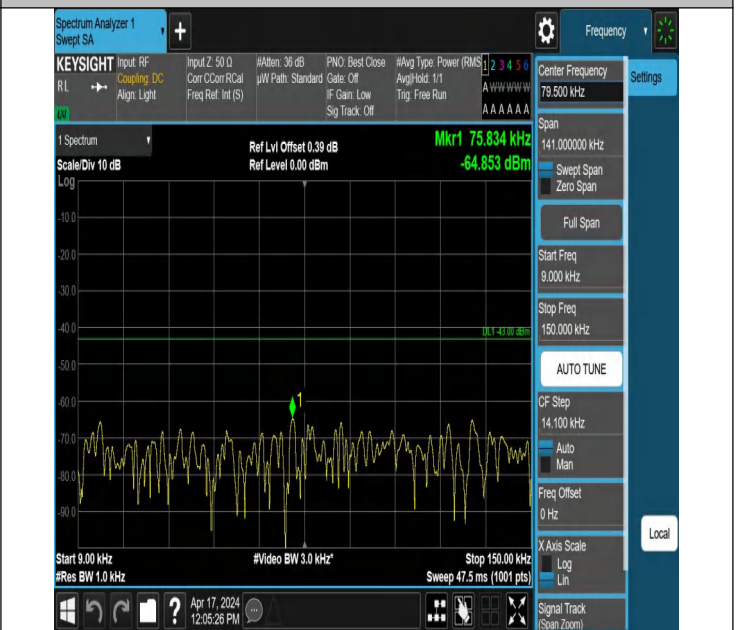
66-66-15MHz-10MHz-QPSK-QPSK-132373-132493-1RB#0-0-1RB #49-0.009~0.15MHz-PASS
