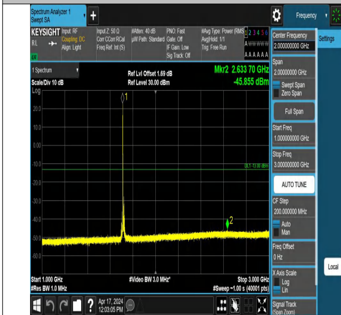
66-66-15MHz-10MHz-QPSK-QPSK-132047-132167-1RB#0-0RB# 0-1000~3000MHz-PASS
