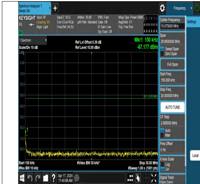
66-66-10MHz-20MHz-QPSK-QPSK-132328-132472-1RB#49-0RB #0-0.15~30MHz-PASS
