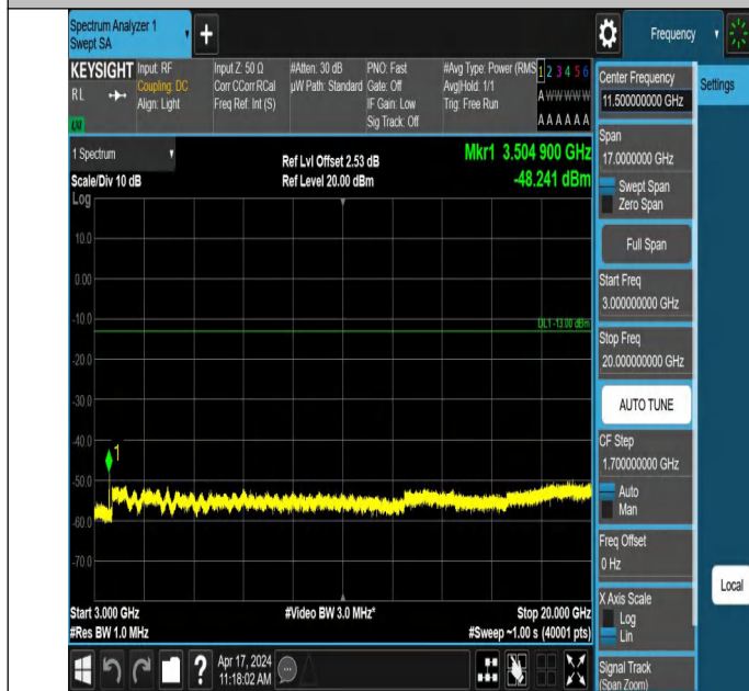
66-66-10MHz-15MHz-QPSK-QPSK-132351-132471-1RB#49-0RB #0-3000~20000MHz-PASS
