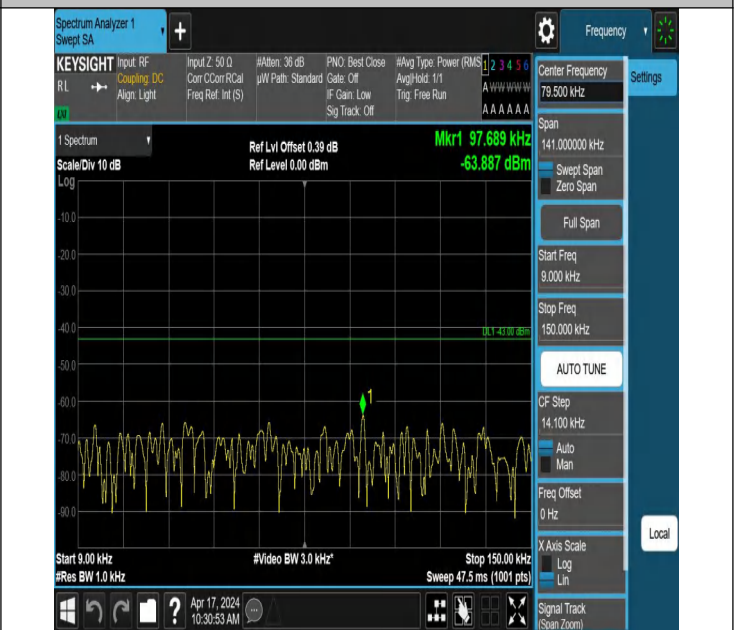
66-66-5MHz-20MHz-QPSK-QPSK-132428-132572-1RB#0-1RB#0 99-0.009~0.15MHz-PASS
