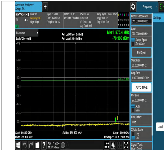
66-66-10MHz-15MHz-QPSK-QPSK-132351-132471-1RB#49-0RB #0-30~1000MHz-PASS
