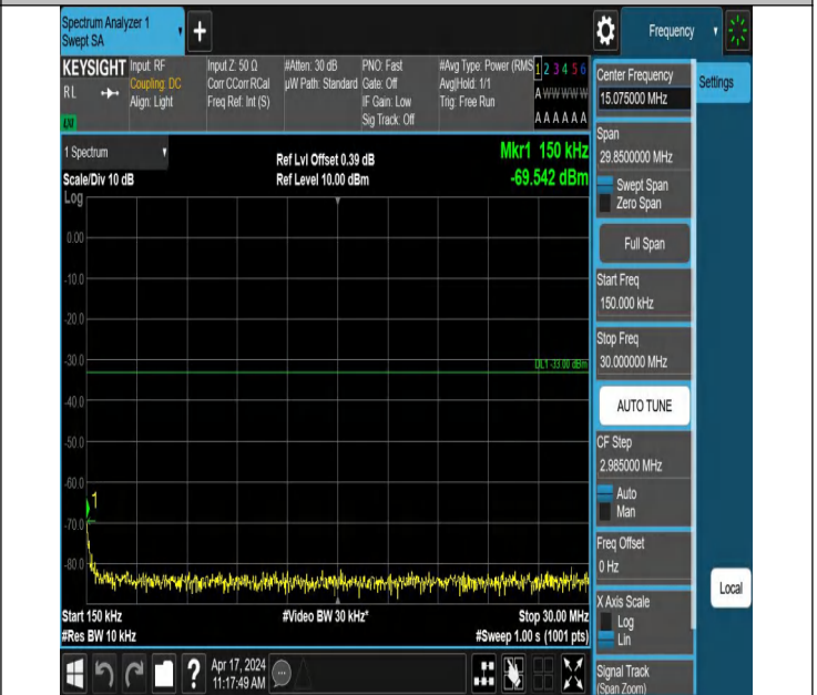
66-66-10MHz-15MHz-QPSK-QPSK-132351-132471-1RB#49-0R B#0-0.15~30MHz-PASS
