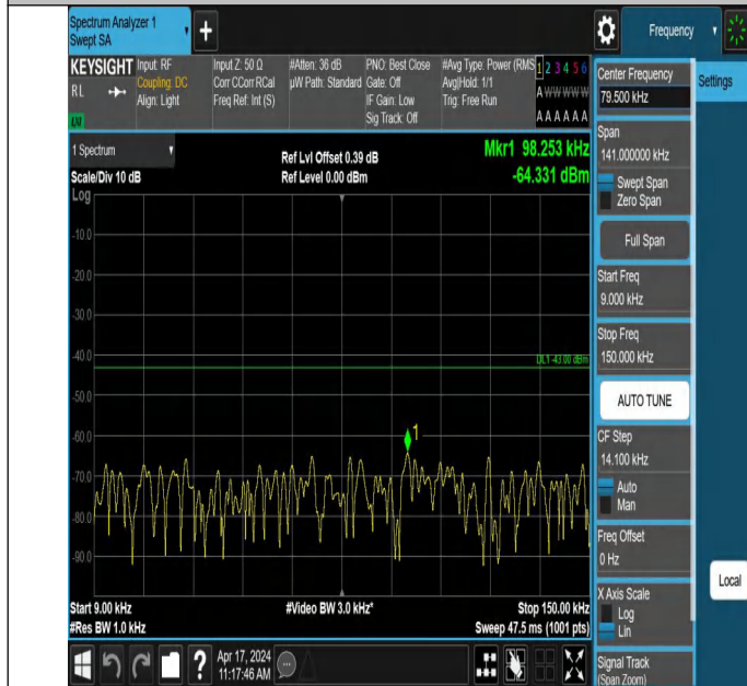
66-66-10MHz-15MHz-QPSK-QPSK-132351-132471-1RB#49-0RB #0-0.009~0.15MHz-PASS
