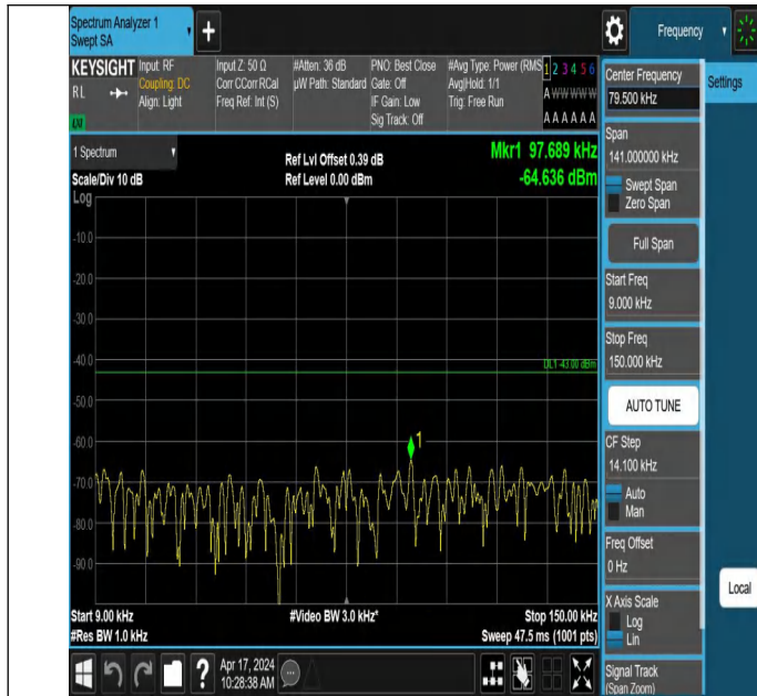
66-66-5MHz-20MHz-QPSK-QPSK-132328-132472-1RB#0-1RB#9 9-0.009~0.15MHz-PASS
