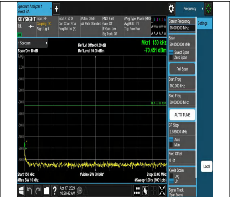
66-66-5MHz-20MHz-QPSK-QPSK-132328-132472-1RB#0-1RB# 99-0.15~30MHz-PASS
