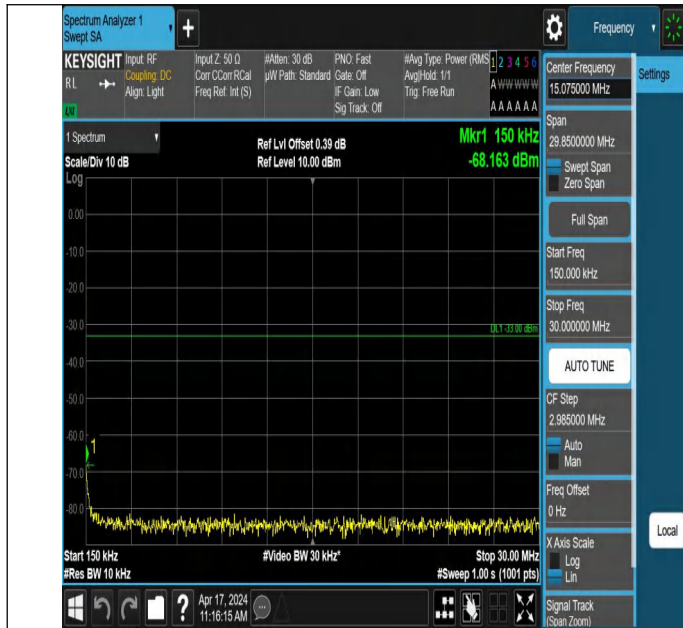
66-66-10MHz-15MHz-QPSK-QPSK-132025-132145-1RB#49-0RB #0-0.15~30MHz-PASS
