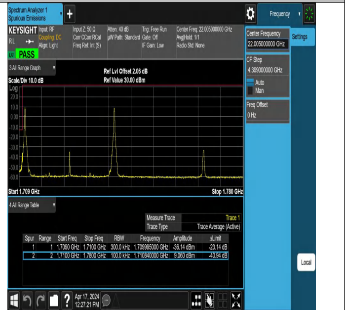
15MHz-15MHz_256QAM@256QAM-256QAM@256QAM_132047-132197_1RB#0@75RB#0-1RB#74@75RB#0
