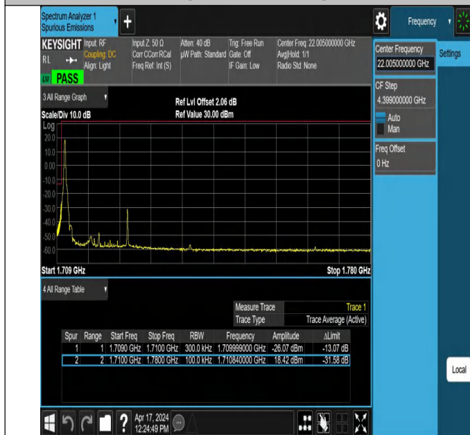
15MHz-15MHz_64QAM@64QAM-64QAM@64QAM_132047-132197_1RB#0@75RB#0-0RB#0@75RB#0
