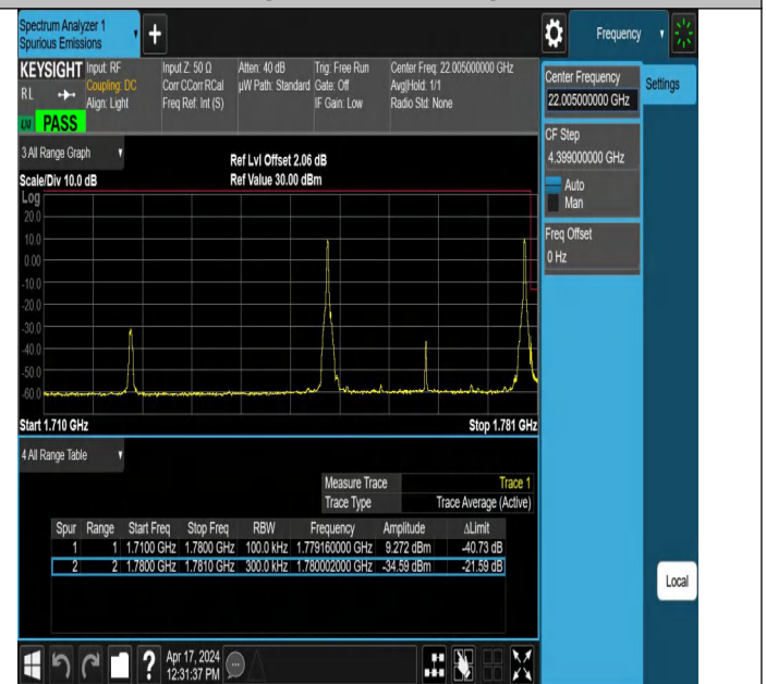
15MHz-15MHz_64QAM@64QAM-64QAM@64QAM_132447-1325 97_1RB#0@75RB#0-1RB#74@75RB#0
