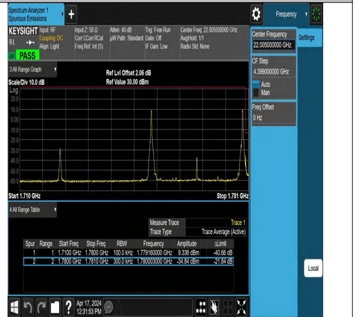
15MHz-15MHz_256QAM@256QAM-256QAM@256QAM_132447- 132597_1RB#0@75RB#0-1RB#74@75RB#0
