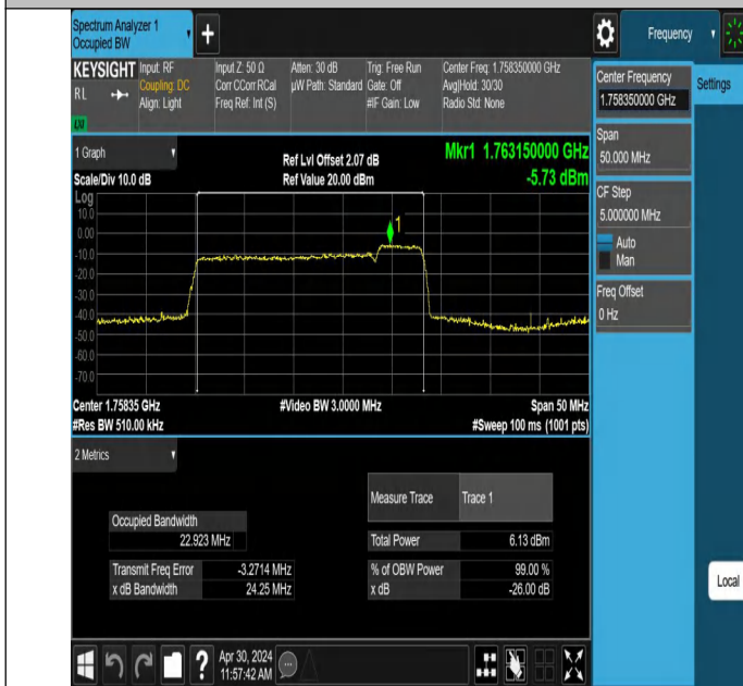
66-66-20MHz-5MHz-256QAM-256QAM-132397-132514-100RB#0- 25RB#0-PASS
