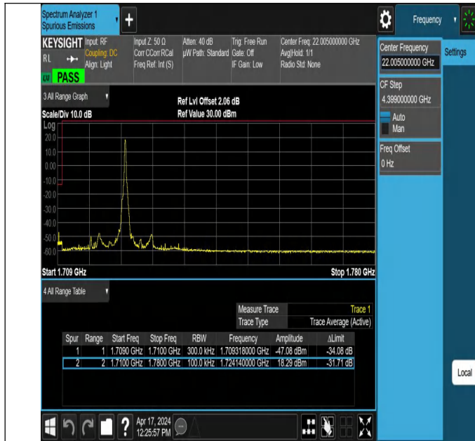
15MHz-15MHz_64QAM@64QAM-64QAM@64QAM_132047-13 2197_1RB#74@75RB#0-0RB#0@75RB#0
