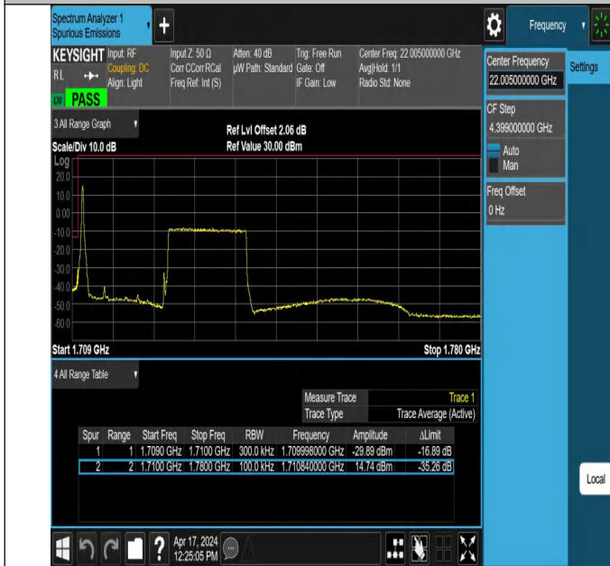
15MHz-15MHz_256QAM@256QAM-256QAM@256QAM_132047-132197_1RB#0@75RB#0-0RB#0@75RB#0
