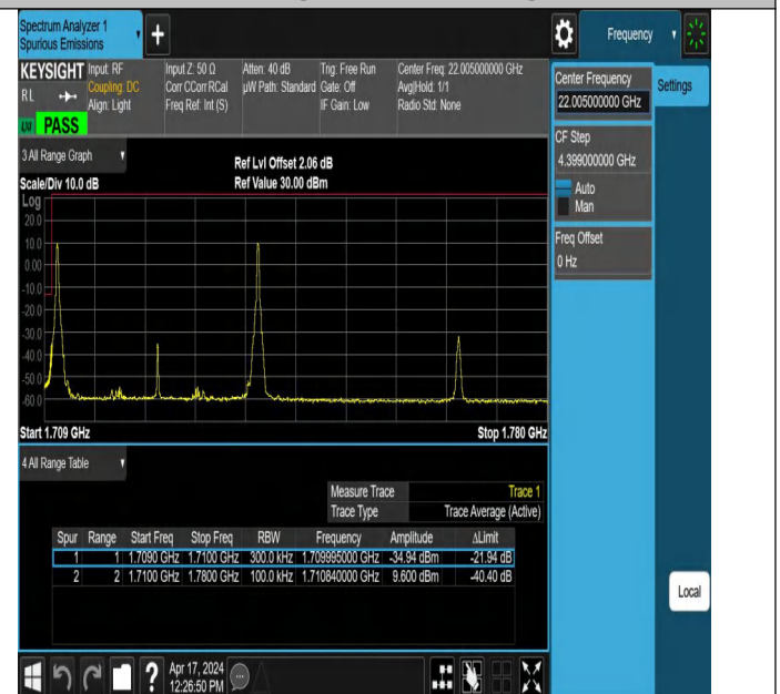
15MHz-15MHz_16QAM@16QAM-16QAM@16QAM_132047-1321 97_1RB#0@75RB#0-1RB#74@75RB#0
