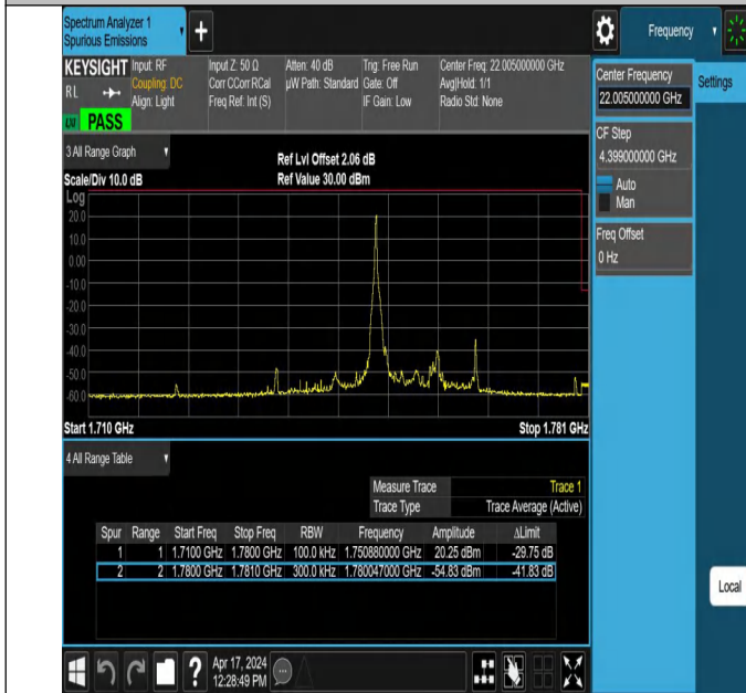
15MHz-15MHz_QPSK@QPSK-QPSK@QPSK_132447-132597_1RB#0@75RB#0-0RB#0@75RB#0
