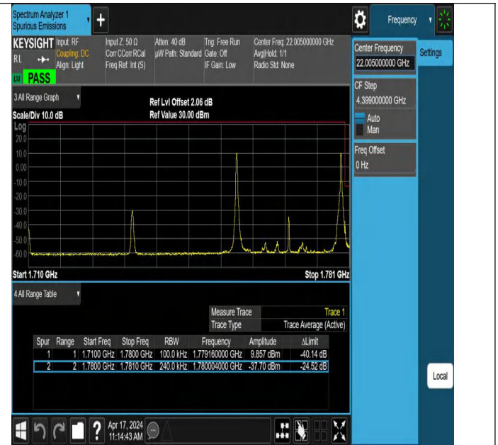
10MHz-15MHz_QPSK@QPSK-QPSK@QPSK_132477-132597_1RB#0@50RB#0-1RB#74@75RB#0
