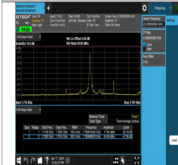
15MHz-15MHz_64QAM@64QAM-64QAM@64QAM_132447-13 2597_1RB#0@75RB#0-0RB#0@75RB#0
