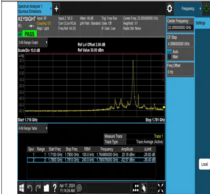
10MHz-15MHz_QPSK@QPSK-QPSK@QPSK_132477-132597_1RB#49@50RB#0-0RB#0@75RB#0
