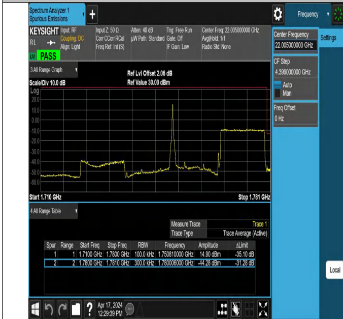
15MHz-15MHz_256QAM@256QAM-256QAM@256QAM_13244 7-132597_1RB#0@75RB#0-0RB#0@75RB#0
