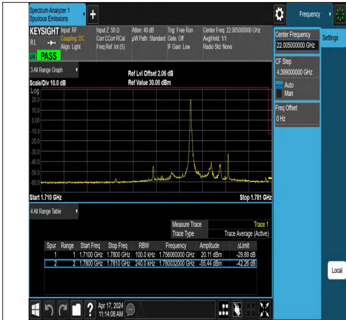
10MHz-15MHz_QPSK@QPSK-QPSK@QPSK_132477-132597_1RB#0@50RB#0-0RB#0@75RB#0
