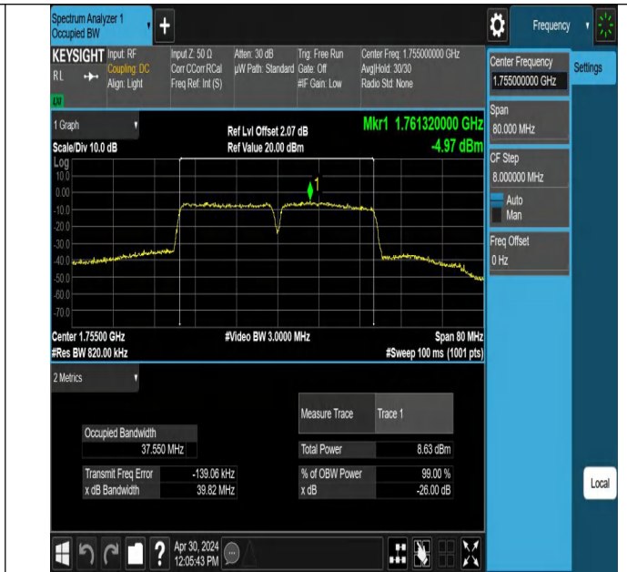
66-66-20MHz-20MHz-64QAM-64QAM-132323-132521-100RB#0-100RB#0-PASS
