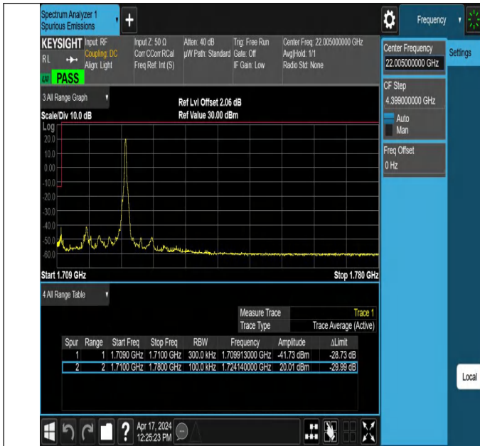
15MHz-15MHz_QPSK@QPSK-QPSK@QPSK_132047-132197_1RB#74@75RB#0-0RB#0@75RB#0
