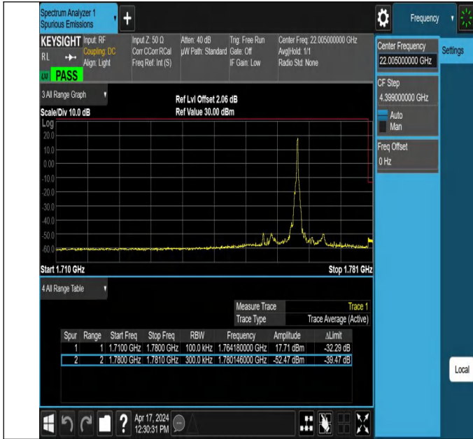
15MHz-15MHz_64QAM@64QAM-64QAM@64QAM_132447-132597_1RB#74@75RB#0-0RB#0@75RB#0
