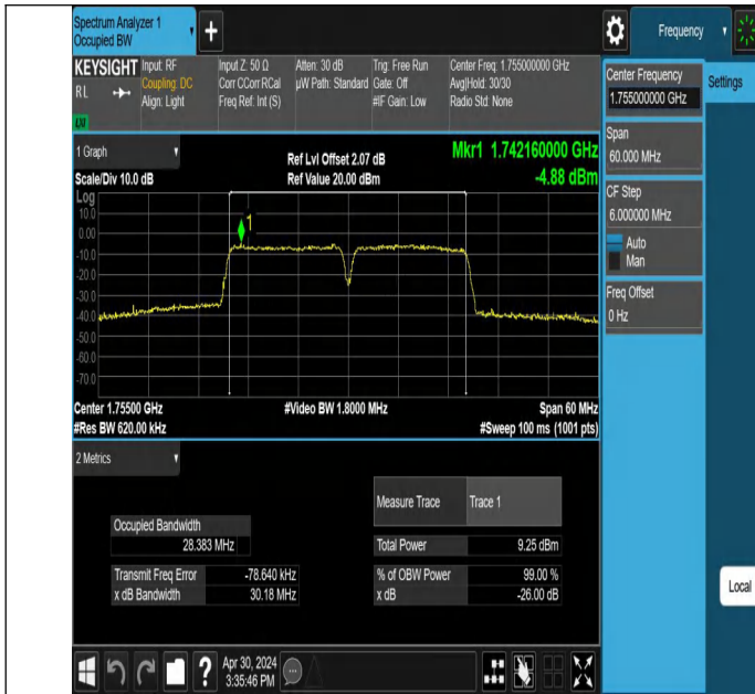
66-66-15MHz-15MHz-QPSK-QPSK-132347-132497-75RB#0-75R B#0-PASS
