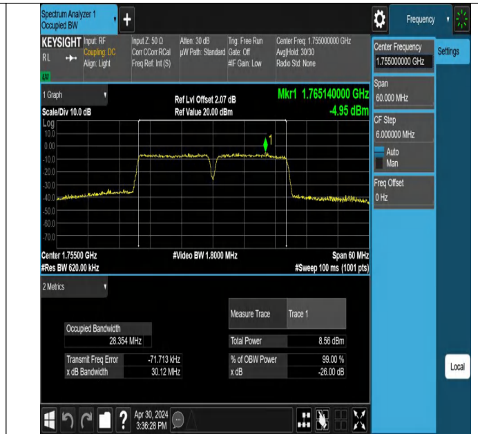
66-66-15MHz-15MHz-64QAM-64QAM-132347-132497-75RB#0-75R B#0-PASS
