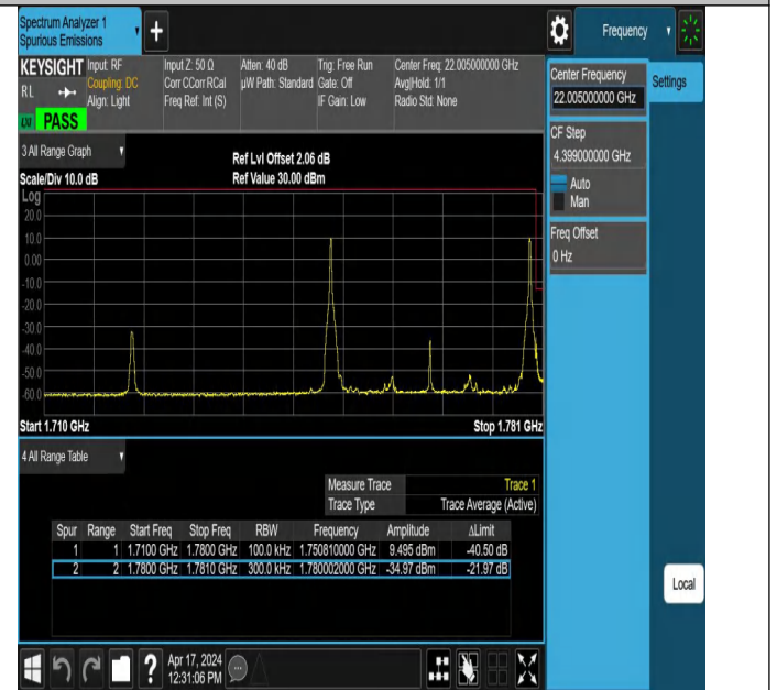
15MHz-15MHz_QPSK@QPSK-QPSK@QPSK_132447-132597_1RB#0@75RB#0-1RB#74@75RB#0
