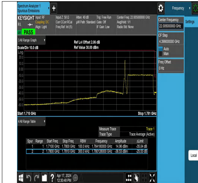
15MHz-15MHz_256QAM@256QAM-256QAM@256QAM_13244 7-132597_1RB#74@75RB#0-0RB#0@75RB#0
