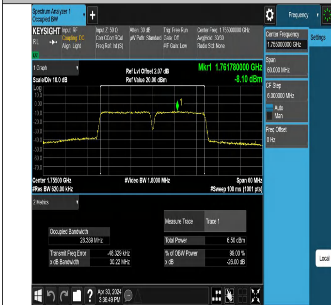
66-66-15MHz-15MHz-256QAM-256QAM-132347-132497-75RB#0-75R B#0-PASS
