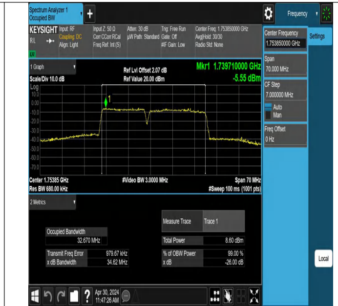
66-66-15MHz-20MHz-64QAM-64QAM-132325-132496-75RB#0-100RB#0-PASS
