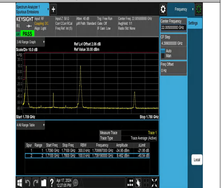
15MHz-15MHz_64QAM@64QAM-64QAM@64QAM_132047-132197_1RB#0@75RB#0-1RB#74@75RB#0
