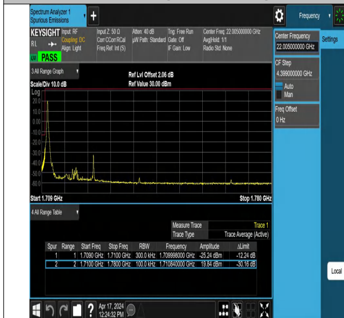
15MHz-15MHz_16QAM@16QAM-16QAM@16QAM_132047-13 2197_1RB#0@75RB#0-0RB#0@75RB#0
