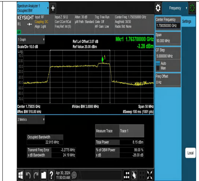
66-66-20MHz-5MHz-64QAM-64QAM-132397-132514-100RB#0- 25RB#0-PASS
