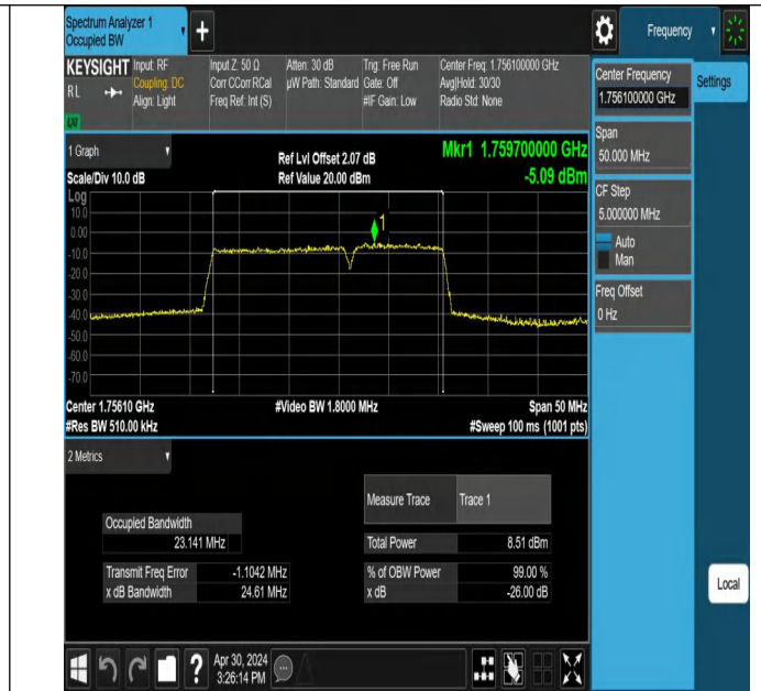
66-66-15MHz-10MHz-64QAM-64QAM-132373-132493-75RB#0-50RB#0-PASS
