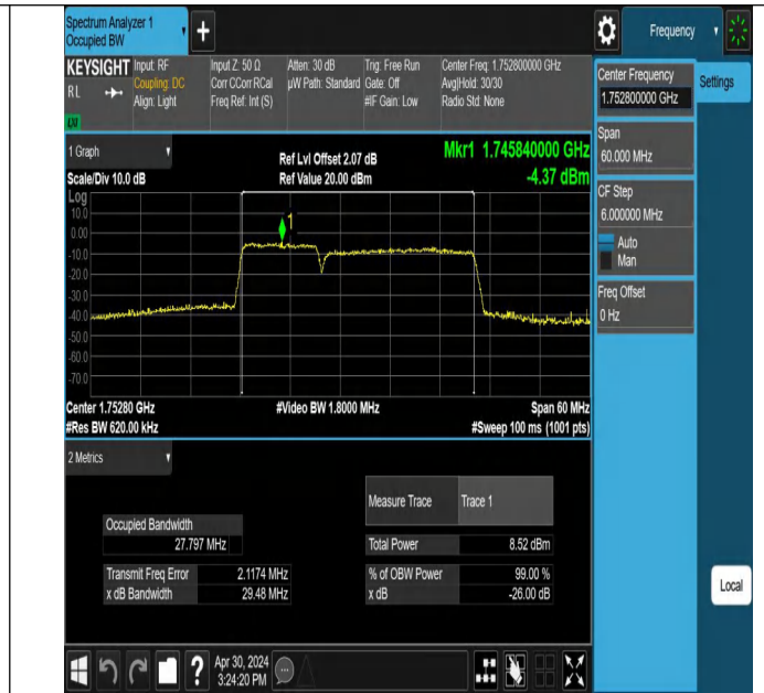
66-66-10MHz-20MHz-64QAM-64QAM-132328-132472-50RB#0-100RB#0-PASS
