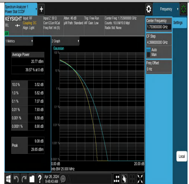
66-66-10MHz-15MHz-16QAM-16QAM-132351-132471-50RB#0- 75RB#0-PASS
