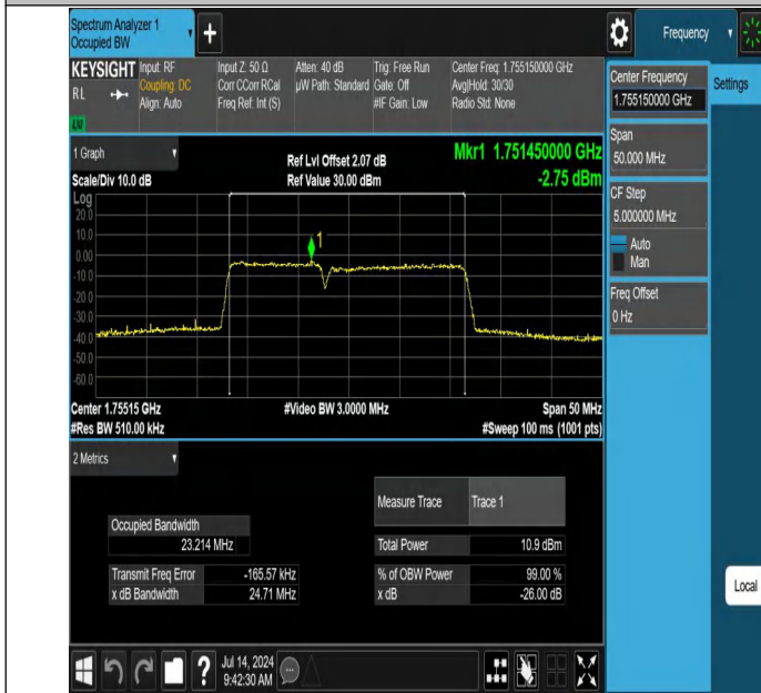
66-66-10MHz-15MHz-256QAM-256QAM-132351-132471-50RB#0-75RB#0-PASS
