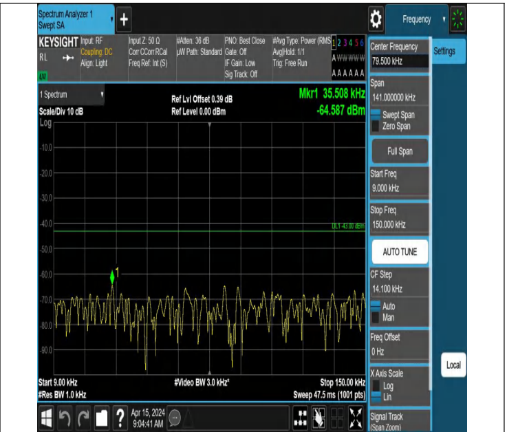
66-66-10MHz-10MHz-QPSK-QPSK-132022-132121-1RB#0-0RB #49-0.009~0.15MHz-PASS
