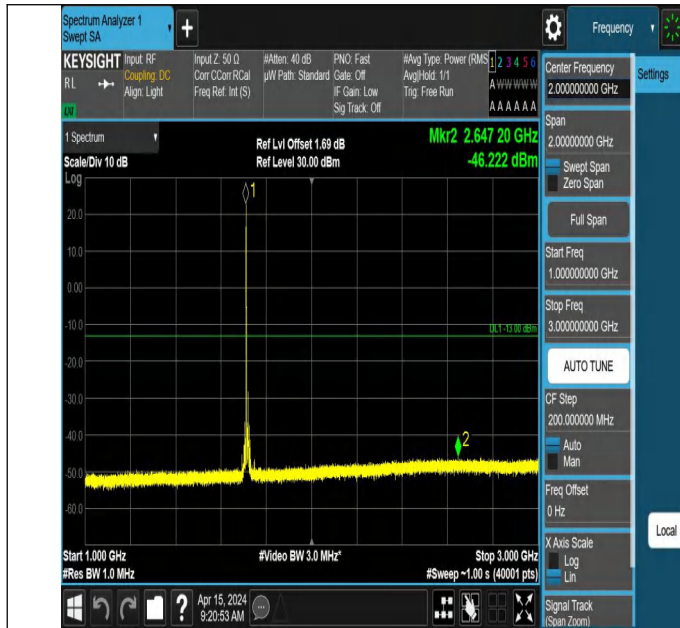
66-66-15MHz-5MHz-QPSK-QPSK-132047-132140-1RB#0-0RB# 0-1000~3000MHz-PASS
