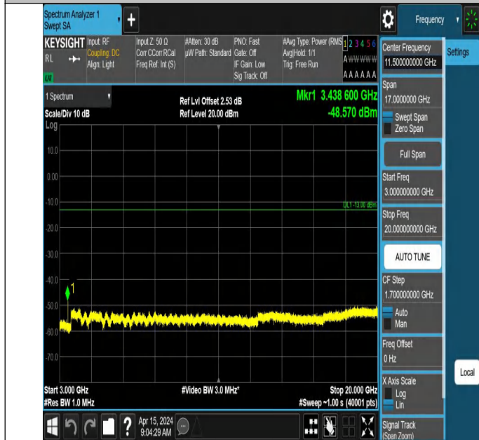
66-66-10MHz-10MHz-QPSK-QPSK-132022-132121-1RB#49-0R B#0-3000~20000MHz-PASS
