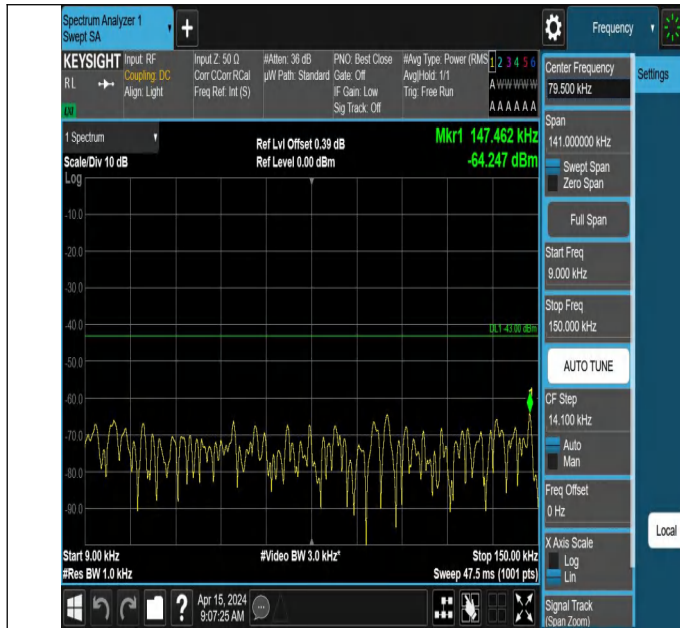
66-66-10MHz-10MHz-QPSK-QPSK-132523-132622-1RB#49-0R B#0-0.009~0.15MHz-PASS
