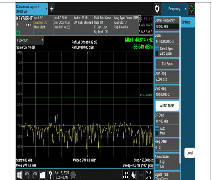
66-66-10MHz-5MHz-QPSK-QPSK-132022-132094-1RB#49-0RB #0-0.009~0.15MHz-PASS
