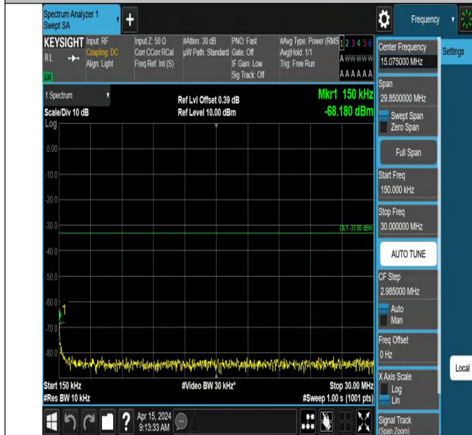
66-66-5MHz-15MHz-QPSK-QPSK-132353-132446-1RB#0-0RB# 0-0.15~30MHz-PASS
