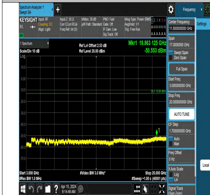
66-66-5MHz-15MHz-QPSK-QPSK-132353-132446-1RB#0-1RB# 74-3000~20000MHz-PASS
