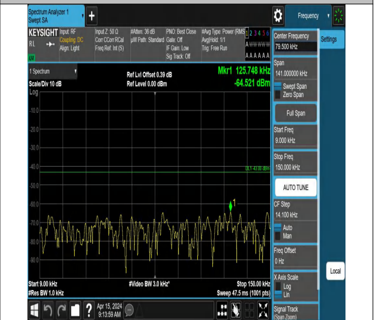
66-66-5MHz-15MHz-QPSK-QPSK-132353-132446-1RB#24-0RB #0-0.009~0.15MHz-PASS
