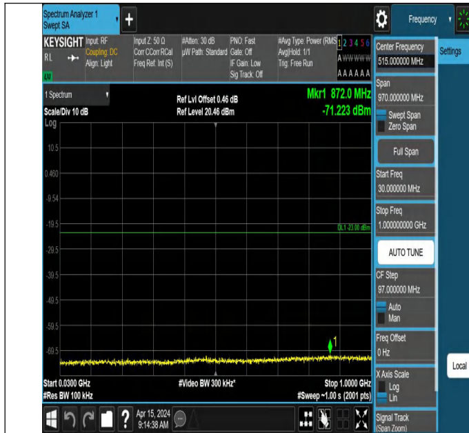
66-66-5MHz-15MHz-QPSK-QPSK-132353-132446-1RB#0-1RB# 74-30~1000MHz-PASS
