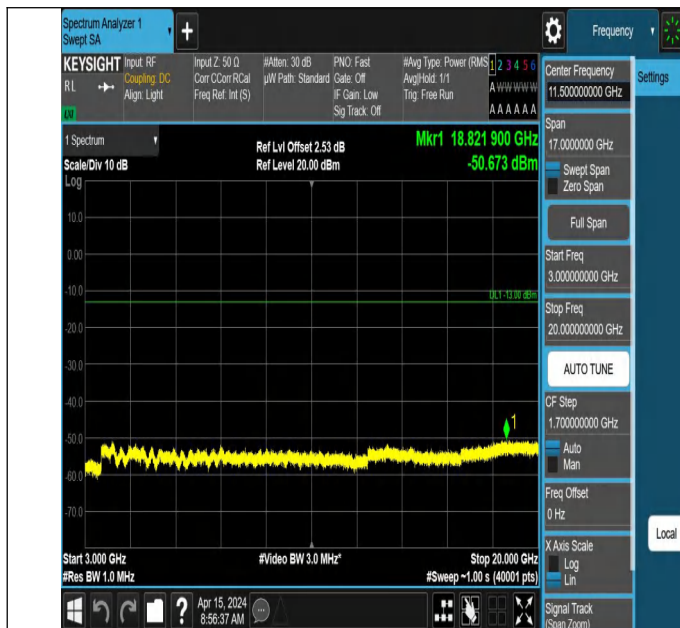
66-66-10MHz-5MHz-QPSK-QPSK-132022-132094-1RB#0-1RB# 24-3000~20000MHz-PASS
