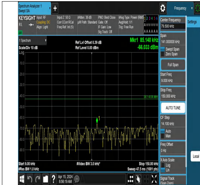
66-66-10MHz-5MHz-QPSK-QPSK-132022-132094-1RB#0-1RB# 24-0.009~0.15MHz-PASS
