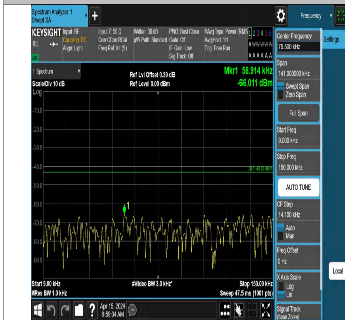
66-66-10MHz-5MHz-QPSK-QPSK-132572-132644-1RB#0-1RB# 24-0.009~0.15MHz-PASS
