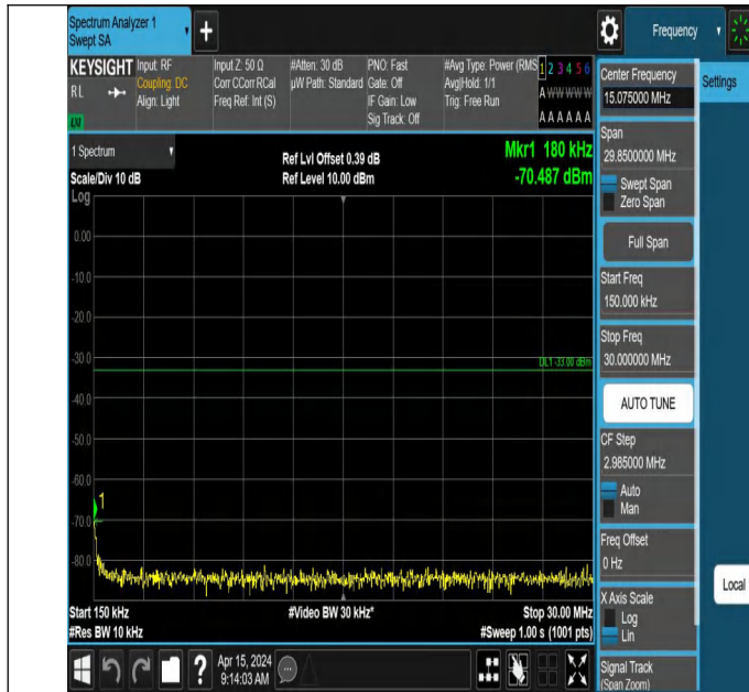
66-66-5MHz-15MHz-QPSK-QPSK-132353-132446-1RB#24-0RB #0-0.15~30MHz-PASS
