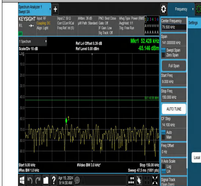
66-66-5MHz-15MHz-QPSK-QPSK-132353-132446-1RB#0-1RB# 74-0.009~0.15MHz-PASS
