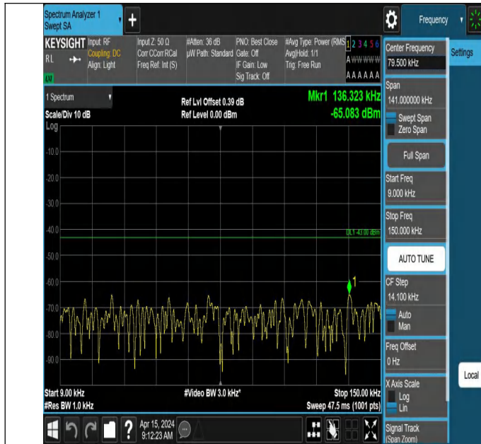
66-66-5MHz-15MHz-QPSK-QPSK-132002-132095-1RB#24-0RB #0-0.009~0.15MHz-PASS
