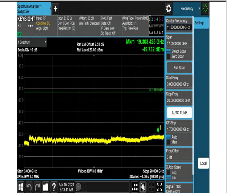
66-66-5MHz-15MHz-QPSK-QPSK-132002-132095-1RB#0-1RB# 74-3000~20000MHz-PASS
