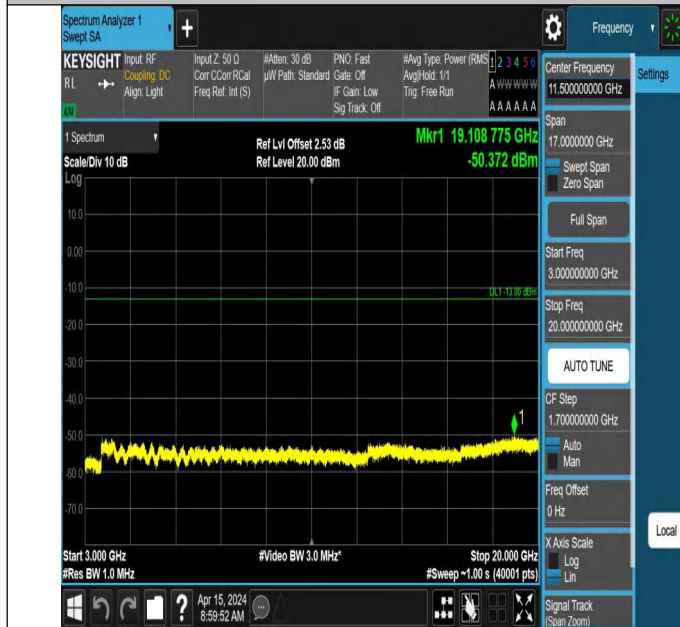
66-66-10MHz-5MHz-QPSK-QPSK-132572-132644-1RB#0-1RB# 24-3000~20000MHz-PASS
