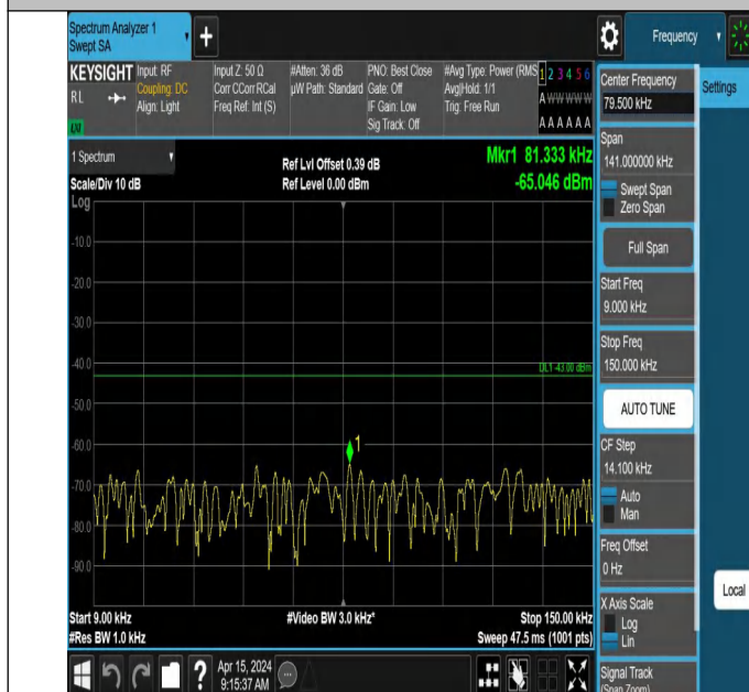
66-66-5MHz-15MHz-QPSK-QPSK-132504-132597-1RB#24-0RB #0-0.009~0.15MHz-PASS
