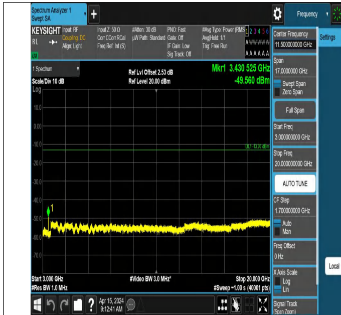
66-66-5MHz-15MHz-QPSK-QPSK-132002-132095-1RB#24-0RB #0-3000~20000MHz-PASS
