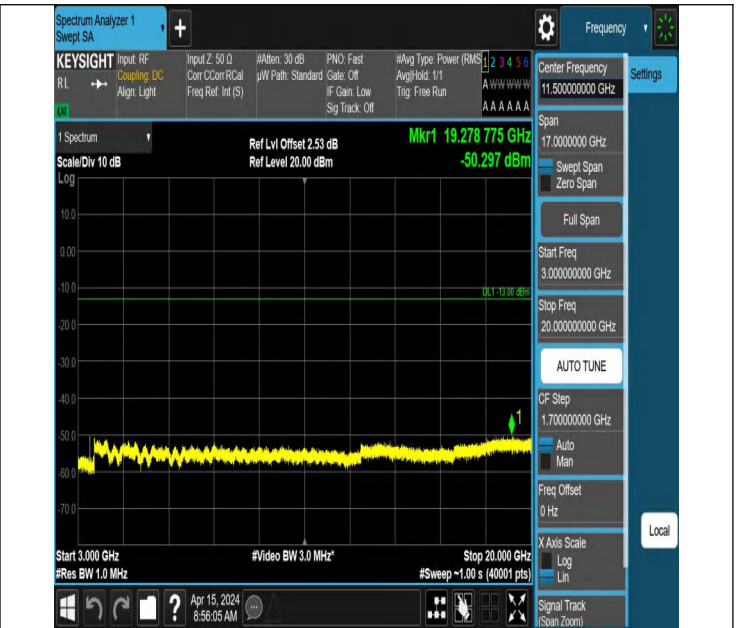
66-66-10MHz-5MHz-QPSK-QPSK-132022-132094-1RB#49-0RB #0-3000~20000MHz-PASS
