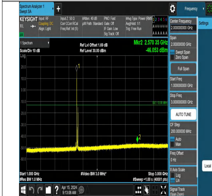
66-66-5MHz-15MHz-QPSK-QPSK-132002-132095-1RB#0-1RB# 74-1000~3000MHz-PASS
