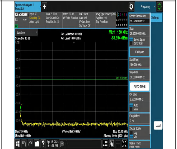
66-66-5MHz-15MHz-QPSK-QPSK-132002-132095-1RB#0-0RB# 0-0.15~30MHz-PASS
