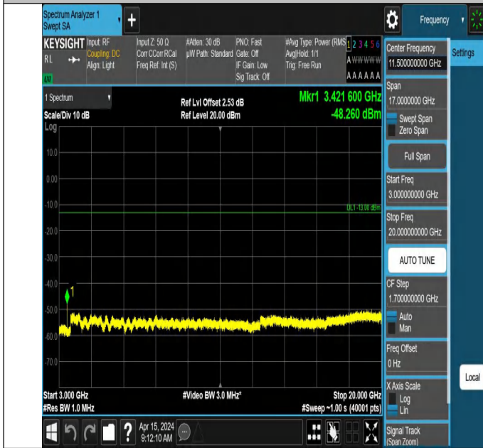
66-66-5MHz-15MHz-QPSK-QPSK-132002-132095-1RB#0-1RB#
