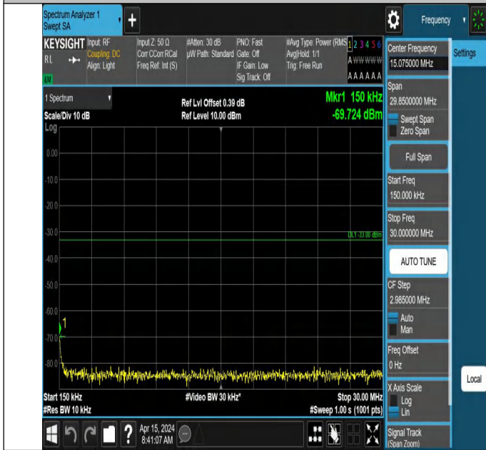
66-66-5MHz-5MHz-QPSK-QPSK-132398-132446-1RB#24-0RB#
