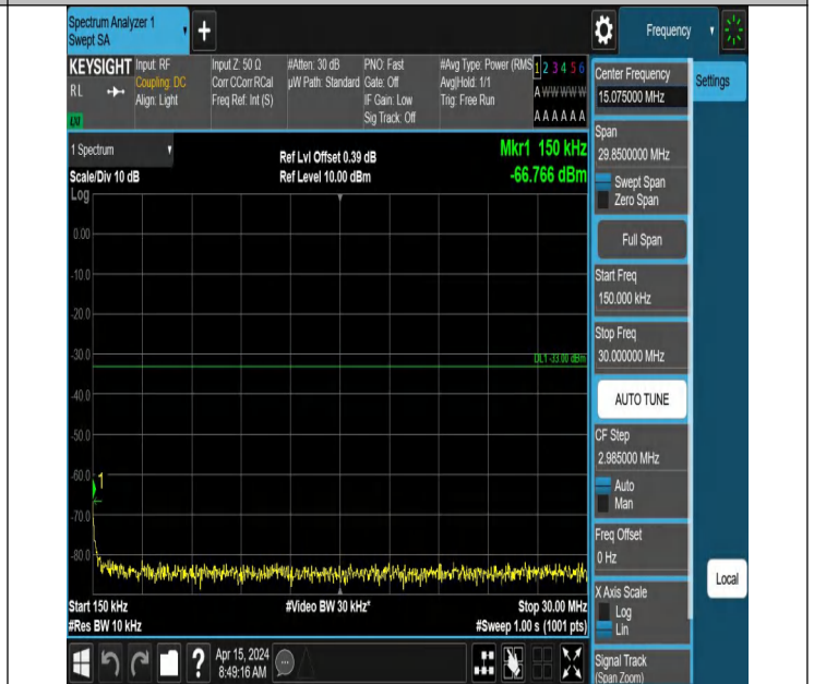
66-66-5MHz-10MHz-QPSK-QPSK-132375-132447-1RB#24-0RB #0-0.15~30MHz-PASS
