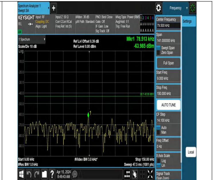
66-66-5MHz-10MHz-QPSK-QPSK-132375-132447-1RB#0-1RB# 49-0.009~0.15MHz-PASS
