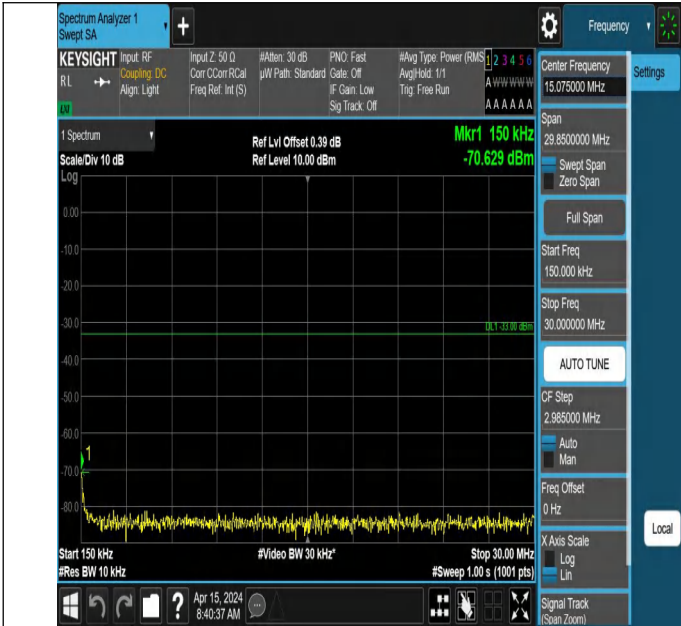
66-66-5MHz-5MHz-QPSK-QPSK-132398-132446-1RB#0-0RB#0-0.15~30MHz-PASS
