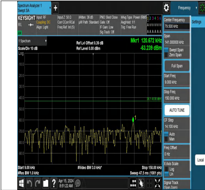
66-66-5MHz-10MHz-QPSK-QPSK-132550-132622-1RB#0-1RB# 49-0.009~0.15MHz-PASS
