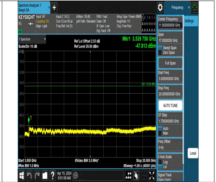
66-66-5MHz-10MHz-QPSK-QPSK-132550-132622-1RB#24-0RB #0-3000~20000MHz-PASS
