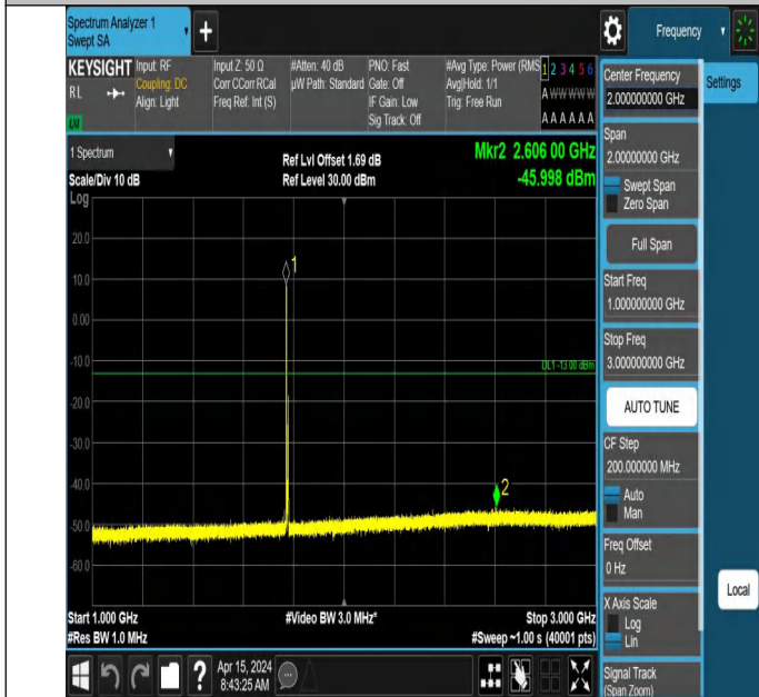
66-66-5MHz-5MHz-QPSK-QPSK-132599-132647-1RB#0-1RB#1 5-1000~3000MHz-PASS
