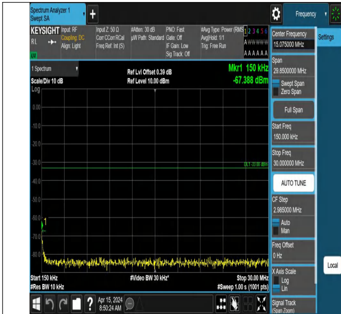
66-66-5MHz-10MHz-QPSK-QPSK-132550-132622-1RB#0-0RB# 0-0.15~30MHz-PASS
