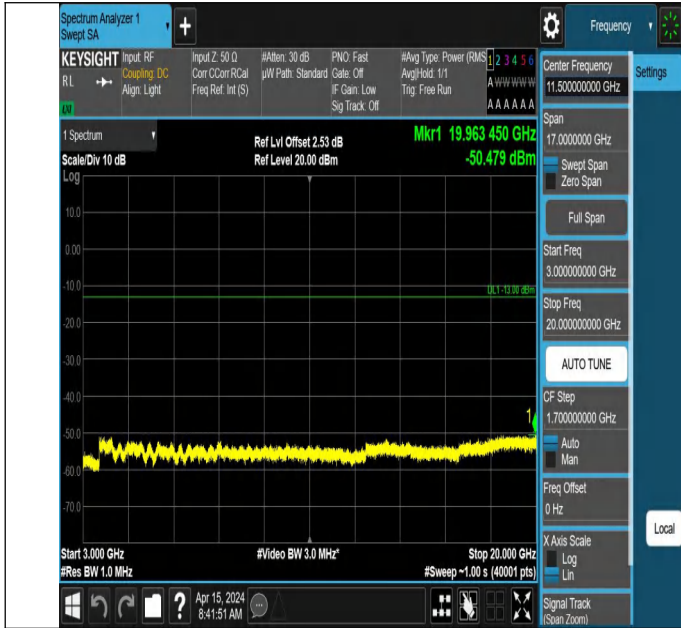
66-66-5MHz-5MHz-QPSK-QPSK-132398-132446-1RB#0-1RB#1
