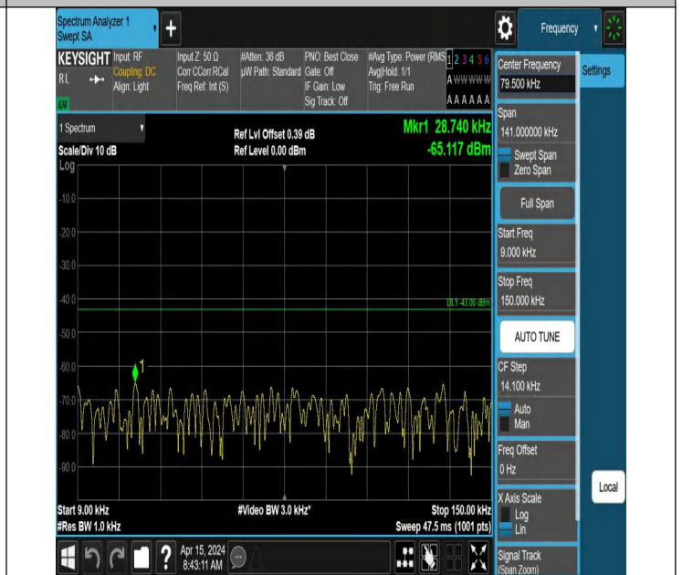
66-66-5MHz-5MHz-QPSK-QPSK-132599-132647-1RB#0-1RB#1 5-0.009~0.15MHz-PASS
