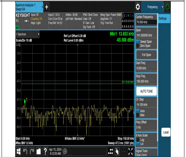
66-66-5MHz-15MHz-QPSK-QPSK-132002-132095-1RB#0-1RB#
