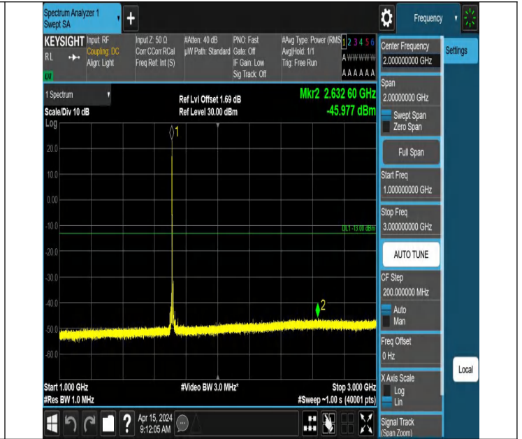
66-66-5MHz-15MHz-QPSK-QPSK-132002-132095-1RB#0-0RB#
