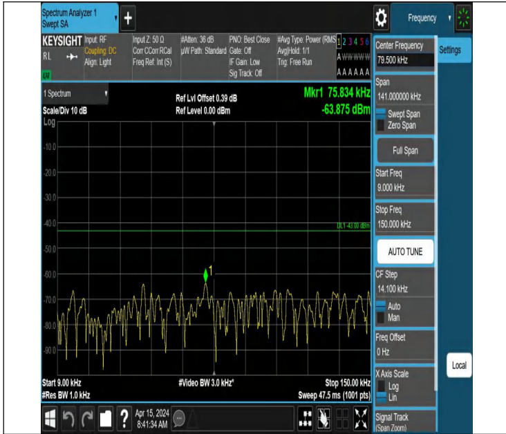
66-66-5MHz-5MHz-QPSK-QPSK-132398-132446-1RB#0-1RB#1
