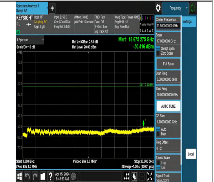
66-66-5MHz-5MHz-QPSK-QPSK-132599-132647-1RB#0-1RB#1 5-3000~20000MHz-PASS
