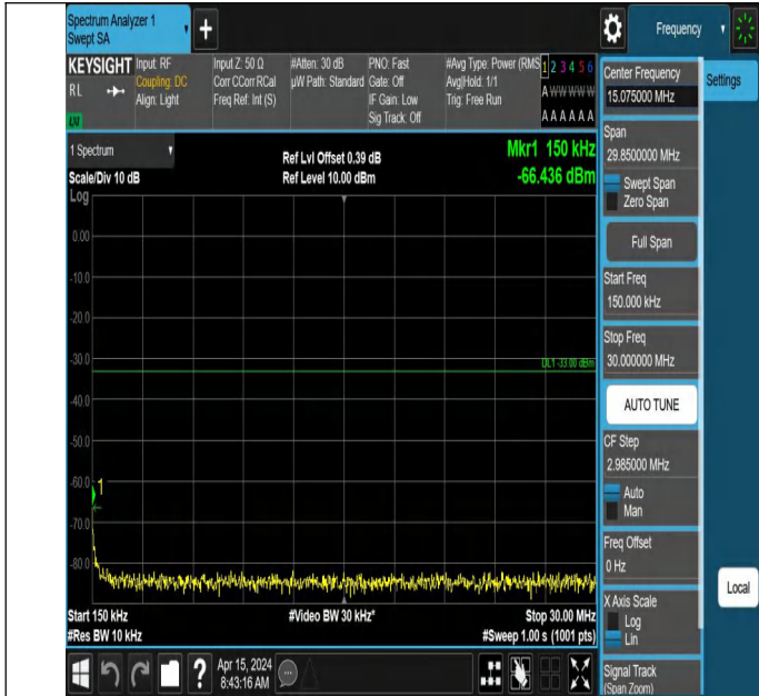
66-66-5MHz-5MHz-QPSK-QPSK-132599-132647-1RB#0-1RB#1 5-0.15~30MHz-PASS
