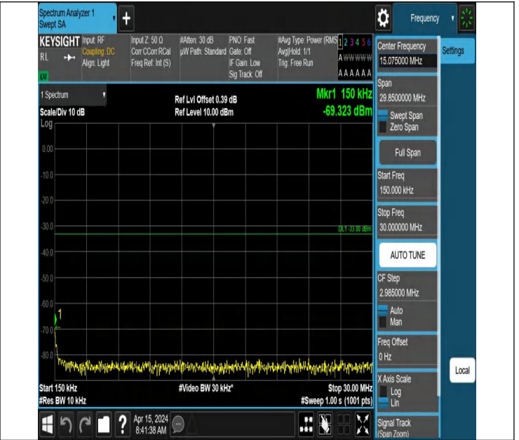
66-66-5MHz-5MHz-QPSK-QPSK-132398-132446-1RB#0-1RB#1
