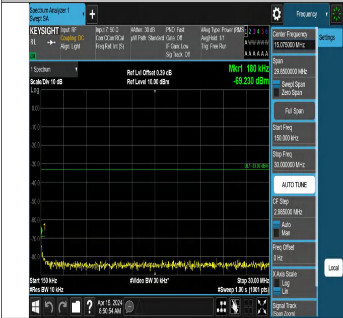
66-66-5MHz-10MHz-QPSK-QPSK-132550-132622-1RB#24-0RB #0-0.15~30MHz-PASS
