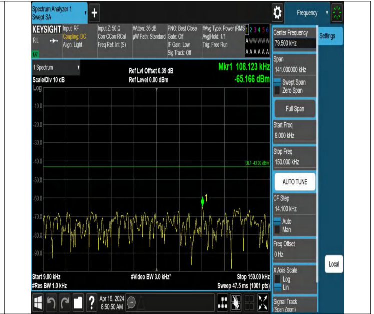
66-66-5MHz-10MHz-QPSK-QPSK-132550-132622-1RB#24-0RB #0-0.009~0.15MHz-PASS
