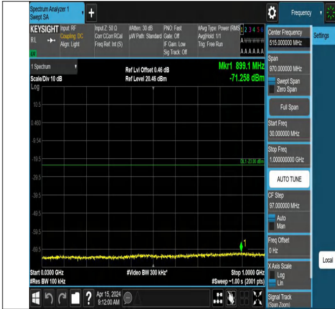
66-66-5MHz-15MHz-QPSK-QPSK-132002-132095-1RB#0-0RB#
