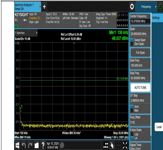
66-66-5MHz-10MHz-QPSK-QPSK-132375-132447-1RB#0-1RB# 49-0.15~30MHz-PASS
