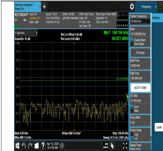
66-66-5MHz-15MHz-QPSK-QPSK-132002-132095-1RB#0-0RB# 0-0.009~0.15MHz-PASS
