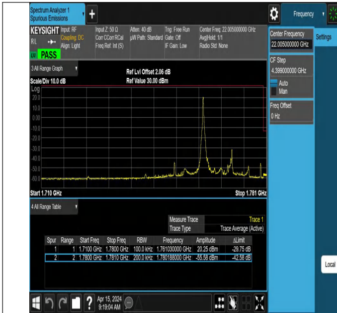
15MHz-5MHz_QPSK@QPSK-QPSK@QPSK_132549-132642_1 RB#0@75RB#0-0RB#0@25RB#0
