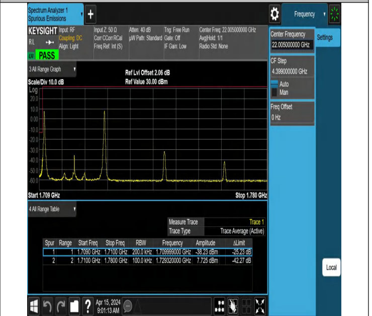
10MHz-10MHz_QPSK@QPSK-QPSK@QPSK_132022-132121_1 1RB#0@50RB#0-1RB#49@50RB#0
