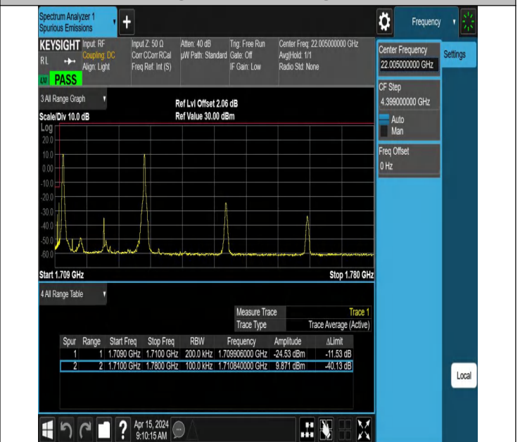
5MHz-15MHz_QPSK@QPSK-QPSK@QPSK_132002-132095_1 RB#0@25RB#0-1RB#74@75RB#0
