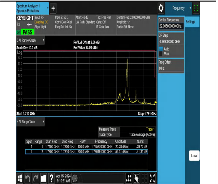
5MHz-15MHz_QPSK@QPSK-QPSK@QPSK_132504-132597_1 RB#24@25RB#0-0RB#0@75RB#0
