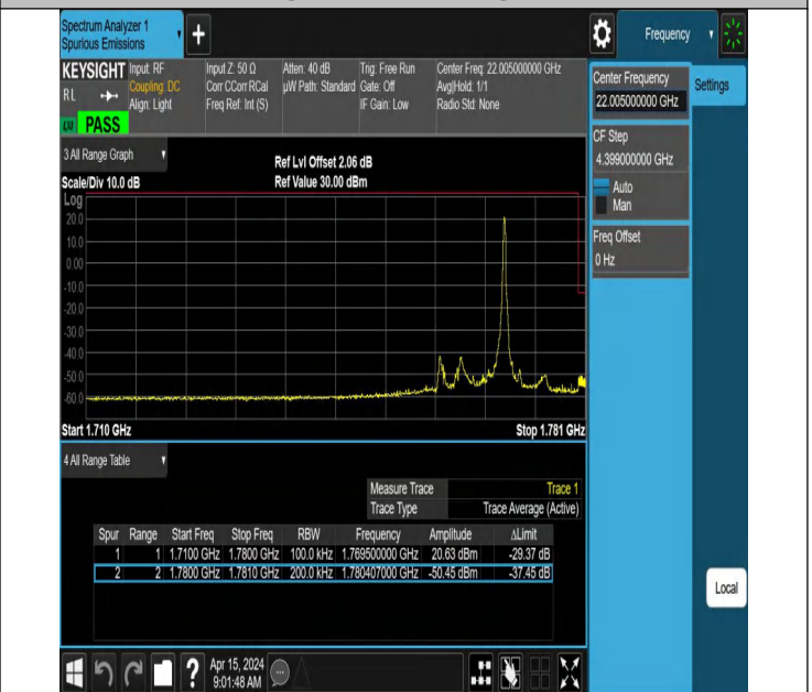
10MHz-10MHz_QPSK@QPSK-QPSK@QPSK_ 132523-132622_ 1RB#49@50RB#0-0RB#0@50RB#0
