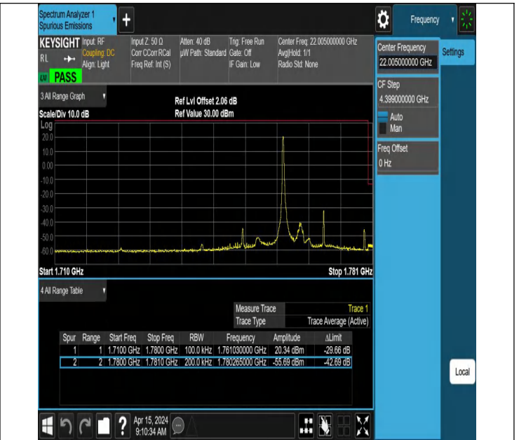
5MHz-15MHz_QPSK@QPSK-QPSK@QPSK_132504-132597_1 RB#0@25RB#0-0RB#0@75RB#0
