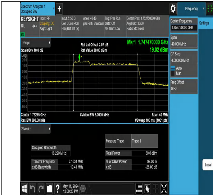
66-66-5MHz-15MHz-QPSK-QPSK-132353-132446-25RB#0-75RB #0-PASS
