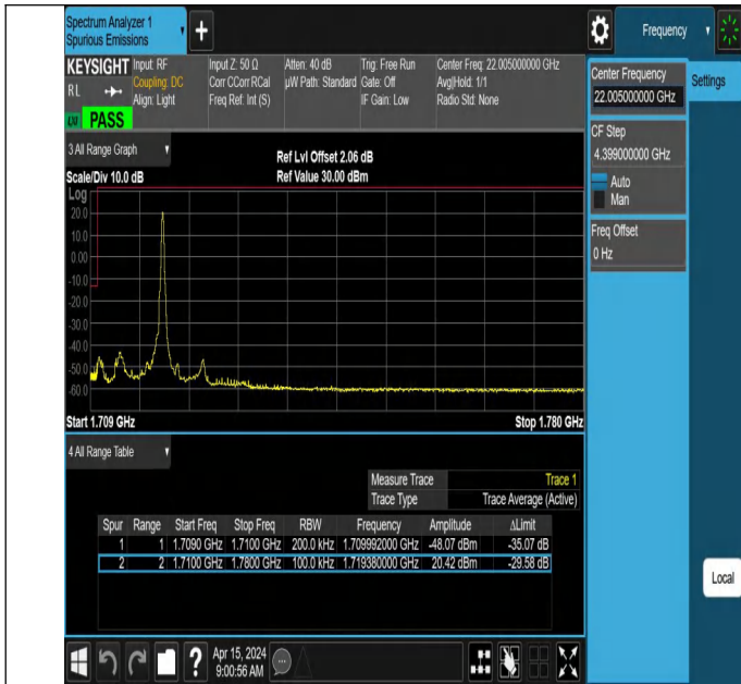
10MHz-10MHz_QPSK@QPSK-QPSK@QPSK_ 132022-132121_ 1RB#49@50RB#0-0RB#0@50RB#0
