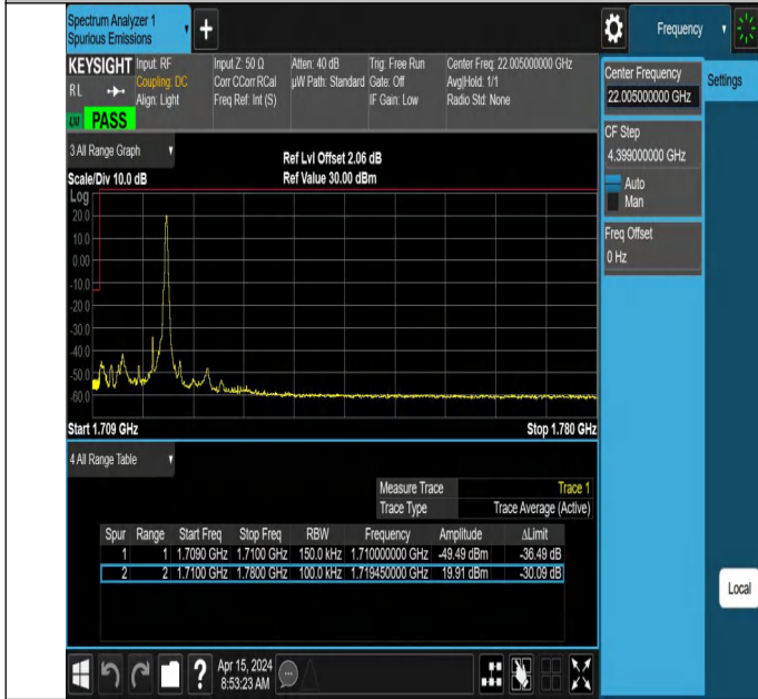
10MHz-5MHz_QPSK@QPSK-QPSK@QPSK_132022-132094_1 RB#49@50RB#0-0RB#0@25RB#0
