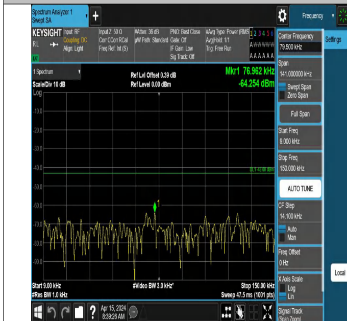
66-66-5MHz-5MHz-QPSK-QPSK-131997-132045-1RB#24-0RB# 0-0.009~0.15MHz-PASS
