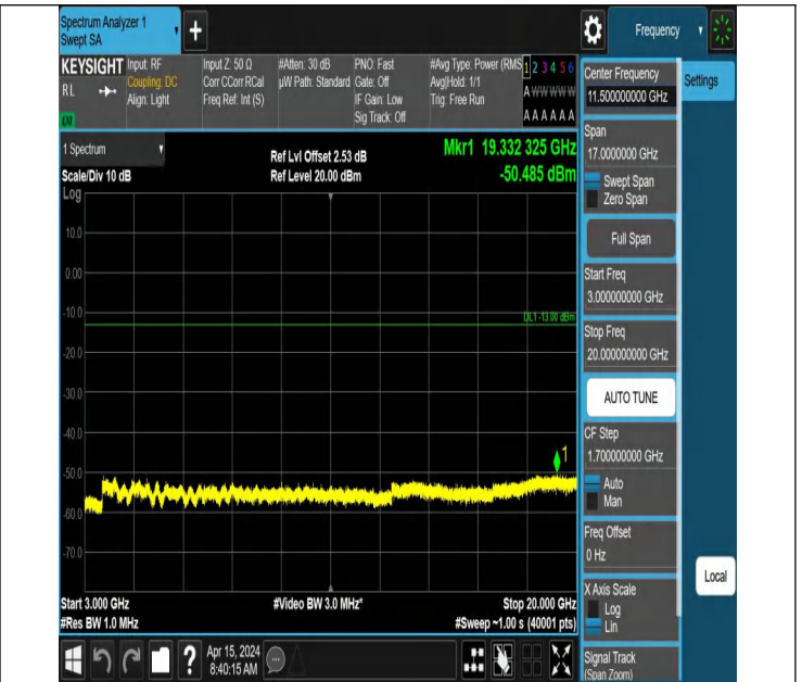
66-66-5MHz-5MHz-QPSK-QPSK-131997-132045-1RB#0-1RB#1 5-3000~20000MHz-PASS
