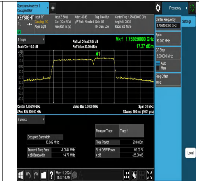
66-66-10MHz-5MHz-64QAM-64QAM-132397-132469-50RB#0-2 5RB#0-PASS
