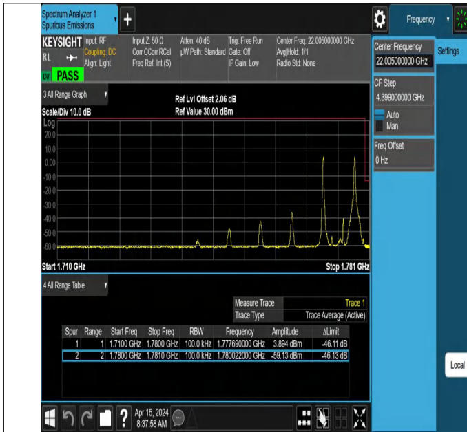
5MHz-5MHz_QPSK@QPSK-QPSK@QPSK_132599-132647_1R B#0@25RB#0-1RB#15@25RB#0
