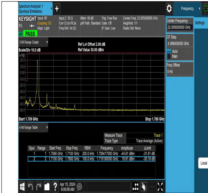
5MHz-15MHz_QPSK@QPSK-QPSK@QPSK_132002-132095_1 RB#24@25RB#0-0RB#0@75RB#0
