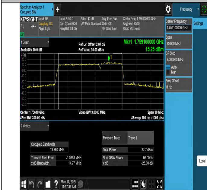
66-66-10MHz-5MHz-256QAM-256QAM-132397-132469-50RB#0-2 5RB#0-PASS
