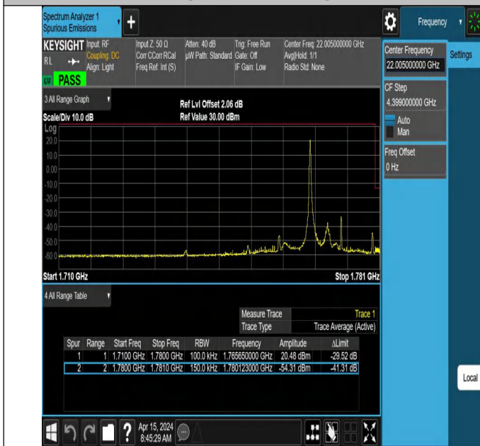
5MHz-10MHz_QPSK@QPSK-QPSK@QPSK_132550-132622_1 RB#0@25RB#0-0RB#0@50RB#0
