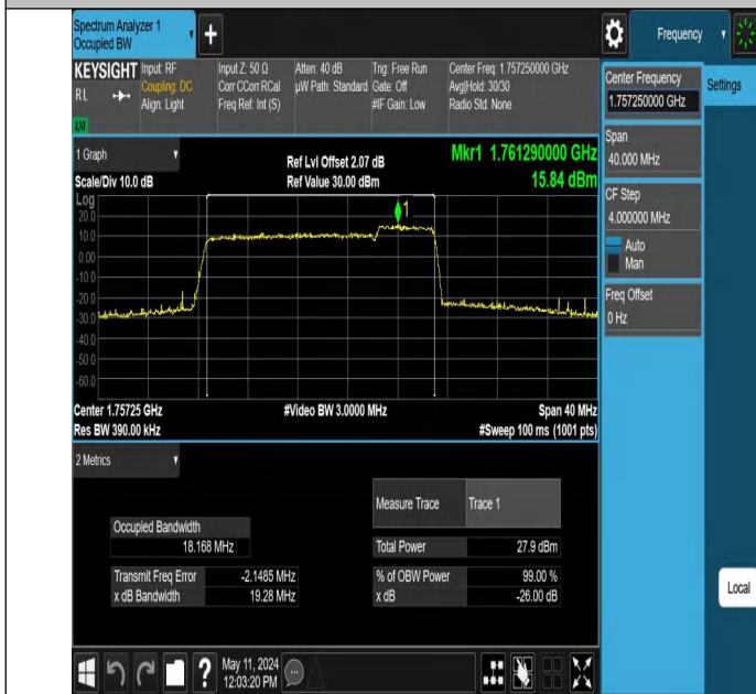
66-66-15MHz-5MHz-256QAM-256QAM-132398-132491-75RB#0-2 5RB#0-PASS
