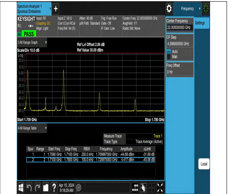
15MHz-5MHz_QPSK@QPSK-QPSK@QPSK_132047-132140_1 RB#0@75RB#0-1RB#24@25RB#0
