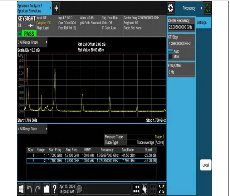
10MHz-5MHz_QPSK@QPSK-QPSK@QPSK_132022-132094_1 RB#0@50RB#0-1RB#24@25RB#0
