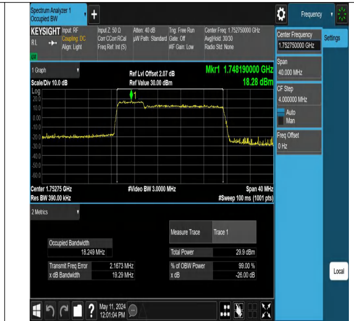
66-66-5MHz-15MHz-64QAM-64QAM-132353-132446-25RB#0-7 5RB#0-PASS
