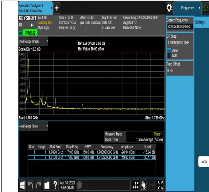
10MHz-5MHz_QPSK@QPSK-QPSK@QPSK_132022-132094_1 RB#0@50RB#0-0RB#0@25RB#0
