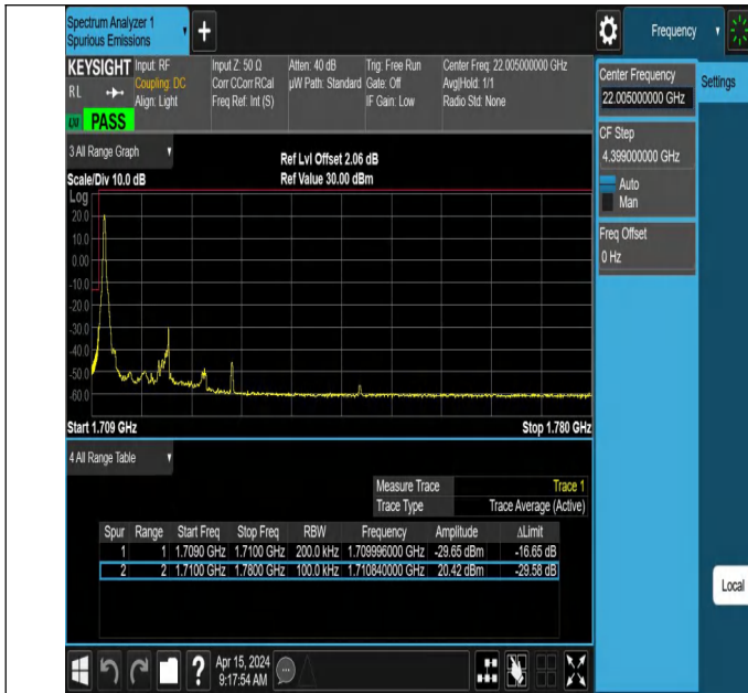
15MHz-5MHz_QPSK@QPSK-QPSK@QPSK_132047-132140_1 RB#0@75RB#0-0RB#0@25RB#0
