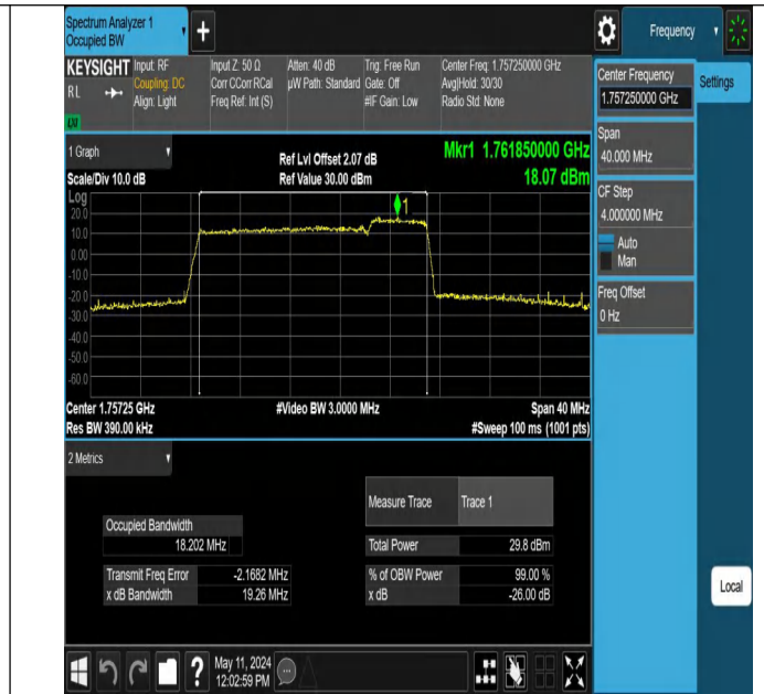
66-66-15MHz-5MHz-64QAM-64QAM-132398-132491-75RB#0-2 5RB#0-PASS
