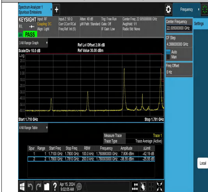
10MHz-10MHz_QPSK@QPSK-QPSK@QPSK_ 132523-132622_ 1RB#0@50RB#0-1RB#49@50RB#0
