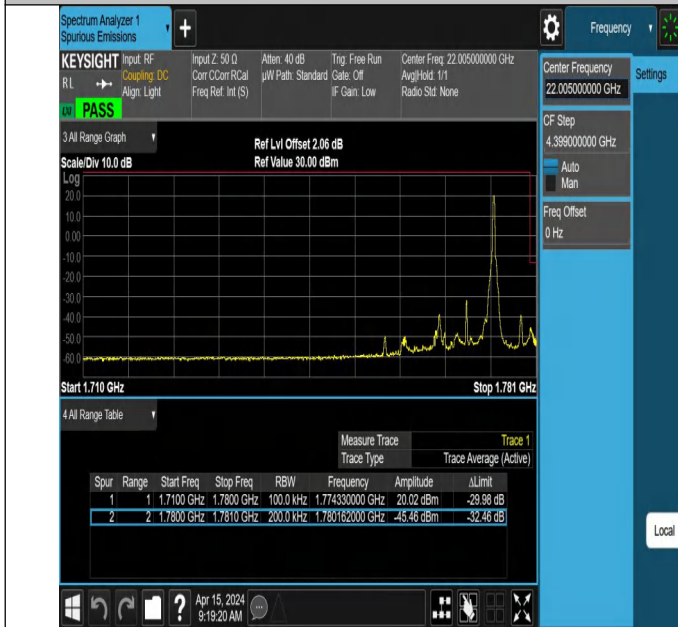
15MHz-5MHz_QPSK@QPSK-QPSK@QPSK_132549-132642_1 RB#74@75RB#0-0RB#0@25RB#0
