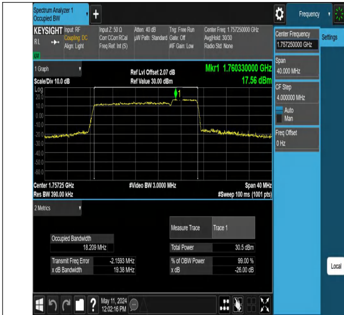
66-66-15MHz-5MHz-QPSK-QPSK-132398-132491-75RB#0-25RB #0-PASS
