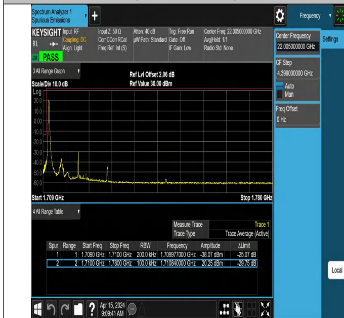
5MHz-15MHz_QPSK@QPSK-QPSK@QPSK_132002-132095_1 RB#0@25RB#0-0RB#0@75RB#0
