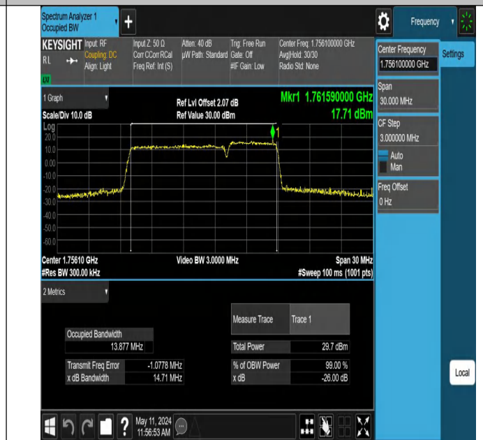
66-66-10MHz-5MHz-16QAM-16QAM-132397-132469-50RB#0-2 5RB#0-PASS
