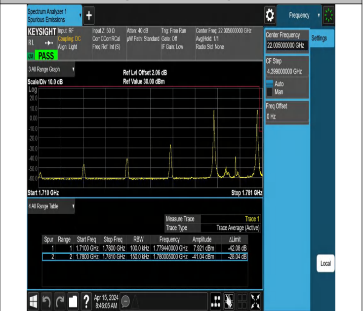
5MHz-10MHz_QPSK@QPSK-QPSK@QPSK_132550-132622_1 RB#0@25RB#0-1RB#49@50RB#0
