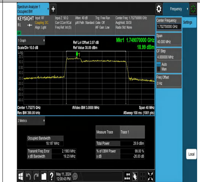
66-66-5MHz-15MHz-16QAM-16QAM-132353-132446-25RB#0-7 5RB#0-PASS
