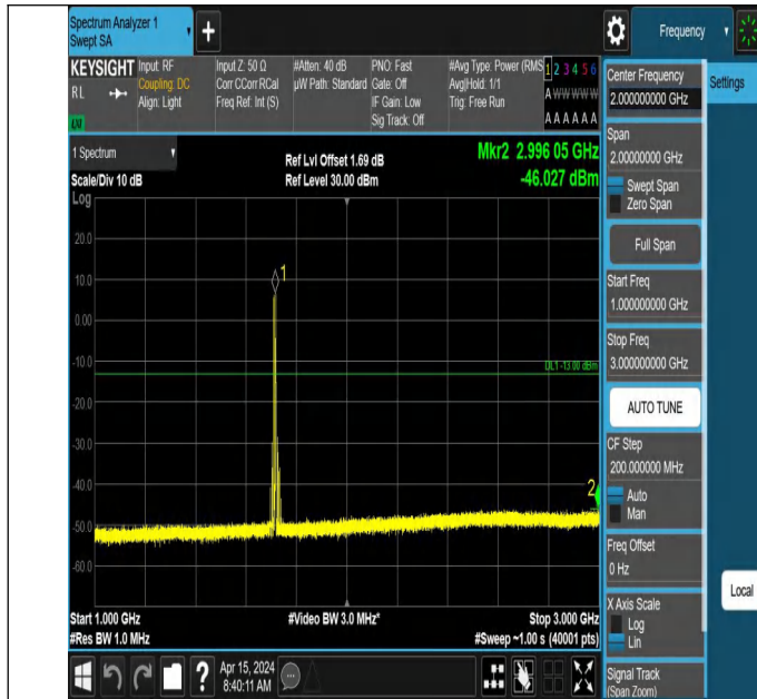
66-66-5MHz-5MHz-QPSK-QPSK-131997-132045-1RB#0-1RB#1 5-1000~3000MHz-PASS
