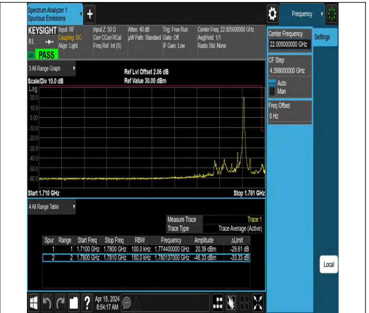
10MHz-5MHz_QPSK@QPSK-QPSK@QPSK_132572-132644_1 RB#49@50RB#0-0RB#0@25RB#0
