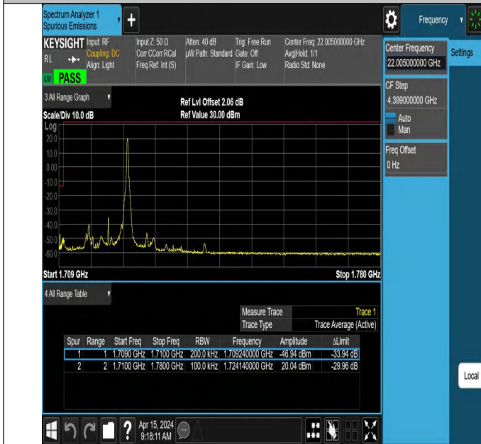
15MHz-5MHz_QPSK@QPSK-QPSK@QPSK_132047-132140_1 RB#74@75RB#0-0RB#0@25RB#0
