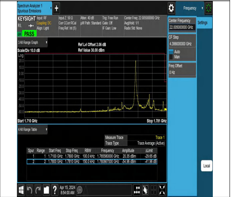
10MHz-5MHz_QPSK@QPSK-QPSK@QPSK_132572-132644_1 RB#0@50RB#0-0RB#0@25RB#0
