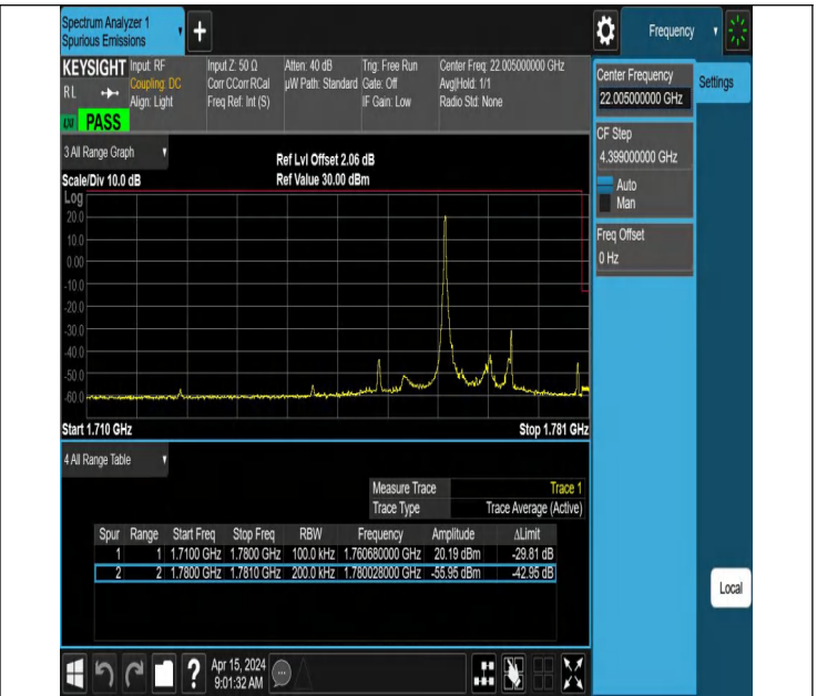
10MHz-10MHz_QPSK@QPSK-QPSK@QPSK_ 132523-132622_ 1RB#0@50RB#0-0RB#0@50RB#0
