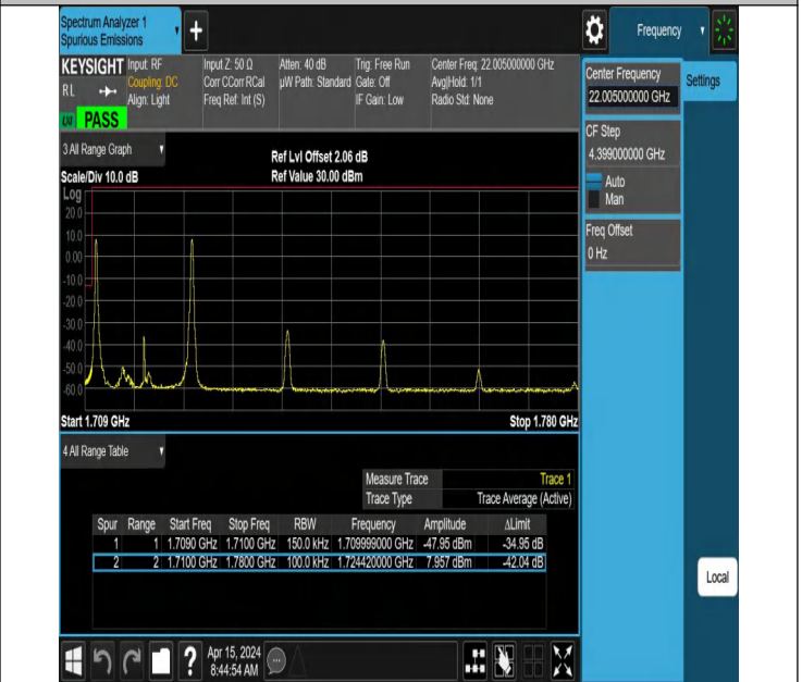
5MHz-10MHz_QPSK@QPSK-QPSK@QPSK_132000-132072_1 RB#0@25RB#0-1RB#49@50RB#0
