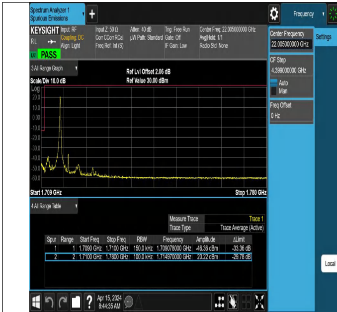
5MHz-10MHz_QPSK@QPSK-QPSK@QPSK_132000-132072_1 RB#24@25RB#0-0RB#0@50RB#0
