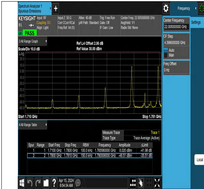
10MHz-5MHz_QPSK@QPSK-QPSK@QPSK_132572-132644_1 RB#0@50RB#0-1RB#24@25RB#0
