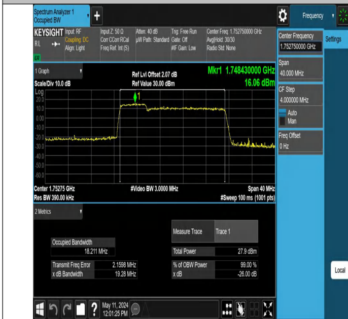
66-66-5MHz-15MHz-256QAM-256QAM-132353-132446-25RB#0-7 5RB#0-PASS
