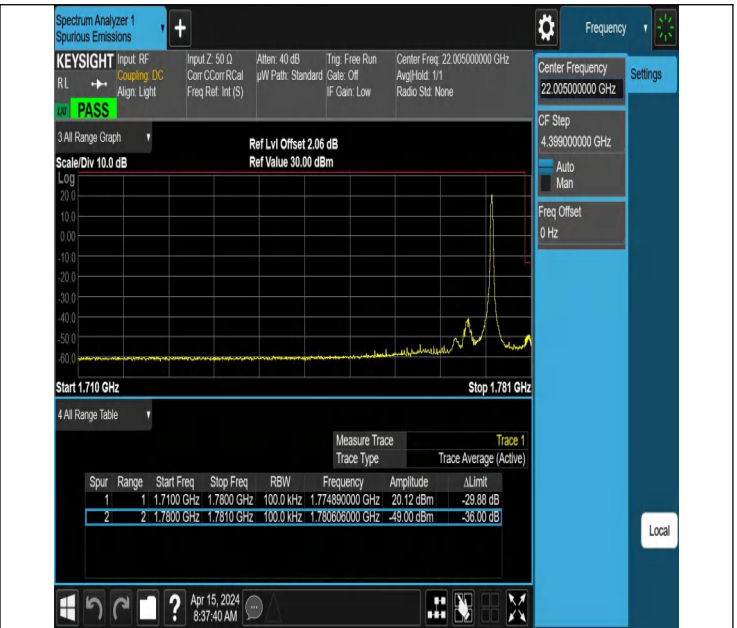
5MHz-5MHz_QPSK@QPSK-QPSK@QPSK_132599-132647_1R B#24@25RB#0-0RB#0@25RB#0
