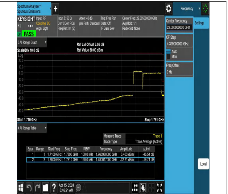
5MHz-10MHz_QPSK@QPSK-QPSK@QPSK_132550-132622_2 5RB#0@25RB#0-50RB#0@50RB#0
