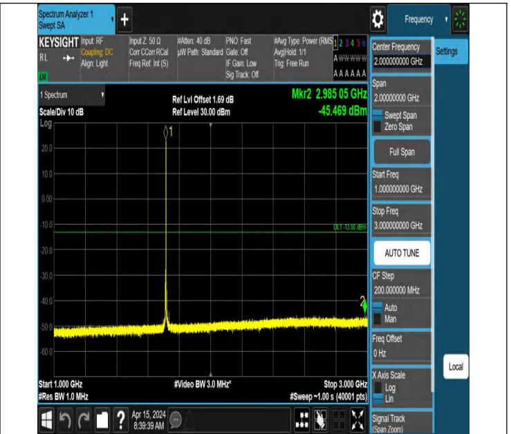
66-66-5MHz-5MHz-QPSK-QPSK-131997-132045-1RB#24-0RB# 0-1000~3000MHz-PASS
