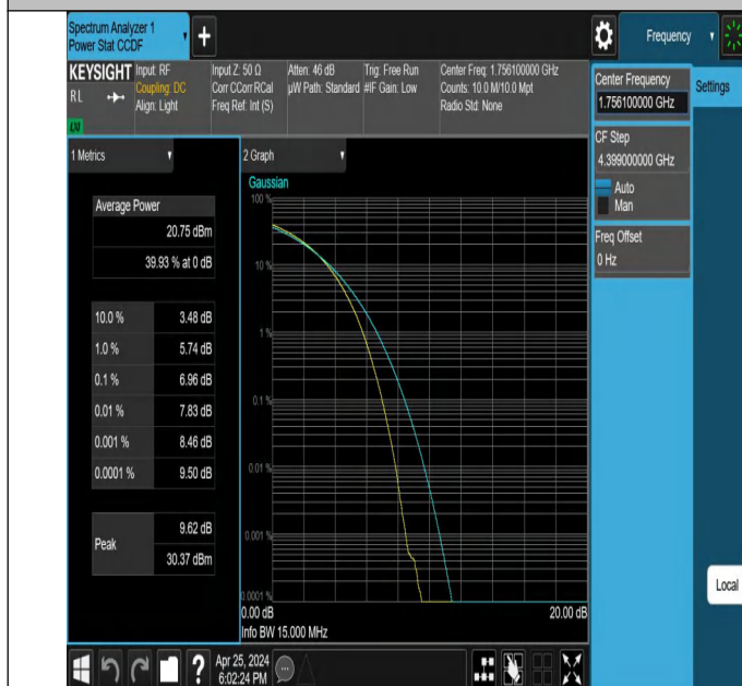
66-66-10MHz-5MHz-16QAM-16QAM-132397-132469-50RB#0-25 RB#0-PASS
