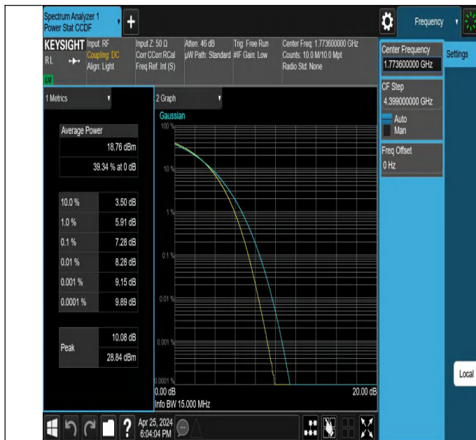
66-66-10MHz-5MHz-256QAM-256QAM-132572-132644-50RB#0- 25RB#0-PASS
