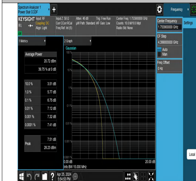
66-66-5MHz-10MHz-16QAM-16QAM-132375-132447-25RB#0-50 RB#0-PASS
