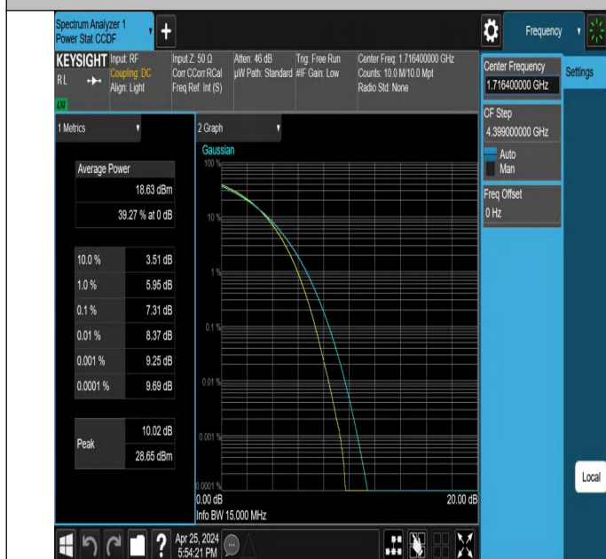
66-66-5MHz-10MHz-256QAM-256QAM-132000-132072-25RB#0- 50RB#0-PASS
