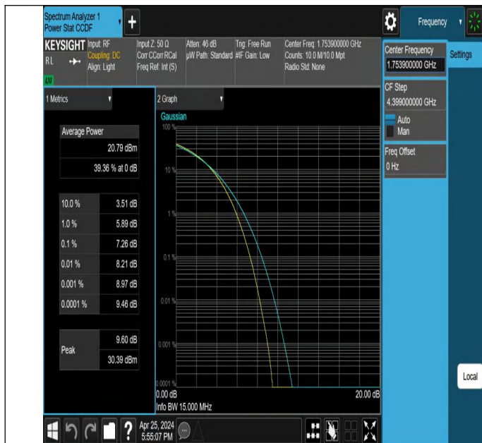
66-66-5MHz-10MHz-64QAM-64QAM-132375-132447-25RB#0-50 RB#0-PASS
