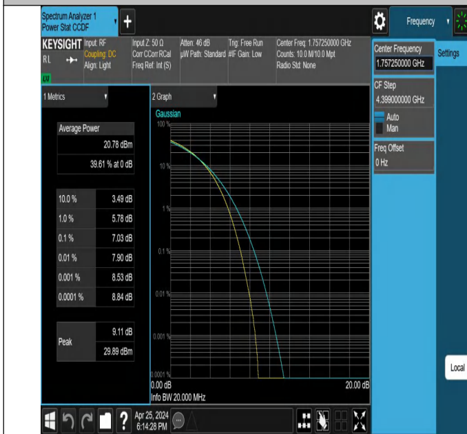
66-66-15MHz-5MHz-16QAM-16QAM-132398-132491-75RB#0-25RB#0-PASS
