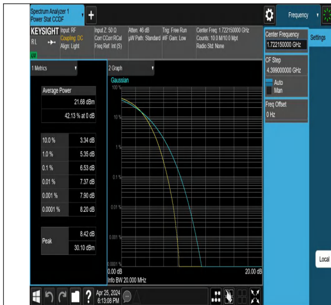
66-66-15MHz-5MHz-QPSK-QPSK-132047-132140-75RB#0-25R B#0-PASS
