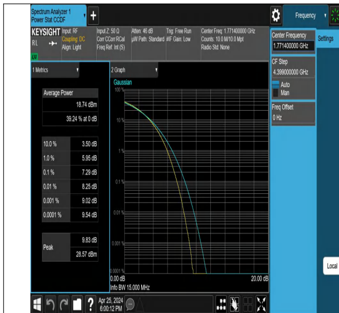
66-66-5MHz-10MHz-256QAM-256QAM-132550-132622-25RB#0- 50RB#0-PASS
