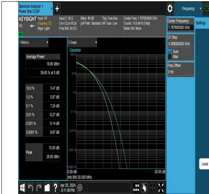
66-66-5MHz-15MHz-256QAM-256QAM-132504-132597-25RB#0-75RB#0-PASS
