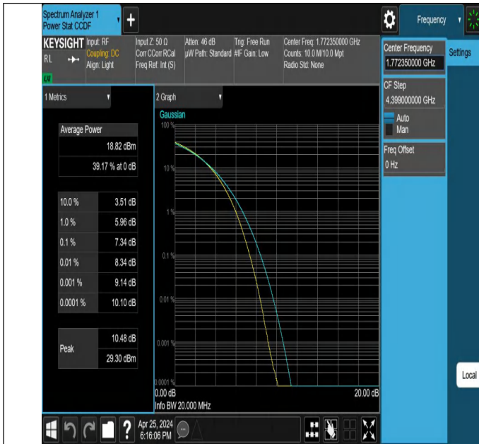
66-66-15MHz-5MHz-256QAM-256QAM-132549-132642-75RB#0-25RB#0-PASS
