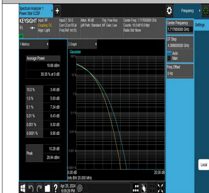
66-66-5MHz-15MHz-256QAM-256QAM-132002-132095-25RB#0- 75RB#0-PASS
