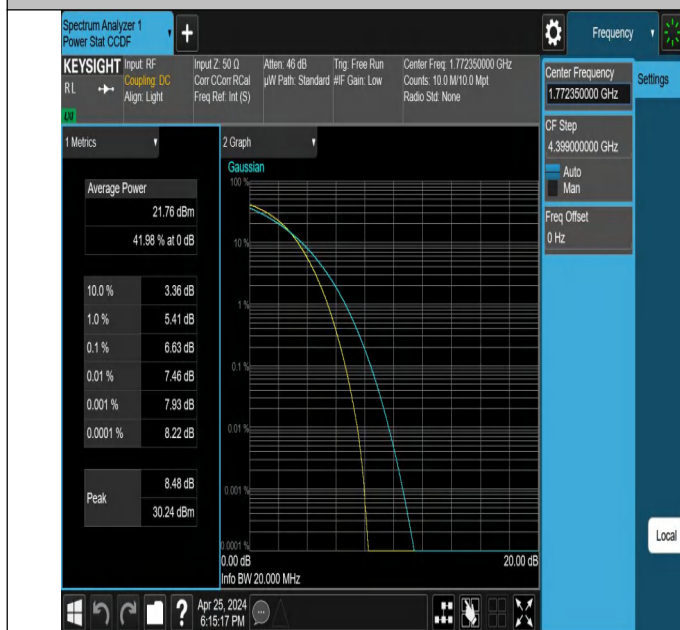
66-66-15MHz-5MHz-QPSK-QPSK-132549-132642-75RB#0-25R B#0-PASS
