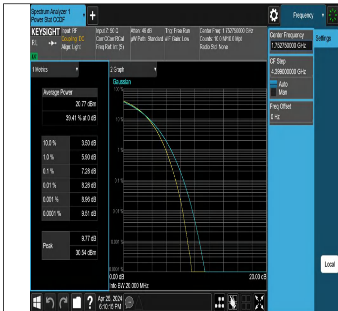
66-66-5MHz-15MHz-64QAM-64QAM-132353-132446-25RB#0-75 RB#0-PASS
