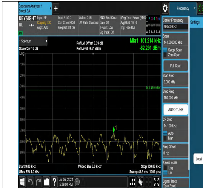
42-42(3450-3550)-20MHz-20MHz-QPSK-QPSK-42190-42388-1R B#0-1RB#99-0.009~0.15MHz-PASS
