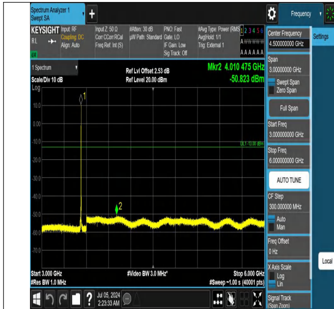
42-42(3450-3550)-15MHz-20MHz-QPSK-QPSK-42819-42990-1R B#74-ORB#0-3000~6000MHz-PASS
