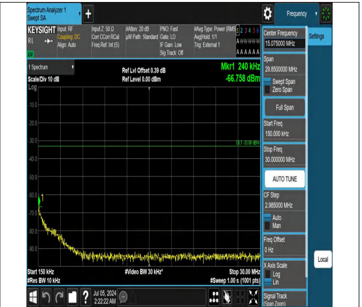
42-42(3450-3550)-15MHz-20MHz-QPSK-QPSK-42819-42990-1R B#74-ORB#0-0.15~30MHz-PASS
