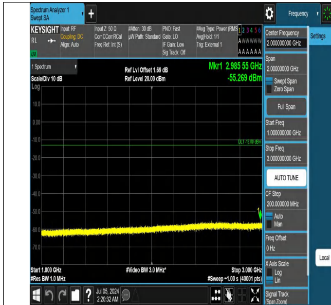
42-42(3450-3550)-15MHz-20MHz-QPSK-QPSK-42819-42990-1R B#0-ORB#0-1000~3000MHz-PASS
