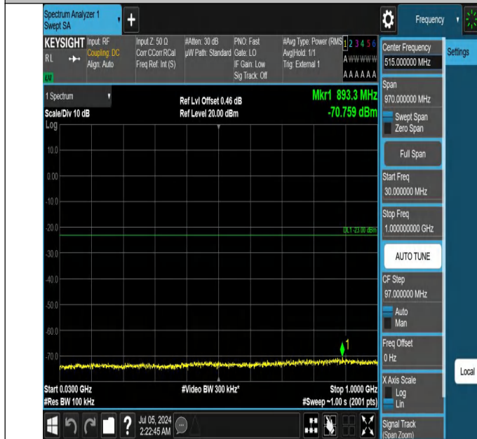
42-42(3450-3550)-15MHz-20MHz-QPSK-QPSK-42819-42990-1R B#74-ORB#0-30~1000MHz-PASS
