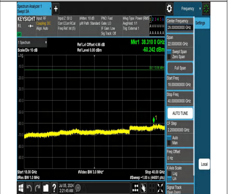
42-42(3450-3550)-15MHz-20MHz-QPSK-QPSK-42819-42990-1R B#0-ORB#0-18000~40000MHz-PASS
