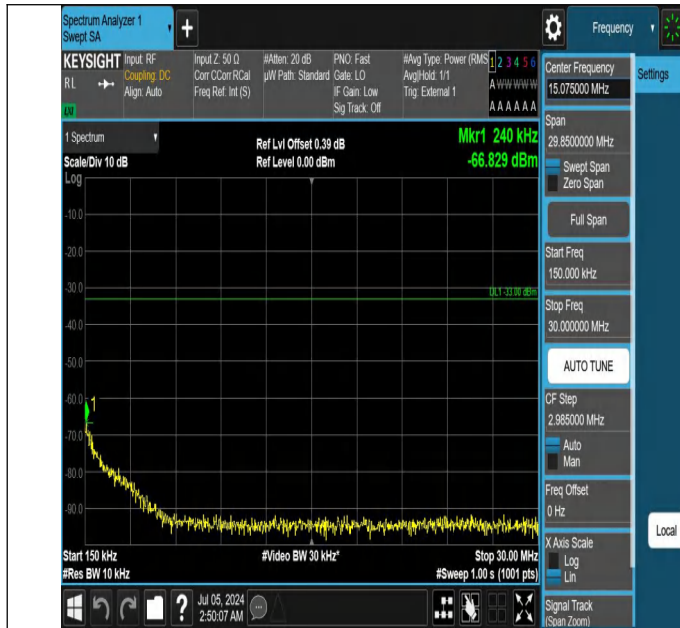
42-42(3450-3550)-20MHz-20MHz-QPSK-QPSK-42590-42788-1R B#0-ORB#0-0.15~30MHz-PASS
