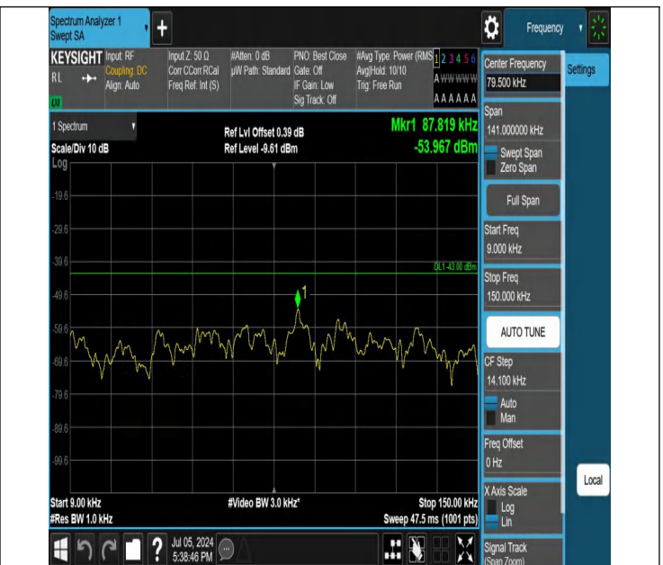
42-42(3450-3550)-20MHz-20MHz-QPSK-QPSK-42190-42388-1R B#99-0RB#0-0.009~0.15MHz-PASS
