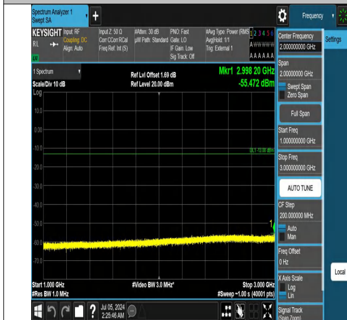
42-42(3450-3550)-15MHz-20MHz-QPSK-QPSK-42819-42990-1R B#0-1RB#99-1000~3000MHz-PASS
