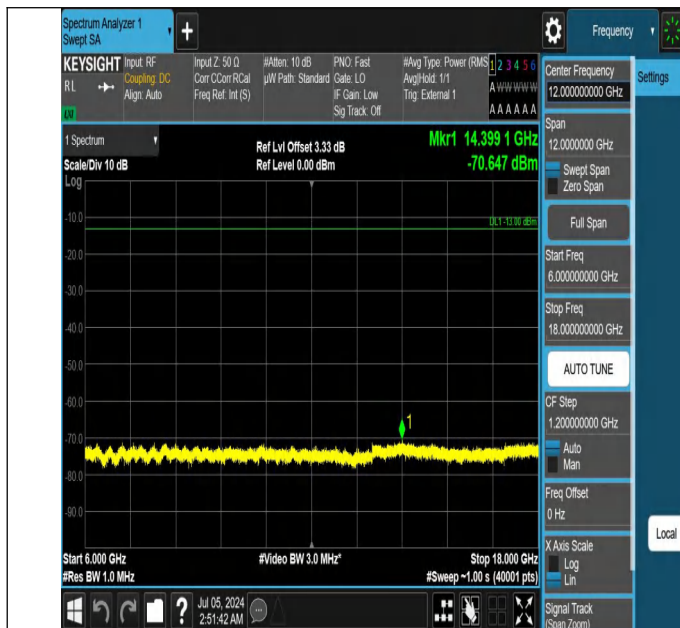
42-42(3450-3550)-20MHz-20MHz-QPSK-QPSK-42590-42788-1R B#0-0RB#0-6000~18000MHz-PASS
