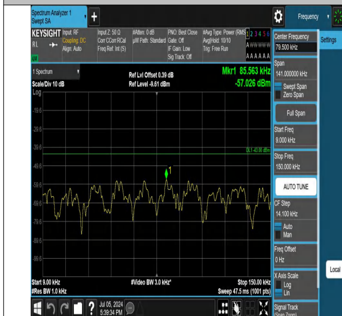
42-42(3450-3550)-20MHz-20MHz-QPSK-QPSK-42590-42788-1R B#99-0RB#0-0.009~0.15MHz-PASS
