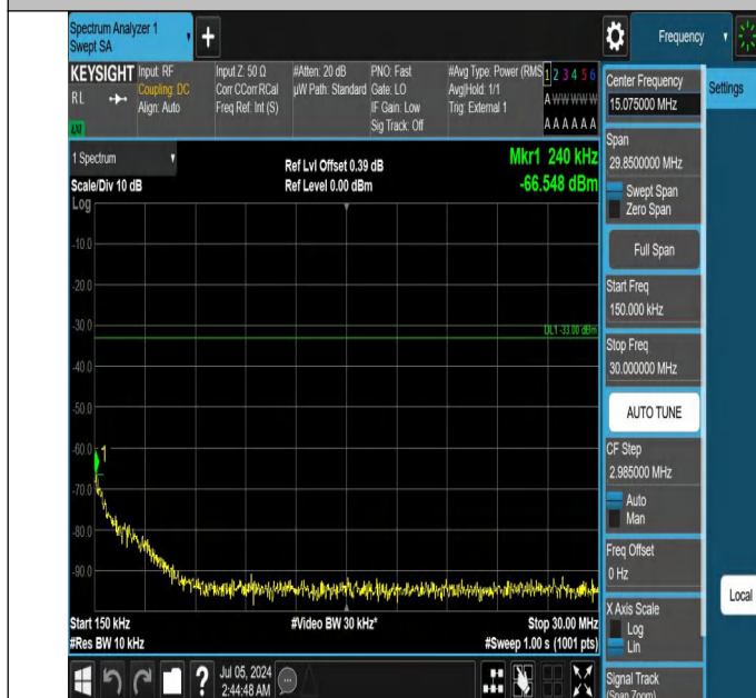
42-42(3450-3550)-20MHz-20MHz-QPSK-QPSK-42190-42388-1R B#99-0RB#0-0.15~30MHz-PASS
