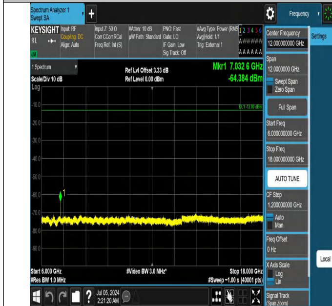
42-42(3450-3550)-15MHz-20MHz-QPSK-QPSK-42819-42990-1R B#0-ORB#0-6000~18000MHz-PASS
