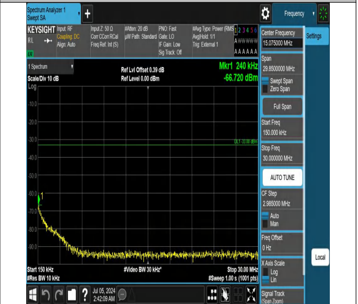
42-42(3450-3550)-20MHz-20MHz-QPSK-QPSK-42190-42388-1R B#0-0RB#0-0.15~30MHz-PASS
