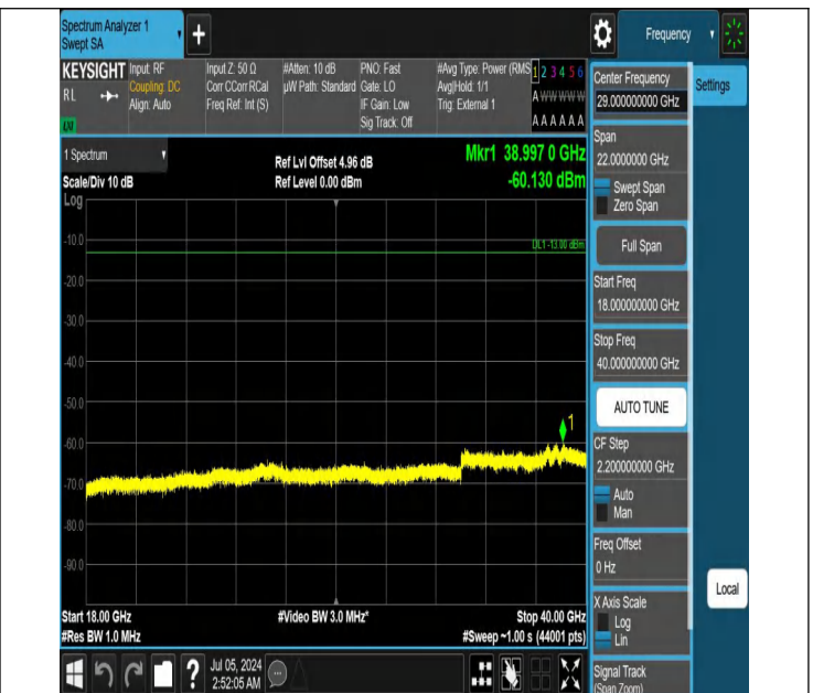
42-42(3450-3550)-20MHz-20MHz-QPSK-QPSK-42590-42788-1R B#0-0RB#0-18000~40000MHz-PASS
