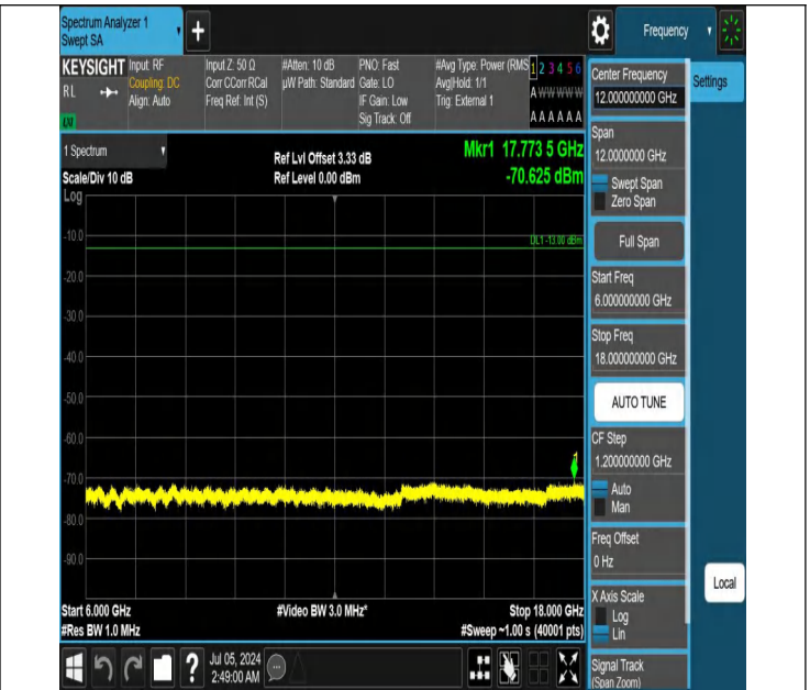
42-42(3450-3550)-20MHz-20MHz-QPSK-QPSK-42190-42388-1R B#0-1RB#99-6000~18000MHz-PASS
