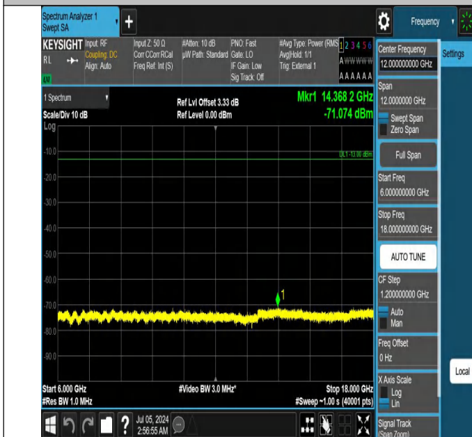
42-42(3450-3550)-20MHz-20MHz-QPSK-QPSK-42590-42788-1R B#0-1RB#99-6000~18000MHz-PASS
