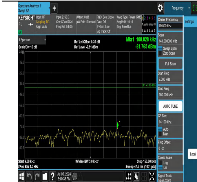
42-42(3450-3550)-20MHz-20MHz-QPSK-QPSK-42792-42990-1R B#0-1RB#99-0.009~0.15MHz-PASS
