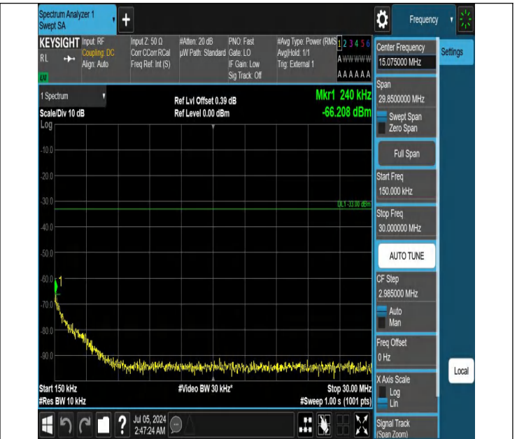
42-42(3450-3550)-20MHz-20MHz-QPSK-QPSK-42190-42388-1R B#0-1RB#99-0.15~30MHz-PASS
