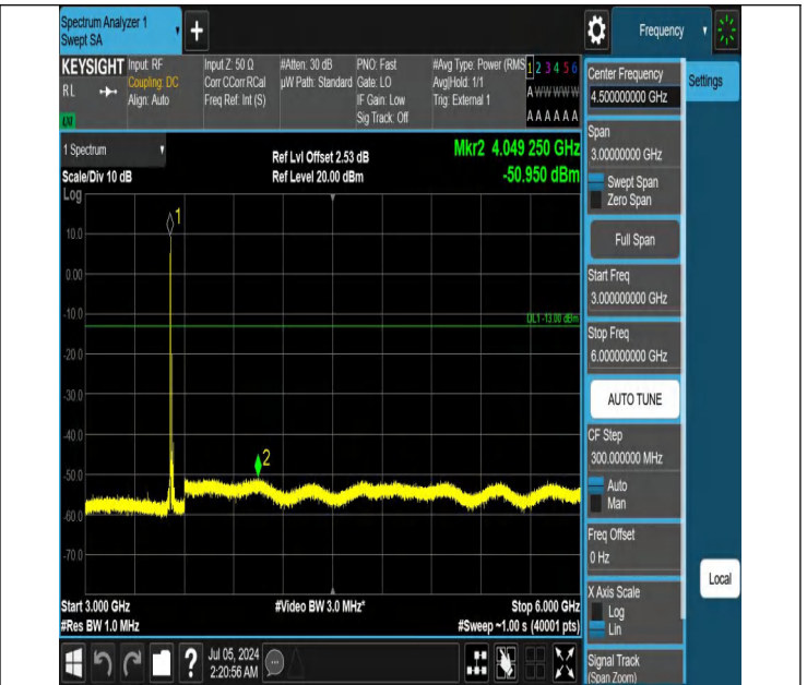
42-42(3450-3550)-15MHz-20MHz-QPSK-QPSK-42819-42990-1R B#0-ORB#0-3000~6000MHz-PASS
