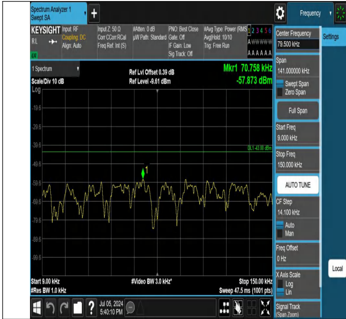
42-42(3450-3550)-20MHz-20MHz-QPSK-QPSK-42792-42990-1R B#0-ORB#0-0.009~0.15MHz-PASS
