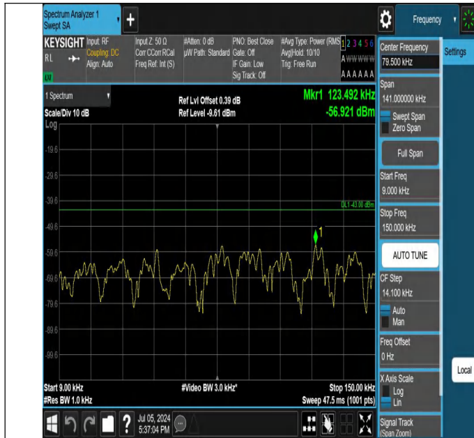
42-42(3450-3550)-15MHz-20MHz-QPSK-QPSK-42819-42990-1R B#74-ORB#0-0.009~0.15MHz-PASS
