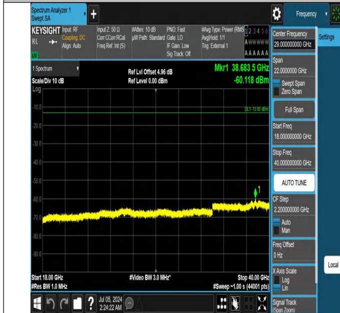
42-42(3450-3550)-15MHz-20MHz-QPSK-QPSK-42819-42990-1R B#74-ORB#0-18000~40000MHz-PASS
