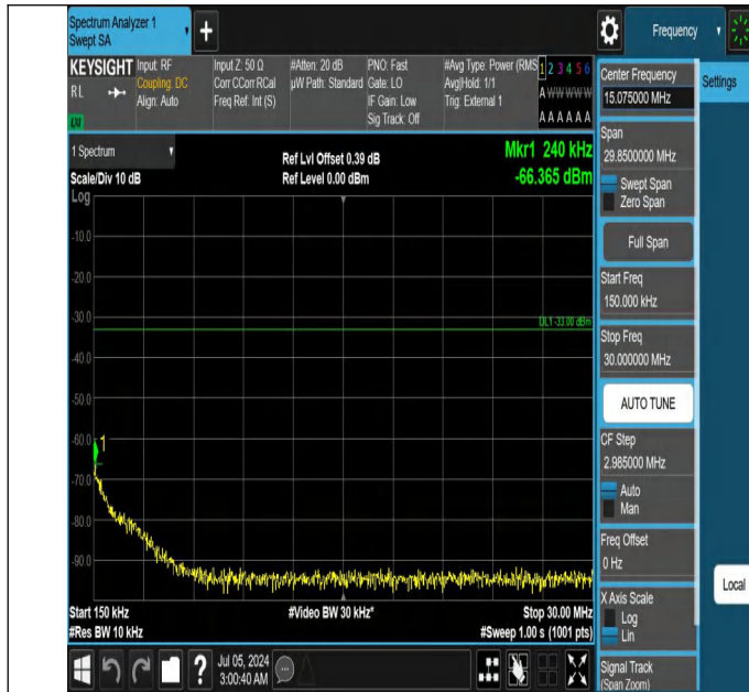
42-42(3450-3550)-20MHz-20MHz-QPSK-QPSK-42792-42990-1R B#99-ORB#0-0.15~30MHz-PASS
