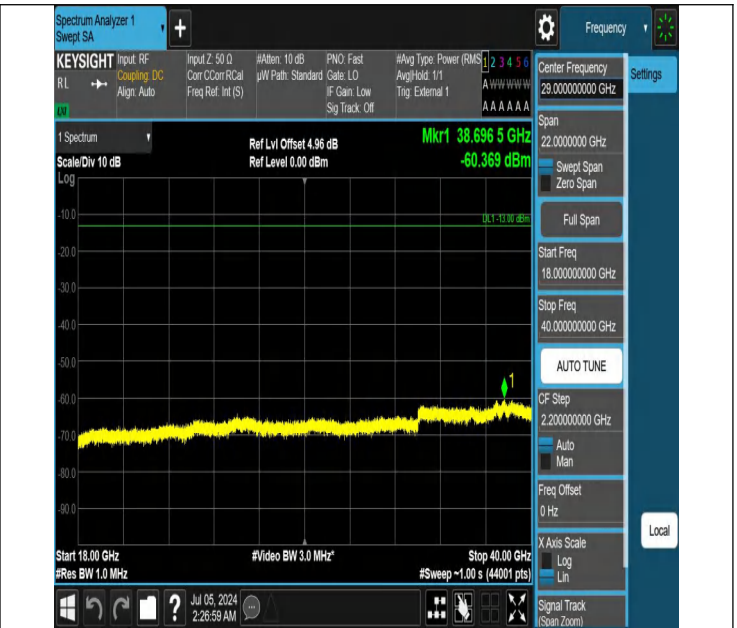
42-42(3450-3550)-15MHz-20MHz-QPSK-QPSK-42819-42990-1R B#0-1RB#99-18000~40000MHz-PASS
