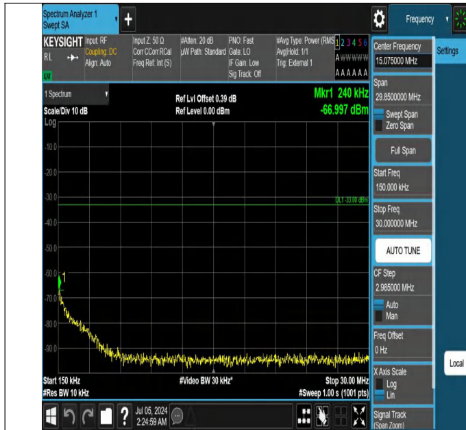
42-42(3450-3550)-15MHz-20MHz-QPSK-QPSK-42819-42990-1R B#0-1RB#99-0.15~30MHz-PASS
