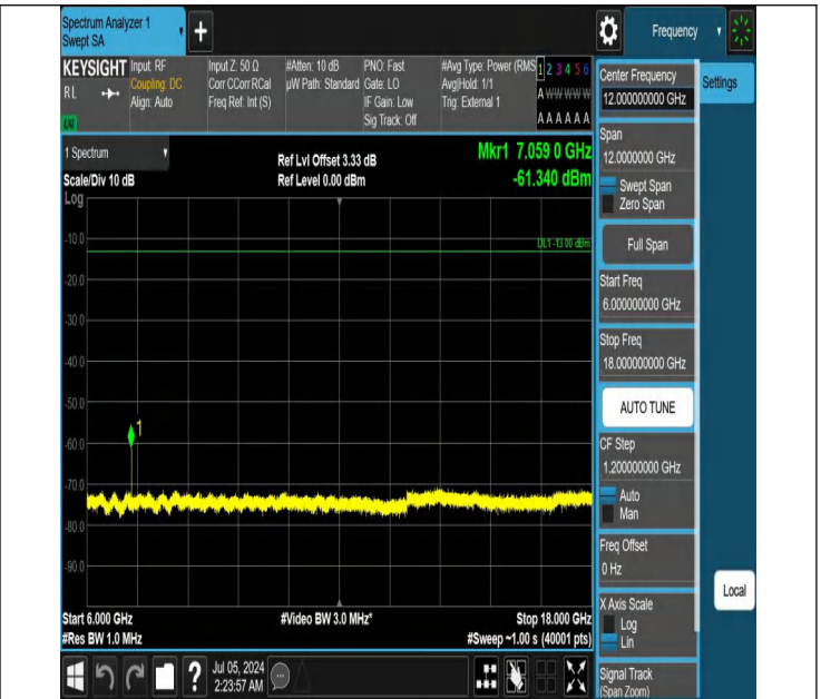
42-42(3450-3550)-15MHz-20MHz-QPSK-QPSK-42819-42990-1R B#74-ORB#0-6000~18000MHz-PASS
