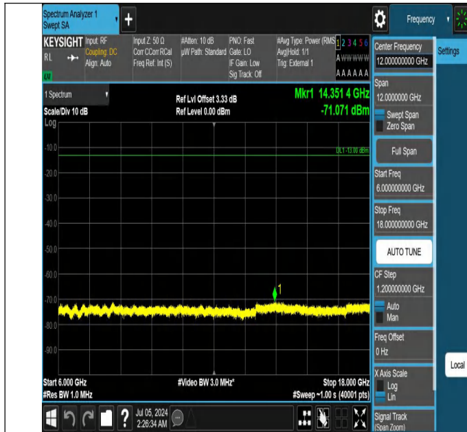
42-42(3450-3550)-15MHz-20MHz-QPSK-QPSK-42819-42990-1R B#0-1RB#99-6000~18000MHz-PASS
