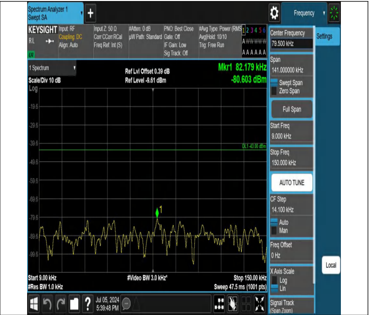
42-42(3450-3550)-20MHz-20MHz-QPSK-QPSK-42590-42788-1R B#0-1RB#99-0.009~0.15MHz-PASS
