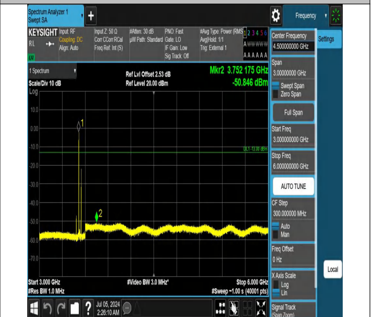
42-42(3450-3550)-15MHz-20MHz-QPSK-QPSK-42819-42990-1R B#0-1RB#99-3000~6000MHz-PASS
