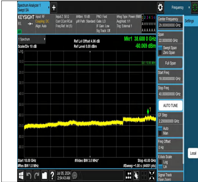
42-42(3450-3550)-20MHz-20MHz-QPSK-QPSK-42590-42788-1R B#99-0RB#0-18000~40000MHz-PASS
