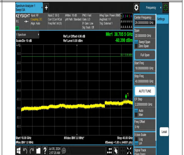
42-42(3450-3550)-20MHz-20MHz-QPSK-QPSK-42590-42788-1R B#0-1RB#99-18000~40000MHz-PASS
