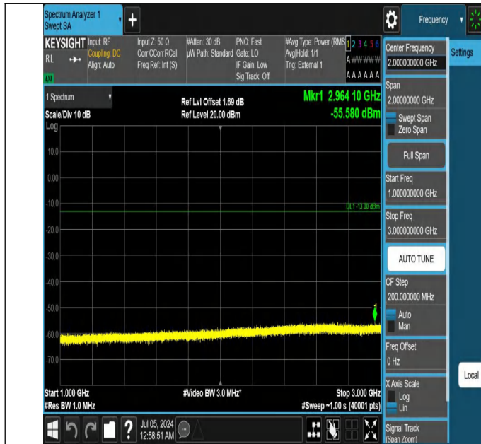
42-42(3450-3550)-5MHz-20MHz-QPSK-QPSK-42590-42707-1RB #24-ORB#0-1000~3000MHz-PASS
