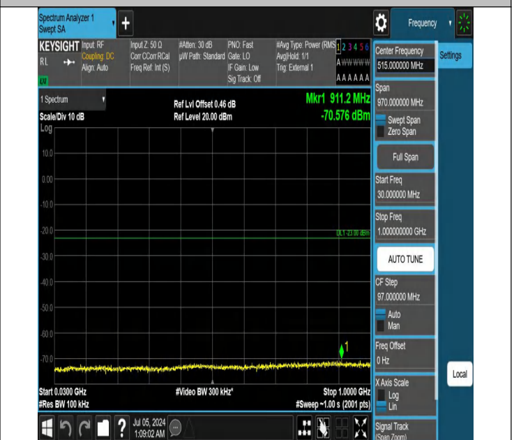
42-42(3450-3550)-5MHz-20MHz-QPSK-QPSK-42873-42990-1RB #0-1RB#99-30~1000MHz-PASS
