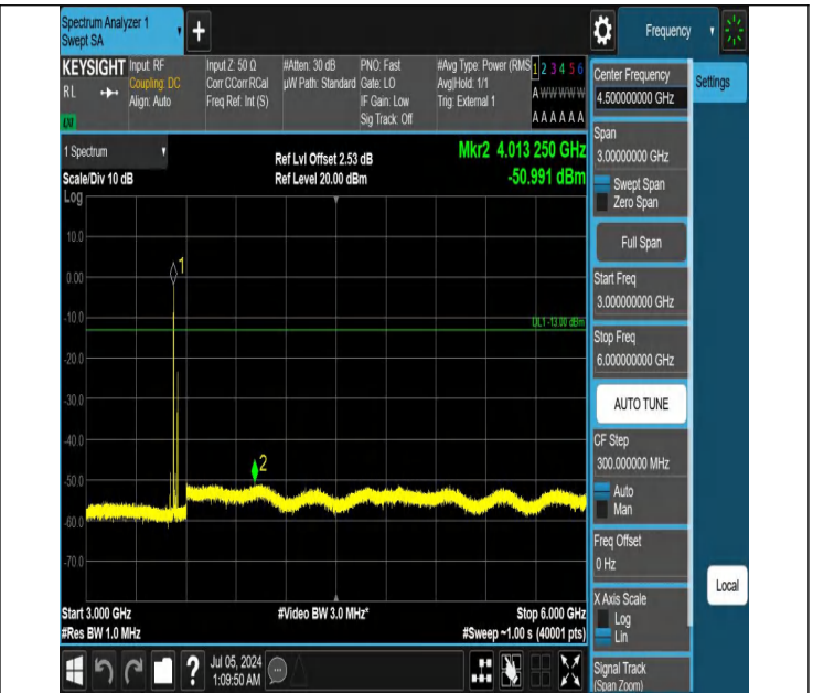
42-42(3450-3550)-5MHz-20MHz-QPSK-QPSK-42873-42990-1RB #0-1RB#99-3000~6000MHz-PASS
