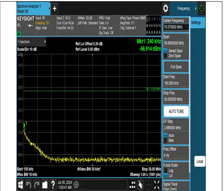
42-42(3450-3550)-5MHz-20MHz-QPSK-QPSK-42590-42707-1RB #0-1RB#99-0.15~30MHz-PASS
