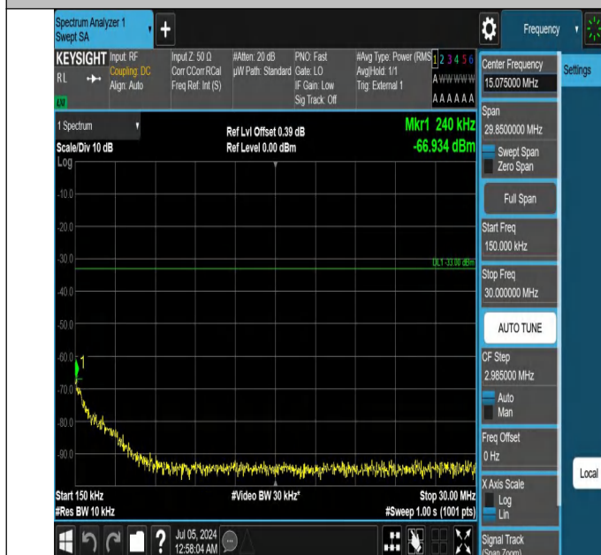
42-42(3450-3550)-5MHz-20MHz-QPSK-QPSK-42590-42707-1RB #24-0RB#0-0.15~30MHz-PASS
