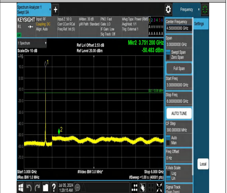
42-42(3450-3550)-10MHz-20MHz-QPSK-QPSK-42140-42284-1R B#49-ORB#0-3000~6000MHz-PASS
