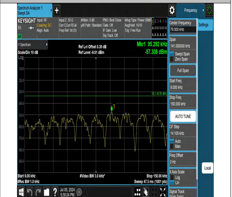
42-42(3450-3550)-5MHz-20MHz-QPSK-QPSK-42873-42990-1RB #0-0RB#0-0.009~0.15MHz-PASS
