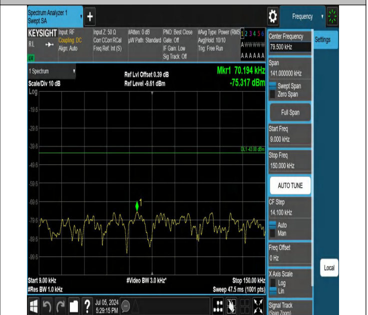
42-42(3450-3550)-5MHz-20MHz-QPSK-QPSK-42115-42232-1RB #0-1RB#99-0.009~0.15MHz-PASS
