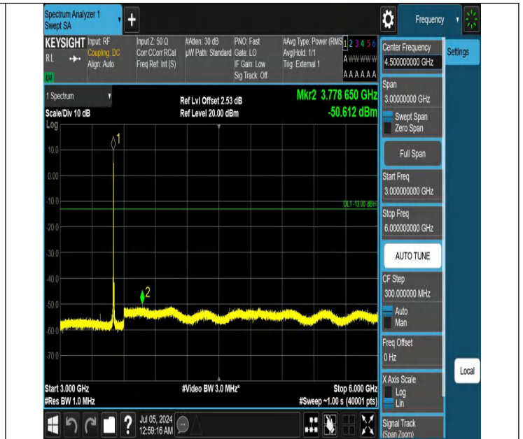
42-42(3450-3550)-5MHz-20MHz-QPSK-QPSK-42590-42707-1RB #24-ORB#0-3000~6000MHz-PASS
