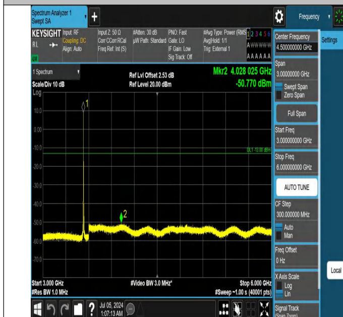
42-42(3450-3550)-5MHz-20MHz-QPSK-QPSK-42873-42990-1RB #24-0RB#0-3000~6000MHz-PASS
