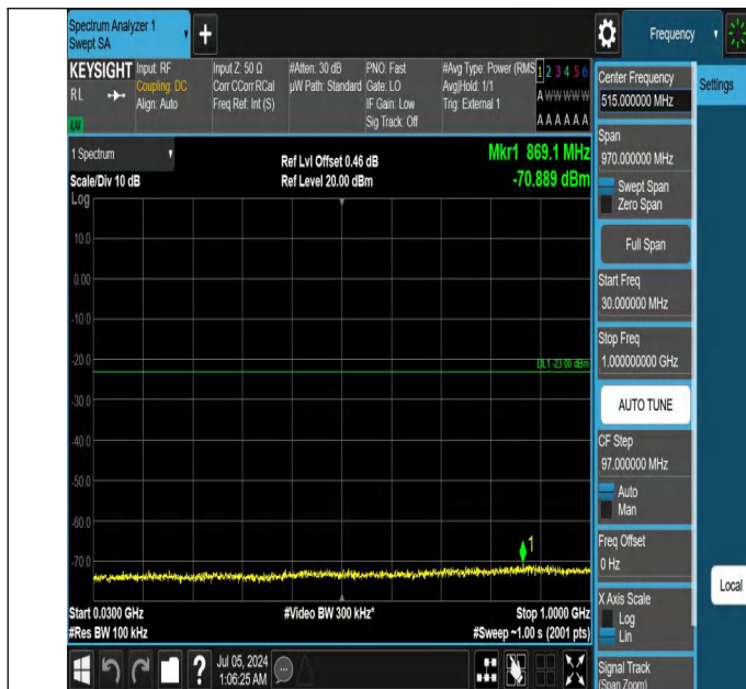
42-42(3450-3550)-5MHz-20MHz-QPSK-QPSK-42873-42990-1RB #24-0RB#0-30~1000MHz-PASS
