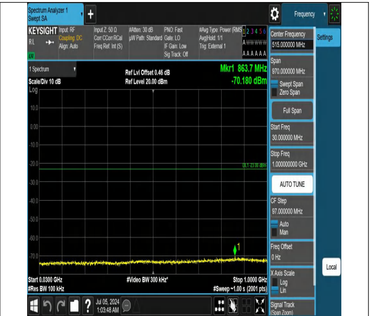
42-42(3450-3550)-5MHz-20MHz-QPSK-QPSK-42873-42990-1RB #0-ORB#0-30~1000MHz-PASS
