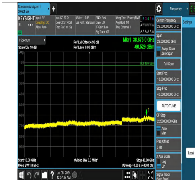
42-42(3450-3550)-5MHz-20MHz-QPSK-QPSK-42590-42707-1RB #0-0RB#0-18000~40000MHz-PASS
