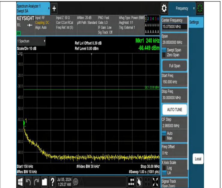
42-42(3450-3550)-10MHz-20MHz-QPSK-QPSK-42140-42284-1R B#0-ORB#0-0.15~30MHz-PASS
