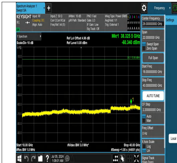
42-42(3450-3550)-5MHz-20MHz-QPSK-QPSK-42873-42990-1RB #24-0RB#0-18000~40000MHz-PASS
