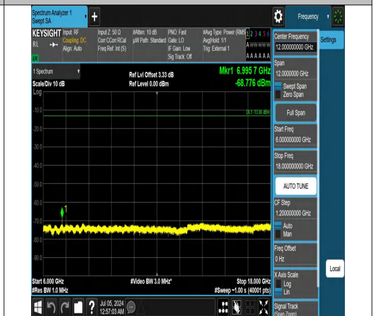
42-42(3450-3550)-5MHz-20MHz-QPSK-QPSK-42590-42707-1RB #0-0RB#0-6000~18000MHz-PASS
