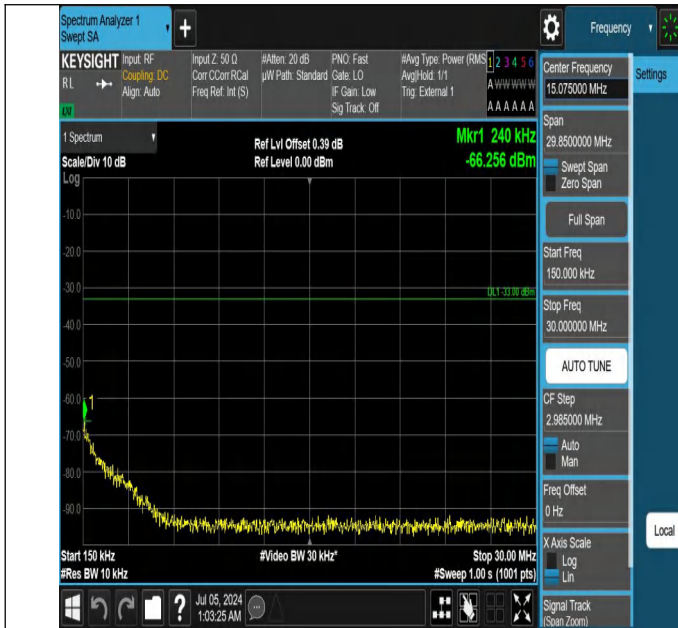
42-42(3450-3550)-5MHz-20MHz-QPSK-QPSK-42873-42990-1RB #0-ORB#0-0.15~30MHz-PASS
