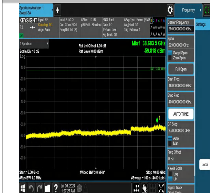
42-42(3450-3550)-10MHz-20MHz-QPSK-QPSK-42140-42284-1R B#0-0RB#0-18000~40000MHz-PASS
