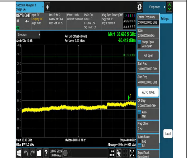
42-42(3450-3550)-5MHz-20MHz-QPSK-QPSK-42590-42707-1RB #24-ORB#0-18000~40000MHz-PASS
