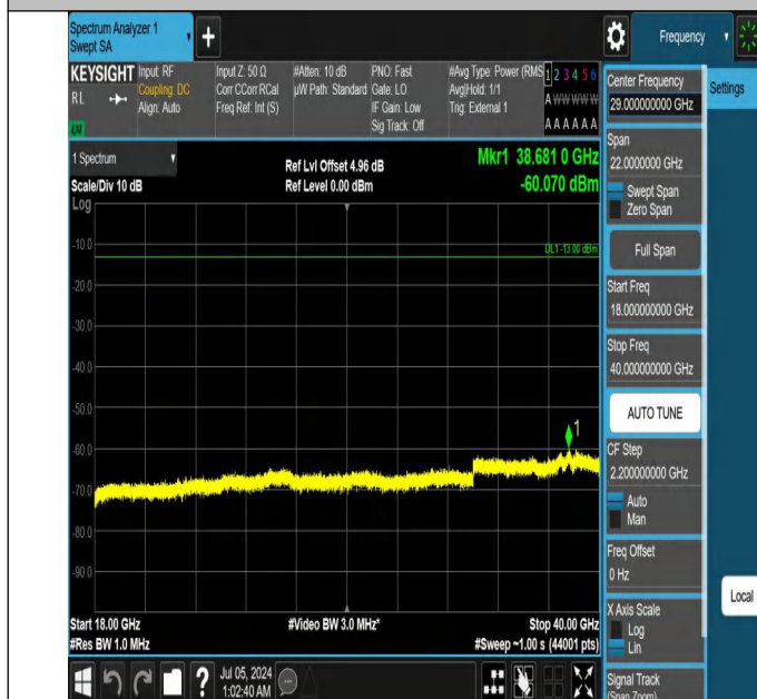
42-42(3450-3550)-5MHz-20MHz-QPSK-QPSK-42590-42707-1RB #0-1RB#99-18000~40000MHz-PASS
