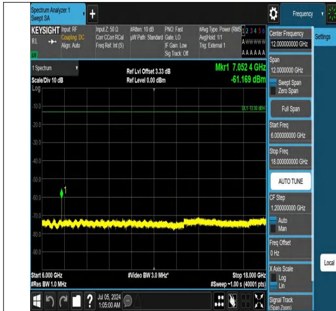
42-42(3450-3550)-5MHz-20MHz-QPSK-QPSK-42873-42990-1RB #0-0RB#0-6000~18000MHz-PASS
