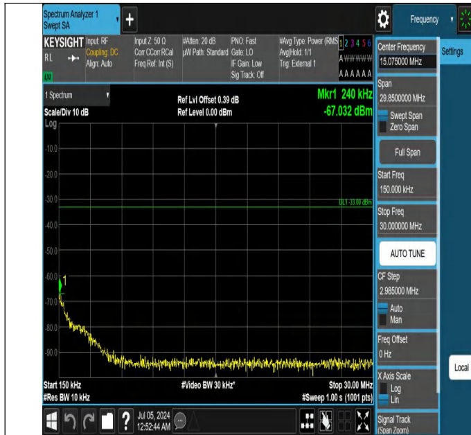
42-42(3450-3550)-5MHz-20MHz-QPSK-QPSK-42115-42232-1RB #0-1RB#99-0.15~30MHz-PASS
