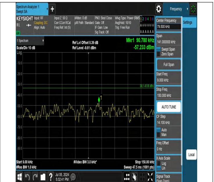
42-42(3450-3550)-10MHz-20MHz-QPSK-QPSK-42590-42734-1R B#0-0RB#0-0.009~0.15MHz-PASS
