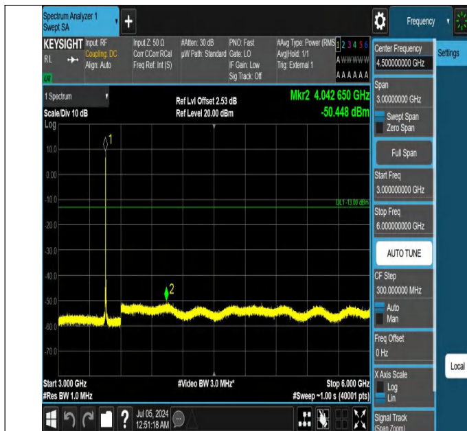
42-42(3450-3550)-5MHz-20MHz-QPSK-QPSK-42115-42232-1RB #24-0RB#0-3000~6000MHz-PASS
