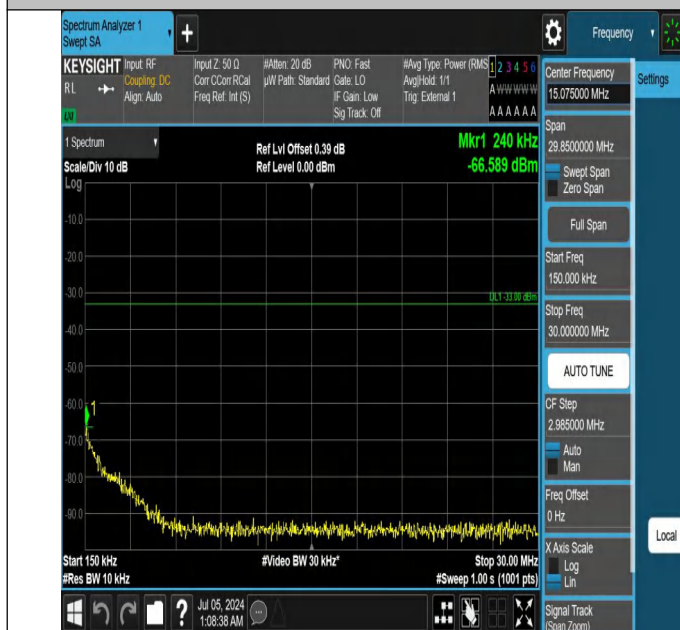
42-42(3450-3550)-5MHz-20MHz-QPSK-QPSK-42873-42990-1RB #0-1RB#99-0.15~30MHz-PASS
