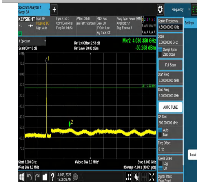
42-42(3450-3550)-5MHz-20MHz-QPSK-QPSK-42590-42707-1RB #0-0RB#0-3000~6000MHz-PASS
