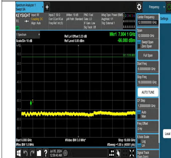
42-42(3450-3550)-5MHz-20MHz-QPSK-QPSK-42590-42707-1RB #24-ORB#0-6000~18000MHz-PASS
