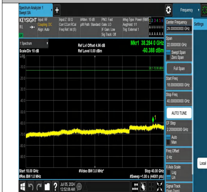
42-42(3450-3550)-5MHz-20MHz-QPSK-QPSK-42115-42232-1RB #24-0RB#0-18000~40000MHz-PASS
