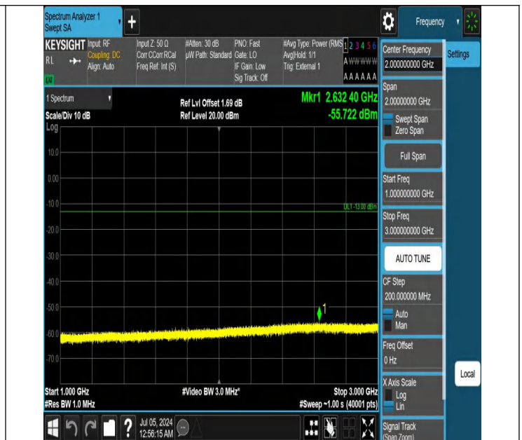
42-42(3450-3550)-5MHz-20MHz-QPSK-QPSK-42590-42707-1RB #0-0RB#0-1000~3000MHz-PASS
