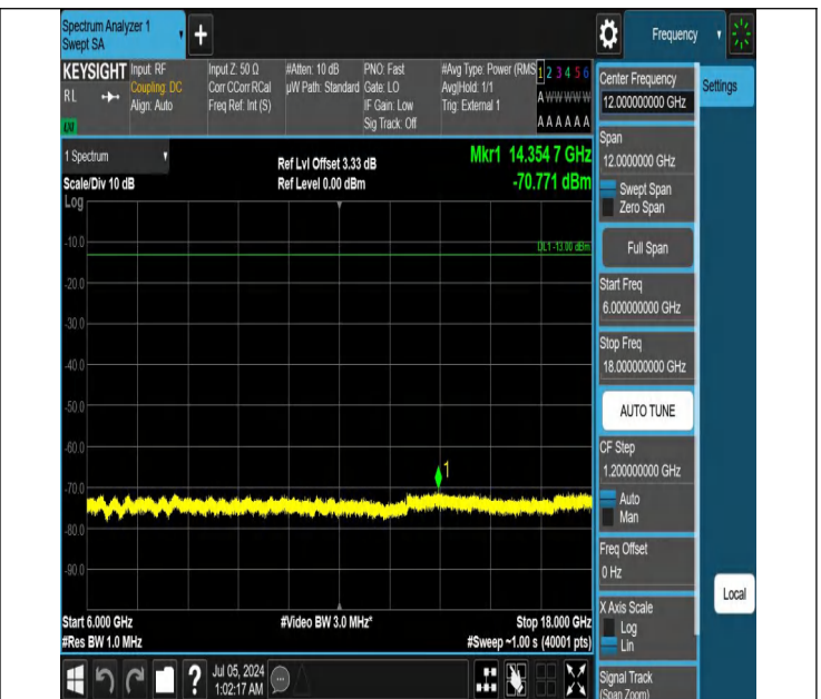
42-42(3450-3550)-5MHz-20MHz-QPSK-QPSK-42590-42707-1RB #0-1RB#99-6000~18000MHz-PASS
