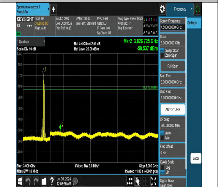
42-42(3450-3550)-5MHz-20MHz-QPSK-QPSK-42115-42232-1RB #0-1RB#99-3000~6000MHz-PASS
