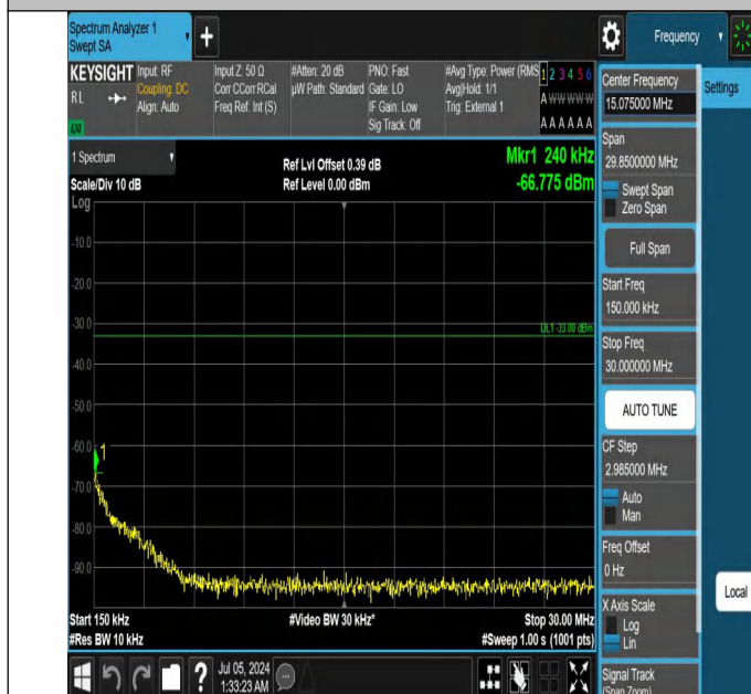
42-42(3450-3550)-10MHz-20MHz-QPSK-QPSK-42590-42734-1R B#0-0RB#0-0.15~30MHz-PASS
