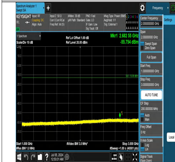
42-42(3450-3550)-5MHz-20MHz-QPSK-QPSK-42115-42232-1RB #0-1RB#99-1000~3000MHz-PASS
