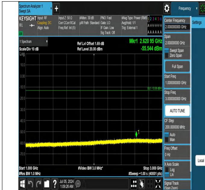
42-42(3450-3550)-5MHz-20MHz-QPSK-QPSK-42873-42990-1RB #0-1RB#99-1000~3000MHz-PASS
