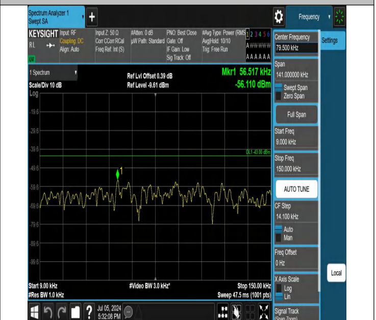
42-42(3450-3550)-10MHz-20MHz-QPSK-QPSK-42140-42284-1R B#49-0RB#0-0.009~0.15MHz-PASS
