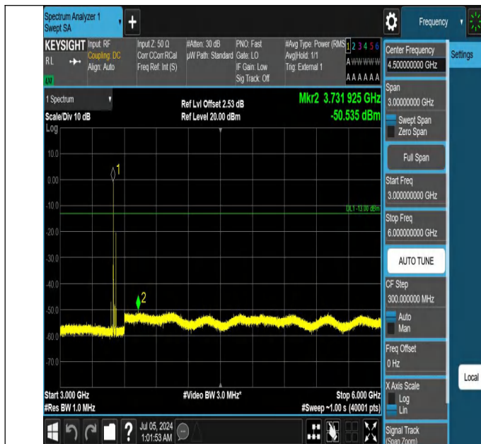
42-42(3450-3550)-5MHz-20MHz-QPSK-QPSK-42590-42707-1RB #0-1RB#99-3000~6000MHz-PASS
