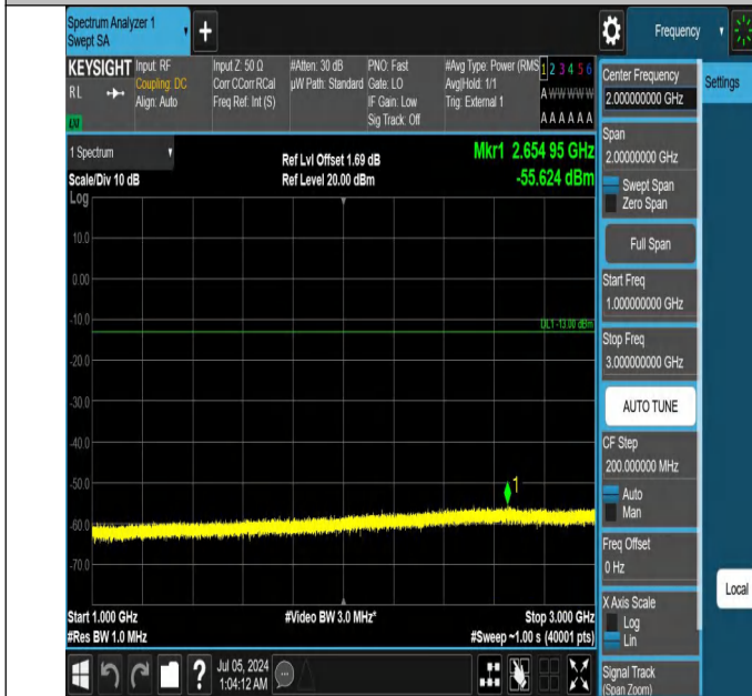
42-42(3450-3550)-5MHz-20MHz-QPSK-QPSK-42873-42990-1RB #0-ORB#0-1000~3000MHz-PASS
