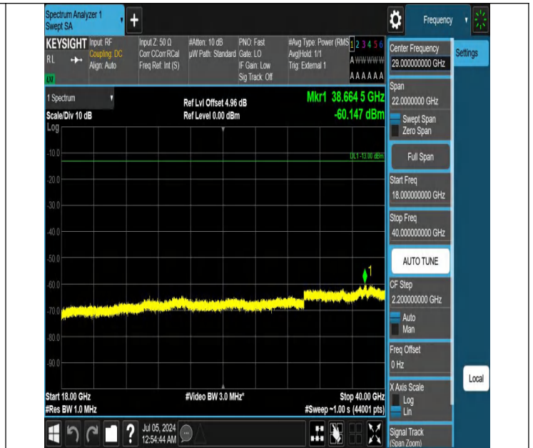
42-42(3450-3550)-5MHz-20MHz-QPSK-QPSK-42115-42232-1RB #0-1RB#99-18000~40000MHz-PASS
