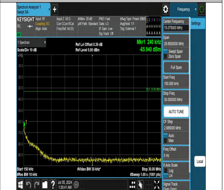
42-42(3450-3550)-10MHz-20MHz-QPSK-QPSK-42140-42284-1R B#0-1RB#99-0.15~30MHz-PASS
