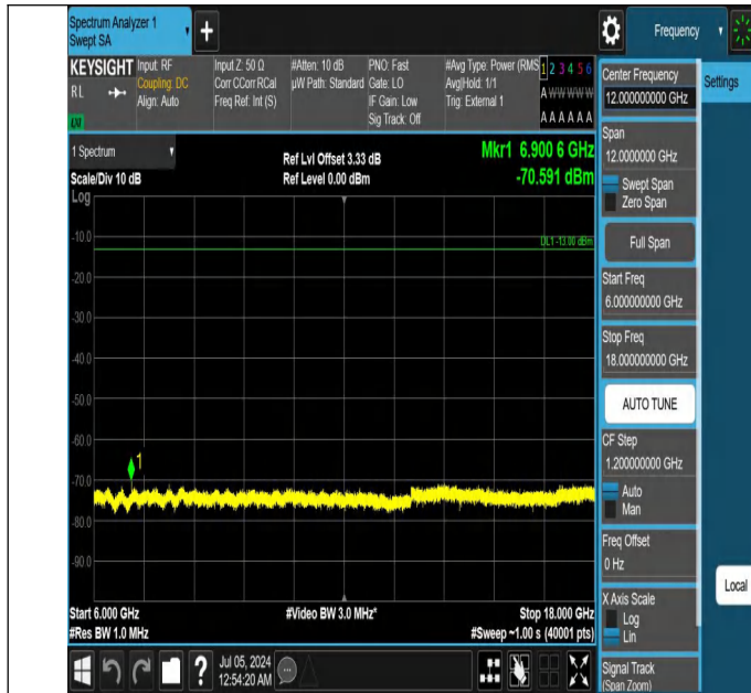
42-42(3450-3550)-5MHz-20MHz-QPSK-QPSK-42115-42232-1RB #0-1RB#99-6000~18000MHz-PASS
