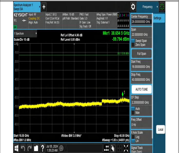
42-42(3450-3550)-10MHz-20MHz-QPSK-QPSK-42590-42734-1R B#0-ORB#0-18000~40000MHz-PASS
