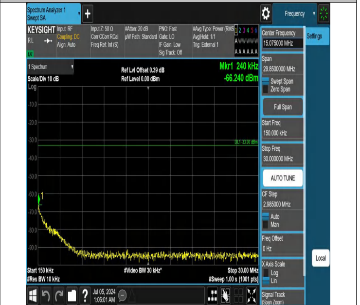
42-42(3450-3550)-5MHz-20MHz-QPSK-QPSK-42873-42990-1RB #24-0RB#0-0.15~30MHz-PASS
