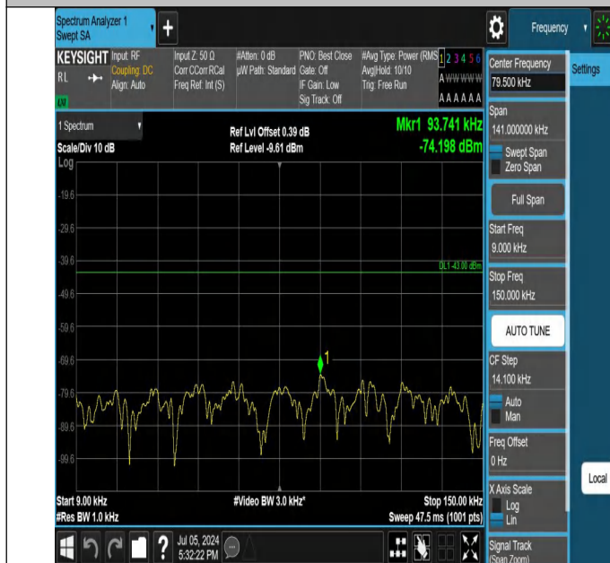
42-42(3450-3550)-10MHz-20MHz-QPSK-QPSK-42140-42284-1R B#0-1RB#99-0.009~0.15MHz-PASS
