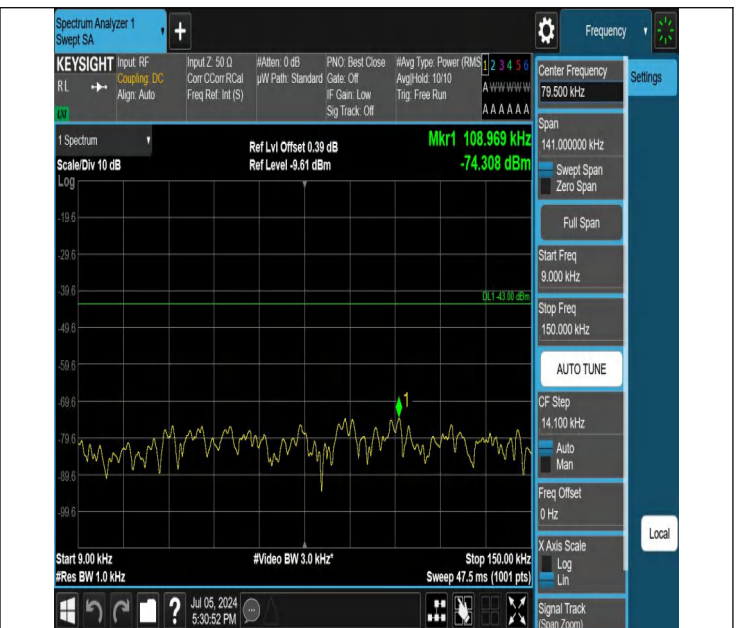
42-42(3450-3550)-5MHz-20MHz-QPSK-QPSK-42873-42990-1RB #0-1RB#99-0.009~0.15MHz-PASS
