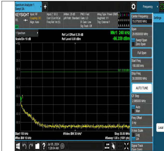
42-42(3450-3550)-10MHz-20MHz-QPSK-QPSK-42140-42284-1R B#49-ORB#0-0.15~30MHz-PASS
