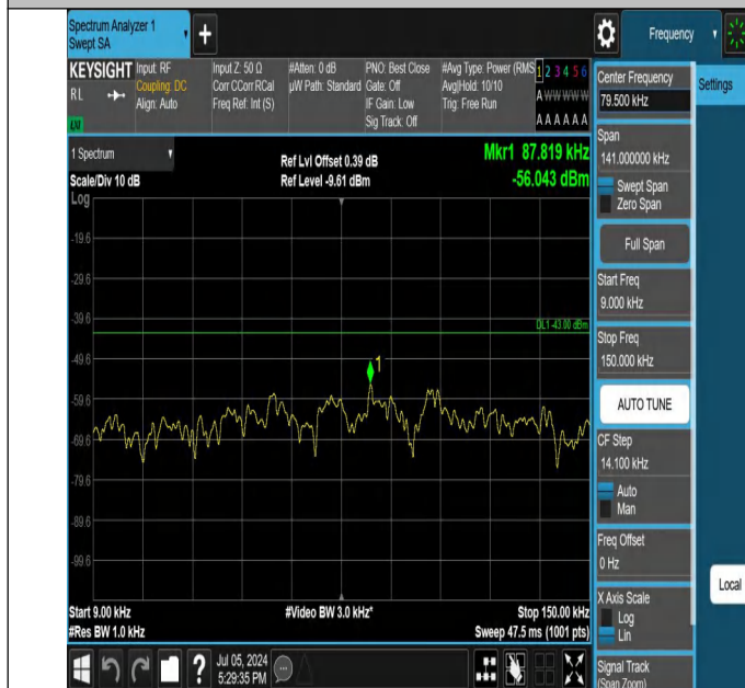
42-42(3450-3550)-5MHz-20MHz-QPSK-QPSK-42590-42707-1RB #0-0RB#0-0.009~0.15MHz-PASS
