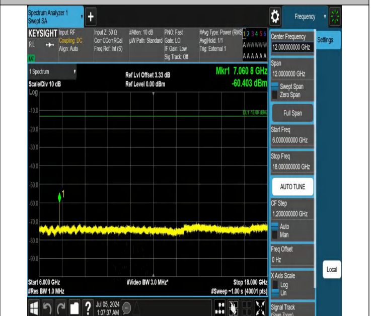
42-42(3450-3550)-5MHz-20MHz-QPSK-QPSK-42873-42990-1RB #24-0RB#0-6000~18000MHz-PASS
