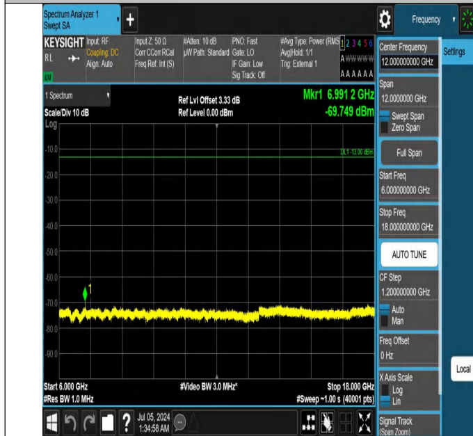
42-42(3450-3550)-10MHz-20MHz-QPSK-QPSK-42590-42734-1R B#0-ORB#0-6000~18000MHz-PASS
