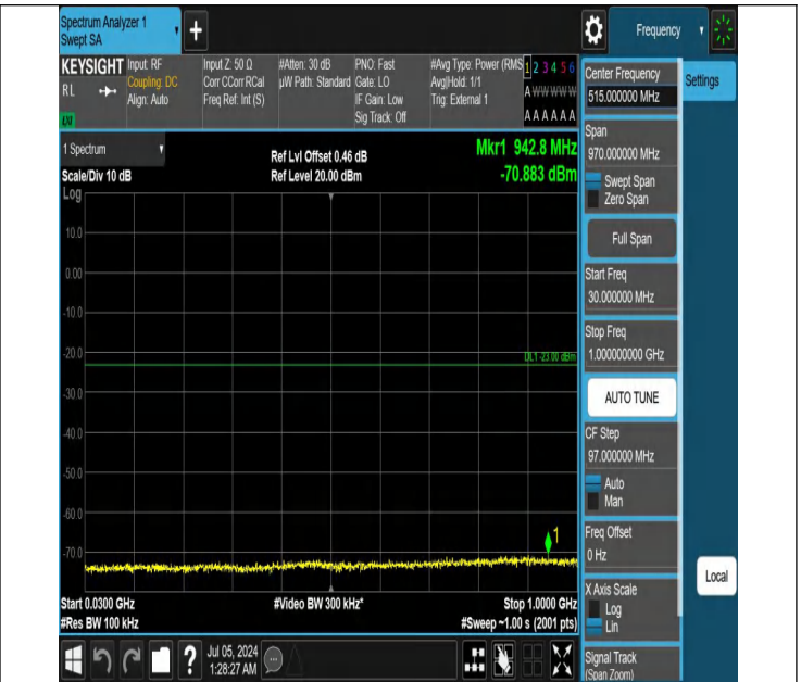
42-42(3450-3550)-10MHz-20MHz-QPSK-QPSK-42140-42284-1R B#49-ORB#0-30~1000MHz-PASS
