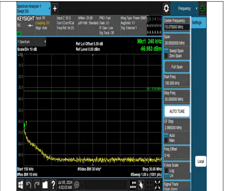
42-42(3450-3550)-20MHz-15MHz-QPSK-QPSK-42844-43015-1R B#0-ORB#0-0.15~30MHz-PASS
