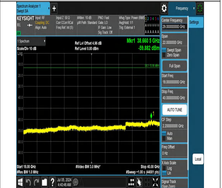
42-42(3450-3550)-20MHz-15MHz-QPSK-QPSK-42190-42361-1R B#99-ORB#0-18000~40000MHz-PASS
