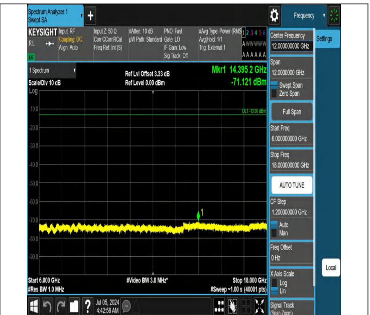
42-42(3450-3550)-20MHz-15MHz-QPSK-QPSK-42190-42361-1R B#0-1RB#74-6000~18000MHz-PASS
