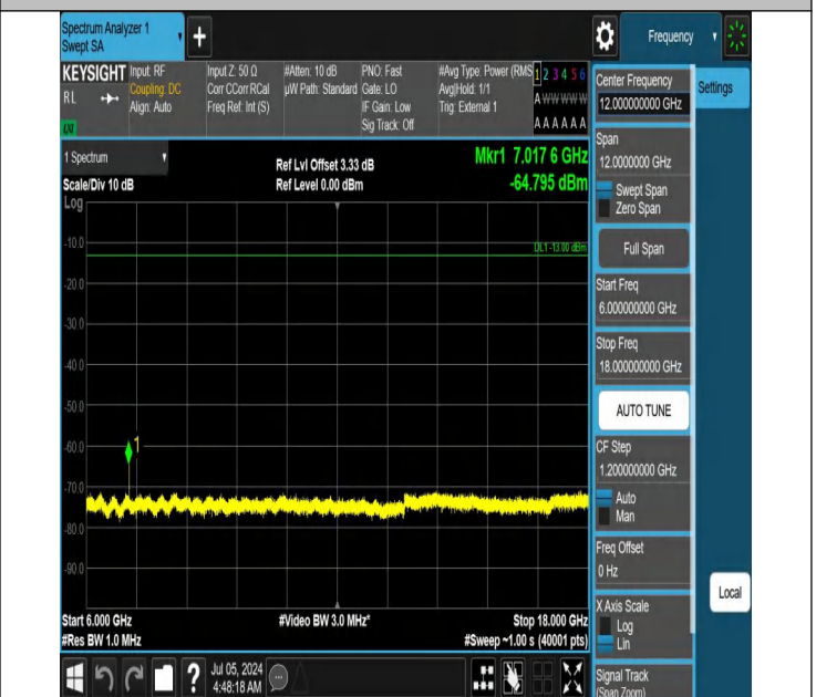
42-42(3450-3550)-20MHz-15MHz-QPSK-QPSK-42590-42761-1R B#99-0RB#0-6000~18000MHz-PASS
