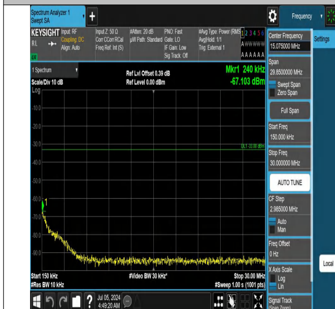
42-42(3450-3550)-20MHz-15MHz-QPSK-QPSK-42590-42761-1R B#0-1RB#74-0.15~30MHz-PASS
