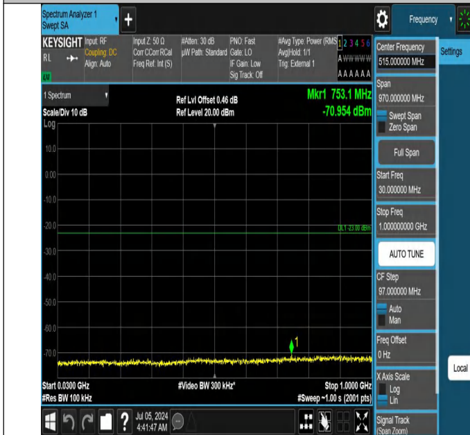
42-42(3450-3550)-20MHz-15MHz-QPSK-QPSK-42190-42361-1R B#0-1RB#74-30~1000MHz-PASS
