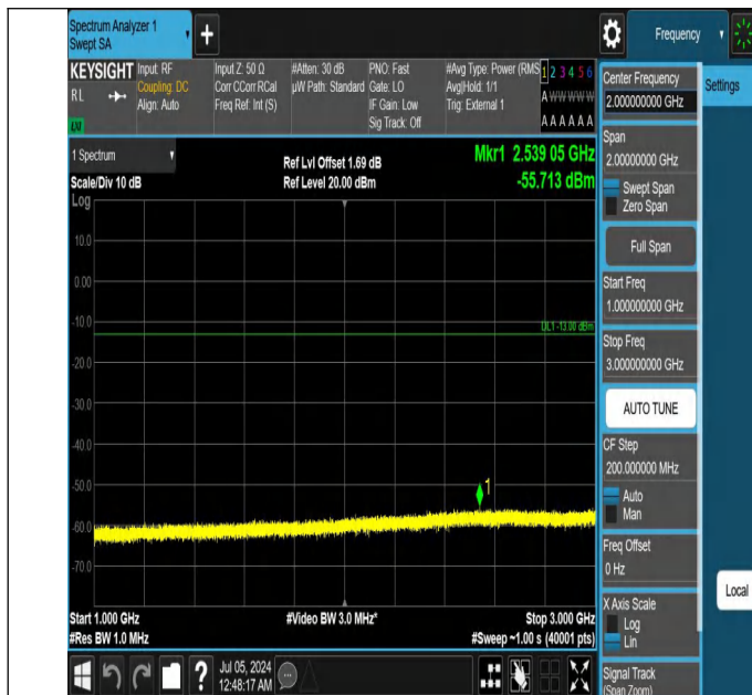
42-42(3450-3550)-5MHz-20MHz-QPSK-QPSK-42115-42232-1RB #0-0RB#0-1000~3000MHz-PASS
