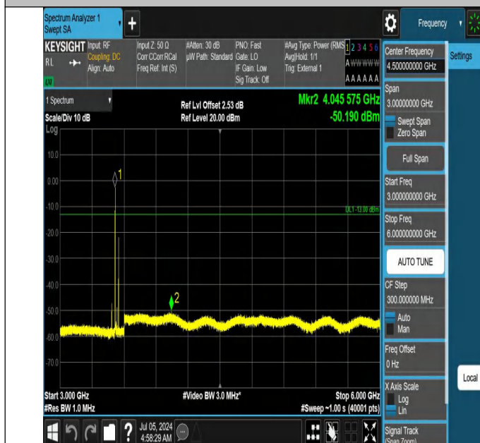
42-42(3450-3550)-20MHz-15MHz-QPSK-QPSK-42844-43015-1R B#0-1RB#74-3000~6000MHz-PASS
