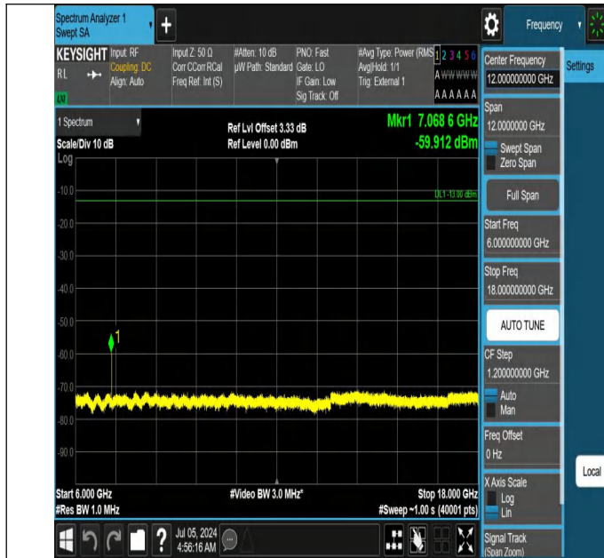
42-42(3450-3550)-20MHz-15MHz-QPSK-QPSK-42844-43015-1R B#99-0RB#0-6000~18000MHz-PASS
