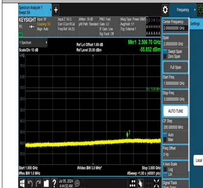
42-42(3450-3550)-20MHz-15MHz-QPSK-QPSK-42590-42761-1R B#0-0RB#0-1000~3000MHz-PASS
