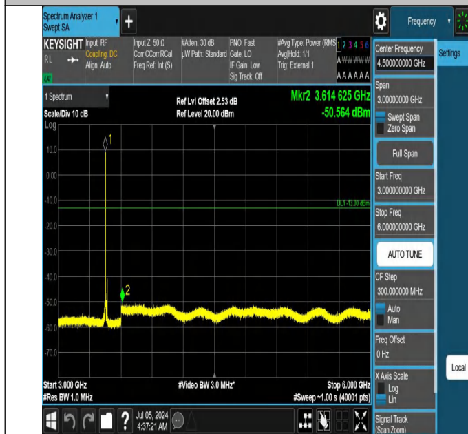
42-42(3450-3550)-20MHz-15MHz-QPSK-QPSK-42190-42361-1R B#0-ORB#0-3000~6000MHz-PASS
