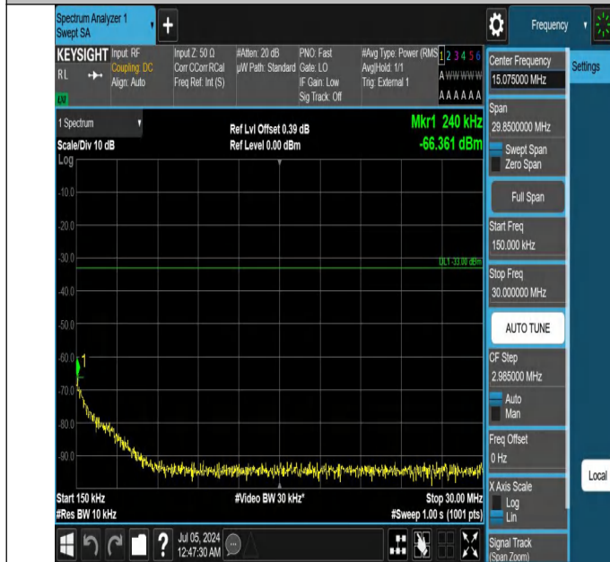
42-42(3450-3550)-5MHz-20MHz-QPSK-QPSK-42115-42232-1RB #0-0RB#0-0.15~30MHz-PASS
