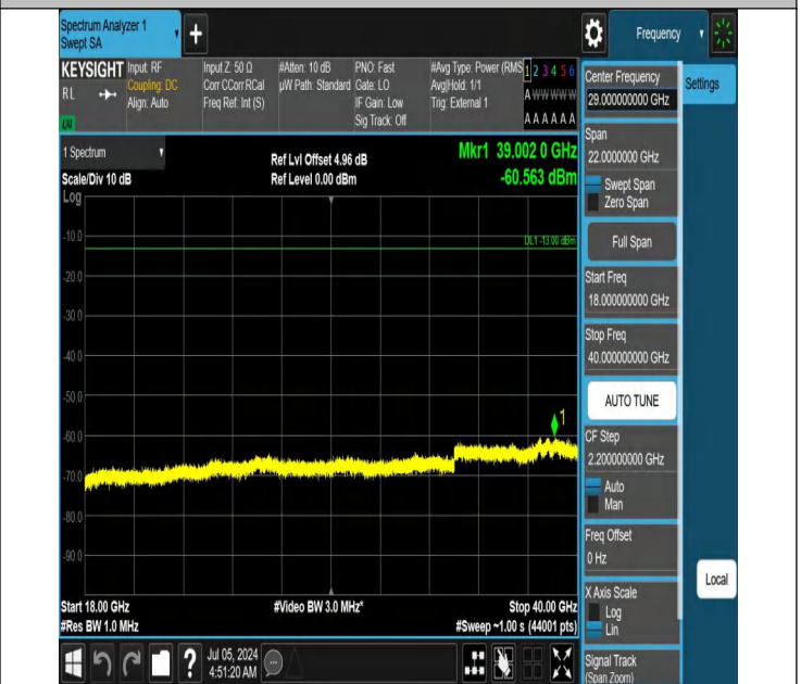
42-42(3450-3550)-20MHz-15MHz-QPSK-QPSK-42590-42761-1R B#0-1RB#74-18000~40000MHz-PASS
