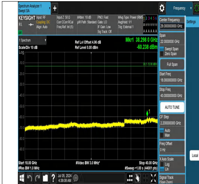
42-42(3450-3550)-20MHz-15MHz-QPSK-QPSK-42190-42361-1R B#0-0RB#0-18000~40000MHz-PASS
