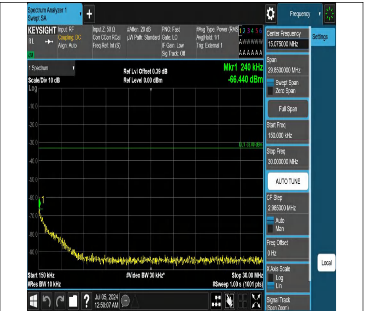
42-42(3450-3550)-5MHz-20MHz-QPSK-QPSK-42115-42232-1RB #24-ORB#0-0.15~30MHz-PASS
