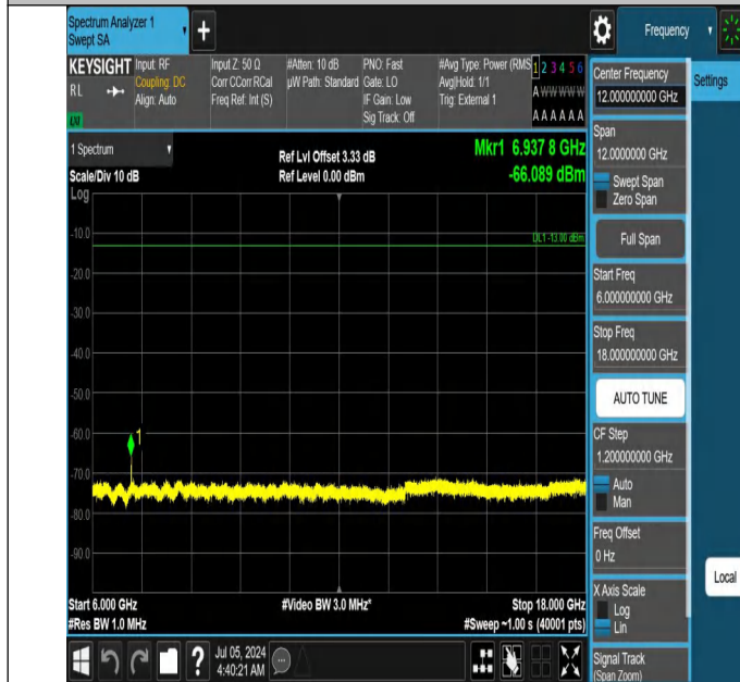
42-42(3450-3550)-20MHz-15MHz-QPSK-QPSK-42190-42361-1R B#99-ORB#0-6000~18000MHz-PASS
