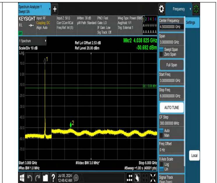
42-42(3450-3550)-5MHz-20MHz-QPSK-QPSK-42115-42232-1RB #0-0RB#0-3000~6000MHz-PASS
