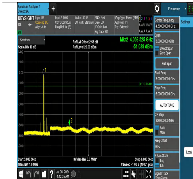
42-42(3450-3550)-20MHz-15MHz-QPSK-QPSK-42190-42361-1R B#0-1RB#74-3000~6000MHz-PASS
