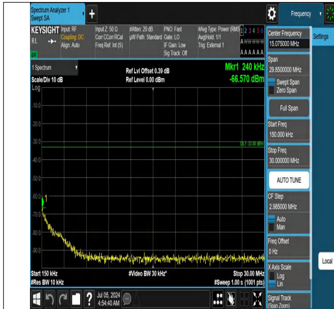
42-42(3450-3550)-20MHz-15MHz-QPSK-QPSK-42844-43015-1R B#99-ORB#0-0.15~30MHz-PASS
