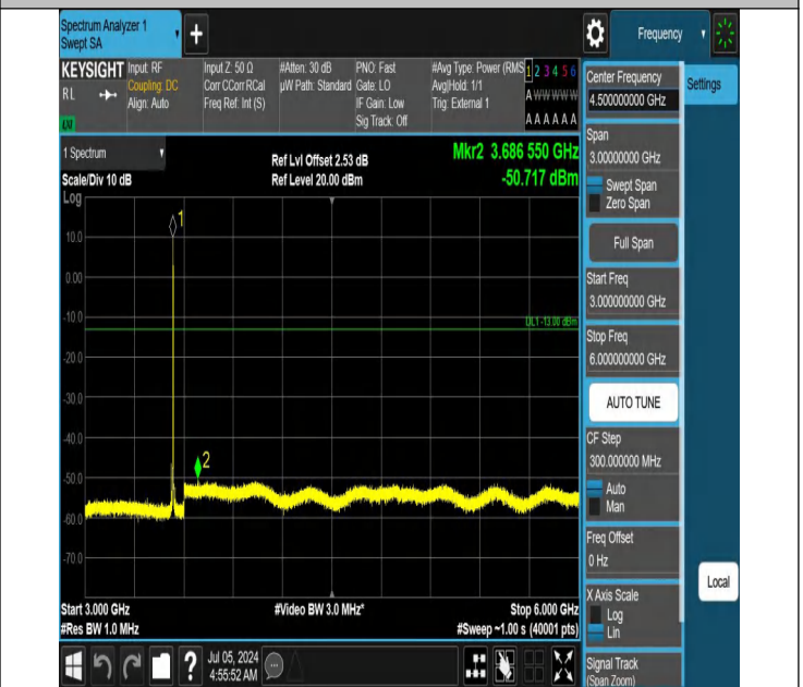
42-42(3450-3550)-20MHz-15MHz-QPSK-QPSK-42844-43015-1R B#99-ORB#0-3000~6000MHz-PASS
