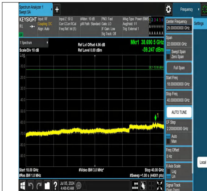
42-42(3450-3550)-20MHz-15MHz-QPSK-QPSK-42590-42761-1R B#99-0RB#0-18000~40000MHz-PASS
