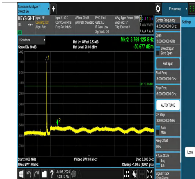
42-42(3450-3550)-20MHz-15MHz-QPSK-QPSK-42844-43015-1R B#0-0RB#0-3000~6000MHz-PASS
