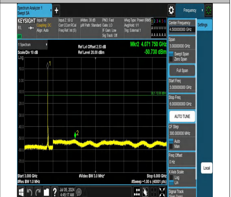
42-42(3450-3550)-20MHz-15MHz-QPSK-QPSK-42590-42761-1R B#0-0RB#0-3000~6000MHz-PASS
