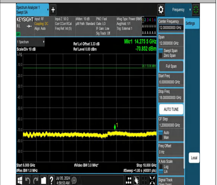
42-42(3450-3550)-20MHz-15MHz-QPSK-QPSK-42844-43015-1R B#0-1RB#74-6000~18000MHz-PASS
