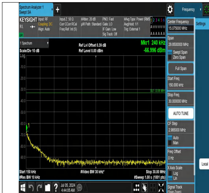
42-42(3450-3550)-20MHz-15MHz-QPSK-QPSK-42590-42761-1R B#0-0RB#0-0.15~30MHz-PASS
