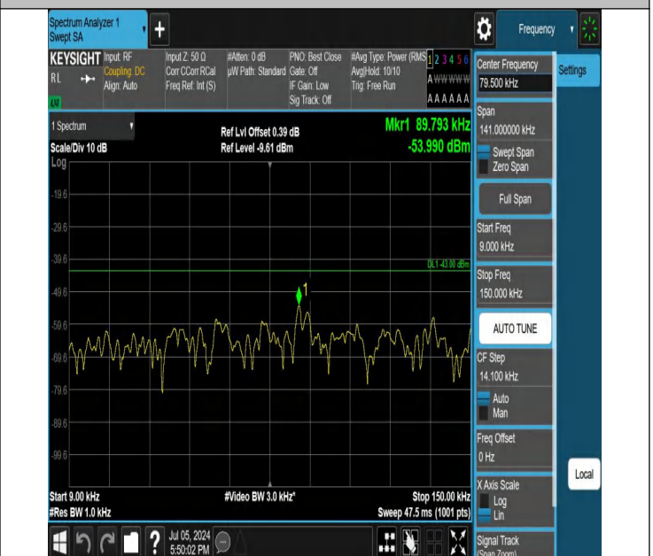
42-42(3450-3550)-20MHz-15MHz-QPSK-QPSK-42590-42761-1R B#0-0RB#0-0.009~0.15MHz-PASS
