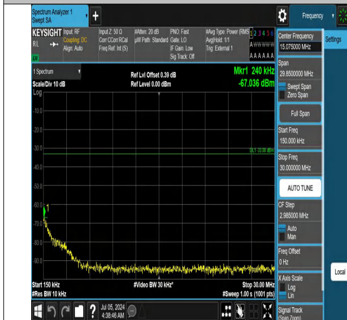
42-42(3450-3550)-20MHz-15MHz-QPSK-QPSK-42190-42361-1R B#99-0RB#0-0.15~30MHz-PASS
