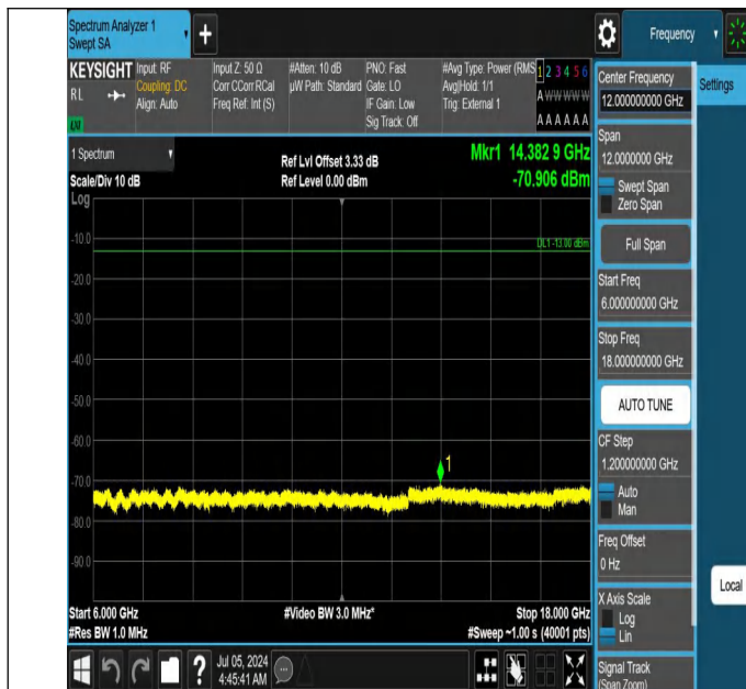
42-42(3450-3550)-20MHz-15MHz-QPSK-QPSK-42590-42761-1R B#0-0RB#0-6000~18000MHz-PASS
