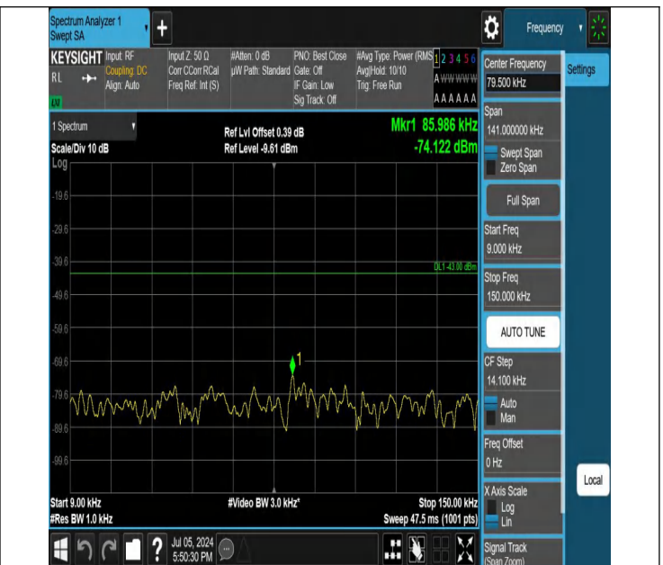
42-42(3450-3550)-20MHz-15MHz-QPSK-QPSK-42590-42761-1R B#0-1RB#74-0.009~0.15MHz-PASS
