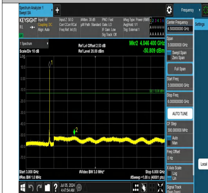
42-42(3450-3550)-20MHz-15MHz-QPSK-QPSK-42590-42761-1R B#99-0RB#0-3000~6000MHz-PASS
