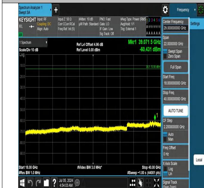
42-42(3450-3550)-20MHz-15MHz-QPSK-QPSK-42844-43015-1R B#0-0RB#0-18000~40000MHz-PASS
