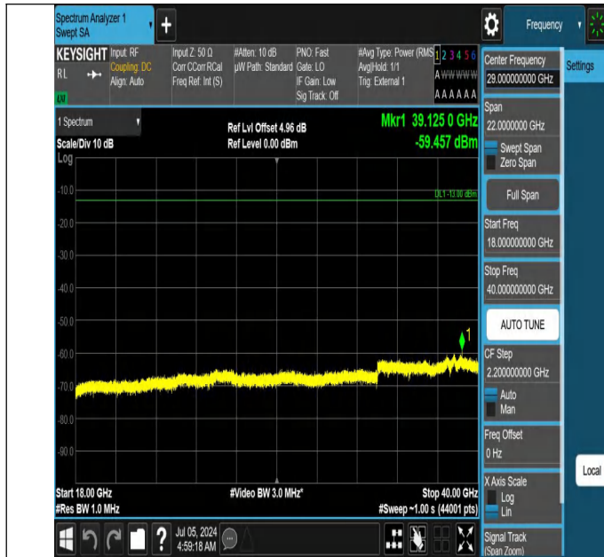
42-42(3450-3550)-20MHz-15MHz-QPSK-QPSK-42844-43015-1R B#0-1RB#74-18000~40000MHz-PASS
