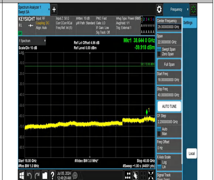
42-42(3450-3550)-5MHz-20MHz-QPSK-QPSK-42115-42232-1RB #0-0RB#0-18000~40000MHz-PASS
