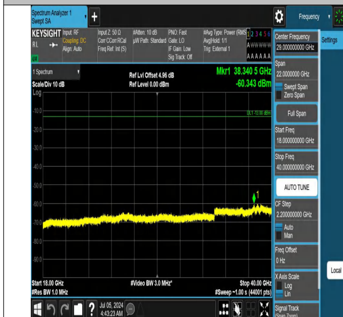
42-42(3450-3550)-20MHz-15MHz-QPSK-QPSK-42190-42361-1R B#0-1RB#74-18000~40000MHz-PASS
