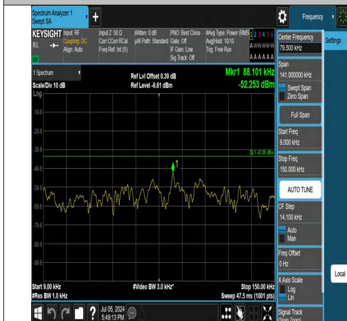
42-42(3450-3550)-20MHz-15MHz-QPSK-QPSK-42190-42361-1R B#0-0RB#0-0.009~0.15MHz-PASS
