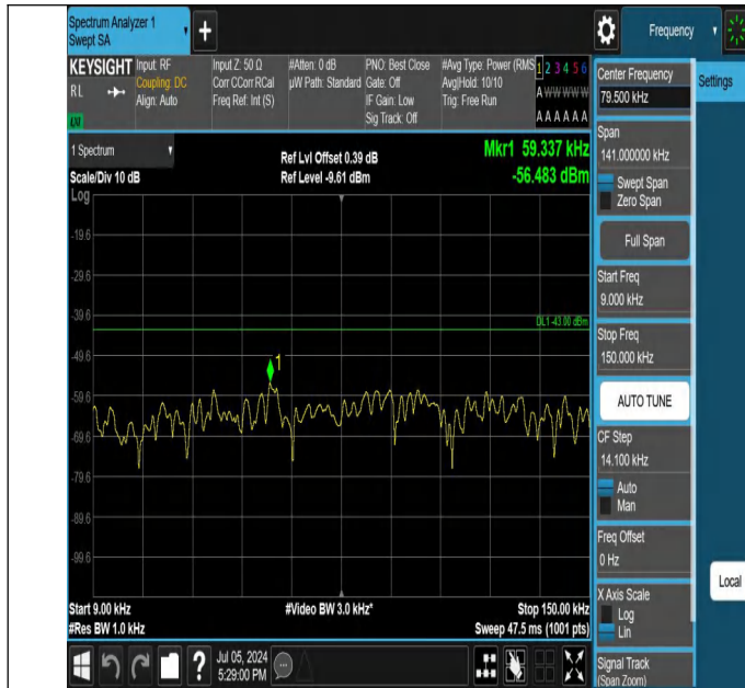
42-42(3450-3550)-5MHz-20MHz-QPSK-QPSK-42115-42232-1RB #24-ORB#0-0.009~0.15MHz-PASS
