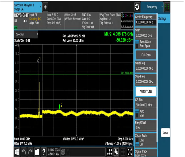
42-42(3450-3550)-20MHz-15MHz-QPSK-QPSK-42590-42761-1R B#0-1RB#74-3000~6000MHz-PASS
