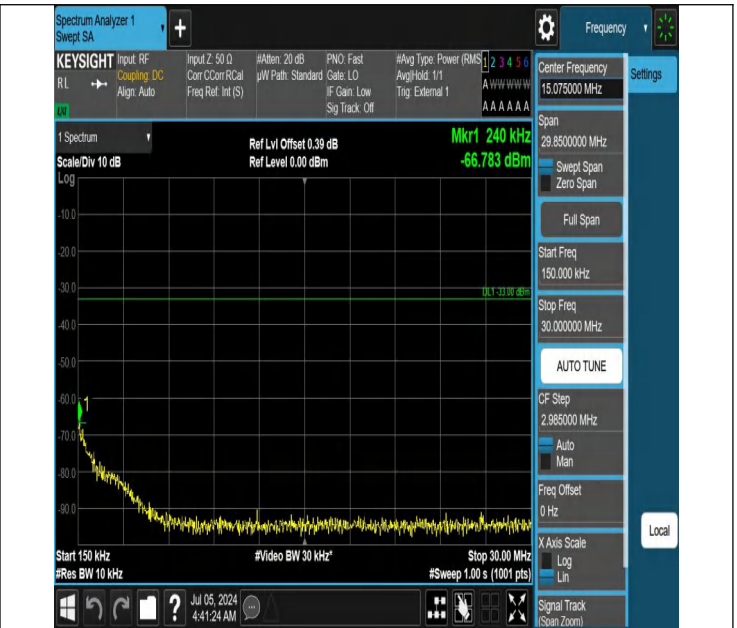
42-42(3450-3550)-20MHz-15MHz-QPSK-QPSK-42190-42361-1R B#0-1RB#74-0.15~30MHz-PASS
