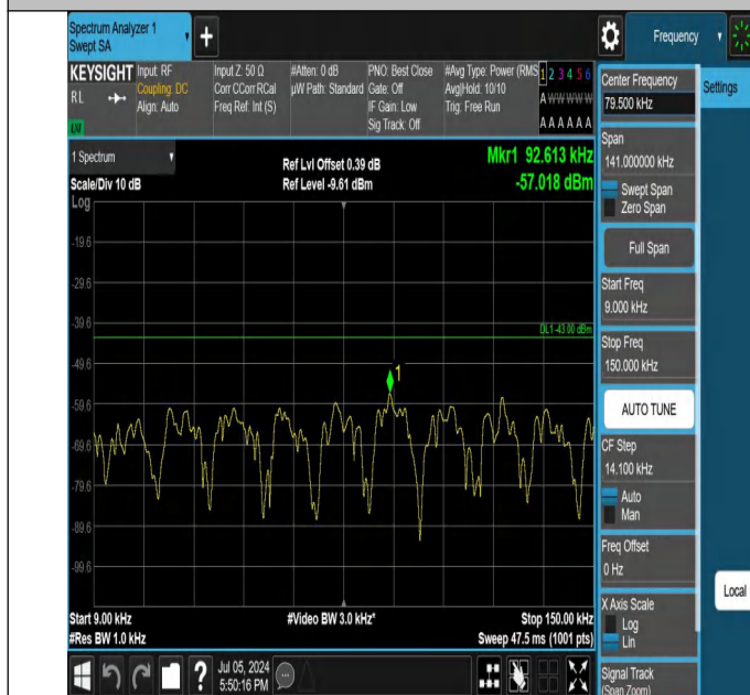
42-42(3450-3550)-20MHz-15MHz-QPSK-QPSK-42590-42761-1R B#99-0RB#0-0.009~0.15MHz-PASS
