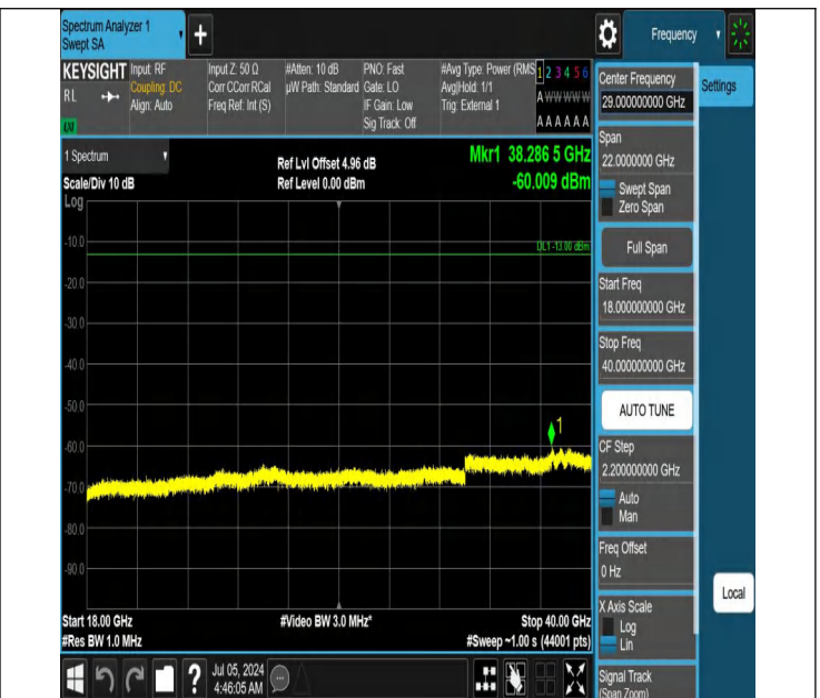
42-42(3450-3550)-20MHz-15MHz-QPSK-QPSK-42590-42761-1R B#0-0RB#0-18000~40000MHz-PASS
