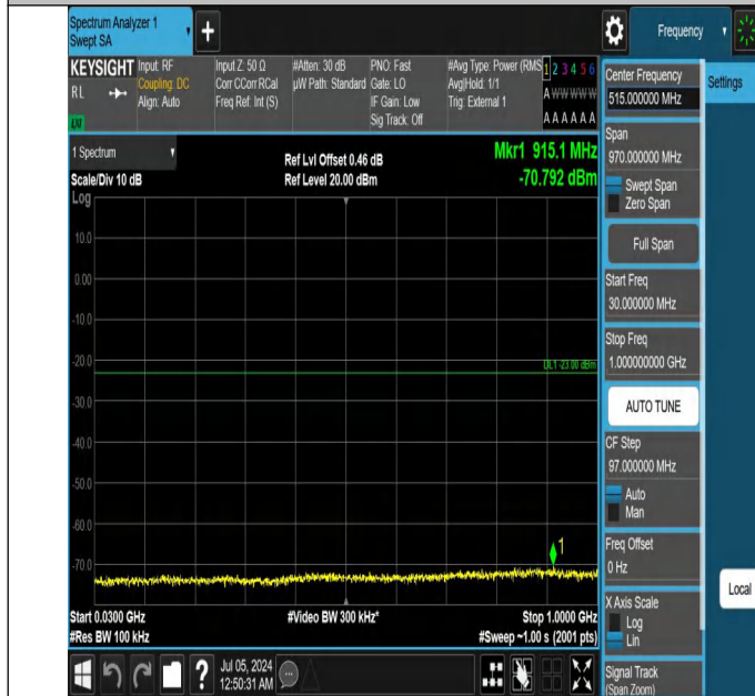
42-42(3450-3550)-5MHz-20MHz-QPSK-QPSK-42115-42232-1RB #24-ORB#0-30~1000MHz-PASS
