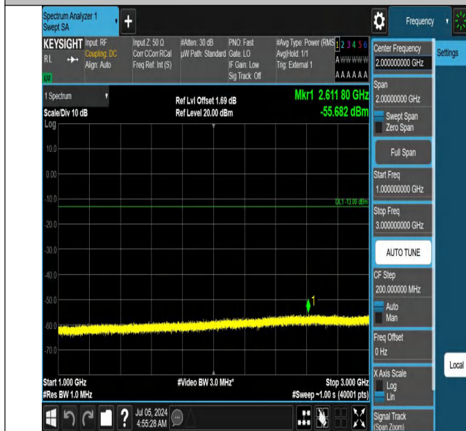
42-42(3450-3550)-20MHz-15MHz-QPSK-QPSK-42844-43015-1R B#99-ORB#0-1000~3000MHz-PASS
