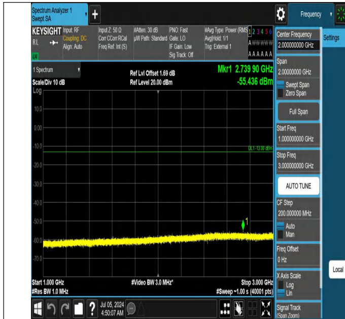
42-42(3450-3550)-20MHz-15MHz-QPSK-QPSK-42590-42761-1R B#0-1RB#74-1000~3000MHz-PASS
