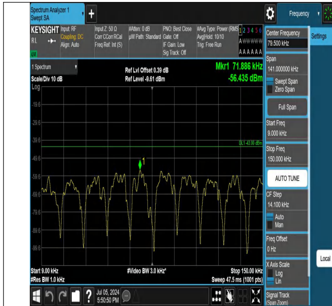
42-42(3450-3550)-20MHz-15MHz-QPSK-QPSK-42844-43015-1R B#0-ORB#0-0.009~0.15MHz-PASS
