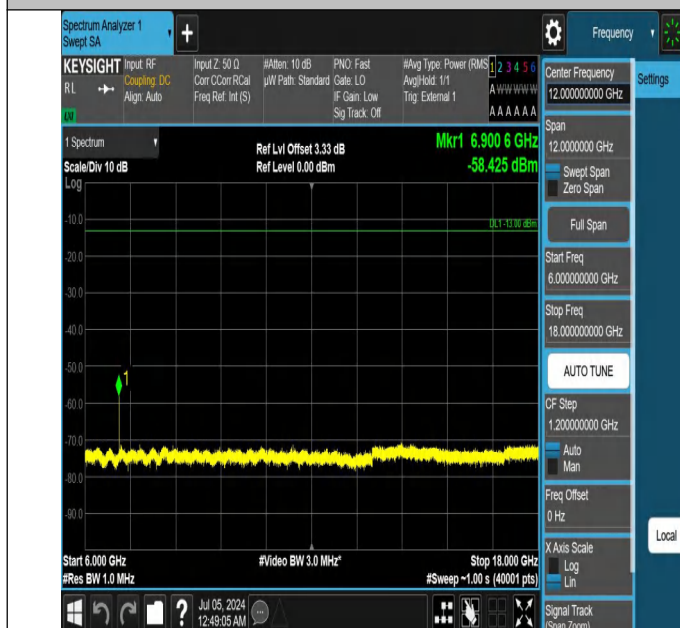
42-42(3450-3550)-5MHz-20MHz-QPSK-QPSK-42115-42232-1RB #0-0RB#0-6000~18000MHz-PASS
