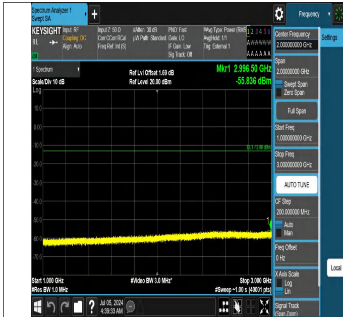
42-42(3450-3550)-20MHz-15MHz-QPSK-QPSK-42190-42361-1R B#99-ORB#0-1000~3000MHz-PASS
