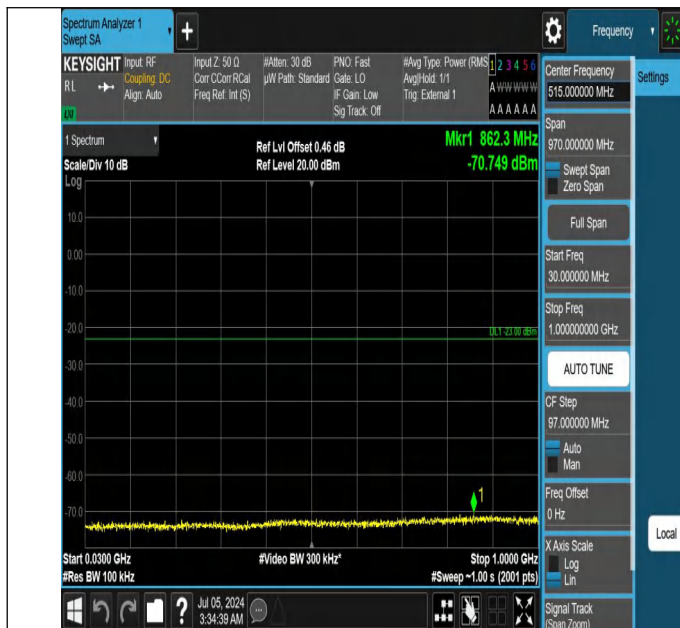
42-42(3450-3550)-20MHz-5MHz-QPSK-QPSK-42948-43065-1RB #0-0RB#0-30~1000MHz-PASS
