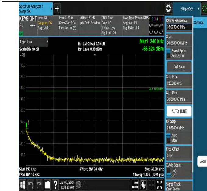
42-42(3450-3550)-20MHz-10MHz-QPSK-QPSK-42590-42734-1R B#99-ORB#0-0.15~30MHz-PASS
