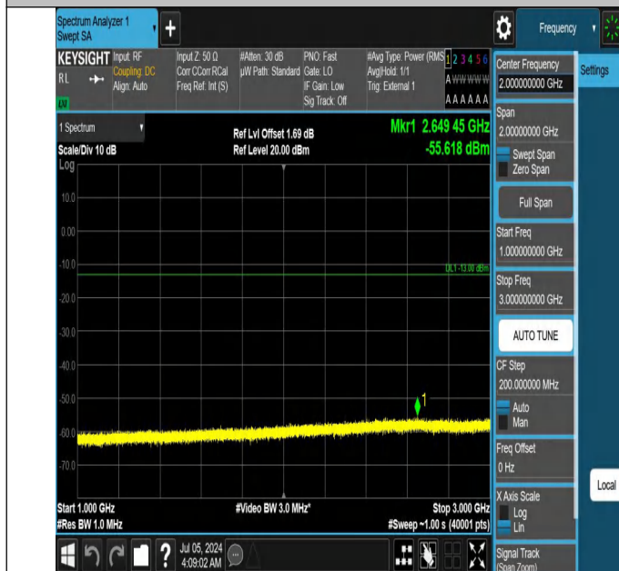
42-42(3450-3550)-20MHz-10MHz-QPSK-QPSK-42590-42734-1R B#99-ORB#0-1000~3000MHz-PASS
