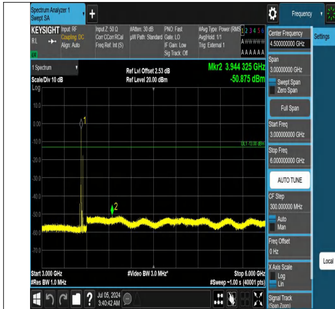
42-42(3450-3550)-20MHz-5MHz-QPSK-QPSK-42948-43065-1RB #0-1RB#24-3000~6000MHz-PASS
