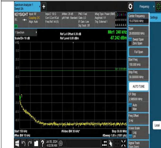
42-42(3450-3550)-20MHz-10MHz-QPSK-QPSK-42190-42334-1R B#0-1RB#49-0.15~30MHz-PASS
