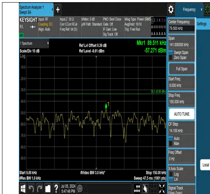
42-42(3450-3550)-20MHz-10MHz-QPSK-QPSK-42896-43040-1R B#99-0RB#0-0.009~0.15MHz-PASS
