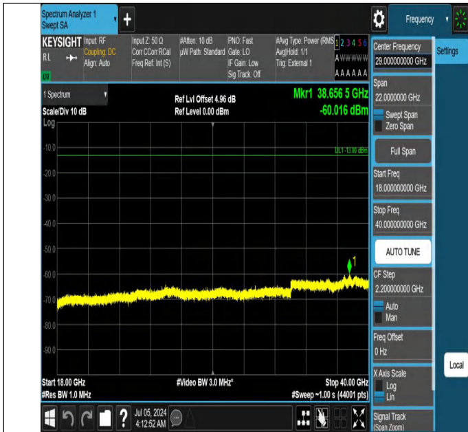
42-42(3450-3550)-20MHz-10MHz-QPSK-QPSK-42590-42734-1R B#0-1RB#49-18000~40000MHz-PASS
