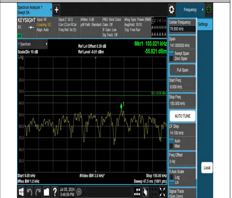
42-42(3450-3550)-20MHz-10MHz-QPSK-QPSK-42590-42734-1R B#99-ORB#0-0.009~0.15MHz-PASS
