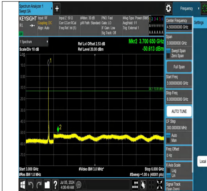
42-42(3450-3550)-20MHz-10MHz-QPSK-QPSK-42590-42734-1R B#0-ORB#0-3000~6000MHz-PASS
