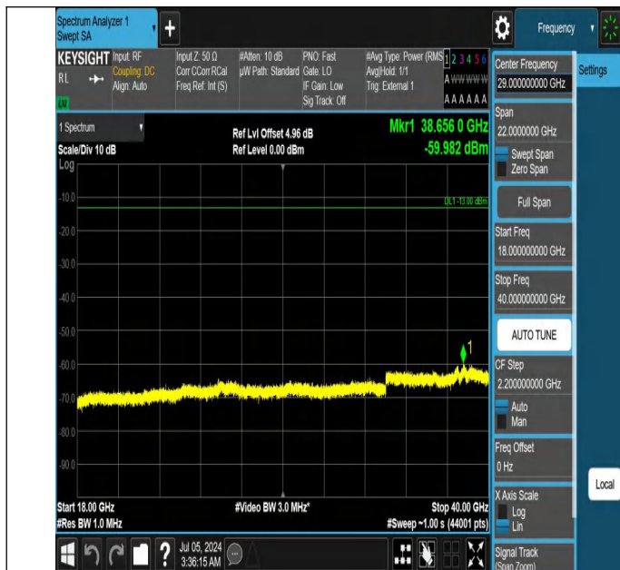
42-42(3450-3550)-20MHz-5MHz-QPSK-QPSK-42948-43065-1RB #0-0RB#0-18000~40000MHz-PASS
