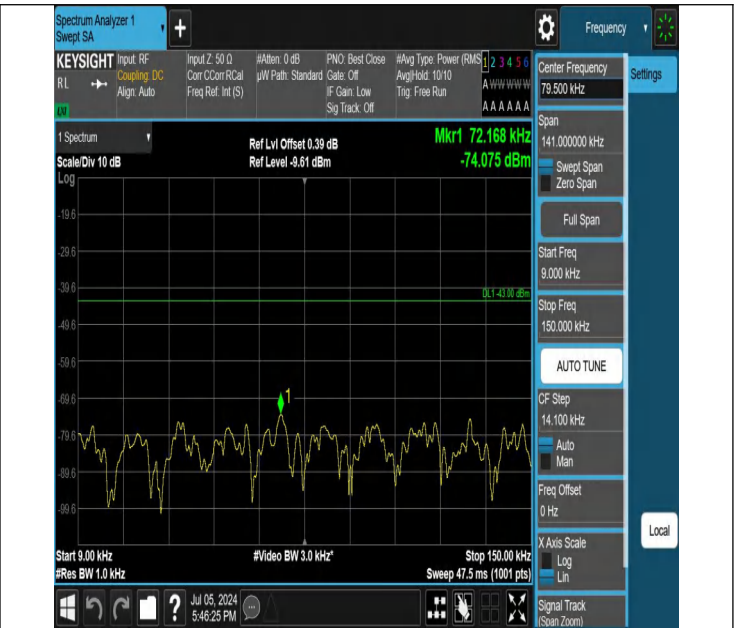
42-42(3450-3550)-20MHz-10MHz-QPSK-QPSK-42190-42334-1R B#0-1RB#49-0.009~0.15MHz-PASS
