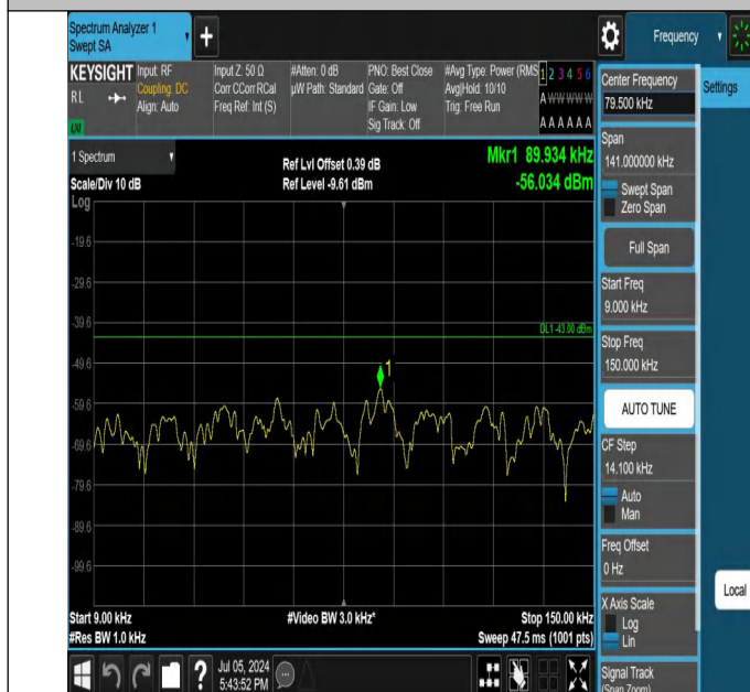
42-42(3450-3550)-20MHz-5MHz-QPSK-QPSK-42948-43065-1RB #0-0RB#0-0.009~0.15MHz-PASS
