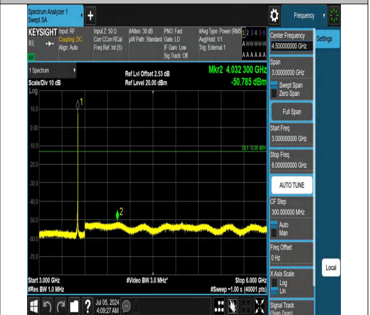
42-42(3450-3550)-20MHz-10MHz-QPSK-QPSK-42590-42734-1R B#99-ORB#0-3000~6000MHz-PASS
