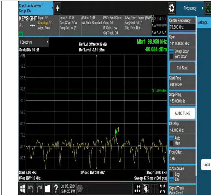
42-42(3450-3550)-20MHz-5MHz-QPSK-QPSK-42948-43065-1RB #0-1RB#24-0.009~0.15MHz-PASS
