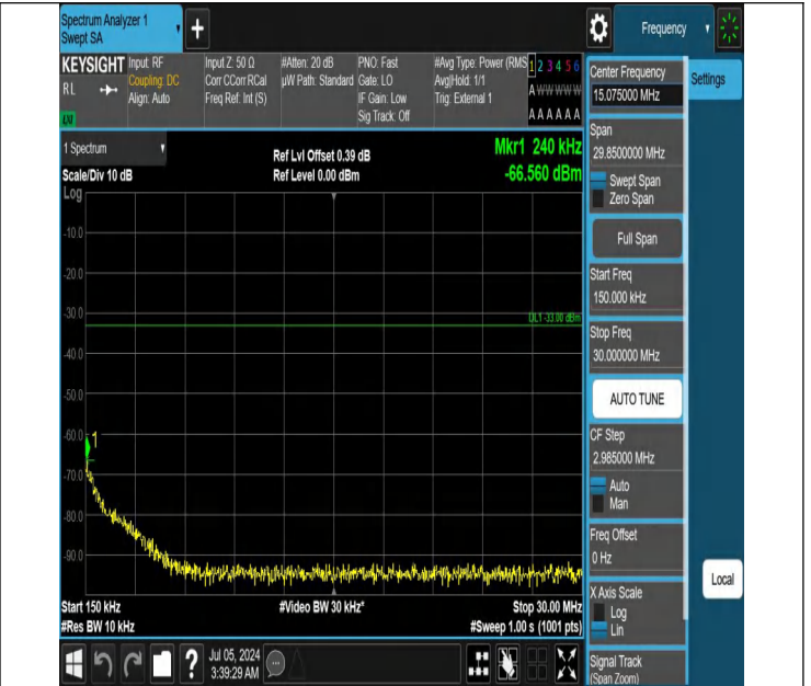
42-42(3450-3550)-20MHz-5MHz-QPSK-QPSK-42948-43065-1RB #0-1RB#24-0.15~30MHz-PASS
