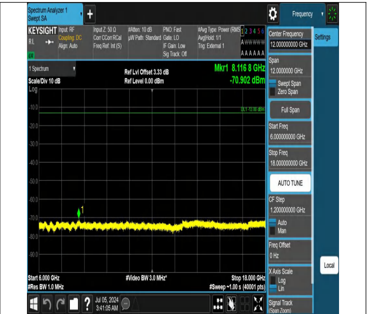
42-42(3450-3550)-20MHz-5MHz-QPSK-QPSK-42948-43065-1RB #0-1RB#24-6000~18000MHz-PASS
