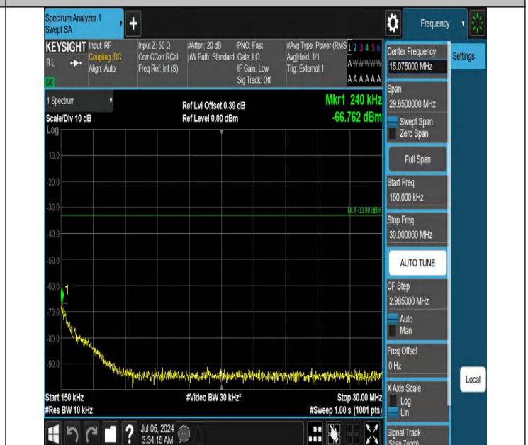
42-42(3450-3550)-20MHz-5MHz-QPSK-QPSK-42948-43065-1RB #0-0RB#0-0.15~30MHz-PASS
