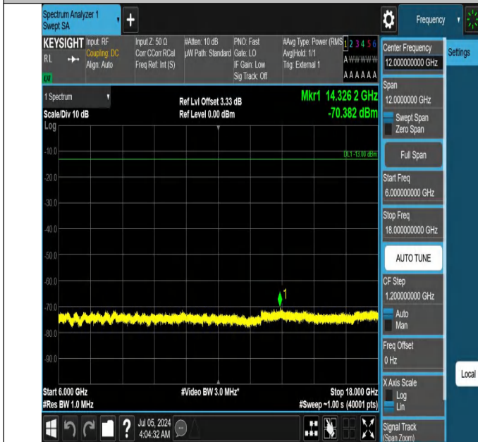
42-42(3450-3550)-20MHz-10MHz-QPSK-QPSK-42190-42334-1R B#0-1RB#49-6000~18000MHz-PASS
