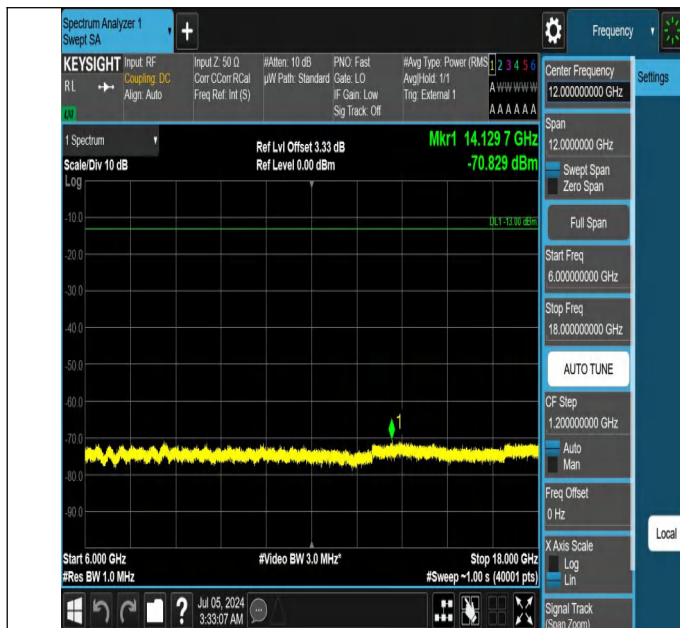
42-42(3450-3550)-20MHz-5MHz-QPSK-QPSK-42590-42707-1RB #0-1RB#24-6000~18000MHz-PASS
