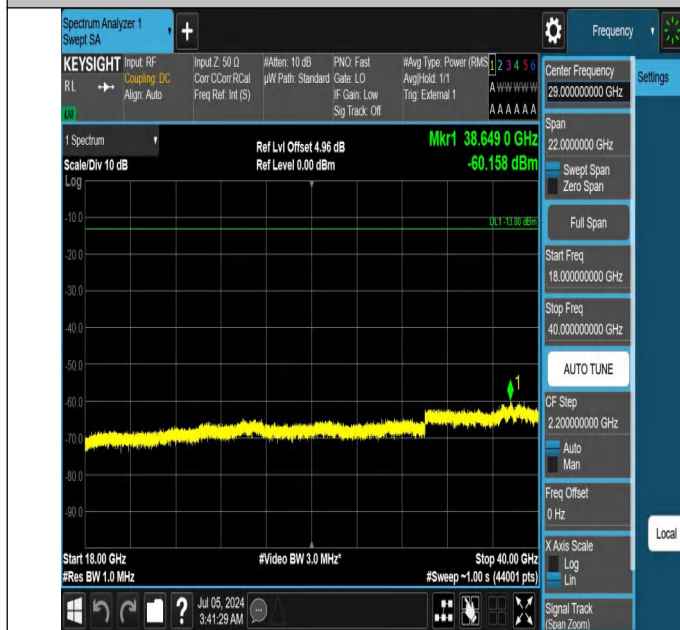
42-42(3450-3550)-20MHz-5MHz-QPSK-QPSK-42948-43065-1RB #0-1RB#24-18000~40000MHz-PASS
