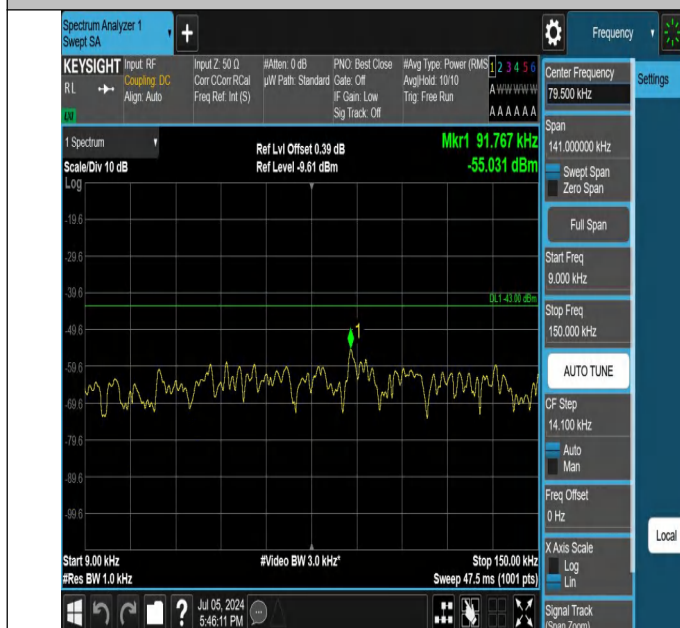
42-42(3450-3550)-20MHz-10MHz-QPSK-QPSK-42190-42334-1R B#99-0RB#0-0.009~0.15MHz-PASS
