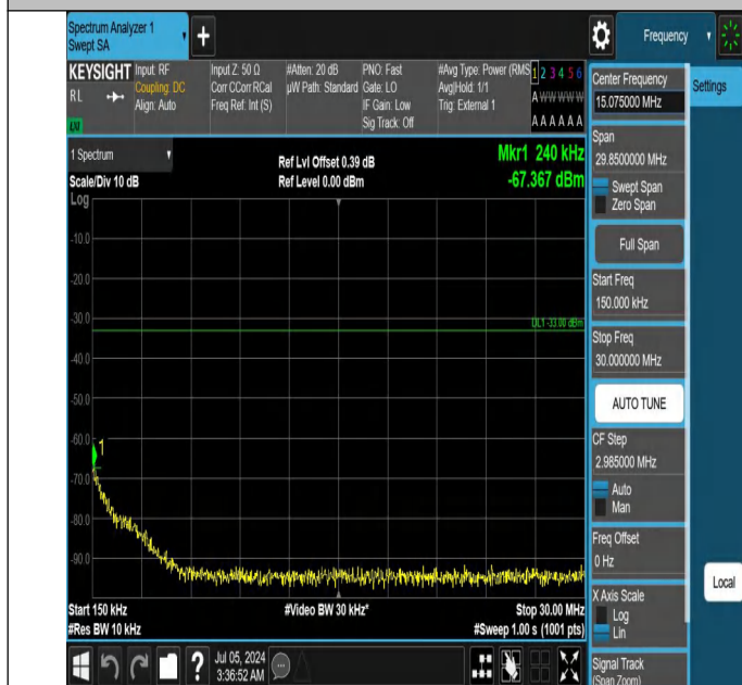
42-42(3450-3550)-20MHz-5MHz-QPSK-QPSK-42948-43065-1RB #99-0RB#0-0.15~30MHz-PASS
