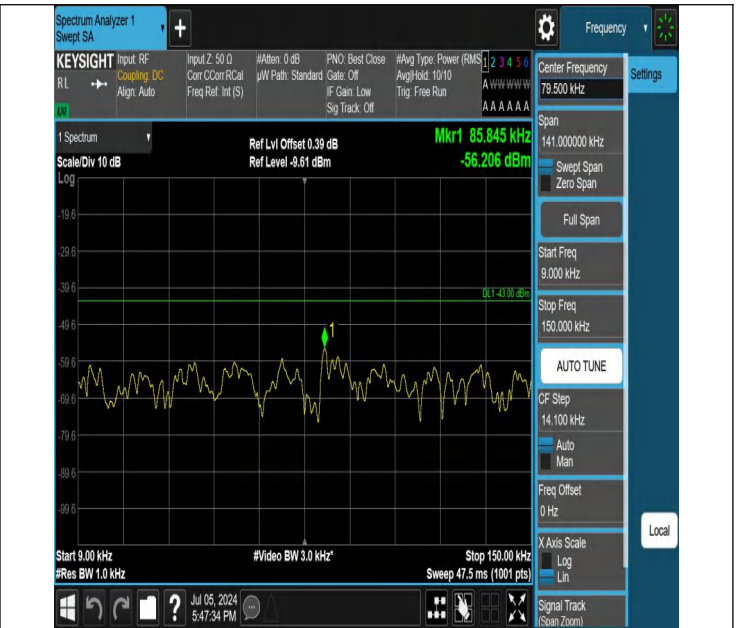
42-42(3450-3550)-20MHz-10MHz-QPSK-QPSK-42896-43040-1R B#0-0RB#0-0.009~0.15MHz-PASS
