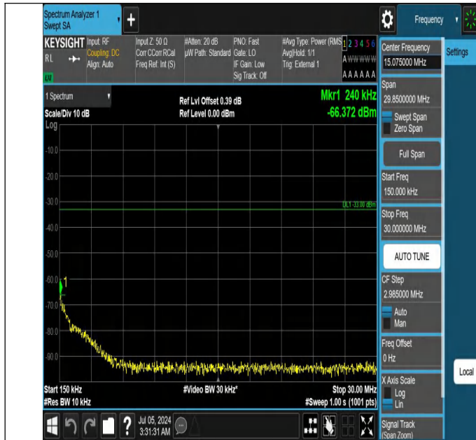
42-42(3450-3550)-20MHz-5MHz-QPSK-QPSK-42590-42707-1RB #0-1RB#24-0.15~30MHz-PASS
