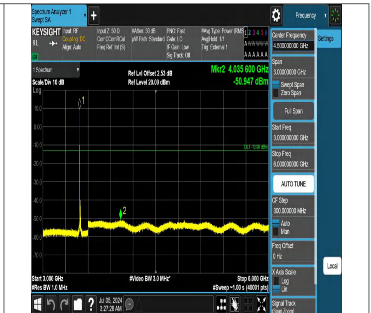
42-42(3450-3550)-20MHz-5MHz-QPSK-QPSK-42590-42707-1RB #0-0RB#0-3000~6000MHz-PASS
