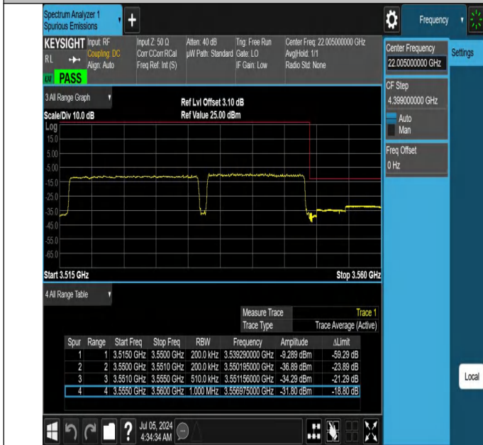
42-42(3450-3550)-20MHz-15MHz-QPSK@QPSK-QPSK@QPSK-42844-43015-100RB#0@100RB#0-75RB#0@75RB#0-PASS
