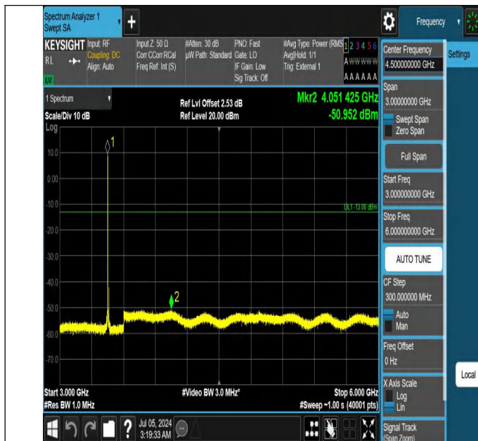
42-42(3450-3550)-20MHz-5MHz-QPSK-QPSK-42190-42307-1RB #0-0RB#0-3000~6000MHz-PASS
