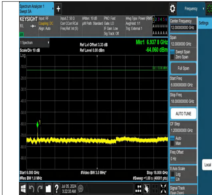
42-42(3450-3550)-20MHz-5MHz-QPSK-QPSK-42190-42307-1RB #99-0RB#0-6000~18000MHz-PASS
