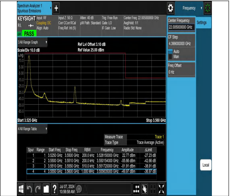
42-42(3450-3550)-5MHz-20MHz-QPSK@QPSK-QPSK@QPSK-4 2873-42990-1RB#0@25RB#0-0RB#0@100RB#0-PASS
