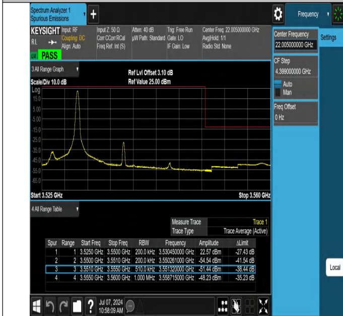
42-42(3450-3550)-5MHz-20MHz-QPSK@QPSK-QPSK@QPSK-4 2873-42990-1RB#24@25RB#0-0RB#0@100RB#0-PASS
