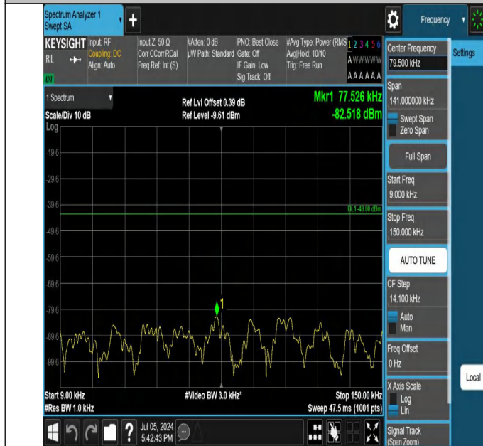
42-42(3450-3550)-20MHz-5MHz-QPSK-QPSK-42190-42307-1RB #0-1RB#24-0.009~0.15MHz-PASS
