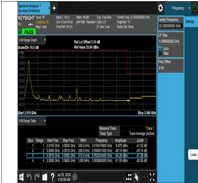
42-42(3450-3550)-20MHz-15MHz-QPSK@QPSK-QPSK@QPSK-42844-43015-1RB#0@100RB#0-0RB#0@75RB#0-PASS
