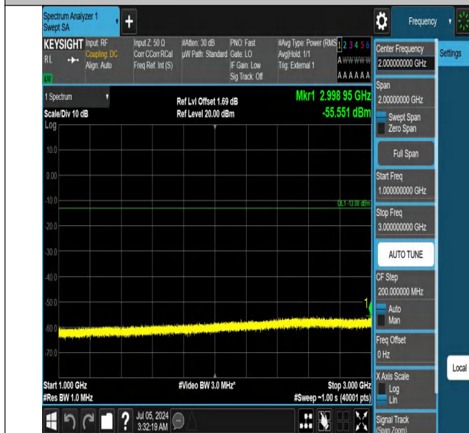
42-42(3450-3550)-20MHz-5MHz-QPSK-QPSK-42590-42707-1RB #0-1RB#24-1000~3000MHz-PASS
