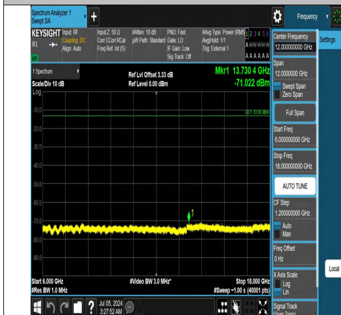
42-42(3450-3550)-20MHz-5MHz-QPSK-QPSK-42590-42707-1RB #0-0RB#0-6000~18000MHz-PASS
