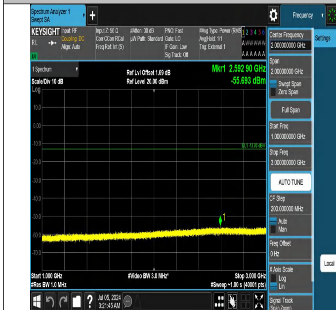
42-42(3450-3550)-20MHz-5MHz-QPSK-QPSK-42190-42307-1RB #99-ORB#0-1000~3000MHz-PASS
