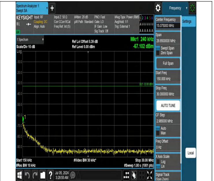
42-42(3450-3550)-20MHz-5MHz-QPSK-QPSK-42590-42707-1RB #99-ORB#0-0.15~30MHz-PASS
