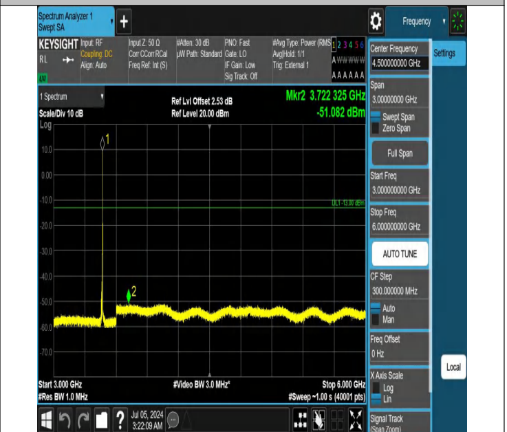
42-42(3450-3550)-20MHz-5MHz-QPSK-QPSK-42190-42307-1RB #99-ORB#0-3000~6000MHz-PASS
