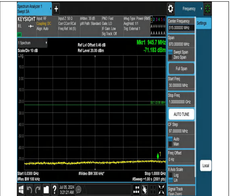
42-42(3450-3550)-20MHz-5MHz-QPSK-QPSK-42190-42307-1RB #99-ORB#0-30~1000MHz-PASS
