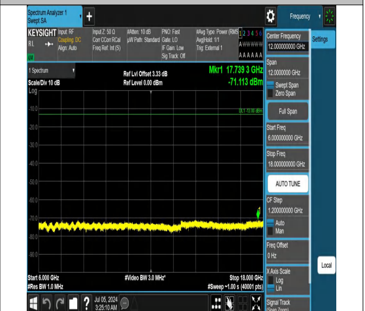
42-42(3450-3550)-20MHz-5MHz-QPSK-QPSK-42190-42307-1RB #0-1RB#24-6000~18000MHz-PASS
