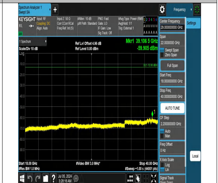
42-42(3450-3550)-20MHz-5MHz-QPSK-QPSK-42590-42707-1RB #0-0RB#0-18000~40000MHz-PASS
