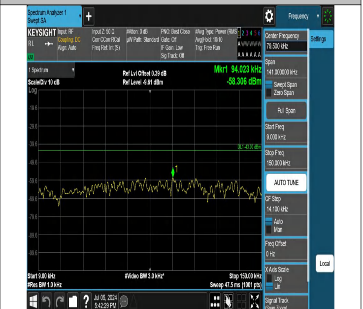
42-42(3450-3550)-20MHz-5MHz-QPSK-QPSK-42190-42307-1RB #99-0RB#0-0.009~0.15MHz-PASS
