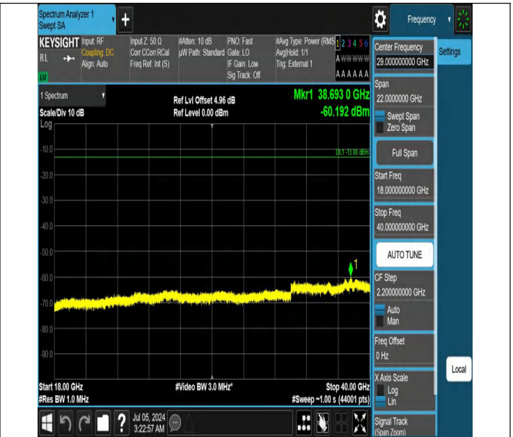
42-42(3450-3550)-20MHz-5MHz-QPSK-QPSK-42190-42307-1RB #99-0RB#0-18000~40000MHz-PASS
