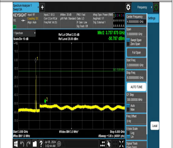
42-42(3450-3550)-20MHz-5MHz-QPSK-QPSK-42590-42707-1RB #0-1RB#24-3000~6000MHz-PASS
