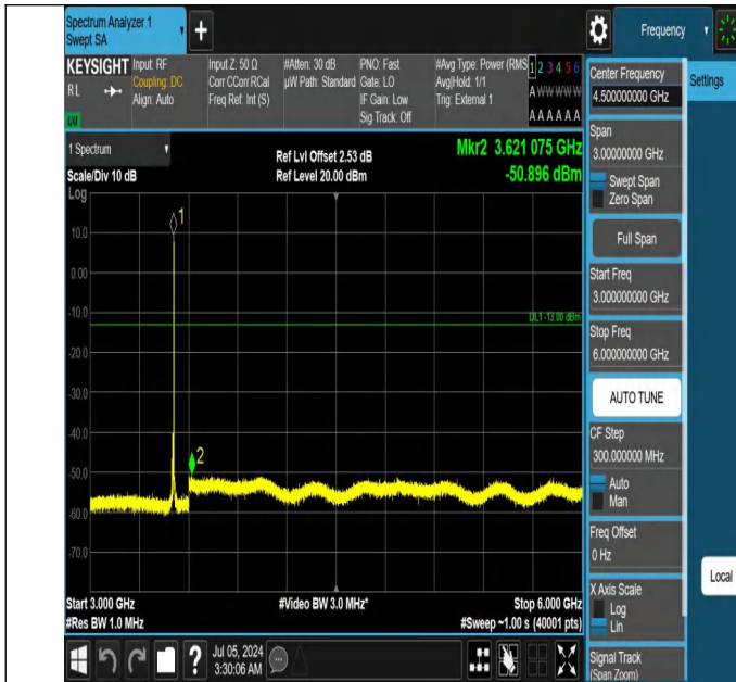
42-42(3450-3550)-20MHz-5MHz-QPSK-QPSK-42590-42707-1RB #99-ORB#0-3000~6000MHz-PASS
