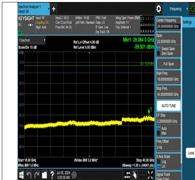
42-42(3450-3550)-20MHz-5MHz-QPSK-QPSK-42190-42307-1RB #0-1RB#24-18000~40000MHz-PASS
