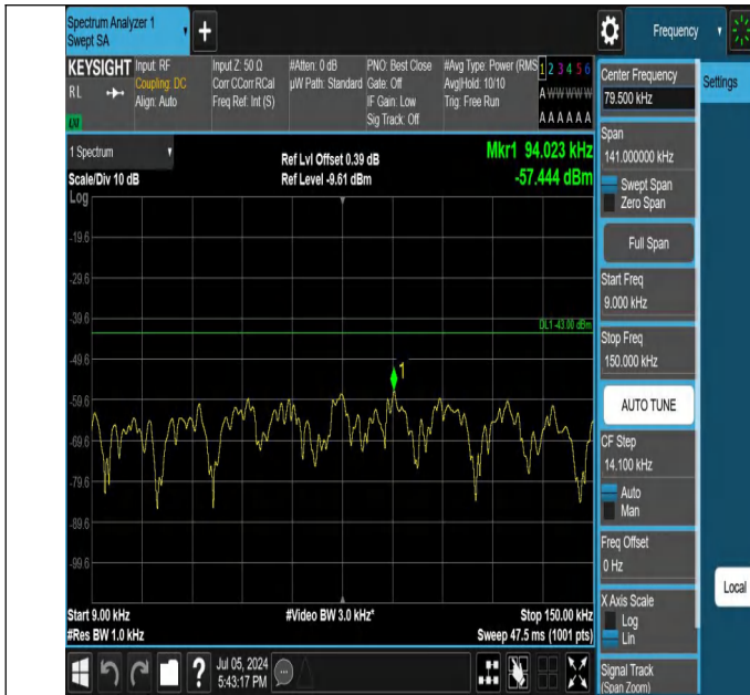
42-42(3450-3550)-20MHz-5MHz-QPSK-QPSK-42590-42707-1RB #99-ORB#0-0.009~0.15MHz-PASS
