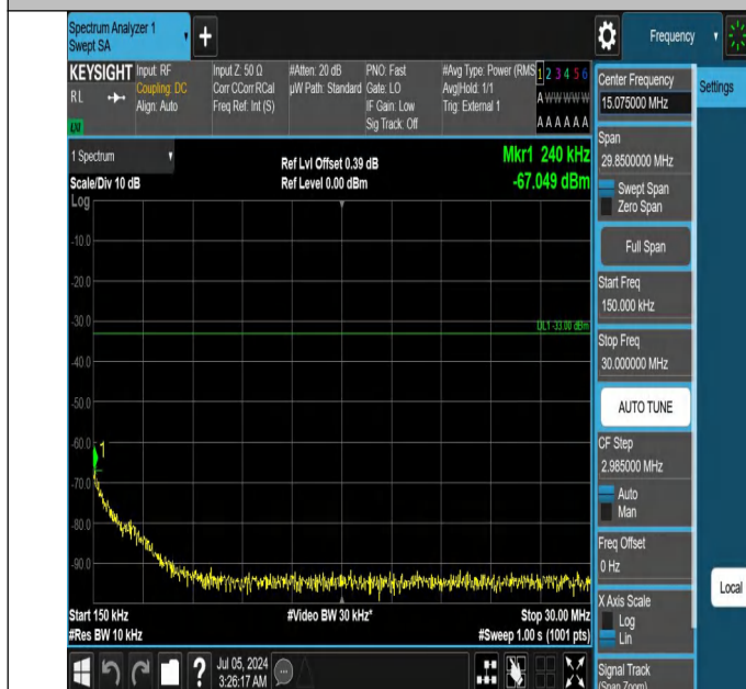
42-42(3450-3550)-20MHz-5MHz-QPSK-QPSK-42590-42707-1RB #0-0RB#0-0.15~30MHz-PASS
