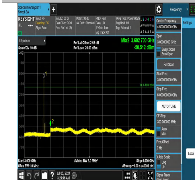
42-42(3450-3550)-20MHz-5MHz-QPSK-QPSK-42190-42307-1RB #0-1RB#24-3000~6000MHz-PASS
