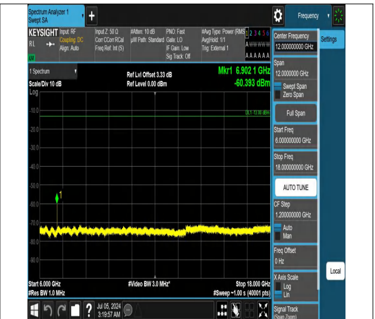
42-42(3450-3550)-20MHz-5MHz-QPSK-QPSK-42190-42307-1RB #0-0RB#0-6000~18000MHz-PASS
