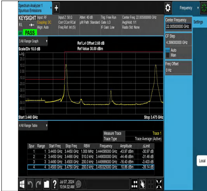
42-42(3450-3550)-5MHz-20MHz-QPSK@QPSK-QPSK@QPSK-4 2115-42232-1RB#0@25RB#0-1RB#99@100RB#0-PASS
