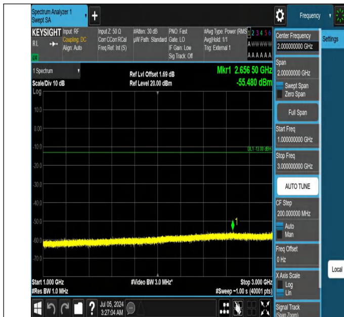
42-42(3450-3550)-20MHz-5MHz-QPSK-QPSK-42590-42707-1RB #0-0RB#0-1000~3000MHz-PASS
