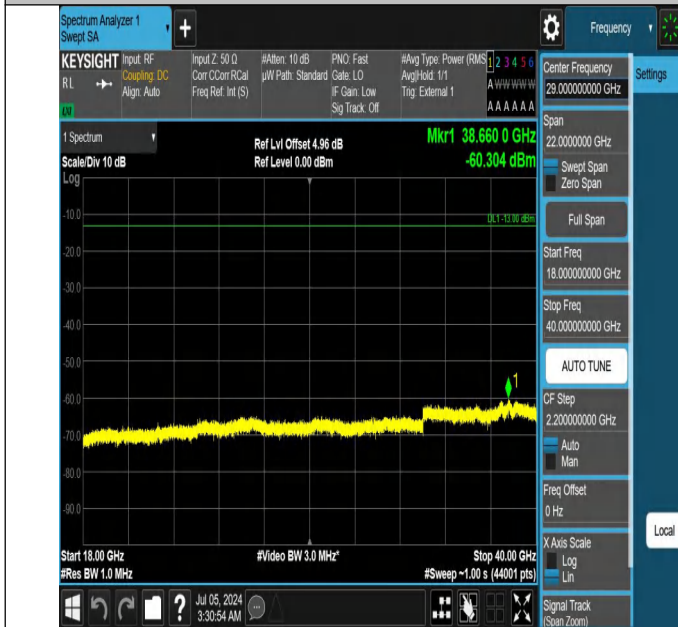
42-42(3450-3550)-20MHz-5MHz-QPSK-QPSK-42590-42707-1RB #99-ORB#0-18000~40000MHz-PASS
