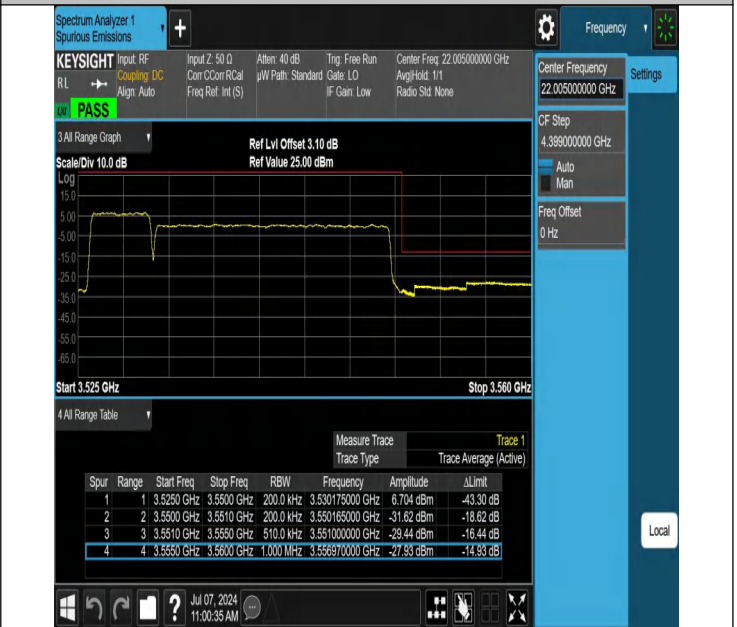
42-42(3450-3550)-5MHz-20MHz-QPSK@QPSK-QPSK@QPSK-4 2873-42990-25RB#0@25RB#0-100RB#0@100RB#0-PASS
