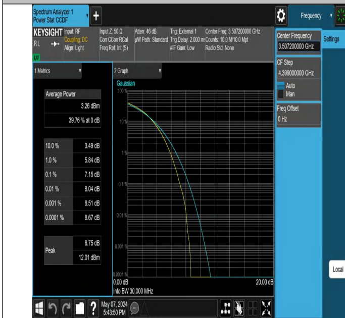
42-42(3450-3550)-10MHz-20MHz-256QAM-256QAM-42590-4273 4-50RB#0-100RB#0-PASS
