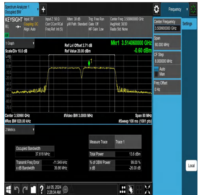
42-42(3450-3550)-20MHz-20MHz-16QAM-16QAM-42590-42788 -100RB#0-100RB#0-PASS
