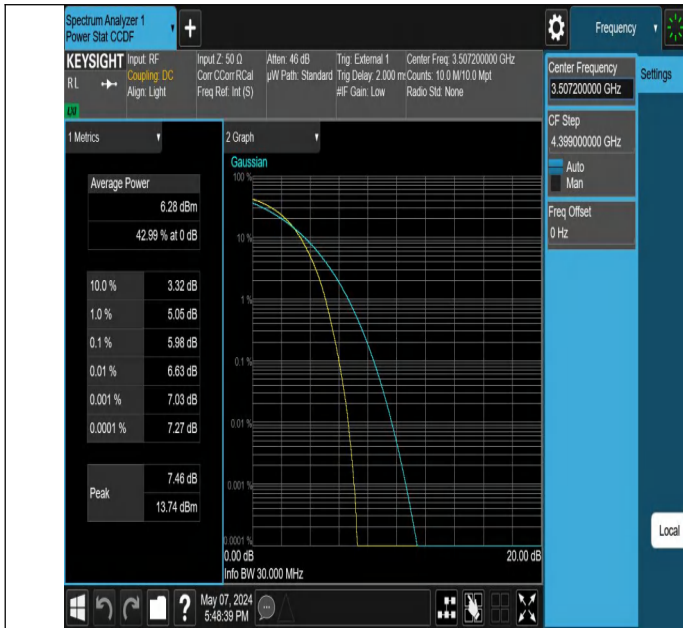
42-42(3450-3550)-20MHz-10MHz-QPSK-QPSK-42590-42734-100 RB#0-50RB#0-PASS
