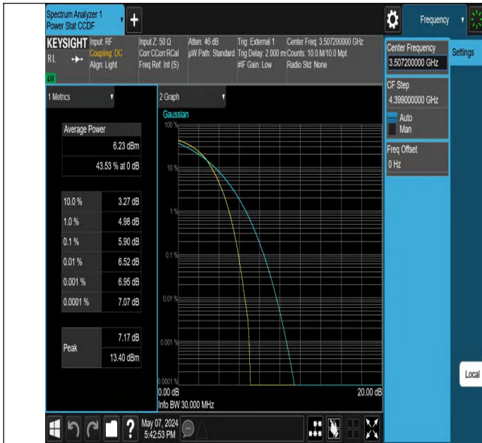
42-42(3450-3550)-10MHz-20MHz-QPSK-QPSK-42590-42734-50R B#0-100RB#0-PASS
