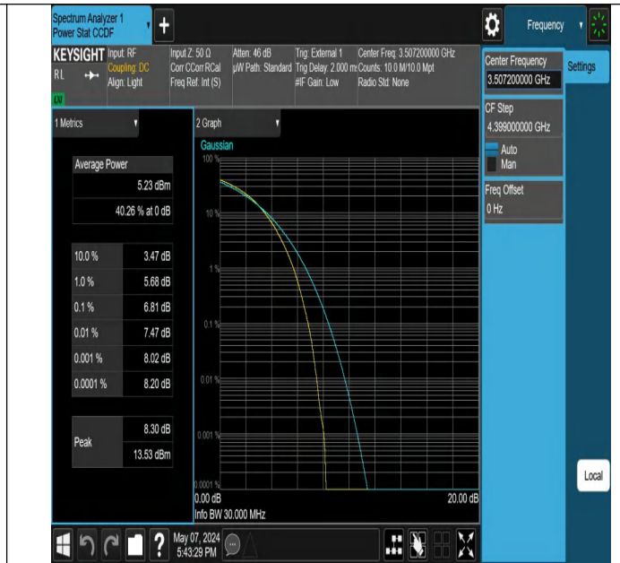
42-42(3450-3550)-10MHz-20MHz-64QAM-64QAM-42590-42734 -50RB#0-100RB#0-PASS
