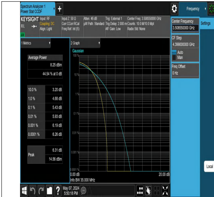
42-42(3450-3550)-20MHz-15MHz-QPSK-QPSK-42590-42761-100 RB#0-75RB#0-PASS
