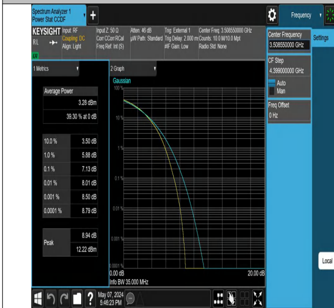
42-42(3450-3550)-15MHz-20MHz-256QAM-256QAM-42590-4276 1-75RB#0-100RB#0-PASS
