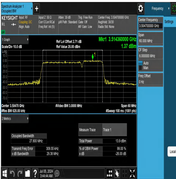
42-42(3450-3550)-20MHz-10MHz-256QAM-256QAM-42590-4273 4-100RB#0-50RB#0-PASS
