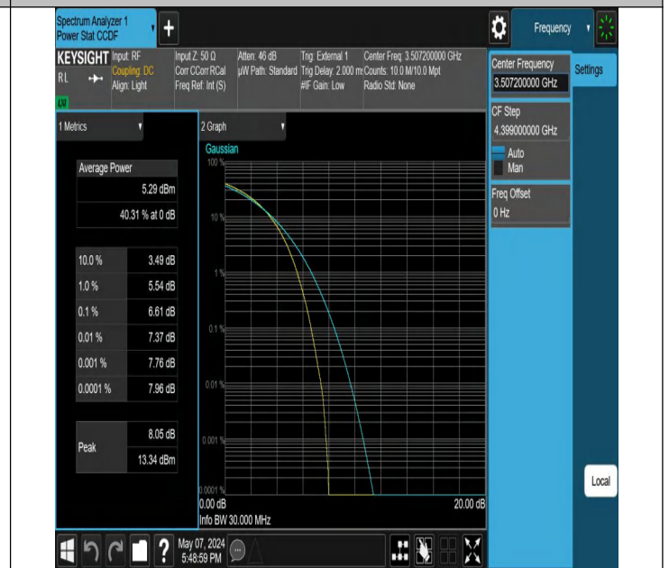
42-42(3450-3550)-20MHz-10MHz-16QAM-16QAM-42590-42734 -100RB#0-50RB#0-PASS
