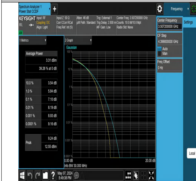
42-42(3450-3550)-20MHz-10MHz-256QAM-256QAM-42590-4273 4-100RB#0-50RB#0-PASS
