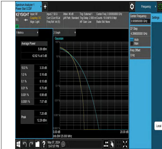
42-42(3450-3550)-20MHz-5MHz-QPSK-QPSK-42590-42707-100RB#0-25RB#0-PASS
