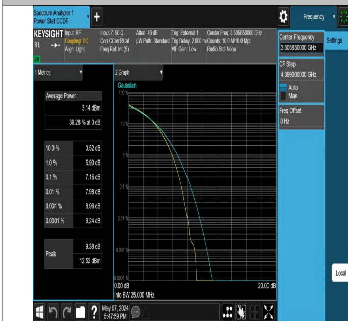
42-42(3450-3550)-20MHz-5MHz-256QAM-256QAM-42590-42707-100RB#0-25RB#0-PASS
