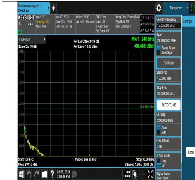
41-41-10MHz-20MHz-QPSK-QPSK-41346-41490-1RB#0-1RB#9 9-0.15~30MHz-PASS
