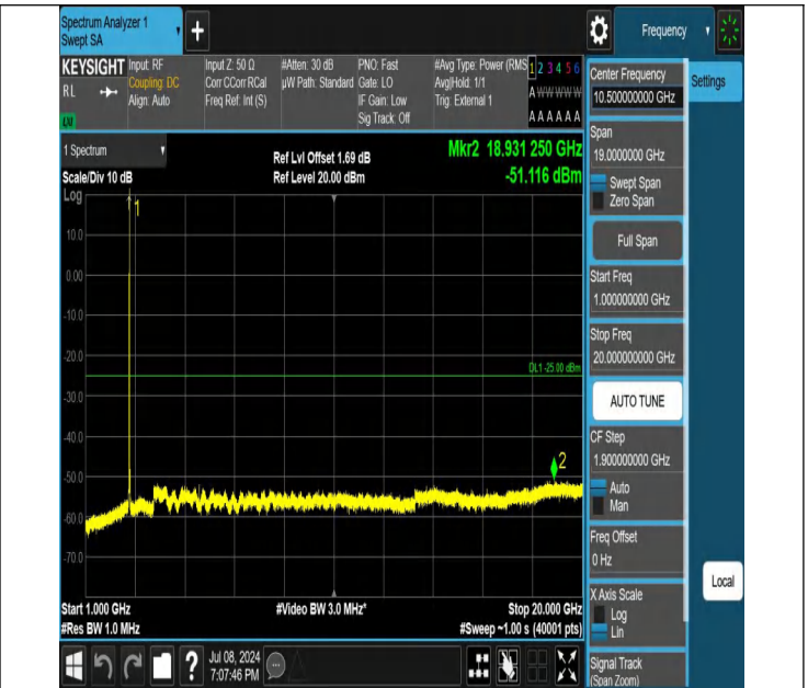
41-41-10MHz-20MHz-QPSK-QPSK-41346-41490-1RB#49-0RB# 0-1000~20000MHz-PASS
