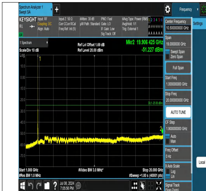
41-41-10MHz-20MHz-QPSK-QPSK-41346-41490-1RB#0-0RB#0- 1000~20000MHz-PASS
