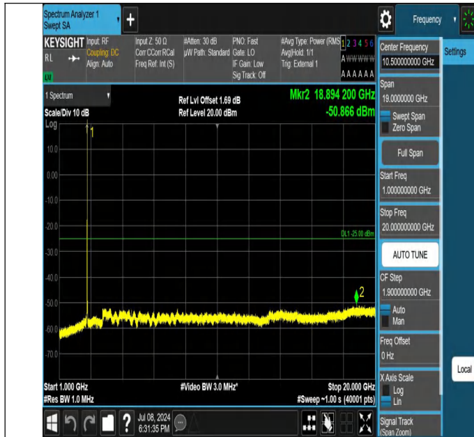
41-41-5MHz-20MHz-QPSK-QPSK-41373-41490-1RB#24-0RB#0-1000~20000MHz-PASS
