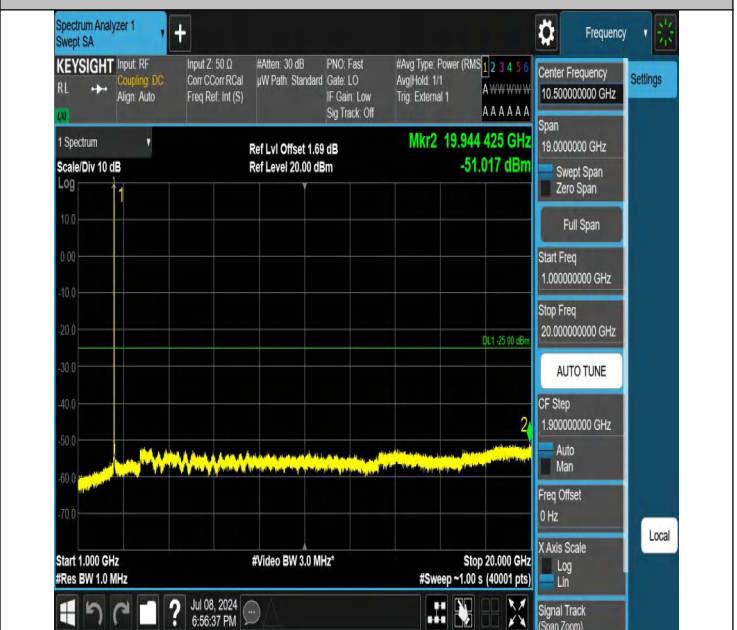
41-41-10MHz-20MHz-QPSK-QPSK-39705-39849-1RB#49-0RB# 0-1000~20000MHz-PASS
