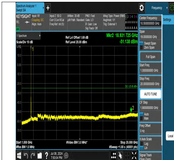
41-41-15MHz-20MHz-QPSK-QPSK-39728-39899-1RB#74-0RB# 0-1000~20000MHz-PASS
