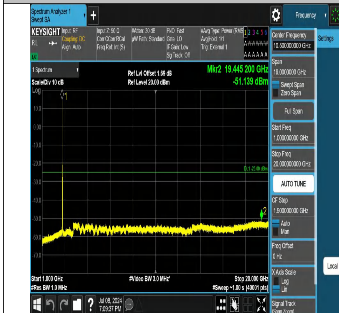
41-41-10MHz-20MHz-QPSK-QPSK-41346-41490-1RB#0-1RB#9 9-1000~20000MHz-PASS
