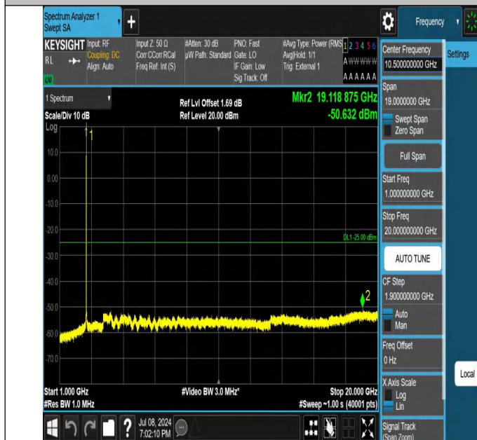
41-41-10MHz-20MHz-QPSK-QPSK-40526-40670-1RB#49-0RB# 0-1000~20000MHz-PASS
