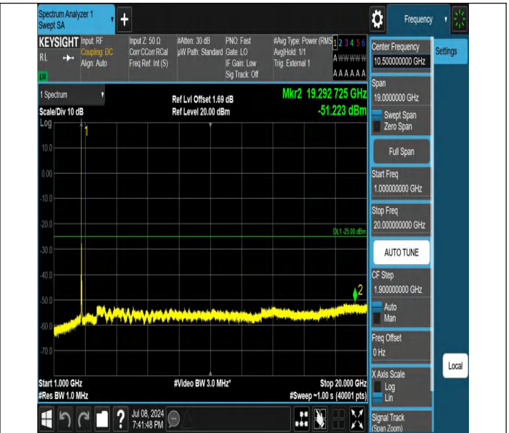
41-41-15MHz-15MHz-QPSK-QPSK-41365-41515-1RB#0-0RB#0-1000~20000MHz-PASS
