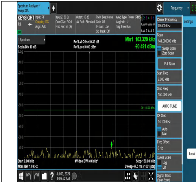
41-41-20MHz-15MHz-QPSK-QPSK-41341-41512-1RB#99-0RB# 0-0.009~0.15MHz-PASS
