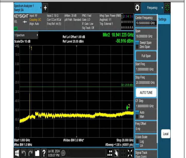
41-41-20MHz-15MHz-QPSK-QPSK-41341-41512-1RB#99-0RB# 0-1000~20000MHz-PASS
