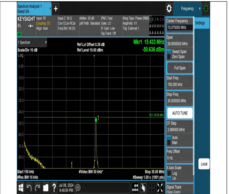
41-41-20MHz-15MHz-QPSK-QPSK-40546-40717-1RB#0-0RB#0-0.15~30MHz-PASS
