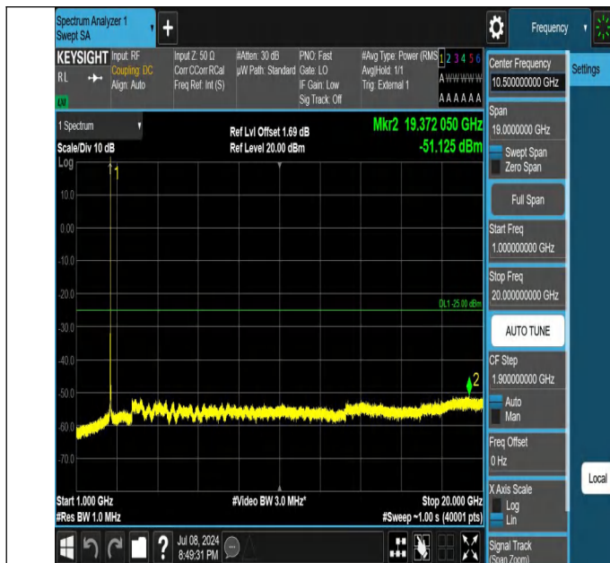
41-41-20MHz-15MHz-QPSK-QPSK-40546-40717-1RB#99-0RB# 0-1000~20000MHz-PASS
