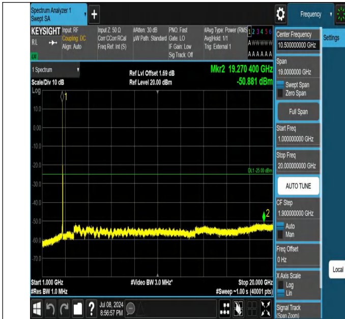
41-41-20MHz-15MHz-QPSK-QPSK-41341-41512-1RB#0-1RB#7 4-1000~20000MHz-PASS
