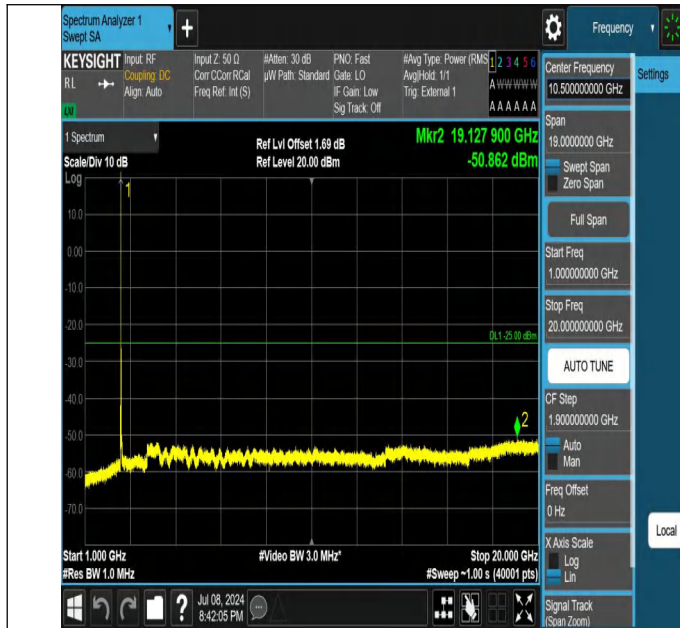
41-41-20MHz-15MHz-QPSK-QPSK-39750-39921-1RB#0-0RB#0-1000~20000MHz-PASS
