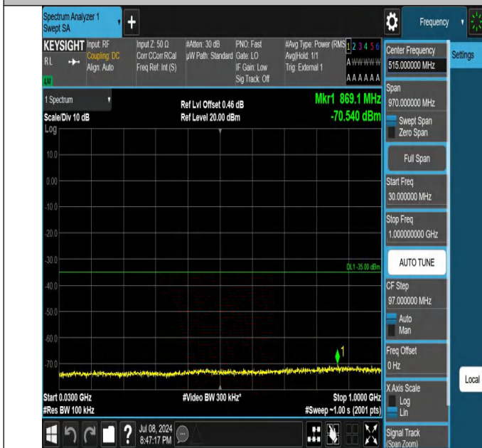
41-41-20MHz-15MHz-QPSK-QPSK-40546-40717-1RB#0-0RB#0-30~1000MHz-PASS
