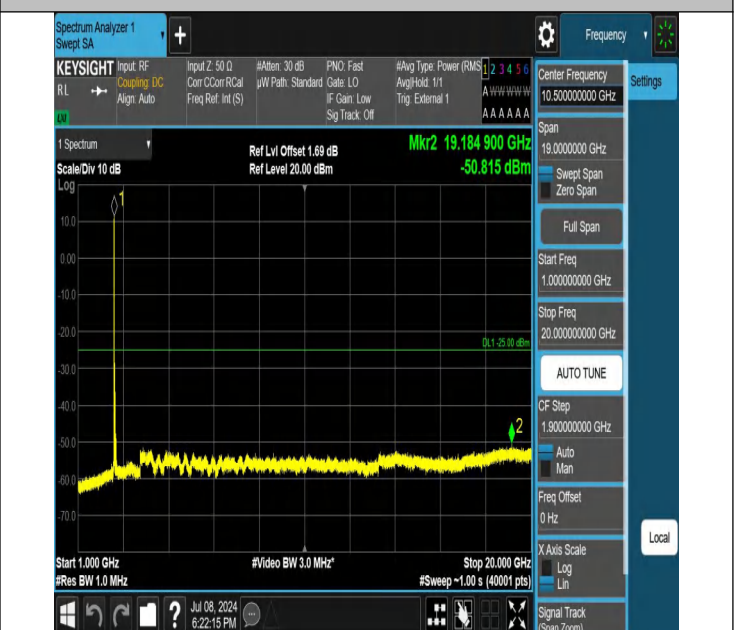
41-41.5MHz-20MHz-QPSK-QPSK-39683-39800-1RB#0-1RB#99- 1000~20000MHz-PASS
