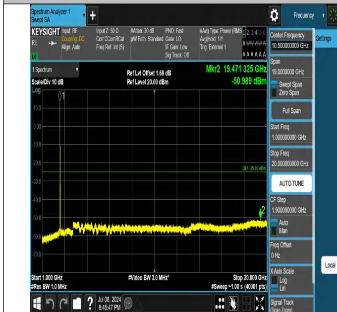
41-41-20MHz-15MHz-QPSK-QPSK-39750-39921-1RB#0-1RB#7 4-1000~20000MHz-PASS
