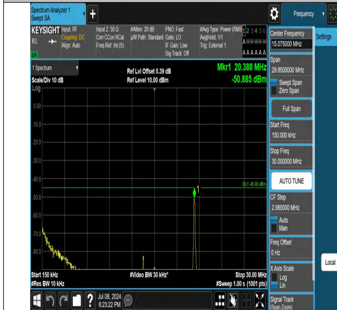
41-41-5MHz-20MHz-QPSK-QPSK-40528-40645-1RB#0-0RB#0-0 .15~30MHz-PASS
