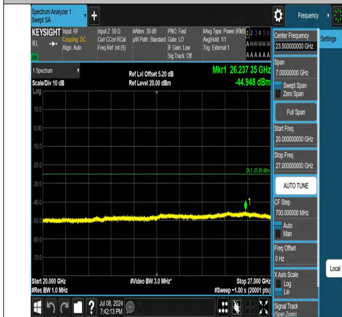
41-41-15MHz-15MHz-QPSK-QPSK-41365-41515-1RB#0-0RB#0-20000~27000MHz-PASS
