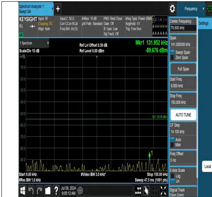
41-41-15MHz-15MHz-QPSK-QPSK-41365-41515-1RB#0-1RB#7 4-0.009~0.15MHz-PASS
