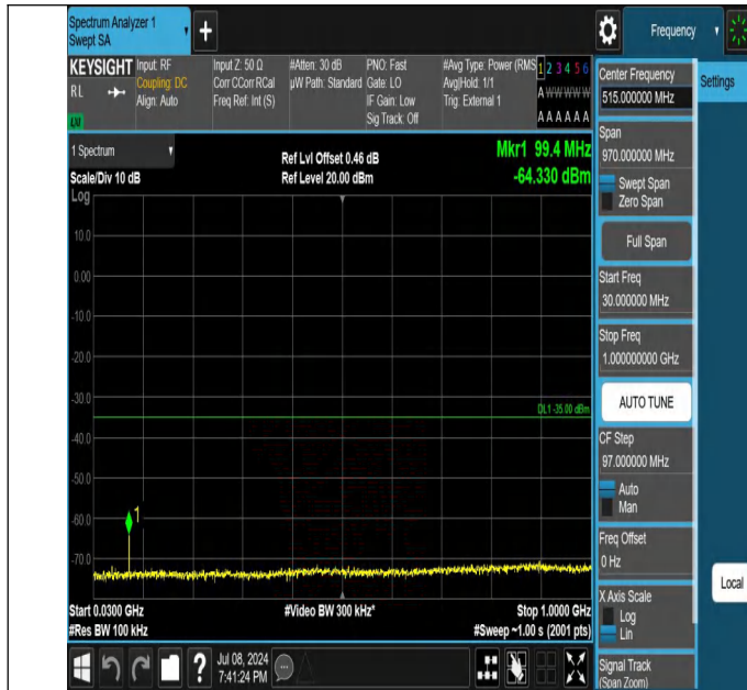
41-41-15MHz-15MHz-QPSK-QPSK-41365-41515-1RB#0-0RB#0-30~1000MHz-PASS
