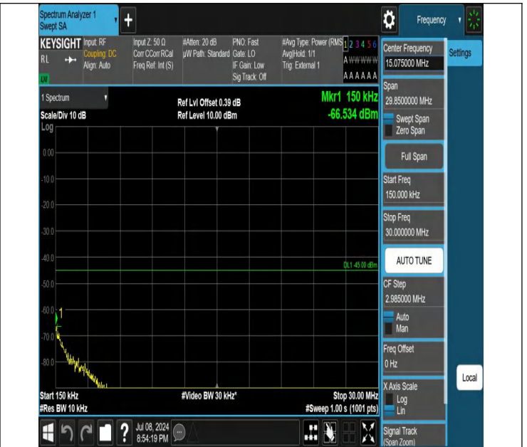
41-41-20MHz-15MHz-QPSK-QPSK-41341-41512-1RB#99-0RB# 0-0.15~30MHz-PASS
