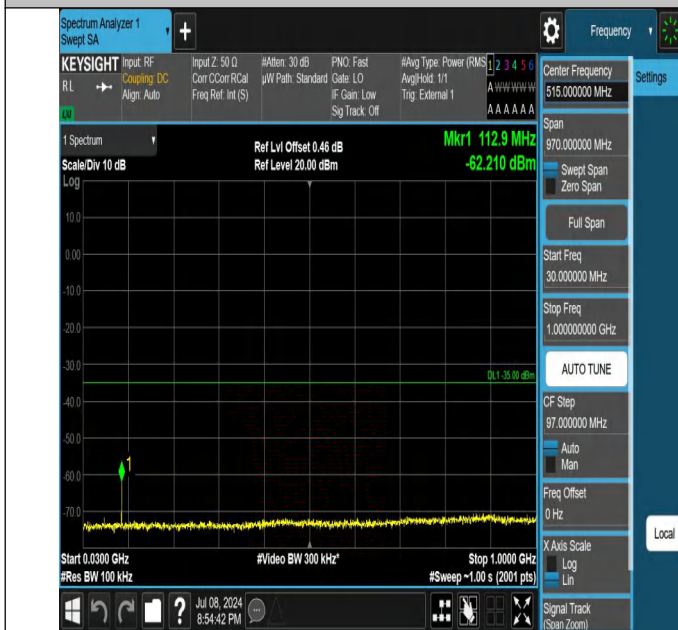
41-41-20MHz-15MHz-QPSK-QPSK-41341-41512-1RB#99-0RB# 0-30~1000MHz-PASS
