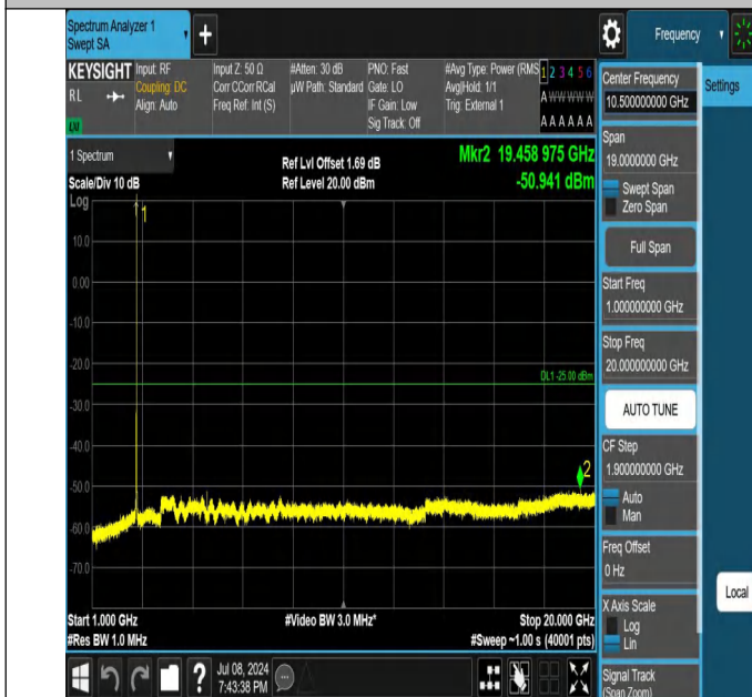
41-41-15MHz-15MHz-QPSK-QPSK-41365-41515-1RB#74-0RB# 0-1000~20000MHz-PASS
