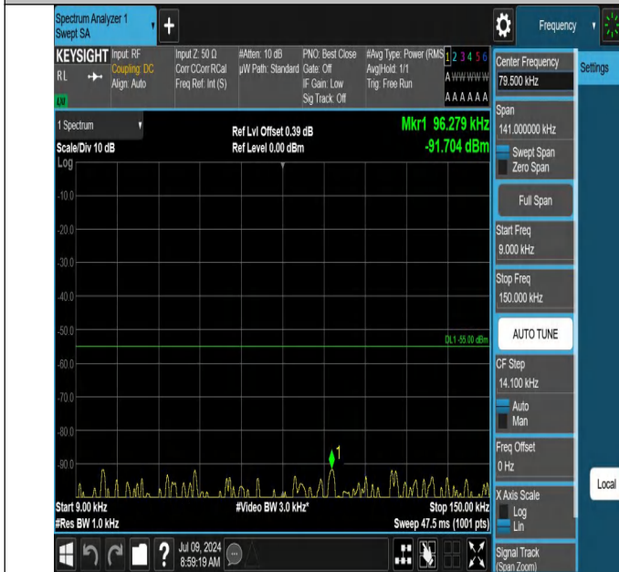
41-41-5MHz-20MHz-QPSK-QPSK-39683-39800-1RB#0-0RB#0-0 .009~0.15MHz-PASS
