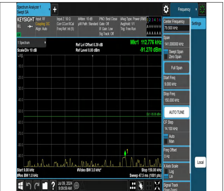
41-41-20MHz-15MHz-QPSK-QPSK-41341-41512-1RB#0-1RB#7 4-0.009~0.15MHz-PASS
