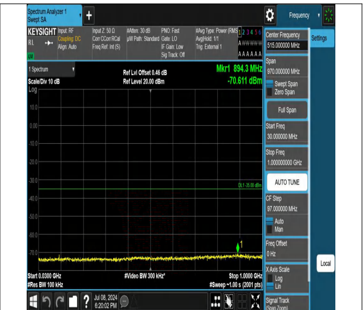
41-41.5MHz-20MHz-QPSK-QPSK-39683-39800-1RB#24-0RB#0- 30~1000MHz-PASS
