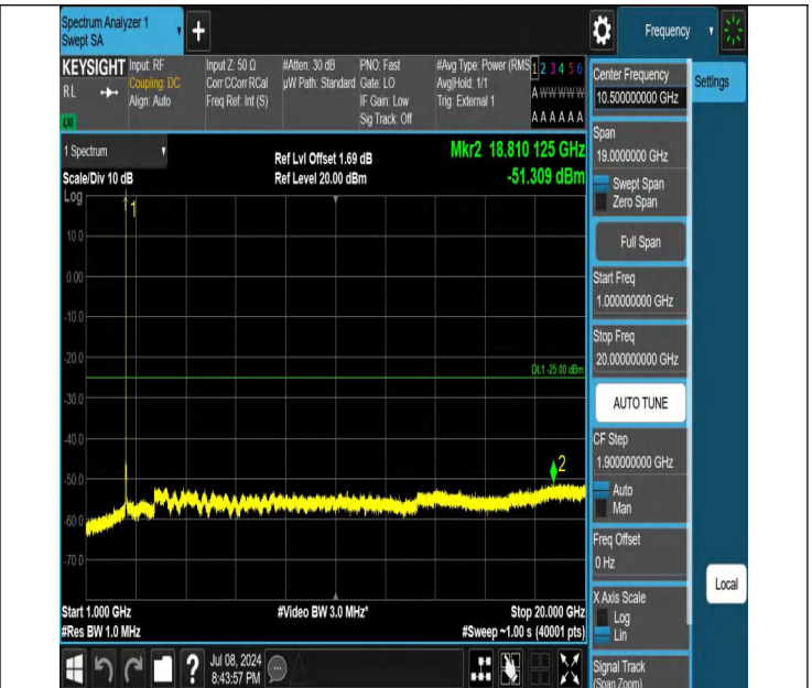
41-41-20MHz-15MHz-QPSK-QPSK-39750-39921-1RB#99-0RB# 0-1000~20000MHz-PASS
