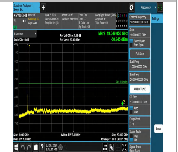
41-41-20MHz-15MHz-QPSK-QPSK-40546-40717-1RB#0-0RB#0-1000~20000MHz-PASS
