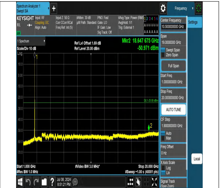
41-41-20MHz-15MHz-QPSK-QPSK-40546-40717-1RB#0-1RB#7 4-1000~20000MHz-PASS
