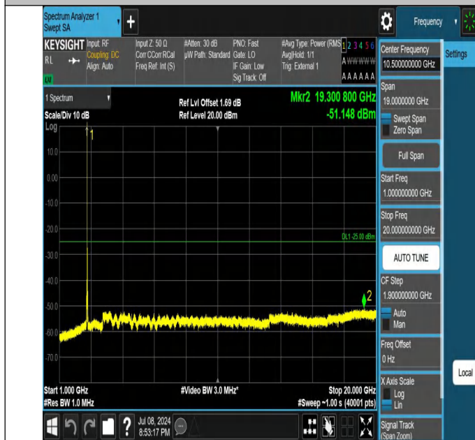
41-41-20MHz-15MHz-QPSK-QPSK-41341-41512-1RB#0-0RB#0-1000~20000MHz-PASS
