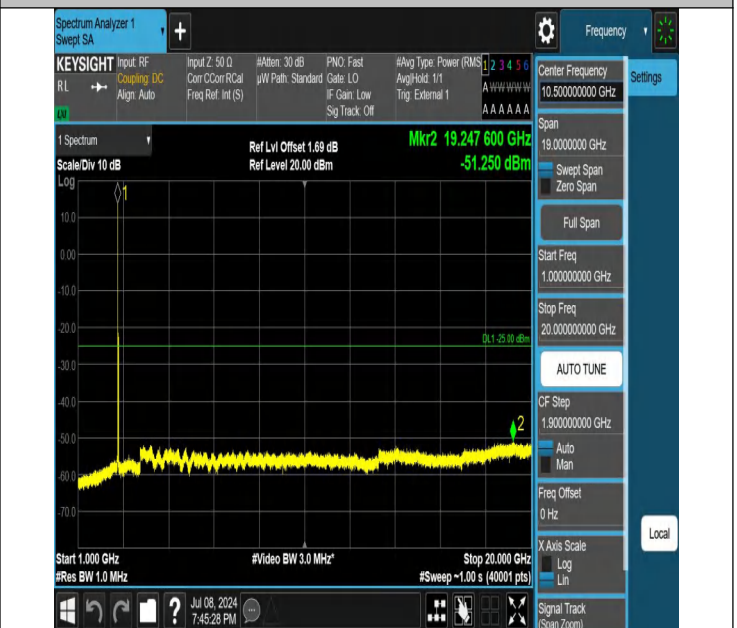
41-41-15MHz-15MHz-QPSK-QPSK-41365-41515-1RB#0-1RB#7 4-1000~20000MHz-PASS
