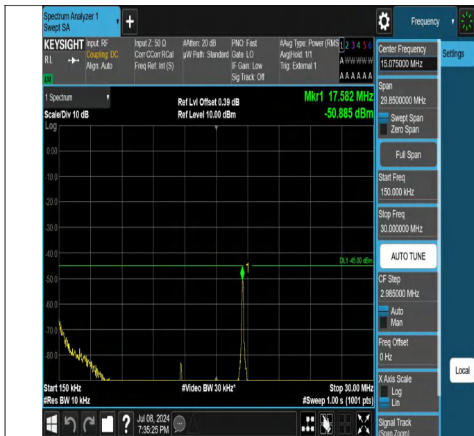
41-41-15MHz-15MHz-QPSK-QPSK-40545-40695-1RB#0-0RB#0- 0.15~30MHz-PASS
