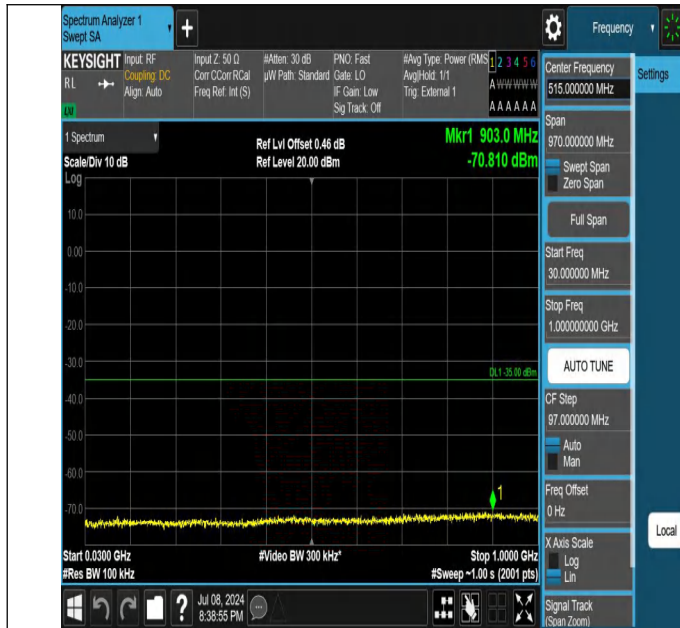
41-41-20MHz-10MHz-QPSK-QPSK-41391-41535-1RB#0-1RB#4 9-30~1000MHz-PASS
