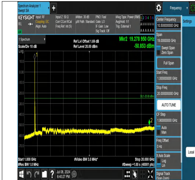
41-41-10MHz-15MHz-QPSK-QPSK-39703-39823-1RB#0-1RB#7 4-1000~20000MHz-PASS
