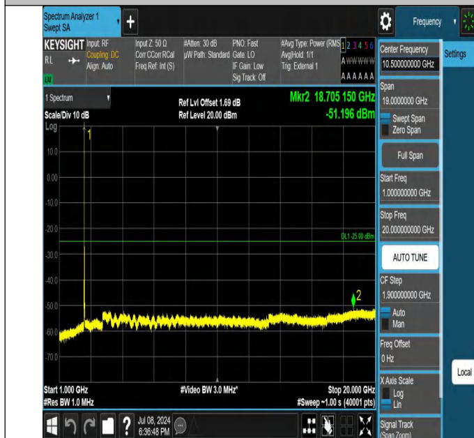
41-41-10MHz-15MHz-QPSK-QPSK-39703-39823-1RB#0-0RB#0- 1000~20000MHz-PASS
