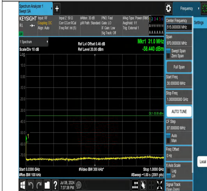
41-41-15MHz-15MHz-QPSK-QPSK-40545-40695-1RB#74-0RB# 0-30~1000MHz-PASS
