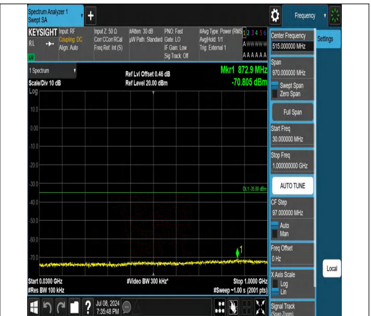
41-41-15MHz-15MHz-QPSK-QPSK-40545-40695-1RB#0-0RB#0- 30~1000MHz-PASS
