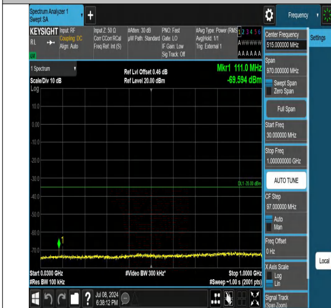
41-41-10MHz-15MHz-QPSK-QPSK-39703-39823-1RB#49-0RB# 0-30~1000MHz-PASS
