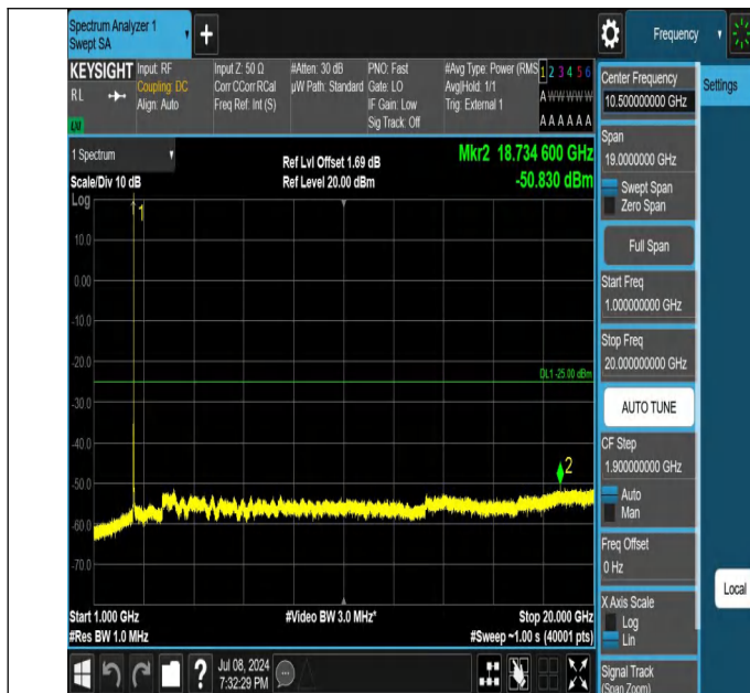
41-41-15MHz-15MHz-QPSK-QPSK-39725-39875-1RB#74-0RB# 0-1000~20000MHz-PASS
