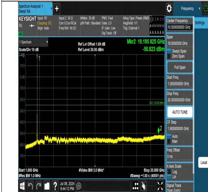
41-41-10MHz-15MHz-QPSK-QPSK-40549-40669-1RB#49-0RB# 0-1000~20000MHz-PASS
