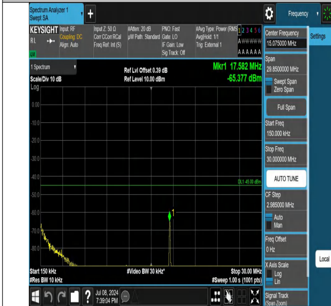
41-41-15MHz-15MHz-QPSK-QPSK-40545-40695-1RB#0-1RB#7 4-0.15~30MHz-PASS
