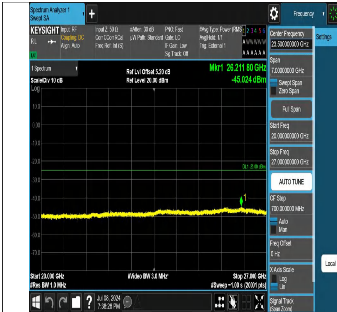
41-41-15MHz-15MHz-QPSK-QPSK-40545-40695-1RB#74-0RB# 0-20000~27000MHz-PASS
