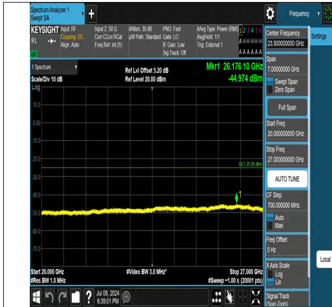
41-41-10MHz-15MHz-QPSK-QPSK-39703-39823-1RB#49-0RB# 0-20000~27000MHz-PASS
