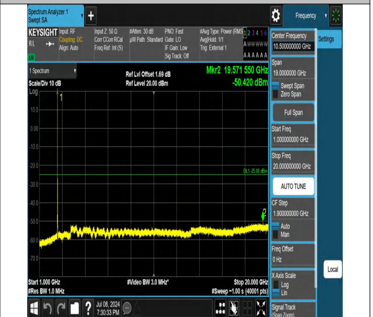
41-41-15MHz-15MHz-QPSK-QPSK-39725-39875-1RB#0-0RB#0-1000~20000MHz-PASS
