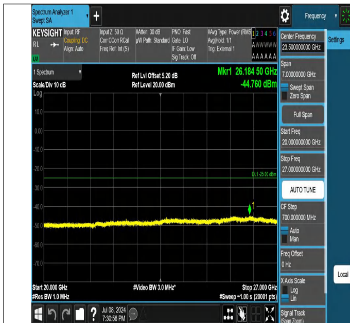
41-41-15MHz-15MHz-QPSK-QPSK-39725-39875-1RB#0-0RB#0- 20000~27000MHz-PASS
