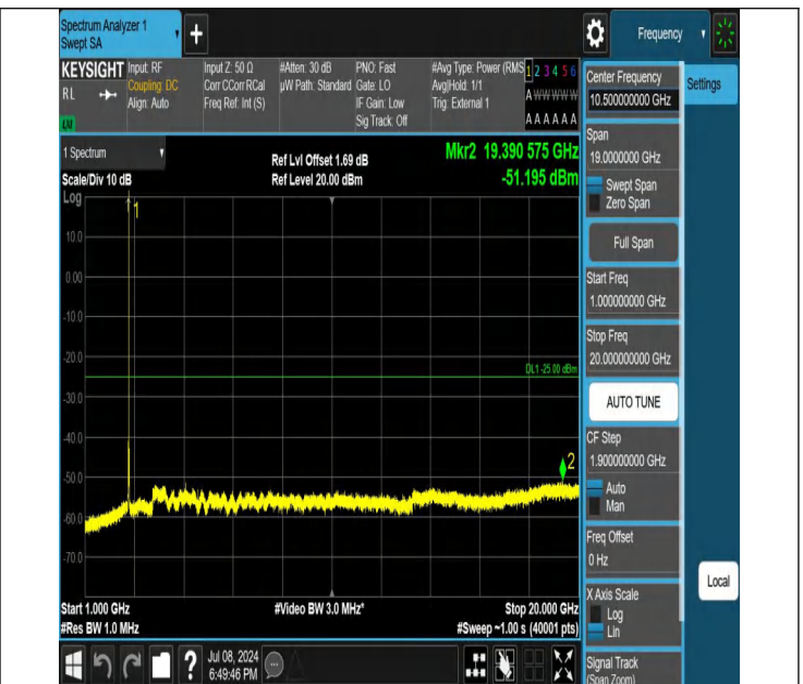
41-41-10MHz-15MHz-QPSK-QPSK-41395-41515-1RB#49-0RB# 0-1000~20000MHz-PASS
