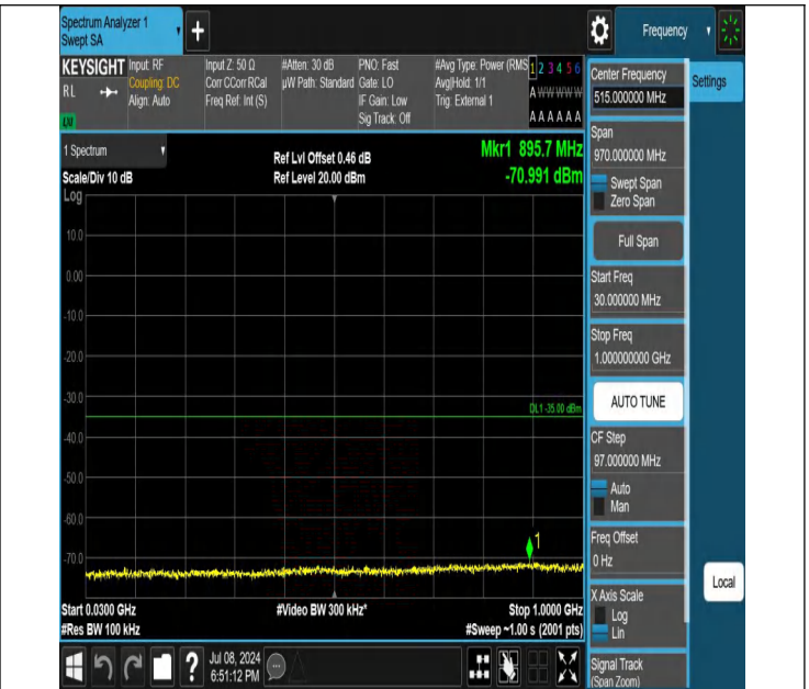
41-41-10MHz-15MHz-QPSK-QPSK-41395-41515-1RB#0-1RB#7 4-30~1000MHz-PASS
