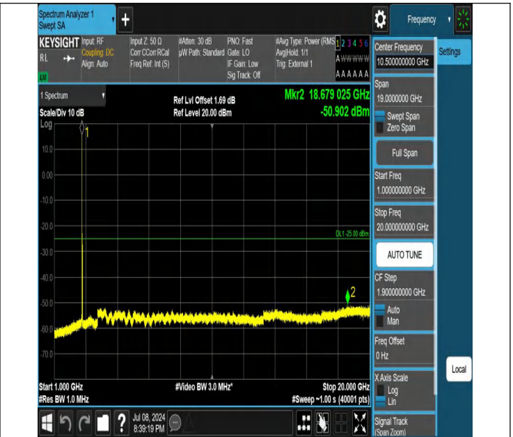
41-41-20MHz-10MHz-QPSK-QPSK-41391-41535-1RB#0-1RB#4 9-1000~20000MHz-PASS
