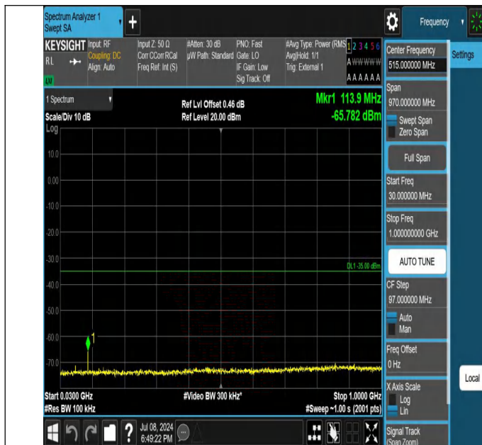
41-41-10MHz-15MHz-QPSK-QPSK-41395-41515-1RB#49-0RB# 0-30~1000MHz-PASS
