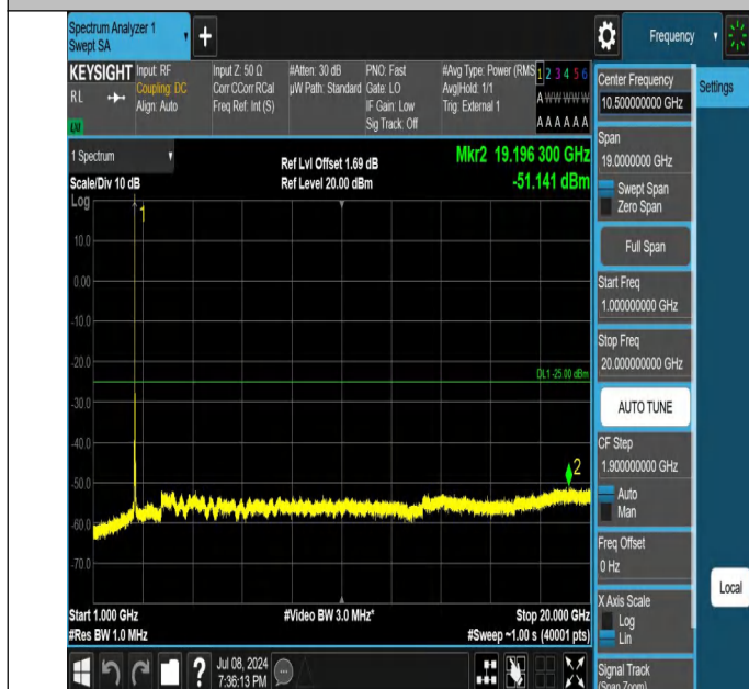
41-41-15MHz-15MHz-QPSK-QPSK-40545-40695-1RB#0-0RB#0- 1000~20000MHz-PASS
