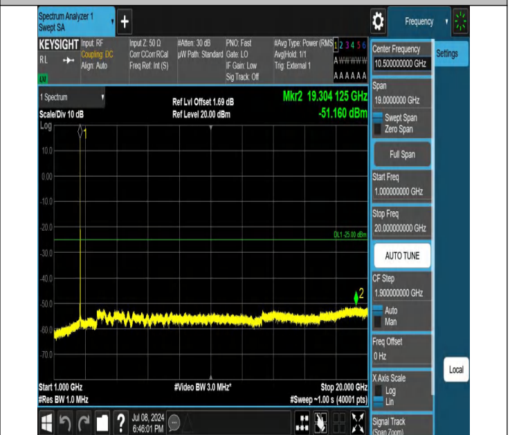
41-41-10MHz-15MHz-QPSK-QPSK-40549-40669-1RB#0-1RB#7 4-1000~20000MHz-PASS
