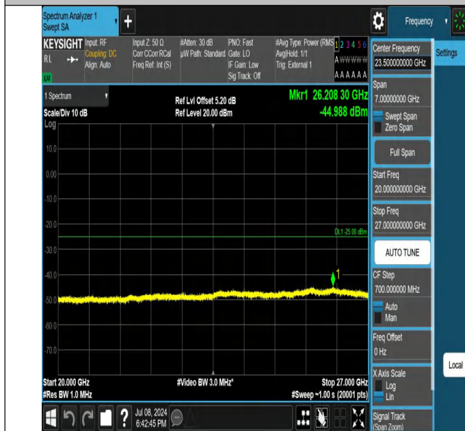
41-41-10MHz-15MHz-QPSK-QPSK-40549-40669-1RB#0-0RB#0-20000~27000MHz-PASS
