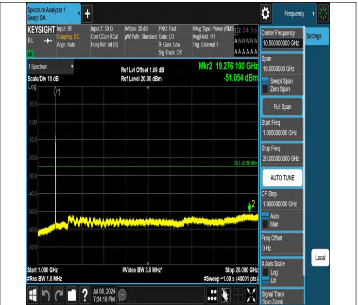
41-41-15MHz-15MHz-QPSK-QPSK-39725-39875-1RB#0-1RB#7 4-1000~20000MHz-PASS
