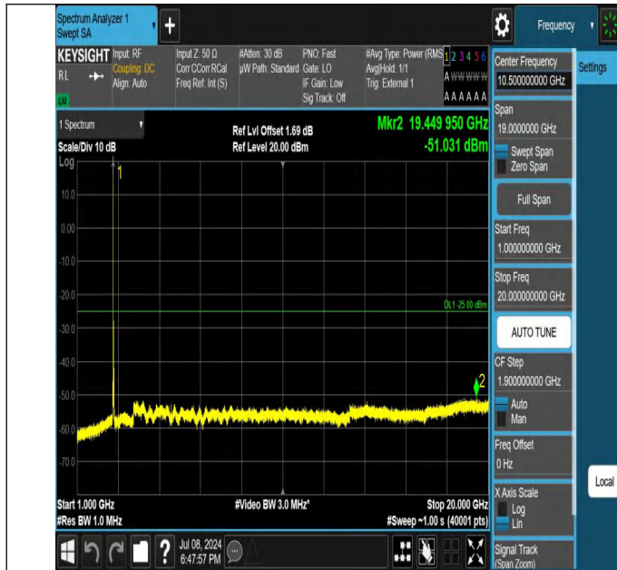
41-41-10MHz-15MHz-QPSK-QPSK-41395-41515-1RB#0-0RB#0-1000~20000MHz-PASS
