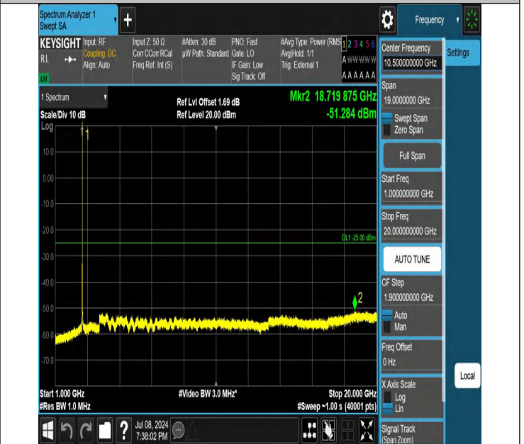
41-41-15MHz-15MHz-QPSK-QPSK-40545-40695-1RB#74-0RB# 0-1000~20000MHz-PASS
