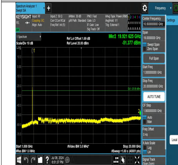
41-41-10MHz-15MHz-QPSK-QPSK-41395-41515-1RB#0-1RB#7 4-1000~20000MHz-PASS
