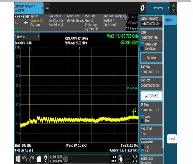
41-41-10MHz-15MHz-QPSK-QPSK-39703-39823-1RB#49-0RB# 0-1000~20000MHz-PASS
