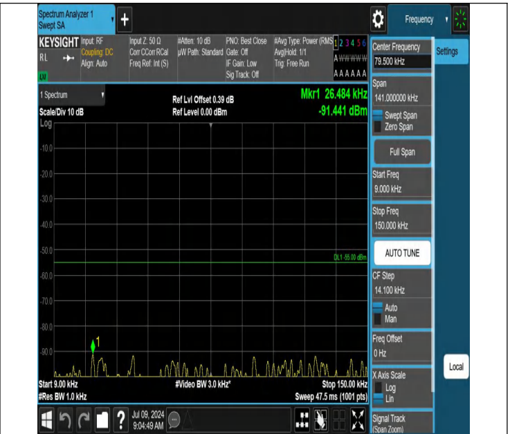
41-41-15MHz-15MHz-QPSK-QPSK-40545-40695-1RB#0-1RB#7 4-0.009~0.15MHz-PASS
