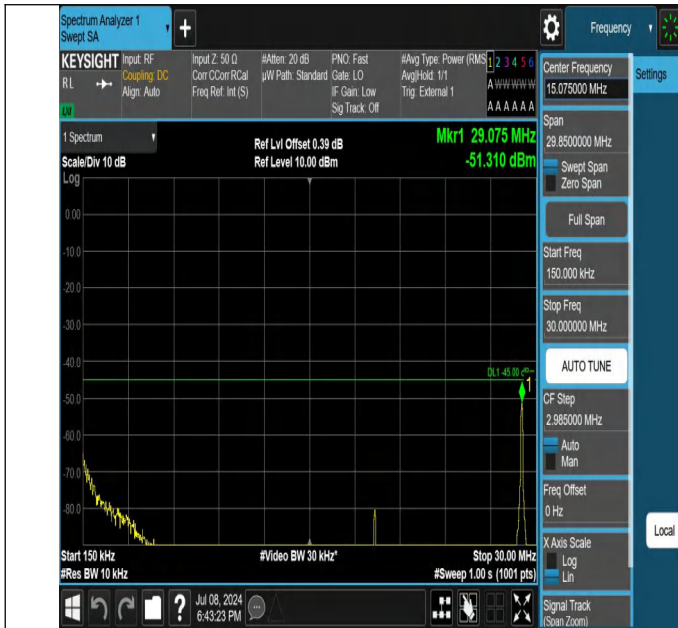
41-41-10MHz-15MHz-QPSK-QPSK-40549-40669-1RB#49-0RB# 0-0.15~30MHz-PASS
