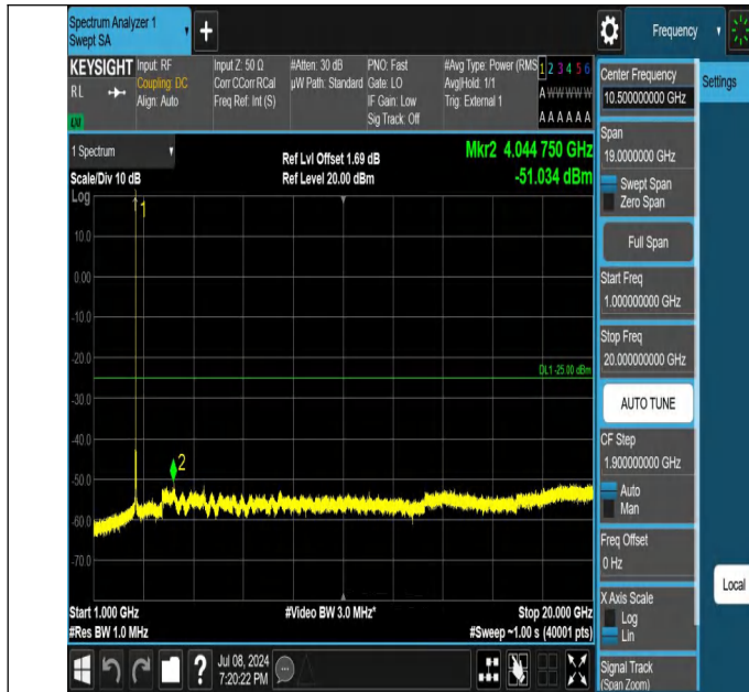
41-41-15MHz-10MHz-QPSK-QPSK-40571-40691-1RB#74-0RB# 0-1000~20000MHz-PASS
