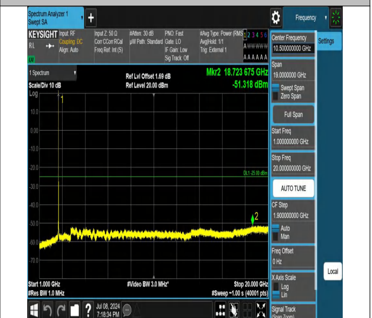
41-41-15MHz-10MHz-QPSK-QPSK-40571-40691-1RB#0-0RB#0- 1000~20000MHz-PASS
