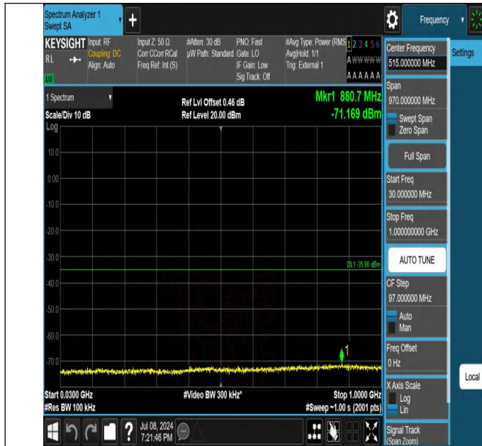
41-41-15MHz-10MHz-QPSK-QPSK-40571-40691-1RB#0-1RB#4 9-30~1000MHz-PASS
