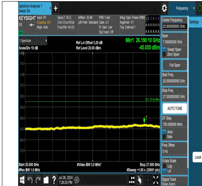
41-41-15MHz-10MHz-QPSK-QPSK-41417-41537-1RB#74-0RB# 0-20000~27000MHz-PASS
