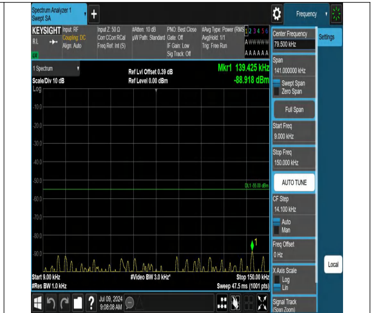
41-41-20MHz-10MHz-QPSK-QPSK-40571-40715-1RB#0-0RB#0- 0.009~0.15MHz-PASS
