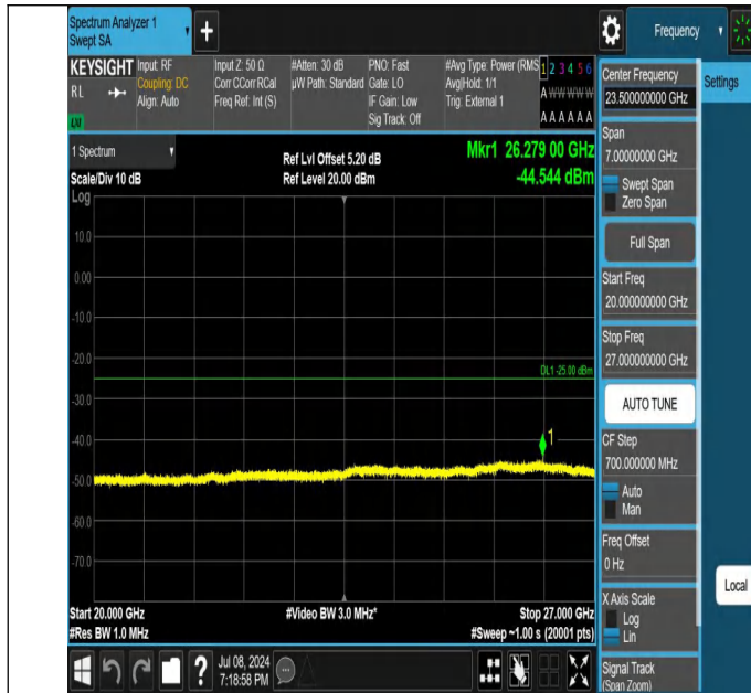
41-41-15MHz-10MHz-QPSK-QPSK-40571-40691-1RB#0-0RB#0- 20000~27000MHz-PASS
