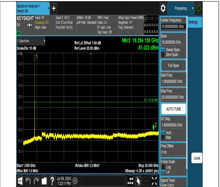
41-41-15MHz-10MHz-QPSK-QPSK-40571-40691-1RB#0-1RB#4 9-1000~20000MHz-PASS
