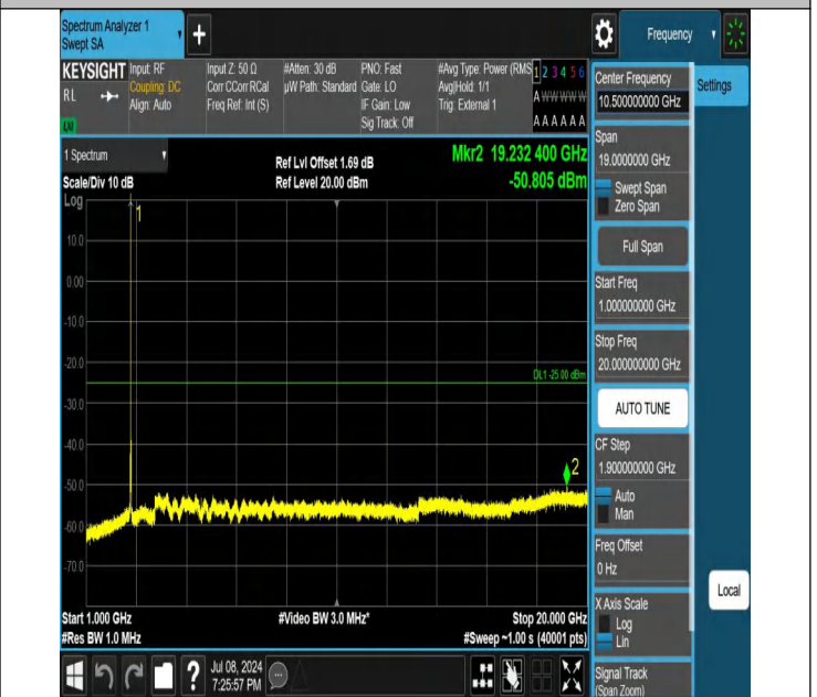
41-41-15MHz-10MHz-QPSK-QPSK-41417-41537-1RB#74-0RB# 0-1000~20000MHz-PASS
