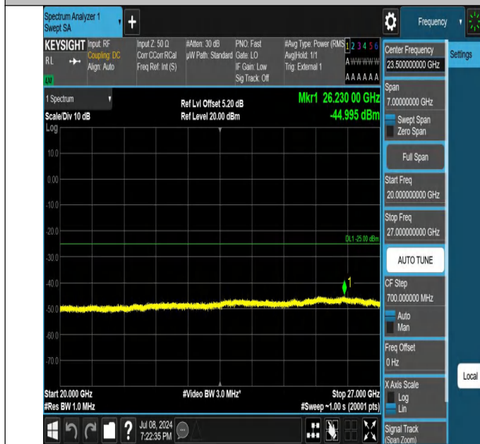
41-41-15MHz-10MHz-QPSK-QPSK-40571-40691-1RB#0-1RB#4 9-20000~27000MHz-PASS
