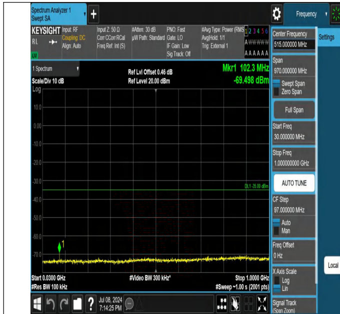
41-41-15MHz-10MHz-QPSK-QPSK-39725-39845-1RB#74-0RB# 0-30~1000MHz-PASS
