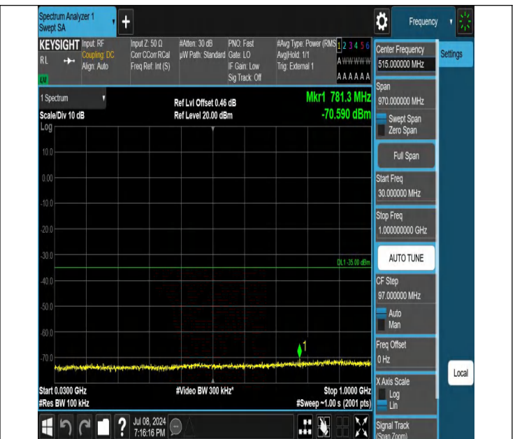
41-41.15MHz-10MHz-QPSK-QPSK-39725-39845-1RB#0-1RB#4 9-30~1000MHz-PASS
