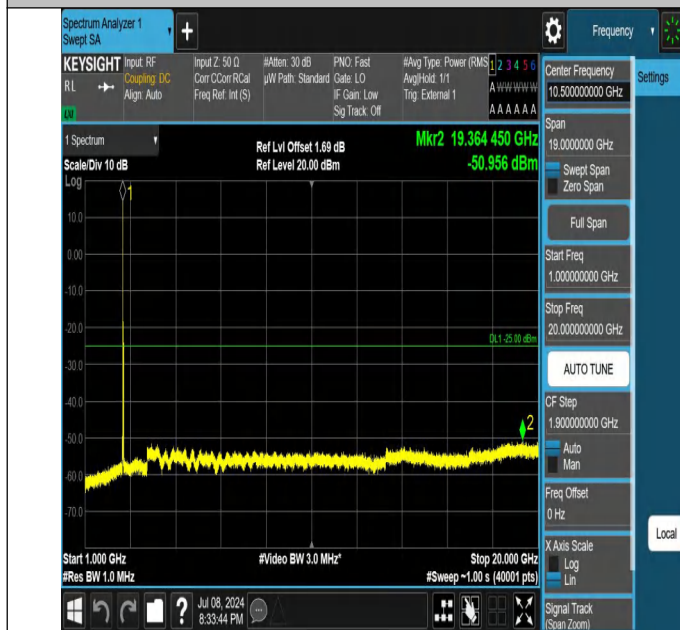
41-41-20MHz-10MHz-QPSK-QPSK-40571-40715-1RB#0-1RB#4 9-1000~20000MHz-PASS
