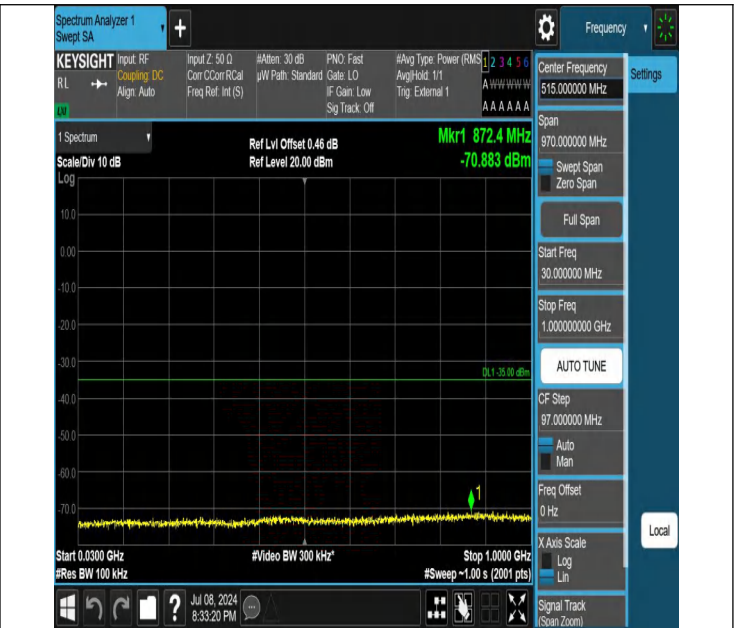
41-41-20MHz-10MHz-QPSK-QPSK-40571-40715-1RB#0-1RB#4 9-30~1000MHz-PASS
