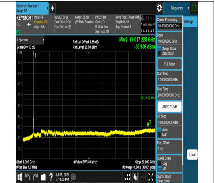
41-41-15MHz-10MHz-QPSK-QPSK-39725-39845-1RB#74-0RB# 0-1000~20000MHz-PASS
