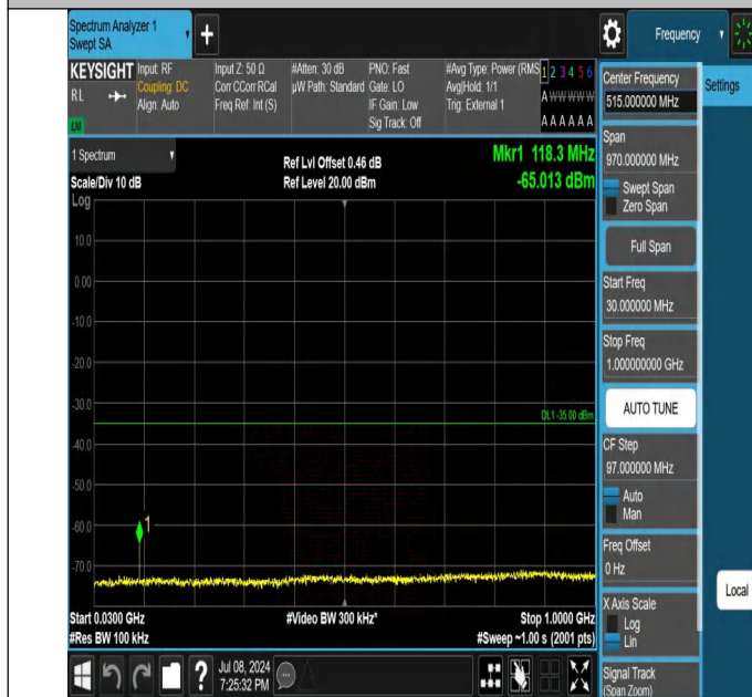
41-41-15MHz-10MHz-QPSK-QPSK-41417-41537-1RB#74-0RB# 0-30~1000MHz-PASS
