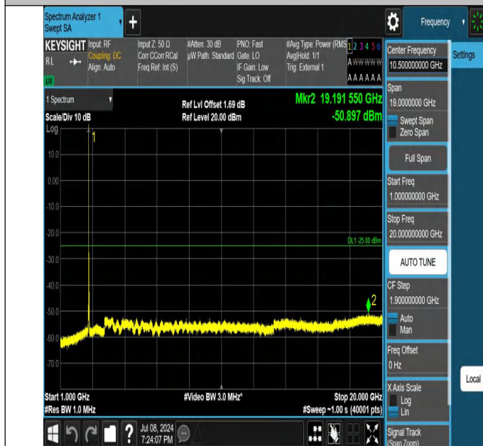
41-41-15MHz-10MHz-QPSK-QPSK-41417-41537-1RB#0-0RB#0- 1000~20000MHz-PASS
