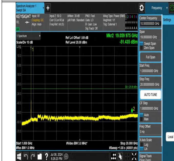
41-41-20MHz-10MHz-QPSK-QPSK-39750-39894-1RB#99-0RB# 0-1000~20000MHz-PASS
