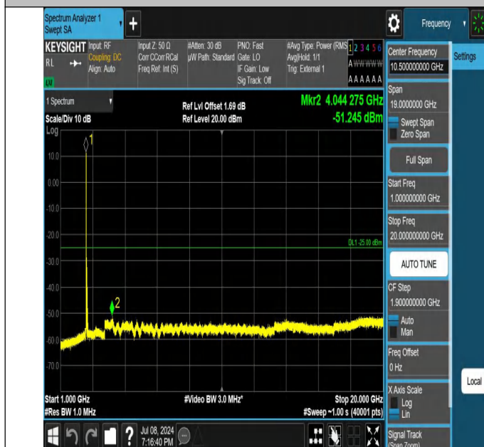
41-41-15MHz-10MHz-QPSK-QPSK-39725-39845-1RB#0-1RB#4 9-1000~20000MHz-PASS
