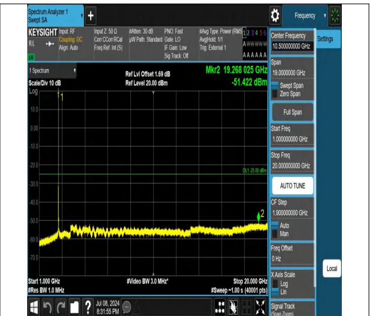
41-41-20MHz-10MHz-QPSK-QPSK-40571-40715-1RB#99-0RB# 0-1000~20000MHz-PASS
