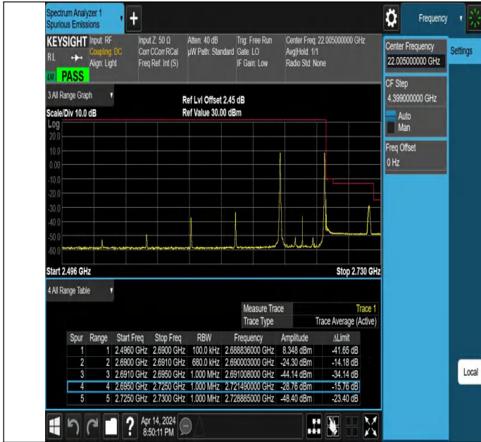
20MHz-15MHz_QPSK@QPSK-QPSK@QPSK_41341-41512_1RB#0@100RB#0-1RB#74@75RB#0
