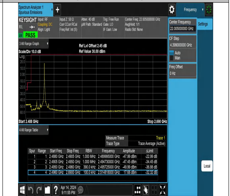
20MHz-20MHz_QPSK@QPSK-QPSK@QPSK_39750-39948_1RB#99@100RB#0-0RB#0@100RB#0
