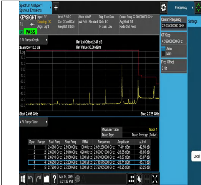
20MHz-10MHz_QPSK@QPSK-QPSK@QPSK_41391-41535_1RB#0@100RB#0-1RB#49@50RB#0
