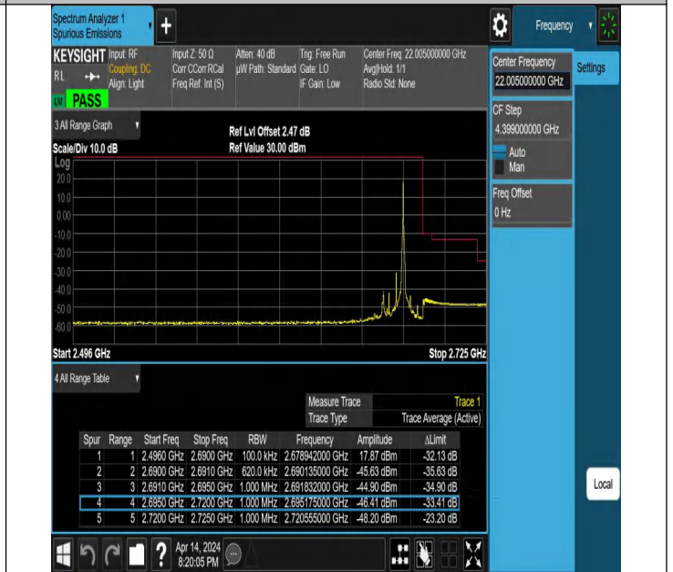
20MHz-10MHz_QPSK@QPSK-QPSK@QPSK_41391-41535_1RB#99@100RB#0-0RB#0@50RB#0
