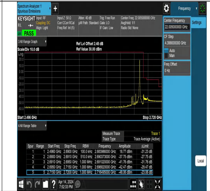
20MHz-5MHz_QPSK@QPSK-QPSK@QPSK_41440-41557_1R B#99@100RB#0-0RB#0@25RB#0
