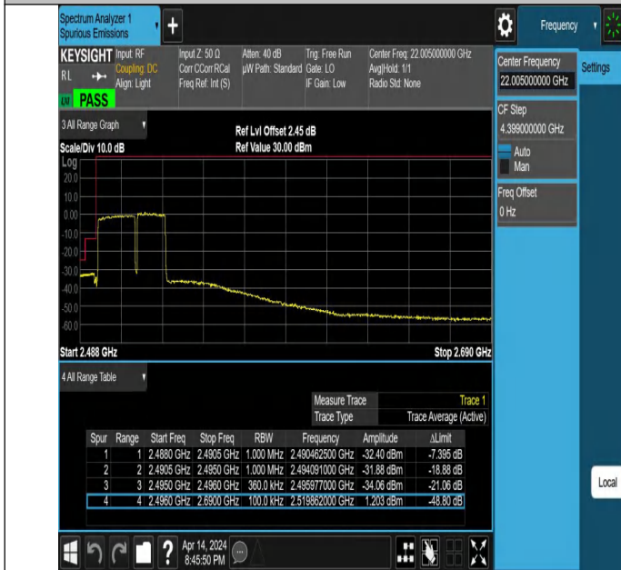
20MHz-15MHz_QPSK@QPSK-QPSK@QPSK_39750-39921_100 RB#0@100RB#0-75RB#0@75RB#0
