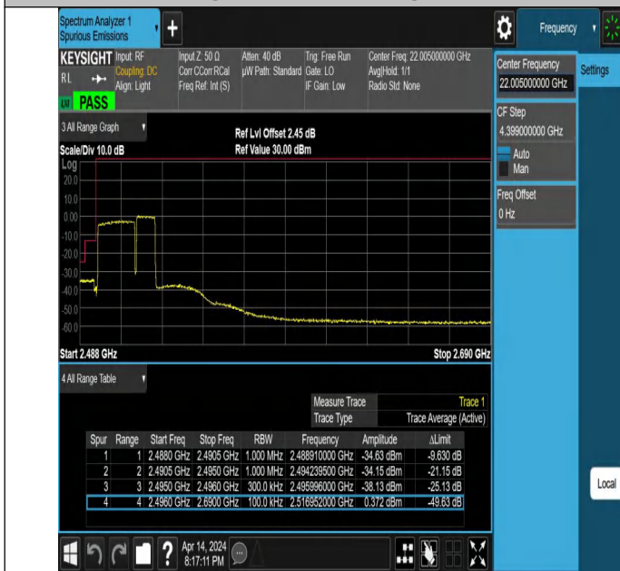
20MHz-10MHz_QPSK@QPSK-QPSK@QPSK_39750-39894_100RB#0@100RB#0-50RB#0@50RB#0
