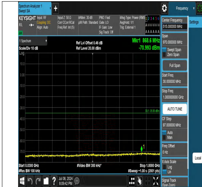
41-41-20MHz-5MHz-QPSK-QPSK-39750-39867-1RB#0-1RB#24- 30~1000MHz-PASS
