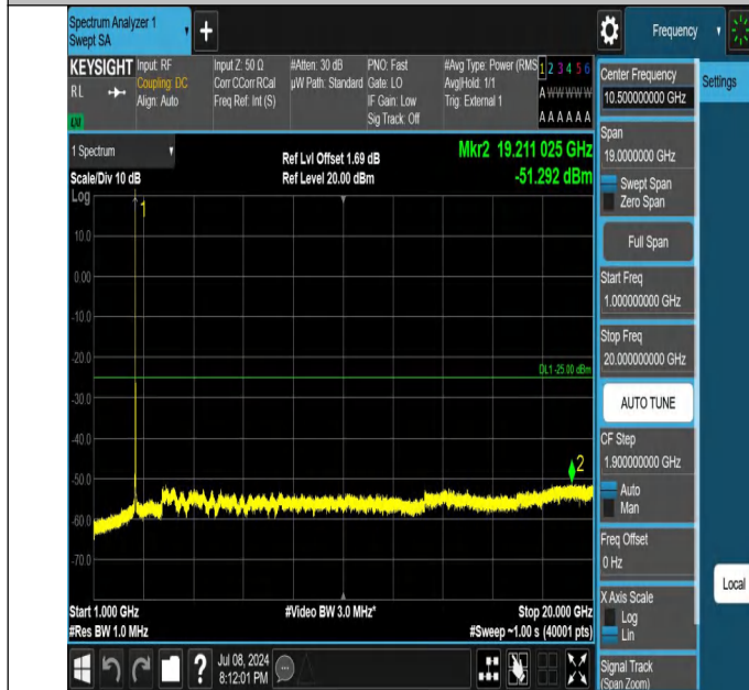
41-41-20MHz-5MHz-QPSK-QPSK-40595-40712-1RB#0-0RB#0-1 000~20000MHz-PASS
