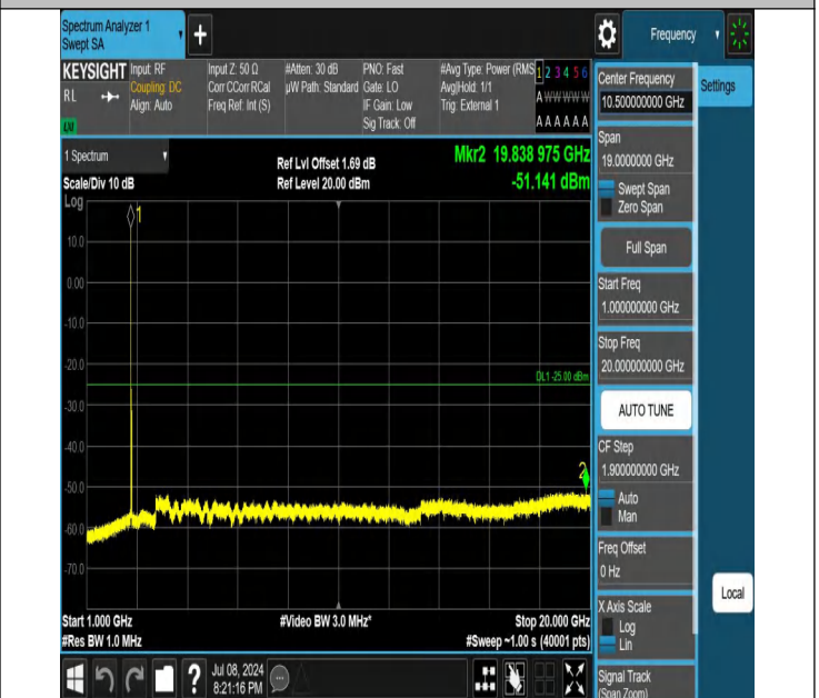
41-41-20MHz-5MHz-QPSK-QPSK-41440-41557-1RB#0-1RB#24- 1000~20000MHz-PASS
