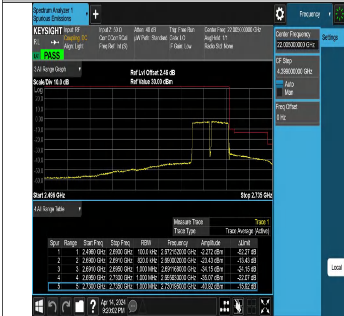
20MHz-20MHz_QPSK@QPSK-QPSK@QPSK_41292-41490_100RB#0@100RB#0-100RB#0@100RB#0
