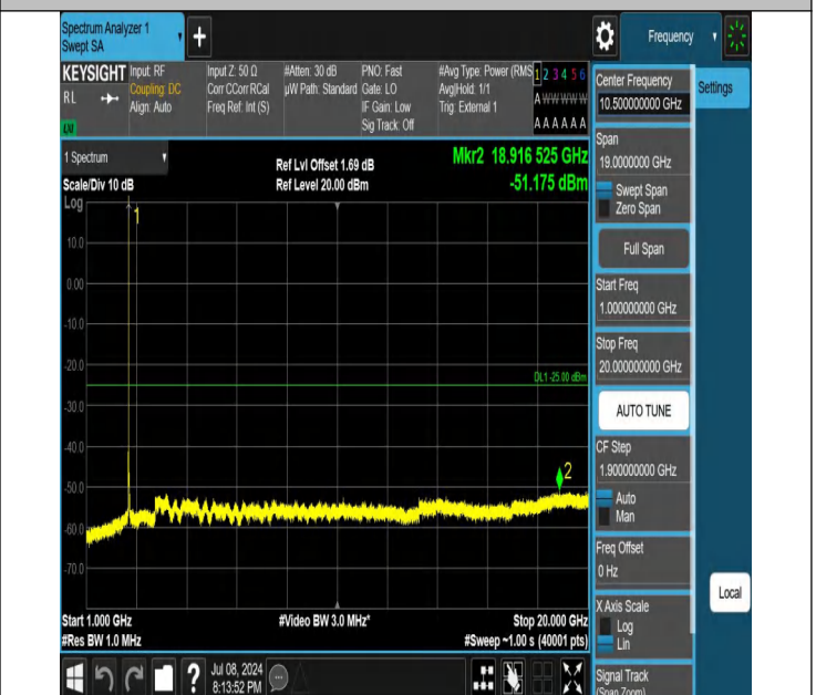
41-41-20MHz-5MHz-QPSK-QPSK-40595-40712-1RB#99-0RB#0- 1000~20000MHz-PASS
