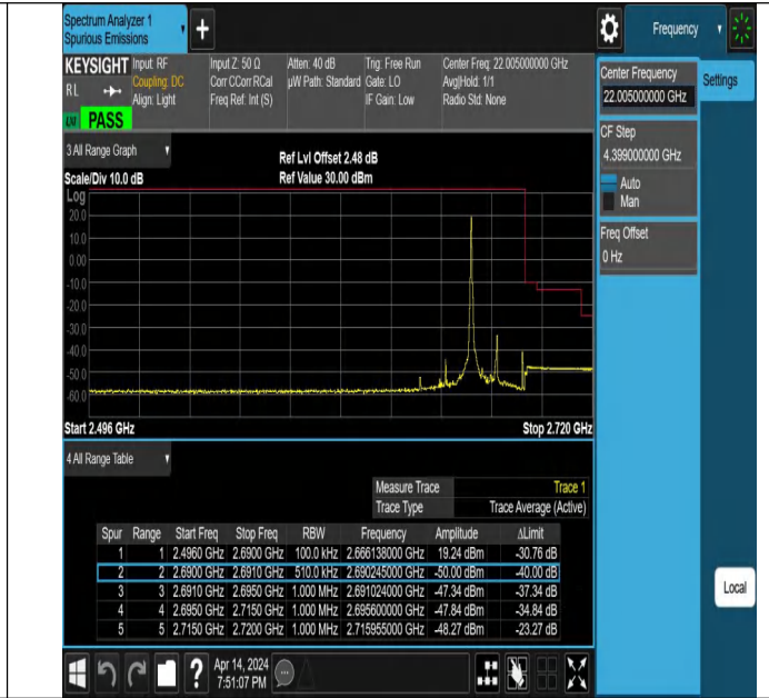
20MHz-5MHz_QPSK@QPSK-QPSK@QPSK_41440-41557_1R B#0@100RB#0-0RB#0@25RB#0
