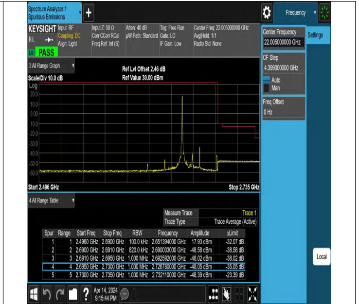
20MHz-20MHz_QPSK@QPSK-QPSK@QPSK_41292-41490_1RB#0@100RB#0-0RB#0@100RB#0
