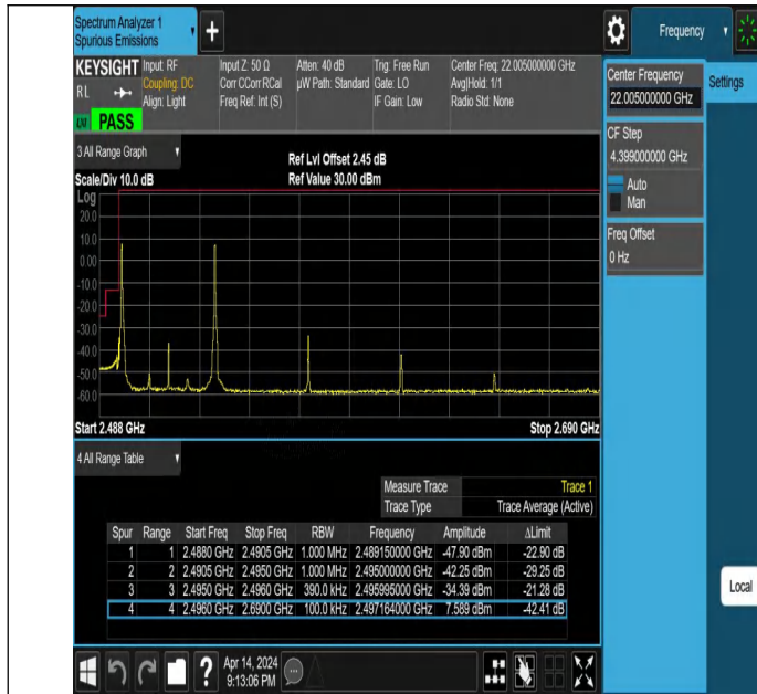
20MHz-20MHz_QPSK@QPSK-QPSK@QPSK_39750-39948_1RB #0@100RB#0-1RB#99@100RB#0
