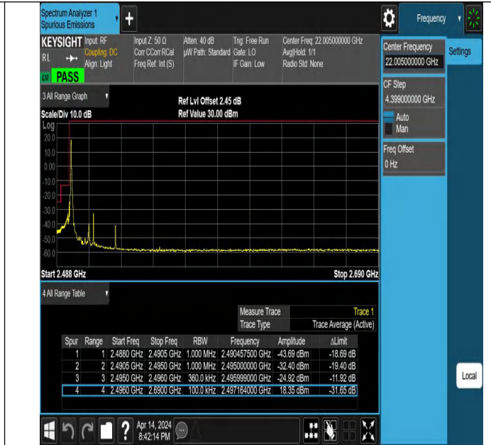
20MHz-15MHz_QPSK@QPSK-QPSK@QPSK_39750-39921_1 RB#0@100RB#0-0RB#0@75RB#0
