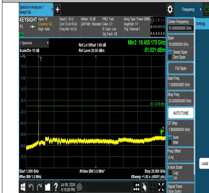
41-41-20MHz-5MHz-QPSK-QPSK-41440-41557-1RB#99-0RB#0- 1000~20000MHz-PASS
