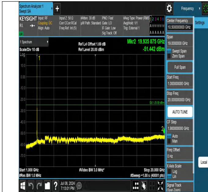
41-41-15MHz-10MHz-QPSK-QPSK-39725-39845-1RB#0-0RB#0-1000~20000MHz-PASS
