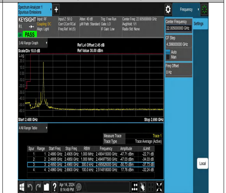
20MHz-10MHz_QPSK@QPSK-QPSK@QPSK_39750-39894_1RB#99@100RB#0-0RB#0@50RB#0
