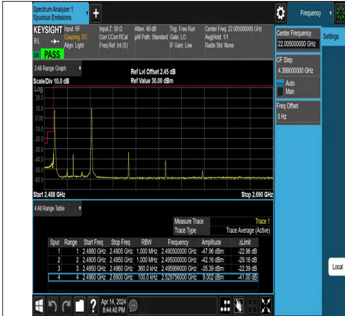
20MHz-15MHz_QPSK@QPSK-QPSK@QPSK_39750-39921_1RB #0@100RB#0-1RB#74@75RB#0
