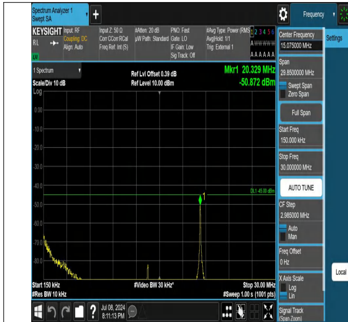
41-41-20MHz-5MHz-QPSK-QPSK-40595-40712-1RB#0-0RB#0-0 .15~30MHz-PASS
