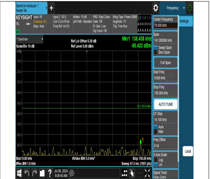
41-41-20MHz-5MHz-QPSK-QPSK-39750-39867-1RB#99-0RB#0- 0.009~0.15MHz-PASS
