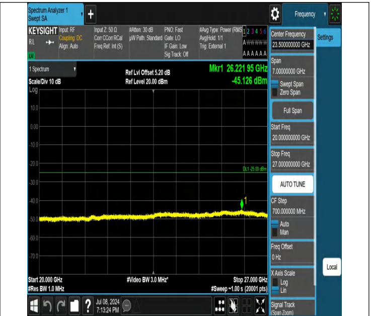
41-41-15MHz-10MHz-QPSK-QPSK-39725-39845-1RB#0-0RB#0-20000~27000MHz-PASS
