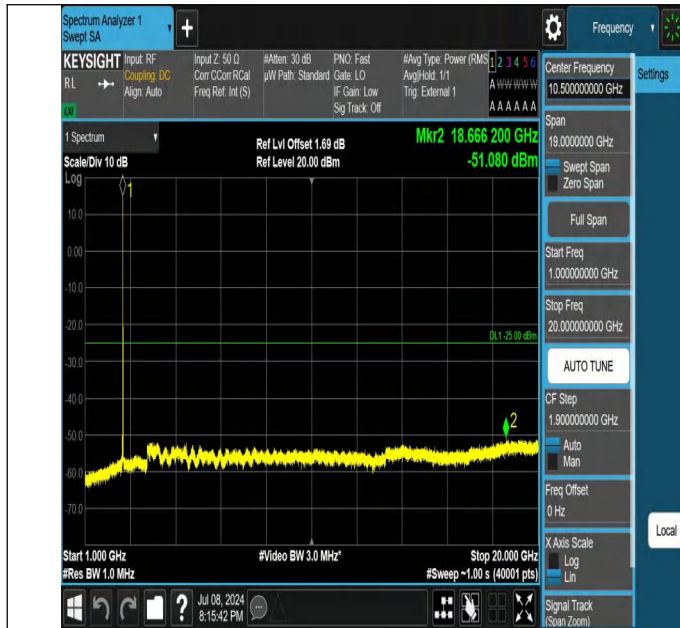
41-41-20MHz-5MHz-QPSK-QPSK-40595-40712-1RB#0-1RB#24- 1000~20000MHz-PASS
