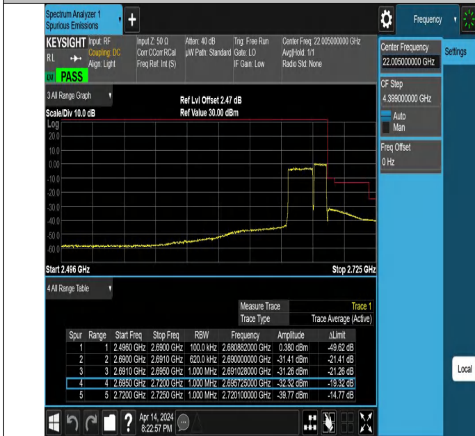
20MHz-10MHz_QPSK@QPSK-QPSK@QPSK_41391-41535_100RB#0@100RB#0-50RB#0@50RB#0
