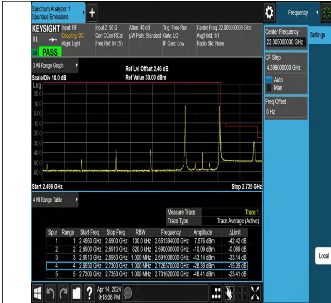
20MHz-20MHz_QPSK@QPSK-QPSK@QPSK_41292-41490_1RB #0@100RB#0-1RB#99@100RB#0
