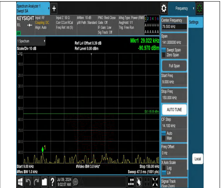
41-41-15MHz-10MHz-QPSK-QPSK-39725-39845-1RB#0-0RB#0-0.009~0.15MHz-PASS
