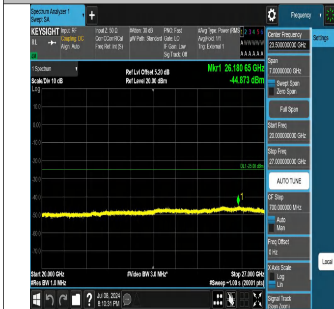
41-41-20MHz-5MHz-QPSK-QPSK-39750-39867-1RB#0-1RB#24- 20000~27000MHz-PASS
