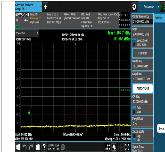
41-41-20MHz-5MHz-QPSK-QPSK-41440-41557-1RB#0-0RB#0-3 0~1000MHz-PASS
