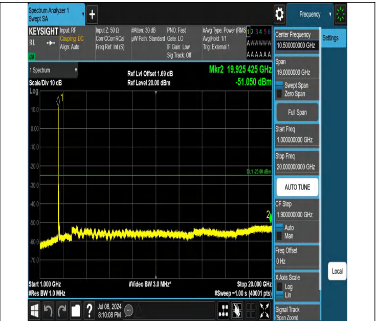
41-41-20MHz-5MHz-QPSK-QPSK-39750-39867-1RB#0-1RB#24- 1000~20000MHz-PASS
