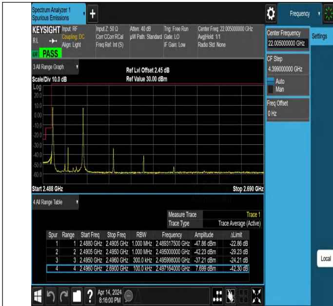
20MHz-10MHz_QPSK@QPSK-QPSK@QPSK_39750-39894_1RB#0@100RB#0-1RB#49@50RB#0
