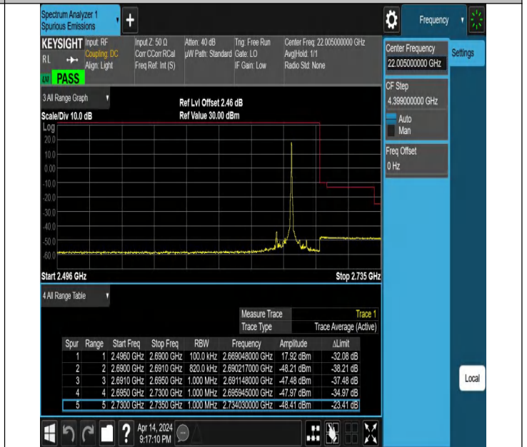
20MHz-20MHz_QPSK@QPSK-QPSK@QPSK_41292-41490_1RB#99@100RB#0-0RB#0@100RB#0
