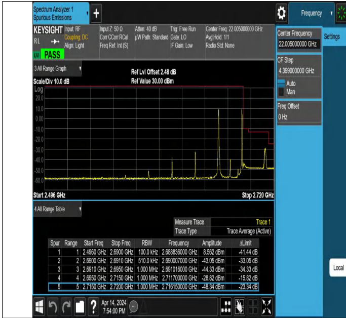
20MHz-5MHz_QPSK@QPSK-QPSK@QPSK_41440-41557_1RB# 0@100RB#0-1RB#24@25RB#0
