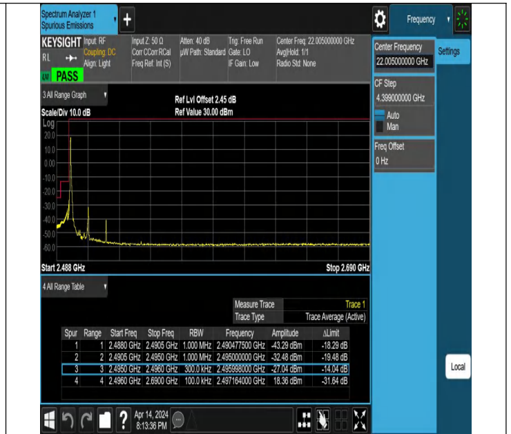
20MHz-10MHz_QPSK@QPSK-QPSK@QPSK_39750-39894_1RB#0@100RB#0-0RB#0@50RB#0
