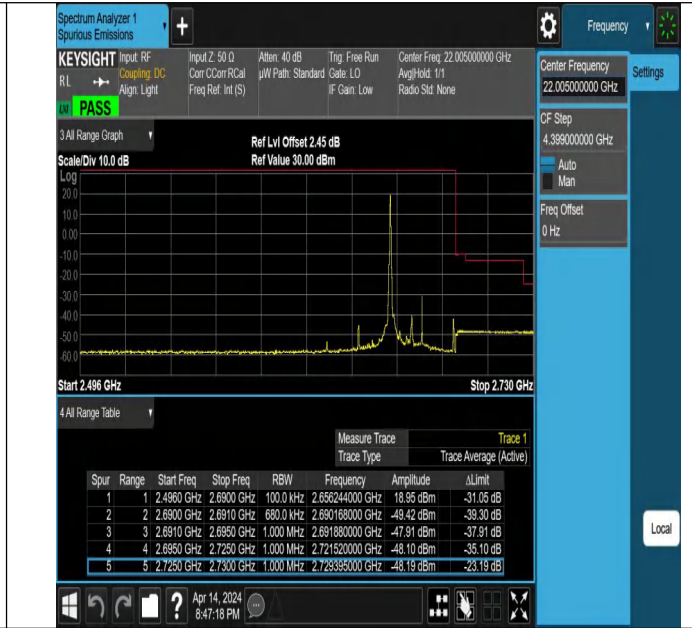
20MHz-15MHz_QPSK@QPSK-QPSK@QPSK_41341-41512_1RB#0@100RB#0-0RB#0@75RB#0
