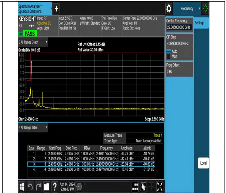
20MHz-20MHz_QPSK@QPSK-QPSK@QPSK_39750-39948_1RB#0@100RB#0-0RB#0@100RB#0
