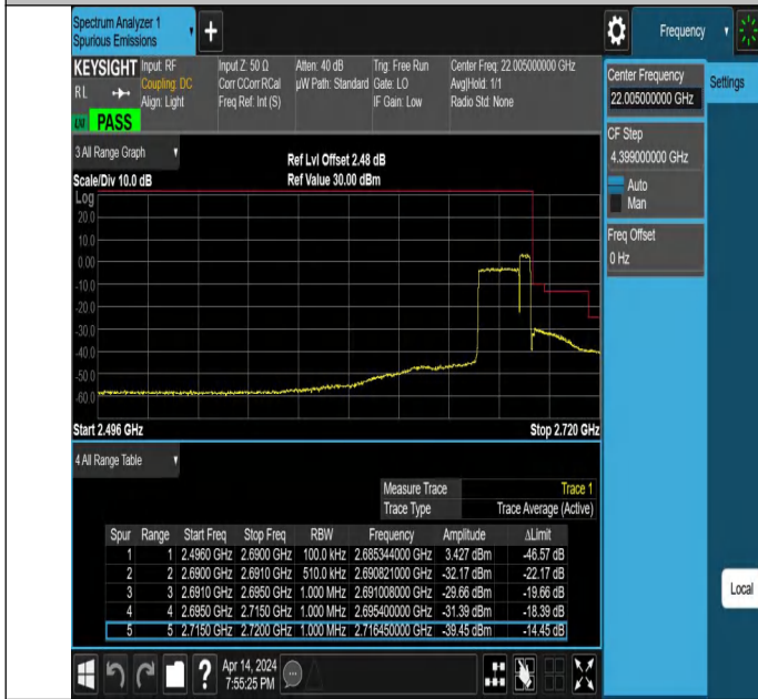
20MHz-5MHz_QPSK@QPSK-QPSK@QPSK_41440-41557_100R B#0@100RB#0-25RB#0@25RB#0
