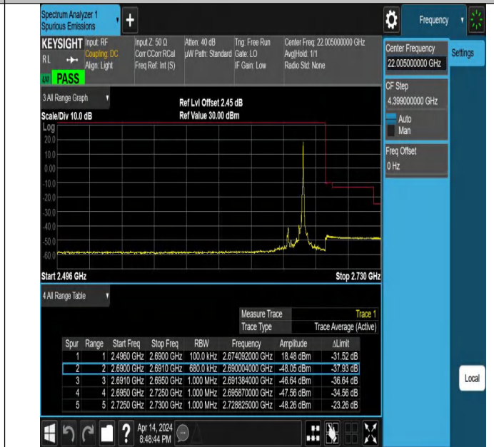
20MHz-15MHz_QPSK@QPSK-QPSK@QPSK_41341-41512_1RB#99@100RB#0-0RB#0@75RB#0
