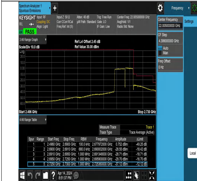
20MHz-15MHz_QPSK@QPSK-QPSK@QPSK_41341-41512_100RB#0@100RB#0-75RB#0@75RB#0
