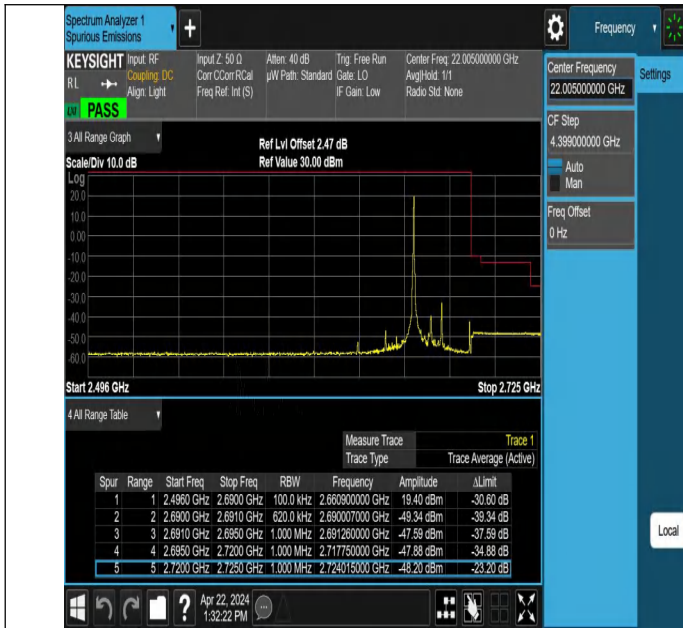
15MHz-15MHz_QPSK@QPSK-QPSK@QPSK_41365-41515_1RB #0@75RB#0-0RB#0@75RB#0
