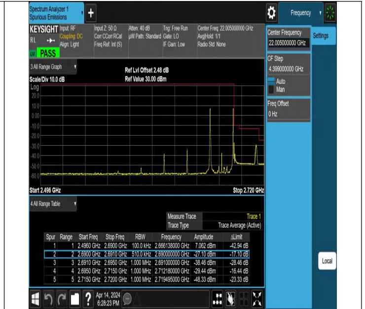
15MHz-10MHz_QPSK@QPSK-QPSK@QPSK_41417-41537_1 RB#0@75RB#0-1RB#49@50RB#0
