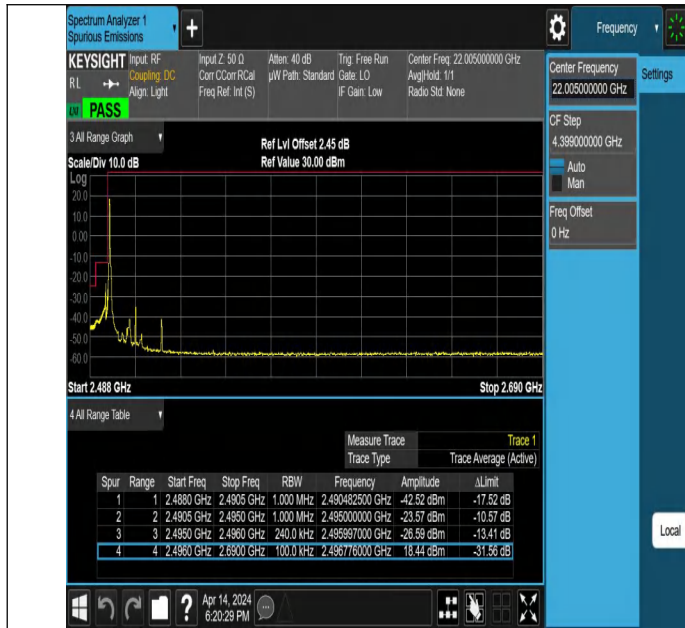
15MHz-10MHz_QPSK@QPSK-QPSK@QPSK_39725-39845_1RB #0@75RB#0-0RB#0@50RB#0
