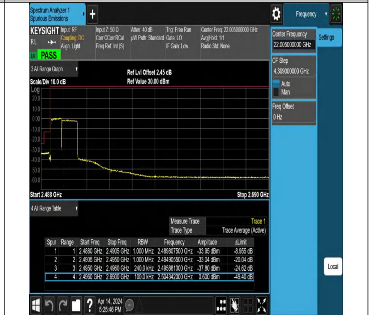
10MHz-15MHz_QPSK@QPSK-QPSK@QPSK_39703-39823_50 RB#0@50RB#0-75RB#0@75RB#0
