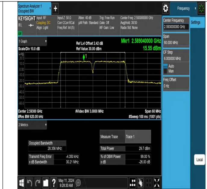
41-41-15MHz-15MHz-64QAM-64QAM-40545-40695-75RB#0-75RB#0-PASS
