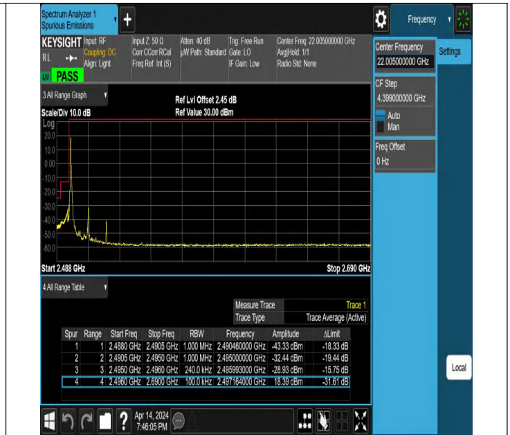
20MHz-5MHz_QPSK@QPSK-QPSK@QPSK_39750-39867_1R B#0@100RB#0-0RB#0@25RB#0
