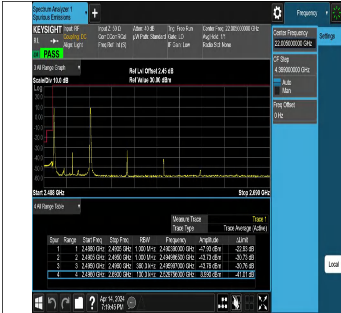
15MHz-20MHz_QPSK@QPSK-QPSK@QPSK_39728-39899_1RB #0@75RB#0-1RB#99@100RB#0
