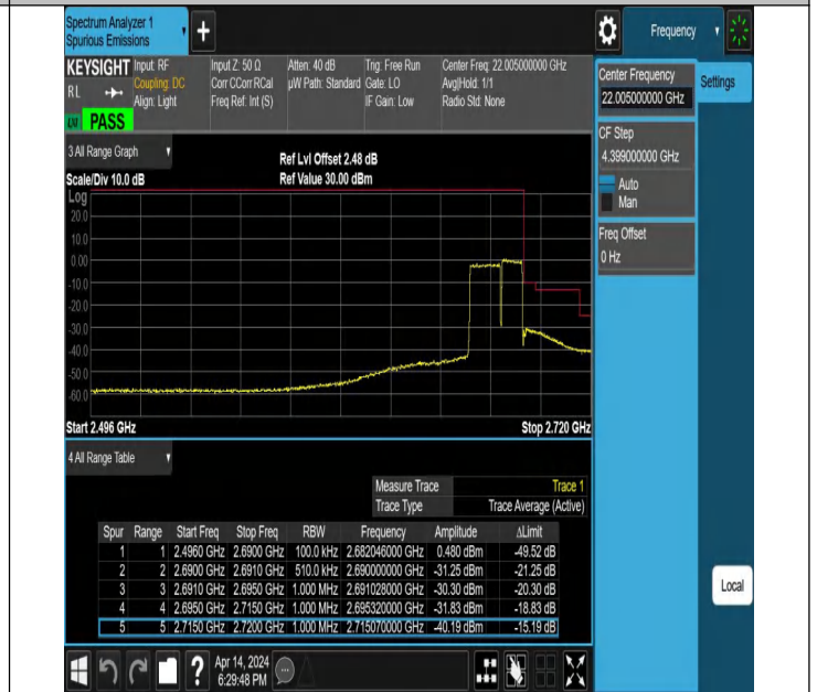
15MHz-10MHz_QPSK@QPSK-QPSK@QPSK_41417-41537_75 RB#0@75RB#0-50RB#0@50RB#0
