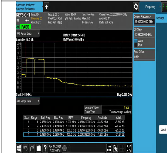
15MHz-20MHz_QPSK@QPSK-QPSK@QPSK_39728-39899_75R B#0@75RB#0-100RB#0@100RB#0
