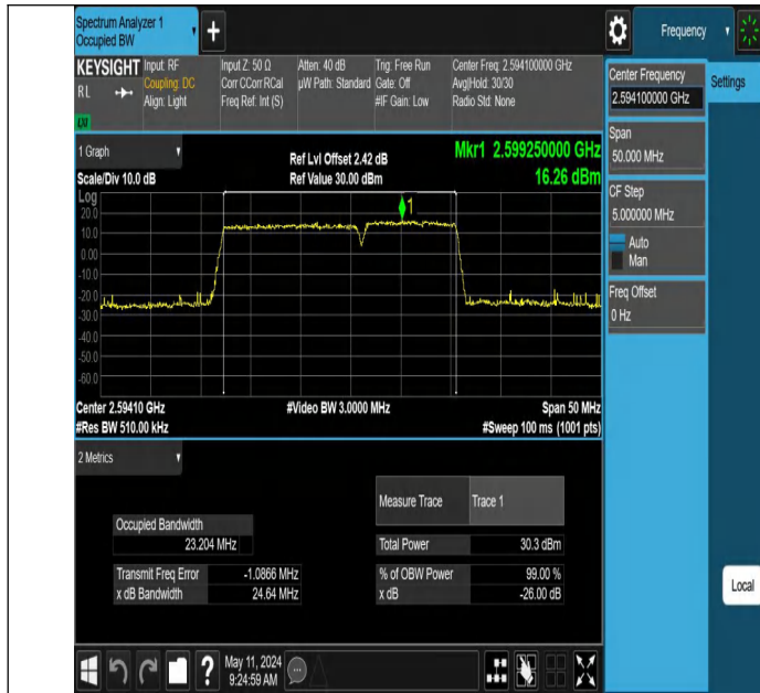
41-41-15MHz-10MHz-QPSK-QPSK-40571-40691-75RB#0-50RB#0-PASS
