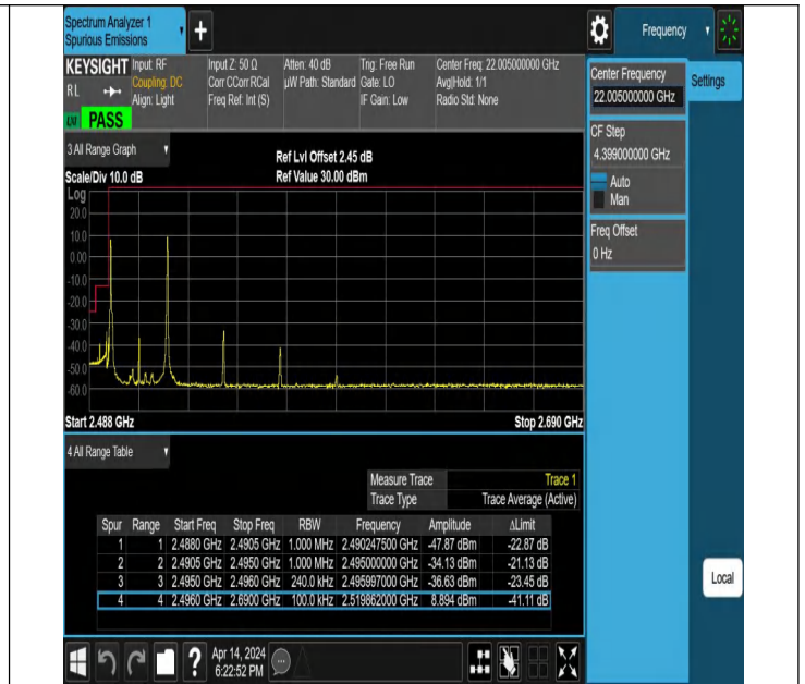
15MHz-10MHz_QPSK@QPSK-QPSK@QPSK_39725-39845_1 RB#0@75RB#0-1RB#49@50RB#0
