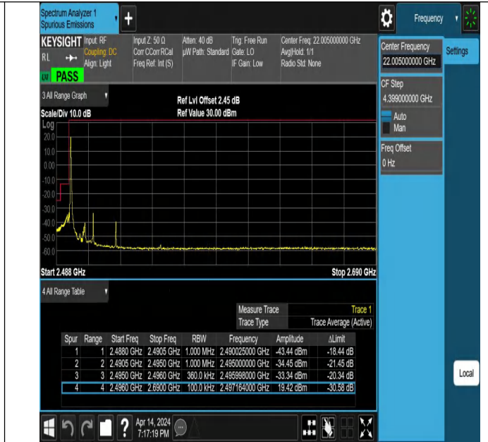
15MHz-20MHz_QPSK@QPSK-QPSK@QPSK_39728-39899_1 RB#0@75RB#0-0RB#0@100RB#0
