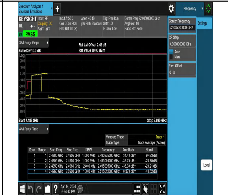
15MHz-10MHz_QPSK@QPSK-QPSK@QPSK_39725-39845_75 RB#0@75RB#0-50RB#0@50RB#0
