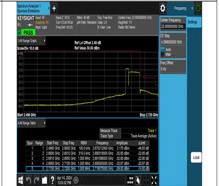
5MHz-20MHz_QPSK@QPSK-QPSK@QPSK_41373-41490_25 RB#0@25RB#0-100RB#0@100RB#0
