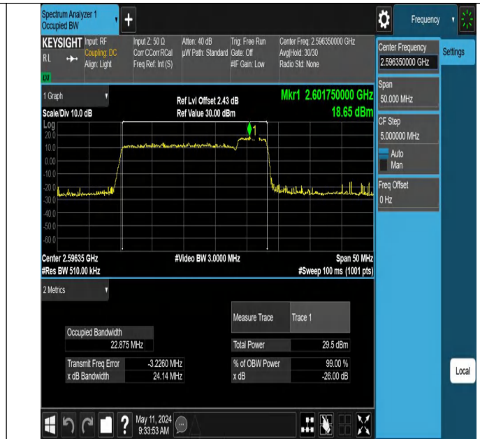
41-41-20MHz-5MHz-64QAM-64QAM-40595-40712-100RB#0-25RB#0-PASS
