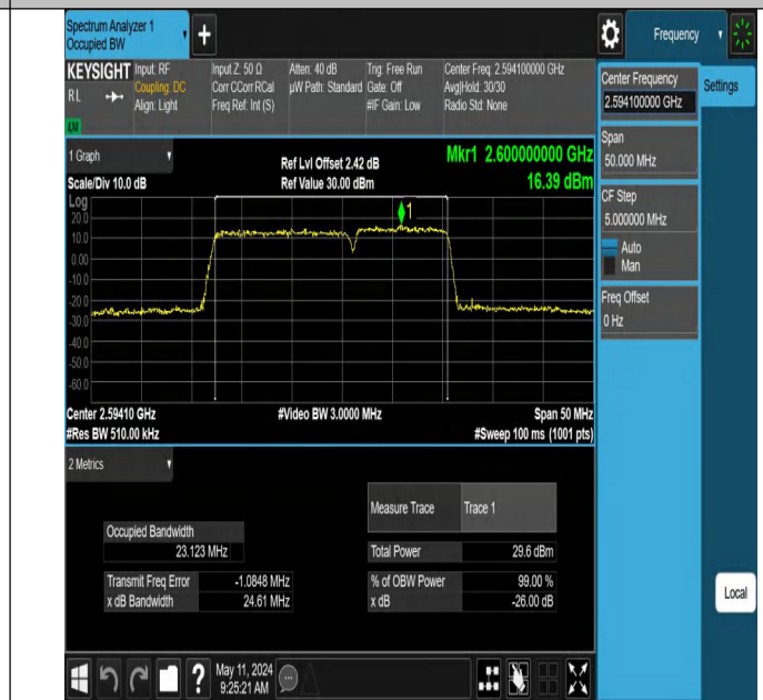
41-41-15MHz-10MHz-16QAM-16QAM-40571-40691-75RB#0-50RB#0-PASS
