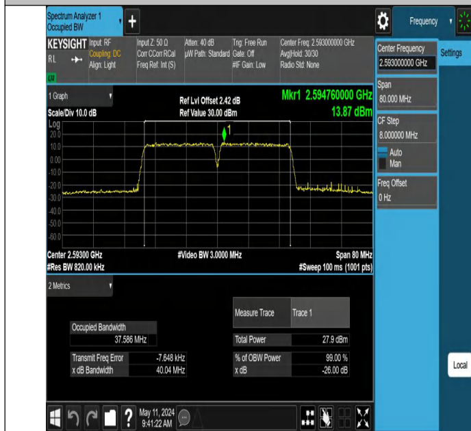
41-41-20MHz-20MHz-256QAM-256QAM-40521-40719-100RB#0-100RB#0-PASS
