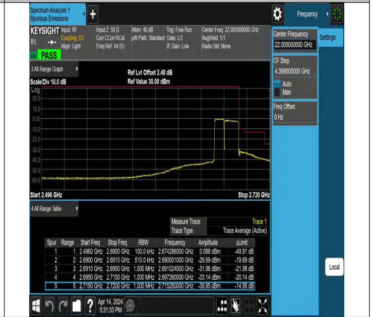
10MHz-15MHz_QPSK@QPSK-QPSK@QPSK_41395-41515_50 RB#0@50RB#0-75RB#0@75RB#0
