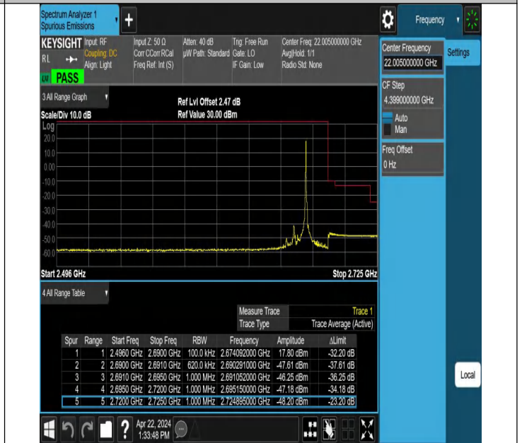
15MHz-15MHz_QPSK@QPSK-QPSK@QPSK_41365-41515_1 RB#74@75RB#0-0RB#0@75RB#0
