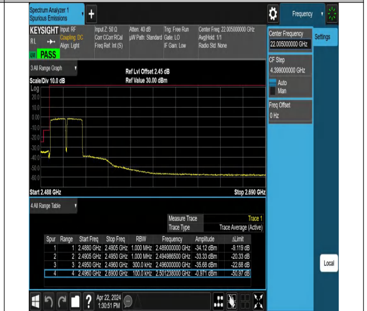
15MHz-15MHz_QPSK@QPSK-QPSK@QPSK_39725-39875_75 RB#0@75RB#0-75RB#0@75RB#0
