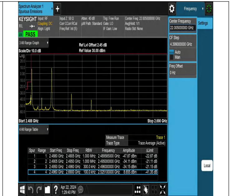
15MHz-15MHz_QPSK@QPSK-QPSK@QPSK_39725-39875_1 RB#0@75RB#0-1RB#74@75RB#0
