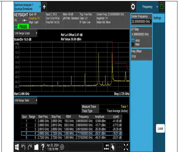
15MHz-15MHz_QPSK@QPSK-QPSK@QPSK_41365-41515_1 RB#0@75RB#0-1RB#74@75RB#0
