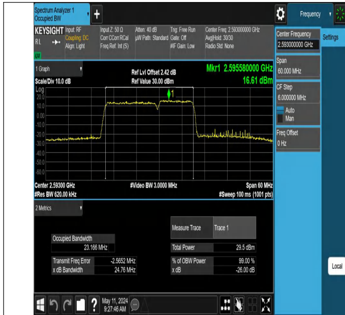
41-41-15MHz-15MHz-QPSK-QPSK-40545-40695-75RB#0-75RB#0-PASS
