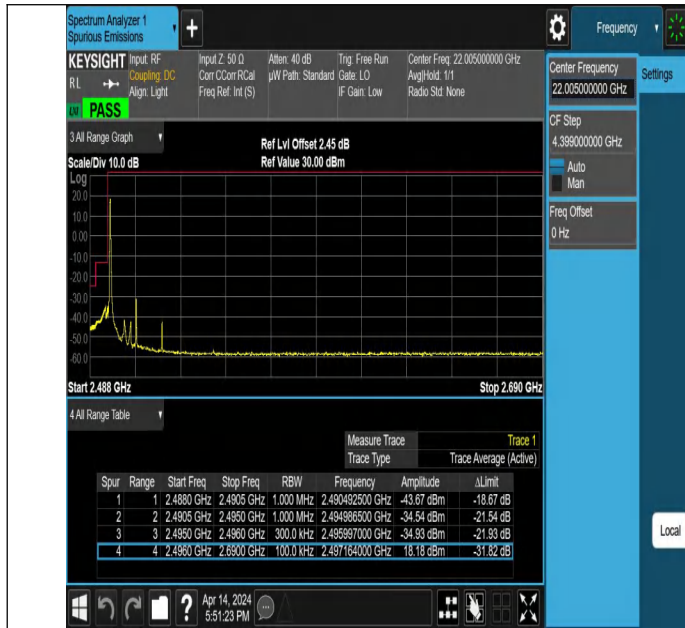
10MHz-20MHz_QPSK@QPSK-QPSK@QPSK_39705-39849_1RB #0@50RB#0-0RB#0@100RB#0
