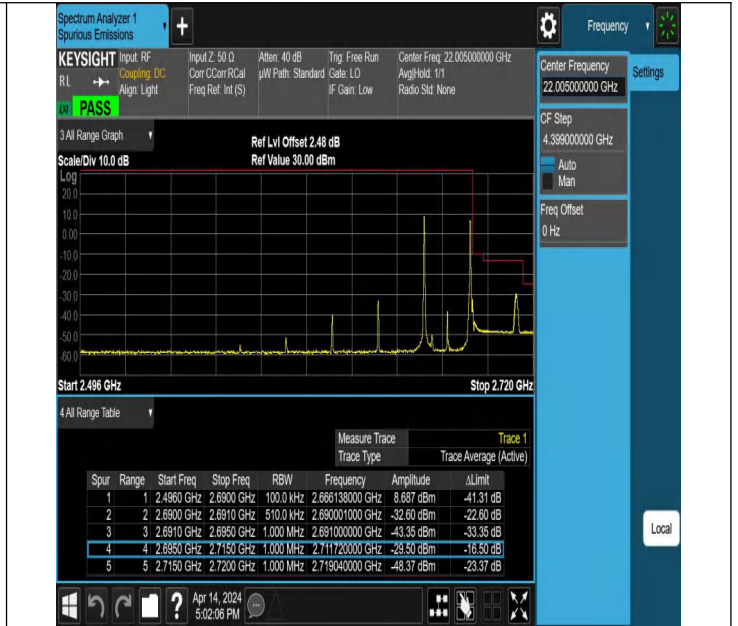
5MHz-20MHz_QPSK@QPSK-QPSK@QPSK_41373-41490_1R B#0@25RB#0-1RB#99@100RB#0
