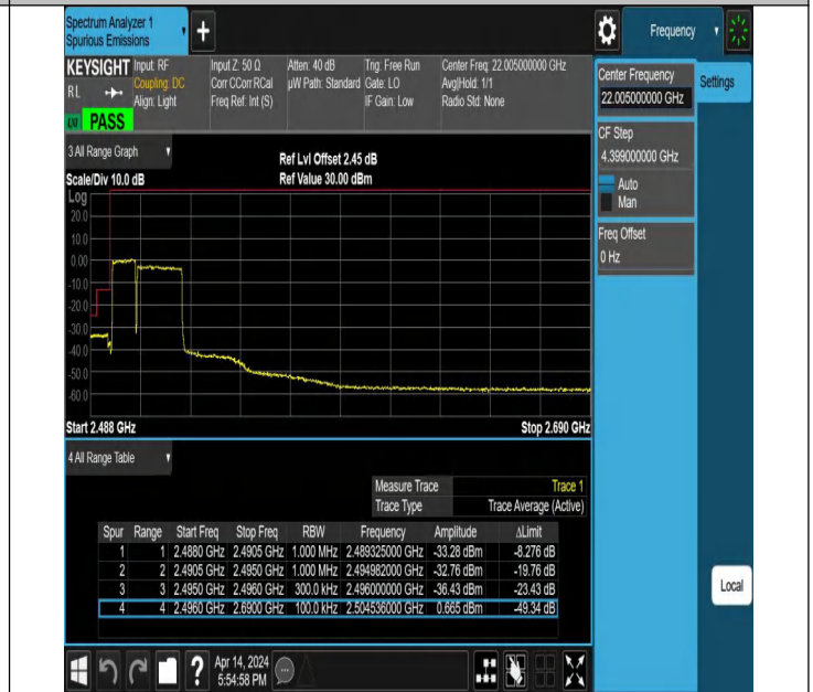
10MHz-20MHz_QPSK@QPSK-QPSK@QPSK_39705-39849_50 RB#0@50RB#0-100RB#0@100RB#0
