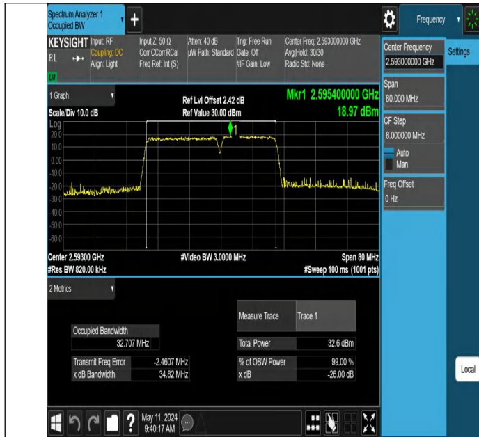
41-41-20MHz-20MHz-QPSK-QPSK-40521-40719-100RB#0-100RB#0-PASS
