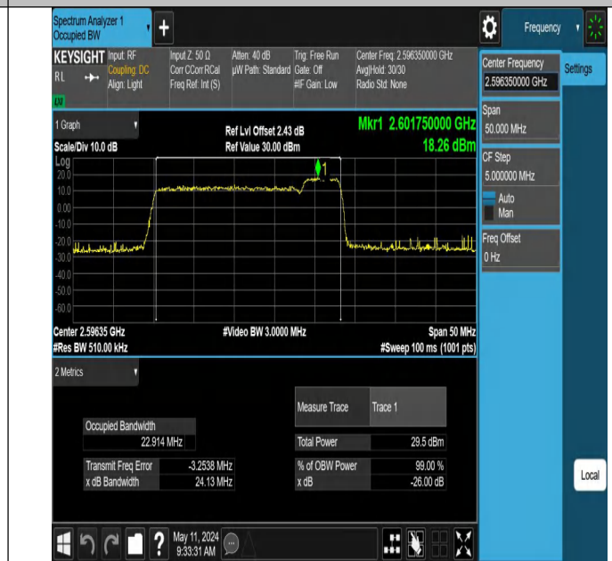
41-41-20MHz-5MHz-16QAM-16QAM-40595-40712-100RB#0-25RB#0-PASS
