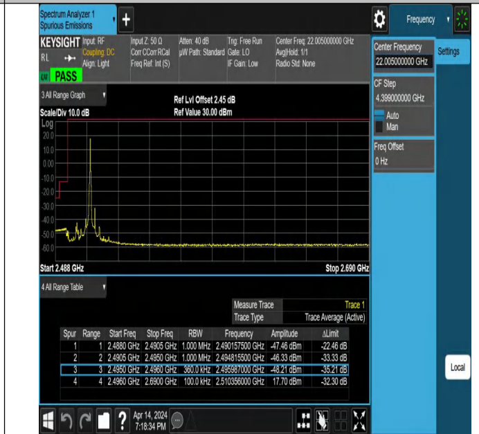
15MHz-20MHz_QPSK@QPSK-QPSK@QPSK_39728-39899_1 RB#74@75RB#0-0RB#0@100RB#0
