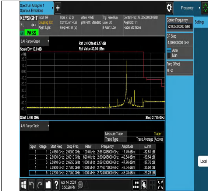
10MHz-20MHz_QPSK@QPSK-QPSK@QPSK_41346-41490_1RB #0@50RB#0-0RB#0@100RB#0
