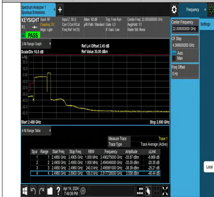
20MHz-5MHz_QPSK@QPSK-QPSK@QPSK_39750-39867_100R B#0@100RB#0-25RB#0@25RB#0
