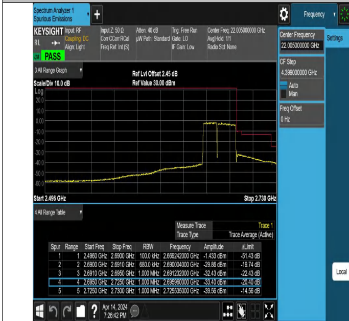
15MHz-20MHz_QPSK@QPSK-QPSK@QPSK_41319-41490_75R B#0@75RB#0-100RB#0@100RB#0
