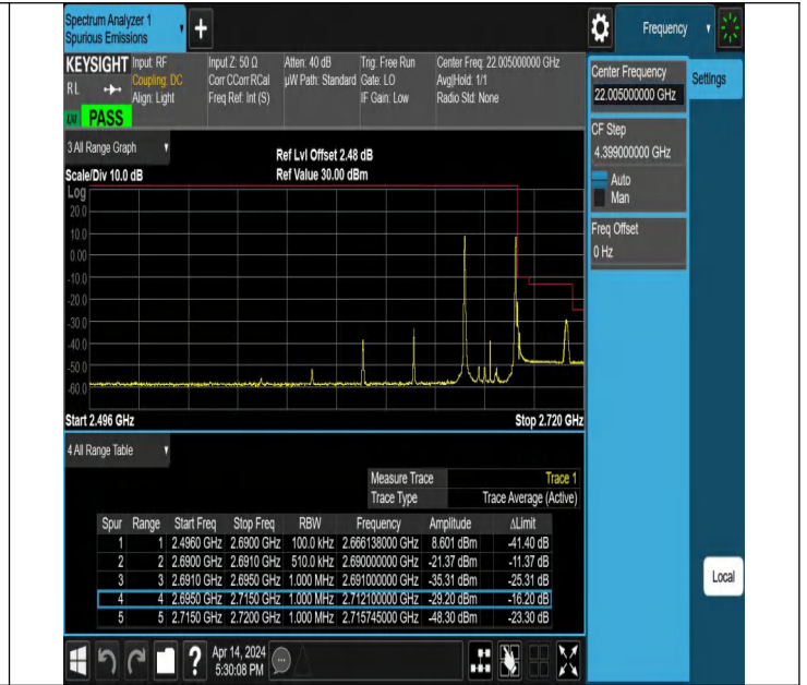
10MHz-15MHz_QPSK@QPSK-QPSK@QPSK_41395-41515_1 RB#0@50RB#0-1RB#74@75RB#0
