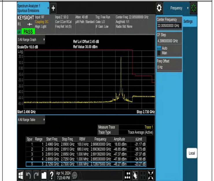
15MHz-20MHz_QPSK@QPSK-QPSK@QPSK_41319-41490_1 RB#74@75RB#0-0RB#0@100RB#0
