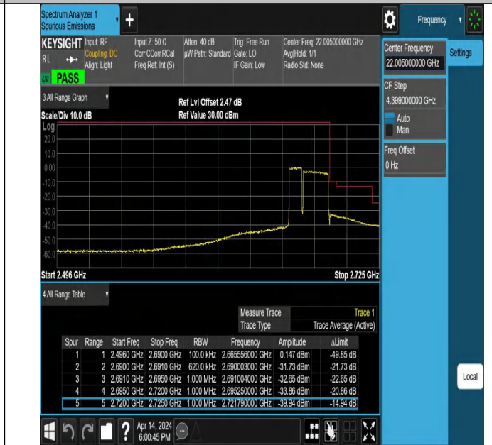
10MHz-20MHz_QPSK@QPSK-QPSK@QPSK_41346-41490_50 RB#0@50RB#0-100RB#0@100RB#0
