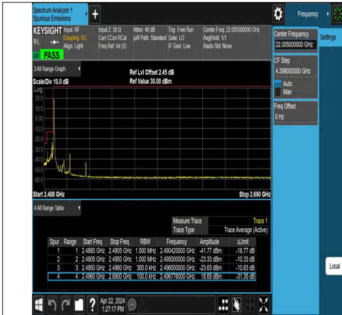
15MHz-15MHz_QPSK@QPSK-QPSK@QPSK_39725-39875_1RB #0@75RB#0-0RB#0@75RB#0
