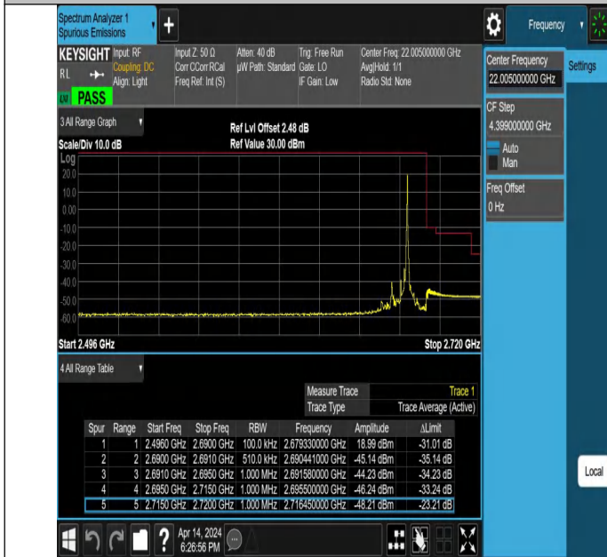
15MHz-10MHz_QPSK@QPSK-QPSK@QPSK_41417-41537_1RB #74@75RB#0-0RB#0@50RB#0
