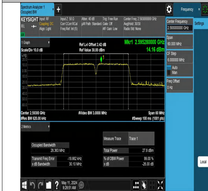
41-41-15MHz-15MHz-256QAM-256QAM-40545-40695-75RB#0-75RB#0-PASS
