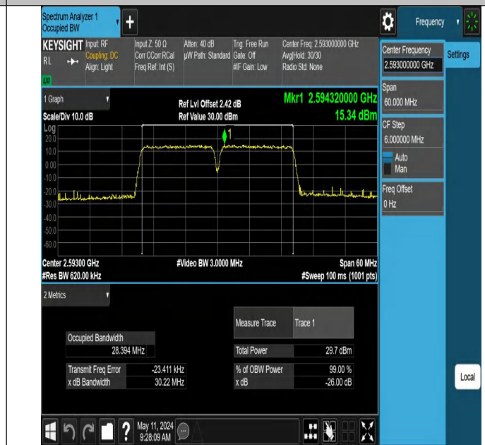
41-41-15MHz-15MHz-16QAM-16QAM-40545-40695-75RB#0-75RB#0-PASS
