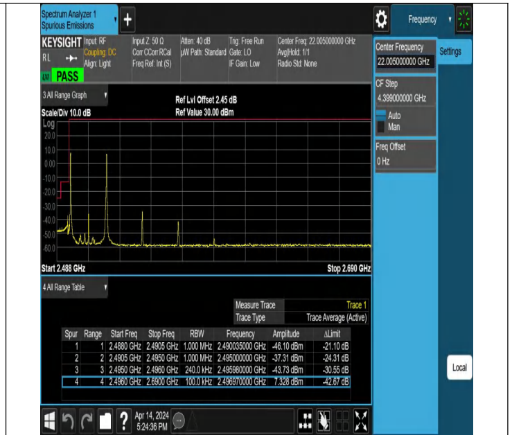
10MHz-15MHz_QPSK@QPSK-QPSK@QPSK_39703-39823_1 RB#0@50RB#0-1RB#74@75RB#0
