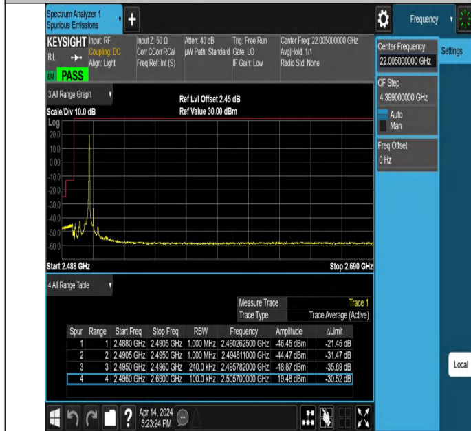
10MHz-15MHz_QPSK@QPSK-QPSK@QPSK_39703-39823_1RB #49@50RB#0-0RB#0@75RB#0
