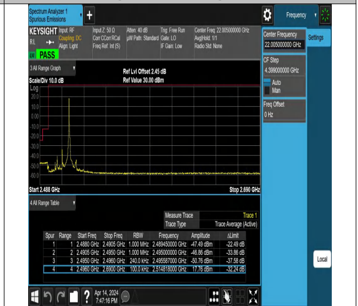
20MHz-5MHz_QPSK@QPSK-QPSK@QPSK_39750-39867_1R B#99@100RB#0-0RB#0@25RB#0
