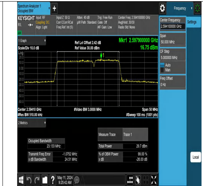
41-41-15MHz-10MHz-64QAM-64QAM-40571-40691-75RB#0-50RB#0-PASS
