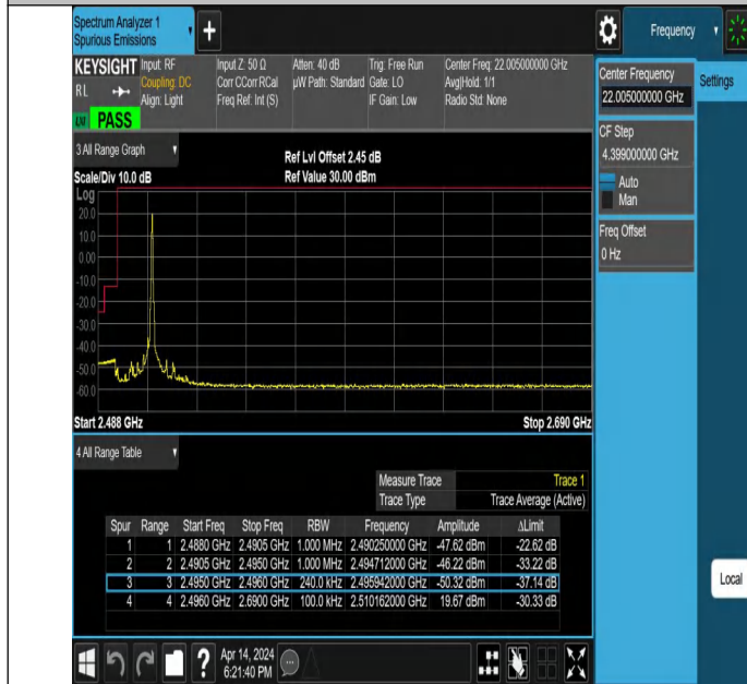
15MHz-10MHz_QPSK@QPSK-QPSK@QPSK_39725-39845_1RB #74@75RB#0-0RB#0@50RB#0
