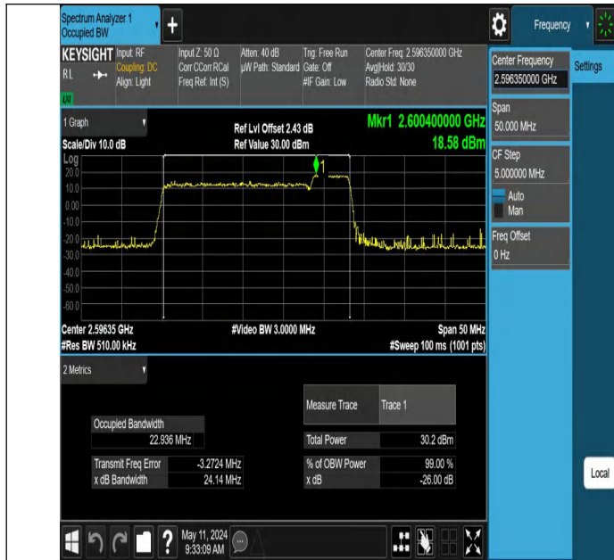
41-41-20MHz-5MHz-QPSK-QPSK-40595-40712-100RB#0-25RB#0-PASS
