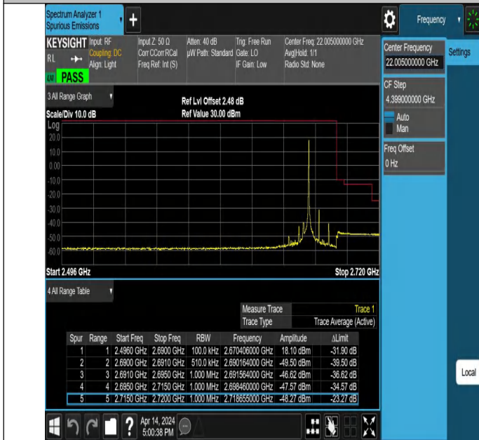
5MHz-20MHz_QPSK@QPSK-QPSK@QPSK_41373-41490_1RB# 24@25RB#0-0RB#0@100RB#0
