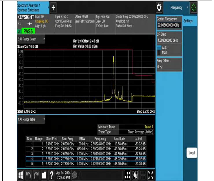
15MHz-20MHz_QPSK@QPSK-QPSK@QPSK_41319-41490_1 RB#0@75RB#0-0RB#0@100RB#0
