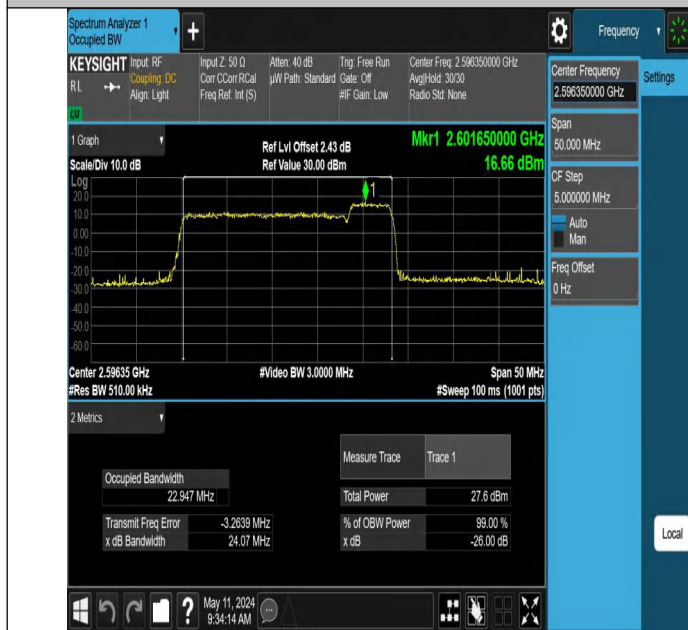
41-41-20MHz-5MHz-256QAM-256QAM-40595-40712-100RB#0-25RB#0-PASS
