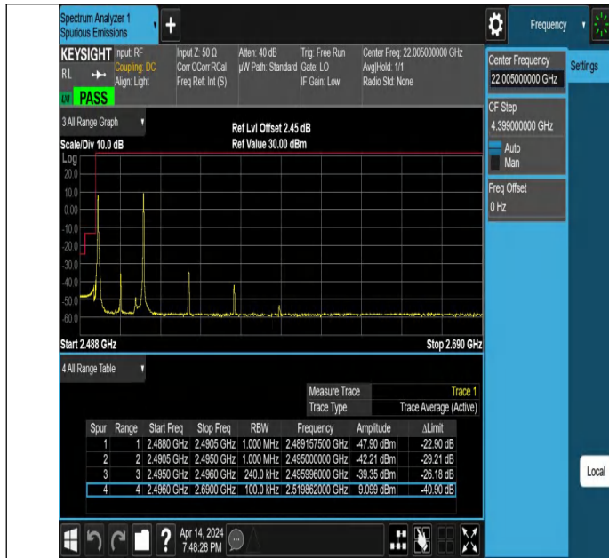
20MHz-5MHz_QPSK@QPSK-QPSK@QPSK_39750-39867_1RB# 0@100RB#0-1RB#24@25RB#0
