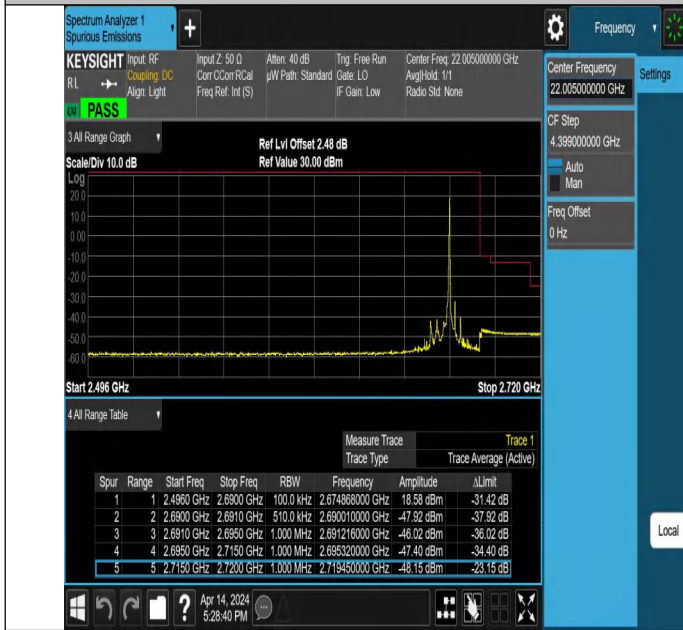
10MHz-15MHz_QPSK@QPSK-QPSK@QPSK_41395-41515_1RB #49@50RB#0-0RB#0@75RB#0
