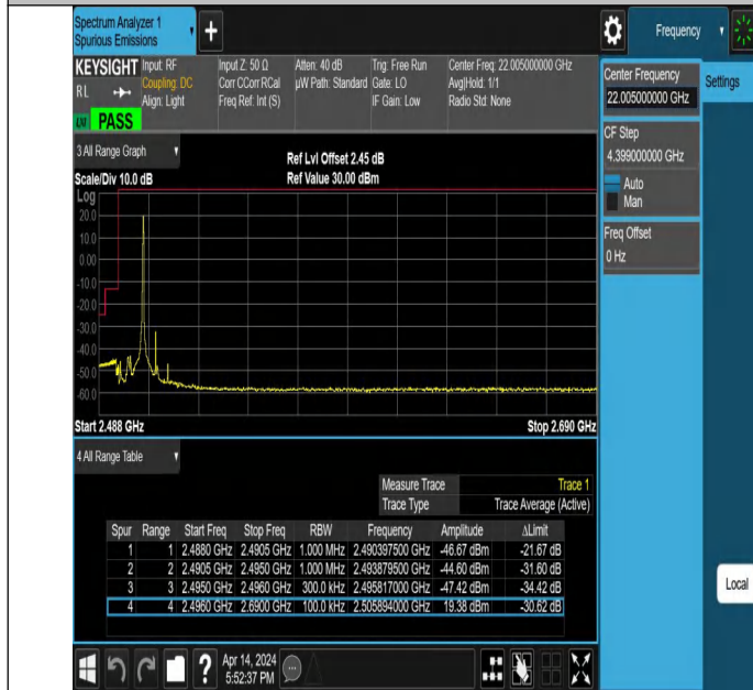
10MHz-20MHz_QPSK@QPSK-QPSK@QPSK_39705-39849_1RB #49@50RB#0-0RB#0@100RB#0
