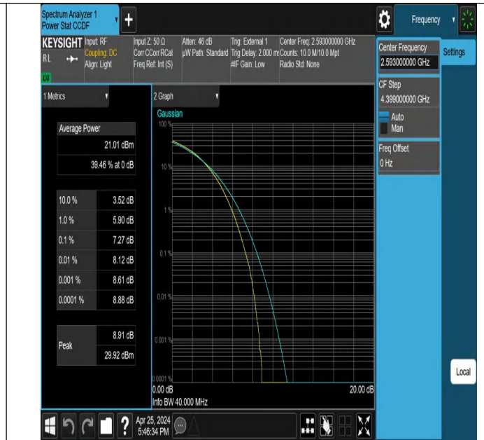
41-41-20MHz-20MHz-64QAM-64QAM-40521-40719-100RB#0-100RB#0-PASS
