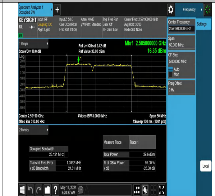
41-41-10MHz-15MHz-16QAM-16QAM-40549-40669-50RB#0-75RB#0-PASS
