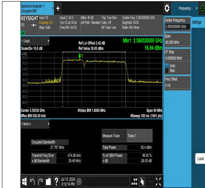
41-41-10MHz-20MHz-QPSK-QPSK-40526-40670-50RB#0-100RB #0-PASS
