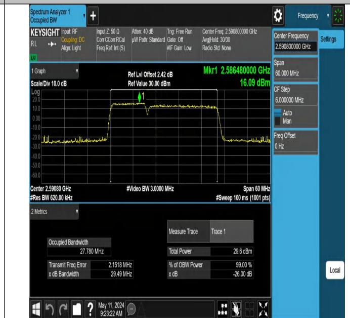
41-41-10MHz-20MHz-16QAM-16QAM-40526-40670-50RB#0-10 ORB#0-PASS
