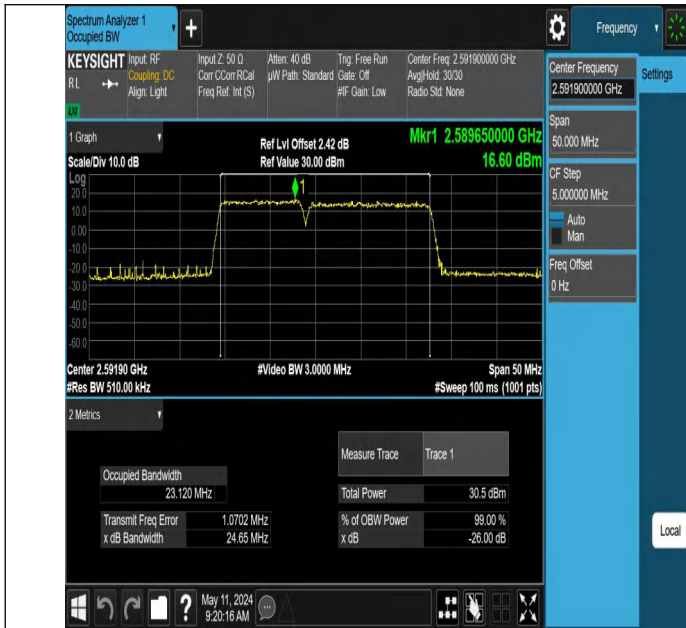
41-41-10MHz-15MHz-QPSK-QPSK-40549-40669-50RB#0-75RB#0-PASS
