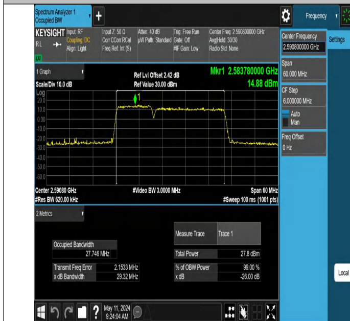
41-41-10MHz-20MHz-256QAM-256QAM-40526-40670-50RB#0-10 ORB#0-PASS
