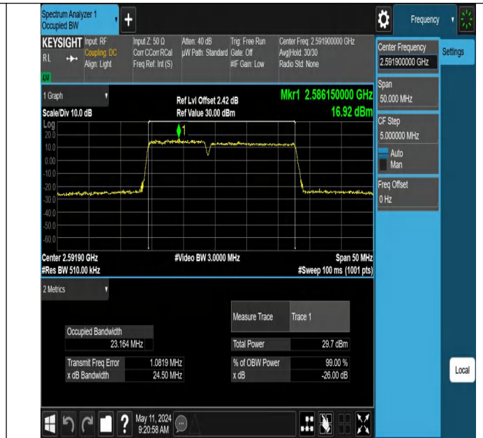
41-41-10MHz-15MHz-64QAM-64QAM-40549-40669-50RB#0-75RB#0-PASS
