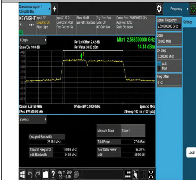
41-41-10MHz-15MHz-256QAM-256QAM-40549-40669-50RB#0-75RB#0-PASS
