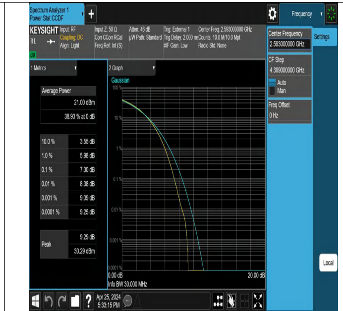
41-41-15MHz-15MHz-64QAM-64QAM-40545-40695-75RB#0-75RB#0-PASS
