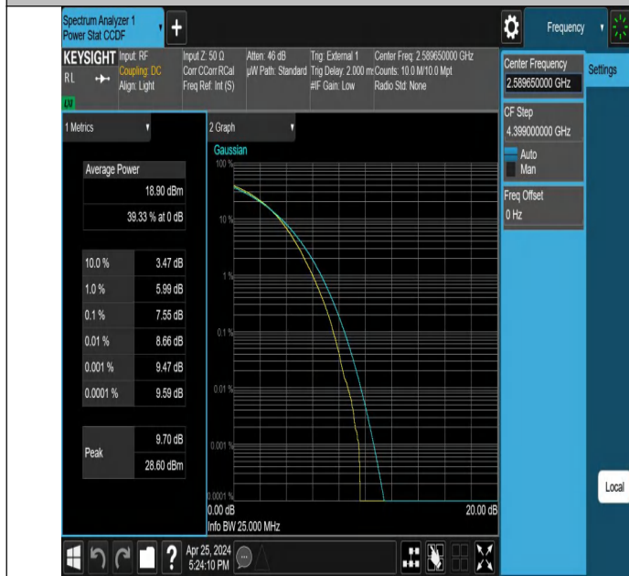
41-41-5MHz-20MHz-256QAM-256QAM-40528-40645-25RB#0-100RB#0-PASS
