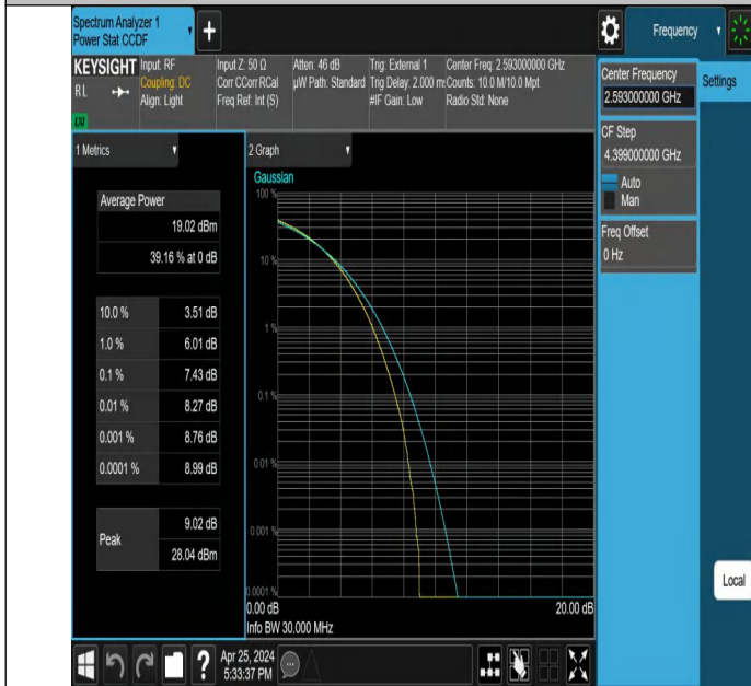
41-41-15MHz-15MHz-256QAM-256QAM-40545-40695-75RB#0-75RB#0-PASS
