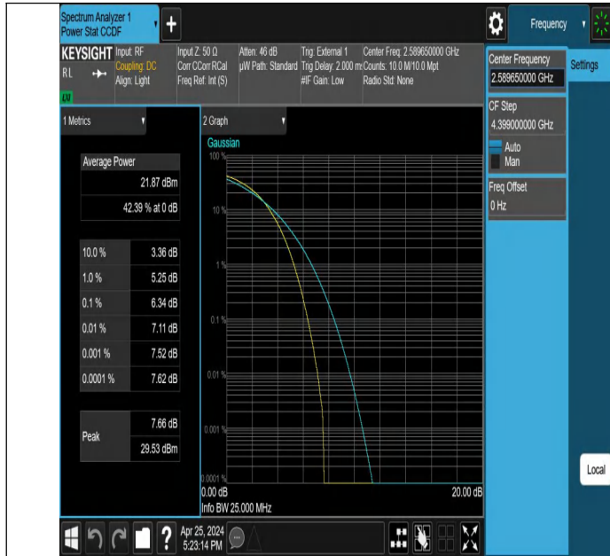
41-41-5MHz-20MHz-QPSK-QPSK-40528-40645-25RB#0-100RB#0-PASS
