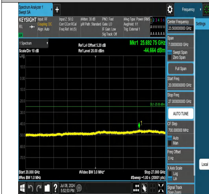
38-38-15MHz-15MHz-QPSK-QPSK-38025-38175-1RB#0-0RB#0-20000~27000MHz-PASS
