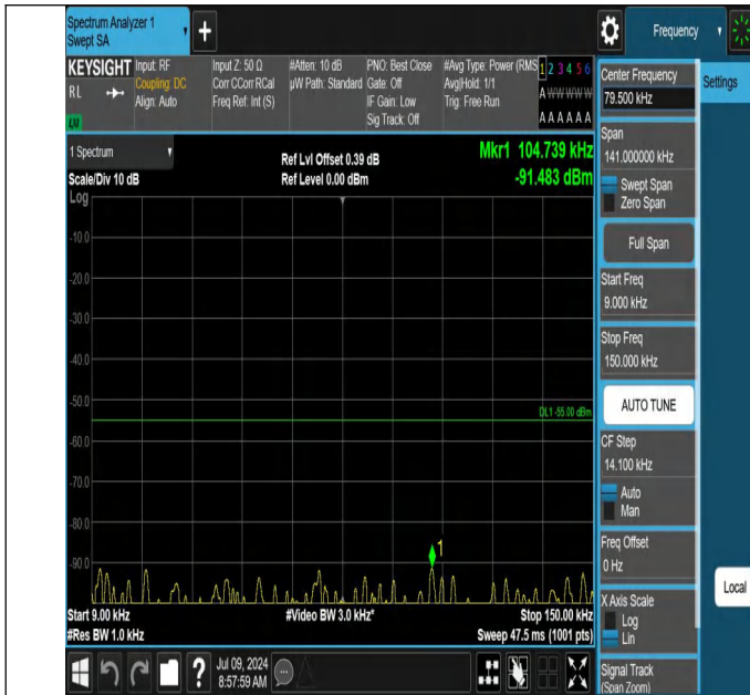
38-38-15MHz-15MHz-QPSK-QPSK-38025-38175-1RB#0-1RB#7 4-0.009~0.15MHz-PASS
