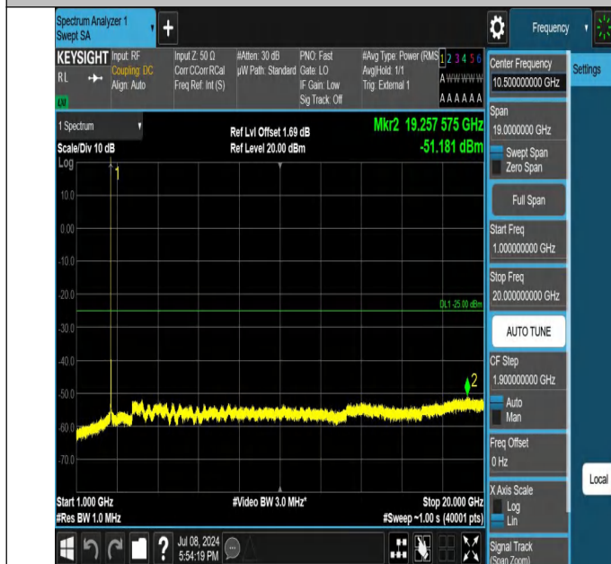
38-38-15MHz-15MHz-QPSK-QPSK-38025-38175-1RB#74-0RB# 0-1000~20000MHz-PASS
