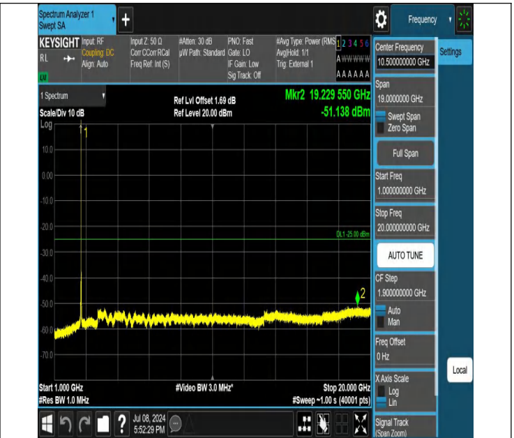
38-38-15MHz-15MHz-QPSK-QPSK-38025-38175-1RB#0-0RB#0-1000~20000MHz-PASS
