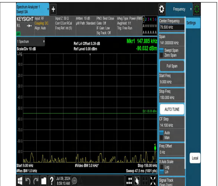
38-38-20MHz-20MHz-QPSK-QPSK-37952-38150-1RB#0-1RB#9 9-0.009~0.15MHz-PASS
