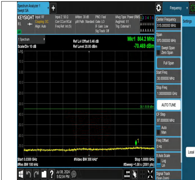
38-38-15MHz-15MHz-QPSK-QPSK-38025-38175-1RB#0-0RB#0-30~1000MHz-PASS
