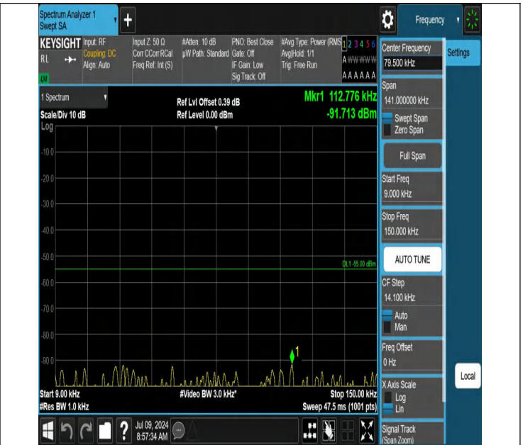
38-38-15MHz-15MHz-QPSK-QPSK-37925-38075-1RB#0-1RB#7 4-0.009~0.15MHz-PASS
