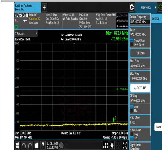
38-38-15MHz-15MHz-QPSK-QPSK-38025-38175-1RB#0-1RB#7 4-30~1000MHz-PASS
