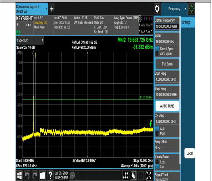
38-38-15MHz-15MHz-QPSK-QPSK-38025-38175-1RB#0-1RB#7 4-1000~20000MHz-PASS
