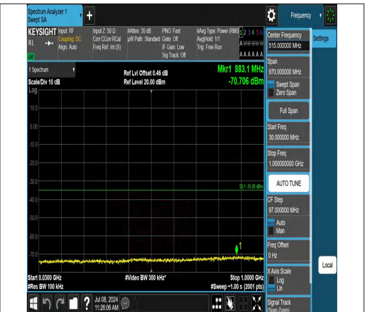
7-7-15MHz-20MHz-QPSK-QPSK-20828-20999-1RB#0-1RB#99-3 0~1000MHz-PASS
