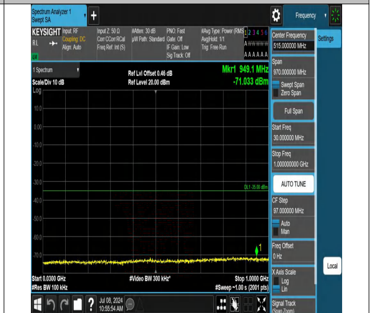
7-7-10MHz-20MHz-QPSK-QPSK-21006-21150-1RB#0-1RB#99-3 0~1000MHz-PASS
