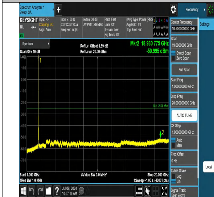
7-7-10MHz-20MHz-QPSK-QPSK-21206-21350-1RB#49-0RB#0-1 000~20000MHz-PASS
