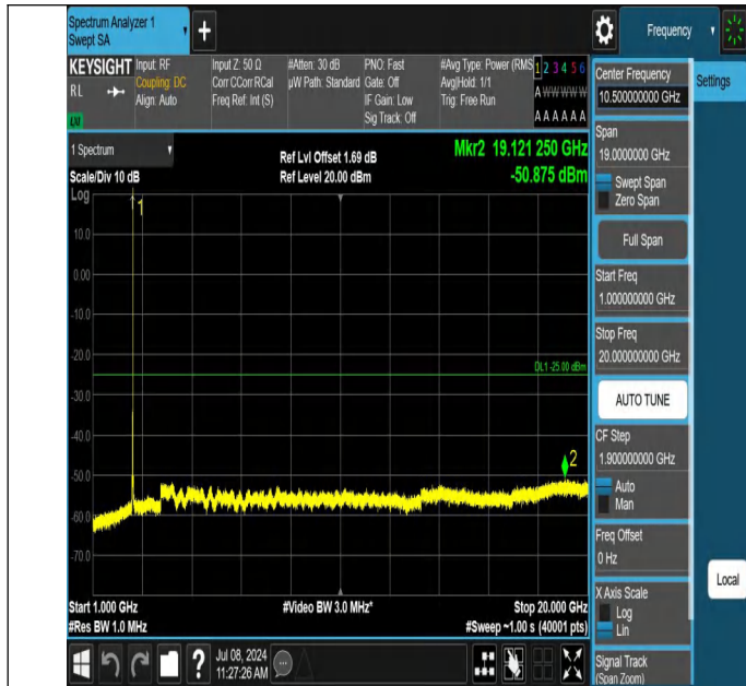
7-7-15MHz-20MHz-QPSK-QPSK-21003-21174-1RB#74-0RB#0-1 000~20000MHz-PASS
