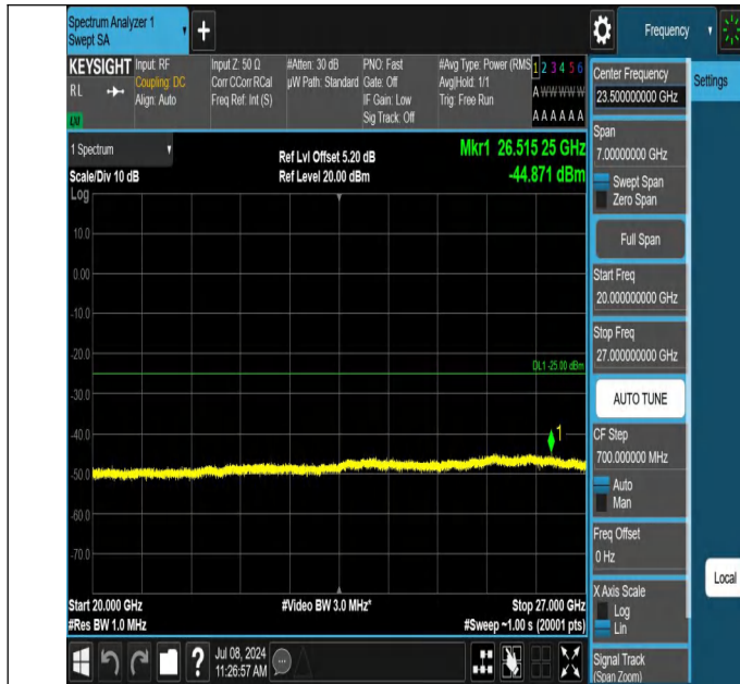
7-7-15MHz-20MHz-QPSK-QPSK-21003-21174-1RB#0-0RB#0-20 000~27000MHz-PASS
