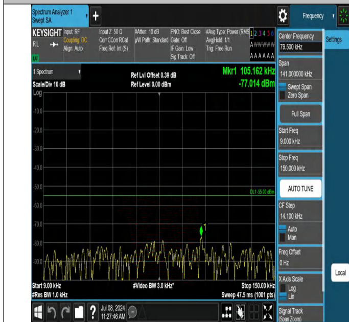
7-7-15MHz-20MHz-QPSK-QPSK-21003-21174-1RB#0-1RB#99-0 .009~0.15MHz-PASS
