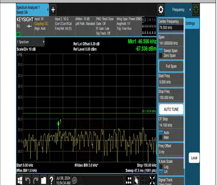
7-7-10MHz-20MHz-QPSK-QPSK-21006-21150-1RB#0-0RB#0-0.0 09~0.15MHz-PASS
