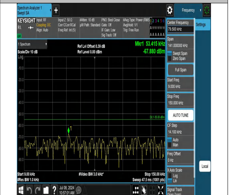
7-7-10MHz-20MHz-QPSK-QPSK-21206-21350-1RB#49-0RB#0-0 .009~0.15MHz-PASS
