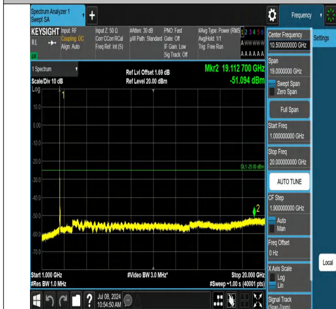
7-7-10MHz-20MHz-QPSK-QPSK-21006-21150-1RB#0-0RB#0-10 00~20000MHz-PASS
