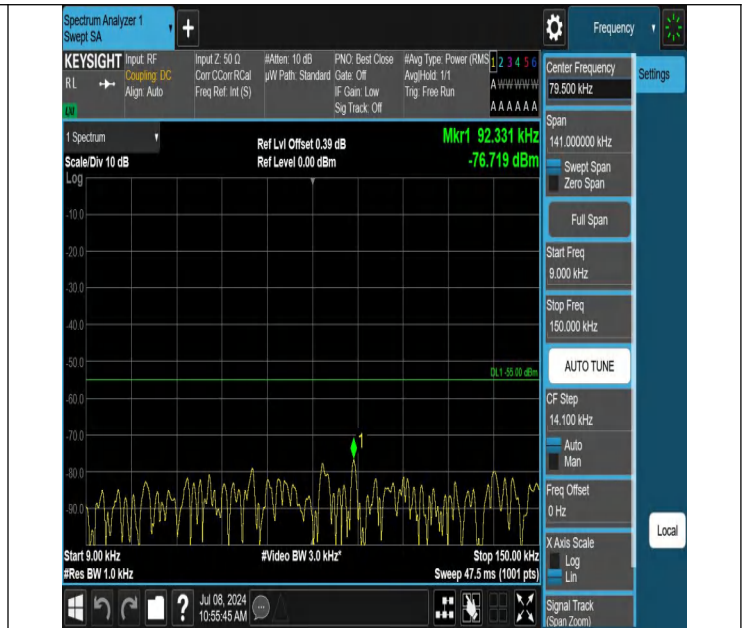
7-7-10MHz-20MHz-QPSK-QPSK-21006-21150-1RB#0-1RB#99-0. 009~0.15MHz-PASS
