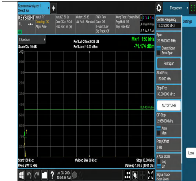
7-7-10MHz-20MHz-QPSK-QPSK-21006-21150-1RB#0-0RB#0-0. 15~30MHz-PASS
