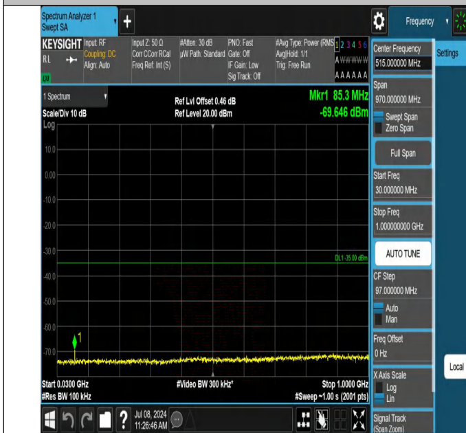
7-7-15MHz-20MHz-QPSK-QPSK-21003-21174-1RB#0-0RB#0-30 ~1000MHz-PASS
