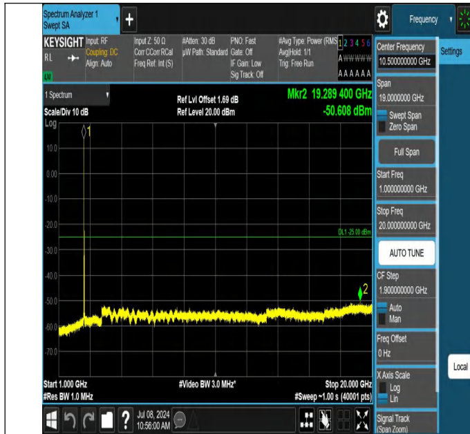
7-7-10MHz-20MHz-QPSK-QPSK-21006-21150-1RB#0-1RB#99-1 000~20000MHz-PASS
