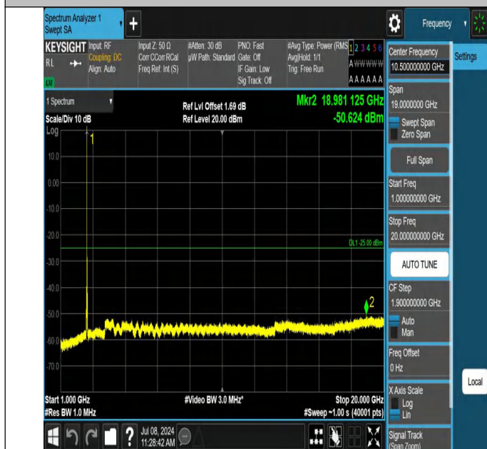
7-7-15MHz-20MHz-QPSK-QPSK-21179-21350-1RB#0-0RB#0-10 00~20000MHz-PASS
