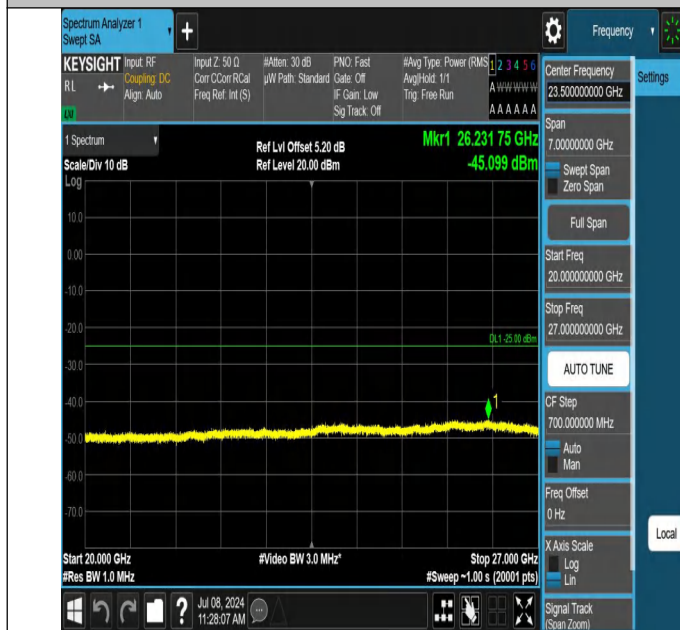
7-7-15MHz-20MHz-QPSK-QPSK-21003-21174-1RB#0-1RB#99-2 0000~27000MHz-PASS
