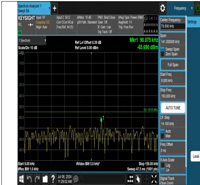
7-7-15MHz-20MHz-QPSK-QPSK-21179-21350-1RB#74-0RB#0-0.009~0.15MHz-PASS
