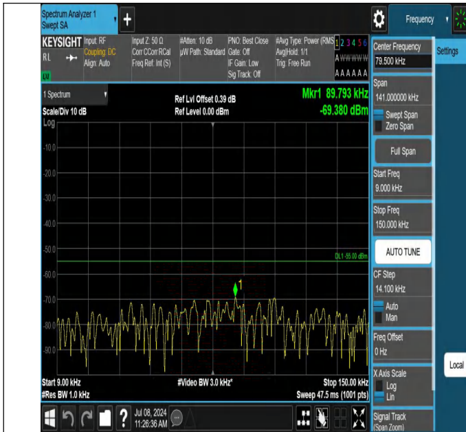
7-7-15MHz-20MHz-QPSK-QPSK-21003-21174-1RB#0-0RB#0-0. 009~0.15MHz-PASS
