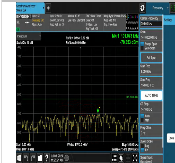
7-7-15MHz-20MHz-QPSK-QPSK-20828-20999-1RB#74-0RB#0-0 .009~0.15MHz-PASS
