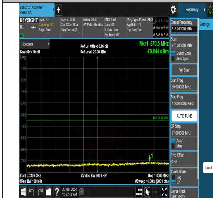
7-7-10MHz-20MHz-QPSK-QPSK-21206-21350-1RB#0-1RB#99-3 0~1000MHz-PASS
