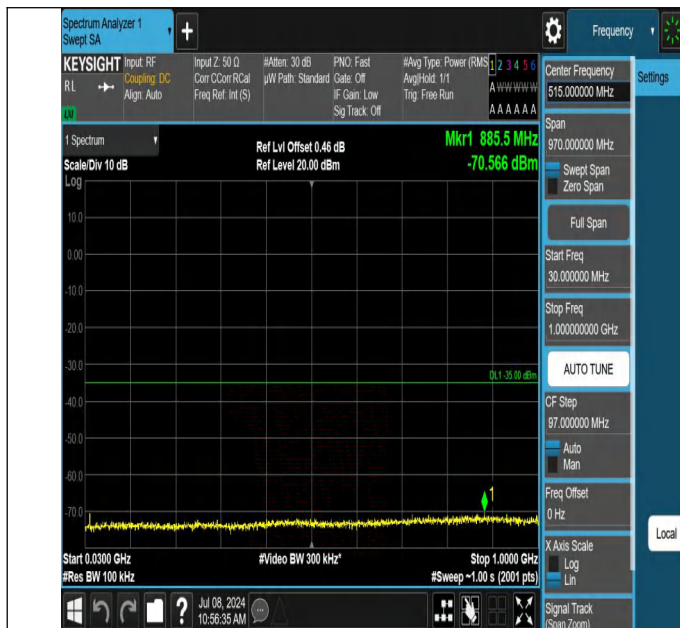
7-7-10MHz-20MHz-QPSK-QPSK-21206-21350-1RB#0-0RB#0-30 ~1000MHz-PASS
