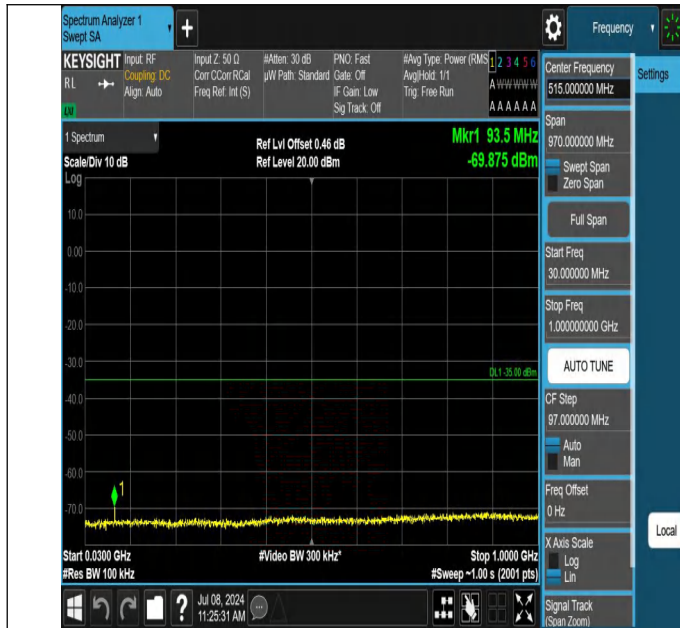
7-7-15MHz-20MHz-QPSK-QPSK-20828-20999-1RB#74-0RB#0-3 0~1000MHz-PASS
