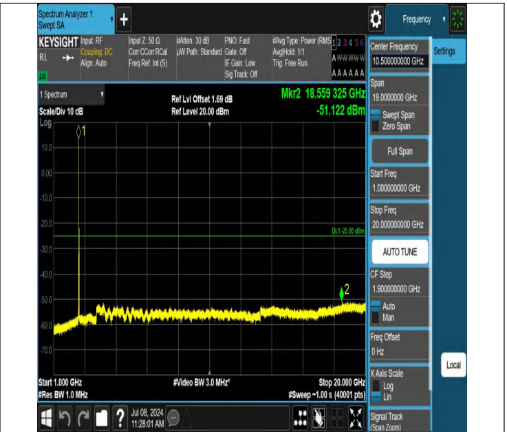
7-7-15MHz-20MHz-QPSK-QPSK-21003-21174-1RB#0-1RB#99-1 000~20000MHz-PASS
