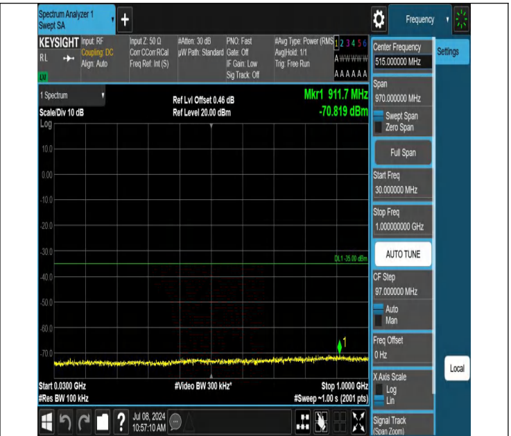
7-7-10MHz-20MHz-QPSK-QPSK-21206-21350-1RB#49-0RB#0-3 0~1000MHz-PASS
