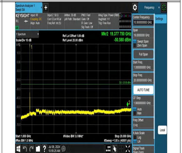
7-7-10MHz-20MHz-QPSK-QPSK-21006-21150-1RB#49-0RB#0-1000~20000MHz-PASS
