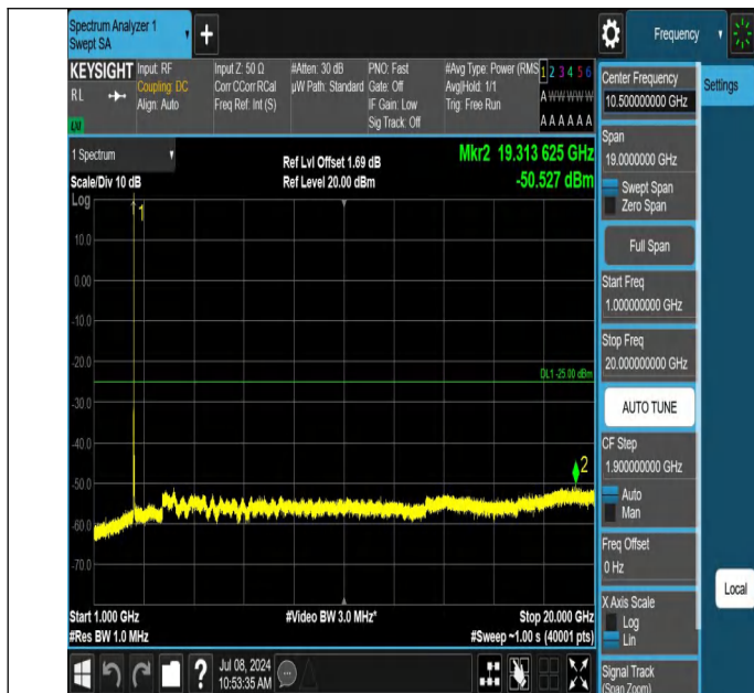
7-7-10MHz-20MHz-QPSK-QPSK-20805-20949-1RB#49-0RB#0-1 000~20000MHz-PASS
