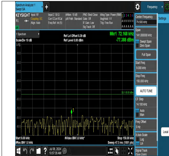
7-7-10MHz-20MHz-QPSK-QPSK-21206-21350-1RB#0-1RB#99-0 .009~0.15MHz-PASS
