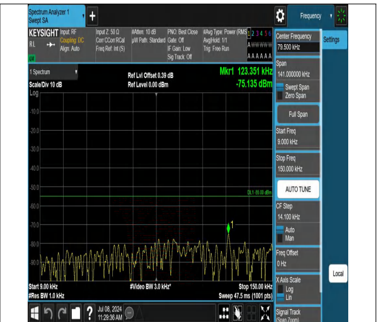
7-7-15MHz-20MHz-QPSK-QPSK-21179-21350-1RB#0-1RB#99-0. 009~0.15MHz-PASS
