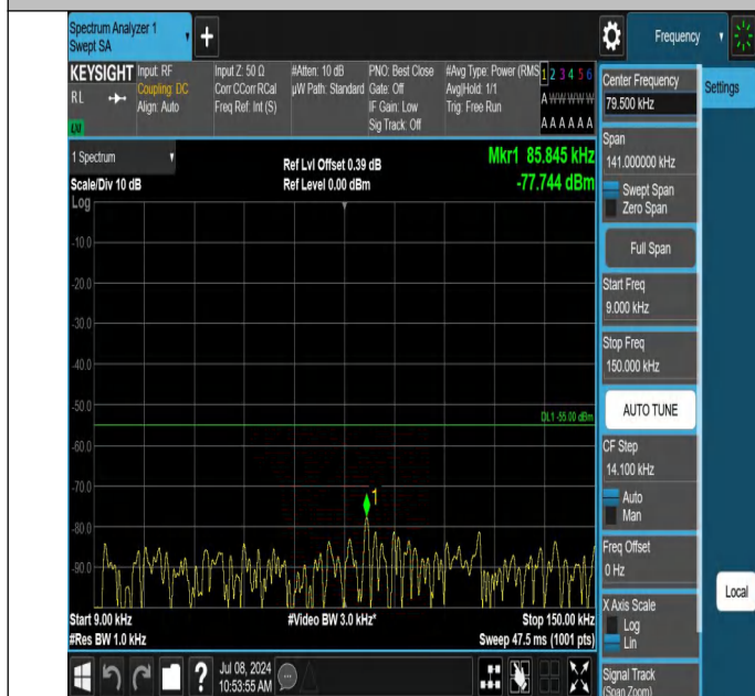
7-7-10MHz-20MHz-QPSK-QPSK-20805-20949-1RB#0-1RB#99-0 .009~0.15MHz-PASS
