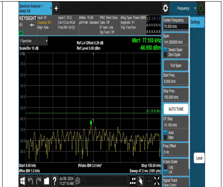
7-7-15MHz-20MHz-QPSK-QPSK-21003-21174-1RB#74-0RB#0-0. 009~0.15MHz-PASS
