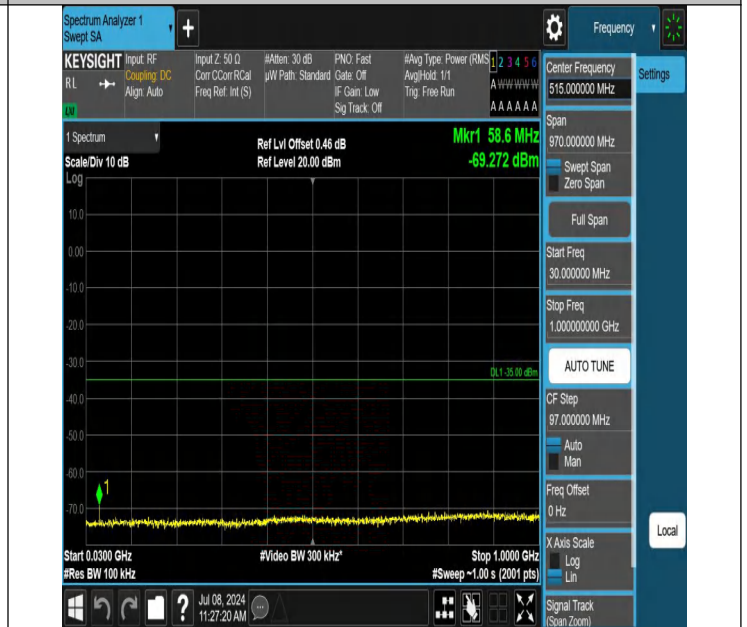
7-7-15MHz-20MHz-QPSK-QPSK-21003-21174-1RB#74-0RB#0-3 0~1000MHz-PASS
