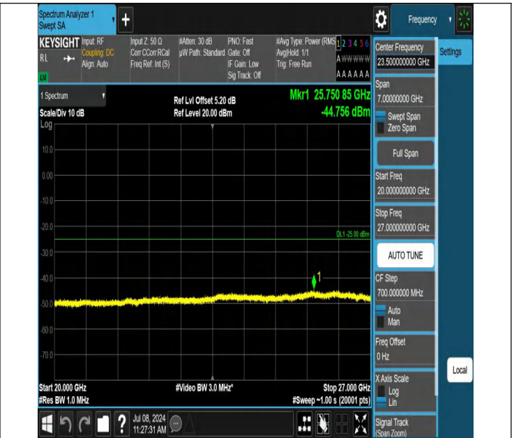
7-7-15MHz-20MHz-QPSK-QPSK-21003-21174-1RB#74-0RB#0-2 0000~27000MHz-PASS
