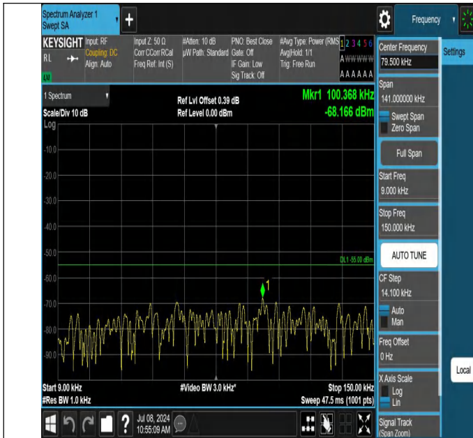
7-7-10MHz-20MHz-QPSK-QPSK-21006-21150-1RB#49-0RB#0-0.009~0.15MHz-PASS
