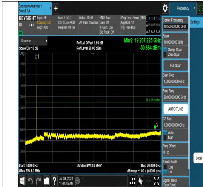
7-7-20MHz-15MHz-QPSK-QPSK-20850-21021-1RB#0-1RB#74-1 000~20000MHz-PASS
