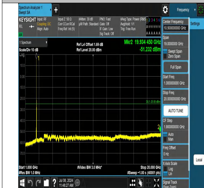
7-7-20MHz-15MHz-QPSK-QPSK-21201-21372-1RB#0-1RB#74-1 000~20000MHz-PASS
