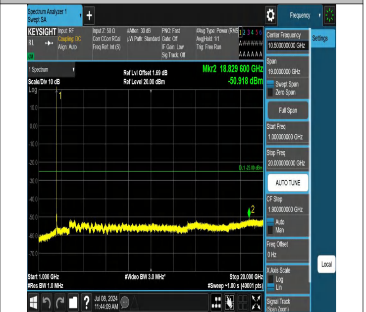
7-7-20MHz-15MHz-QPSK-QPSK-20850-21021-1RB#99-0RB#0-1 000~20000MHz-PASS
