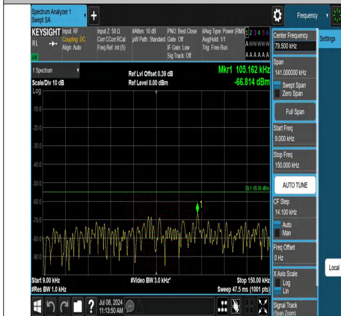
7-7-15MHz-15MHz-QPSK-QPSK-21025-21175-1RB#74-0RB#0-0 .009~0.15MHz-PASS
