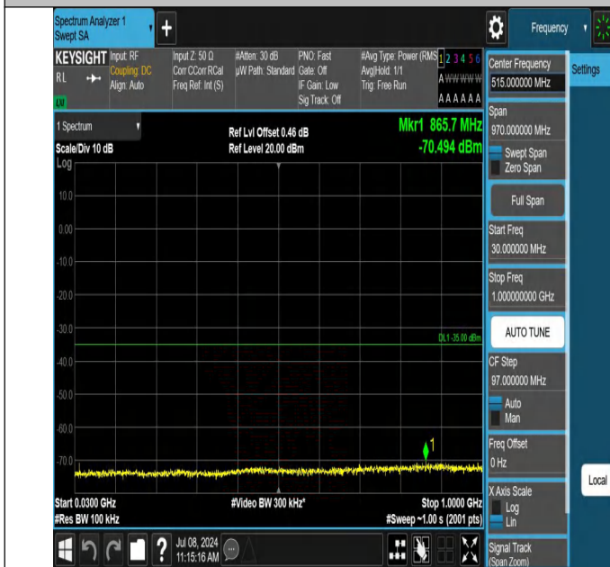
7-7-15MHz-15MHz-QPSK-QPSK-21225-21375-1RB#0-0RB#0-30 ~1000MHz-PASS
