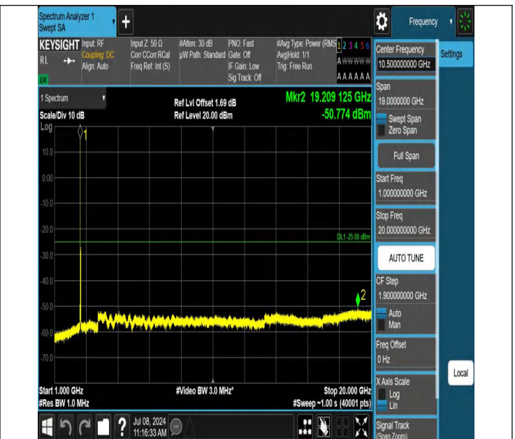
7-7-15MHz-15MHz-QPSK-QPSK-21225-21375-1RB#0-1RB#74-1 000~20000MHz-PASS
