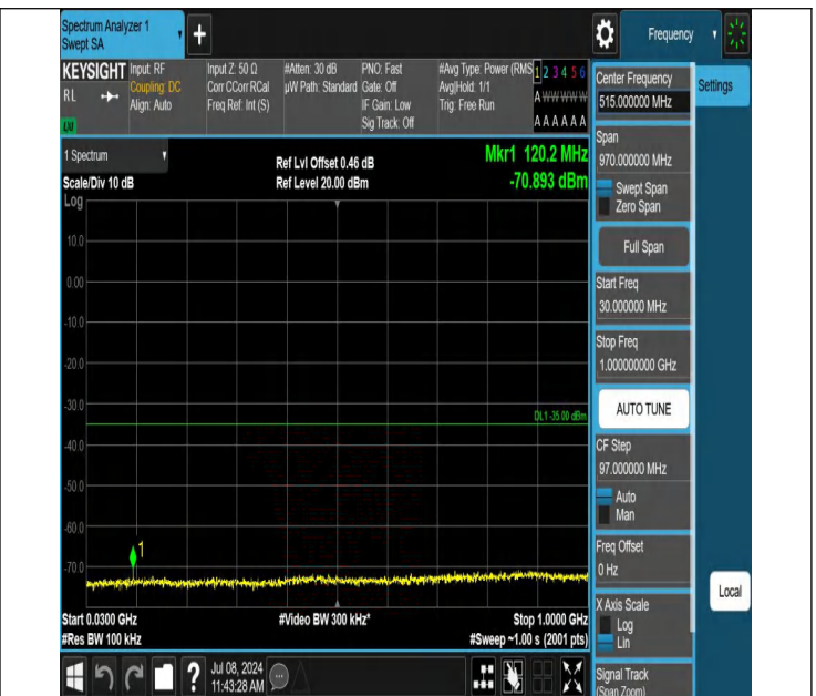
7-7-20MHz-15MHz-QPSK-QPSK-20850-21021-1RB#0-0RB#0-30 ~1000MHz-PASS
