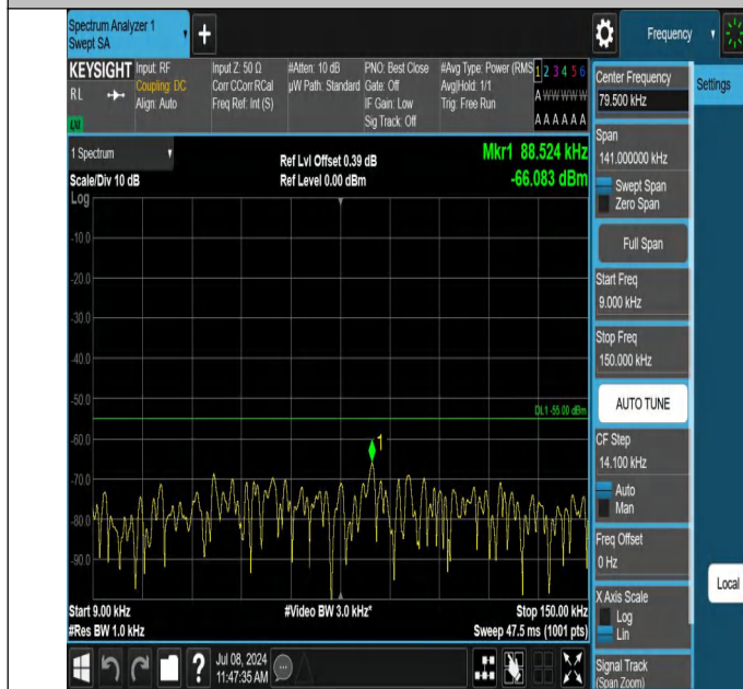
7-7-20MHz-15MHz-QPSK-QPSK-21201-21372-1RB#99-0RB#0-0 .009~0.15MHz-PASS
