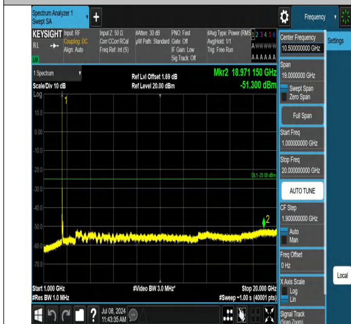
7-7-20MHz-15MHz-QPSK-QPSK-20850-21021-1RB#0-0RB#0-10 00~20000MHz-PASS
