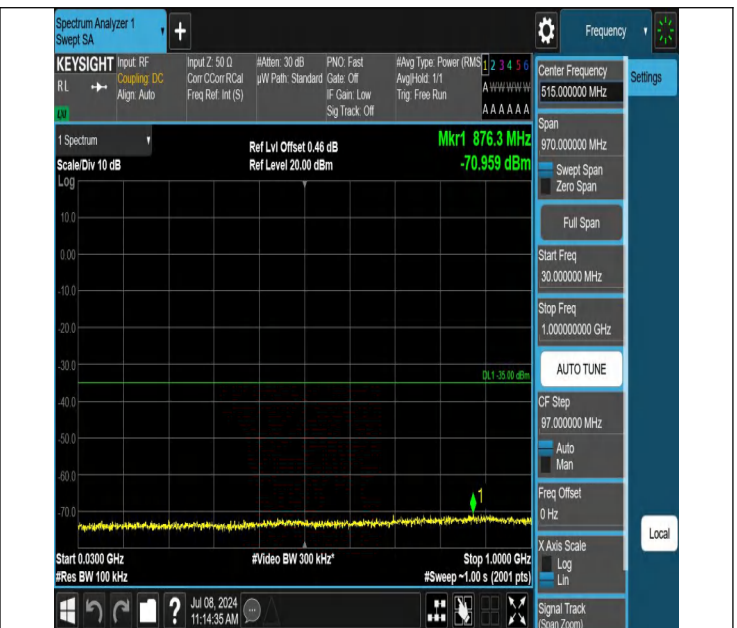
7-7-15MHz-15MHz-QPSK-QPSK-21025-21175-1RB#0-1RB#74-3 0~1000MHz-PASS
