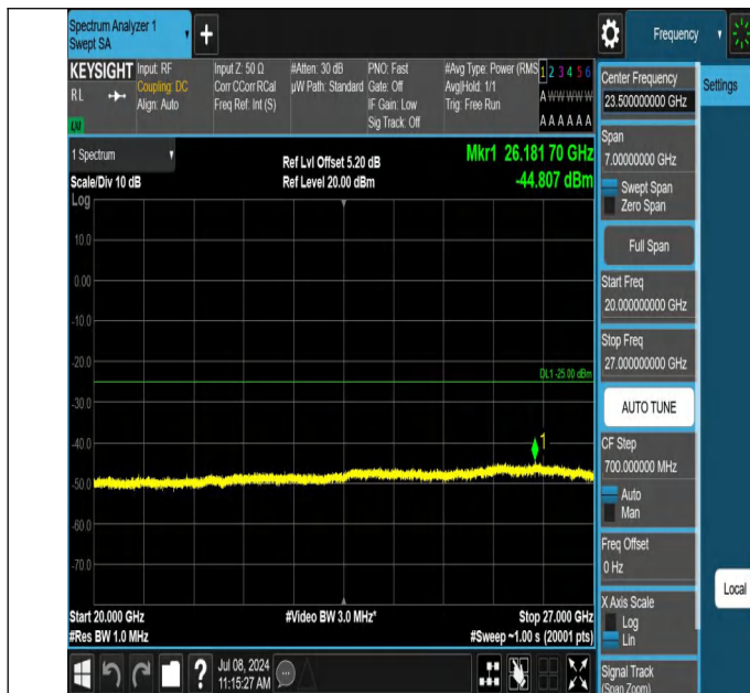
7-7-15MHz-15MHz-QPSK-QPSK-21225-21375-1RB#0-0RB#0-20 000~27000MHz-PASS
