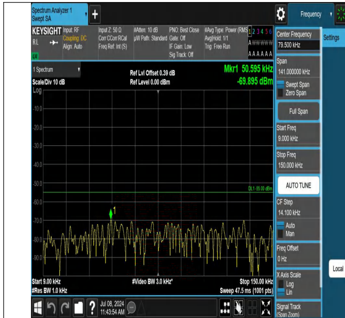
7-7-20MHz-15MHz-QPSK-QPSK-20850-21021-1RB#99-0RB#0-0 .009~0.15MHz-PASS
