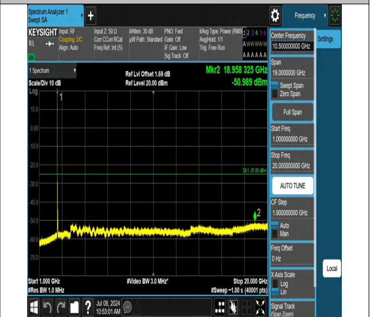
7-7-10MHz-20MHz-QPSK-QPSK-20805-20949-1RB#0-ORB#0-10 00~20000MHz-PASS
