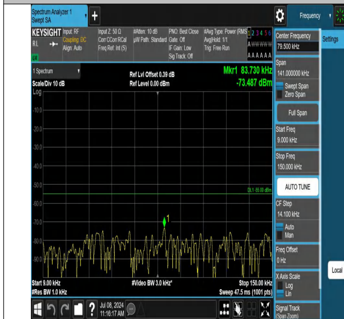
7-7-15MHz-15MHz-QPSK-QPSK-21225-21375-1RB#0-1RB#74-0 .009~0.15MHz-PASS
