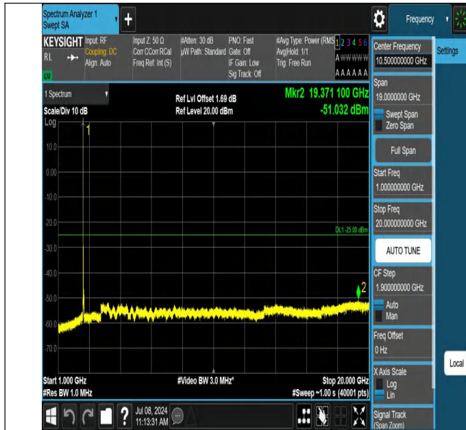
7-7-15MHz-15MHz-QPSK-QPSK-21025-21175-1RB#0-0RB#0-10 00~20000MHz-PASS
