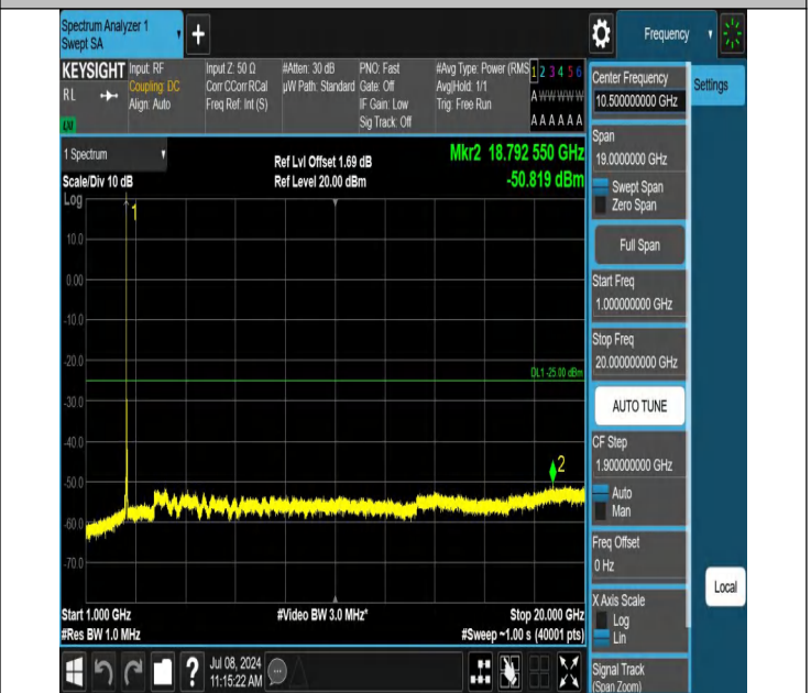
7-7-15MHz-15MHz-QPSK-QPSK-21225-21375-1RB#0-0RB#0-10 00~20000MHz-PASS
