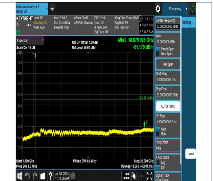
7-7-15MHz-15MHz-QPSK-QPSK-21025-21175-1RB#74-0RB#0-1 000~20000MHz-PASS
