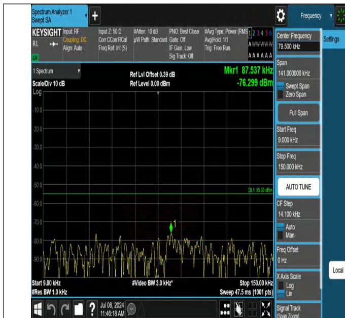
7-7-20MHz-15MHz-QPSK-QPSK-21026-21197-1RB#0-1RB#74-0 .009~0.15MHz-PASS
