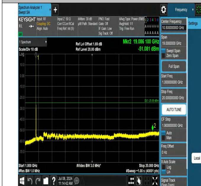
7-7-15MHz-15MHz-QPSK-QPSK-21025-21175-1RB#0-1RB#74-1 000~20000MHz-PASS
