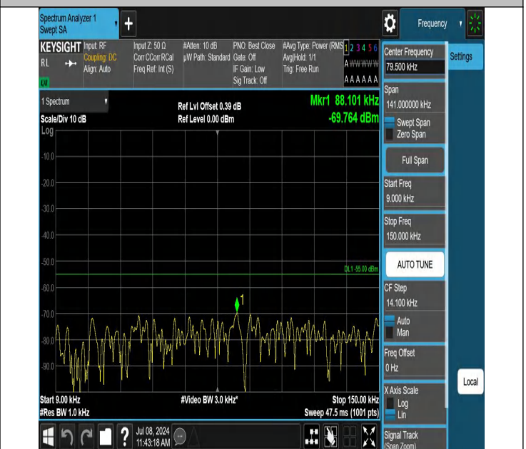
7-7-20MHz-15MHz-QPSK-QPSK-20850-21021-1RB#0-0RB#0-0. 009~0.15MHz-PASS
