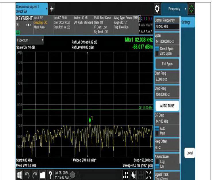
7-7-15MHz-15MHz-QPSK-QPSK-21225-21375-1RB#74-0RB#0-0 .009~0.15MHz-PASS
