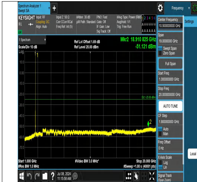
7-7-15MHz-15MHz-QPSK-QPSK-21225-21375-1RB#74-0RB#0-1 000~20000MHz-PASS
