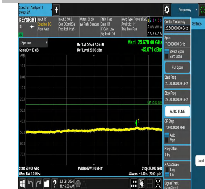
7-7-15MHz-15MHz-QPSK-QPSK-21225-21375-1RB#0-1RB#74-2 0000~27000MHz-PASS
