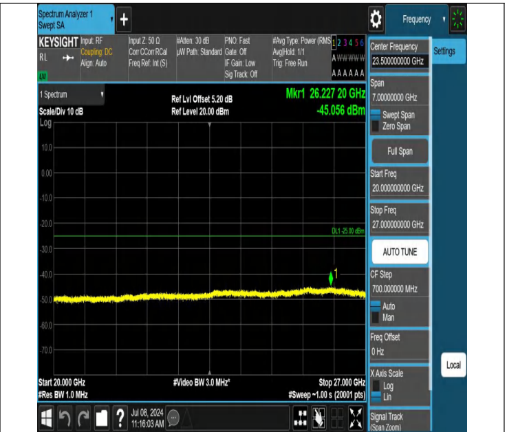
7-7-15MHz-15MHz-QPSK-QPSK-21225-21375-1RB#74-0RB#0-2 0000~27000MHz-PASS
