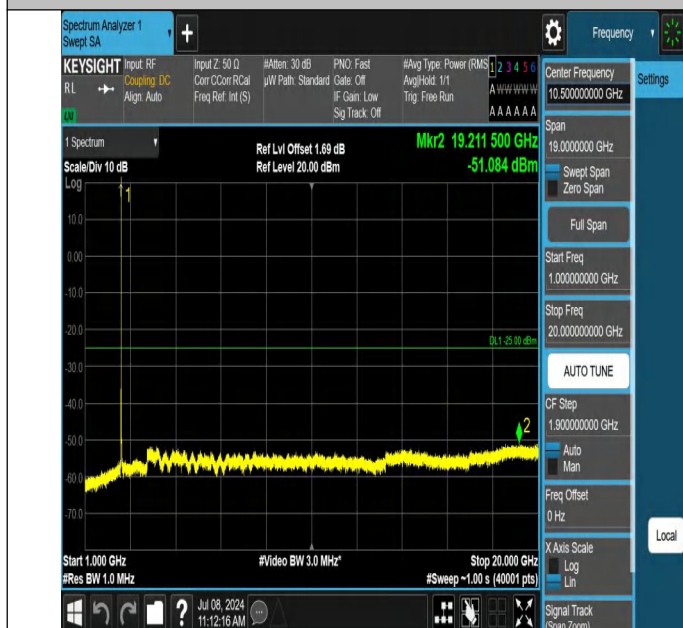
7-7-15MHz-15MHz-QPSK-QPSK-20825-20975-1RB#74-0RB#0-1 000~20000MHz-PASS
