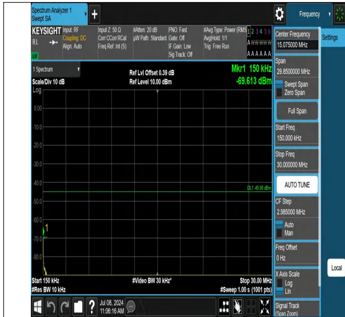
7-7-15MHz-10MHz-QPSK-QPSK-21277-21397-1RB#74-0RB#0-0 .15~30MHz-PASS
