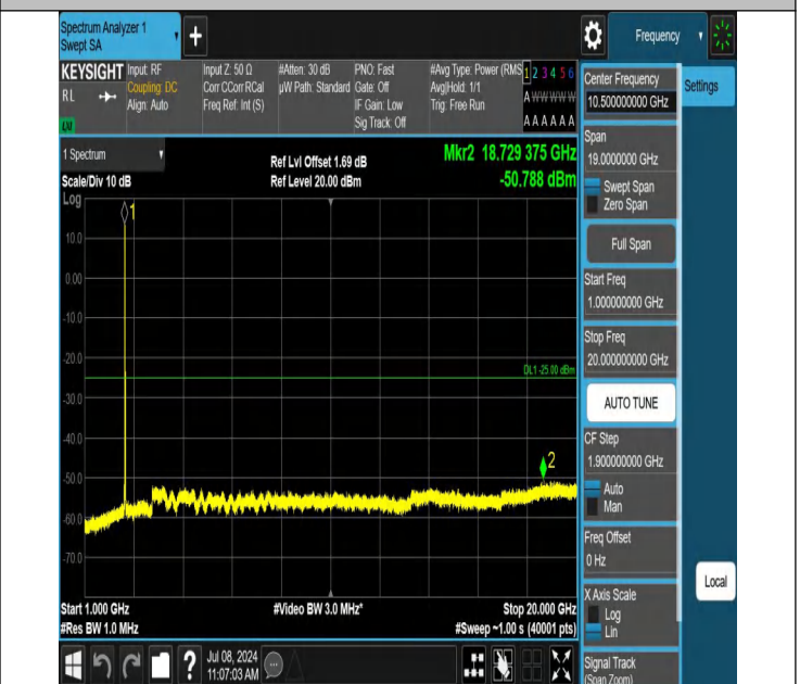
7-7-15MHz-10MHz-QPSK-QPSK-21277-21397-1RB#0-1RB#49-1 000~20000MHz-PASS
