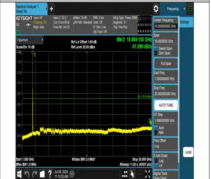
7-7-15MHz-15MHz-QPSK-QPSK-20825-20975-1RB#0-1RB#74-1 000~20000MHz-PASS
