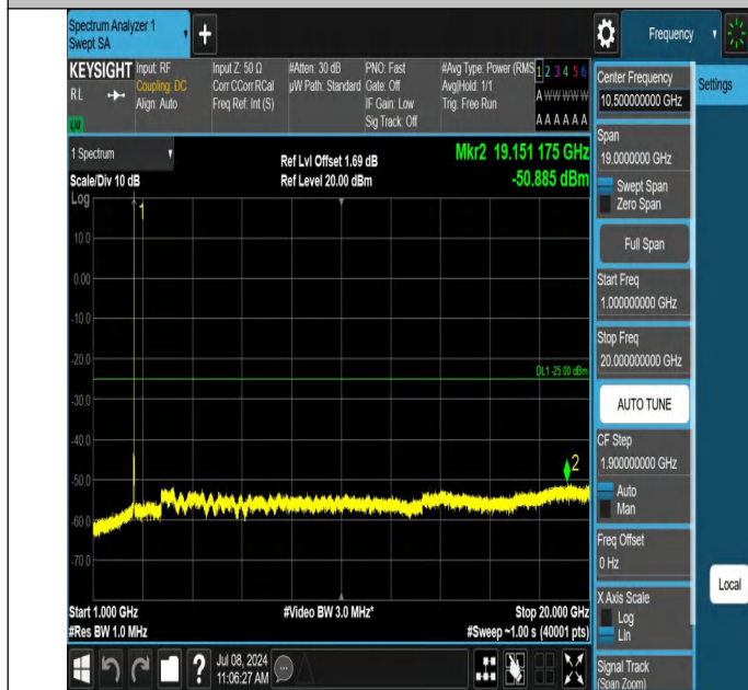
7-7-15MHz-10MHz-QPSK-QPSK-21277-21397-1RB#74-0RB#0-1 000~20000MHz-PASS
