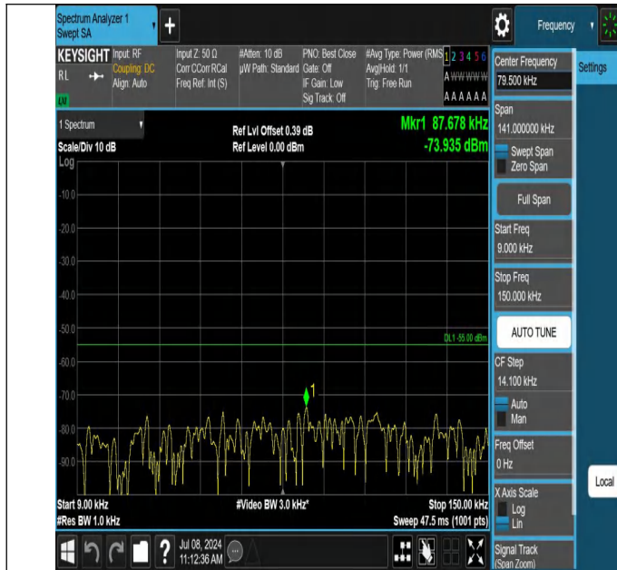
7-7-15MHz-15MHz-QPSK-QPSK-20825-20975-1RB#0-1RB#74-0 .009~0.15MHz-PASS
