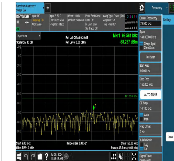
7-7-20MHz-10MHz-QPSK-QPSK-21251-21395-1RB#99-0RB#0-0 .009~0.15MHz-PASS
