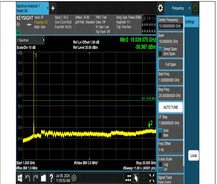
7-7-15MHz-10MHz-QPSK-QPSK-21277-21397-1RB#0-0RB#0-10 00~20000MHz-PASS
