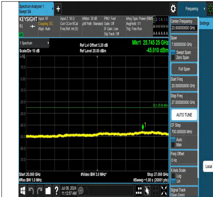
7-7-15MHz-15MHz-QPSK-QPSK-20825-20975-1RB#0-1RB#74-2 0000~27000MHz-PASS
