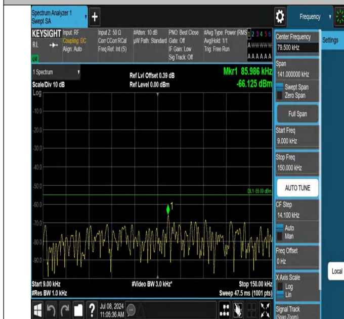
7-7-15MHz-10MHz-QPSK-QPSK-21277-21397-1RB#0-0RB#0-0. 009~0.15MHz-PASS
