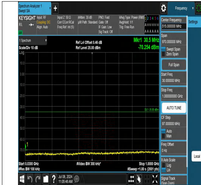
7-7-15MHz-10MHz-QPSK-QPSK-21277-21397-1RB#0-0RB#0-30 ~1000MHz-PASS
