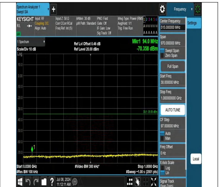
7-7-15MHz-15MHz-QPSK-QPSK-20825-20975-1RB#74-0RB#0-3 0~1000MHz-PASS
