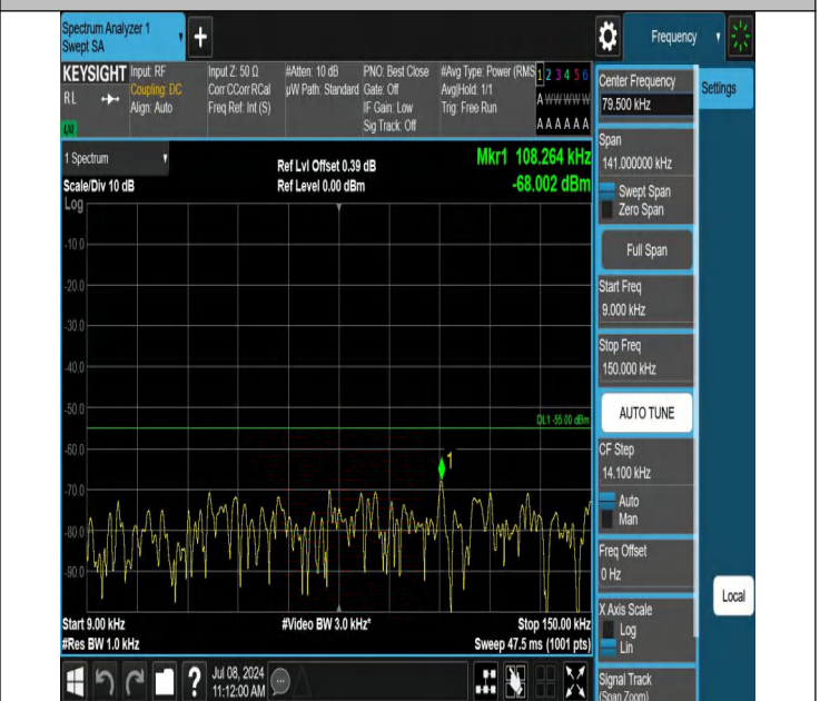
7-7-15MHz-15MHz-QPSK-QPSK-20825-20975-1RB#74-0RB#0-0 .009~0.15MHz-PASS
