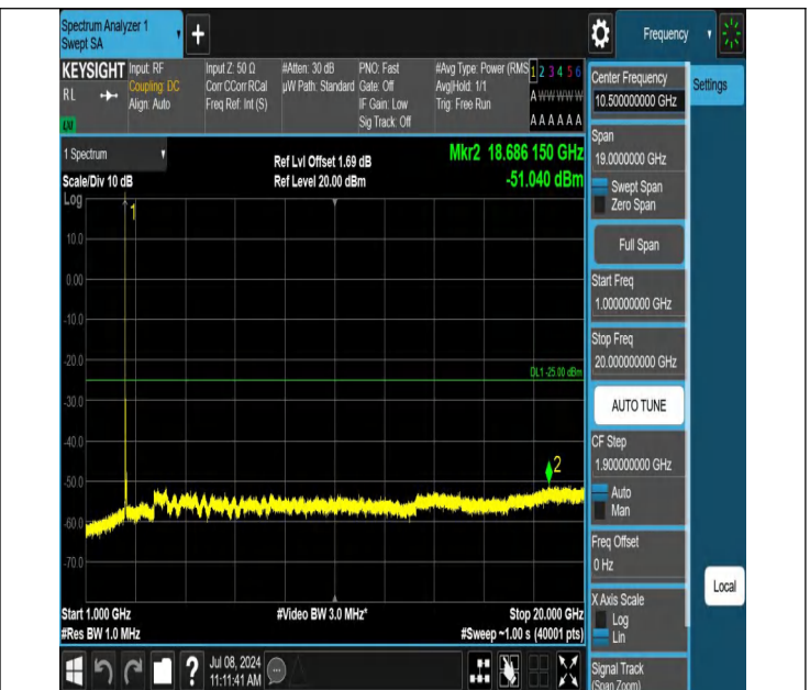
7-7-15MHz-15MHz-QPSK-QPSK-20825-20975-1RB#0-0RB#0-10 00~20000MHz-PASS
