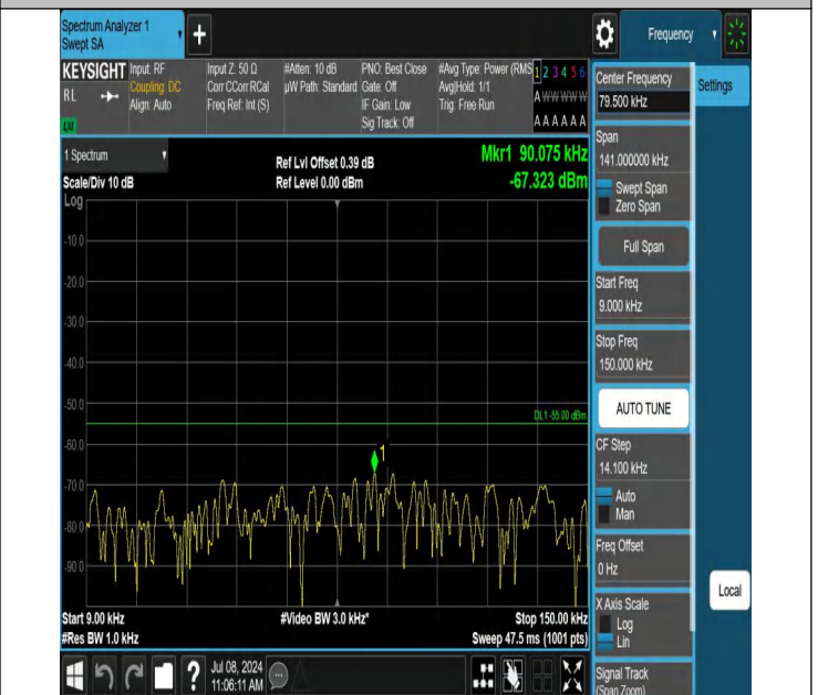
7-7-15MHz-10MHz-QPSK-QPSK-21277-21397-1RB#74-0RB#0-0 .009~0.15MHz-PASS
