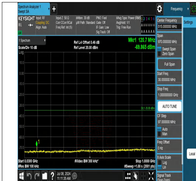
7-7-15MHz-15MHz-QPSK-QPSK-20825-20975-1RB#0-0RB#0-30 ~1000MHz-PASS
