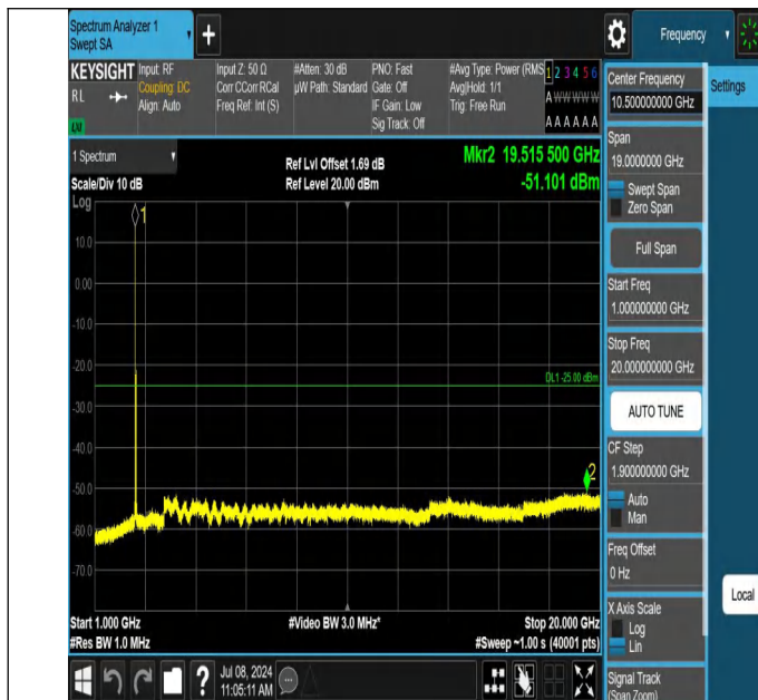
7-7-15MHz-10MHz-QPSK-QPSK-21051-21171-1RB#0-1RB#49-1 000~20000MHz-PASS
