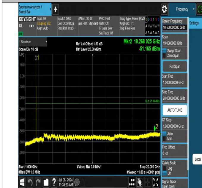
7-7-20MHz-10MHz-QPSK-QPSK-20850-20994-1RB#0-1RB#49-1 000~20000MHz-PASS
