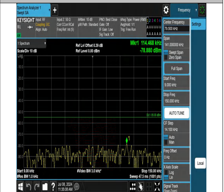
7-7-20MHz-10MHz-QPSK-QPSK-20850-20994-1RB#0-1RB#49-0 .009~0.15MHz-PASS
