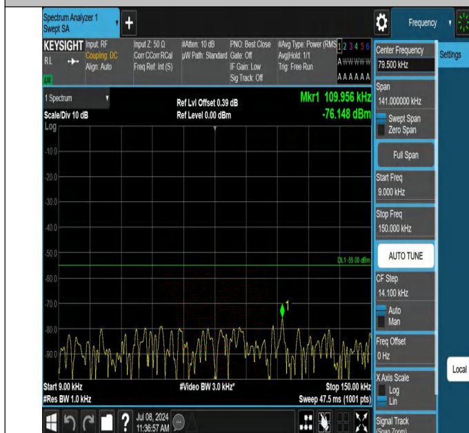
7-7-20MHz-10MHz-QPSK-QPSK-21051-21195-1RB#0-1RB#49-0 .009~0.15MHz-PASS
