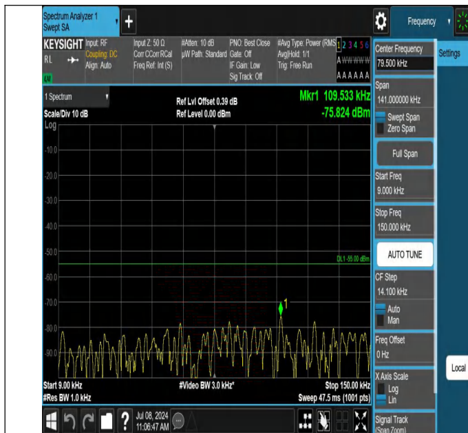
7-7-15MHz-10MHz-QPSK-QPSK-21277-21397-1RB#0-1RB#49-0 .009~0.15MHz-PASS
