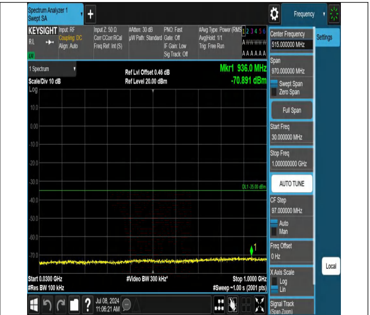
7-7-15MHz-10MHz-QPSK-QPSK-21277-21397-1RB#74-0RB#0-3 0~1000MHz-PASS
