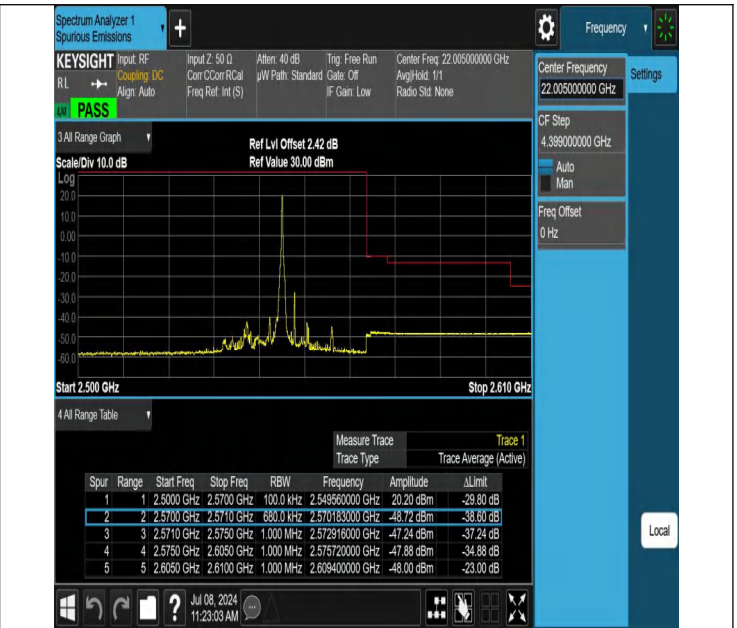
7-7-15MHz-20MHz-QPSK@QPSK-QPSK@QPSK-21179-21350-1 RB#74@75RB#0-0RB#0@100RB#0-PASS
