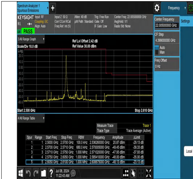
7-7-15MHz-20MHz-QPSK@QPSK-QPSK@QPSK-21179-21350-1 RB#0@75RB#0-0RB#0@100RB#0-PASS
