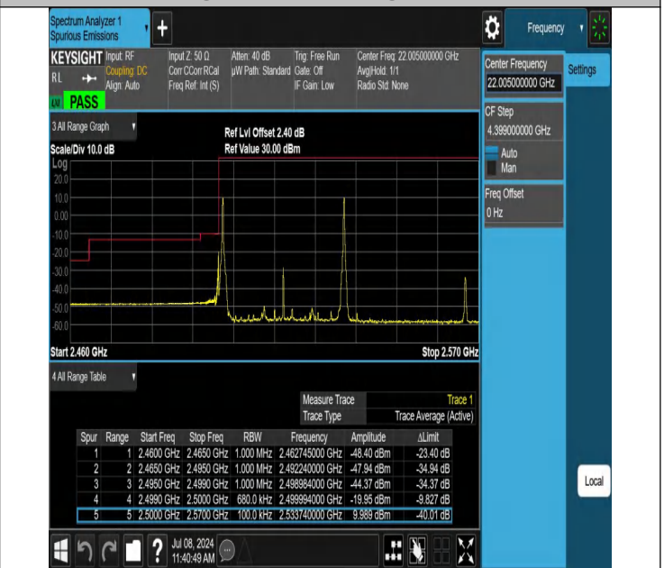
7-7-20MHz-15MHz-QPSK@QPSK-QPSK@QPSK-20850-21021-1RB#0@100RB#0-1RB#74@75RB#0-PASS
