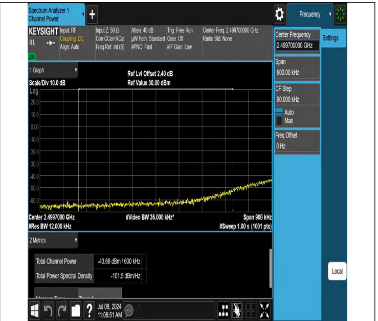
7-7-15MHz-15MHz-QPSK@QPSK-QPSK@QPSK-20825-20975-1RB#0@75RB#0-1RB#74@75RB#0-PASS_Final1
