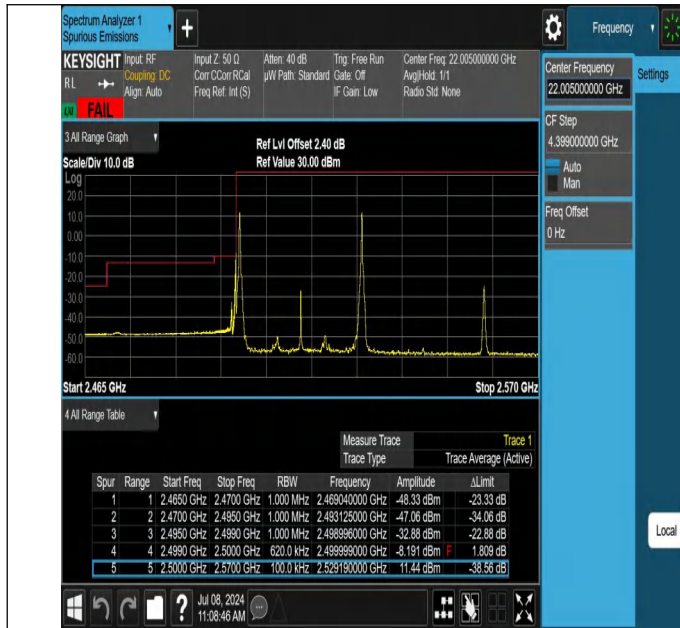
7-7-15MHz-15MHz-QPSK@QPSK-QPSK@QPSK-20825-20975-1RB#0@75RB#0-1RB#74@75RB#0-FAIL
