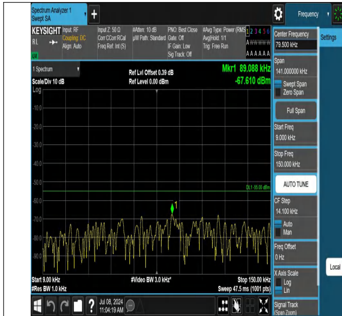
7-7-15MHz-10MHz-QPSK-QPSK-21051-21171-1RB#74-0RB#0-0.009~0.15MHz-PASS
