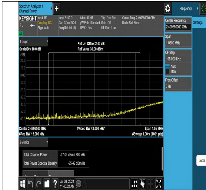
7-7-20MHz-15MHz-QPSK@QPSK-QPSK@QPSK-20850-21021-1RB#0@100RB#0-0RB#0@75RB#0-PASS_Final1
