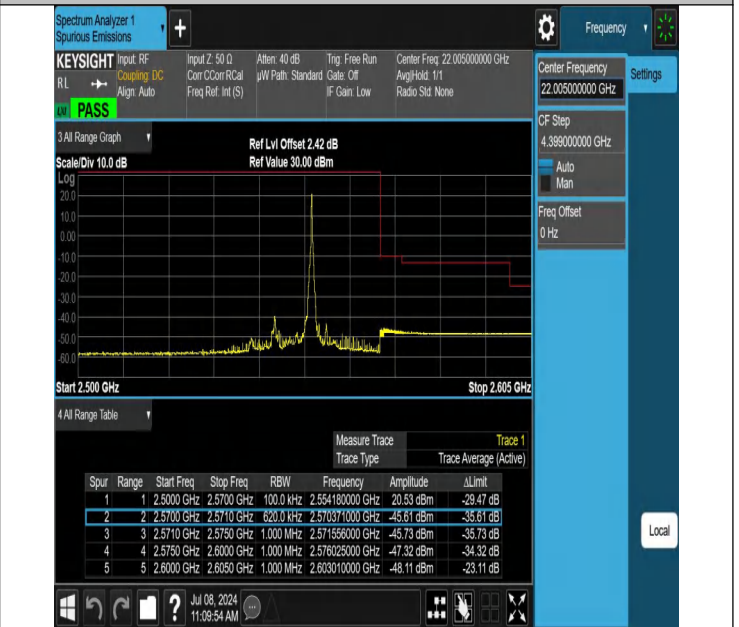
7-7-15MHz-15MHz-QPSK@QPSK-QPSK@QPSK-21225-21375-1RB#74@75RB#0-0RB#0@75RB#0-PASS
