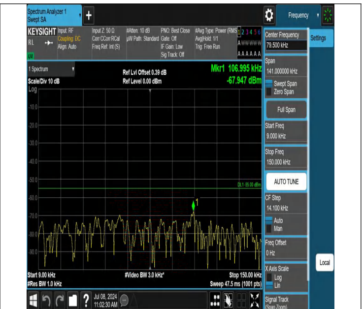
7-7-15MHz-10MHz-QPSK-QPSK-20825-20945-1RB#74-0RB#0-0 .009~0.15MHz-PASS
