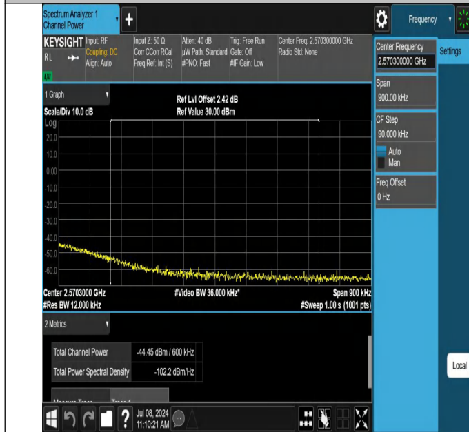
7-7-15MHz-15MHz-QPSK@QPSK-QPSK@QPSK-21225-21375-1RB#0@75RB#0-1RB#74@75RB#0-PASS_Final1
