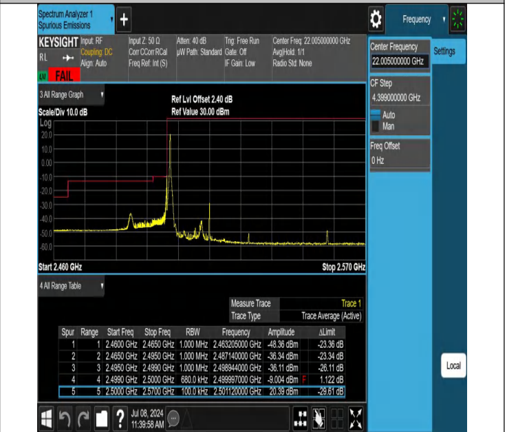
7-7-20MHz-15MHz-QPSK@QPSK-QPSK@QPSK-20850-21021-1RB#0@100RB#0-0RB#0@75RB#0-FAIL
