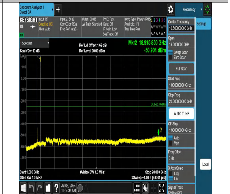
7-7-15MHz-10MHz-QPSK-QPSK-21051-21171-1RB#74-0RB#0-1000~20000MHz-PASS
