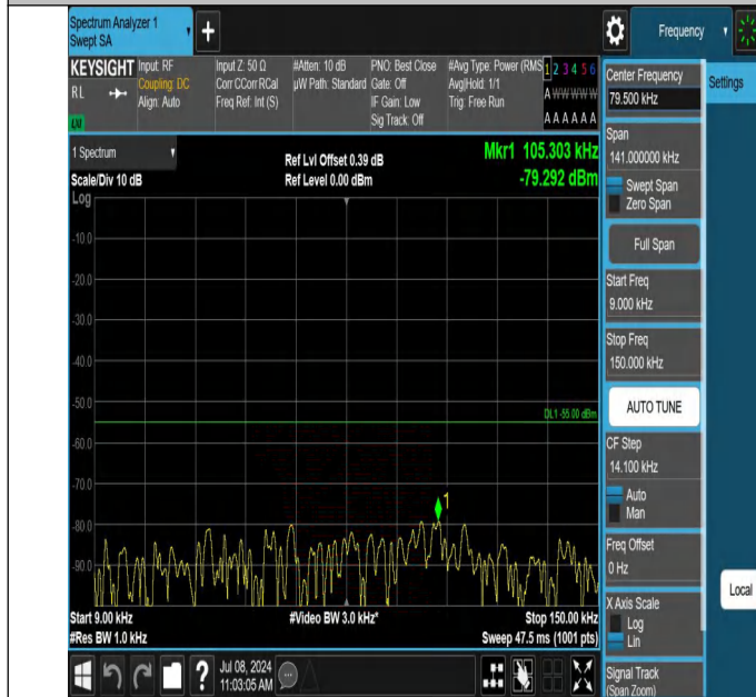
7-7-15MHz-10MHz-QPSK-QPSK-20825-20945-1RB#0-1RB#49-0 .009~0.15MHz-PASS
