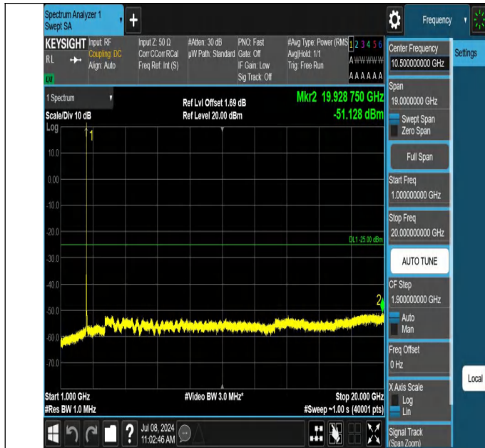
7-7-15MHz-10MHz-QPSK-QPSK-20825-20945-1RB#74-0RB#0-1 000~20000MHz-PASS
