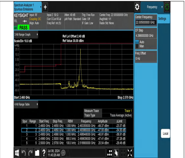
7-7-20MHz-15MHz-QPSK@QPSK-QPSK@QPSK-20850-21021-1RB#99@100RB#0-0RB#0@75RB#0-PASS
