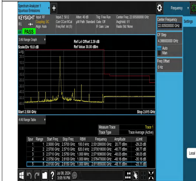
7-7-20MHz-20MHz-QPSK@QPSK-QPSK@QPSK-21152-21350-1RB#0@100RB#0-0RB#0@100RB#0-PASS
