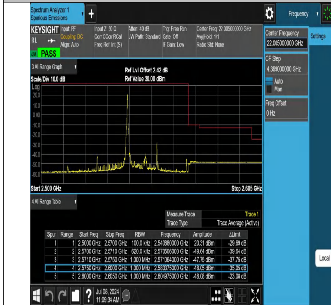
7-7-15MHz-15MHz-QPSK@QPSK-QPSK@QPSK-21225-21375-1RB#0@75RB#0-0RB#0@75RB#0-PASS
