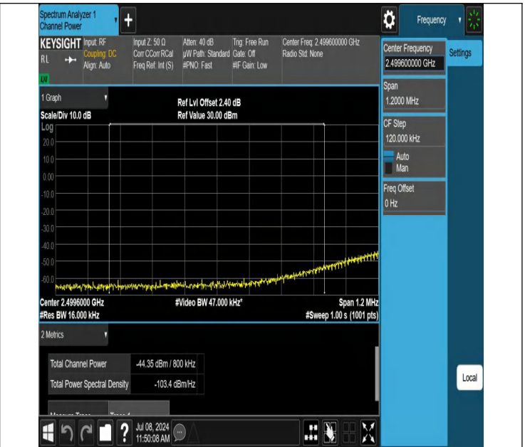
7-7-20MHz-20MHz-QPSK@QPSK-QPSK@QPSK-20850-21048-1RB#0@100RB#0-1RB#99@100RB#0-PASS_Final1
