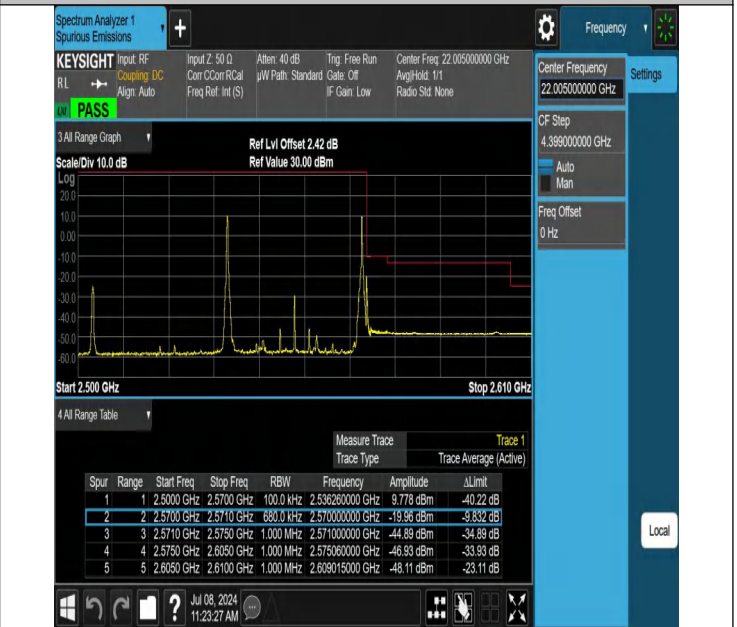
7-7-15MHz-20MHz-QPSK@QPSK-QPSK@QPSK-21179-21350-1 RB#0@75RB#0-1RB#99@100RB#0-PASS
