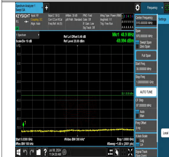
7-7-15MHz-10MHz-QPSK-QPSK-21051-21171-1RB#74-0RB#0-30~1000MHz-PASS
