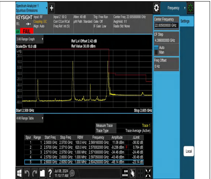
7-7-15MHz-15MHz-QPSK@QPSK-QPSK@QPSK-21225-21375-1RB#0@75RB#0-1RB#74@75RB#0-FAIL
