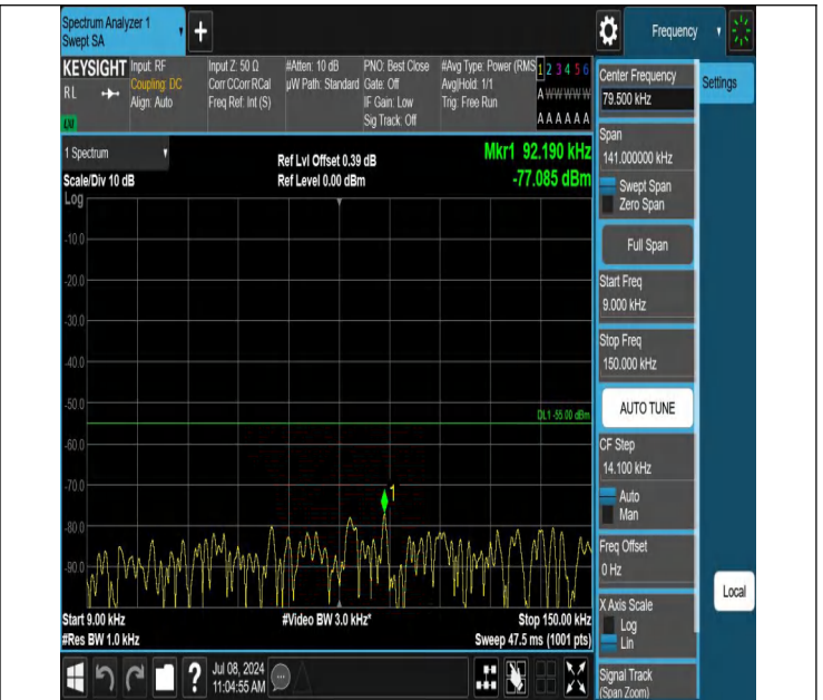
7-7-15MHz-10MHz-QPSK-QPSK-21051-21171-1RB#0-1RB#49-0. 009~0.15MHz-PASS
