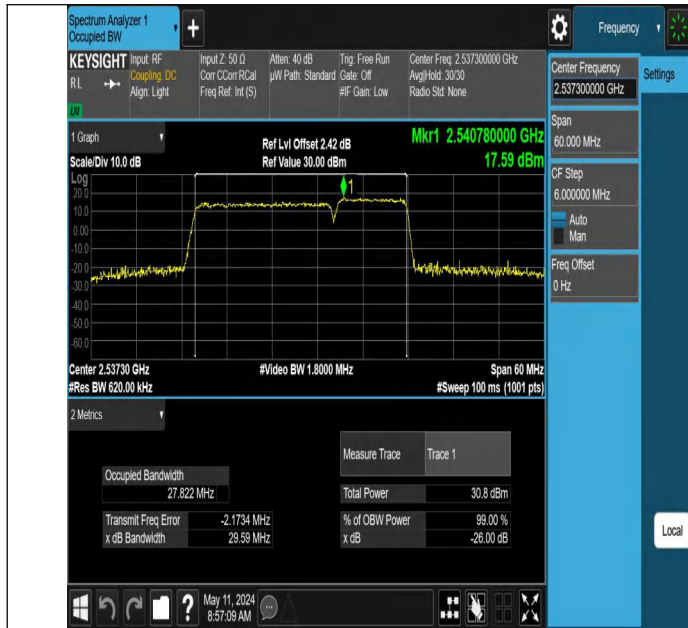
7-7-20MHz-10MHz-QPSK-QPSK-21051-21195-100RB#0-50RB#0-0 PASS
