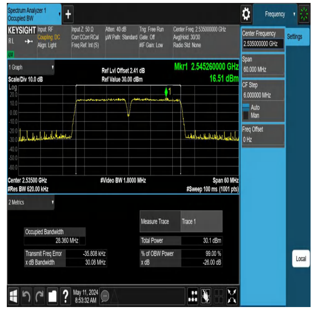
7-7-15MHz-15MHz-64QAM-64QAM-21025-21175-75RB#0-75RB #0-PASS
