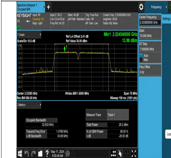
7-7-15MHz-20MHz-256QAM-256QAM-21003-21174-75RB#0-100 RB#0-PASS
