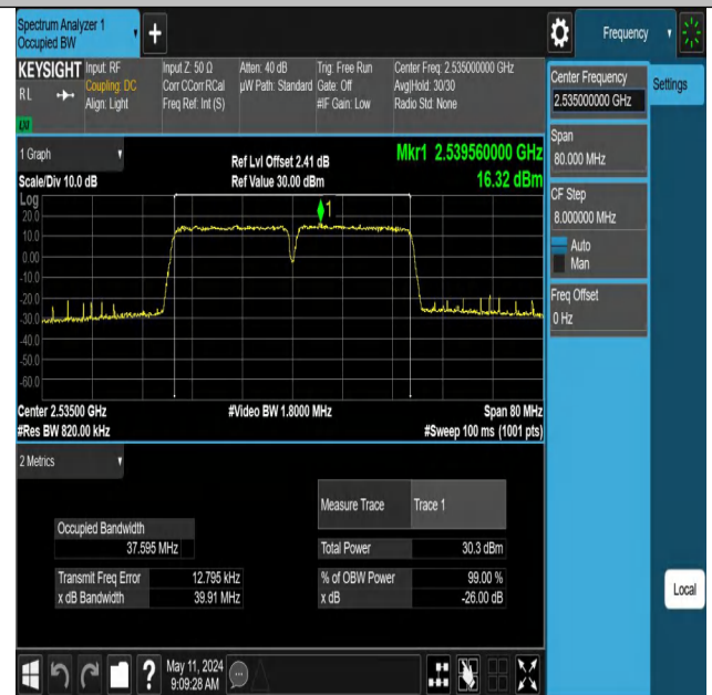
7-7-20MHz-20MHz-16QAM-16QAM-21001-21199-100RB#0-100RB#0-PASS
