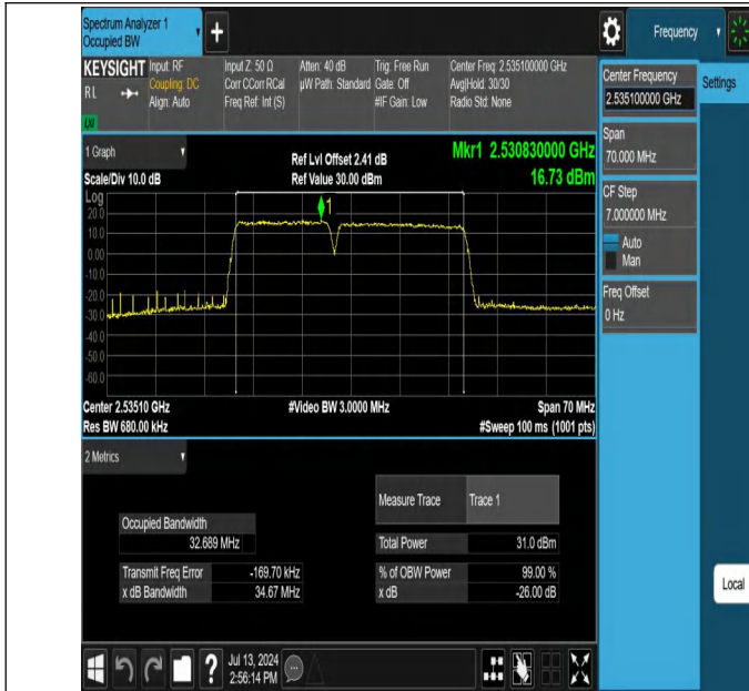
7-7-15MHz-20MHz-QPSK-QPSK-21003-21174-75RB#0-100RB#0- PASS
