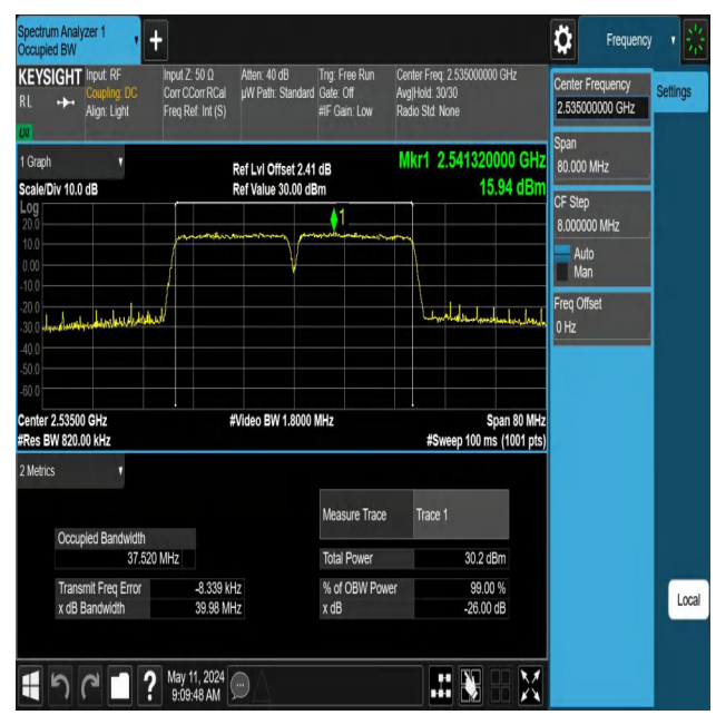
7-7-20MHz-20MHz-64QAM-64QAM-21001-21199-100RB#0-100RB#0-PASS
