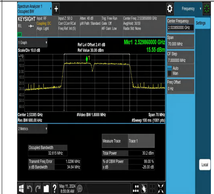
7-7-15MHz-20MHz-16QAM-16QAM-21003-21174-75RB#0-100R B#0-PASS
