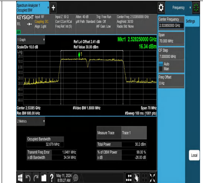
7-7-15MHz-20MHz-64QAM-64QAM-21003-21174-75RB#0-100R B#0-PASS
