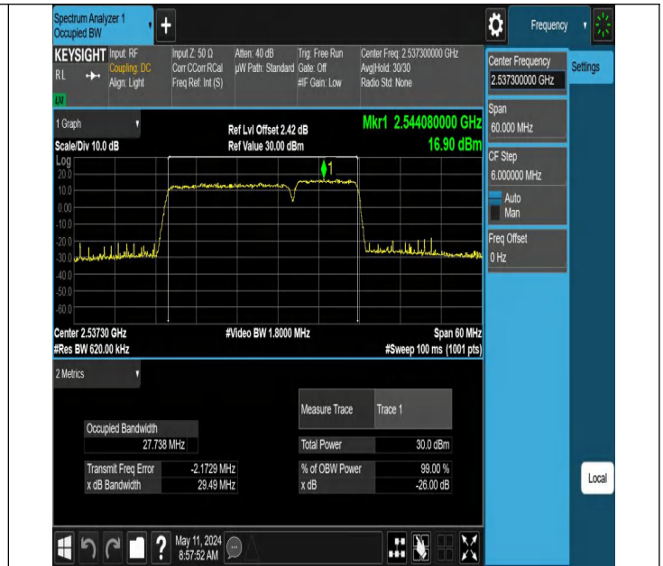
7-7-20MHz-10MHz-64QAM-64QAM-21051-21195-100RB#0-50RB#0-PASS
