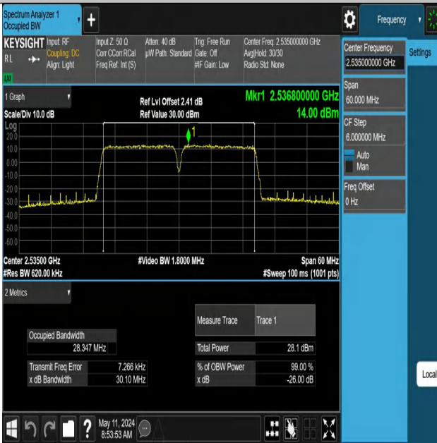
7-7-15MHz-15MHz-256QAM-256QAM-21025-21175-75RB#0-75R B#0-PASS
