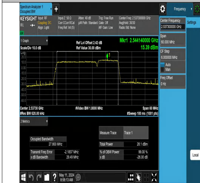
7-7-20MHz-10MHz-256QAM-256QAM-21051-21195-100RB#0-50RB#0-PASS
