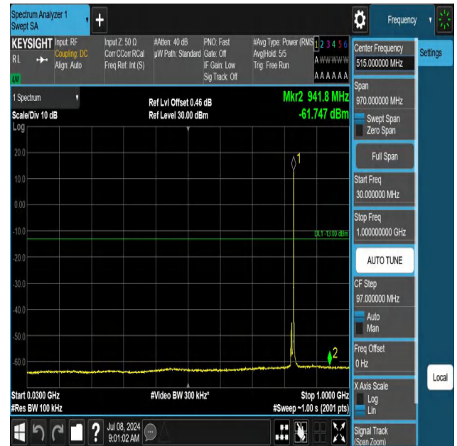
5-5-10MHz-10MHz-QPSK-QPSK-20450-20549-1RB#49-0RB#0-3 0~1000MHz-PASS
