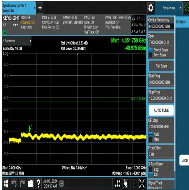
5-5-10MHz-10MHz-QPSK-QPSK-20476-20575-1RB#49-0RB#0-3 000~10000MHz-PASS
