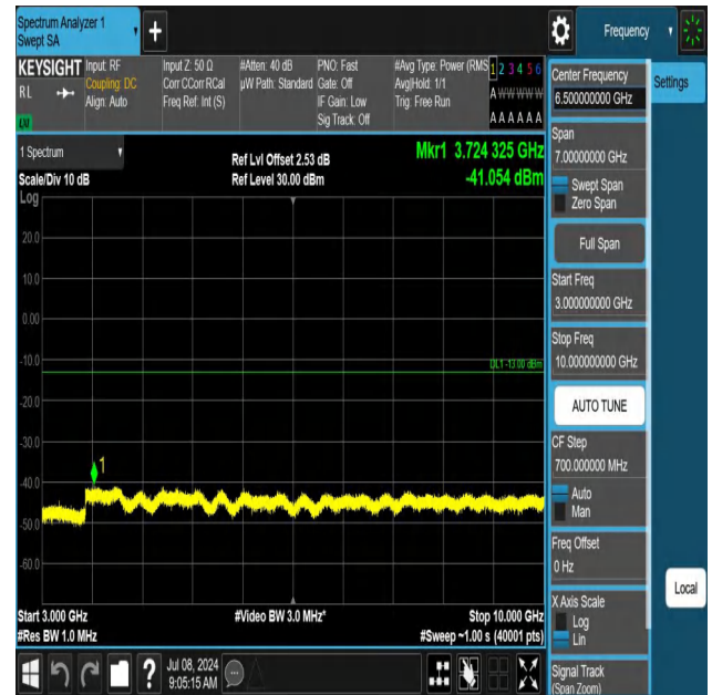
5-5-10MHz-10MHz-QPSK-QPSK-20501-20600-1RB#49-0RB#0-3 000~10000MHz-PASS
