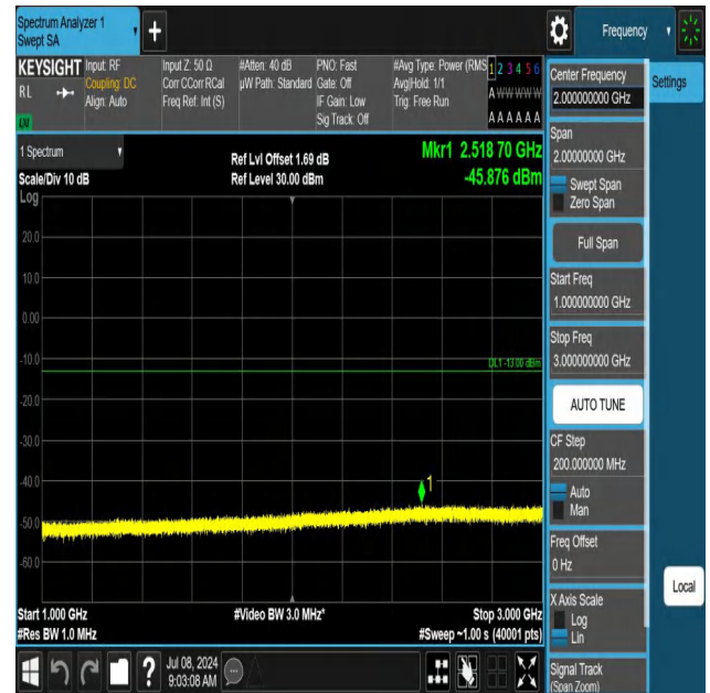
5-5-10MHz-10MHz-QPSK-QPSK-20476-20575-1RB#49-0RB#0-1 000~3000MHz-PASS
