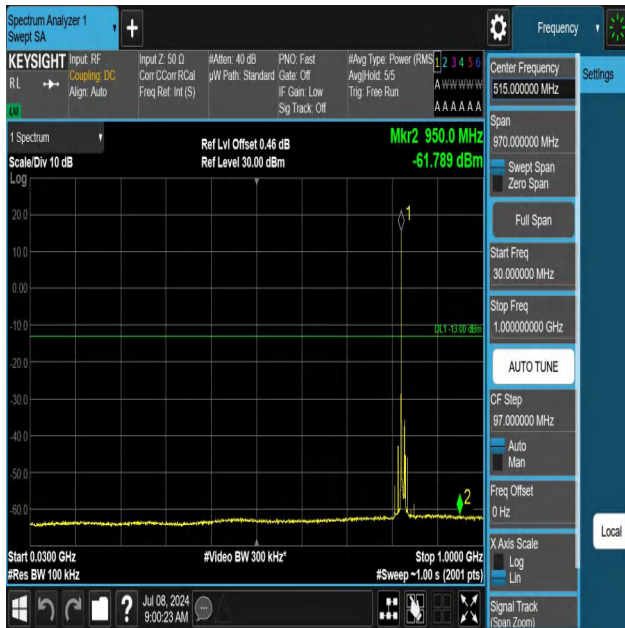
5-5-10MHz-10MHz-QPSK-QPSK-20450-20549-1RB#0-ORB#0-30 ~1000MHz-PASS
