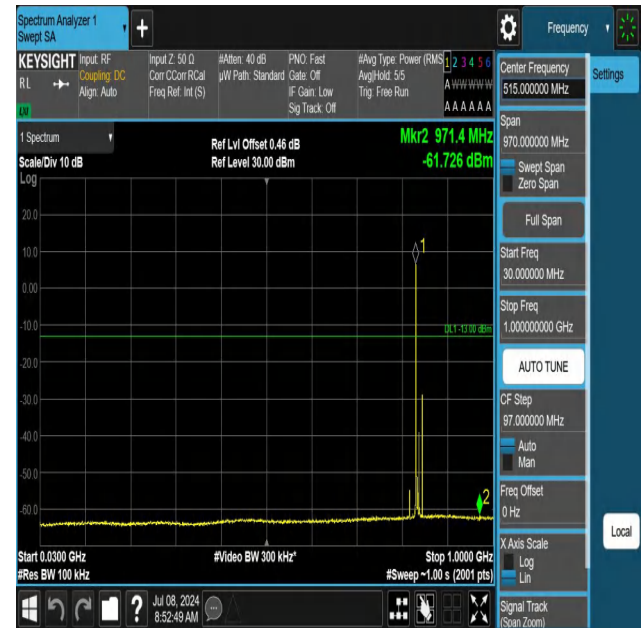
5-5-5MHz-10MHz-QPSK-QPSK-20528-20600-1RB#0-1RB#49-30 ~1000MHz-PASS
