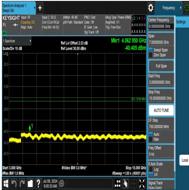
5-5-10MHz-10MHz-QPSK-QPSK-20450-20549-1RB#0-0RB#0-30 00~10000MHz-PASS
