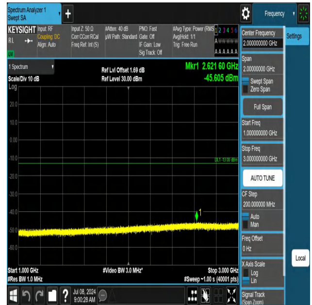
5-5-10MHz-10MHz-QPSK-QPSK-20450-20549-1RB#0-ORB#0-10 00~3000MHz-PASS
