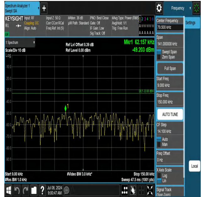
5-5-10MHz-10MHz-QPSK-QPSK-20450-20549-1RB#49-0RB#0-0 .009~0.15MHz-PASS
