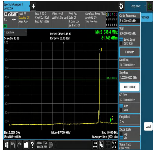
5-5-10MHz-10MHz-QPSK-QPSK-20501-20600-1RB#49-0RB#0-3 0~1000MHz-PASS
