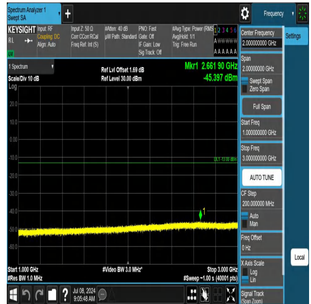
5-5-10MHz-10MHz-QPSK-QPSK-20501-20600-1RB#0-1RB#49-1 000~3000MHz-PASS
