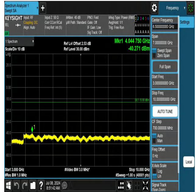
5-5-5MHz-10MHz-QPSK-QPSK-20528-20600-1RB#0-ORB#0-300 0~10000MHz-PASS
