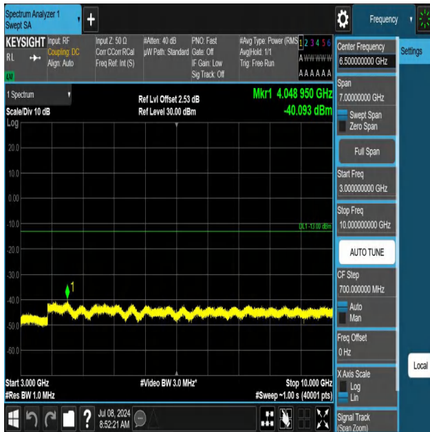
5-5-5MHz-10MHz-QPSK-QPSK-20528-20600-1RB#24-0RB#0-30 00~10000MHz-PASS
