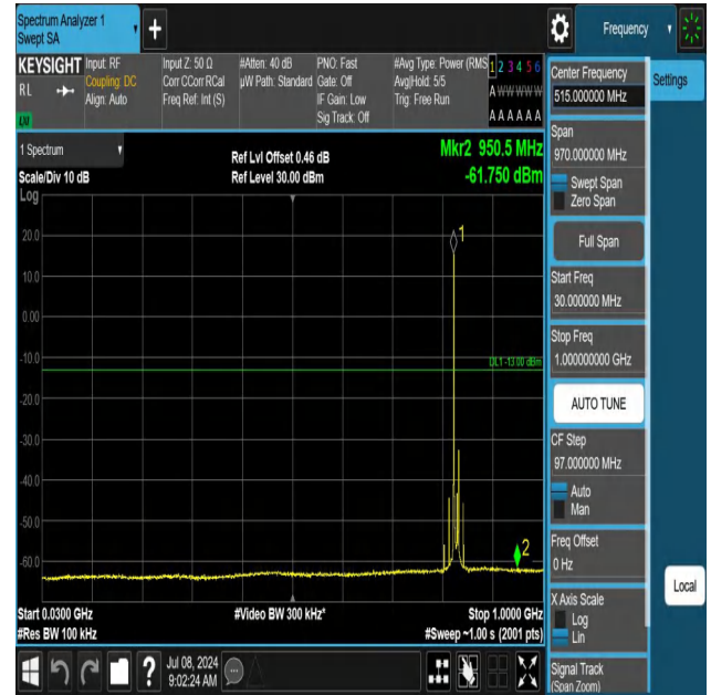
5-5-10MHz-10MHz-QPSK-QPSK-20476-20575-1RB#0-ORB#0-30 ~1000MHz-PASS
