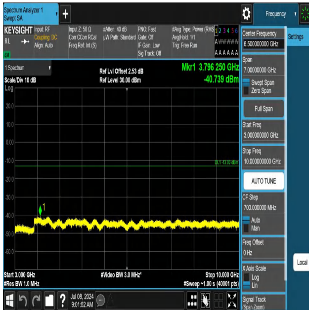
5-5-10MHz-10MHz-QPSK-QPSK-20450-20549-1RB#0-1RB#49-3 000~10000MHz-PASS
