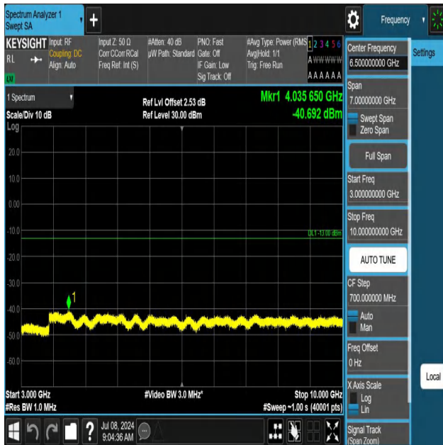
5-5-10MHz-10MHz-QPSK-QPSK-20501-20600-1RB#0-ORB#0-30 00~10000MHz-PASS
