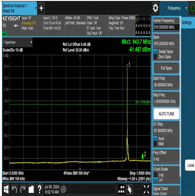
5-5-5MHz-10MHz-QPSK-QPSK-20528-20600-1RB#24-0RB#0-30 ~1000MHz-PASS
