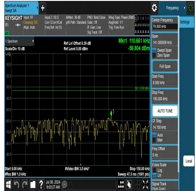
5-5-10MHz-10MHz-QPSK-QPSK-20476-20575-1RB#0-1RB#49-0 .009~0.15MHz-PASS
