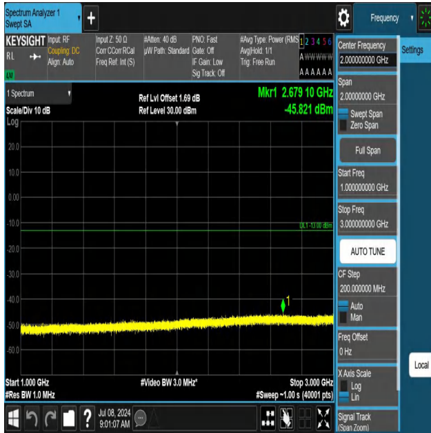
5-5-10MHz-10MHz-QPSK-QPSK-20450-20549-1RB#49-0RB#0-1 000~3000MHz-PASS
