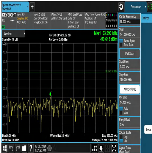
5-5-10MHz-10MHz-QPSK-QPSK-20450-20549-1RB#0-1RB#49-0 .009~0.15MHz-PASS
