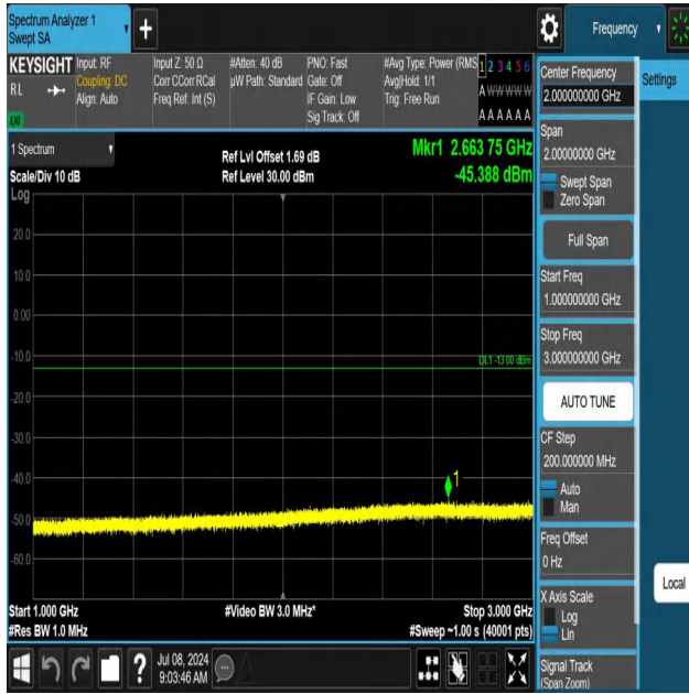
5-5-10MHz-10MHz-QPSK-QPSK-20476-20575-1RB#0-1RB#49-1 000~3000MHz-PASS
