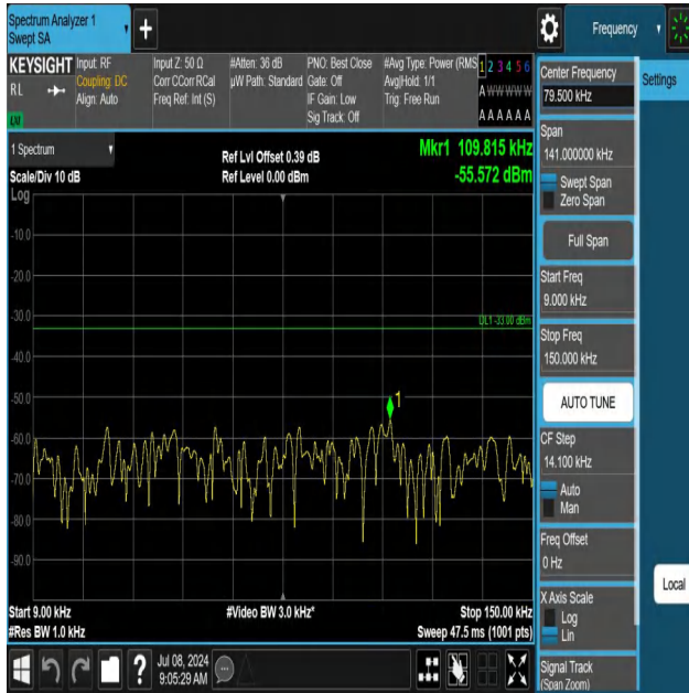
5-5-10MHz-10MHz-QPSK-QPSK-20501-20600-1RB#0-1RB#49-0 .009~0.15MHz-PASS
