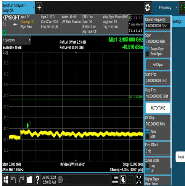
5-5-5MHz-10MHz-QPSK-QPSK-20478-20550-1RB#0-1RB#49-30 00~10000MHz-PASS
