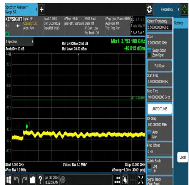
5-5-5MHz-10MHz-QPSK-QPSK-20528-20600-1RB#0-1RB#49-30 00~10000MHz-PASS
