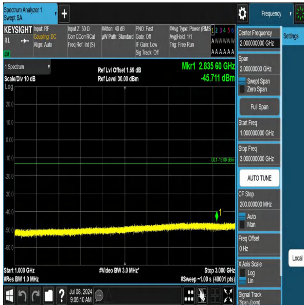
5-5-10MHz-10MHz-QPSK-QPSK-20501-20600-1RB#49-0RB#0-1 000~3000MHz-PASS
