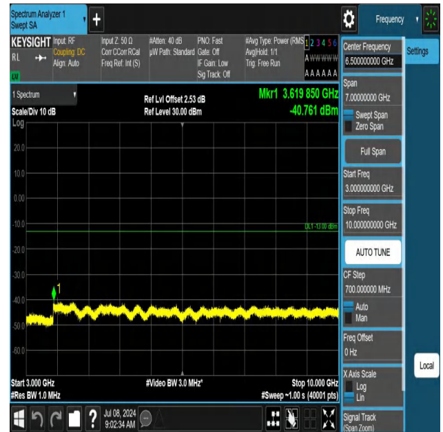
5-5-10MHz-10MHz-QPSK-QPSK-20476-20575-1RB#0-ORB#0-30 00~10000MHz-PASS
