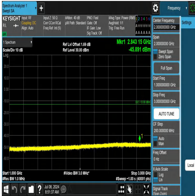
5-5-5MHz-10MHz-QPSK-QPSK-20528-20600-1RB#0-ORB#0-100 0~3000MHz-PASS
