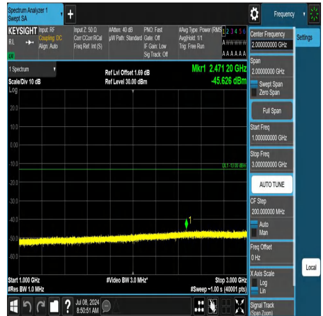
5-5-5MHz-10MHz-QPSK-QPSK-20478-20550-1RB#0-1RB#49-10 00~3000MHz-PASS
