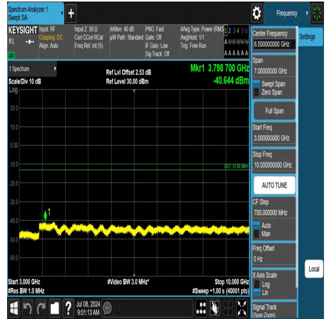
5-5-10MHz-10MHz-QPSK-QPSK-20450-20549-1RB#49-0RB#0-3 000~10000MHz-PASS
