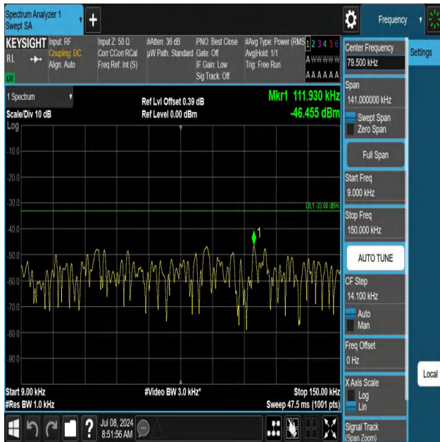
5-5-5MHz-10MHz-QPSK-QPSK-20528-20600-1RB#24-ORB#0-0. 009~0.15MHz-PASS
