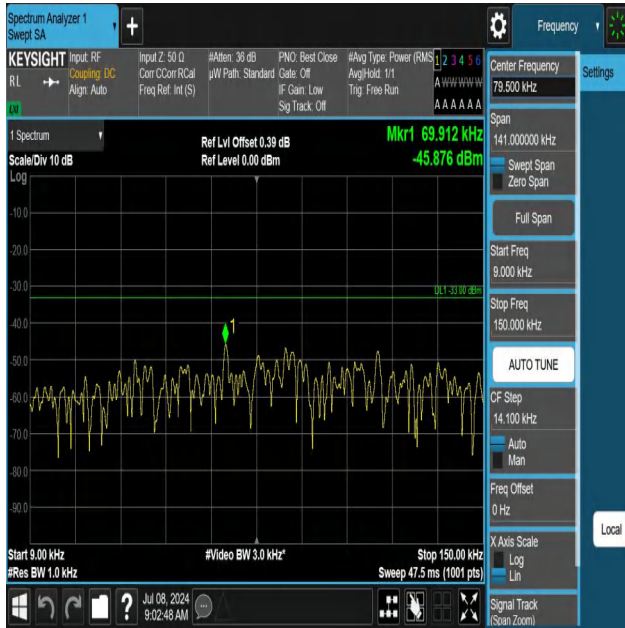
5-5-10MHz-10MHz-QPSK-QPSK-20476-20575-1RB#49-0RB#0-0 .009~0.15MHz-PASS
