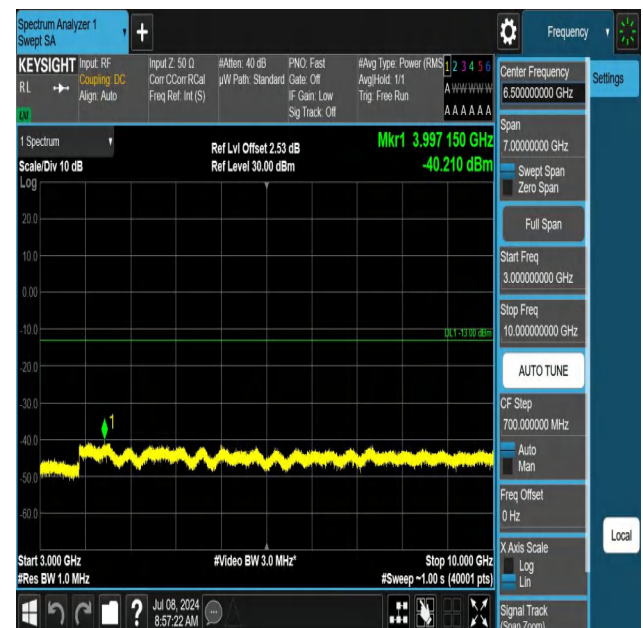
5-5-10MHz-5MHz-QPSK-QPSK-20500-20572-1RB#0-1RB#24-30 00~10000MHz-PASS
