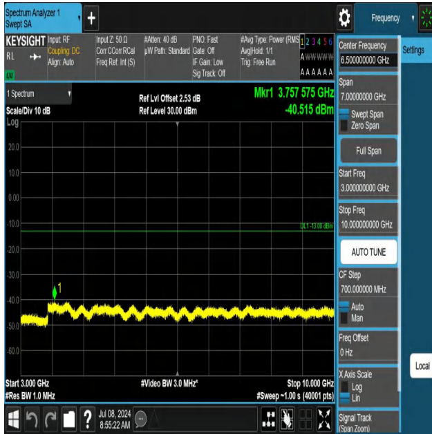
5-5-10MHz-5MHz-QPSK-QPSK-20450-20522-1RB#0-1RB#24-30 00~10000MHz-PASS
