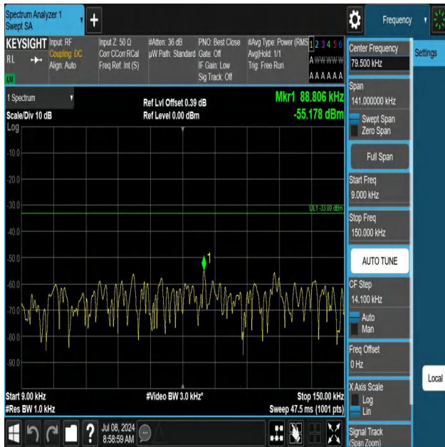
5-5-10MHz-5MHz-QPSK-QPSK-20550-20622-1RB#0-1RB#24-0. 009~0.15MHz-PASS
