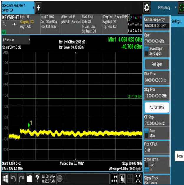
5-5-10MHz-5MHz-QPSK-QPSK-20550-20622-1RB#0-ORB#0-300 0~10000MHz-PASS
