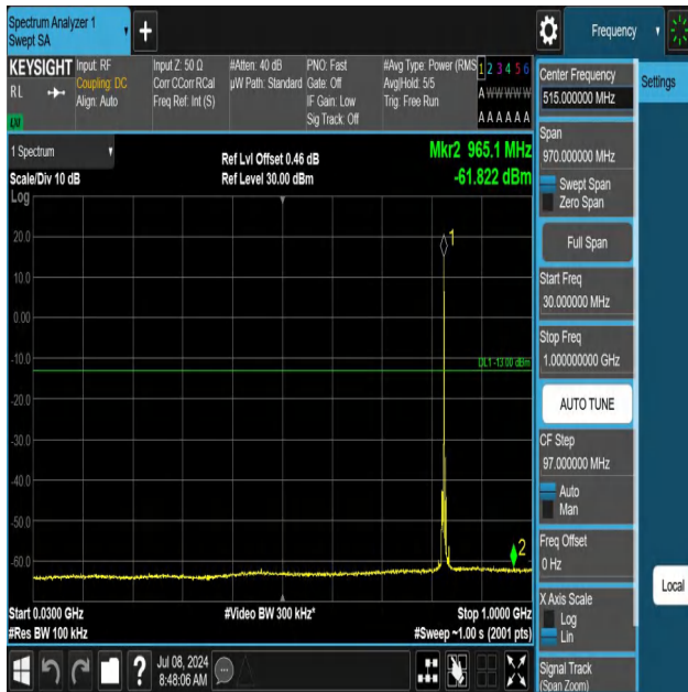
5-5-5MHz-10MHz-QPSK-QPSK-20428-20500-1RB#24-ORB#0-30 ~1000MHz-PASS
