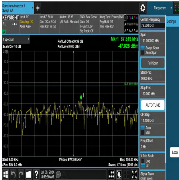
5-5-10MHz-5MHz-QPSK-QPSK-20450-20522-1RB#0-0RB#0-0.0 09~0.15MHz-PASS
