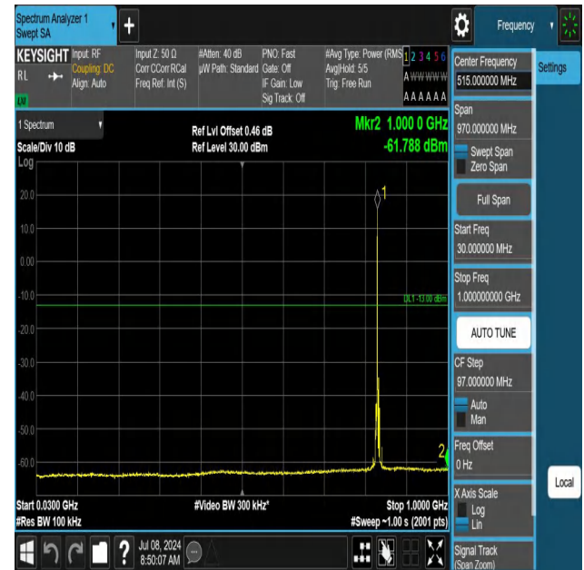
5-5-5MHz-10MHz-QPSK-QPSK-20478-20550-1RB#24-0RB#0-30 ~1000MHz-PASS
