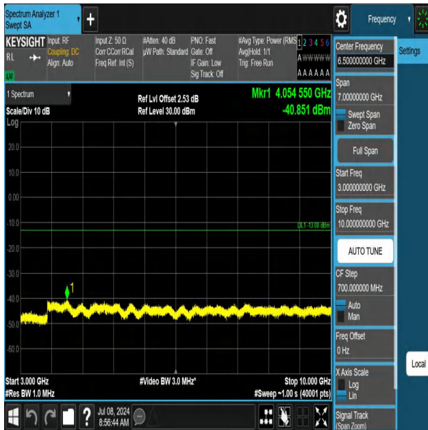
5-5-10MHz-5MHz-QPSK-QPSK-20500-20572-1RB#49-0RB#0-30 00~10000MHz-PASS
