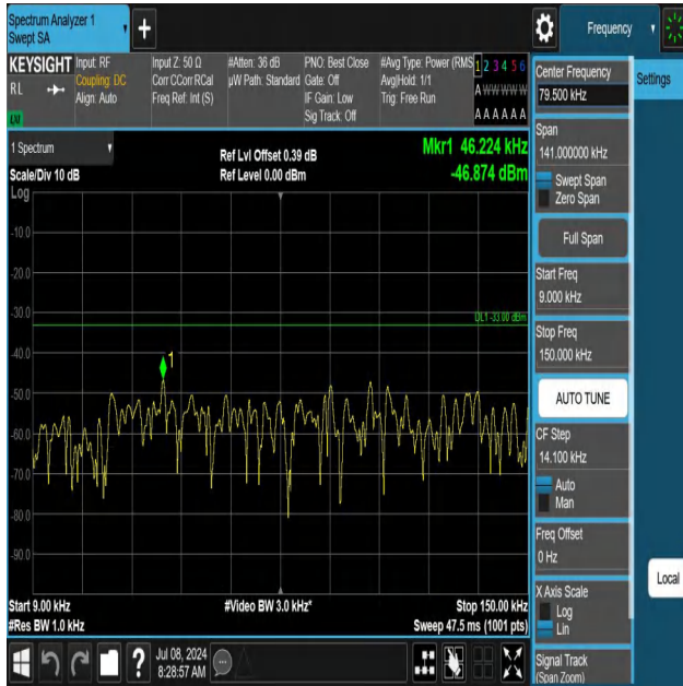
5-5-3MHz-5MHz-QPSK-QPSK-20586-20625-1RB#14-0RB#0-0.0 09~0.15MHz-PASS
