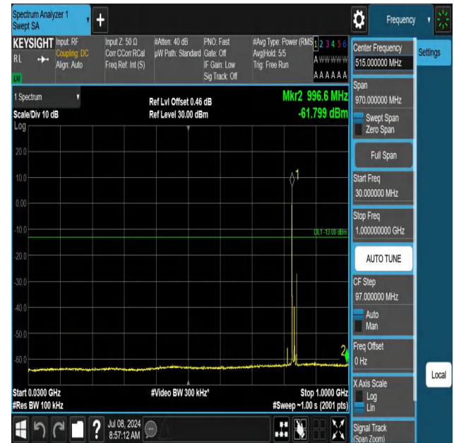
5-5-10MHz-5MHz-QPSK-QPSK-20500-20572-1RB#0-1RB#24-30 ~1000MHz-PASS
