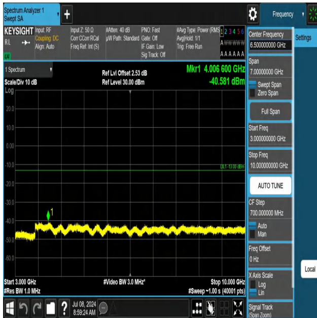
5-5-10MHz-5MHz-QPSK-QPSK-20550-20622-1RB#0-1RB#24-30 00~10000MHz-PASS
