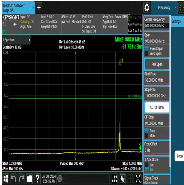
5-5-10MHz-5MHz-QPSK-QPSK-20500-20572-1RB#49-0RB#0-30 ~1000MHz-PASS
