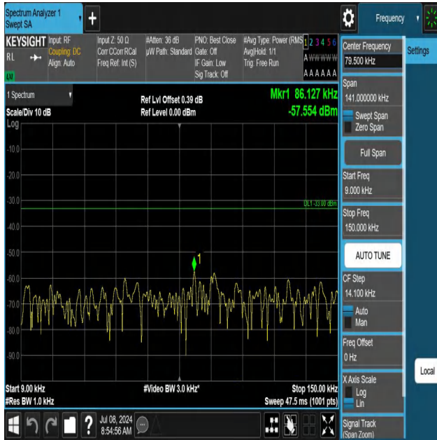
5-5-10MHz-5MHz-QPSK-QPSK-20450-20522-1RB#0-1RB#24-0. 009~0.15MHz-PASS
