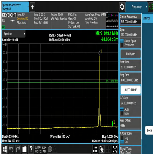
5-5-10MHz-5MHz-QPSK-QPSK-20550-20622-1RB#0-0RB#0-30~ 1000MHz-PASS
