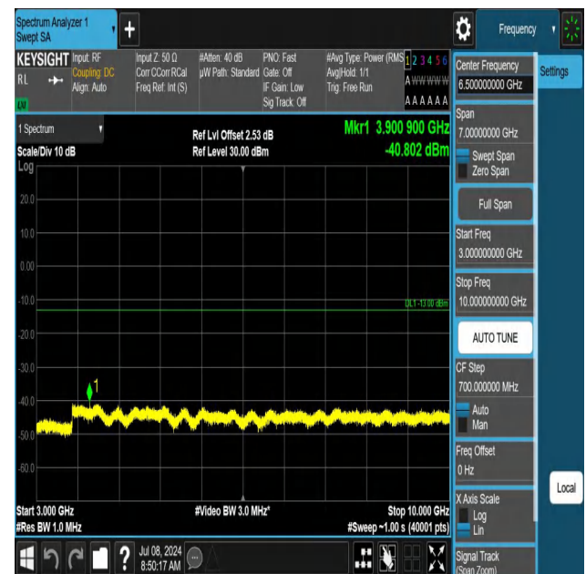
5-5-5MHz-10MHz-QPSK-QPSK-20478-20550-1RB#24-0RB#0-30 00~10000MHz-PASS
