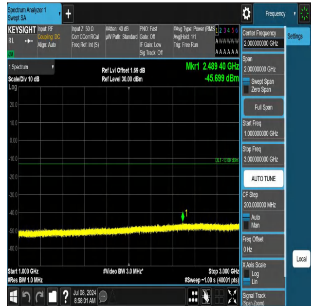
5-5-10MHz-5MHz-QPSK-QPSK-20550-20622-1RB#0-0RB#0-100 0~3000MHz-PASS
