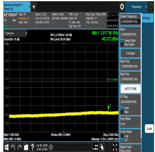
5-5-10MHz-5MHz-QPSK-QPSK-20450-20522-1RB#0-1RB#24-10 00~3000MHz-PASS
