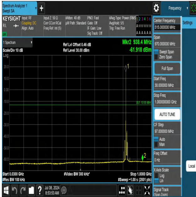
5-5-10MHz-5MHz-QPSK-QPSK-20450-20522-1RB#0-ORB#0-30~ 1000MHz-PASS
