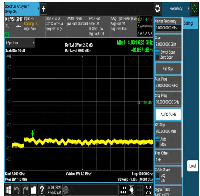
5-5-10MHz-5MHz-QPSK-QPSK-20450-20522-1RB#49-ORB#0-30 00~10000MHz-PASS
