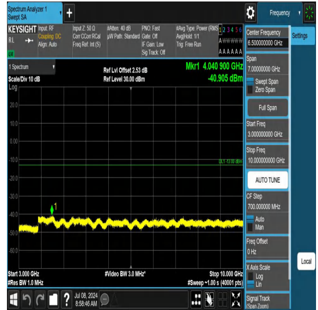
5-5-10MHz-5MHz-QPSK-QPSK-20550-20622-1RB#49-0RB#0-30 00~10000MHz-PASS
