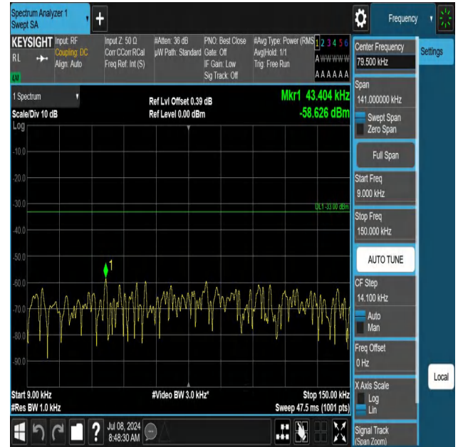
5-5-5MHz-10MHz-QPSK-QPSK-20428-20500-1RB#0-1RB#49-0. 009~0.15MHz-PASS
