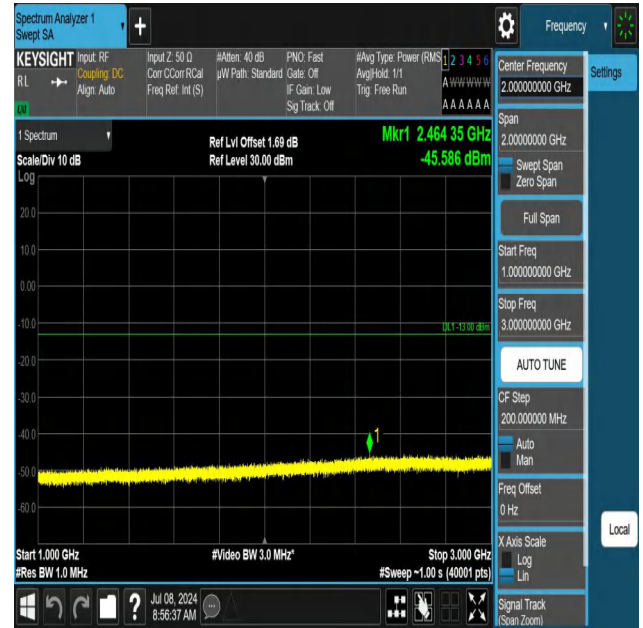
5-5-10MHz-5MHz-QPSK-QPSK-20500-20572-1RB#49-0RB#0-10 00~3000MHz-PASS
