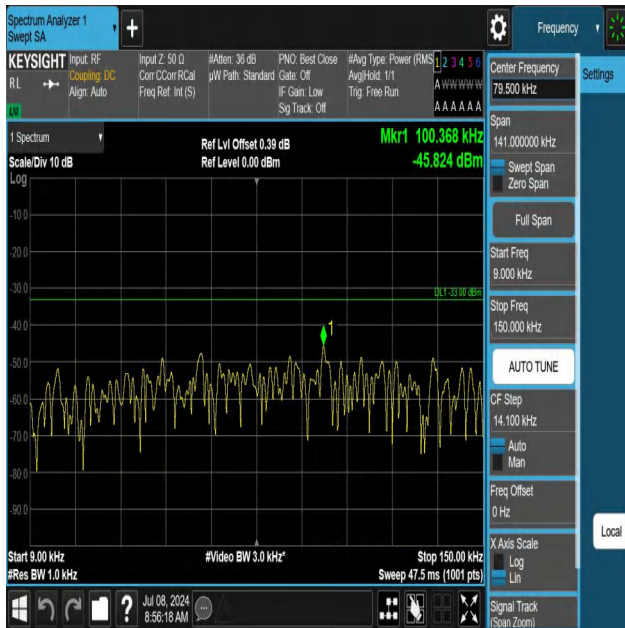
5-5-10MHz-5MHz-QPSK-QPSK-20500-20572-1RB#49-ORB#0-0. 009~0.15MHz-PASS
