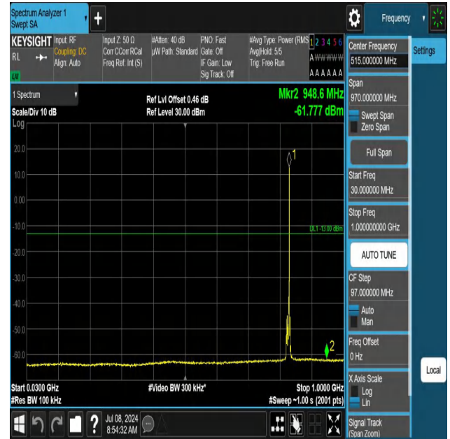
5-5-10MHz-5MHz-QPSK-QPSK-20450-20522-1RB#49-ORB#0-30 ~1000MHz-PASS
