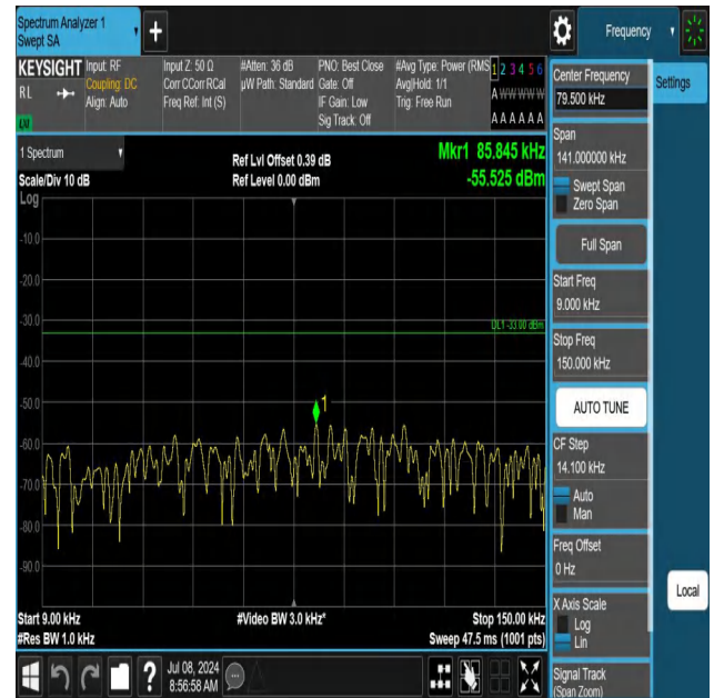
5-5-10MHz-5MHz-QPSK-QPSK-20500-20572-1RB#0-1RB#24-0. 009~0.15MHz-PASS
