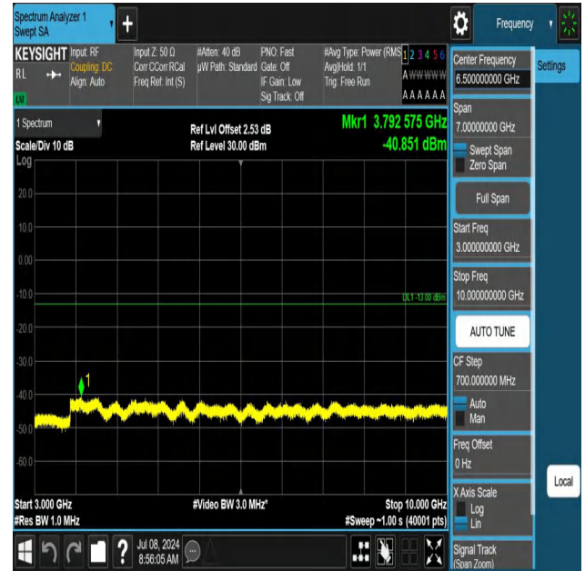
5-5-10MHz-5MHz-QPSK-QPSK-20500-20572-1RB#0-ORB#0-300 0~10000MHz-PASS
