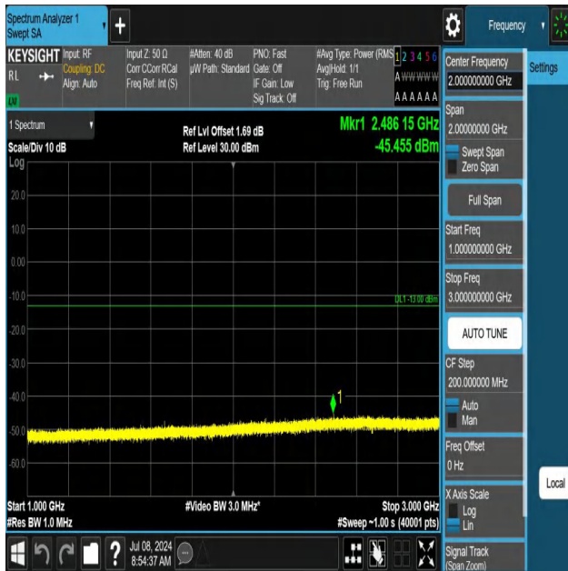
5-5-10MHz-5MHz-QPSK-QPSK-20450-20522-1RB#49-ORB#0-10 00~3000MHz-PASS
