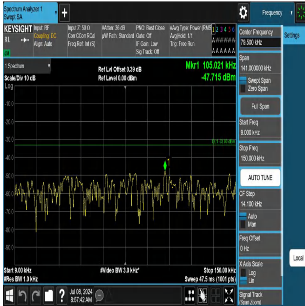
5-5-10MHz-5MHz-QPSK-QPSK-20550-20622-1RB#0-0RB#0-0.0 09~0.15MHz-PASS
