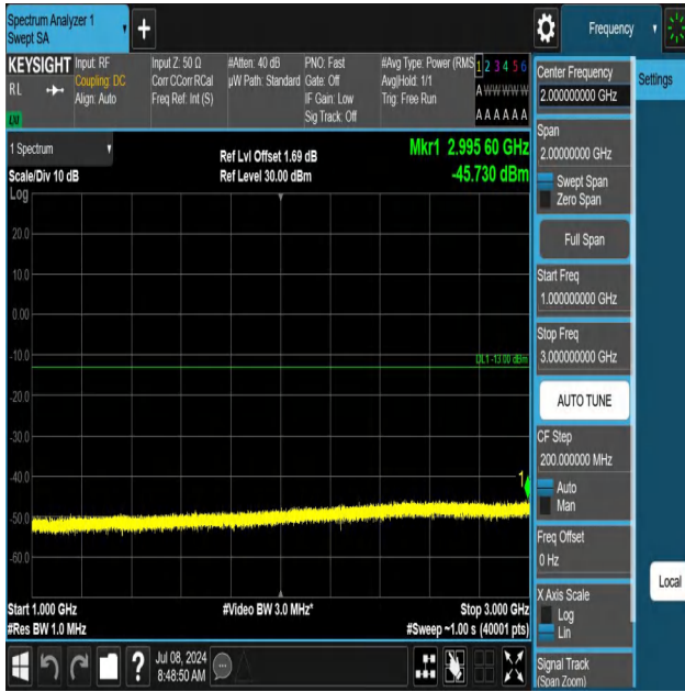
5-5-5MHz-10MHz-QPSK-QPSK-20428-20500-1RB#0-1RB#49-10 00~3000MHz-PASS
