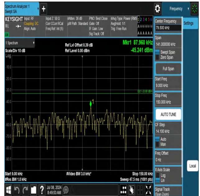
5-5-5MHz-10MHz-QPSK-QPSK-20478-20550-1RB#24-ORB#0-0. 009~0.15MHz-PASS
