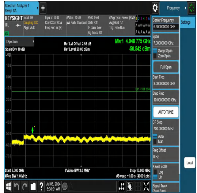
5-5-3MHz-5MHz-QPSK-QPSK-20586-20625-1RB#0-1RB#24-300 0~10000MHz-PASS
