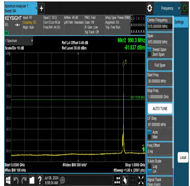
5-5-10MHz-5MHz-QPSK-QPSK-20550-20622-1RB#49-ORB#0-30 ~1000MHz-PASS
