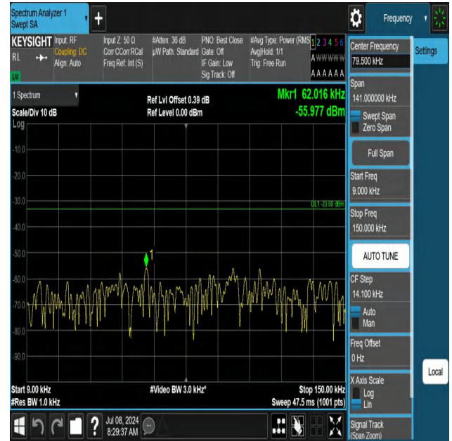
5-5-3MHz-5MHz-QPSK-QPSK-20586-20625-1RB#0-1RB#24-0.0 09~0.15MHz-PASS
