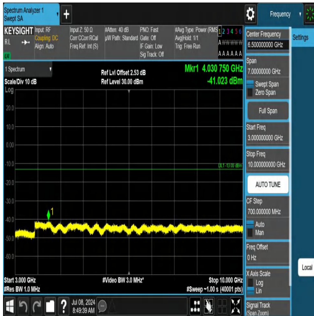
5-5-5MHz-10MHz-QPSK-QPSK-20478-20550-1RB#0-ORB#0-300 0~10000MHz-PASS
