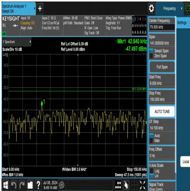
5-5-5MHz-10MHz-QPSK-QPSK-20478-20550-1RB#0-0RB#0-0.0 09~0.15MHz-PASS
