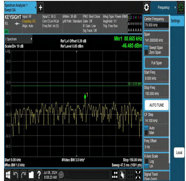
5-5-10MHz-5MHz-QPSK-QPSK-20550-20622-1RB#49-ORB#0-0. 009~0.15MHz-PASS
