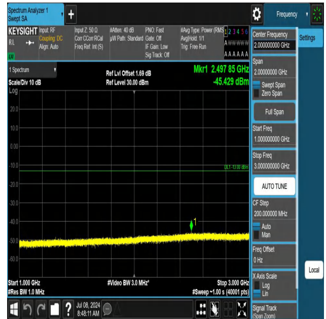
5-5-5MHz-10MHz-QPSK-QPSK-20428-20500-1RB#24-ORB#0-10 00~3000MHz-PASS
