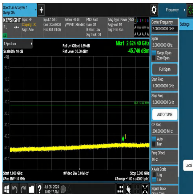
5-5-10MHz-5MHz-QPSK-QPSK-20500-20572-1RB#0-1RB#24-10 00~3000MHz-PASS
