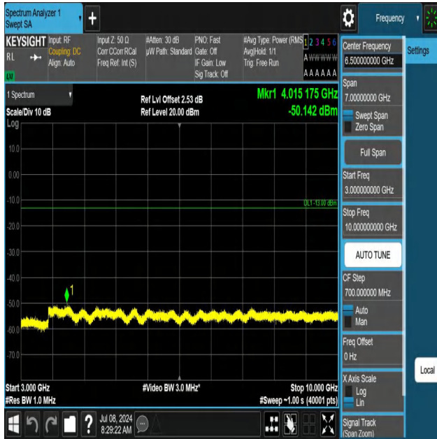
5-5-3MHz-5MHz-QPSK-QPSK-20586-20625-1RB#14-0RB#0-300 0~10000MHz-PASS
