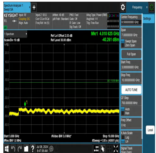
5-5-5MHz-10MHz-QPSK-QPSK-20428-20500-1RB#0-ORB#0-300 0~10000MHz-PASS
