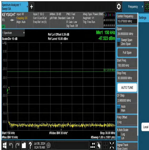
5-5-3MHz-5MHz-QPSK-QPSK-20416-20455-1RB#0-0RB#0-0.15 ~30MHz-PASS
