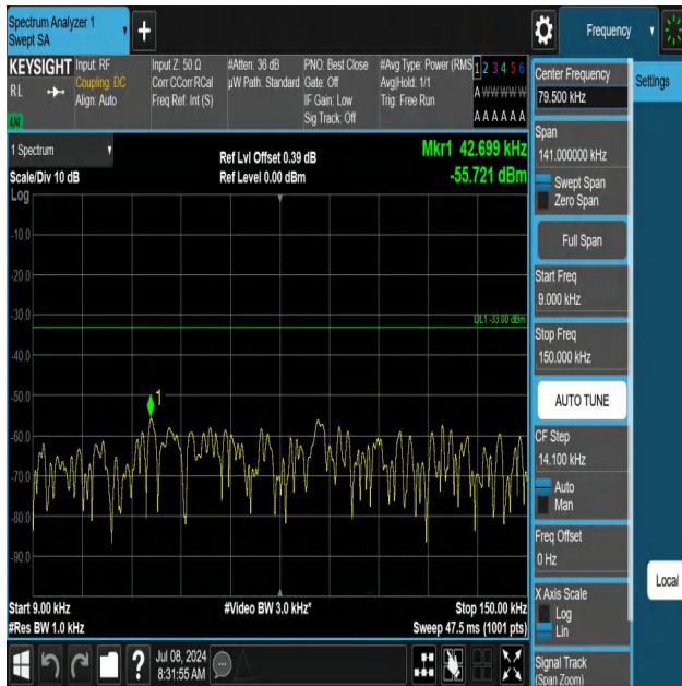
5-5-5MHz-3MHz-QPSK-QPSK-20425-20464-1RB#0-1RB#15-0.0 09~0.15MHz-PASS
