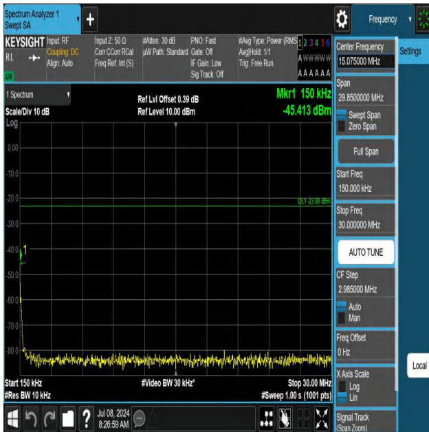
5-5-3MHz-5MHz-QPSK-QPSK-20501-20540-1RB#14-0RB#0-0.1 5~30MHz-PASS
