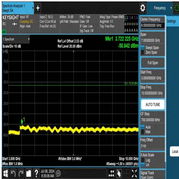
5-5-5MHz-3MHz-QPSK-QPSK-20595-20634-1RB#0-ORB#0-3000 ~10000MHz-PASS
