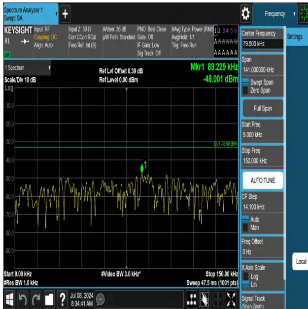
5-5-5MHz-3MHz-QPSK-QPSK-20595-20634-1RB#0-0RB#0-0.00 9~0.15MHz-PASS
