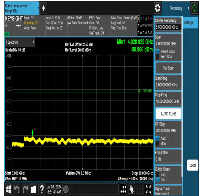
5-5-5MHz-3MHz-QPSK-QPSK-20425-20464-1RB#24-0RB#0-300 0~10000MHz-PASS
