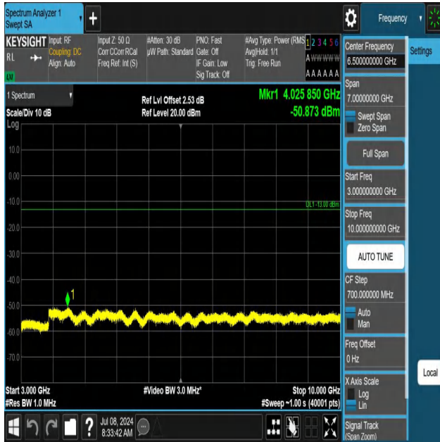
5-5-5MHz-3MHz-QPSK-QPSK-20510-20549-1RB#24-0RB#0-300 0~10000MHz-PASS
