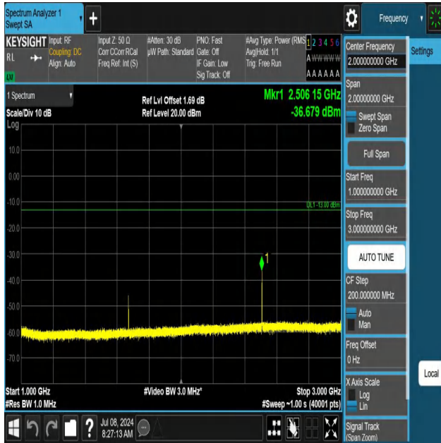
5-5-3MHz-5MHz-QPSK-QPSK-20501-20540-1RB#14-0RB#0-100 0~3000MHz-PASS
