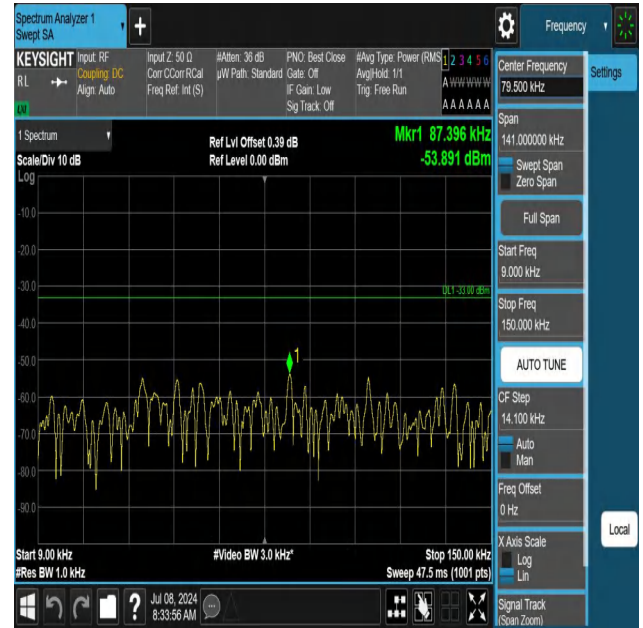
5-5-5MHz-3MHz-QPSK-QPSK-20510-20549-1RB#0-1RB#15-0.0 09~0.15MHz-PASS
