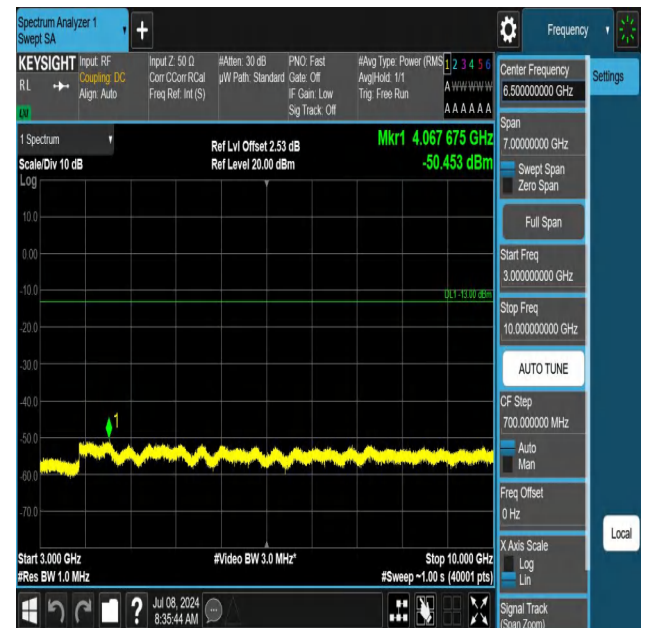
5-5-5MHz-3MHz-QPSK-QPSK-20595-20634-1RB#24-0RB#0-300 0~10000MHz-PASS
