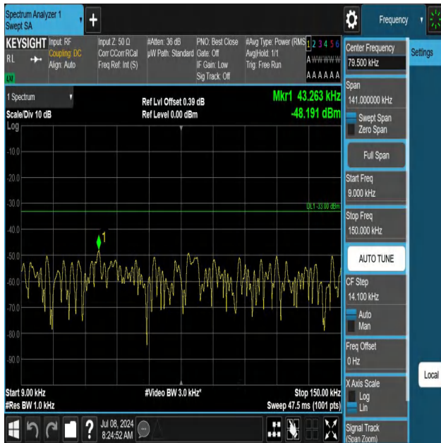
5-5-3MHz-5MHz-QPSK-QPSK-20416-20455-1RB#14-0RB#0-0.0 09~0.15MHz-PASS
