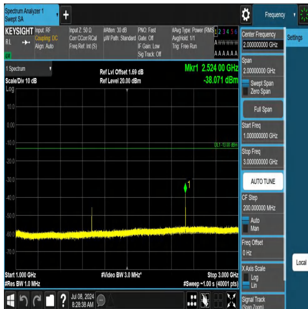
5-5-3MHz-5MHz-QPSK-QPSK-20586-20625-1RB#0-0RB#0-1000 ~3000MHz-PASS
