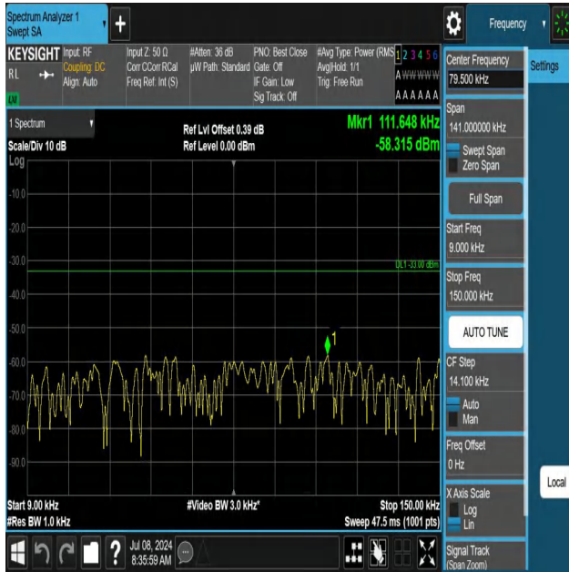
5-5-5MHz-3MHz-QPSK-QPSK-20595-20634-1RB#0-1RB#15-0.0 09~0.15MHz-PASS
