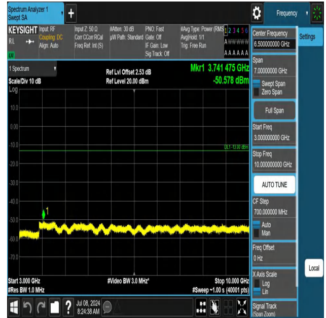
5-5-3MHz-5MHz-QPSK-QPSK-20416-20455-1RB#0-0RB#0-3000 ~10000MHz-PASS
