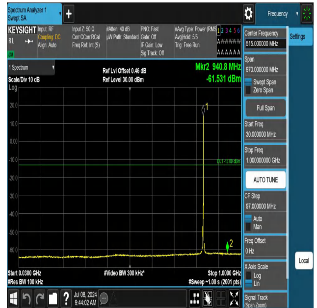
5-5-3MHz-5MHz-QPSK-QPSK-20501-20540-1RB#14-0RB#0-30~ 1000MHz-PASS
