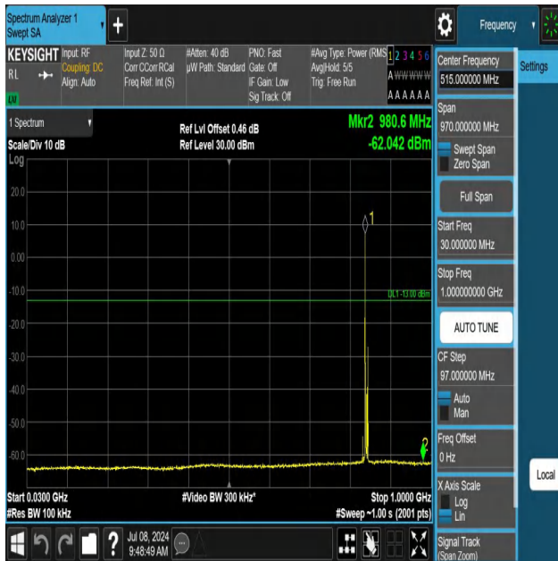
5-5-5MHz-3MHz-QPSK-QPSK-20595-20634-1RB#0-1RB#15-30~ 1000MHz-PASS
