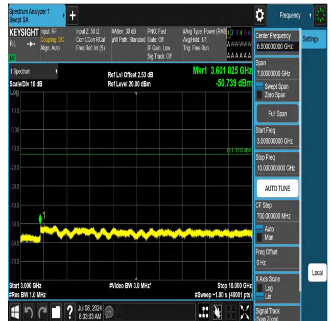
5-5-5MHz-3MHz-QPSK-QPSK-20510-20549-1RB#0-0RB#0-3000 ~10000MHz-PASS
