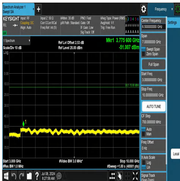
5-5-3MHz-5MHz-QPSK-QPSK-20501-20540-1RB#0-1RB#24-300 0~10000MHz-PASS
