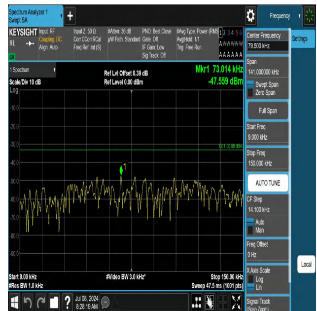
5-5-3MHz-5MHz-QPSK-QPSK-20586-20625-1RB#0-0RB#0-0.00 9~0.15MHz-PASS
