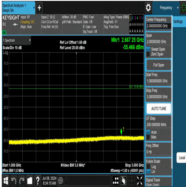
5-5-5MHz-3MHz-QPSK-QPSK-20510-20549-1RB#0-1RB#15-100 0~3000MHz-PASS
