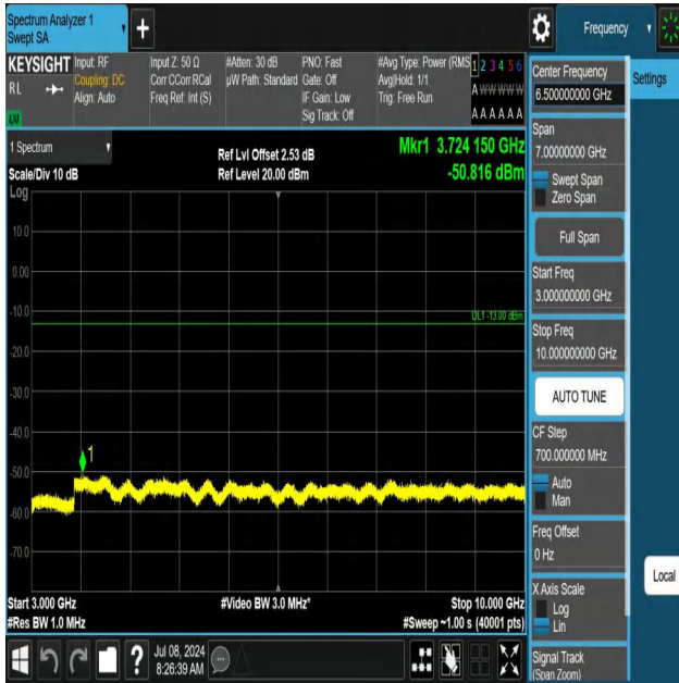
5-5-3MHz-5MHz-QPSK-QPSK-20501-20540-1RB#0-0RB#0-3000 ~10000MHz-PASS
