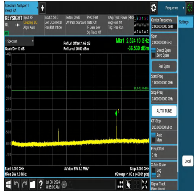
5-5-5MHz-3MHz-QPSK-QPSK-20595-20634-1RB#0-ORB#0-1000 ~3000MHz-PASS
