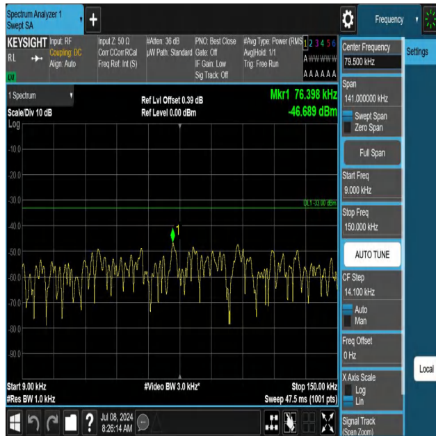
5-5-3MHz-5MHz-QPSK-QPSK-20501-20540-1RB#0-0RB#0-0.00 9~0.15MHz-PASS
