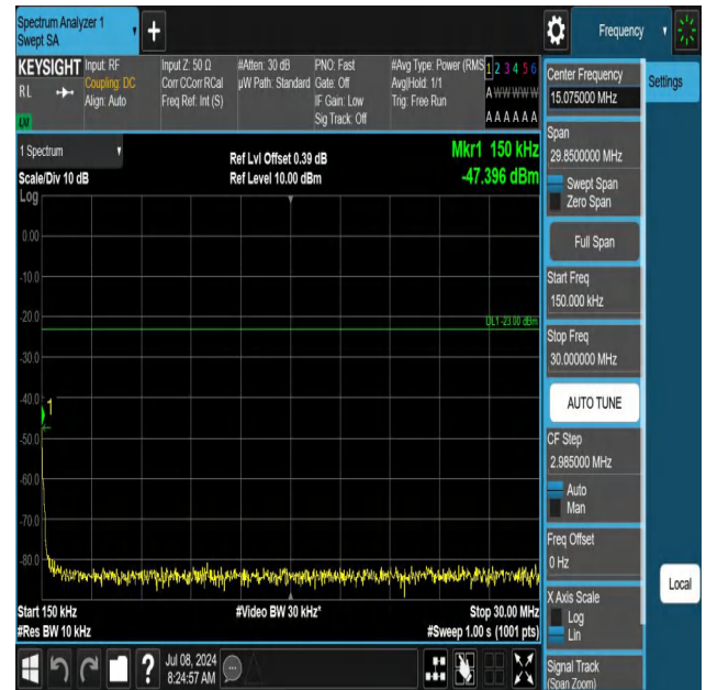
5-5-3MHz-5MHz-QPSK-QPSK-20416-20455-1RB#14-0RB#0-0.1 5~30MHz-PASS
