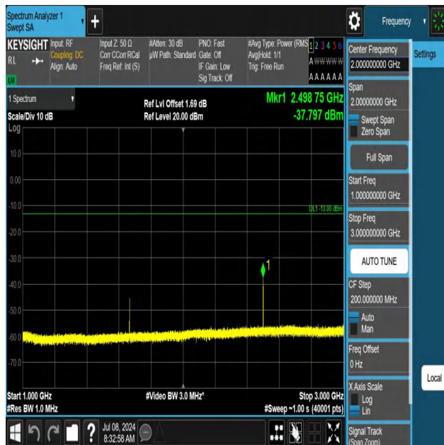
5-5-5MHz-3MHz-QPSK-QPSK-20510-20549-1RB#0-0RB#0-1000 ~3000MHz-PASS
