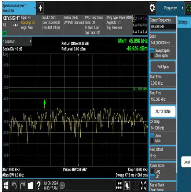
5-5-5MHz-3MHz-QPSK-QPSK-20510-20549-1RB#24-0RB#0-0.0 09~0.15MHz-PASS
