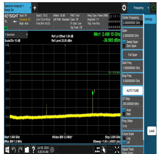
5-5-3MHz-5MHz-QPSK-QPSK-20501-20540-1RB#0-0RB#0-1000 ~3000MHz-PASS
