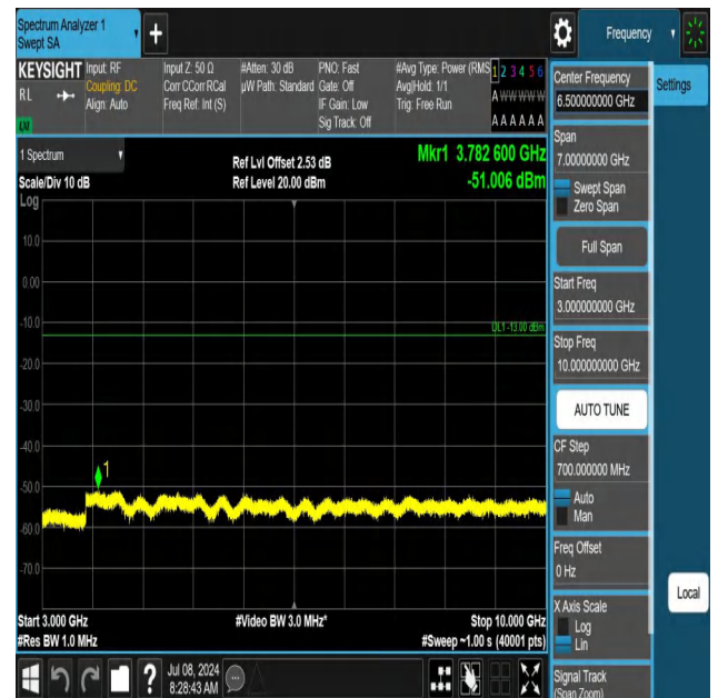
5-5-3MHz-5MHz-QPSK-QPSK-20586-20625-1RB#0-0RB#0-3000 ~10000MHz-PASS
