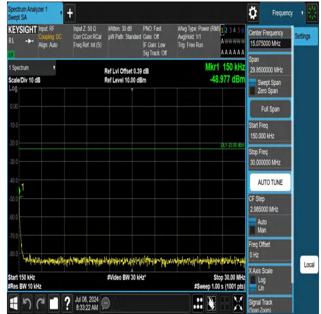
5-5-5MHz-3MHz-QPSK-QPSK-20510-20549-1RB#24-0RB#0-0.1 5~30MHz-PASS
