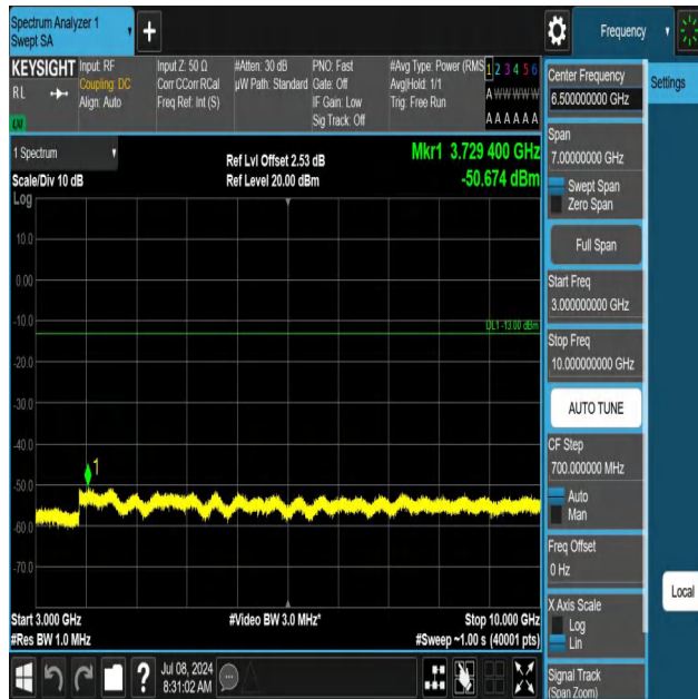
5-5-5MHz-3MHz-QPSK-QPSK-20425-20464-1RB#0-0RB#0-3000 ~10000MHz-PASS
