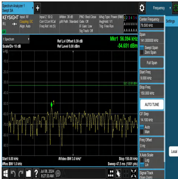
5-5-3MHz-5MHz-QPSK-QPSK-20501-20540-1RB#0-1RB#24-0.0 09~0.15MHz-PASS
