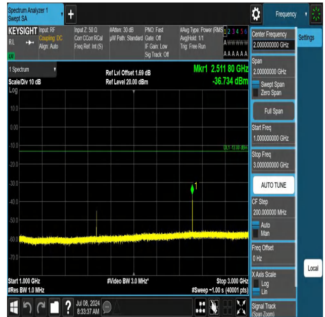
5-5-5MHz-3MHz-QPSK-QPSK-20510-20549-1RB#24-0RB#0-100 0~3000MHz-PASS
