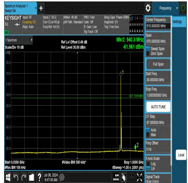
5-5-5MHz-3MHz-QPSK-QPSK-20510-20549-1RB#0-1RB#15-30~ 1000MHz-PASS
