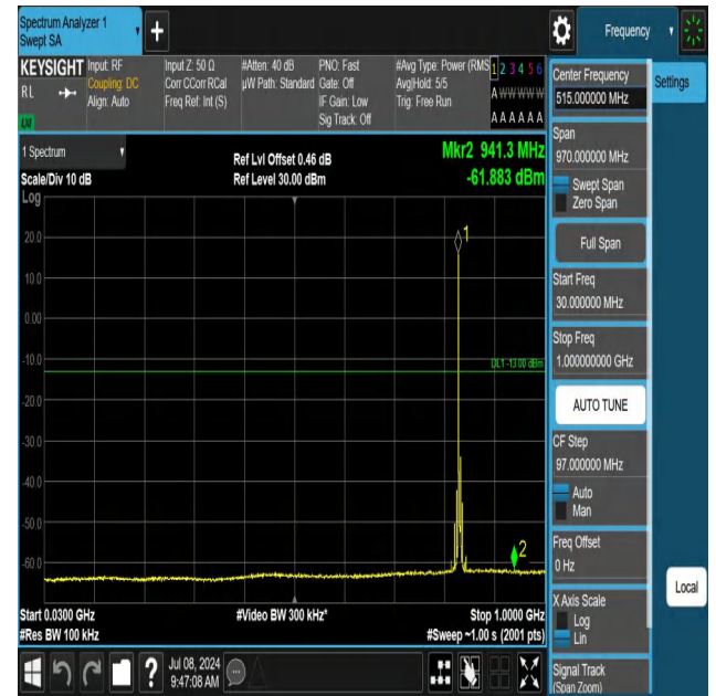
5-5-5MHz-3MHz-QPSK-QPSK-20510-20549-1RB#0-0RB#0-30~1 000MHz-PASS
