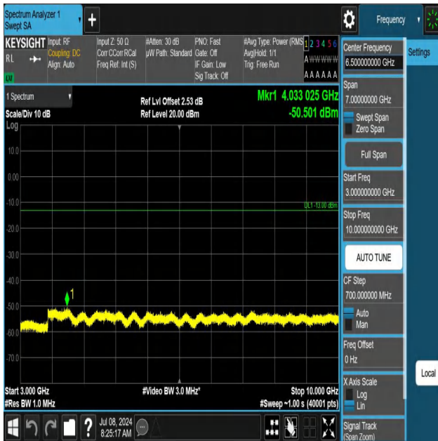
5-5-3MHz-5MHz-QPSK-QPSK-20416-20455-1RB#14-0RB#0-300 0~10000MHz-PASS
