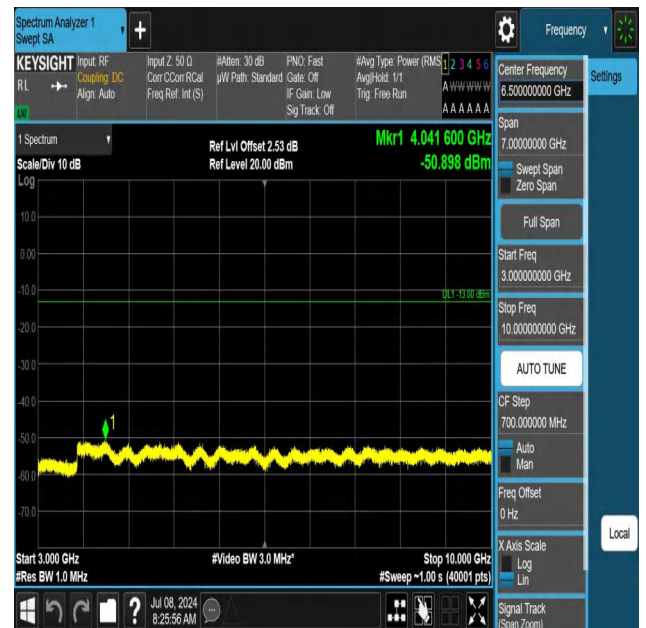
5-5-3MHz-5MHz-QPSK-QPSK-20416-20455-1RB#0-1RB#24-300 0~10000MHz-PASS
