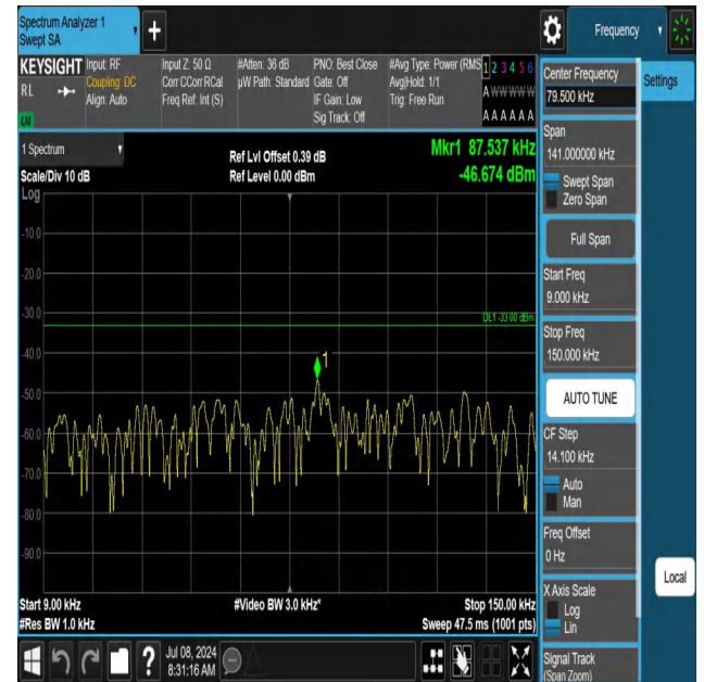
5-5-5MHz-3MHz-QPSK-QPSK-20425-20464-1RB#24-0RB#0-0.0 09~0.15MHz-PASS
