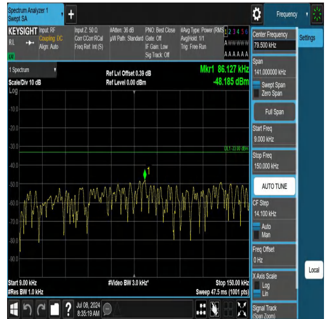
5-5-5MHz-3MHz-QPSK-QPSK-20595-20634-1RB#24-ORB#0-0.0 09~0.15MHz-PASS
