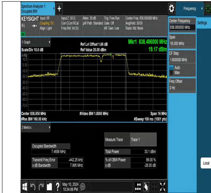
5-5-5MHz-3MHz-QPSK-QPSK-20510-20549-25RB#0-15RB#0-PA SS
