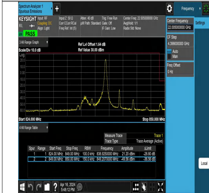
5MHz-10MHz_QPSK@QPSK-QPSK@QPSK_20528-20600_1RB #24@25RB#0-0RB#0@50RB#0
