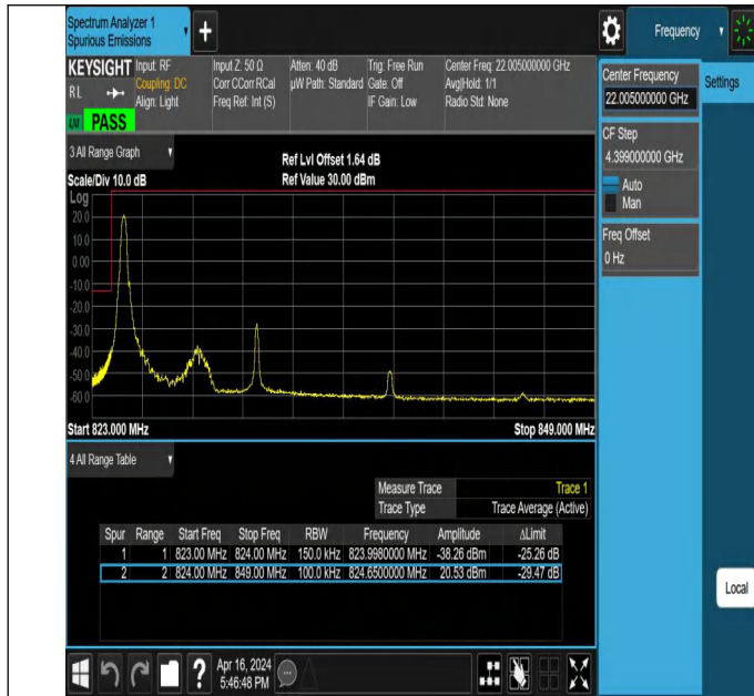
5MHz-10MHz_QPSK@QPSK-QPSK@QPSK_20428-20500_1RB #0@25RB#0-0RB#0@50RB#0
