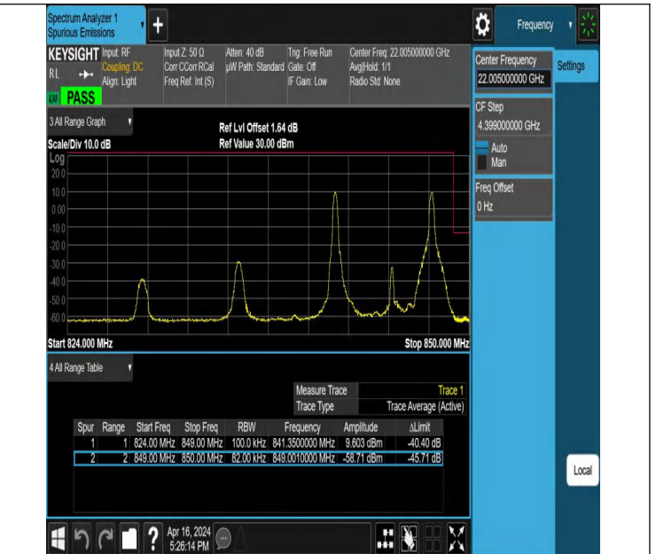
5MHz-3MHz_QPSK@QPSK-QPSK@QPSK_20595-20634_1RB#0@25RB#0-1RB#15@15RB#0
