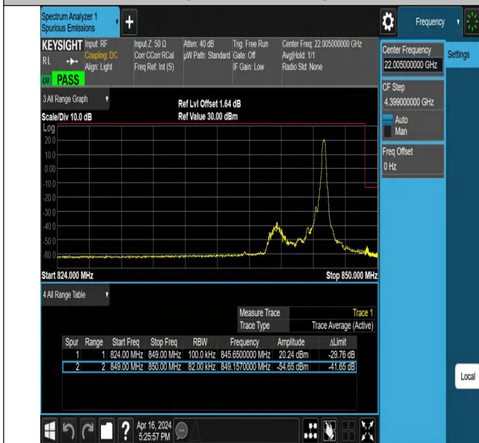
5MHz-3MHz_QPSK@QPSK-QPSK@QPSK_20595-20634_1RB#24@25RB#0-0RB#0@15RB#0
