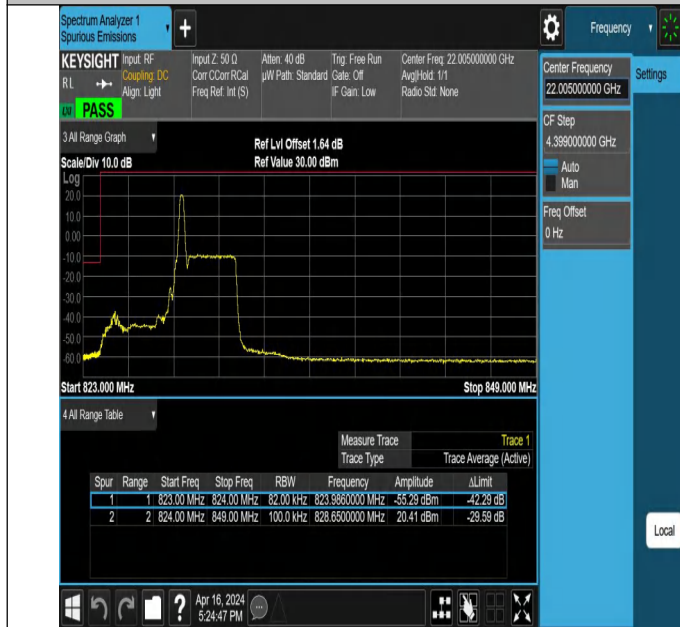
5MHz-3MHz_QPSK@QPSK-QPSK@QPSK_20425-20464_1RB#24@25RB#0-0RB#0@15RB#0
