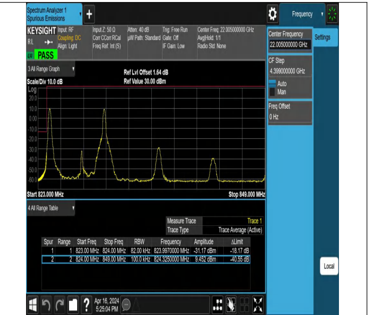
5MHz-3MHz_QPSK@QPSK-QPSK@QPSK_20425-20464_1RB#0@25RB#0-1RB#15@15RB#0
