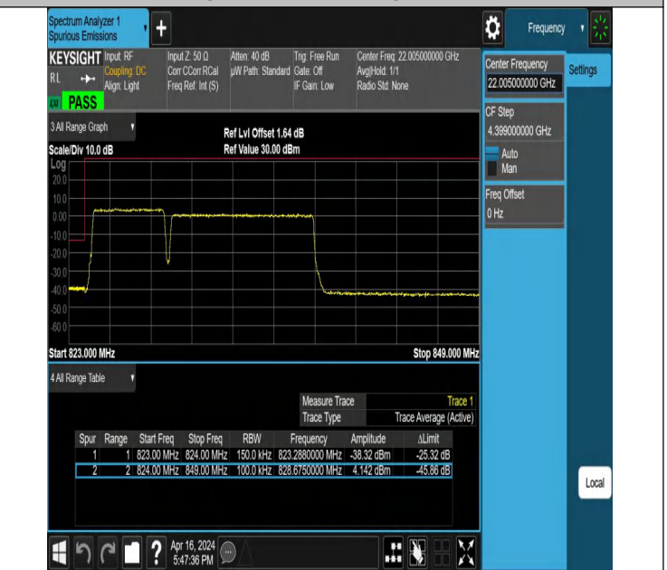
5MHz-10MHz_QPSK@QPSK-QPSK@QPSK_20428-20500_25R B#0@25RB#0-50RB#0@50RB#0
