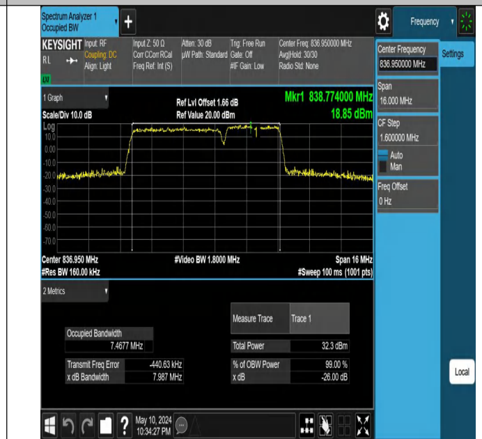
5-5-5MHz-3MHz-16QAM-16QAM-20510-20549-25RB#0-15RB# 0-PASS
