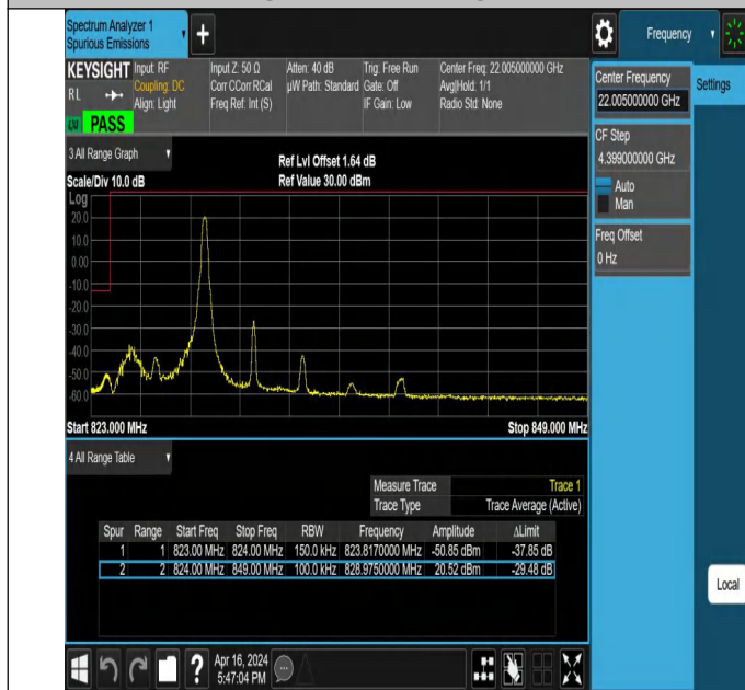
5MHz-10MHz_QPSK@QPSK-QPSK@QPSK_20428-20500_1RB #24@25RB#0-0RB#0@50RB#0
