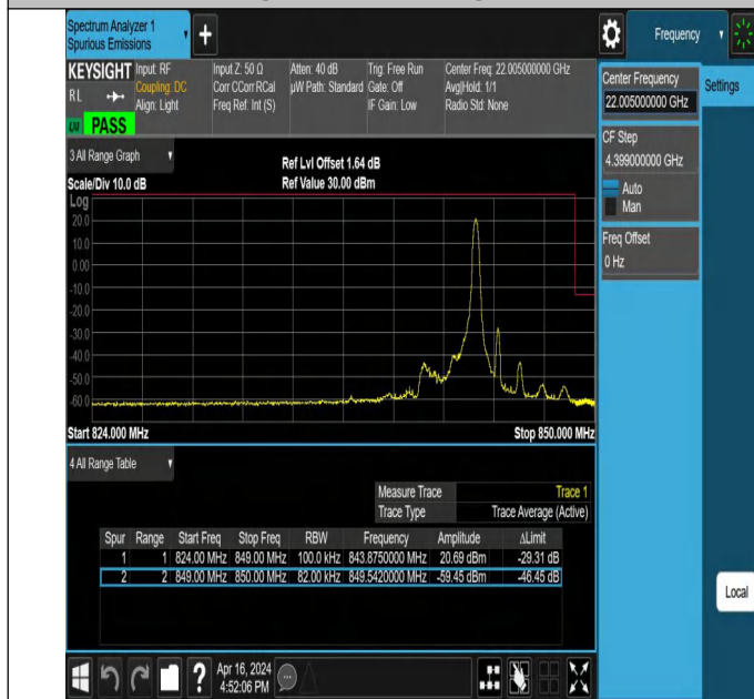
3MHz-5MHz_QPSK@QPSK-QPSK@QPSK_20586-20625_1RB# 14@15RB#0-0RB#0@25RB#0
