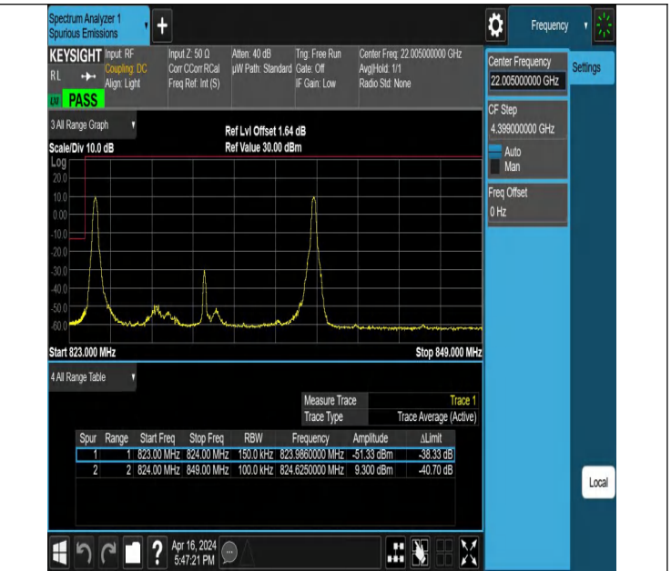
5MHz-10MHz_QPSK@QPSK-QPSK@QPSK_20428-20500_1RB #0@25RB#0-1RB#49@50RB#0
