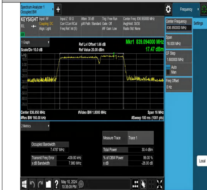
5-5-5MHz-3MHz-256QAM-256QAM-20510-20549-25RB#0-15RB# 0-PASS
