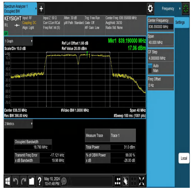
5-5-10MHz-10MHz-64QAM-64QAM-20476-20575-50RB#0-50R B#0-PASS
