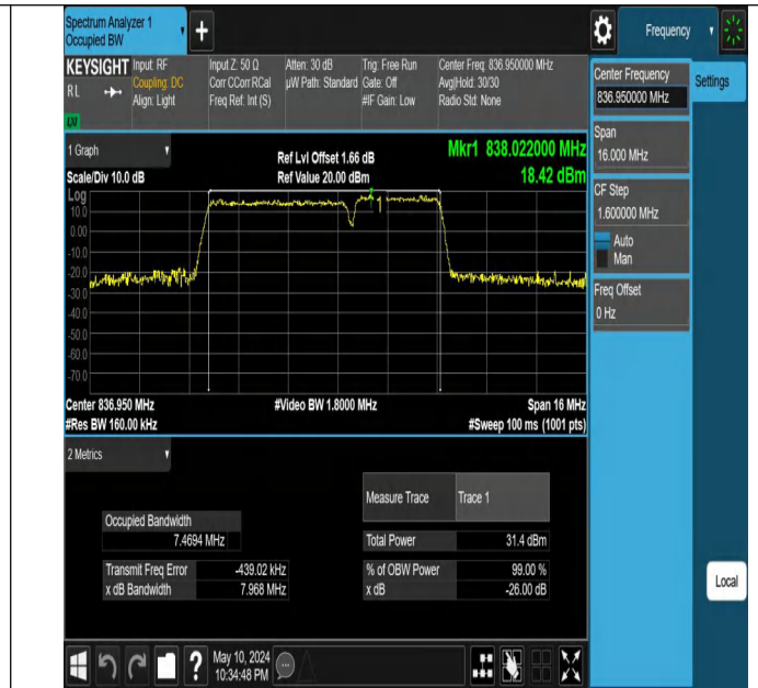
5-5-5MHz-3MHz-64QAM-64QAM-20510-20549-25RB#0-15RB# 0-PASS
