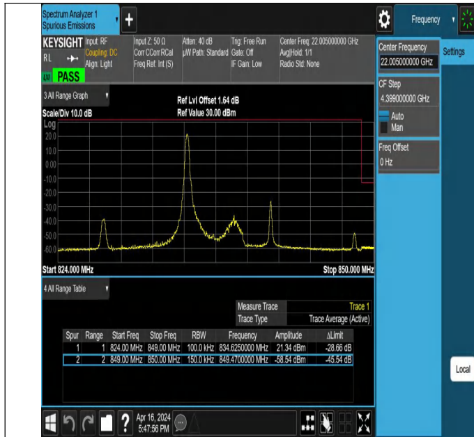
5MHz-10MHz_QPSK@QPSK-QPSK@QPSK_20528-20600_1RB #0@25RB#0-0RB#0@50RB#0
