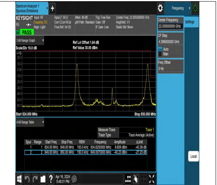
5MHz-10MHz_QPSK@QPSK-QPSK@QPSK_20528-20600_1RB #0@25RB#0-1RB#49@50RB#0
