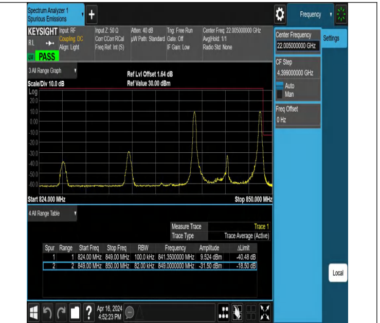
3MHz-5MHz_QPSK@QPSK-QPSK@QPSK_20586-20625_1RB# 0@15RB#0-1RB#24@25RB#0
