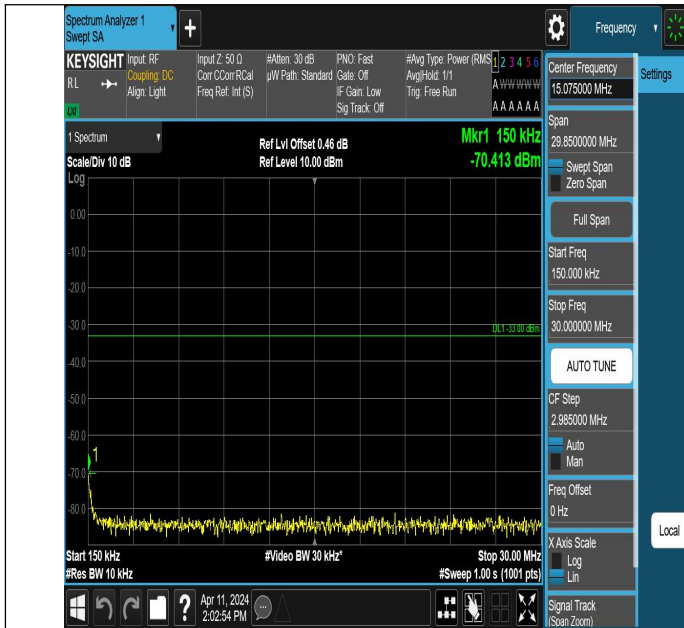
Band66_10MHz_QPSK_132622_1RB#0_0.15~30_0.15~30
