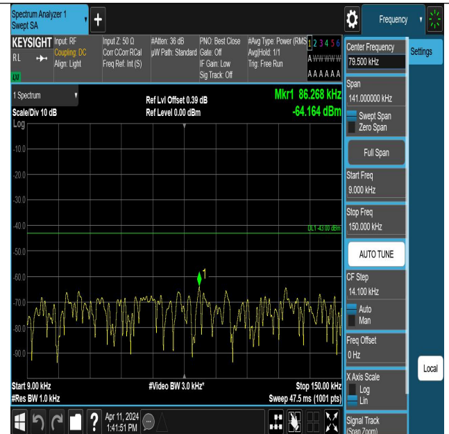
Band66_3MHz_QPSK_132657_1RB#0_0.009~0.15_0.009~0.15
