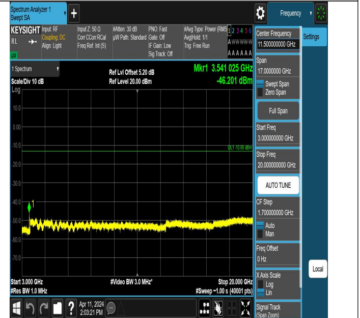
Band66_10MHz_QPSK_132622_1RB#0_3000~20000_3000~200
