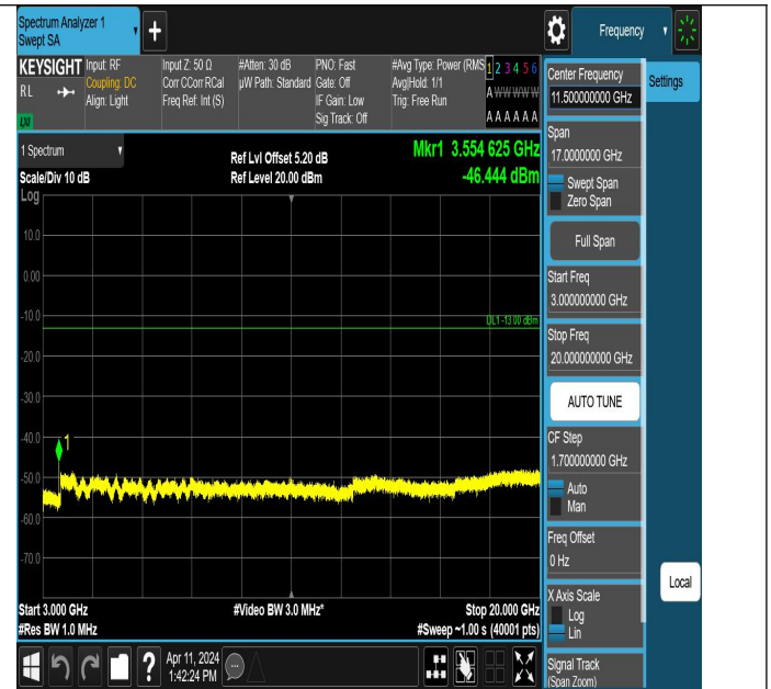
Band66_3MHz_QPSK_132657_1RB#0_3000~20000_3000~2000
