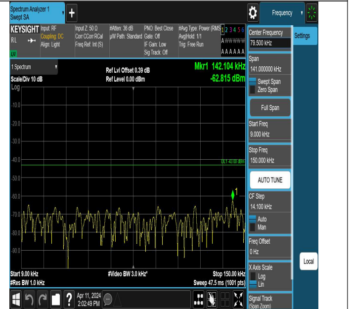
Band66_10MHz_QPSK_132622_1RB#0_0.009~0.15_0.009~0.15
