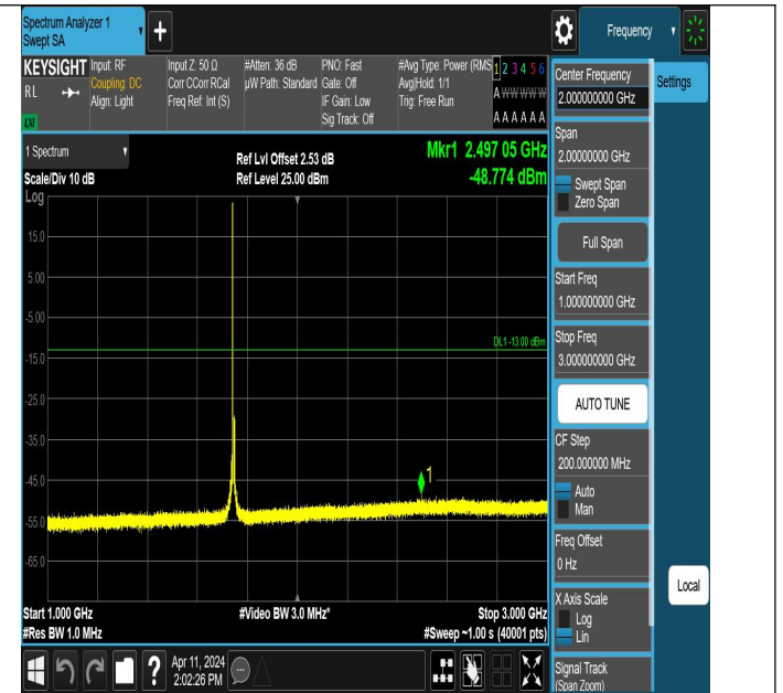
Band66_10MHz_QPSK_132322_1RB#0_1000~3000_1000~3000
