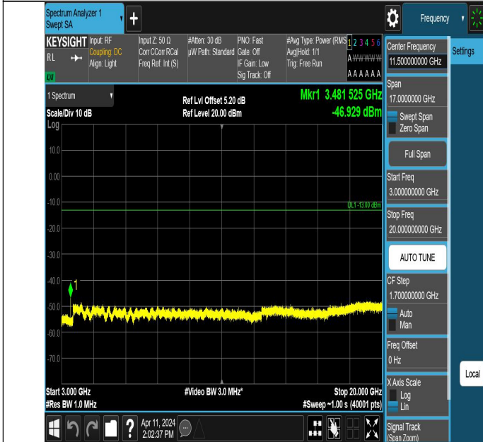
Band66_10MHz_QPSK_132322_1RB#0_3000~20000_3000~2000
