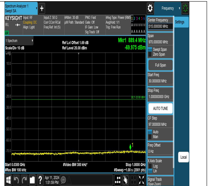
Band66_5MHz_QPSK_132322_1RB#0_30~1000_30~1000
