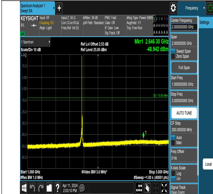
Band66_10MHz_QPSK_132622_1RB#0_1000~3000_1000~3000
