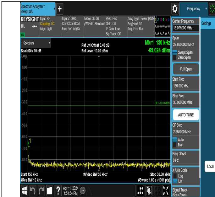
Band66_5MHz_QPSK_132322_1RB#0_0.15~30_0.15~30
