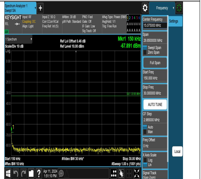
Band66_5MHz_QPSK_131997_1RB#0_0.15~30_0.15~30
