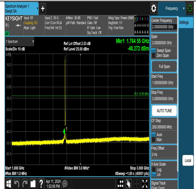
Band66_5MHz_QPSK_132647_1RB#0_1000~3000_1000~3000
