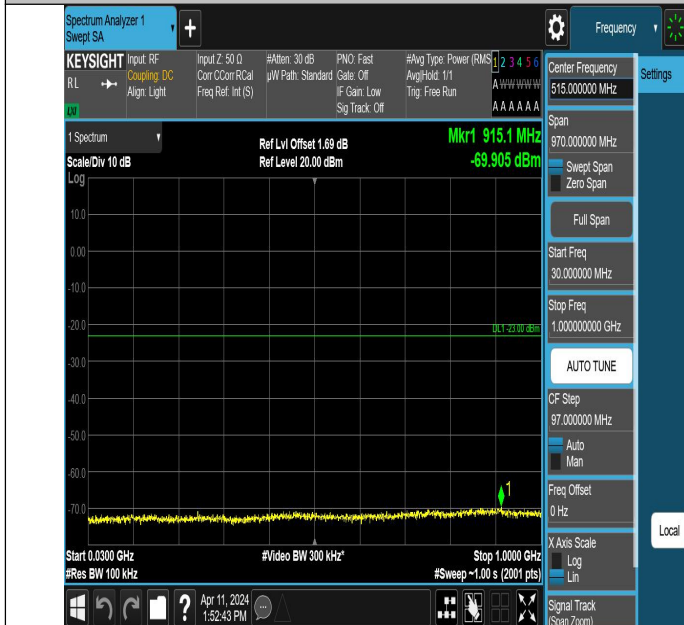
Band66_5MHz_QPSK_132647_1RB#0_30~1000_30~1000
