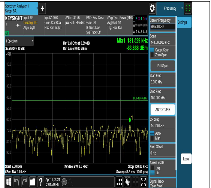
Band66_10MHz_QPSK_132022_1RB#0_0.009~0.15_0.009~0.15
