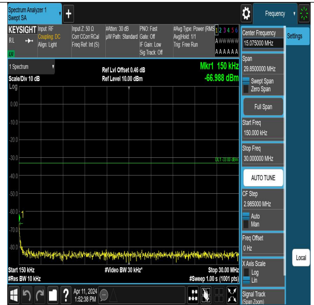
Band66_5MHz_QPSK_132647_1RB#0_0.15~30_0.15~30
