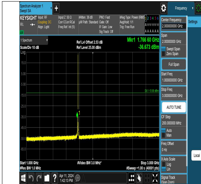
Band66_3MHz_QPSK_132657_1RB#0_1000~3000_1000~3000
