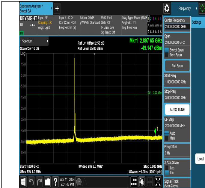
Band66_10MHz_QPSK_132022_1RB#0_1000~3000_1000~3000
