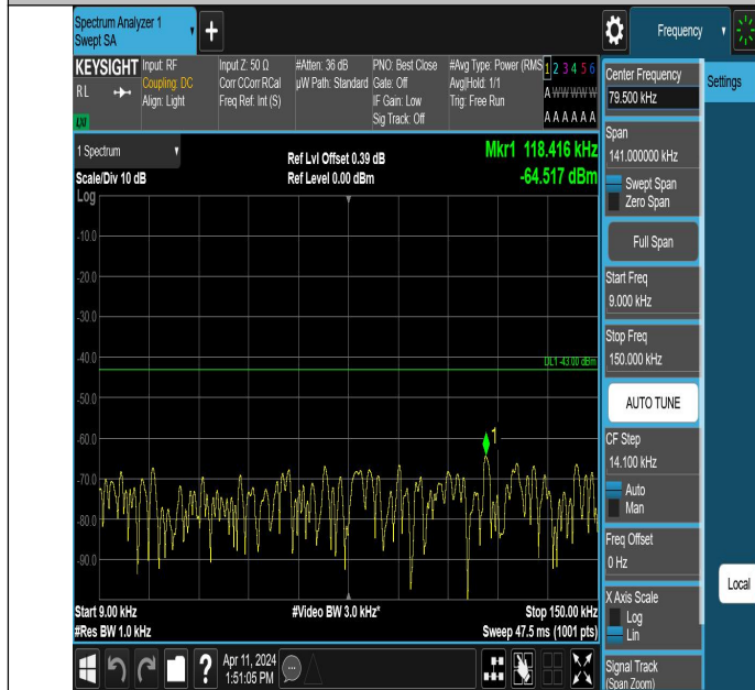
Band66_5MHz_QPSK_131997_1RB#0_0.009~0.15_0.009~0.15
