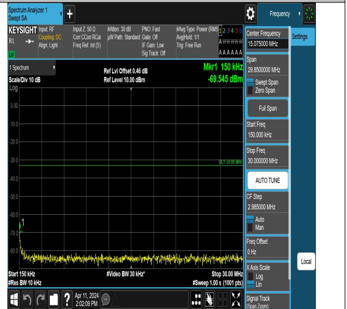
Band66_10MHz_QPSK_132322_1RB#0_0.15~30_0.15~30
