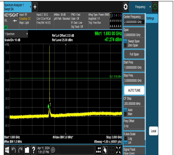
Band66_5MHz_QPSK_131997_1RB#0_1000~3000_1000~3000
