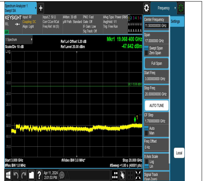
Band66_10MHz_QPSK_132022_1RB#0_3000~20000_3000~20000
