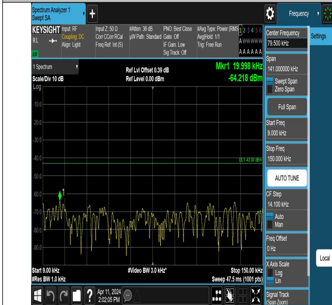
Band66_10MHz_QPSK_132322_1RB#0_0.009~0.15_0.009~0.15
