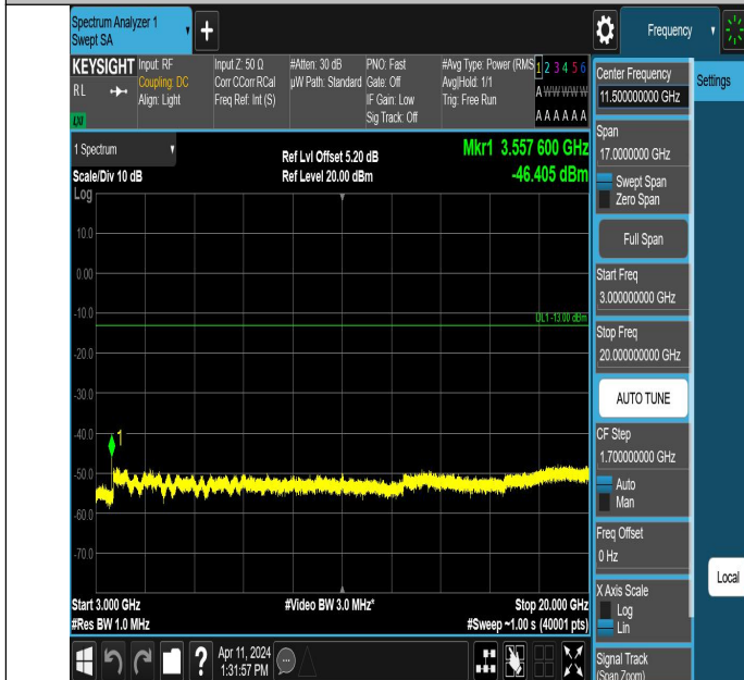
Band66_1.4MHz_QPSK_132665_1RB#0_3000~20000_3000~200
