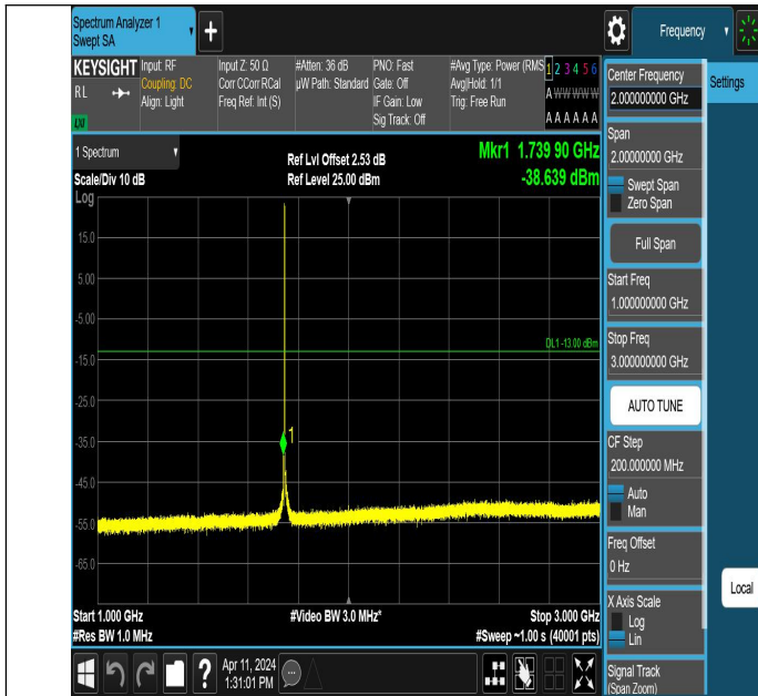
Band66_1.4MHz_QPSK_132322_1RB#0_1000~3000_1000~3000
