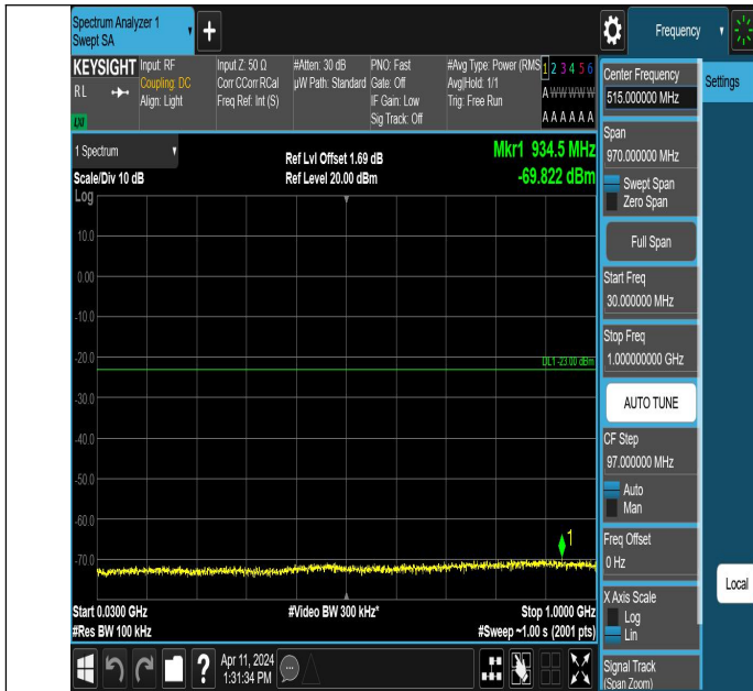
Band66_1.4MHz_QPSK_132665_1RB#0_30~1000_30~1000
