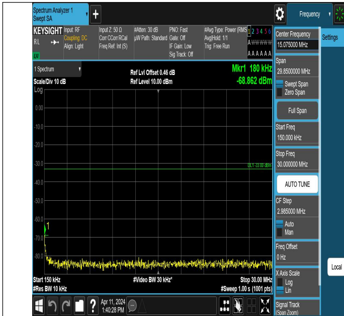
Band66_3MHz_QPSK_131987_1RB#0_0.15~30_0.15~30
