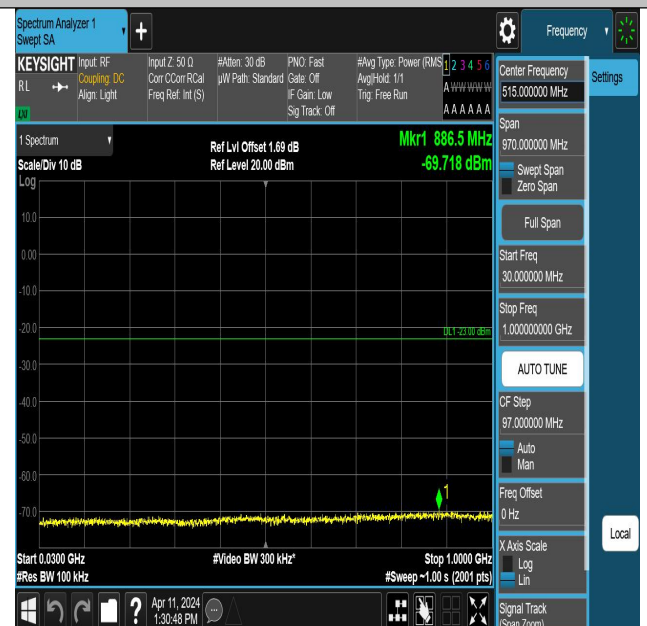
Band66_1.4MHz_QPSK_132322_1RB#0_30~1000_30~1000
