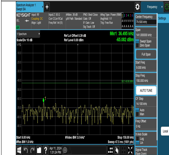
Band66_1.4MHz_QPSK_132665_1RB#0_0.009~0.15_0.009~0.15
