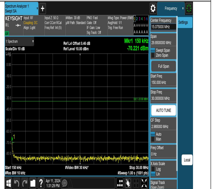
Band66_1.4MHz_QPSK_132665_1RB#0_0.15~30_0.15~30
