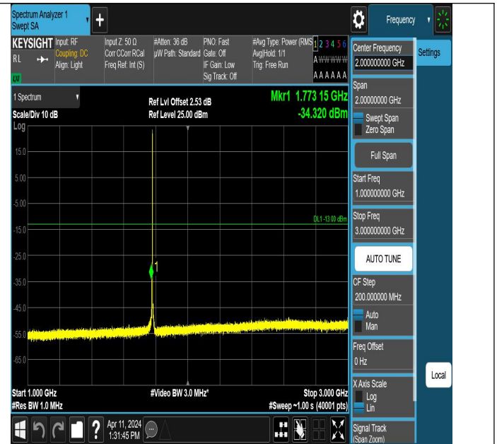
Band66_1.4MHz_QPSK_132665_1RB#0_1000~3000_1000~3000
