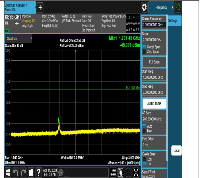
Band66_3MHz_QPSK_132322_1RB#0_1000~3000_1000~3000
