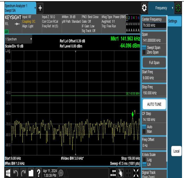
Band66_1.4MHz_QPSK_132322_1RB#0_0.009~0.15_0.009~0.15
