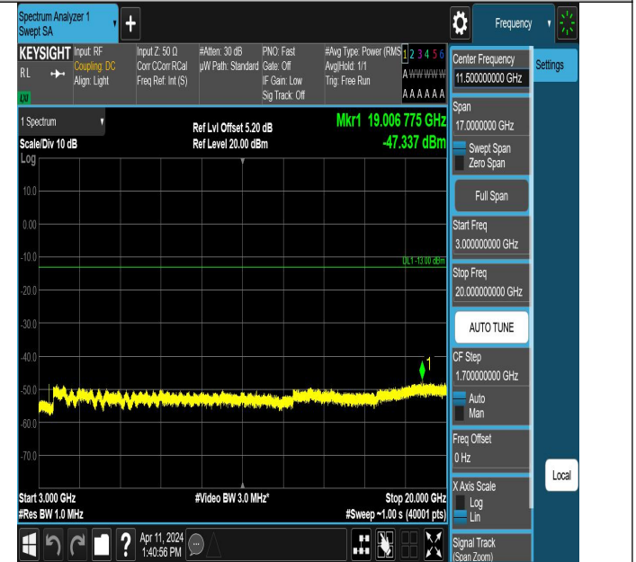
Band66_3MHz_QPSK_131987_1RB#0_3000~20000_3000~2000
