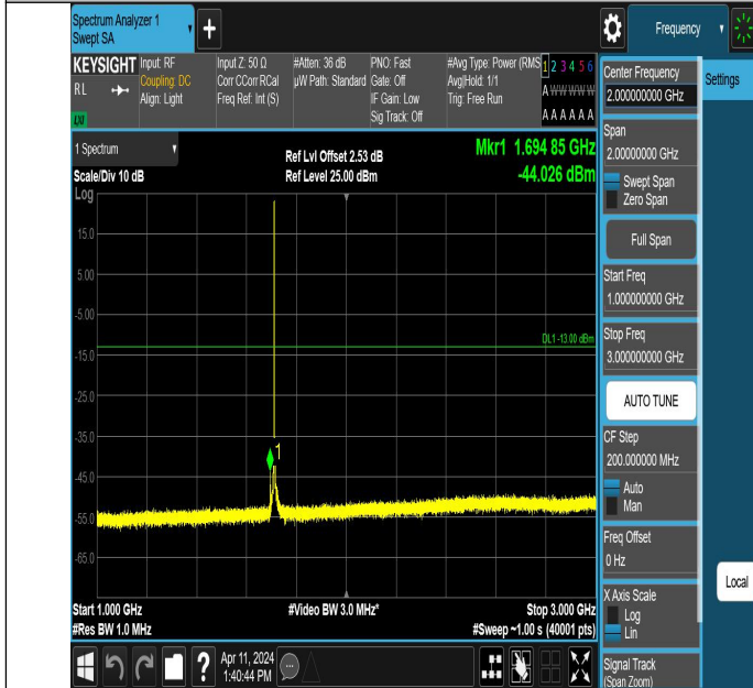
Band66_3MHz_QPSK_131987_1RB#0_1000~3000_1000~3000
