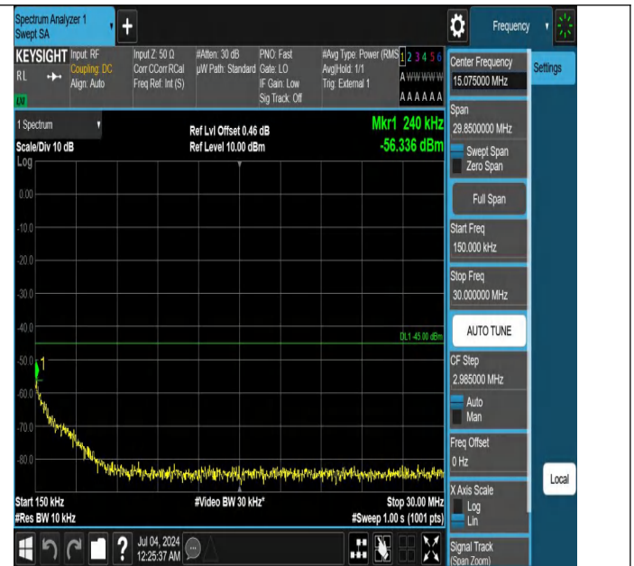
Band41-5MHz-QPSK-39675-1RB#0-0.15~30-PASS
