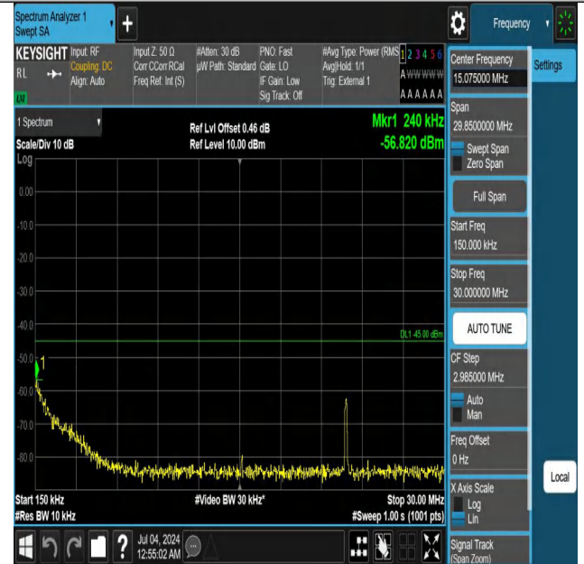
Band41-20MHz-QPSK-40620-1RB#0-0.15~30-PASS
