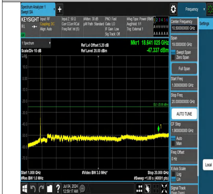
Band41-20MHz-QPSK-41490-1RB#0-1000~20000-PASS
