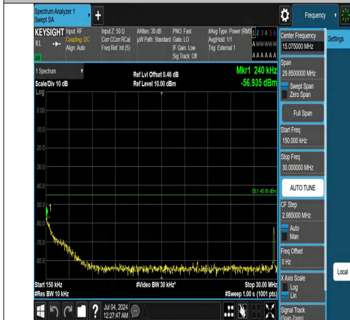
Band41-5MHz-QPSK-40620-1RB#0-0.15~30-PASS
