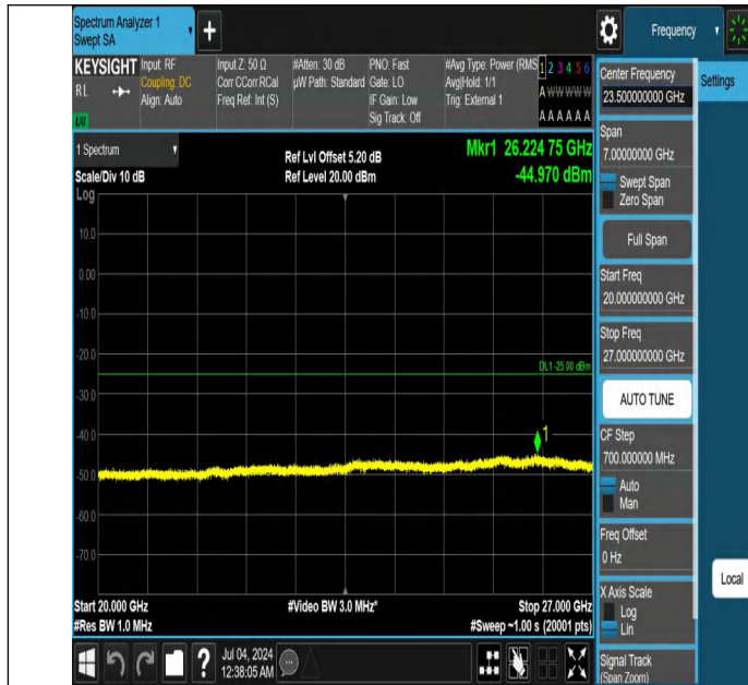
Band41-10MHz-QPSK-40620-1RB#0-20000~27000-PASS
