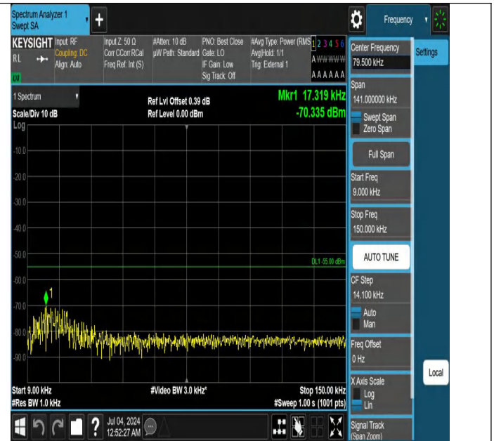
Band41-20MHz-QPSK-39750-1RB#0-0.009~0.15-PASS
