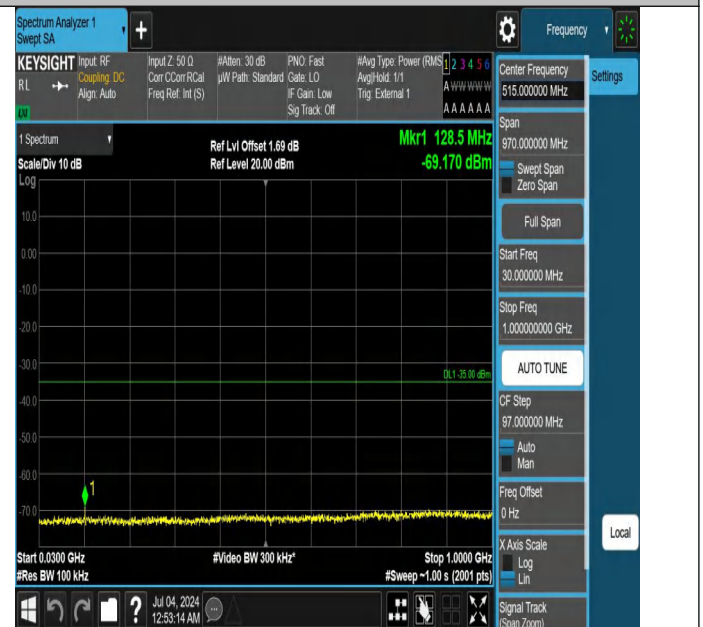
Band41-20MHz-QPSK-39750-1RB#0-30~1000-PASS
