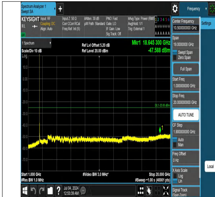
Band41-20MHz-QPSK-39750-1RB#0-1000~20000-PASS
