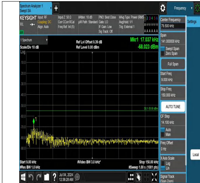
Band41-10MHz-QPSK-40620-1RB#0-0.009~0.15-PASS
