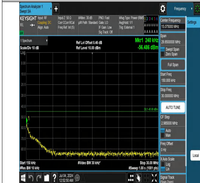
Band41-20MHz-QPSK-39750-1RB#0-0.15~30-PASS
