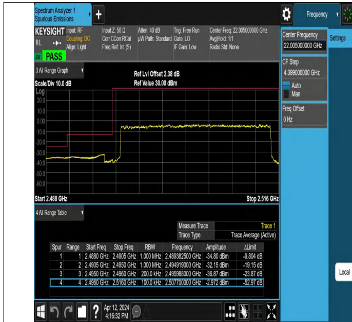
Band41_20MHz_QPSK_39750_100RB#0
