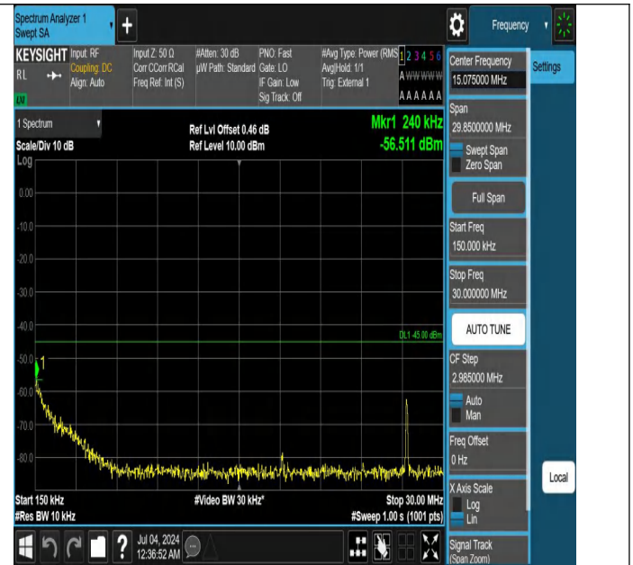
Band41-10MHz-QPSK-40620-1RB#0-0.15~30-PASS
