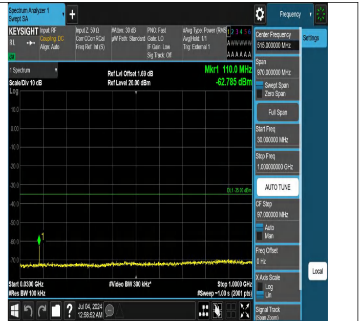
Band41-20MHz-QPSK-41490-1RB#0-30~1000-PASS
