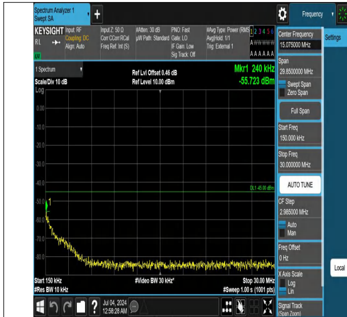
Band41-20MHz-QPSK-41490-1RB#0-0.15~30-PASS
