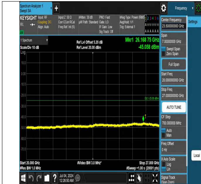
Band41-5MHz-QPSK-39675-1RB#0-20000~27000-PASS
