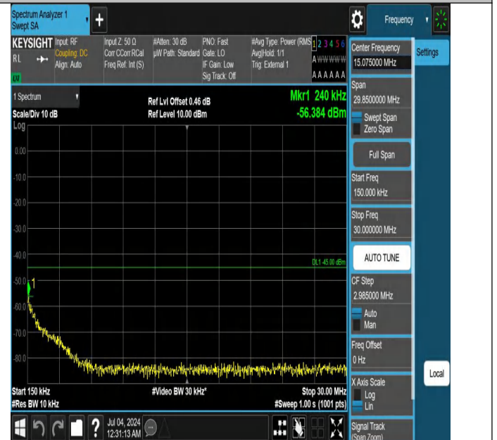
Band41-5MHz-QPSK-41565-1RB#0-0.15~30-PASS
