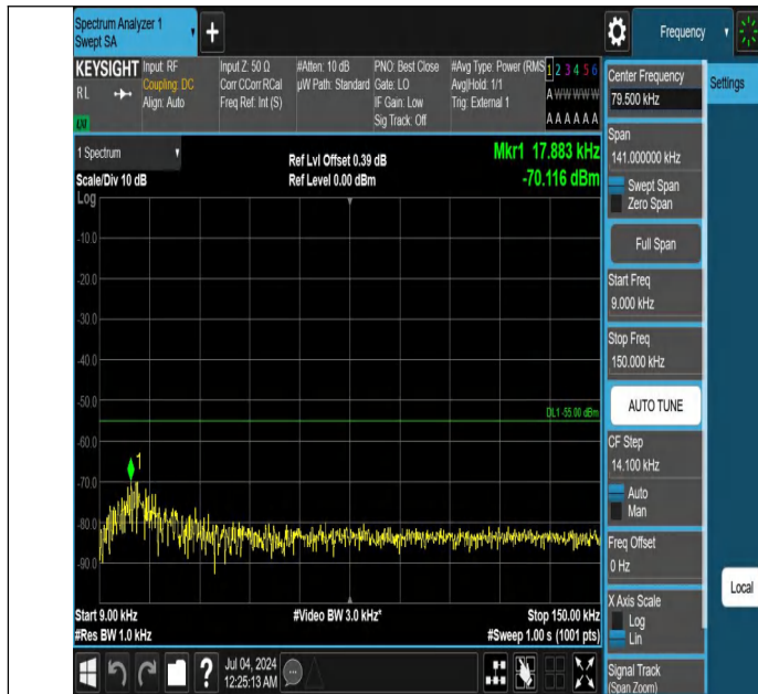
Band41-5MHz-QPSK-39675-1RB#0-0.009~0.15-PASS
