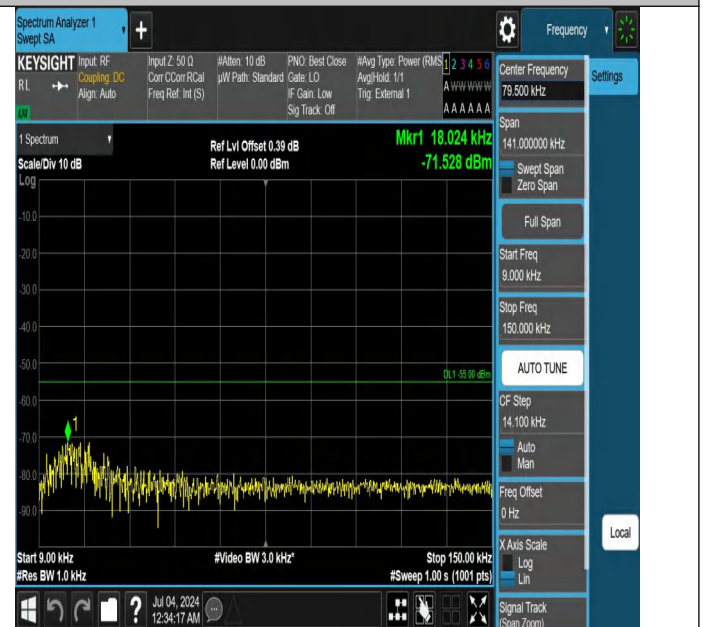
Band41-10MHz-QPSK-39700-1RB#0-0.009~0.15-PASS
