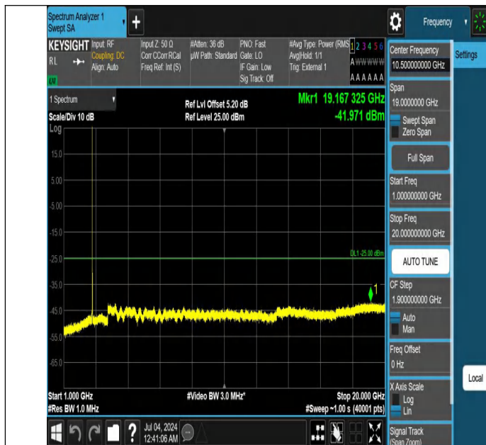
Band41-10MHz-QPSK-41540-1RB#0-1000~20000-PASS
