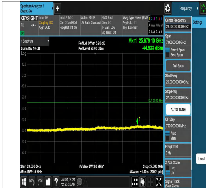
Band41-15MHz-QPSK-41515-1RB#0-20000~27000-PASS
