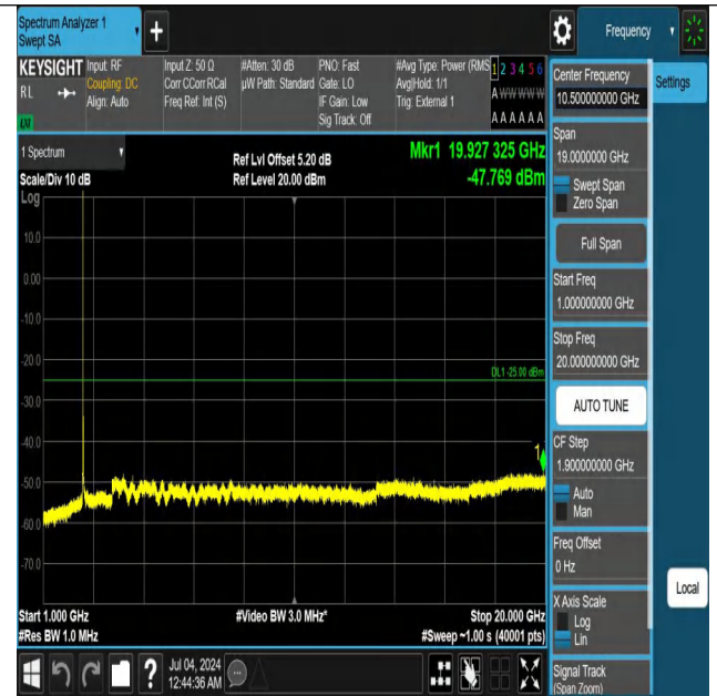
Band41-15MHz-QPSK-39725-1RB#0-1000~20000-PASS
