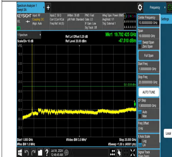
Band41-15MHz-QPSK-40620-1RB#0-1000~20000-PASS
