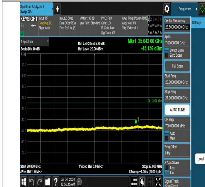
Band41-20MHz-QPSK-40620-1RB#0-20000~27000-PASS
