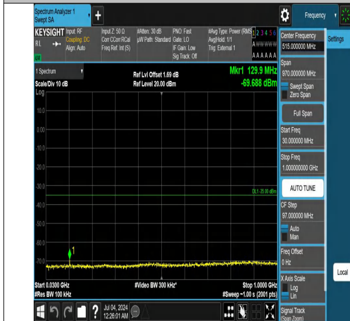
Band41-5MHz-QPSK-39675-1RB#0-30~1000-PASS
