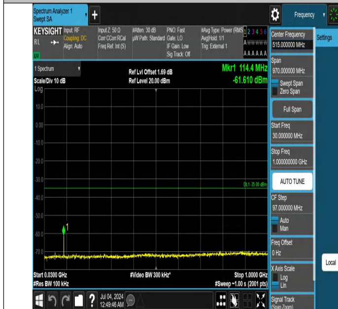
Band41-15MHz-QPSK-41515-1RB#0-30~1000-PASS
