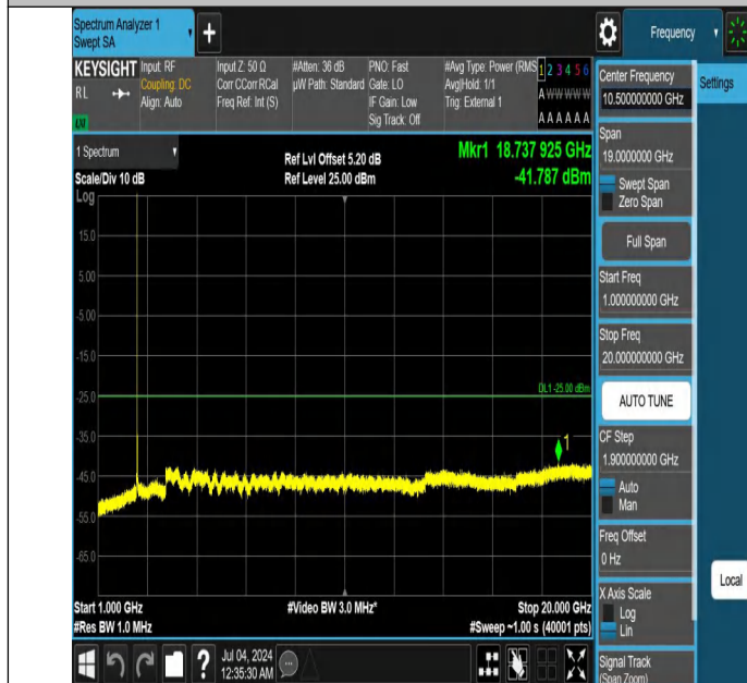
Band41-10MHz-QPSK-39700-1RB#0-1000~20000-PASS
