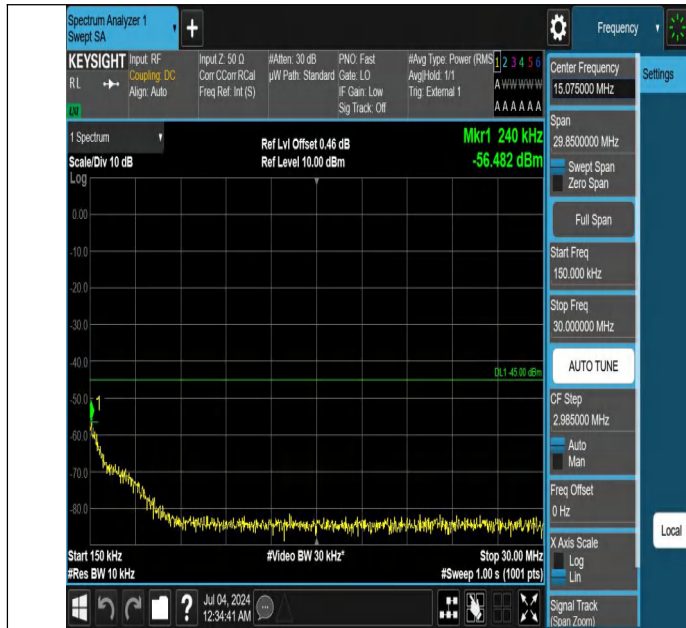
Band41-10MHz-QPSK-39700-1RB#0-0.15~30-PASS
