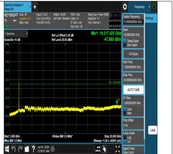
Band41-20MHz-QPSK-40620-1RB#0-1000~20000-PASS
