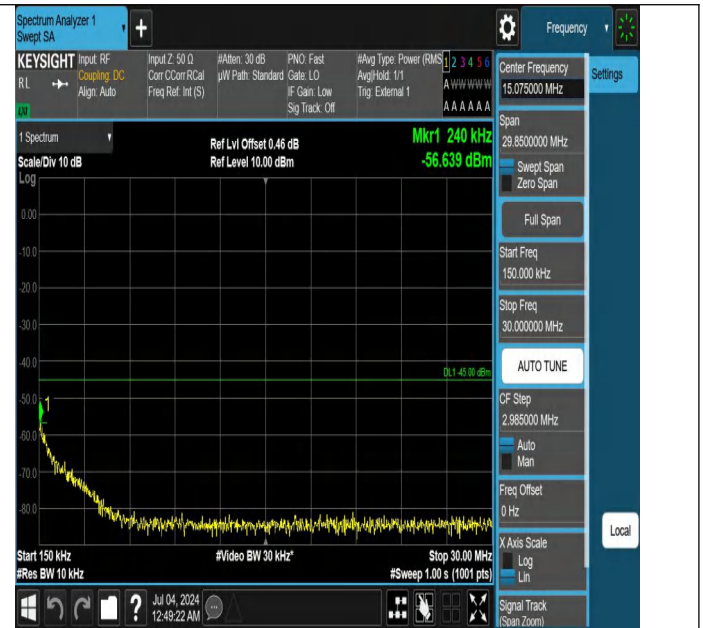
Band41-15MHz-QPSK-41515-1RB#0-0.15~30-PASS
