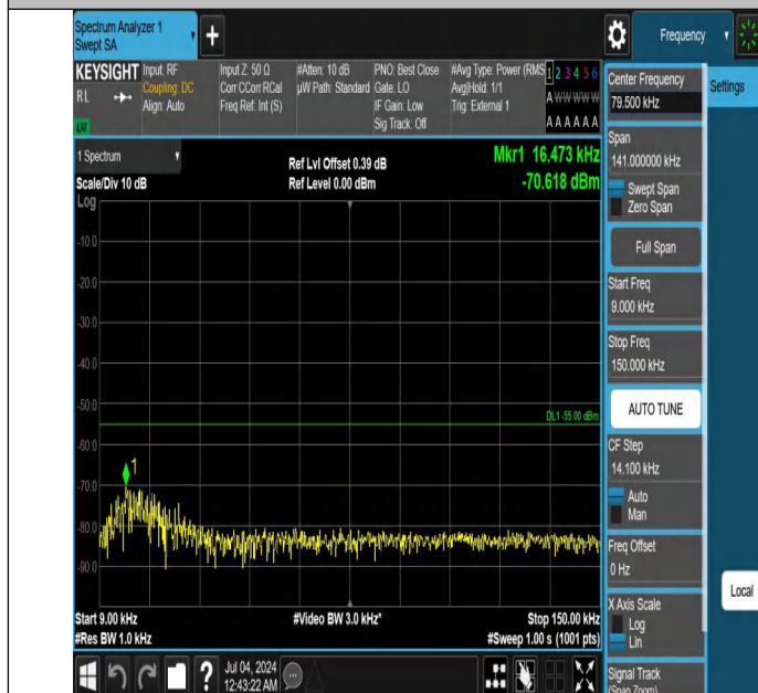
Band41-15MHz-QPSK-39725-1RB#0-0.009~0.15-PASS
