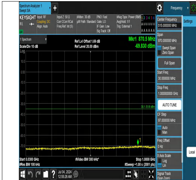
Band41-20MHz-QPSK-40620-1RB#0-30~1000-PASS
