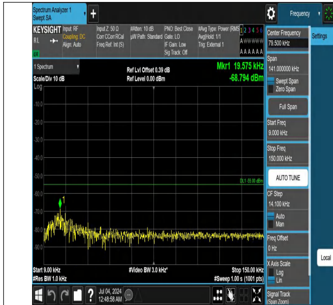
Band41-15MHz-QPSK-41515-1RB#0-0.009~0.15-PASS
