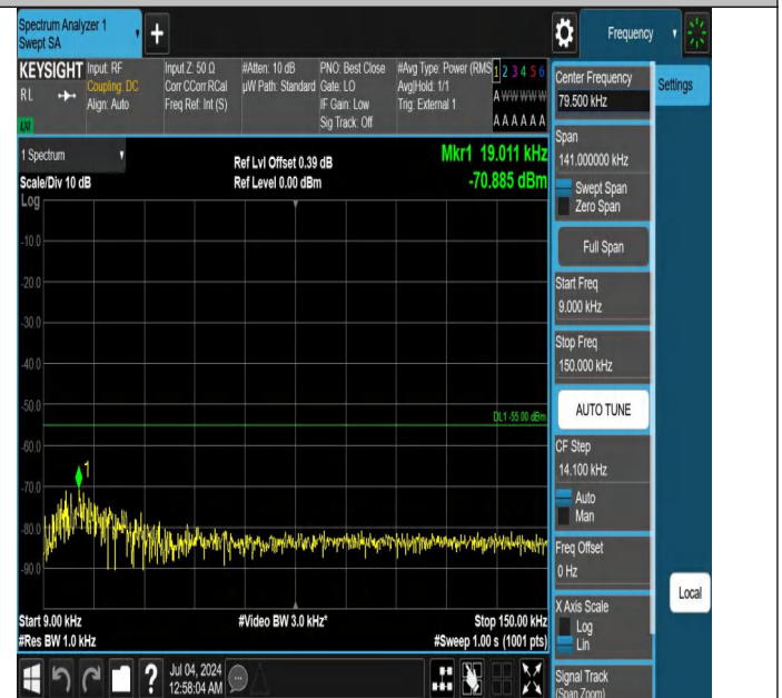
Band41-20MHz-QPSK-41490-1RB#0-0.009~0.15-PASS
