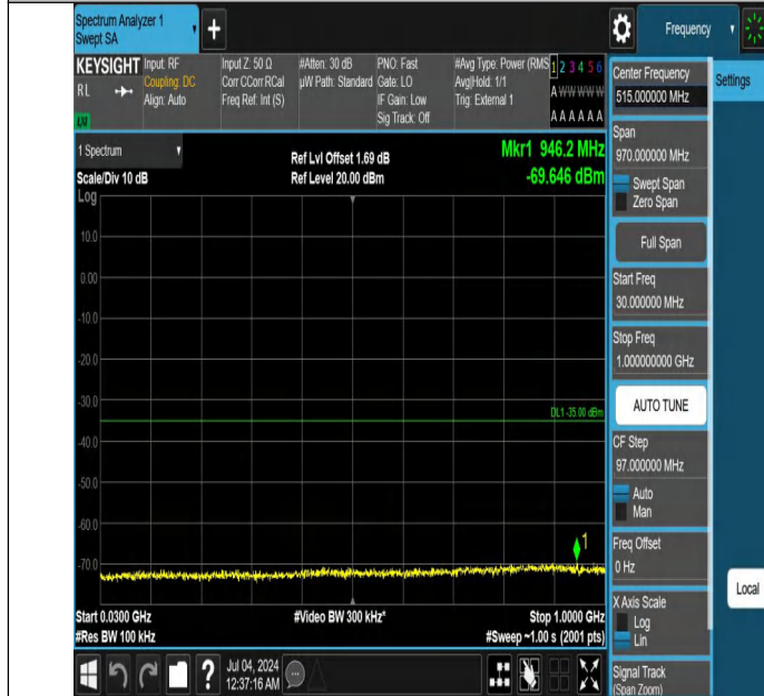
Band41-10MHz-QPSK-40620-1RB#0-30~1000-PASS
