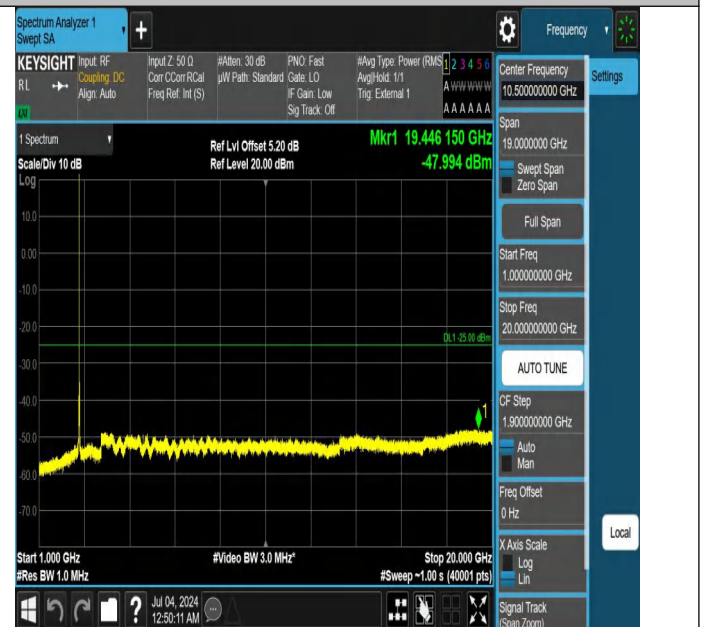
Band41-15MHz-QPSK-41515-1RB#0-1000~20000-PASS
