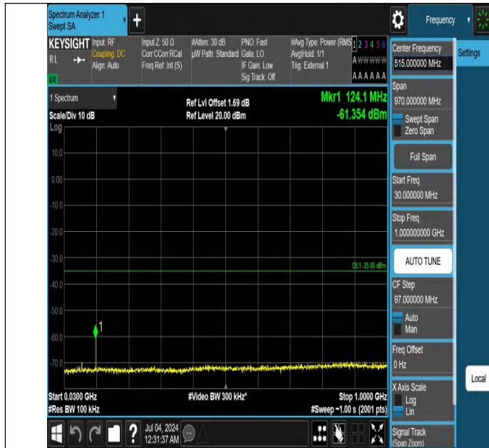
Band41-5MHz-QPSK-41565-1RB#0-30~1000-PASS
