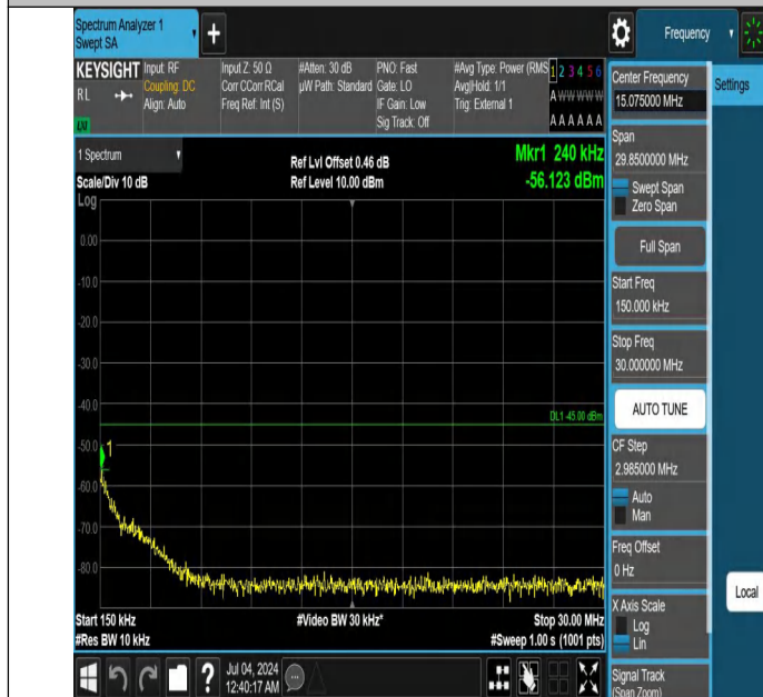
Band41-10MHz-QPSK-41540-1RB#0-0.15~30-PASS
