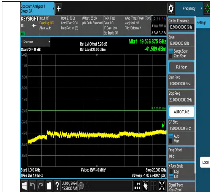
Band41-5MHz-QPSK-40620-1RB#0-1000~20000-PASS
