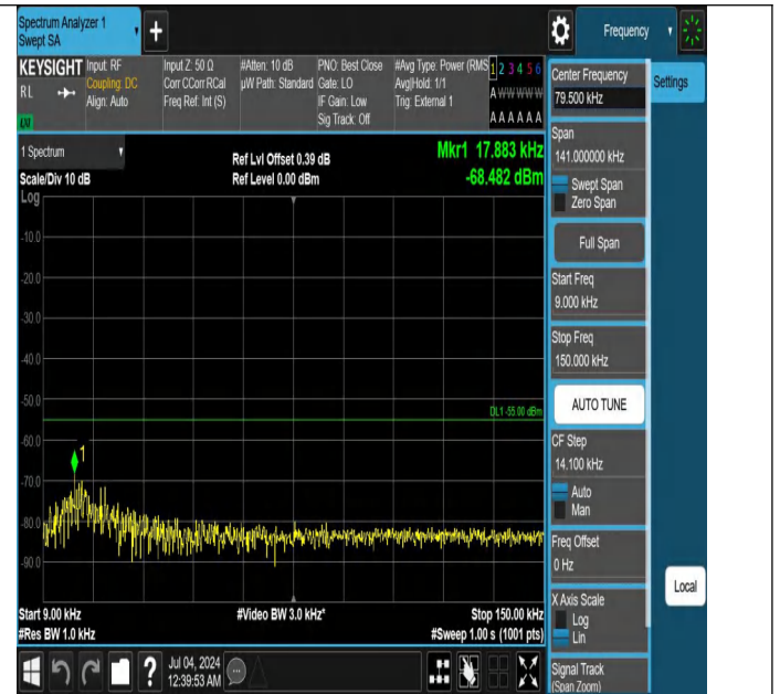
Band41-10MHz-QPSK-41540-1RB#0-0.009~0.15-PASS
