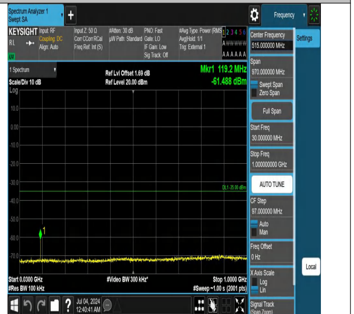
Band41-10MHz-QPSK-41540-1RB#0-30~1000-PASS
