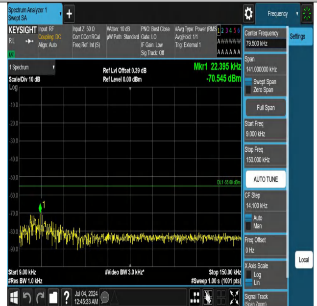
Band41-15MHz-QPSK-40620-1RB#0-0.009~0.15-PASS
