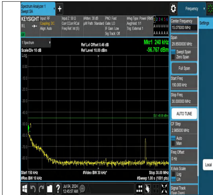
Band41-15MHz-QPSK-40620-1RB#0-0.15~30-PASS
