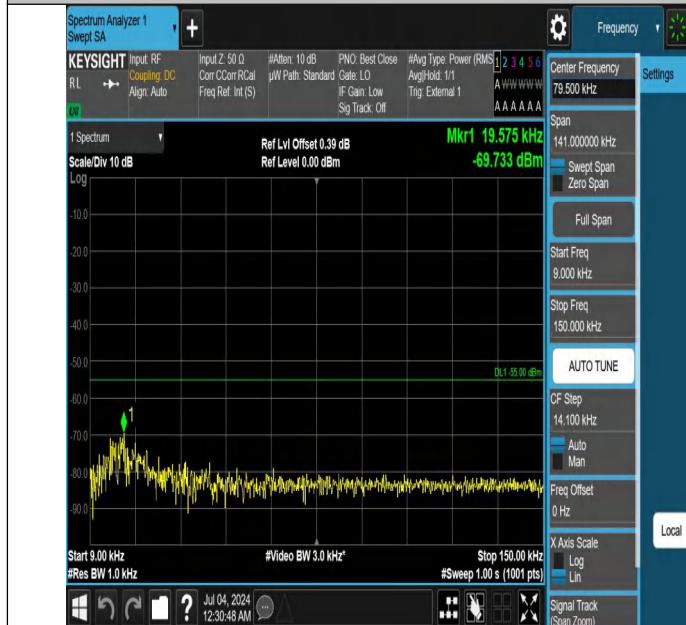
Band41-5MHz-QPSK-41565-1RB#0-0.009~0.15-PASS
