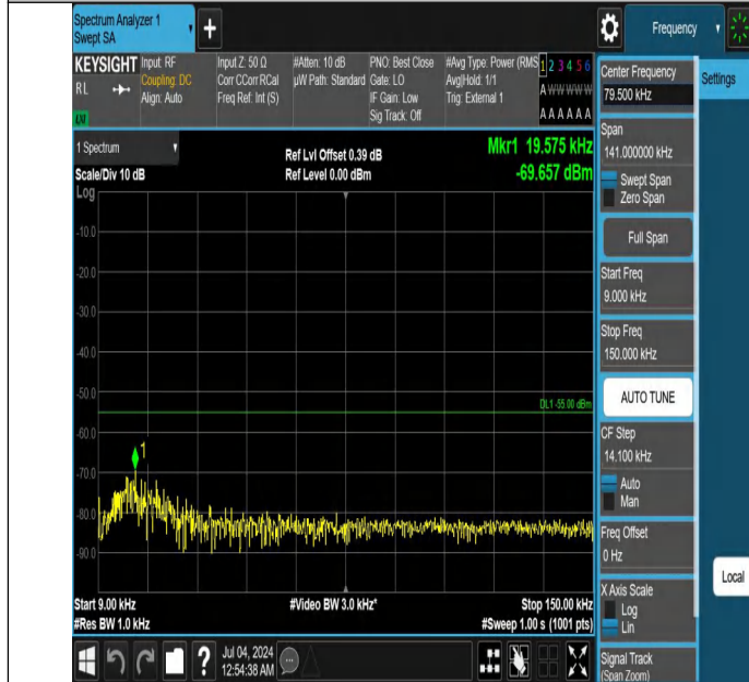
Band41-20MHz-QPSK-40620-1RB#0-0.009~0.15-PASS
