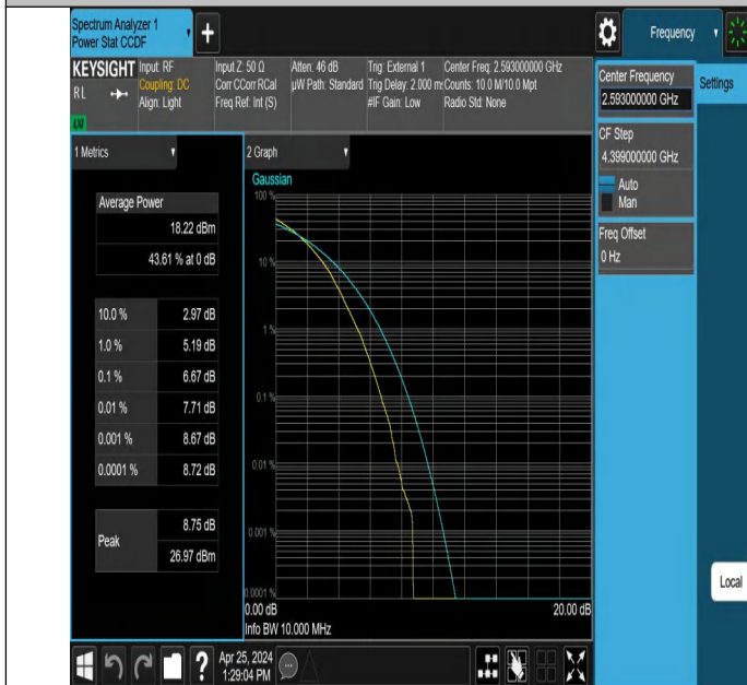
Band41-10MHz-256QAM-40620-50RB#0-PASS
