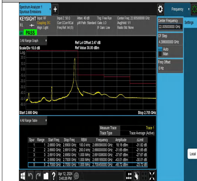
Band41_10MHz_QPSK_41540_1RB#49
