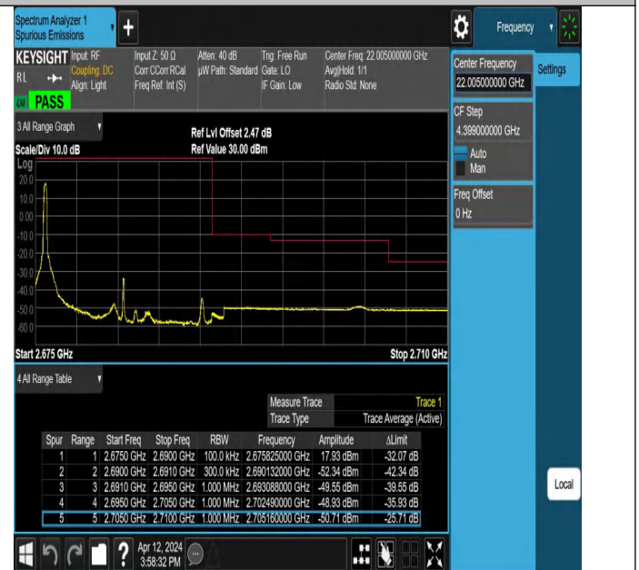
Band41_15MHz_QPSK_41515_1RB#0
