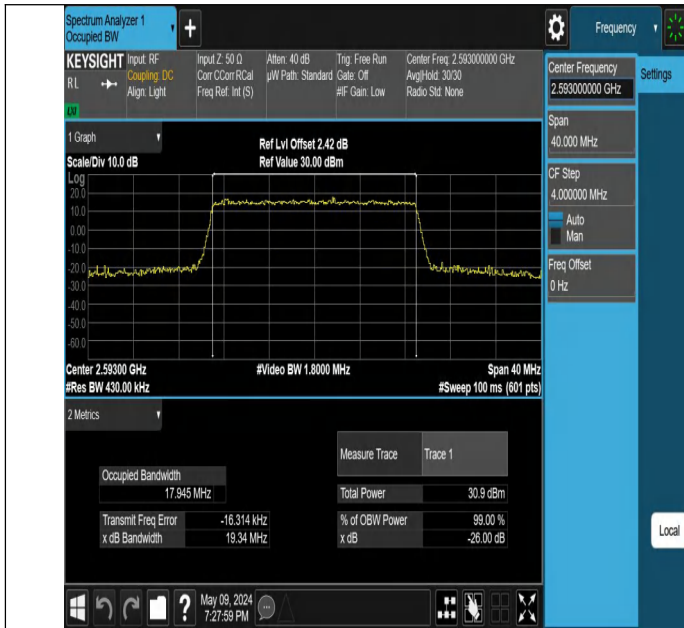
Band41-20MHz-QPSK-40620-100RB#0-PASS
