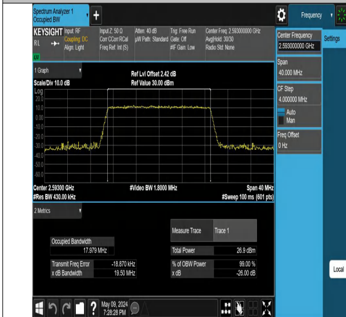
Band41-20MHz-256QAM-40620-100RB#0-PASS
