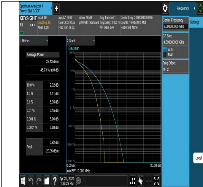
Band41-10MHz-QPSK-40620-50RB#0-PASS
