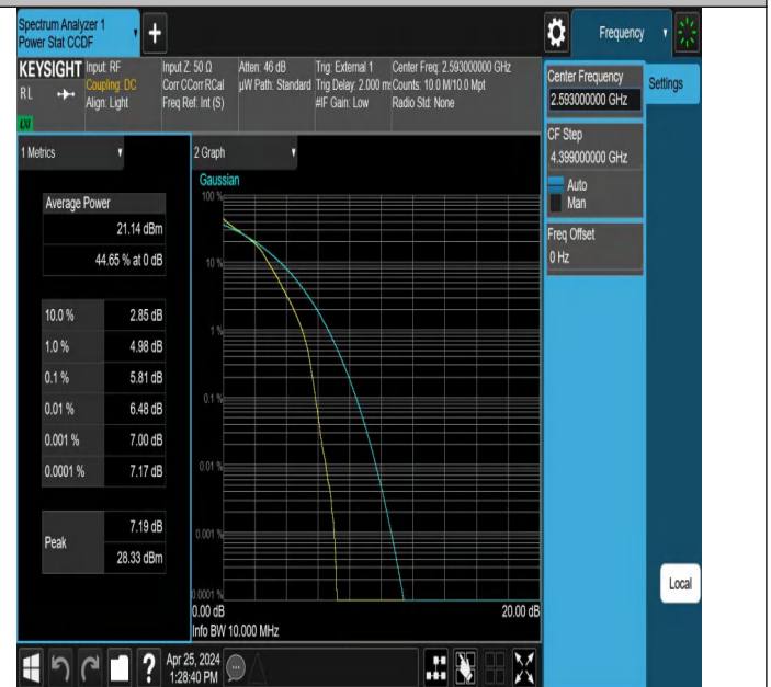
Band41-10MHz-16QAM-40620-50RB#0-PASS
