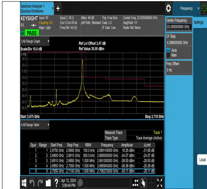
Band41_15MHz_QPSK_41515_1RB#74
