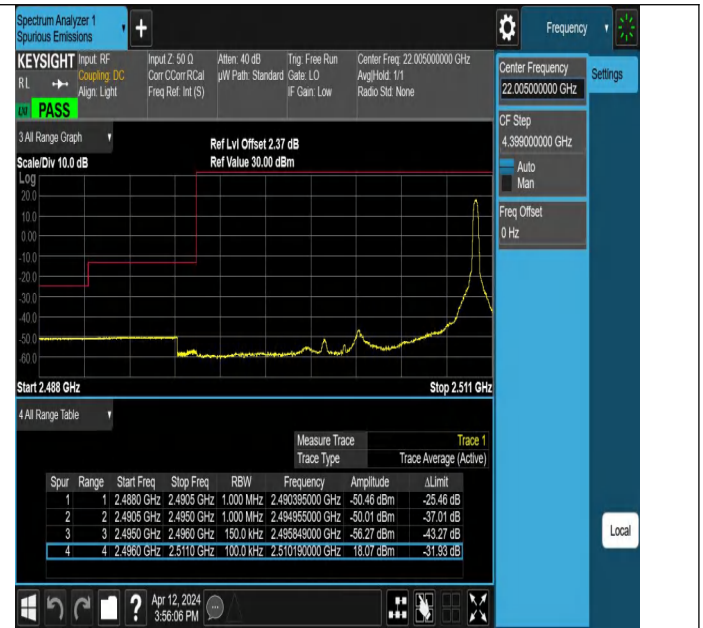
Band41_15MHz_QPSK_39725_1RB#74
