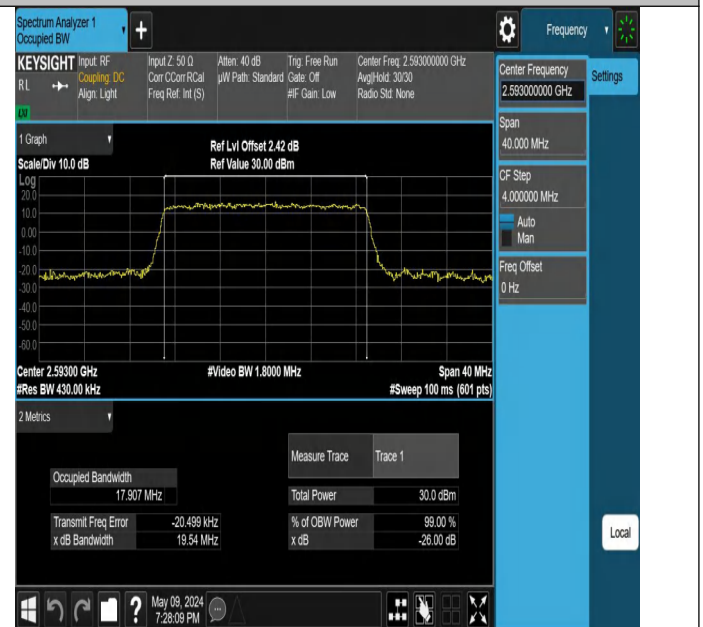
Band41-20MHz-16QAM-40620-100RB#0-PASS
