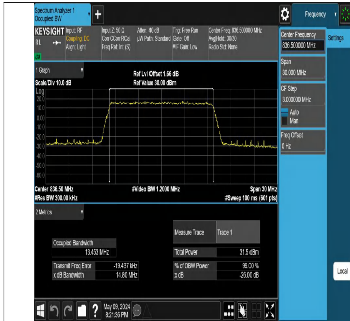
Band26(824-849)-15MHz-QPSK-26915-75RB#0-PASS
