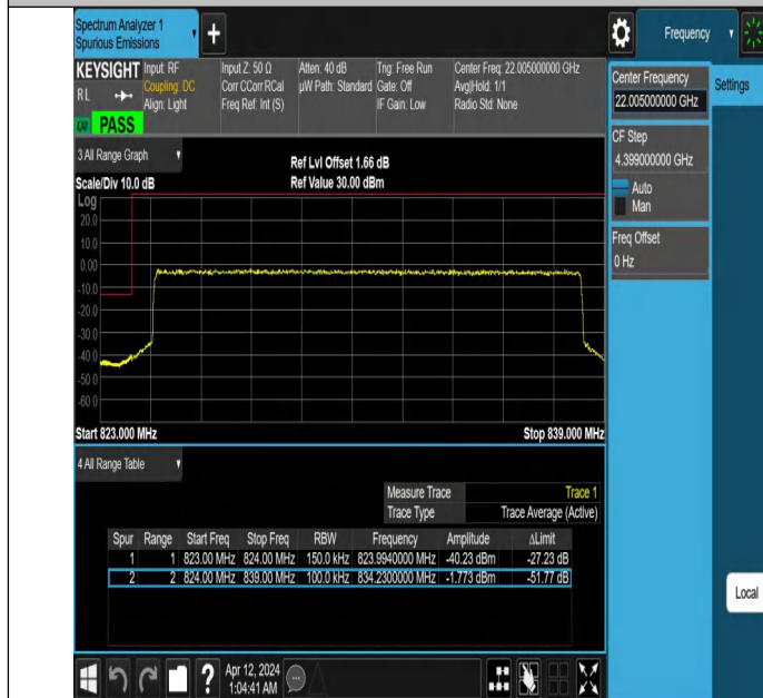
Band26_15MHz_QPSK_26865_75RB#0
