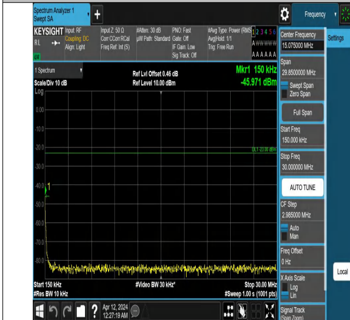
Band26_1.4MHz_QPSK_26915_1RB#0_0.15~30_0.15~30
