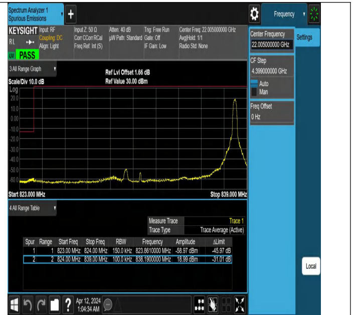
Band26_15MHz_QPSK_26865_1RB#74
