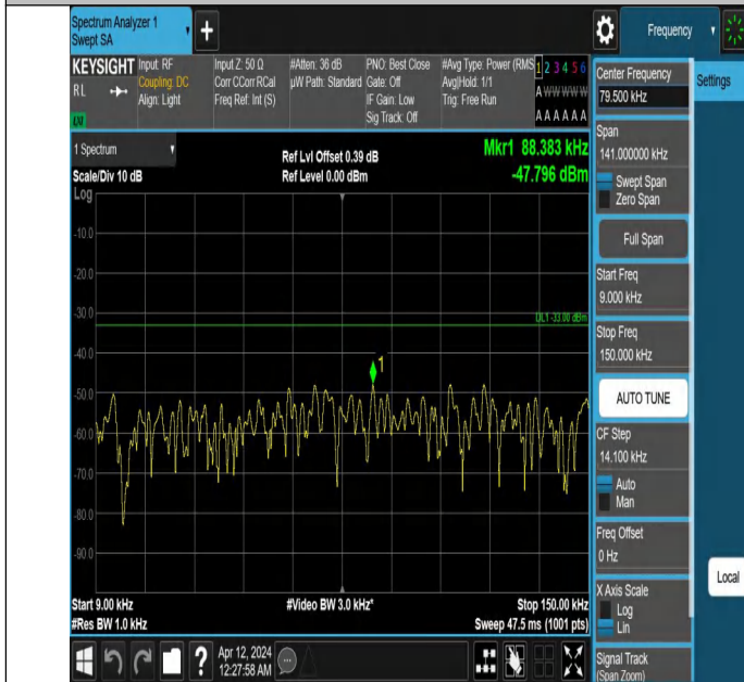
Band26_1.4MHz_QPSK_27033_1RB#0_0.009~0.15_0.009~0.15
