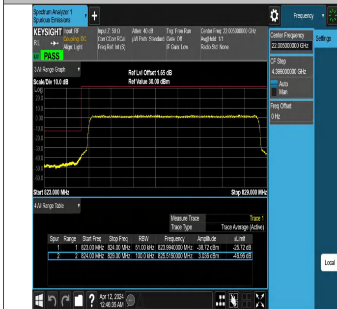
Band26_5MHz_QPSK_26815_25RB#0
