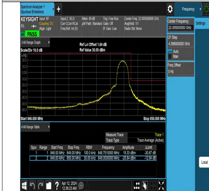
Band26_3MHz_QPSK_27025_1RB#14
