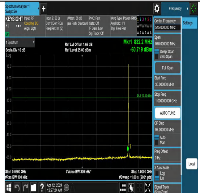
Band26_1.4MHz_QPSK_26915_1RB#0_30~1000_30~1000
