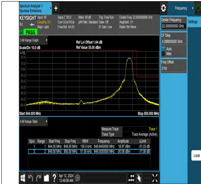
Band26_5MHz_QPSK_27015_1RB#24
