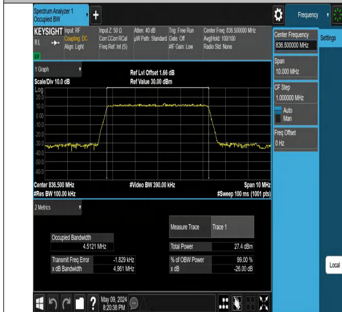
Band26(824-849)-5MHz-256QAM-26915-25RB#0-PASS
