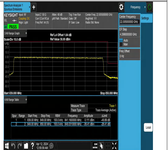
Band26_10MHz_QPSK_26990_50RB#0
