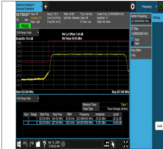
Band26_3MHz_QPSK_26805_15RB#0
