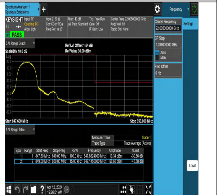
Band26_1.4MHz_QPSK_27033_1RB#0
