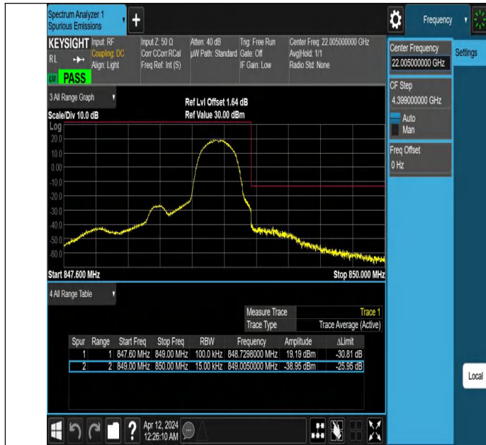
Band26_1.4MHz_QPSK_27033_1RB#5
