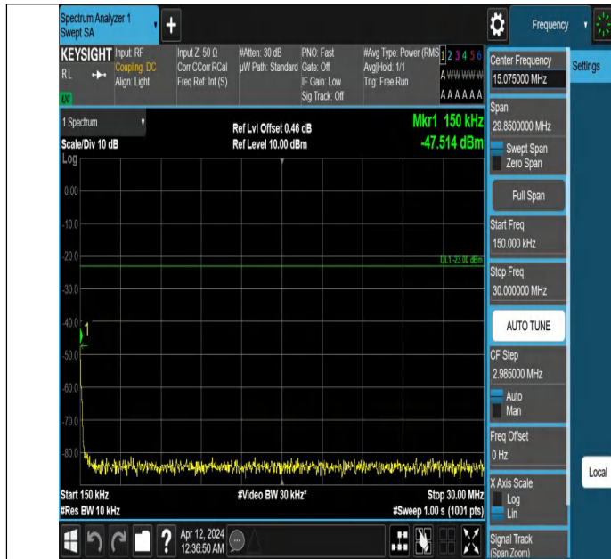
Band26_3MHz_QPSK_26805_1RB#0_0.15~30_0.15~30
