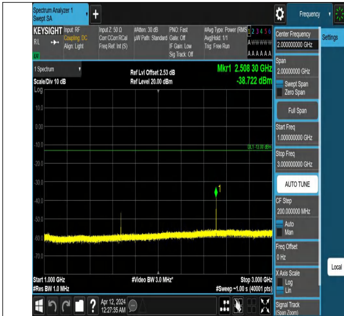
Band26_1.4MHz_QPSK_26915_1RB#0_1000~3000_1000~3000
