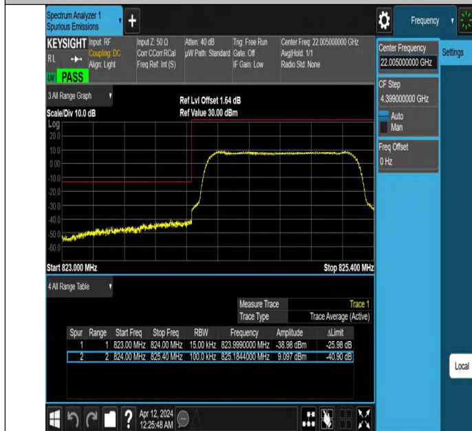
Band26_1.4MHz_QPSK_26797_6RB#0
