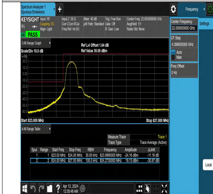
Band26_3MHz_QPSK_26805_1RB#0
