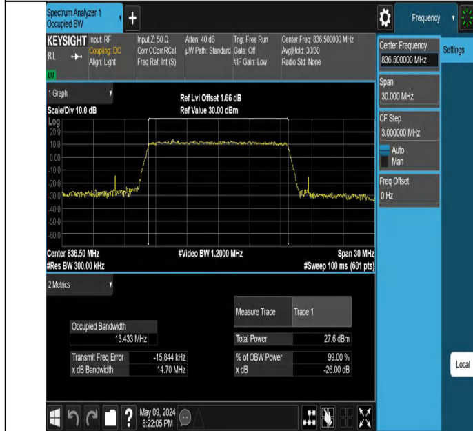
Band26(824-849)-15MHz-256QAM-26915-75RB#0-PASS
