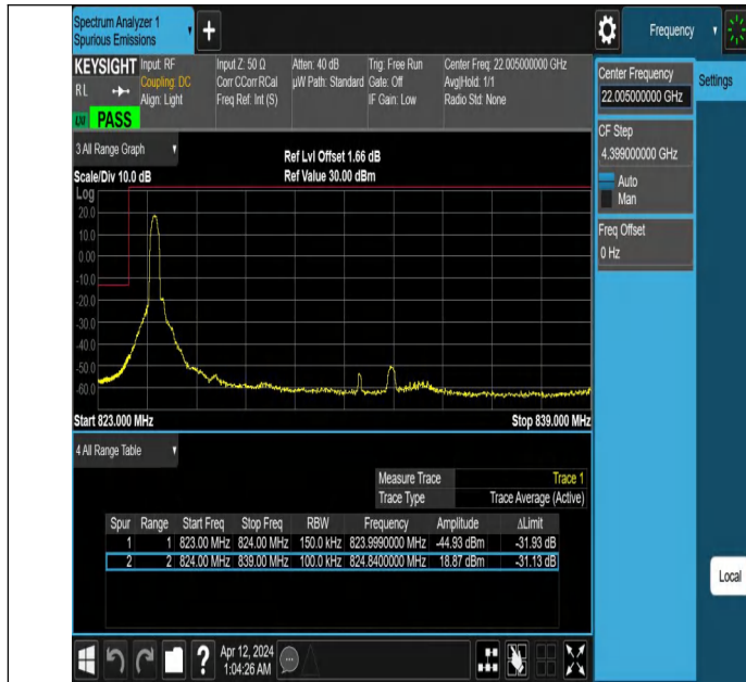
Band26_15MHz_QPSK_26865_1RB#0
