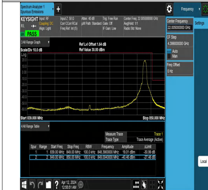
Band26_10MHz_QPSK_26990_1RB#49
