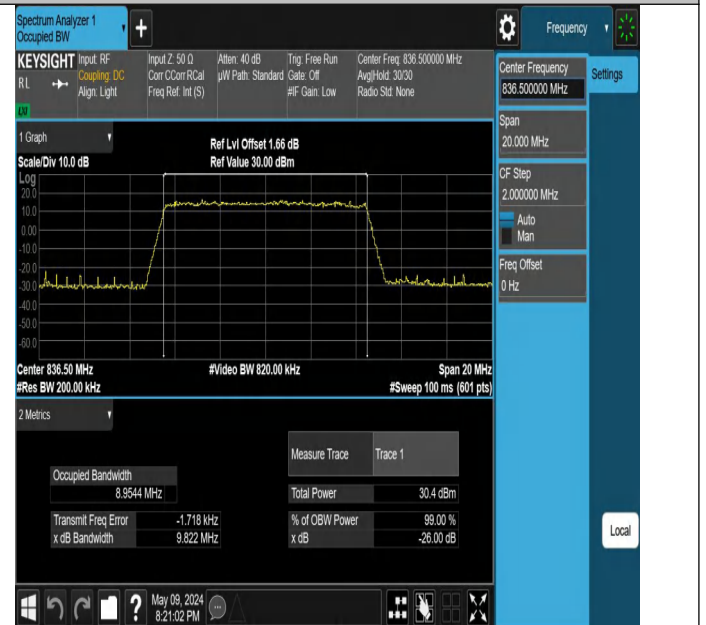
Band26(824-849)-10MHz-16QAM-26915-50RB#0-PASS
