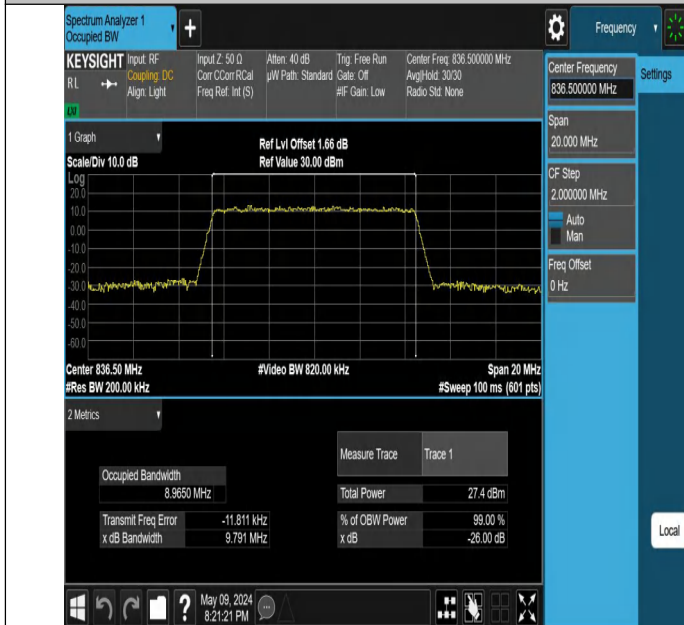
Band26(824-849)-10MHz-256QAM-26915-50RB#0-PASS
