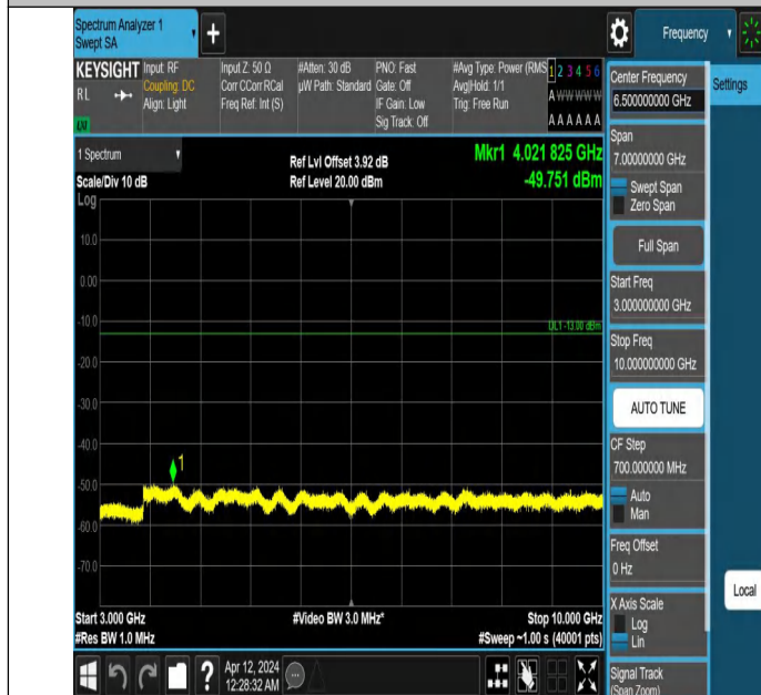
Band26_1.4MHz_QPSK_27033_1RB#0_3000~10000_3000~1000
