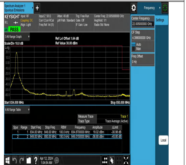
Band26_15MHz_QPSK_26965_1RB#0
