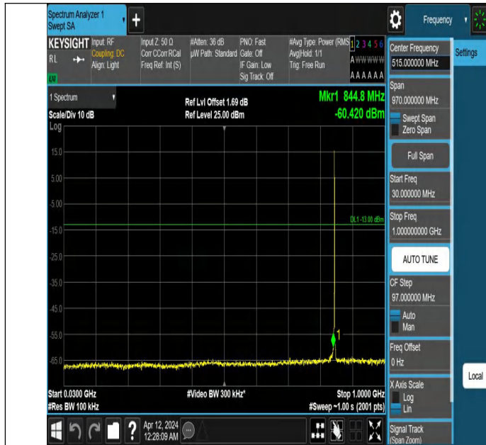
Band26_1.4MHz_QPSK_27033_1RB#0_30~1000_30~1000
