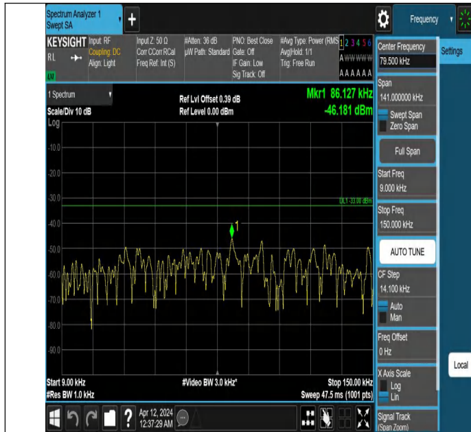
Band26_3MHz_QPSK_26915_1RB#0_0.009~0.15_0.009~0.15
