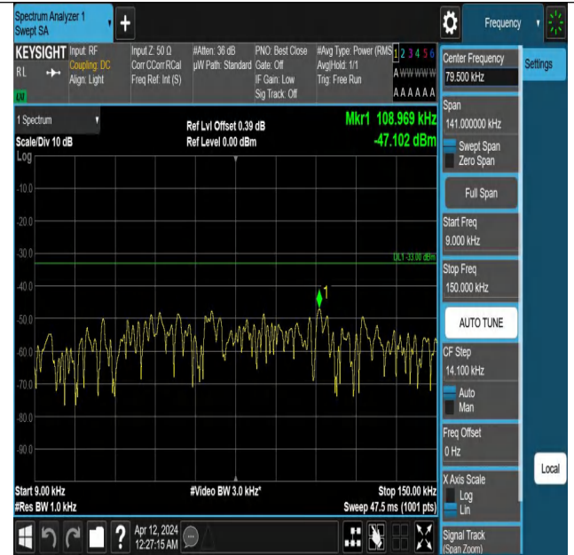
Band26_1.4MHz_QPSK_26915_1RB#0_0.009~0.15_0.009~0.15
