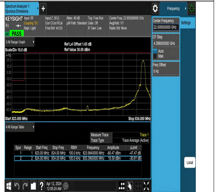
Band26_10MHz_QPSK_26840_1RB#49
