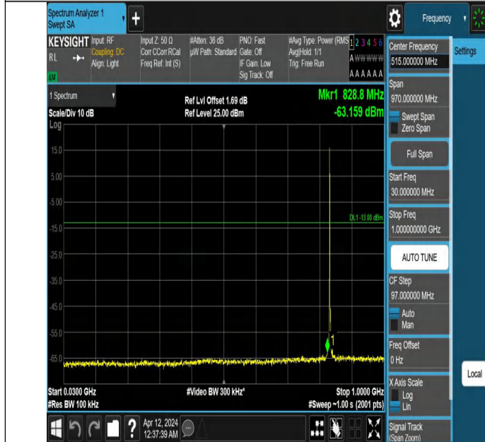
Band26_3MHz_QPSK_26915_1RB#0_30~1000_30~1000
