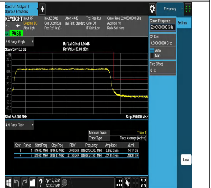
Band26_3MHz_QPSK_27025_15RB#0
