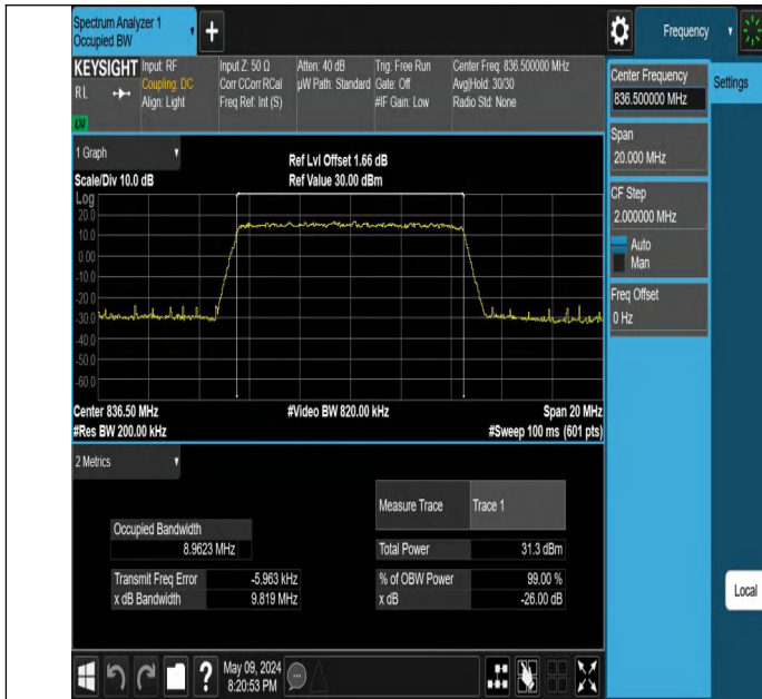
Band26(824-849)-10MHz-QPSK-26915-50RB#0-PASS
