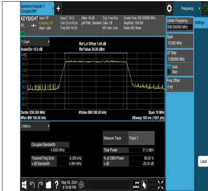
Band26(824-849)-5MHz-QPSK-26915-25RB#0-PASS
