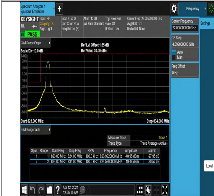
Band26_10MHz_QPSK_26840_1RB#0
