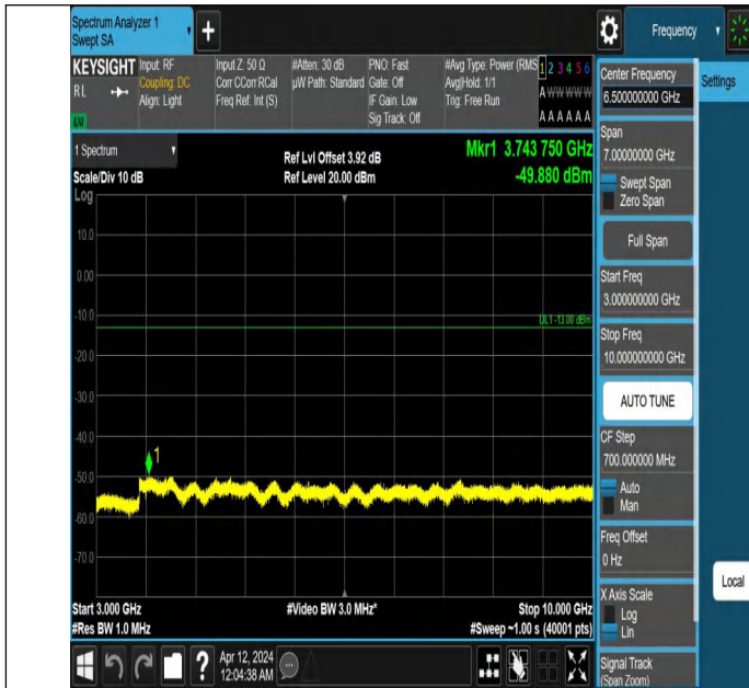
Band26(814-824)-3MHz-QPSK-26740-1RB#0-3000~10000-PASS
