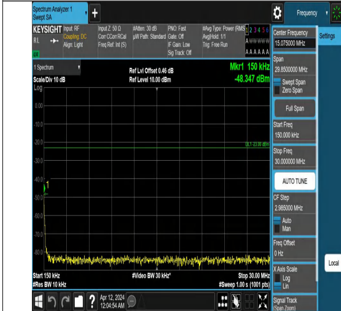
Band26(814-824)-3MHz-QPSK-26775-1RB#0-0.15~30-PASS
