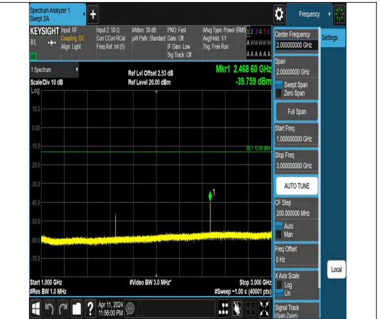
Band26(814-824)-1.4MHz-QPSK-26783-1RB#0-1000~3000-PASS
