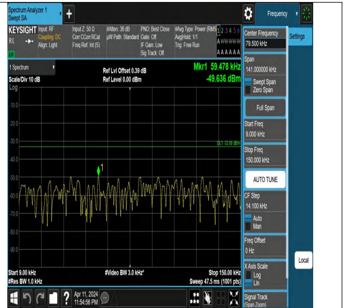
Band26(814-824)-1.4MHz-QPSK-26740-1RB#0-0.009~0.15-PASS
