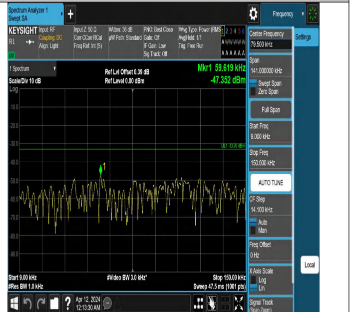
Band26(814-824)-5MHz-QPSK-26740-1RB#0-0.009~0.15-PASS
