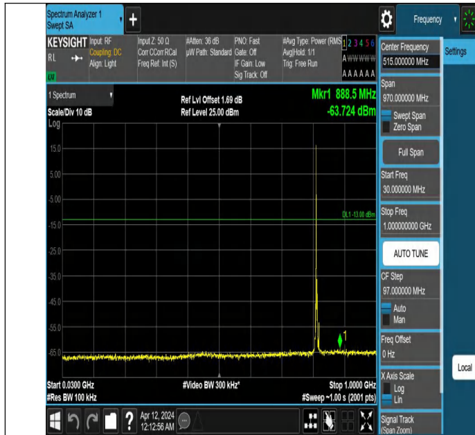
Band26(814-824)-5MHz-QPSK-26715-1RB#0-30~1000-PASS
