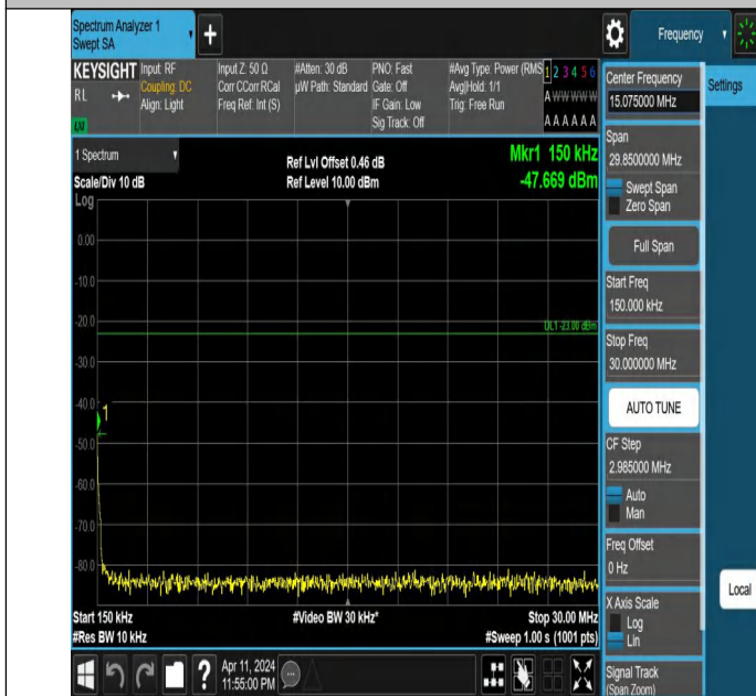
Band26(814-824)-1.4MHz-QPSK-26740-1RB#0-0.15~30-PASS
