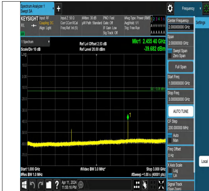
Band26(814-824)-1.4MHz-QPSK-26740-1RB#0-1000~3000-PASS
