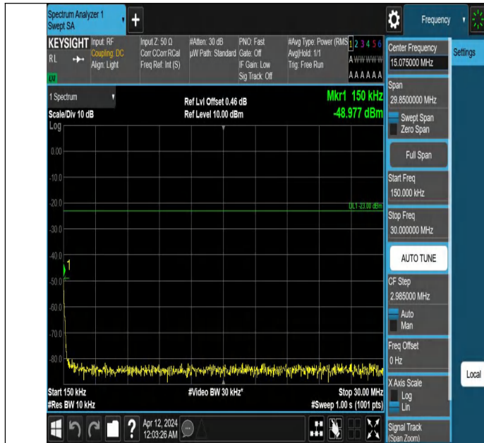
Band26(814-824)-3MHz-QPSK-26705-1RB#0-0.15~30-PASS
