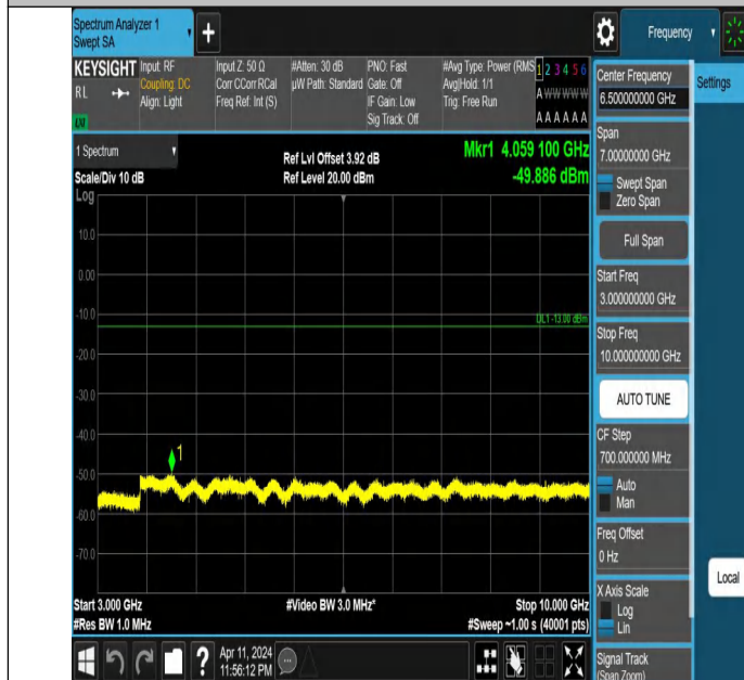
Band26(814-824)-1.4MHz-QPSK-26783-1RB#0-3000~10000-PASS
