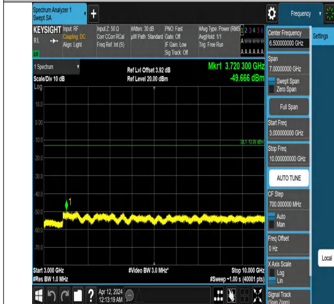
Band26(814-824)-5MHz-QPSK-26715-1RB#0-3000~10000-PASS
