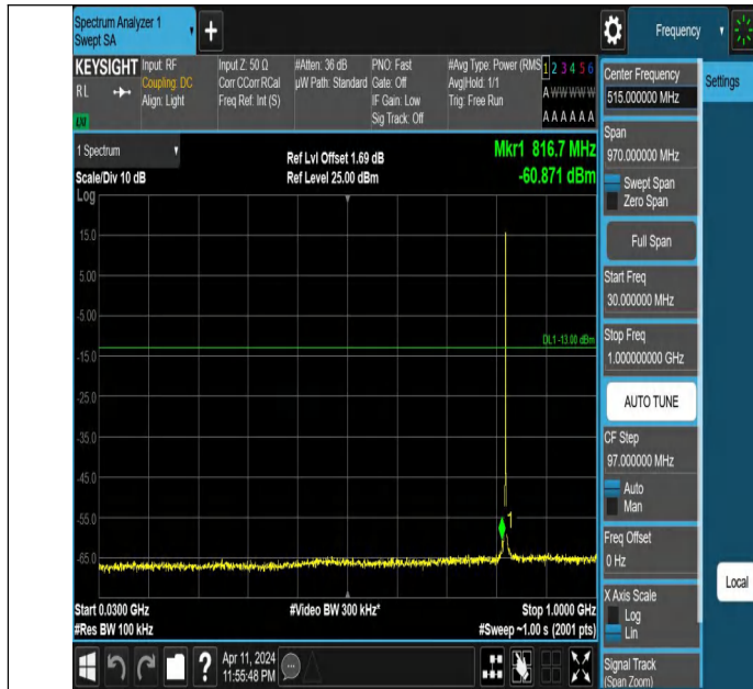
Band26(814-824)-1.4MHz-QPSK-26783-1RB#0-30~1000-PASS
