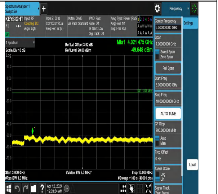
Band26(814-824)-3MHz-QPSK-26705-1RB#0-3000~10000-PASS
