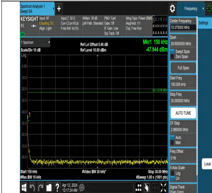
Band26(814-824)-10MHz-QPSK-26740-1RB#0-0.15~30-PASS
