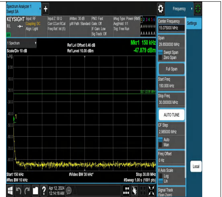
Band26(814-824)-5MHz-QPSK-26765-1RB#0-0.15~30-PASS
