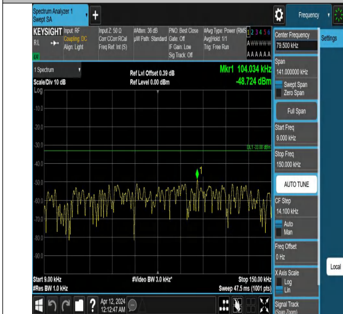
Band26(814-824)-5MHz-QPSK-26715-1RB#0-0.009~0.15-PASS
