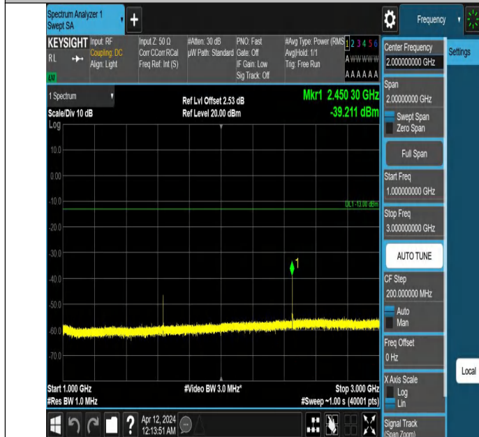
Band26(814-824)-5MHz-QPSK-26740-1RB#0-1000~3000-PASS
