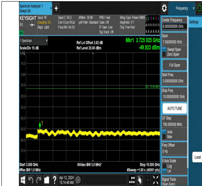
Band26(814-824)-5MHz-QPSK-26765-1RB#0-3000~10000-PASS
