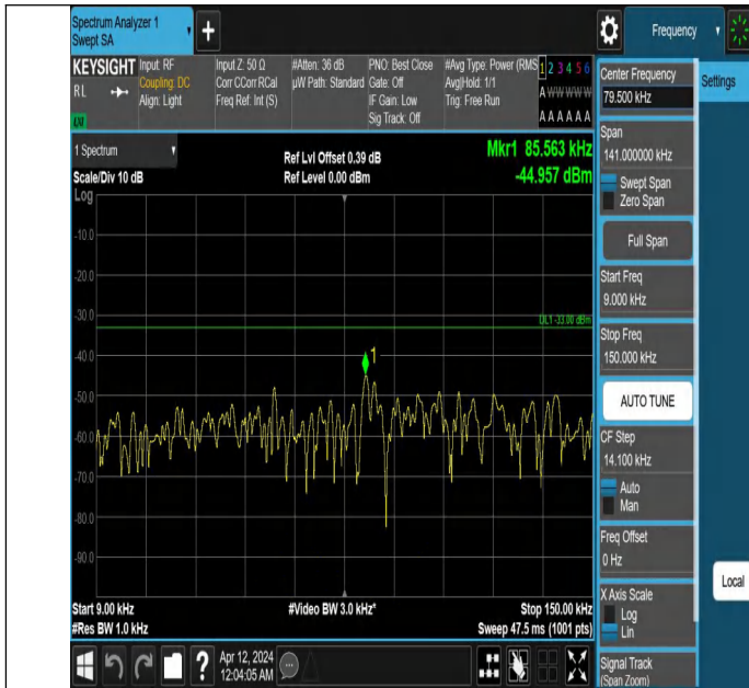
Band26(814-824)-3MHz-QPSK-26740-1RB#0-0.009~0.15-PASS
