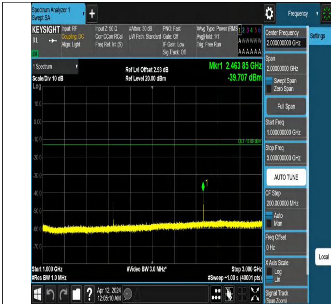
Band26(814-824)-3MHz-QPSK-26775-1RB#0-1000~3000-PASS
