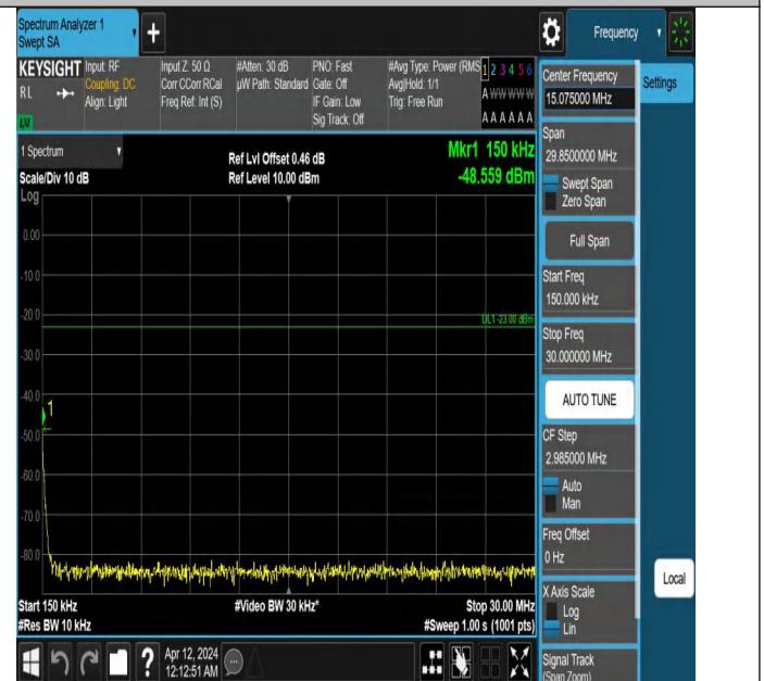
Band26(814-824)-5MHz-QPSK-26715-1RB#0-0.15~30-PASS
