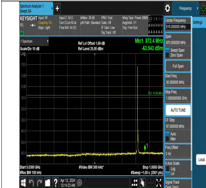
Band26(814-824)-5MHz-QPSK-26765-1RB#0-30~1000-PASS
