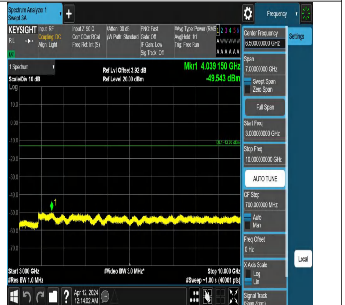
Band26(814-824)-5MHz-QPSK-26740-1RB#0-3000~10000-PASS
