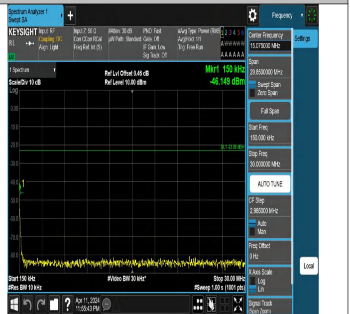
Band26(814-824)-1.4MHz-QPSK-26783-1RB#0-0.15~30-PASS
