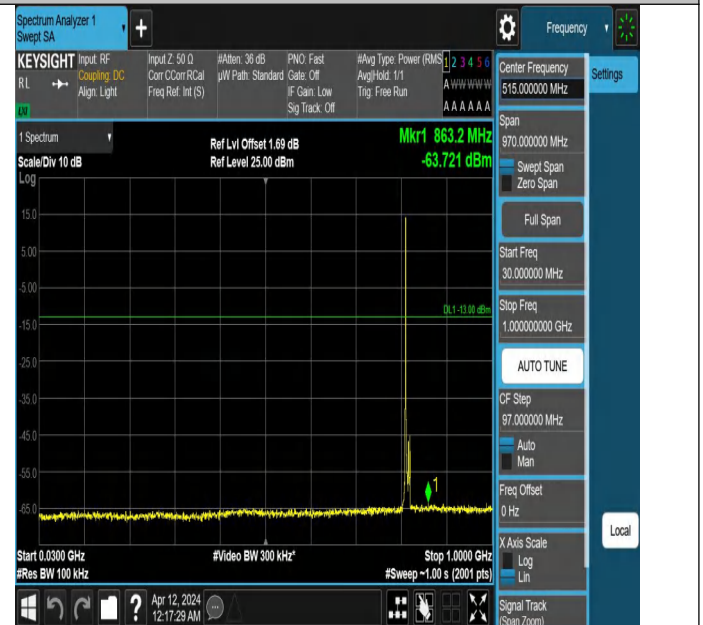
Band26(814-824)-10MHz-QPSK-26740-1RB#0-30~1000-PASS
