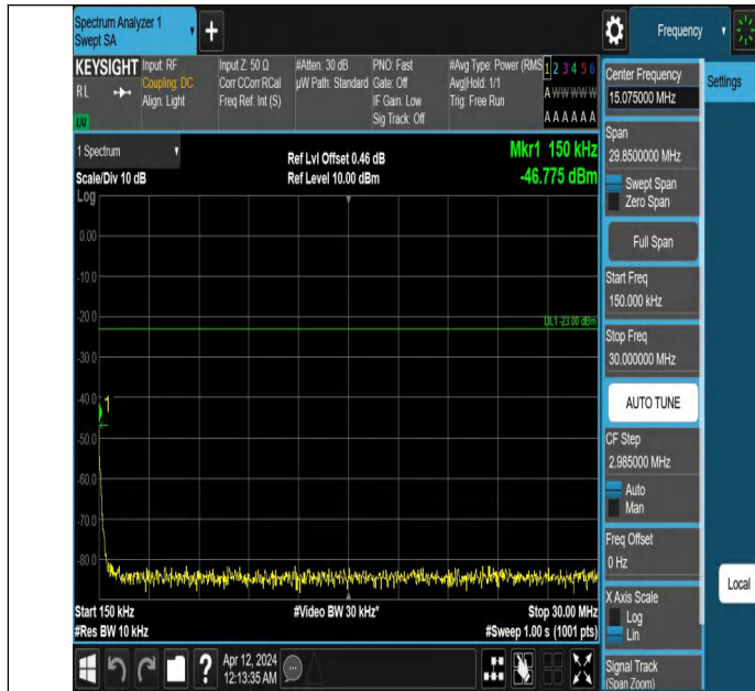
Band26(814-824)-5MHz-QPSK-26740-1RB#0-0.15~30-PASS
