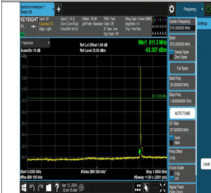
Band26(814-824)-3MHz-QPSK-26740-1RB#0-30~1000-PASS
