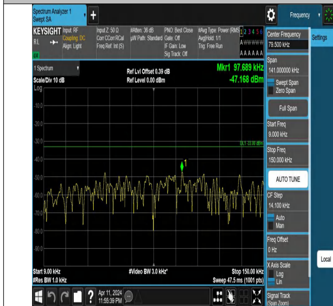
Band26(814-824)-1.4MHz-QPSK-26783-1RB#0-0.009~0.15-PASS
