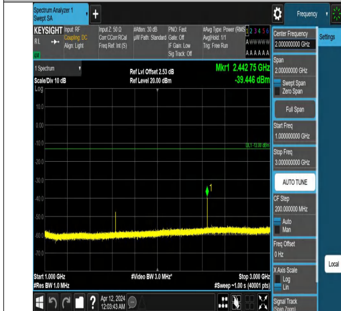
Band26(814-824)-3MHz-QPSK-26705-1RB#0-1000~3000-PASS
