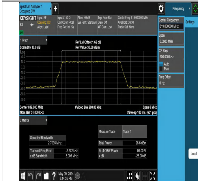
Band26(814-824)-3MHz-256QAM-26740-15RB#0-PASS
