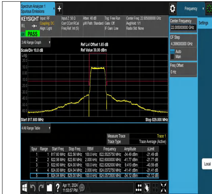
Band26(814-824)-1.4MHz-QPSK-26783-6RB#0-PASS
