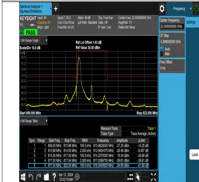
Band26(814-824)-3MHz-QPSK-26705-1RB#0-PASS
