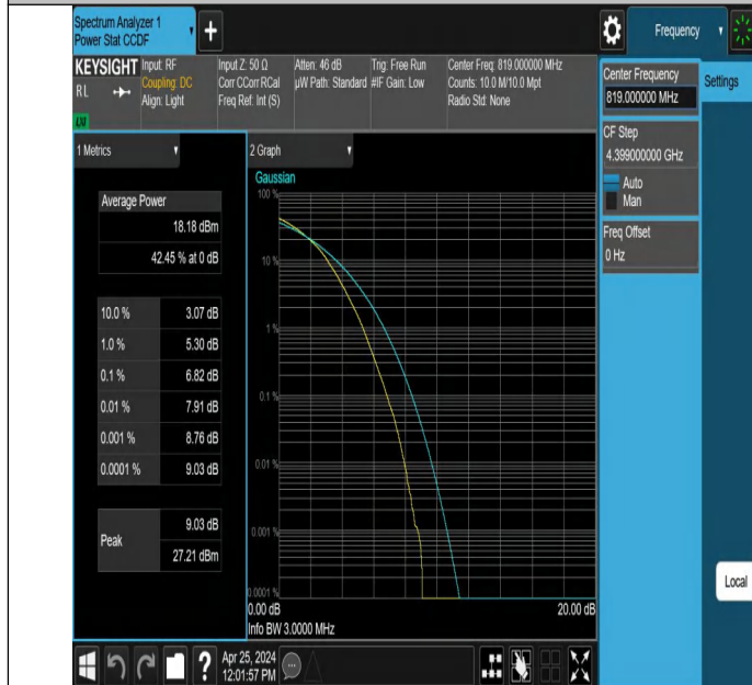
Band26(814-824)-3MHz-256QAM-26740-15RB#0-PASS
