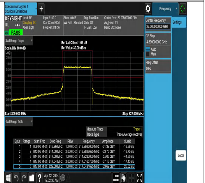
Band26(814-824)-3MHz-QPSK-26705-15RB#0-PASS
