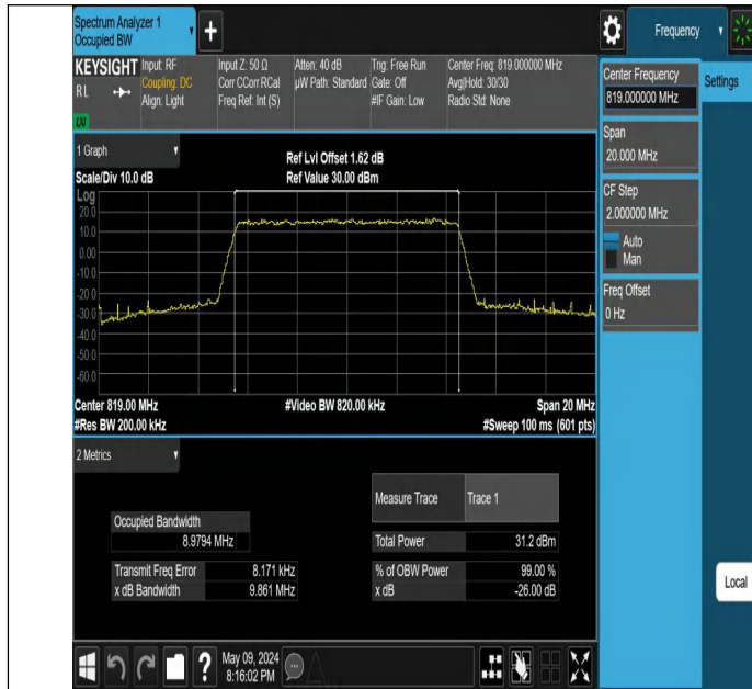
Band26(814-824)-10MHz-QPSK-26740-50RB#0-PASS
