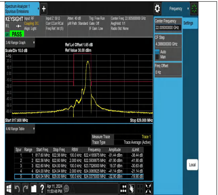
Band26(814-824)-1.4MHz-QPSK-26783-1RB#5-PASS
