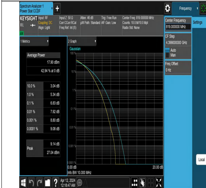
Band26(814-824)-10MHz-256QAM-26740-50RB#0-PASS
