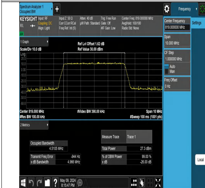
Band26(814-824)-5MHz-256QAM-26740-25RB#0-PASS
