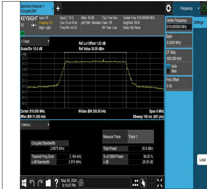
Band26(814-824)-3MHz-QPSK-26740-15RB#0-PASS
