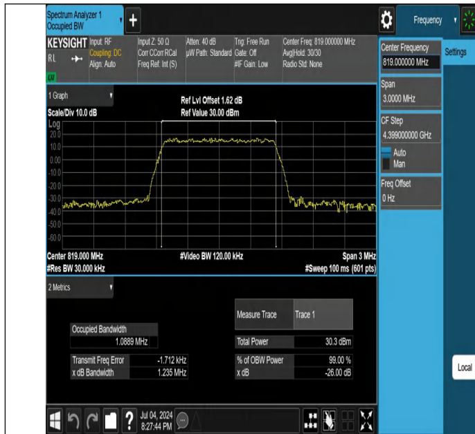
Band26(814-824)-1.4MHz-QPSK-26740-6RB#0-PASS
