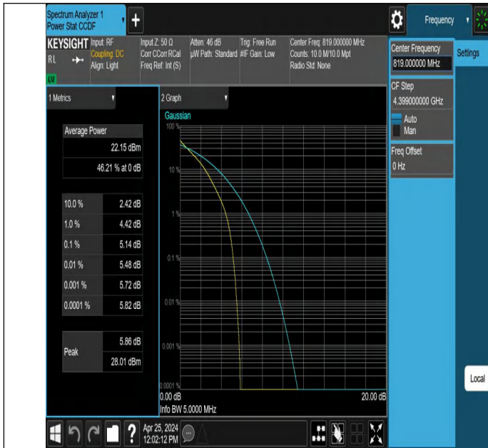
Band26(814-824)-5MHz-QPSK-26740-25RB#0-PASS
