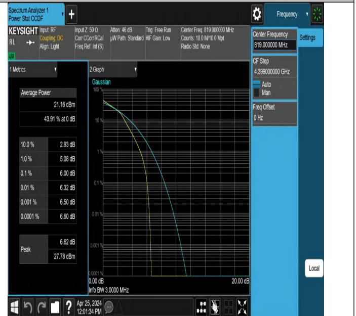
Band26(814-824)-3MHz-16QAM-26740-15RB#0-PASS
