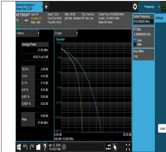
Band26(814-824)-10MHz-QPSK-26740-50RB#0-PASS
