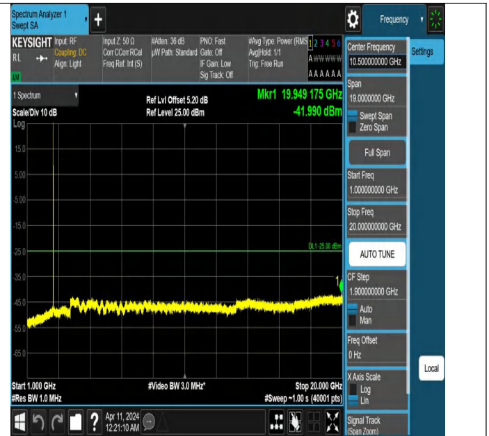
Band7_5MHz_QPSK_21425_1RB#0_1000~20000_1000~20000
