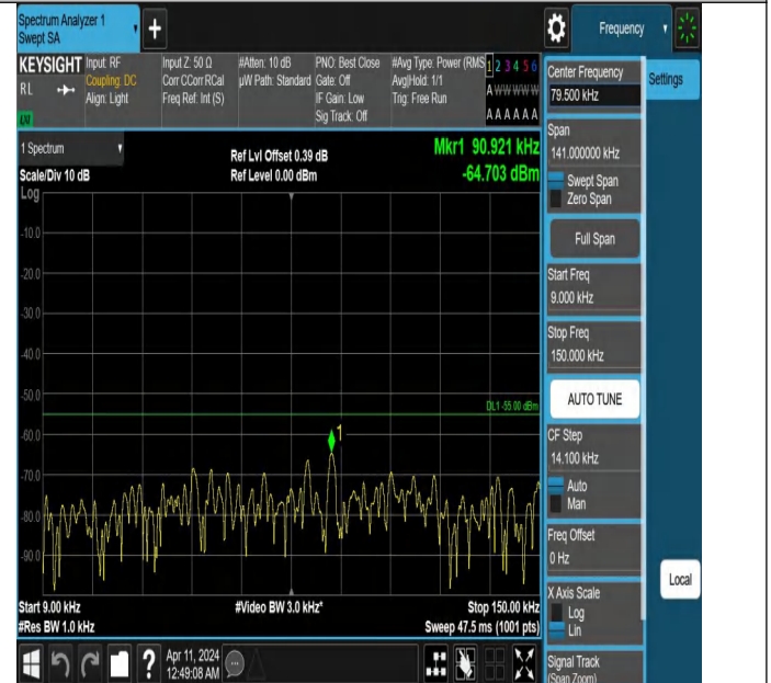
Band7_20MHz_QPSK_21350_1RB#0_0.009~0.15_0.009~0.15
