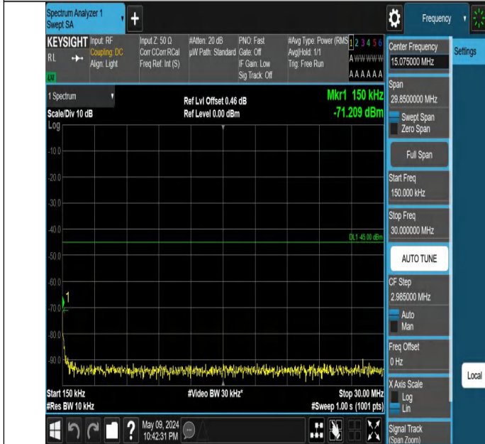
Band7_20MHz_QPSK_20850_1RB#0_0.15~30_0.15~30
