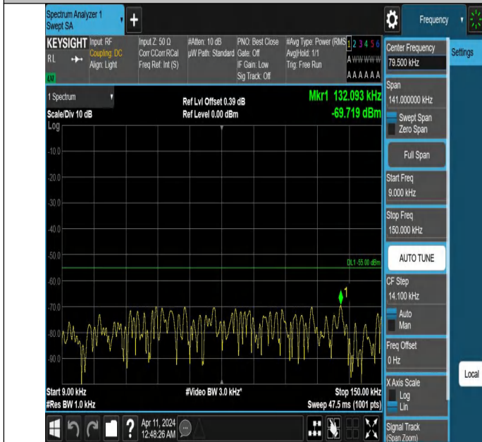
Band7_20MHz_QPSK_21100_1RB#0_0.009~0.15_0.009~0.15
