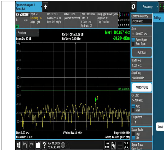
Band7_20MHz_QPSK_20850_1RB#0_0.009~0.15_0.009~0.15
