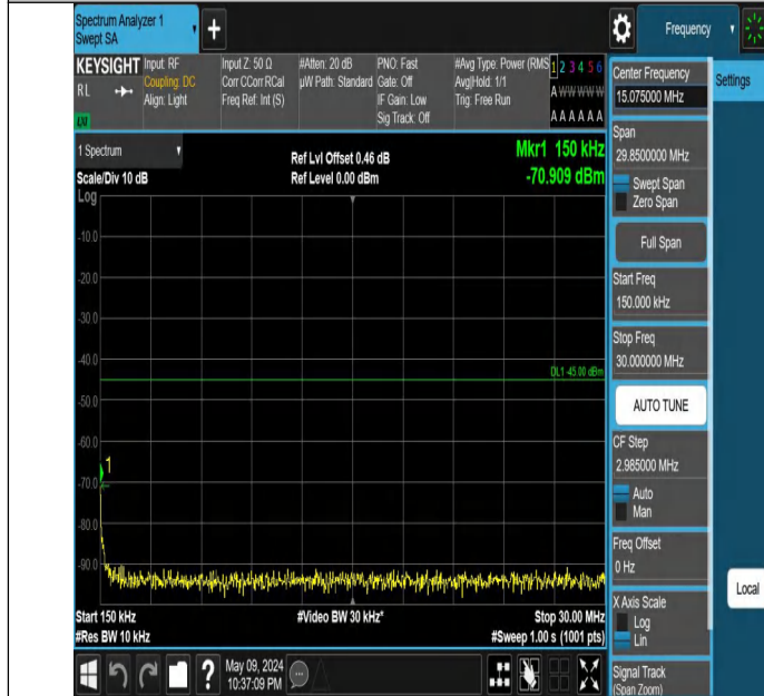
Band7_5MHz_QPSK_21100_1RB#0_0.15~30_0.15~30
