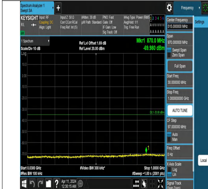
Band7_10MHz_QPSK_21400_1RB#0_30~1000_30~1000
