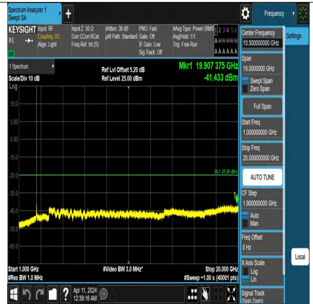
Band7_15MHz_QPSK_21100_1RB#0_1000~20000_1000~20000
