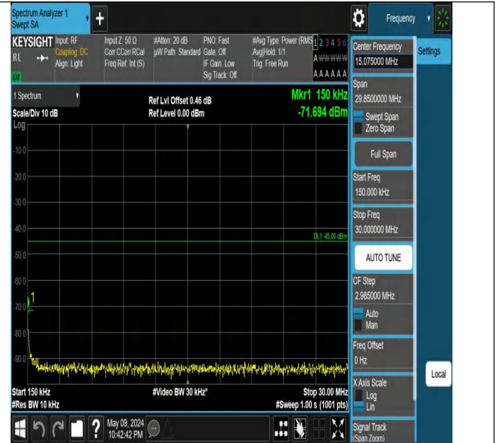
Band7_20MHz_QPSK_21100_1RB#0_0.15~30_0.15~30
