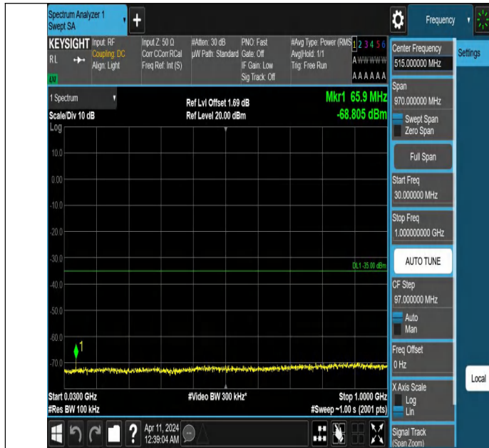
Band7_15MHz_QPSK_21100_1RB#0_30~1000_30~1000
