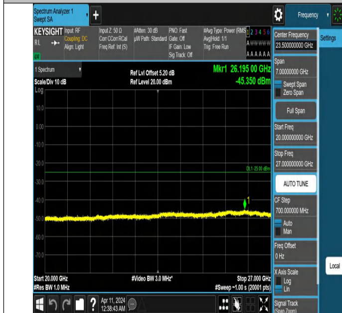
Band7_15MHz_QPSK_20825_1RB#0_20000~27000_20000~270
