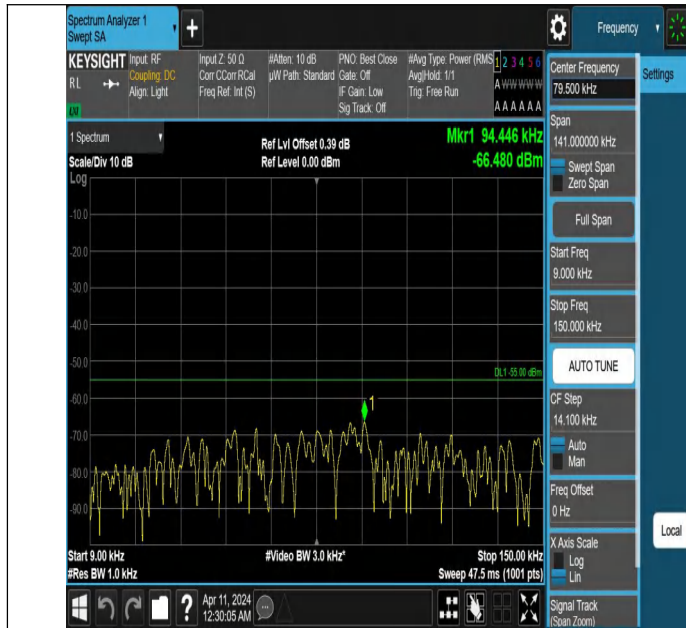
Band7_10MHz_QPSK_21400_1RB#0_0.009~0.15_0.009~0.15
