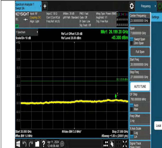
Band7_20MHz_QPSK_21100_1RB#0_20000~27000_20000~2700
