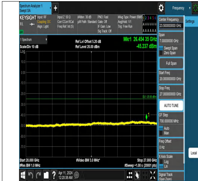
Band7_5MHz_QPSK_21100_1RB#0_20000~27000_20000~27000
