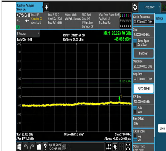
Band7_5MHz_QPSK_21425_1RB#0_20000~27000_20000~27000
