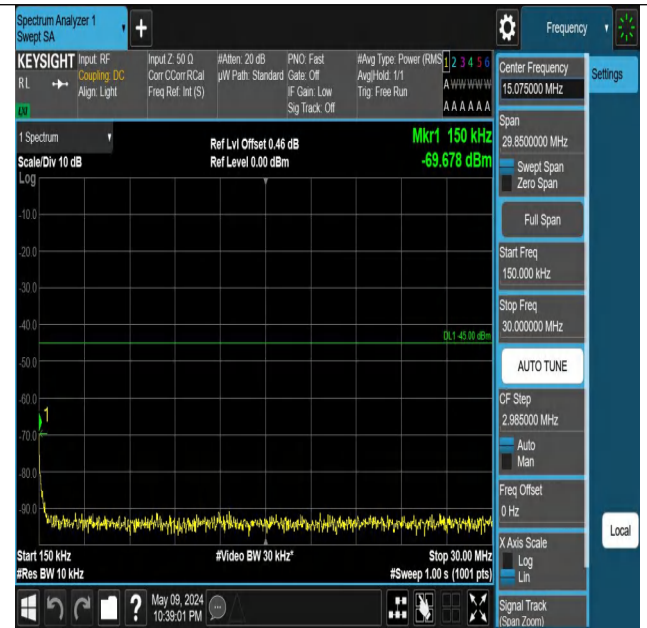
Band7_10MHz_QPSK_21100_1RB#0_0.15~30_0.15~30
