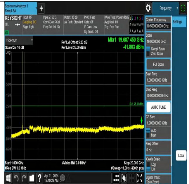
Band7_20MHz_QPSK_21350_1RB#0_1000~20000_1000~20000
