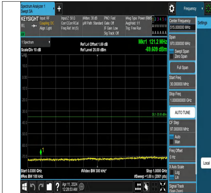
Band7_10MHz_QPSK_20800_1RB#0_30~1000_30~1000
