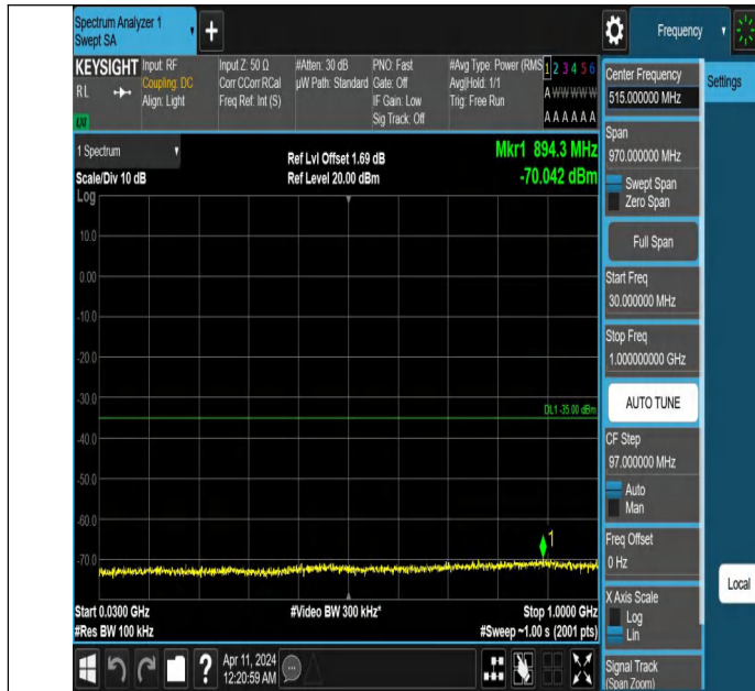
Band7_5MHz_QPSK_21425_1RB#0_30~1000_30~1000
