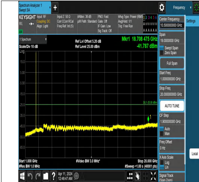
Band7_20MHz_QPSK_21100_1RB#0_1000~20000_1000~20000
