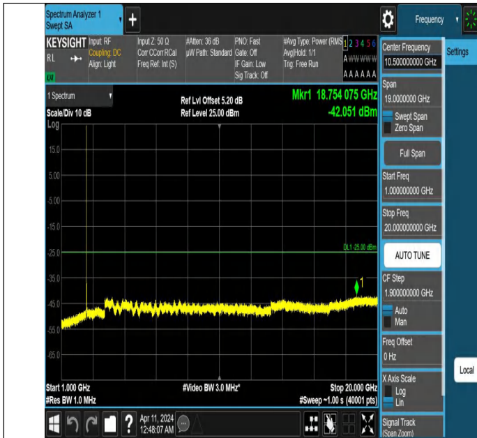
Band7_20MHz_QPSK_20850_1RB#0_1000~20000_1000~20000
