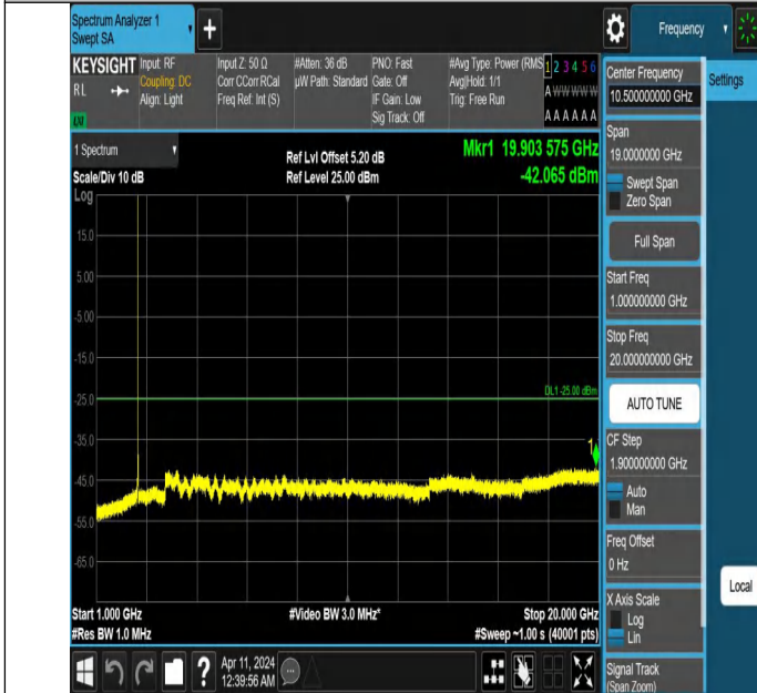
Band7_15MHz_QPSK_21375_1RB#0_1000~20000_1000~20000
