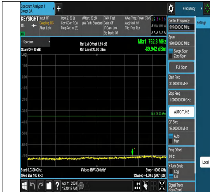
Band7_20MHz_QPSK_21350_1RB#0_30~1000_30~1000
