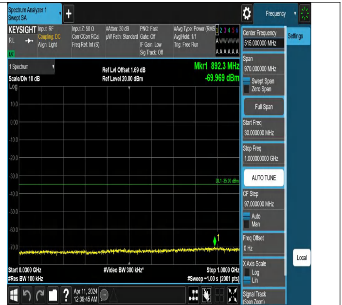
Band7_15MHz_QPSK_21375_1RB#0_30~1000_30~1000
