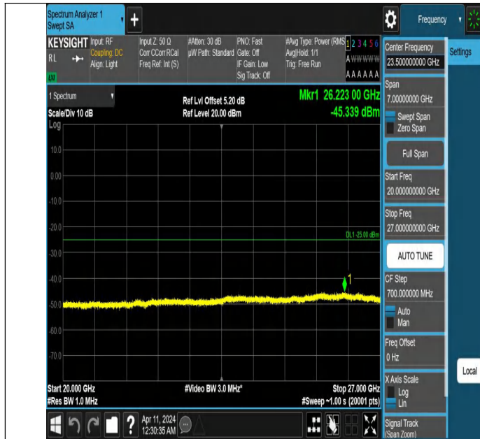
Band7_10MHz_QPSK_21400_1RB#0_20000~27000_20000~27000
