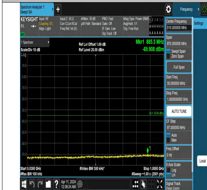
Band7_15MHz_QPSK_20825_1RB#0_30~1000_30~1000
