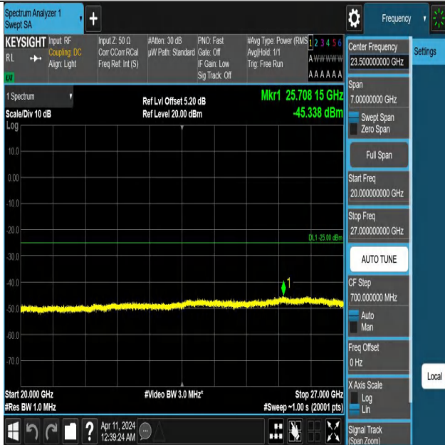
Band7_15MHz_QPSK_21100_1RB#0_20000~27000_20000~2700
