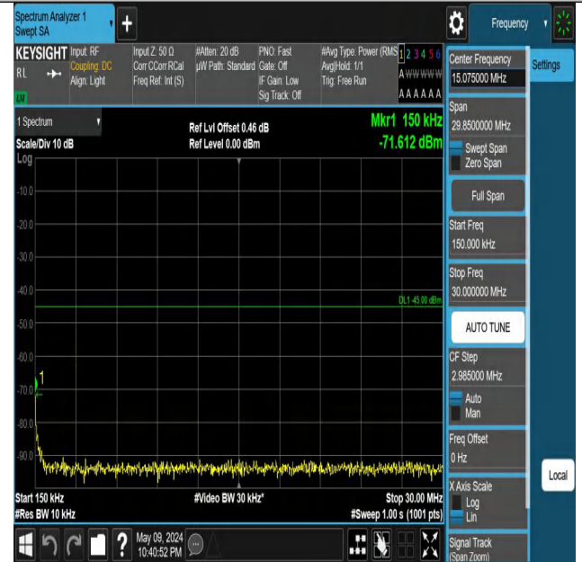
Band7_15MHz_QPSK_21100_1RB#0_0.15~30_0.15~30
