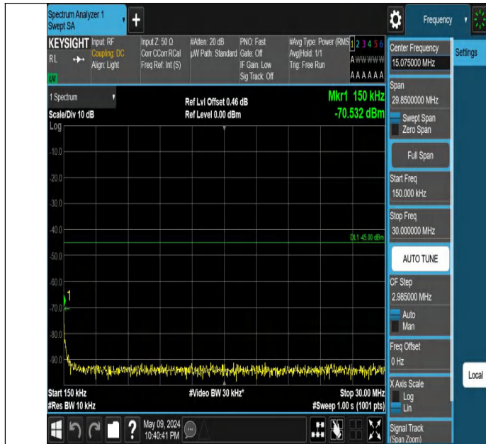
Band7_15MHz_QPSK_20825_1RB#0_0.15~30_0.15~30
