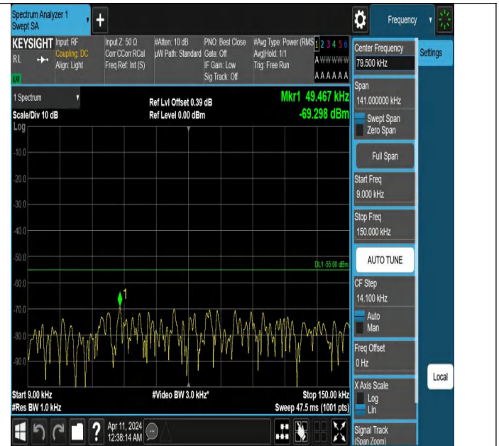
Band7_15MHz_QPSK_20825_1RB#0_0.009~0.15_0.009~0.15
