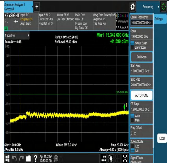
Band7_10MHz_QPSK_21400_1RB#0_1000~20000_1000~20000
