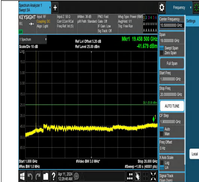
Band7_10MHz_QPSK_21100_1RB#0_1000~20000_1000~20000
