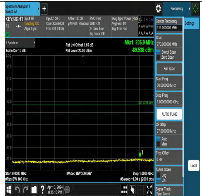
Band4_3MHz_QPSK_19965_1RB#0_30~1000_30~1000
