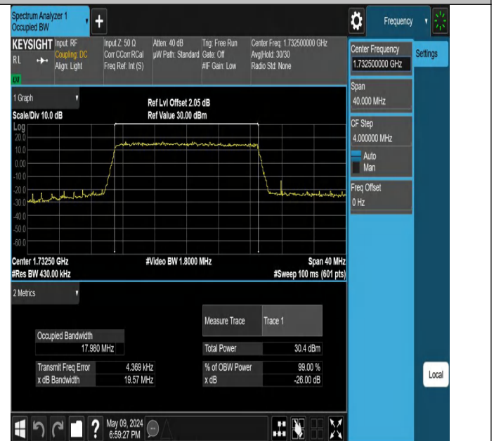
Band4-20MHz-16QAM-20175-100RB#0-PASS
