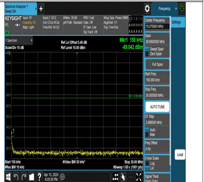
Band4_1.4MHz_QPSK_20393_1RB#0_0.15~30_0.15~30
