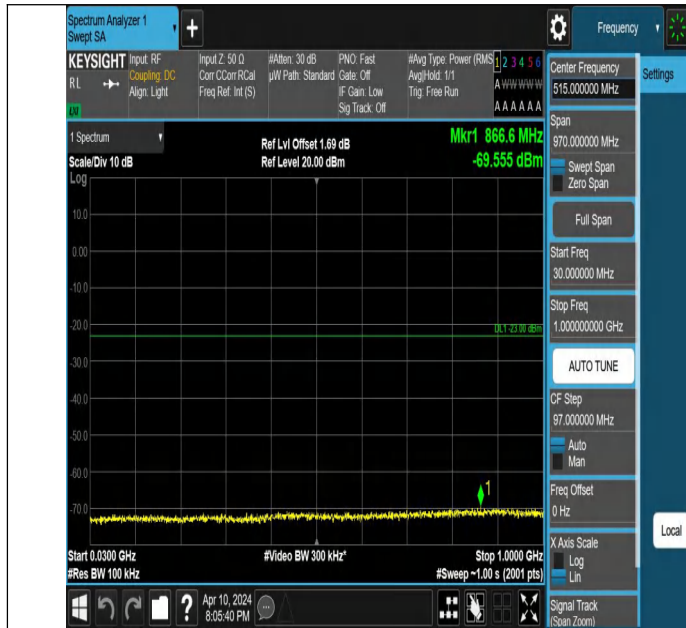
Band4_1.4MHz_QPSK_20393_1RB#0_30~1000_30~1000
