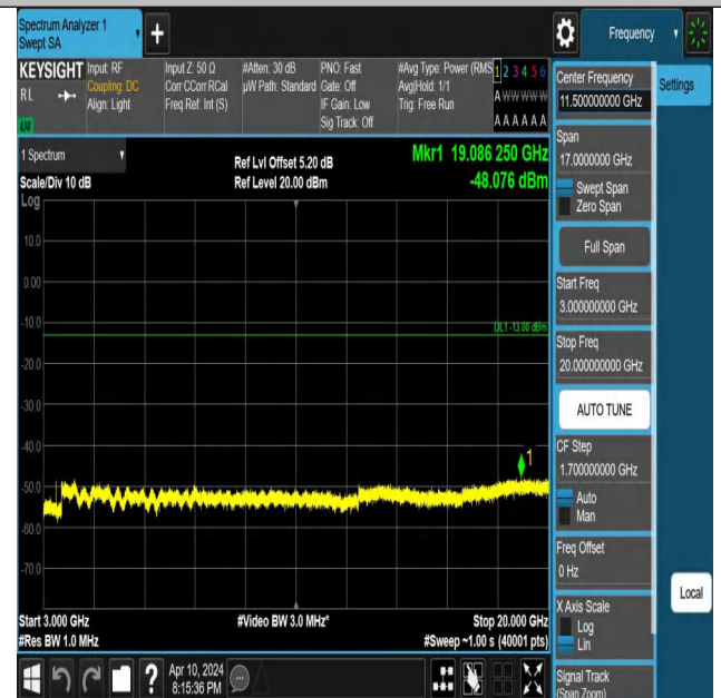
Band4_3MHz_QPSK_19965_1RB#0_3000~20000_3000~20000
