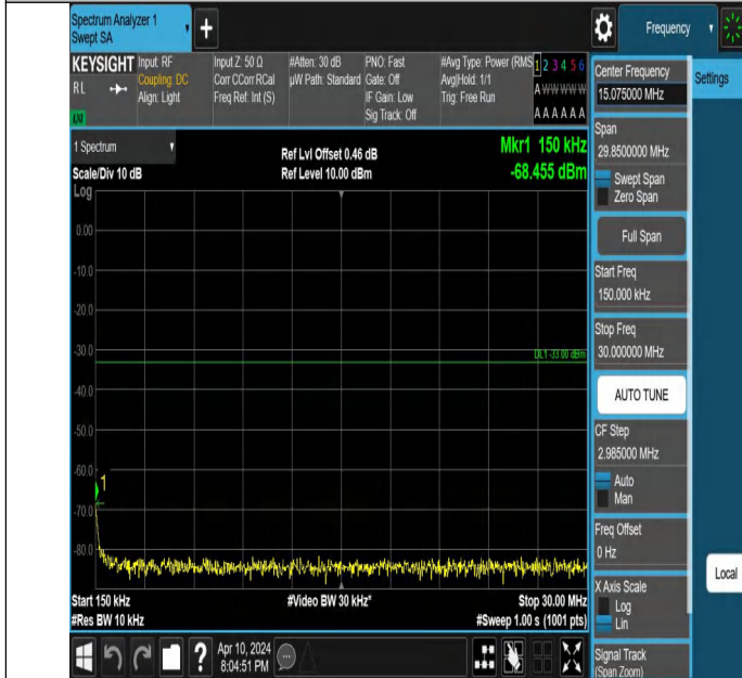
Band4_1.4MHz_QPSK_20175_1RB#0_0.15~30_0.15~30
