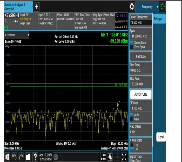
Band4_3MHz_QPSK_19965_1RB#0_0.009~0.15_0.009~0.15
