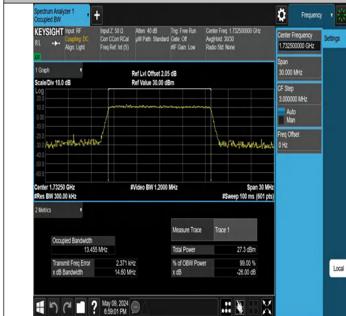
Band4-15MHz-256QAM-20175-75RB#0-PASS
