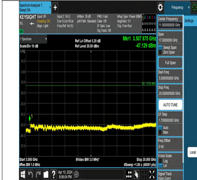
Band4_1.4MHz_QPSK_20393_1RB#0_3000~20000_3000~20000
