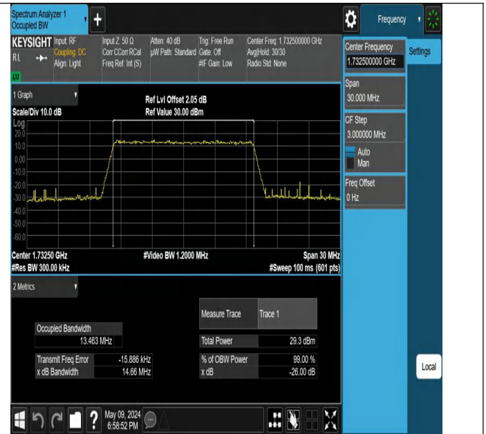
Band4-15MHz-64QAM-20175-75RB#0-PASS
