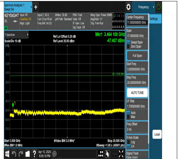
Band4_1.4MHz_QPSK_20175_1RB#0_3000~20000_3000~20000
