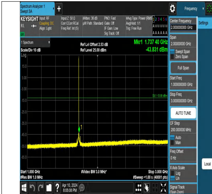
Band4_1.4MHz_QPSK_20175_1RB#0_1000~3000_1000~3000
