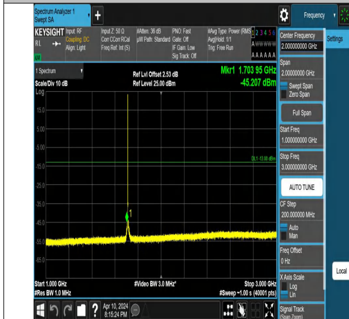
Band4_3MHz_QPSK_19965_1RB#0_1000~3000_1000~3000
