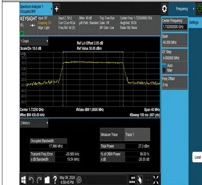
Band4-20MHz-256QAM-20175-100RB#0-PASS
