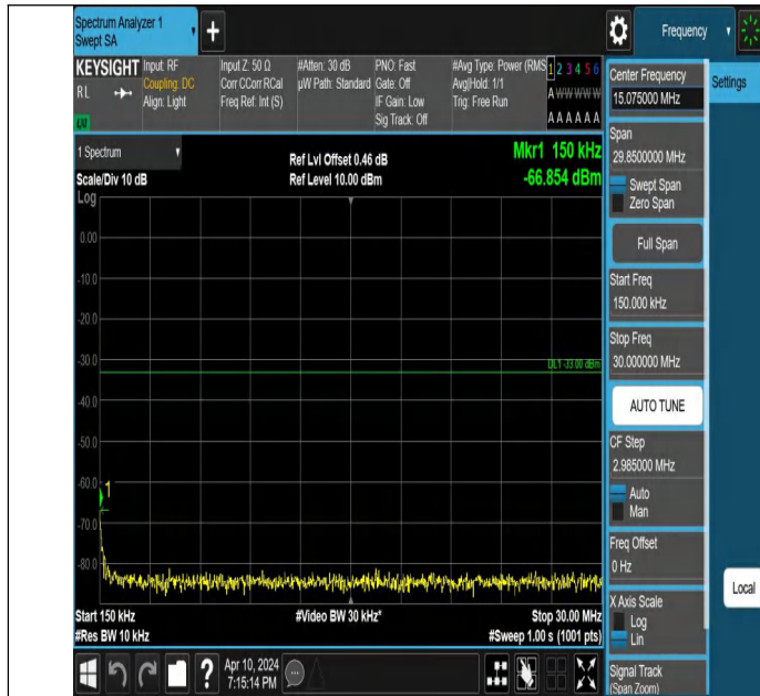
Band2_3MHz_QPSK_18615_1RB#0_0.15~30_0.15~30
