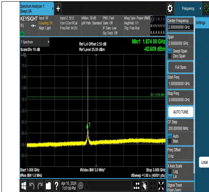
Band2_1.4MHz_QPSK_18900_1RB#0_1000~3000_1000~3000
