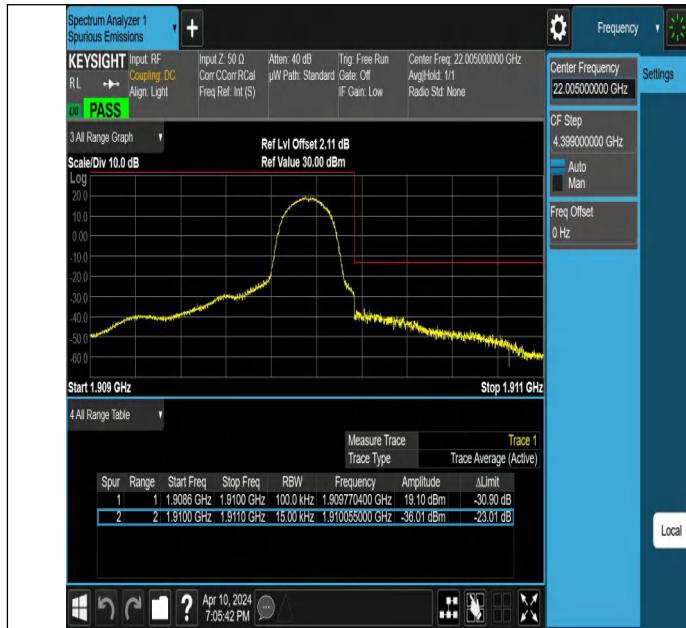
Band2_1.4MHz_QPSK_19193_1RB#5
