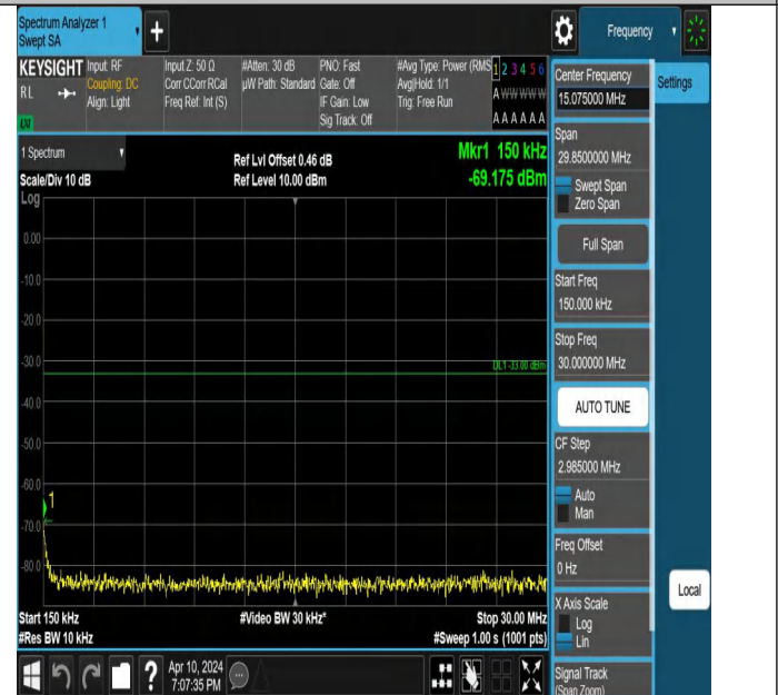
Band2_1.4MHz_QPSK_19193_1RB#0_0.15~30_0.15~30
