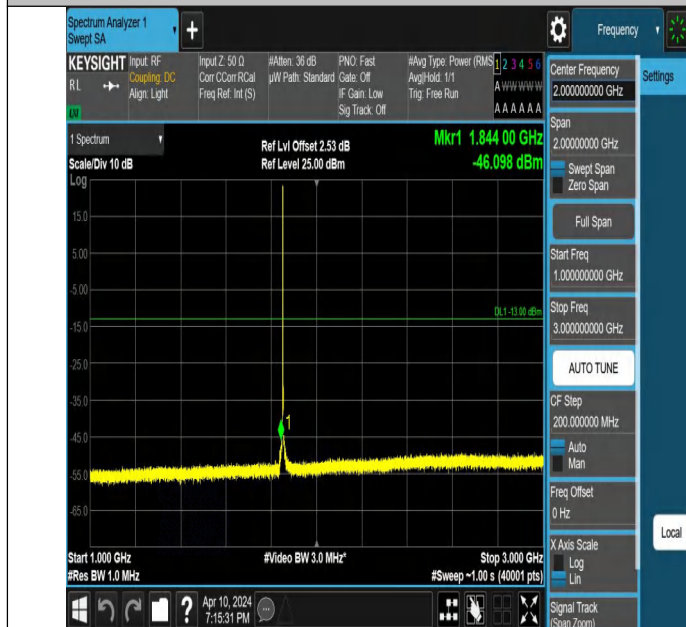
Band2_3MHz_QPSK_18615_1RB#0_1000~3000_1000~3000
