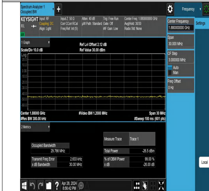
Band2-15MHz-256QAM-18900-75RB#0-PASS
