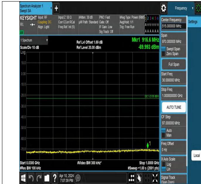
Band2_1.4MHz_QPSK_19193_1RB#0_30~1000_30~1000
