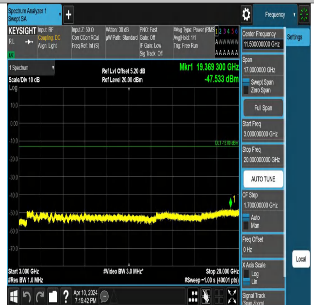
Band2_3MHz_QPSK_18615_1RB#0_3000~20000_3000~20000
