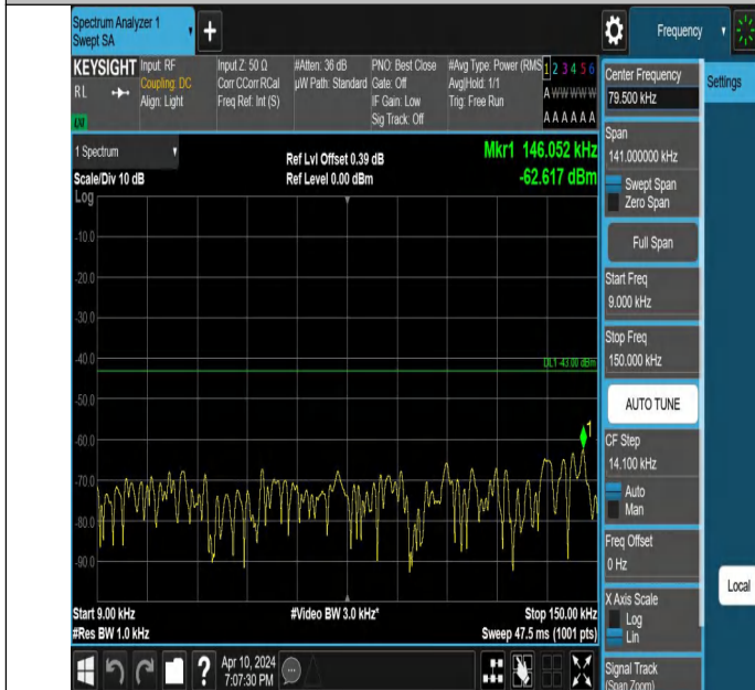
Band2_1.4MHz_QPSK_19193_1RB#0_0.009~0.15_0.009~0.15
