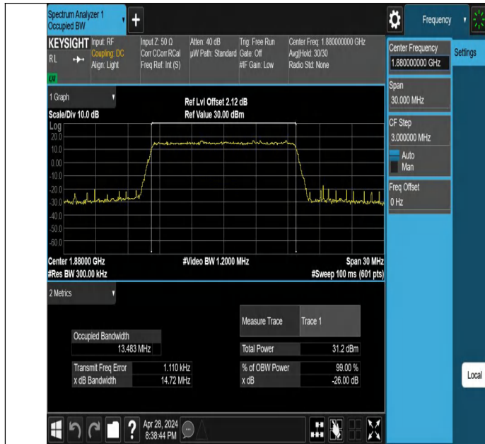
Band2-15MHz-QPSK-18900-75RB#0-PASS
