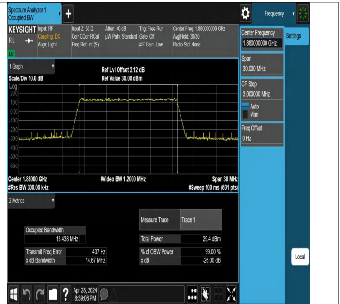
Band2-15MHz-64QAM-18900-75RB#0-PASS
