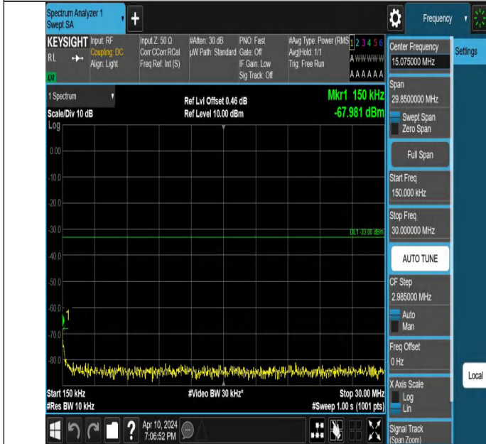
Band2_1.4MHz_QPSK_18900_1RB#0_0.15~30_0.15~30
