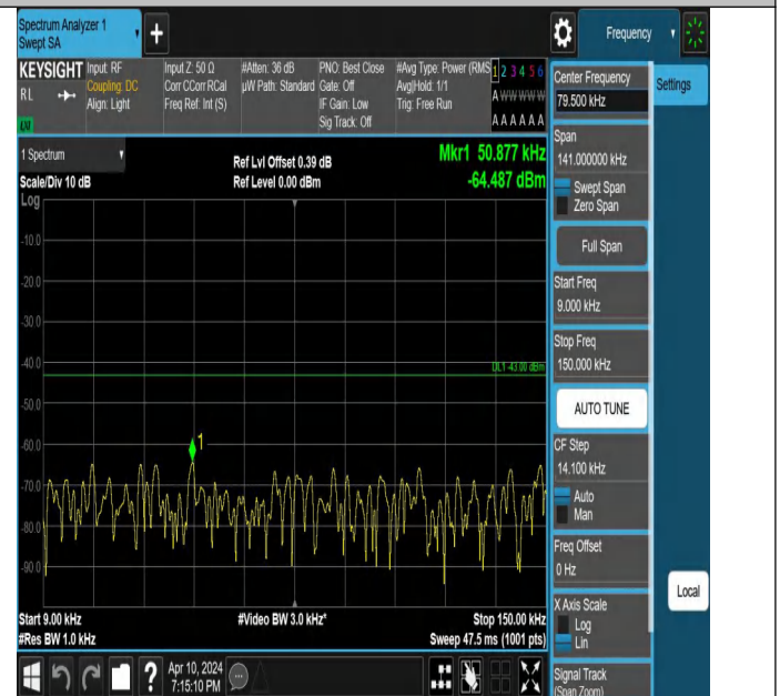
Band2_3MHz_QPSK_18615_1RB#0_0.009~0.15_0.009~0.15
