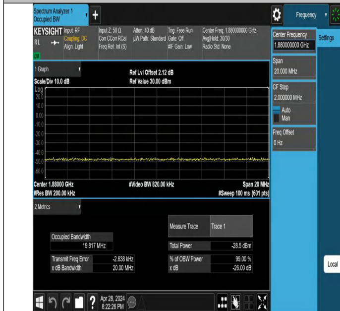
Band2-10MHz-256QAM-18900-50RB#0-PASS
