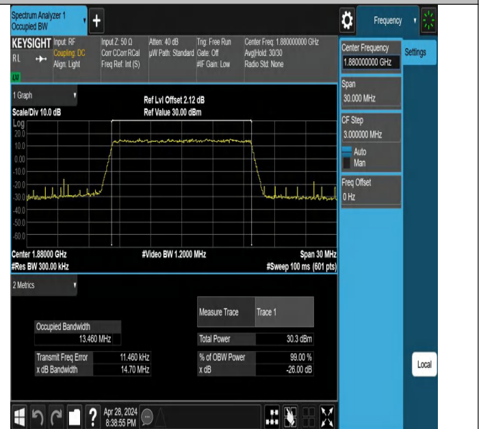
Band2-15MHz-16QAM-18900-75RB#0-PASS
