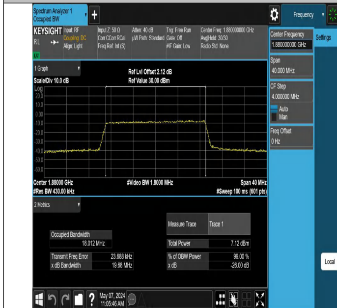
Band2-20MHz-256QAM-18900-100RB#0-PASS
