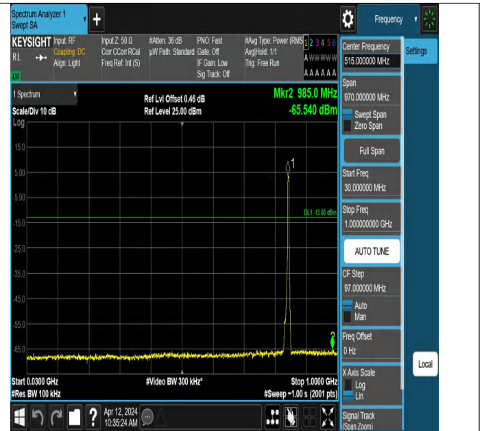
Band5-4233-4-30~1000MHz-PASS
