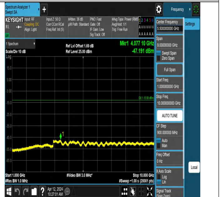
Band5-4233-1-1000~10000MHz-PASS
