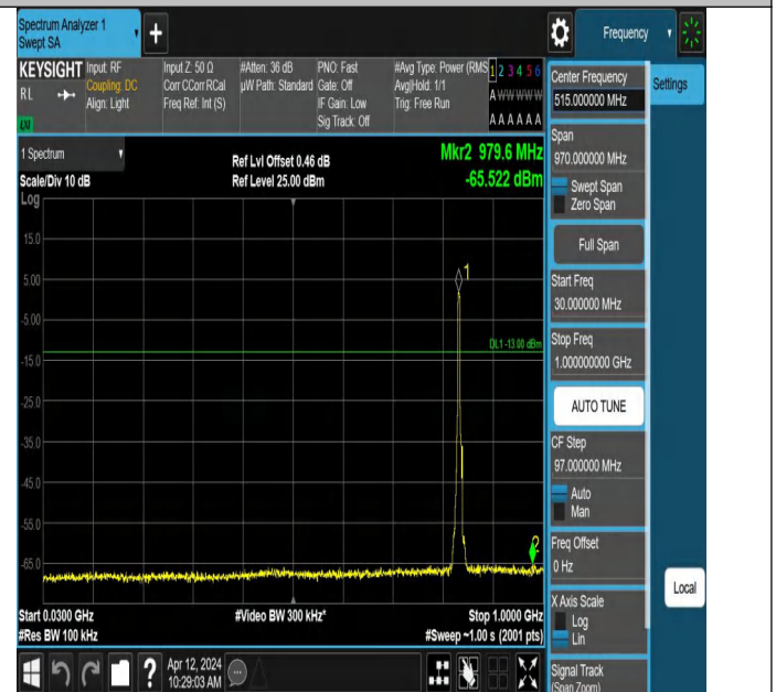
Band5-4182-2-30~1000MHz-PASS
