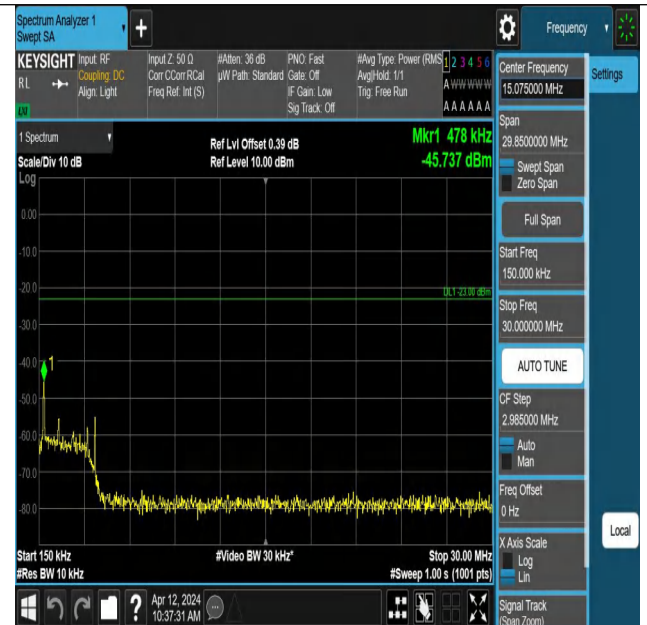
Band5-4233-5-0.15~30MHz-PASS
