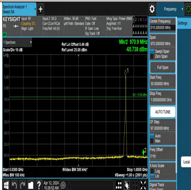
Band5-4233-1-30~1000MHz-PASS
