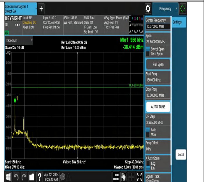
Band5-4182-4-0.15~30MHz-PASS
