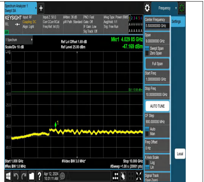
Band5-4132-3-1000~10000MHz-PASS
