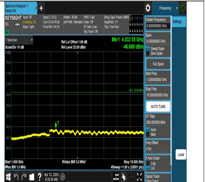
Band5-4182-1000~10000MHz-PASS
