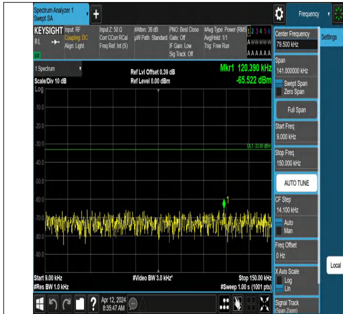
Band5-4233-0.009~0.15MHz-PASS
