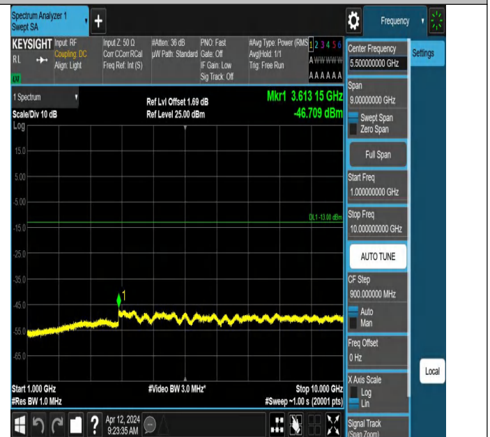
Band5-4233-4-1000~10000MHz-PASS
