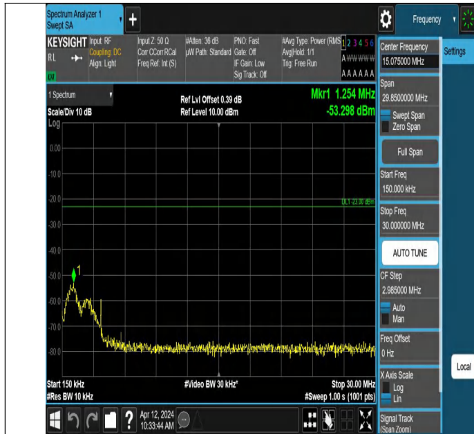
Band5-4132-4-0.15~30MHz-PASS
