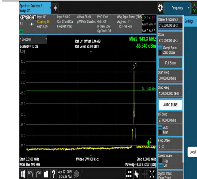
Band5-4182-30~1000MHz-PASS
