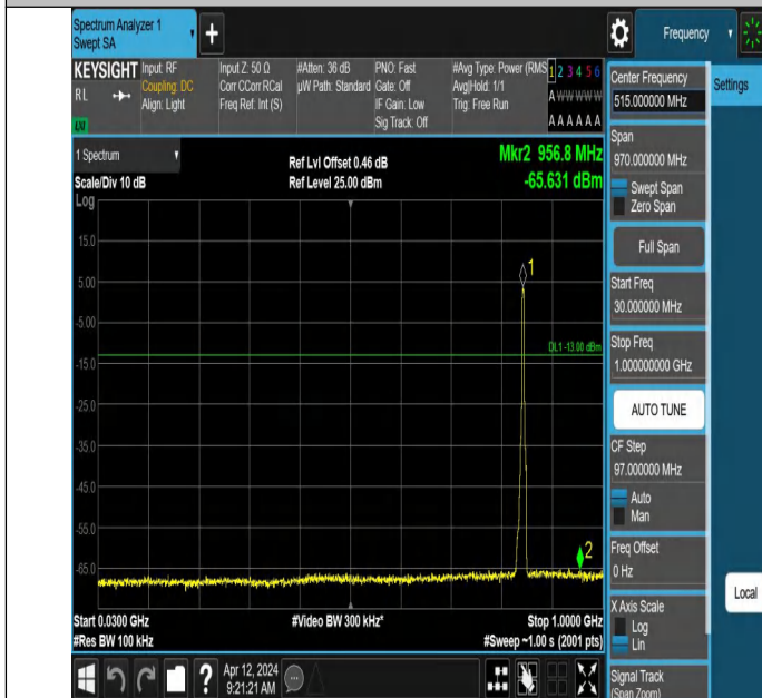
Band5-4233-3-30~1000MHz-PASS
