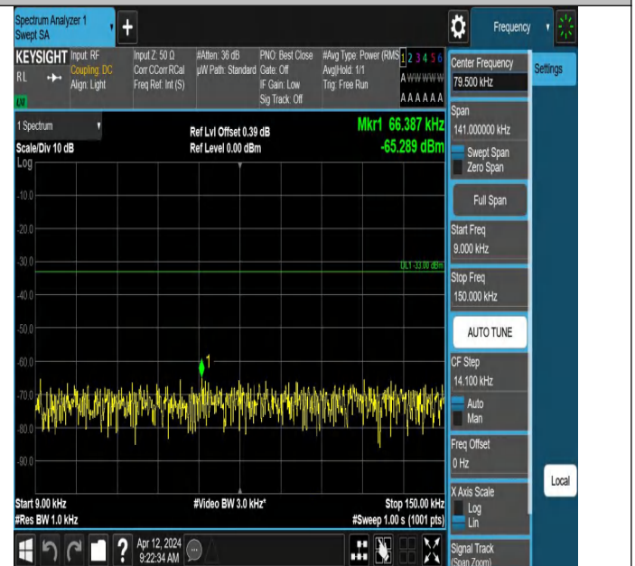
Band5-4182-4-0.009~0.15MHz-PASS
