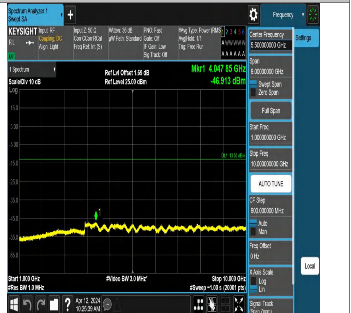
Band5-4132-1-1000~10000MHz-PASS
