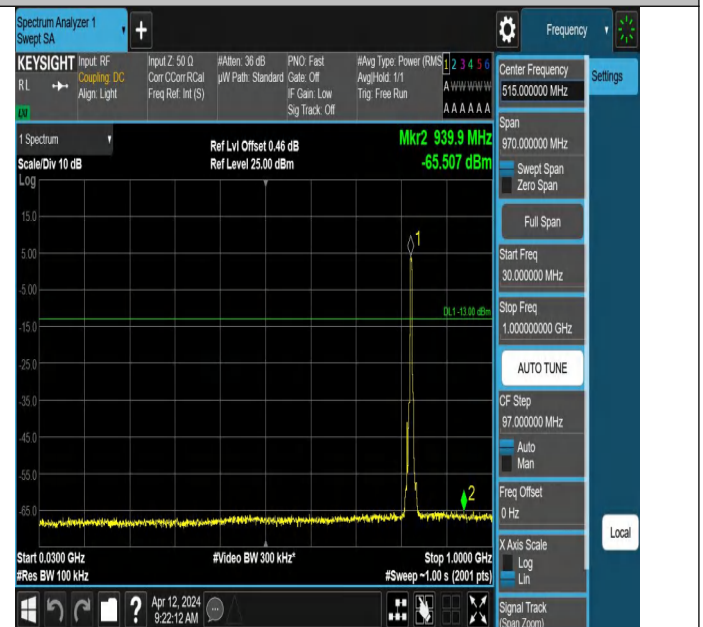
Band5-4132-4-30~1000MHz-PASS
