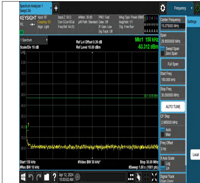
Band4-1413-1-0.15~30MHz-PASS
