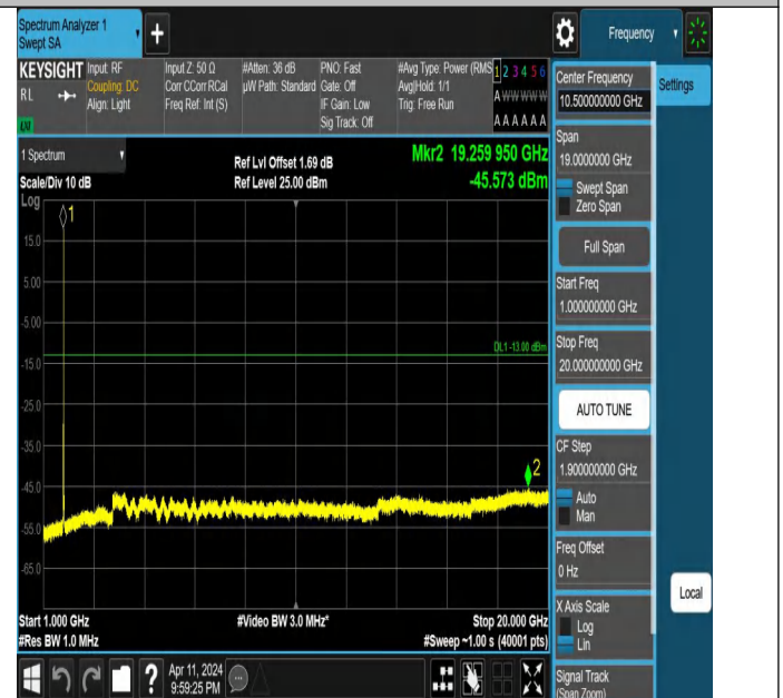
Band4-1513-1000~20000MHz-PASS
