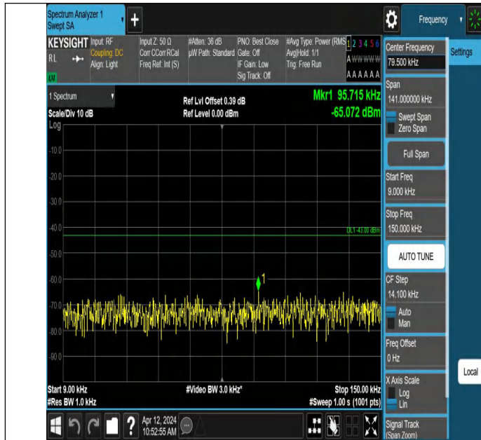
Band4-1413-1-0.009~0.15MHz-PASS
