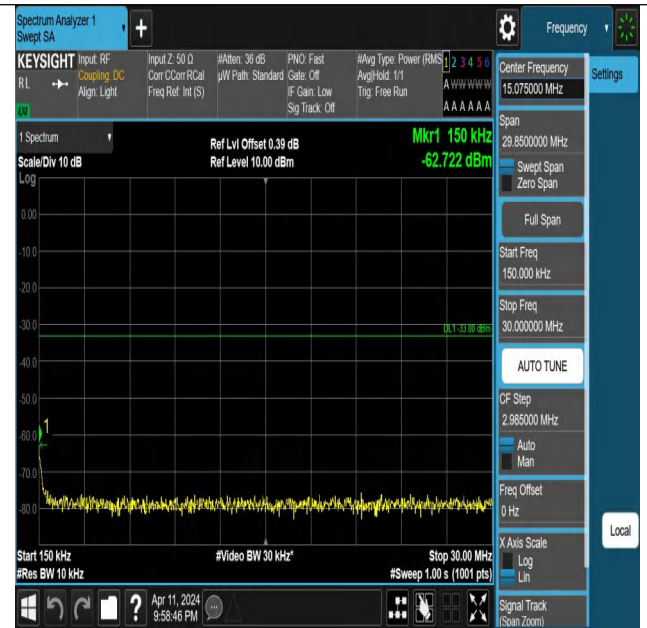
Band4-1413-0.15~30MHz-PASS
