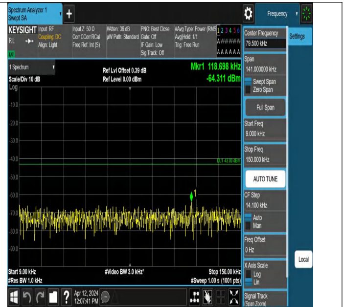
Band4-1312-2-0.009~0.15MHz-PASS
