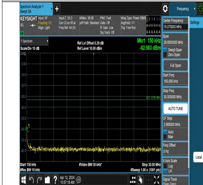
Band4-1413-3-0.15~30MHz-PASS
