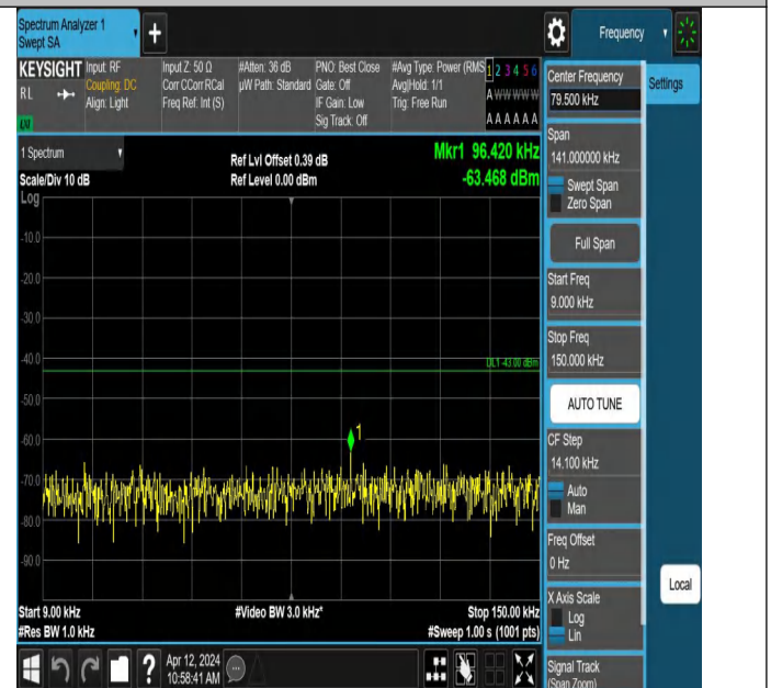
Band4-1312-4-0.009~0.15MHz-PASS
