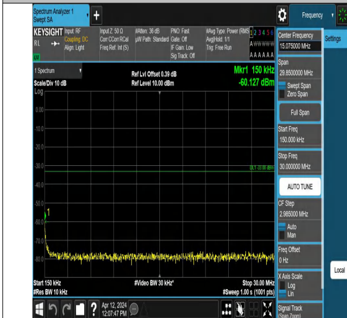
Band4-1312-2-0.15~30MHz-PASS
