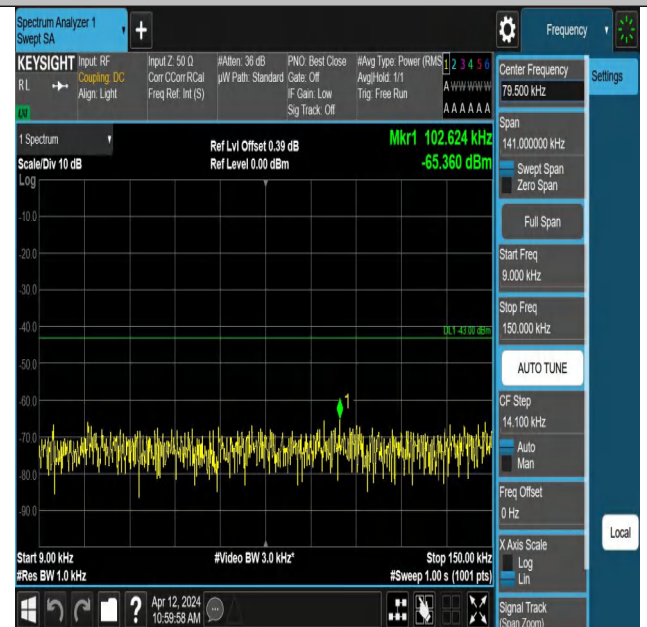
Band4-1513-4-0.009~0.15MHz-PASS
