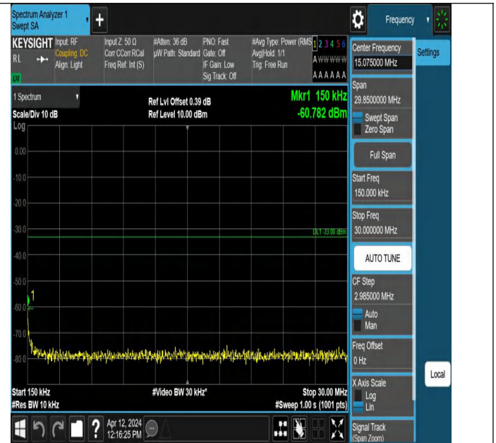
Band4-1312-5-0.15~30MHz-PASS
