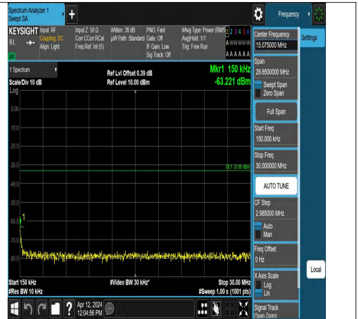
Band4-1312-1-0.15~30MHz-PASS
