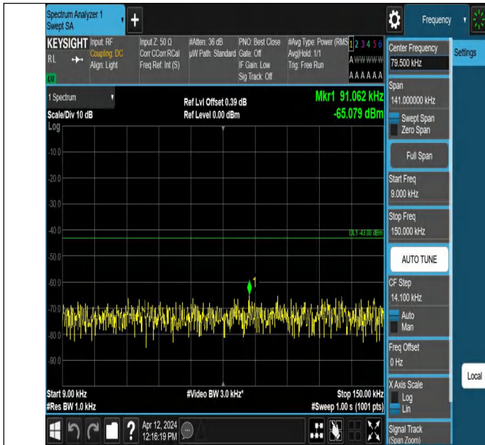
Band4-1312-5-0.009~0.15MHz-PASS
