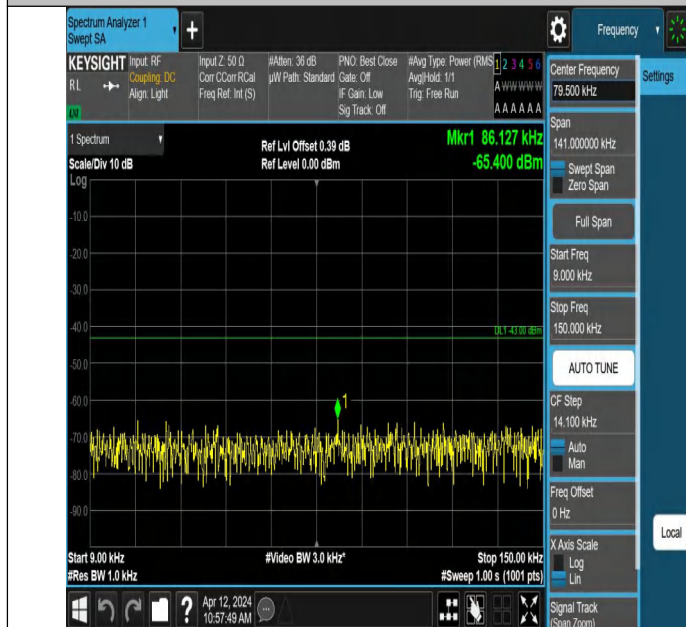
Band4-1513-3-0.009~0.15MHz-PASS
