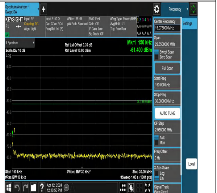
Band4-1312-3-0.15~30MHz-PASS
