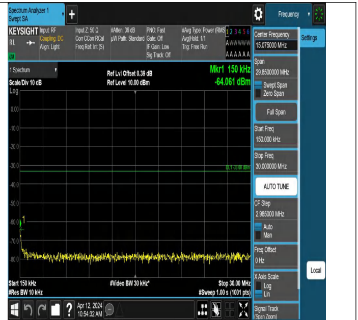
Band4-1312-2-0.15~30MHz-PASS
