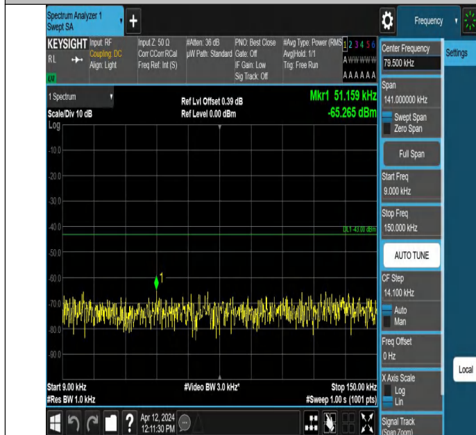
Band4-1413-3-0.009~0.15MHz-PASS
