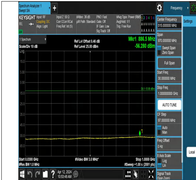
Band4-1513-1-30~1000MHz-PASS
