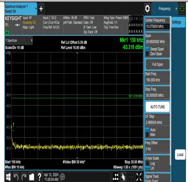
Band4-1513-4-0.15~30MHz-PASS
