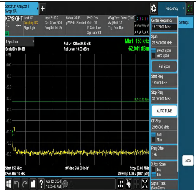
Band4-1513-2-0.15~30MHz-PASS
