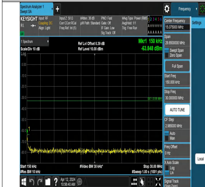
Band4-1312-3-0.15~30MHz-PASS
