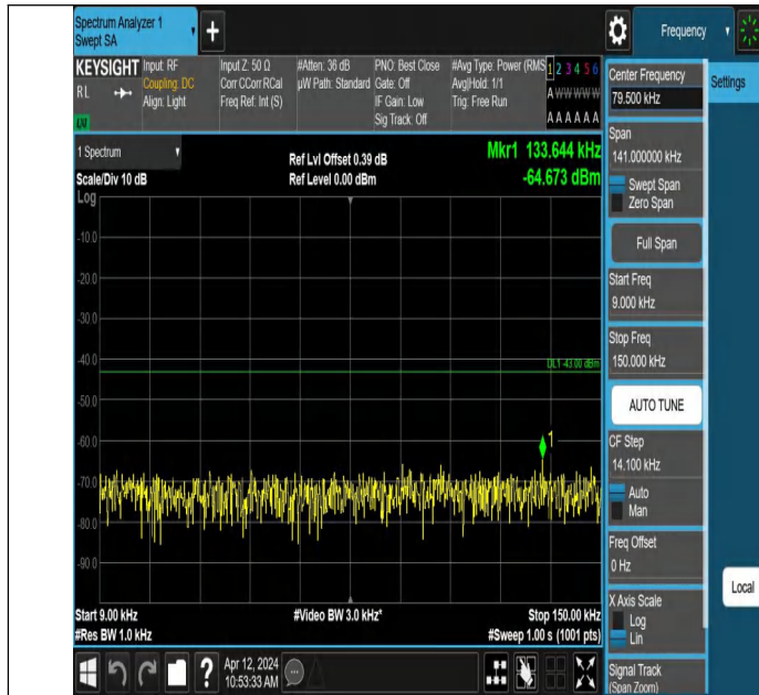
Band4-1513-1-0.009~0.15MHz-PASS
