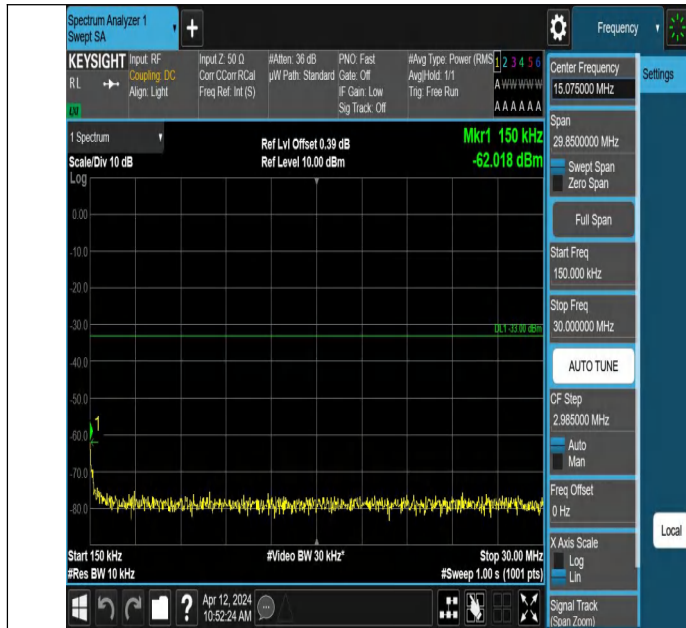
Band4-1312-1-0.15~30MHz-PASS
