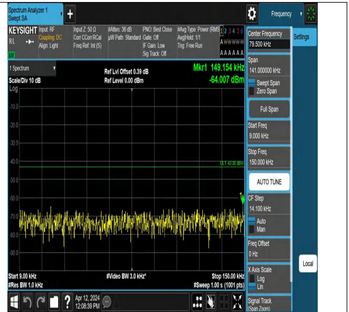
Band4-1413-2-0.009~0.15MHz-PASS
