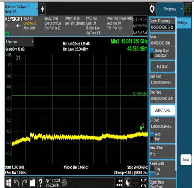
Band4-1413-1000~20000MHz-PASS
