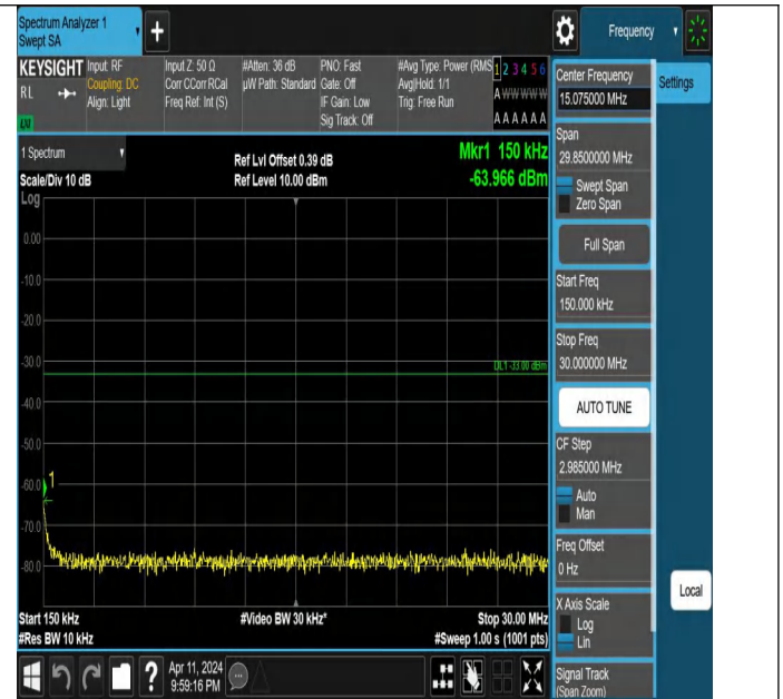
Band4-1513-0.15~30MHz-PASS
