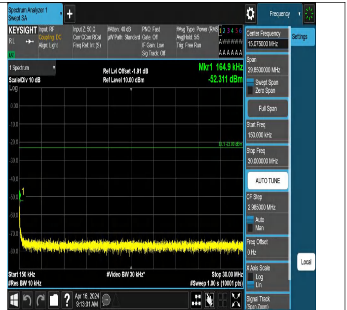
EGPRS850-251-8-0.15~30MHz-PASS
