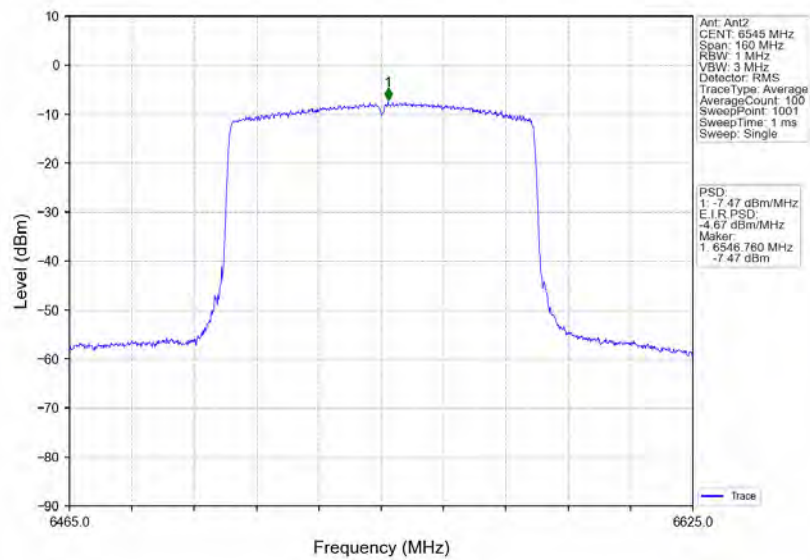
802.11ax(HEW80)_HCH_6545MHz_RU996_Left_MIMO_NTNV
