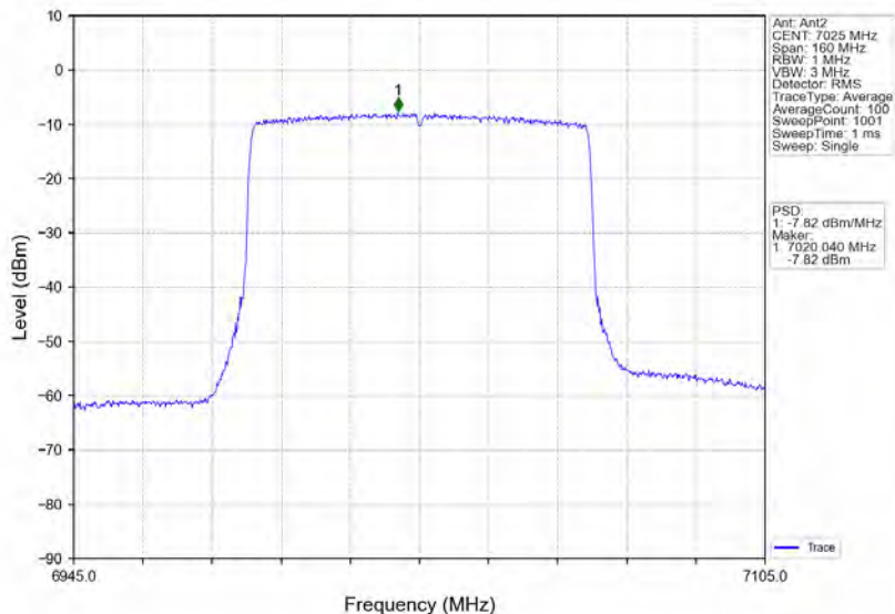
802.11ax(HEW80)_HCH_7025MHz_RU996_Left_MIMO_NTNV
