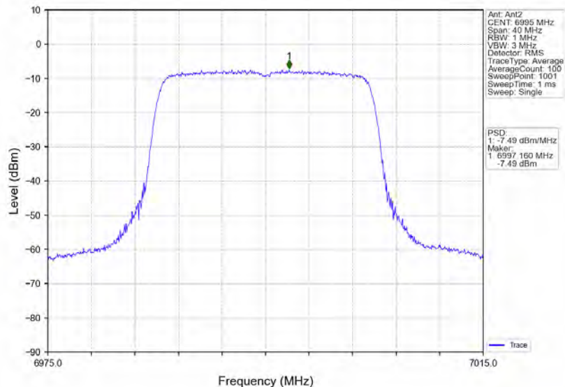
802.11ax(HEW20)_MCH_6995MHz_RU242_Left_MIMO_NTNV
