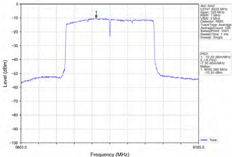
802.11ax(HEW160)_LCH_6025MHz_2xRU996_Left_MIMO_NTNV
