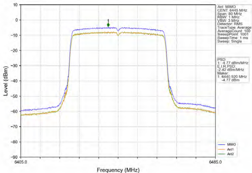
802.11ax(HEW40)_LCH_6445MHz_RU484_Left_MIMO_NTNV
