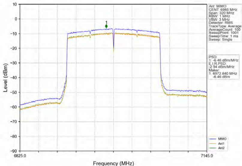
802.11ax(HEW160)_MCH_6985MHz_2xRU996_Left_MIMO_NTNV
