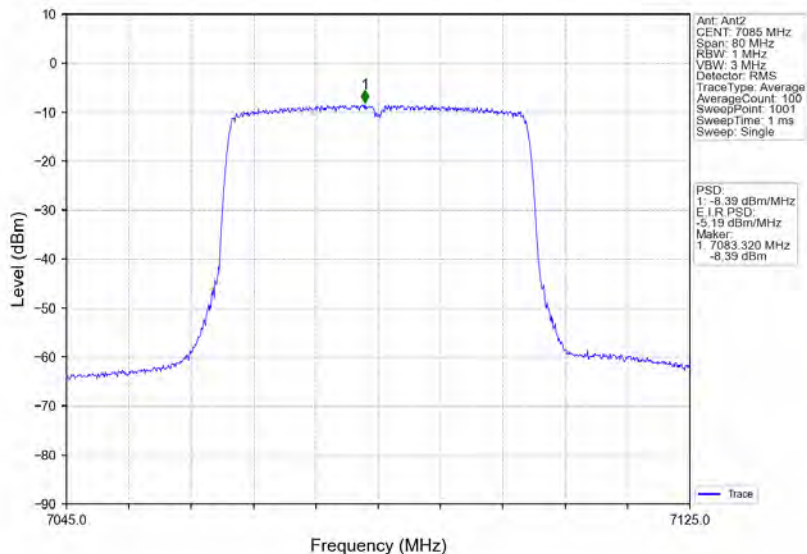
802.11ax(HEW40)_HCH_7085MHz_RU484_Left_MIMO_NTNV
