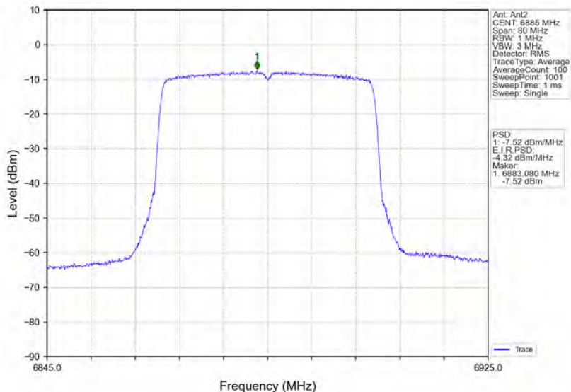
802.11ax(HEW40)_HCH_6885MHz_RU484_Left_MIMO_NTNV
