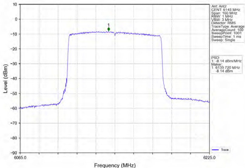
802.11ax(HEW80)_MCH_6145MHz_RU996_Left_MIMO_NTNV
