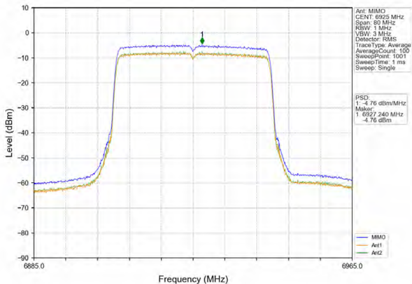
802.11ax(HEW40)_LCH_6925MHz_RU484_Left_MIMO_NTNV
