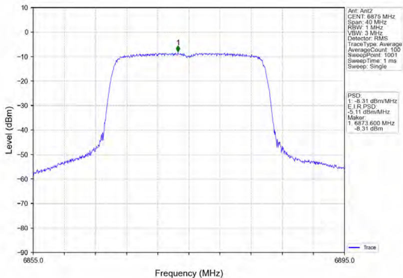
802.11ax(HEW20)_HCH_6875MHz_RU242_Left_Ant2_NTNV
